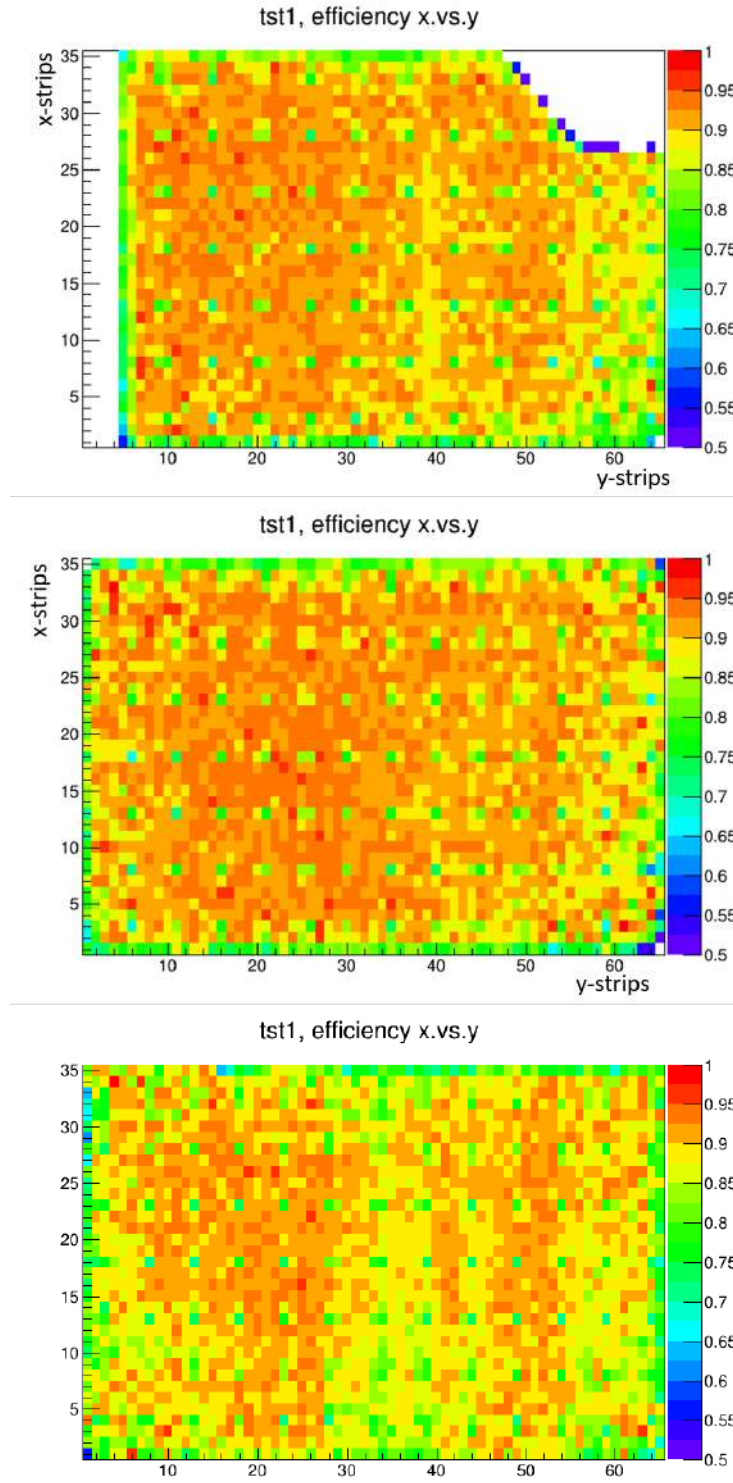
Figure 2.24: Efficiency maps of half RPCs 361-11 at 8700 V (first panel), 374-11 at 8600 V (second panel) and 368-11 at 8600 V (third panel).
