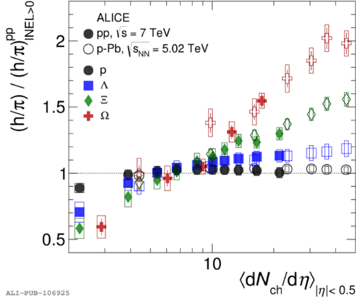
Figure 1.10: Particle yield ratios to pions normalized to the values measured in the inclusive INEL>0 (see Chapter 3) pp sample. The results are shown for pp and p-Pb collisions both normalized to the inclusive INEL>0 pp sample [47].
