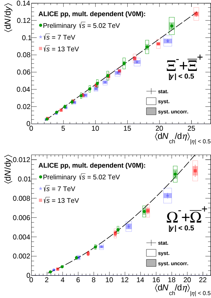
Figure 4.6: \Xi^- + \Xi^+ (top panel) and \Omega^- + \Omega^+ (bottom panel) p_T -integrated yields as a function of charged-particle multiplicity at \sqrt{s} = 5.02 TeV are represented in green. These present results are compared with the previous pp analyses at \sqrt{s} = 7 TeV [55] (blue points) and \sqrt{s} = 13 TeV [56] (red points). The statistical and total systematic uncertainties are represented by error bars and boxes, respectively. Shadowed boxes show the uncorrelated systematic uncertainties across charged-particle multiplicity. The black dashed line represents for \Xi^- + \Xi^+ the linear fit to the \langle dN/dy \rangle while for \Omega^- + \Omega^+ the second order polynomial fit.
