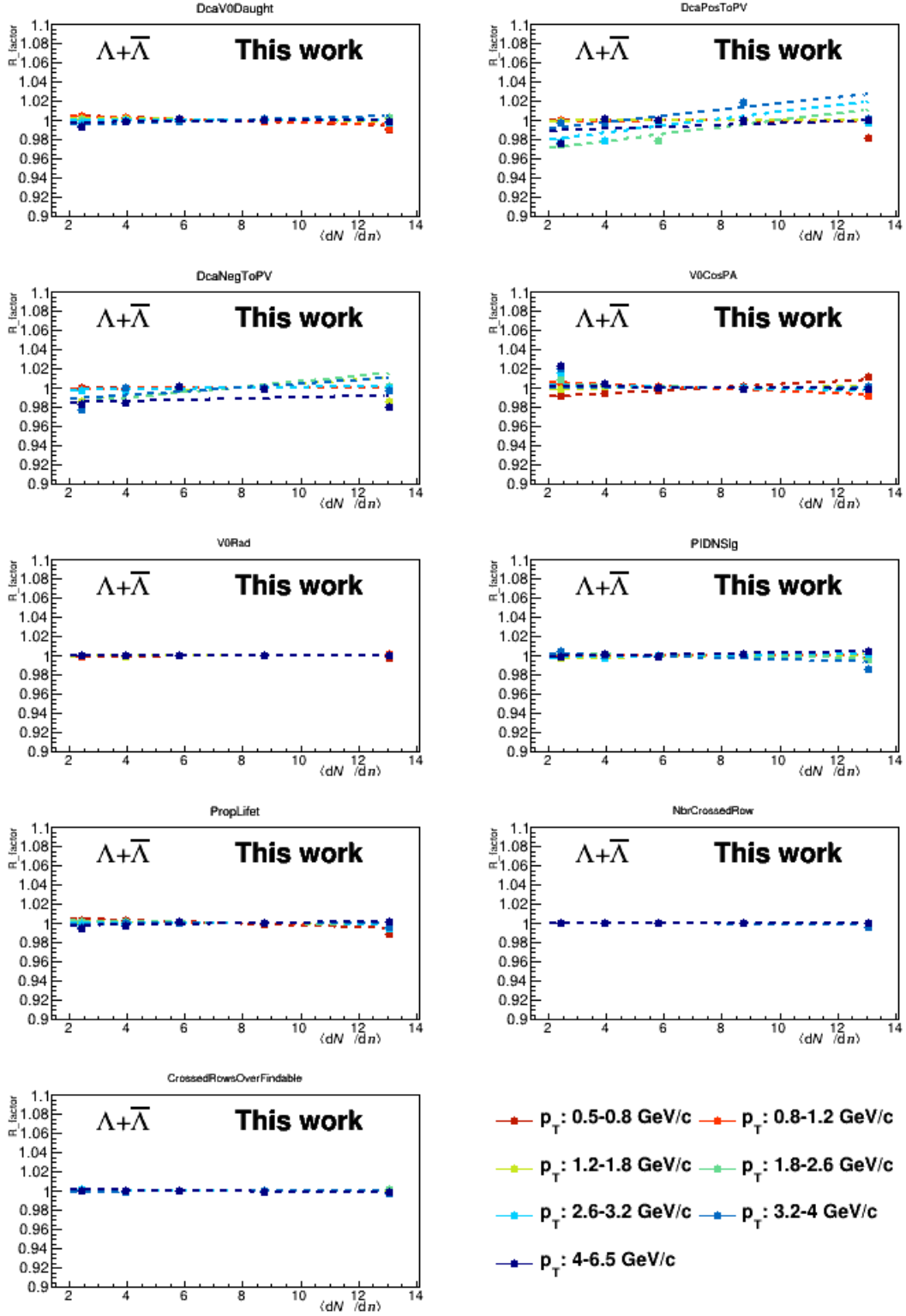
Figure 3.48: R-factors for \Lambda + \bar{\Lambda} as a function of multiplicity in p_T intervals and for different variable cuts as indicated.
