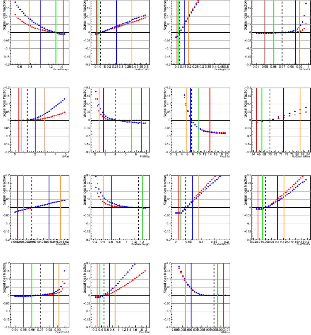
Figure B.7: The signal-loss fractions for \bar{\Omega}^+ in integrated multiplicity and p_T are shown. The data are in blue and MC in red. The orange, blue, green and red lines represent, respectively, the loosest, loose, tight and tightest cuts. The black dashed line corresponds to the default variable cut. These figures were obtained in this work.
