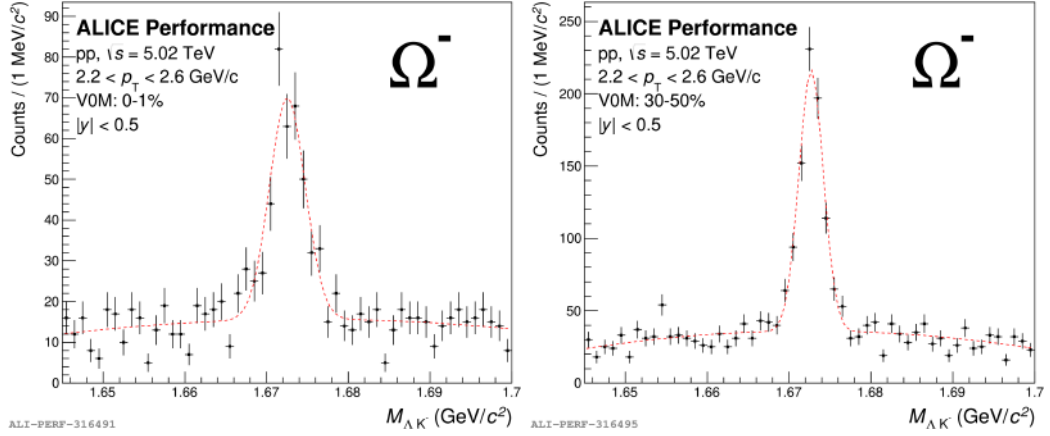
Figure 3.10: \Omega^- invariant mass spectra in two multiplicity bins in 2.2 < p_T < 2.6 \text{ GeV}/c . The red function is the peak plus background function.
