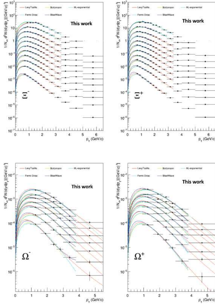
Figure C.6: The corrected spectra for \Xi^- and \Xi^+ (top panels) and \Omega^- and \bar{\Omega}^+ (bottom panels) are fitted with Boltzmann, Levy-Tsallis, m_T -exponential, Fermi Dirac and Blast Wave functions for p_T from 0 to 3.5 GeV/c. Scalar factors are applied to better display the spectra but neither they nor the multiplicity classes are indicated since the focus is on the five fits.
