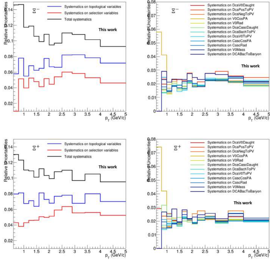
Figure C.2: The left panels show for \Xi^- and \Xi^+ in integrated multiplicity as a function of p_T the total systematic uncertainties in black, the systematic uncertainties due to the topological cuts in blue and the ones from selection variables in red. The right panels show for \Xi^- and \Xi^+ the single contribution to the systematic uncertainties from every topological variable.
