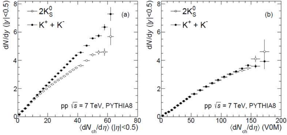
Figure 3.4: The left panel shows K^\pm and K_S^0 as a function of multiplicity selected at mid-rapidity in PYTHIA 8 simulations of pp collisions at \sqrt{s} = 7 TeV. The right panel shows K^\pm and K_0^S as a function of multiplicity selected at forward/backward pseudorapidity in PYTHIA 8 simulations of pp collisions at \sqrt{s} = 7 TeV [117].
