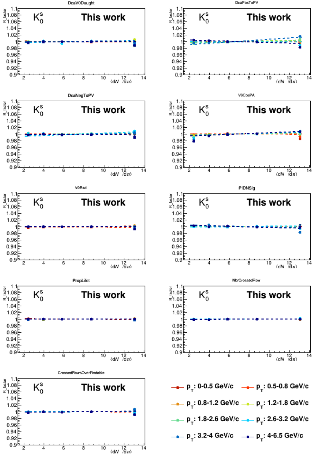
Figure 3.47: R-factors for K_s^0 as a function of multiplicity in p_T intervals and for different variable cuts as indicated.
