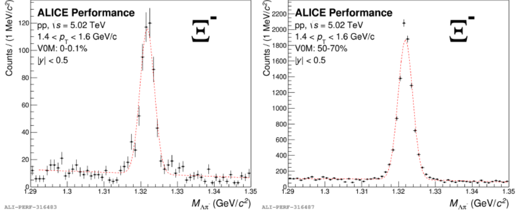
Figure 3.9: \Xi^- invariant mass spectra in two multiplicity bins in 1.4 < p_T < 1.6 \text{ GeV}/c . The red function is the peak plus background function.
