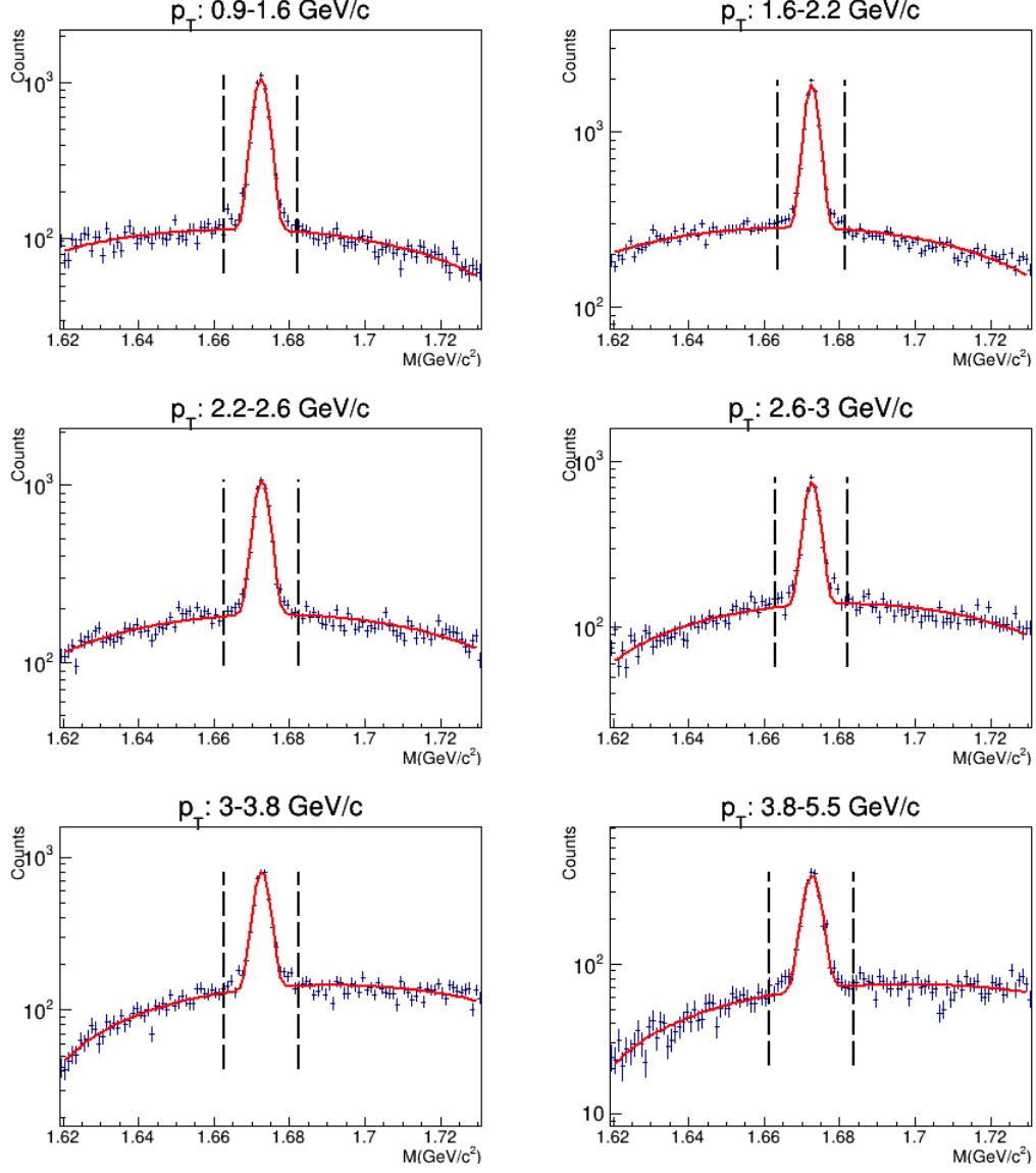
Figure A.7: \bar{\Omega}^+ Invariant mass spectra for all p_T bins for integrated multiplicity. These figures were obtained in this work.
