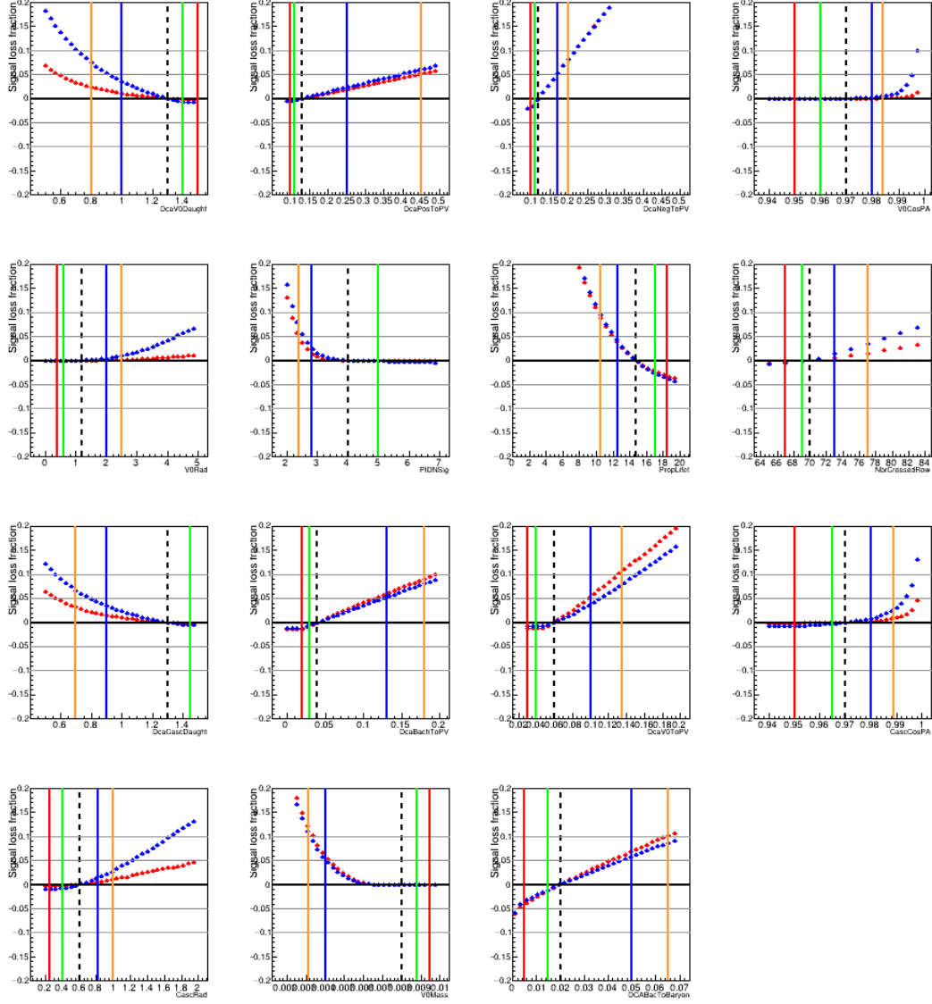
Figure B.5: The signal-loss fractions for \Xi^- in integrated multiplicity and p_T are shown. The data are in blue and MC in red. The orange, blue, green and red lines represent, respectively, the loosest, loose, tight and tightest cuts. The black dashed line corresponds to the default variable cut. These figures were obtained in this work.
