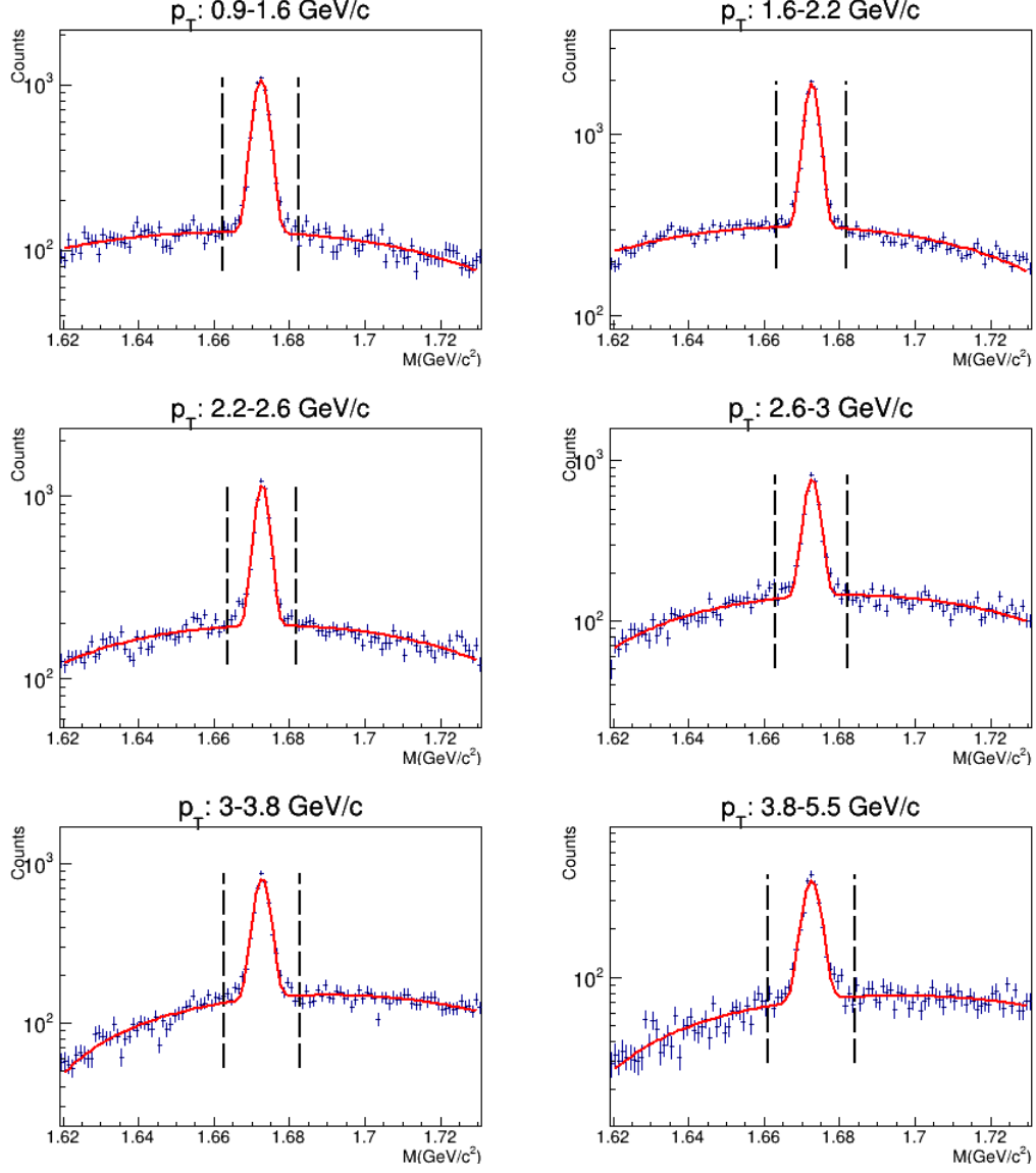
Figure A.6: \bar{\Omega}^- Invariant mass spectra for all p_T bins for integrated multiplicity. These figures were obtained in this work.
