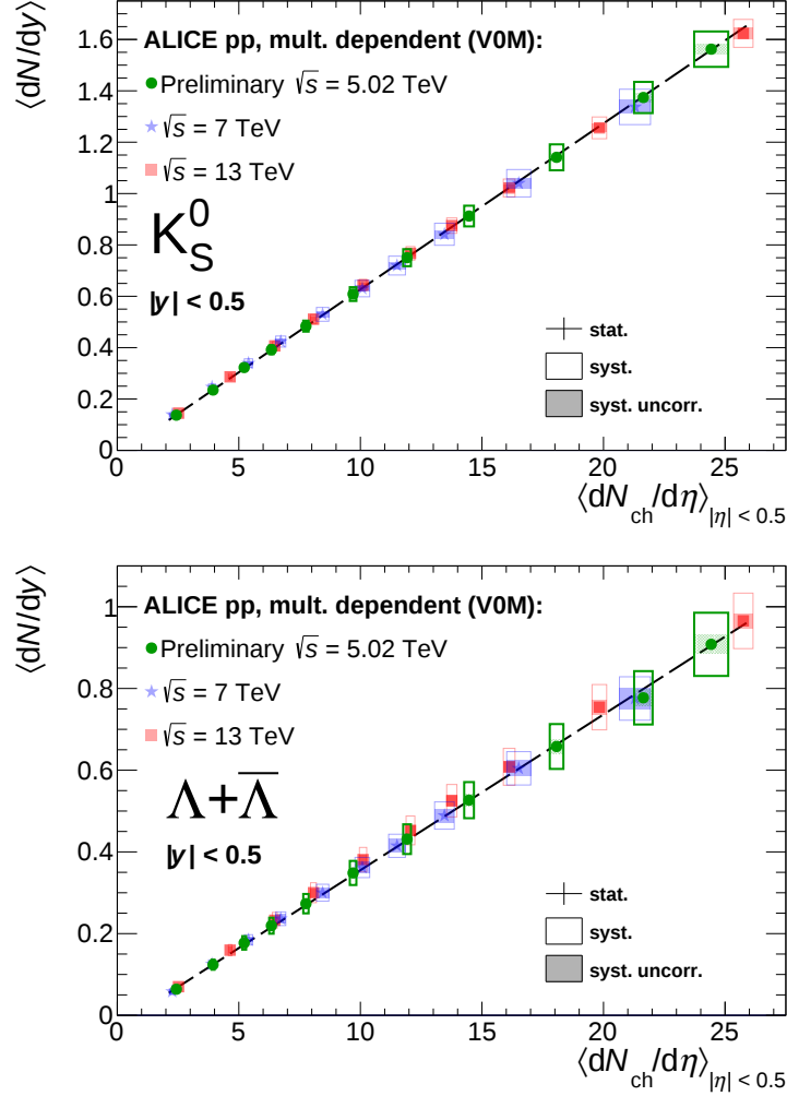
Figure 4.5: K_S^0 (top panel) and \Lambda + \bar{\Lambda} (bottom panel) p_{\mathbf{T}} -integrated yields as a function of charged-particle multiplicity at \sqrt{s} = 5.02 TeV are represented in green. These present results are compared with the previous pp analyses at \sqrt{s} = 7 TeV [55] (blue points) and \sqrt{s} = 13 TeV [56] (red points). The statistical and total systematic uncertainties are represented by error bars and boxes, respectively. Shaded boxes show the uncorrelated systematic uncertainties across multiplicity. The black dashed lines represent the linear fit to the \langle dN/dy \rangle .
