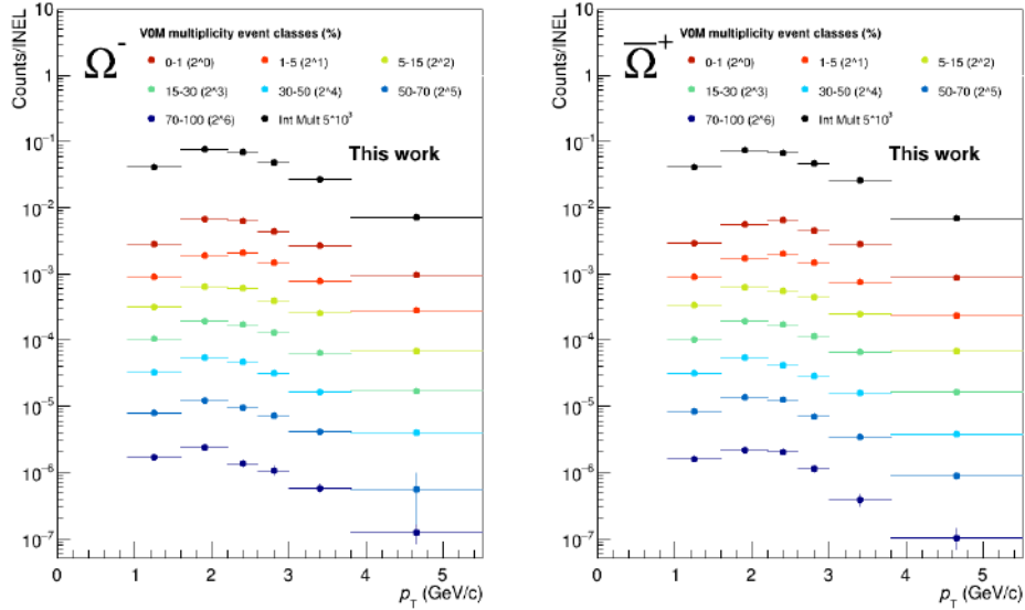
Figure 3.14: \Omega^- and \bar{\Omega}^+ raw spectra as a function of p_T in multiplicity classes and integrated multiplicity.
