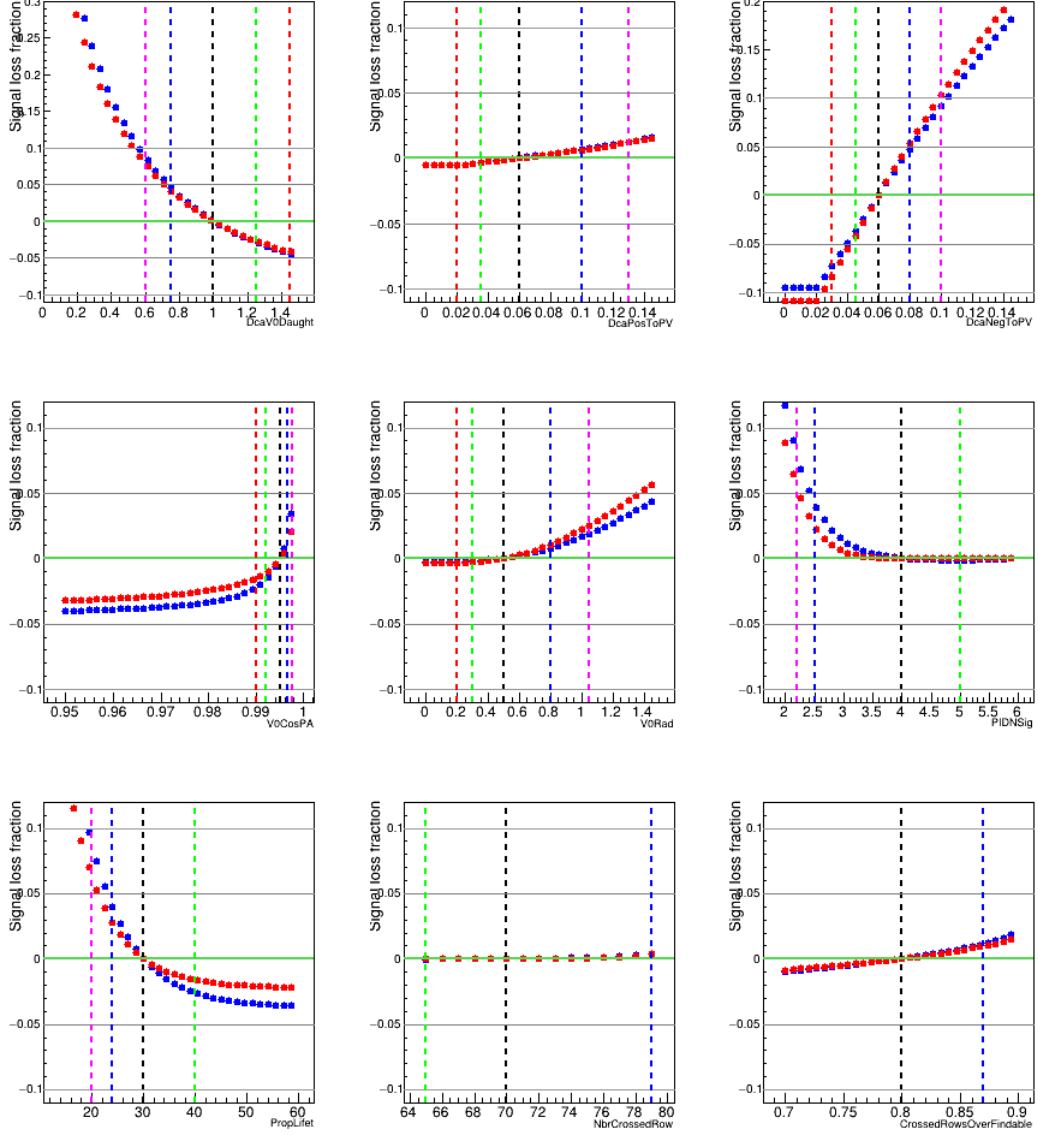
Figure B.3: The signal-loss fractions for \bar{\Lambda} in integrated multiplicity and p_{\mathbf{T}} are shown. The data are in blue and MC in red. The magenta, blue, green and red lines represent, respectively, the loosest, loose, tight and tightest cuts. The black dashed line corresponds to the default variable cut. These figures were obtained in this work.
