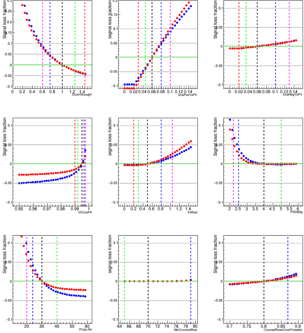
Figure B.2: The signal extraction fraction for \Lambda in integrated multiplicity and p_T are shown. The data are in blue and MC in red. The magenta, blue, green and red lines represent, respectively, the loosest, loose, tight and tightest cuts. The black dashed line corresponds to the default variable cut. These figures were obtained in this work.
