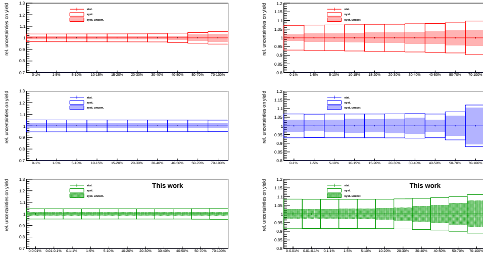
Figure C.8: K_S^0 (left side) and \Lambda + \bar{\Lambda} (right side) relative uncertainties on p_{\mathbf{T}} -integrated yields at \sqrt{s} = 5.02 TeV (green) vs multiplicity are shown compared with the previous results at \sqrt{s} = 7 TeV [55] (blue) and \sqrt{s} = 13 TeV [56] (red).
