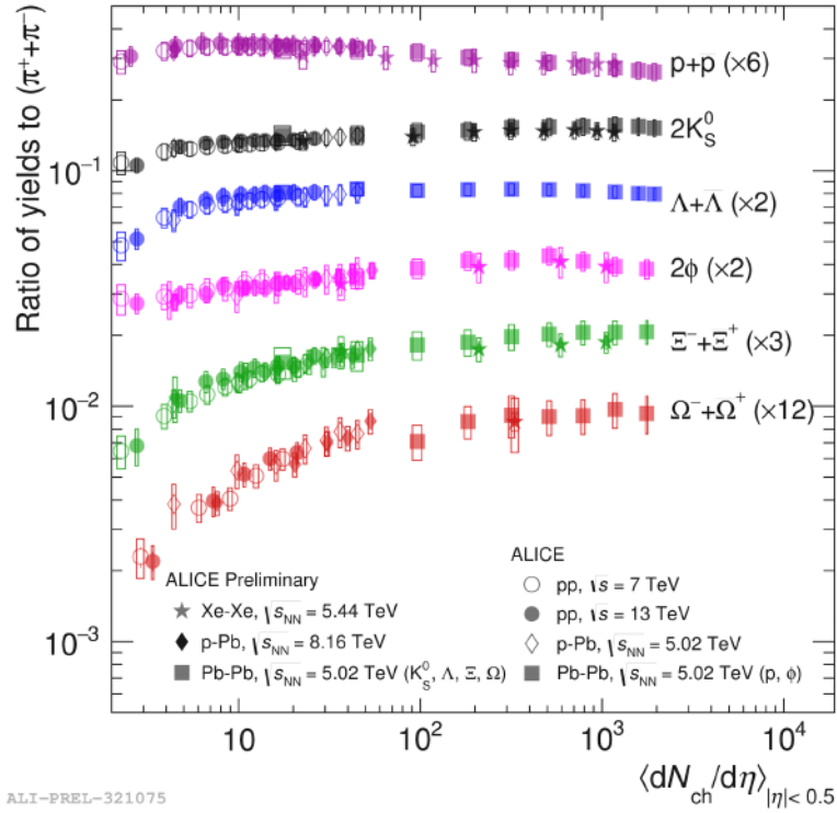
Figure 1.12: Ratio of integrated yields of K_S^0 , \Lambda + \bar{\Lambda} , \Xi^- + \Xi^+ , \Omega^- + \bar{\Omega}^+ , \phi and p w.r.t. pions as a function of \langle dN_{ch}/d\eta \rangle at mid-rapidity measured by ALICE in different colliding systems [54].
