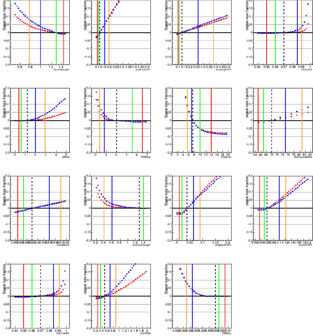
Figure B.6: The signal-loss fractions for \Omega^- in integrated multiplicity and p_{\text{T}} are shown. The data are in blue and MC in red. The orange, blue, green and red lines represent, respectively, the loosest, loose, tight and tightest cuts. The black dashed line corresponds to the default variable cut. These figures were obtained in this work.
