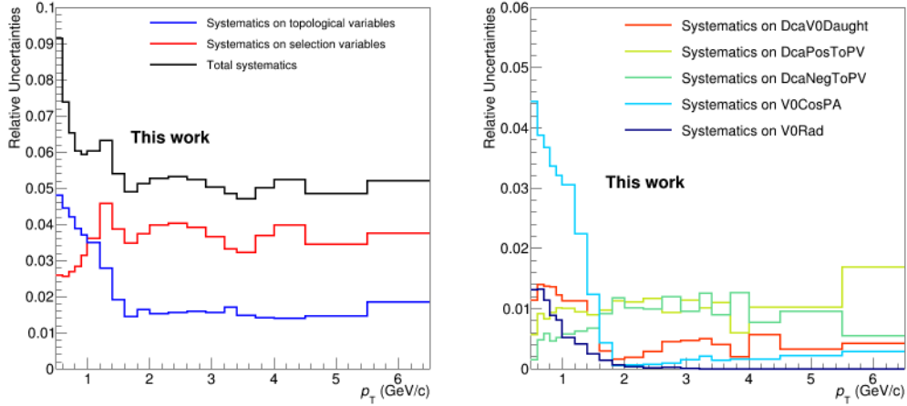
Figure 3.44: The left panel shows for \Lambda + \bar{\Lambda} in integrated multiplicity as a function of p_T the total systematic uncertainties in black, the systematic uncertainties due to the topological cuts in blue and the ones from selection variables in red. The right figure shows for \Lambda + \bar{\Lambda} the single contribution to the systematic uncertainties from every topological variable.
