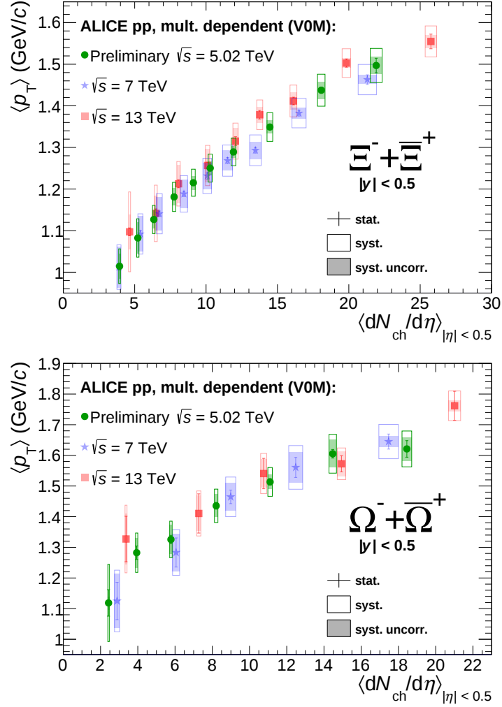
Figure 4.8: \Xi^- + \Xi^+ (top panel) and \Omega^- + \Omega^+ (bottom panel) \langle p_T \rangle at \sqrt{s} = 5.02 TeV is compared with the previous results at \sqrt{s} = 7 TeV [55] and \sqrt{s} = 13 TeV [56]. The three analyses present compatible results.
