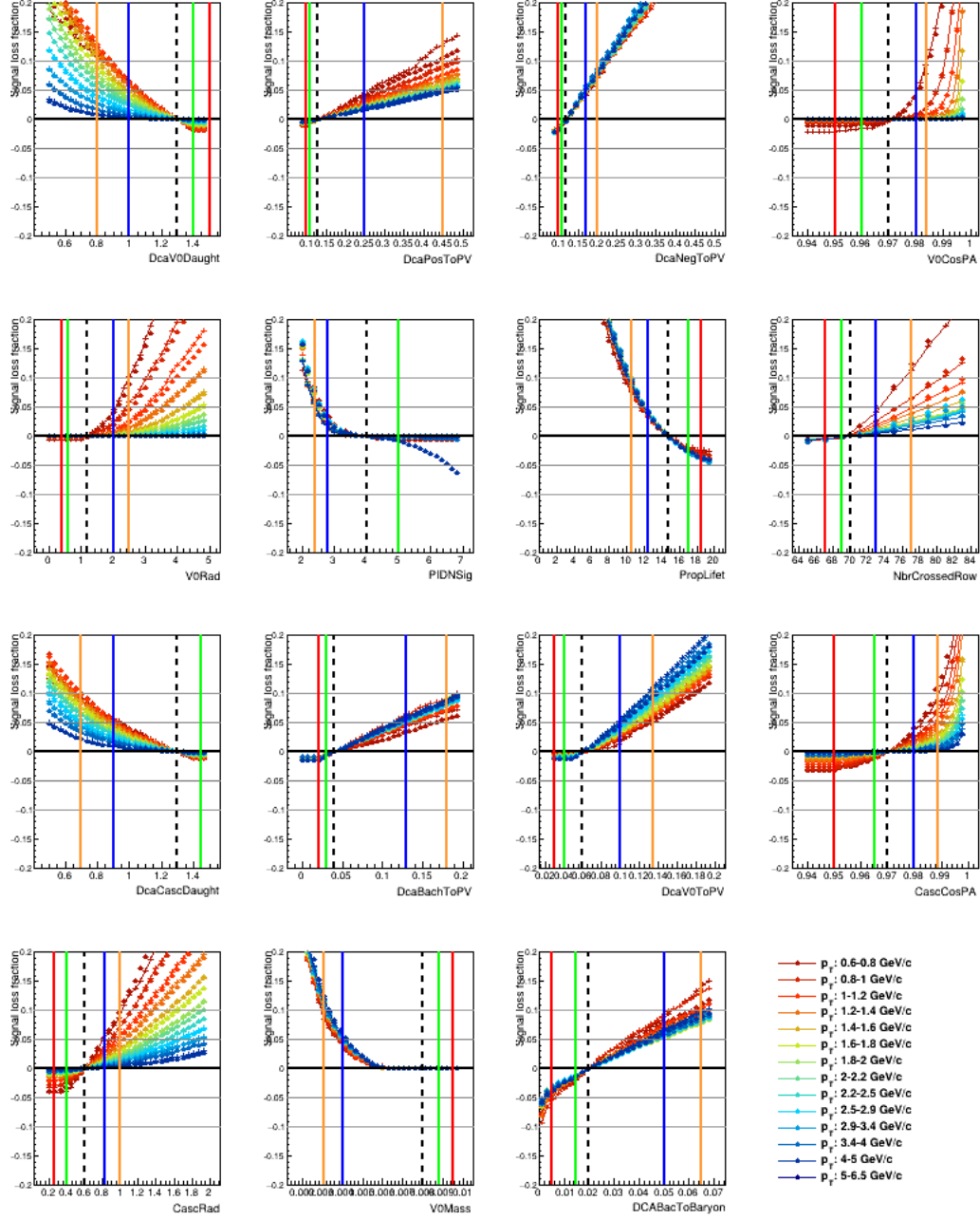
Figure 3.40: The signal-loss fractions for \Xi^- in the 14 p_T intervals (see legend) are shown. The data are the full points while the MC are the lines and cross points. The orange, blue, green and red lines represent, respectively, the loosest, loose, tight and tightest cuts. The black dashed line corresponds to the default variable cut. These figures were obtained in this work.
