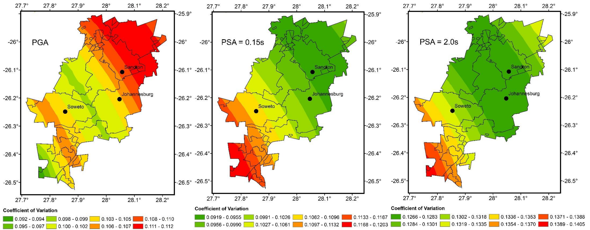
Figure 8-16: COV results for the sensitivity analysis for b -value.
