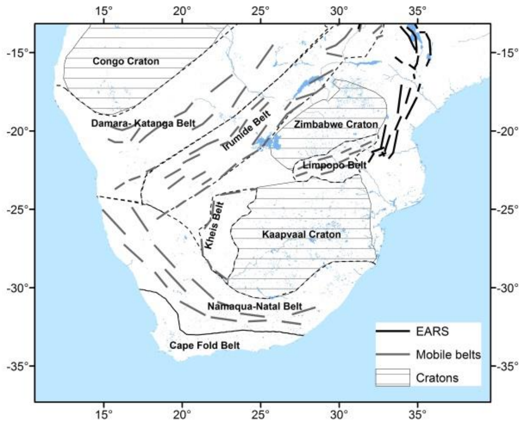
Figure 3-1: Regional geological settings of southern Africa showing mobile belts and Archaean cratons (Manzunzu et al., 2019).
