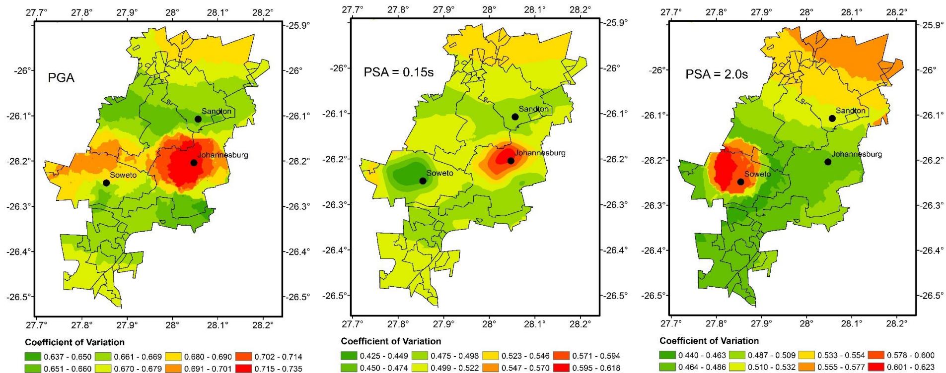
Figure 8-15: COV results for GMPE seismic hazard sensitivity analysis.
