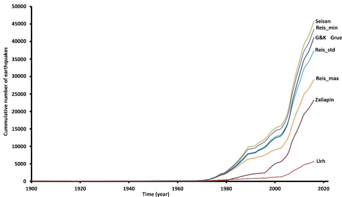
Figure 4-18: Cumulative number of events for the declustered catalogues obtained using several declustering algorithms. G&K is the Gardner and Knopoff (1974) method; Grue is the Grünthal (1985) method; Reis_min, Reis_std and Reis_max are the minimum, mean and maximum standard deviations for the Reasenber (1985) method respectively; Urh is the Uhrhammer method; and Seisan and Zaliapin are the Seisan and Zaliapin methods, respectively.
