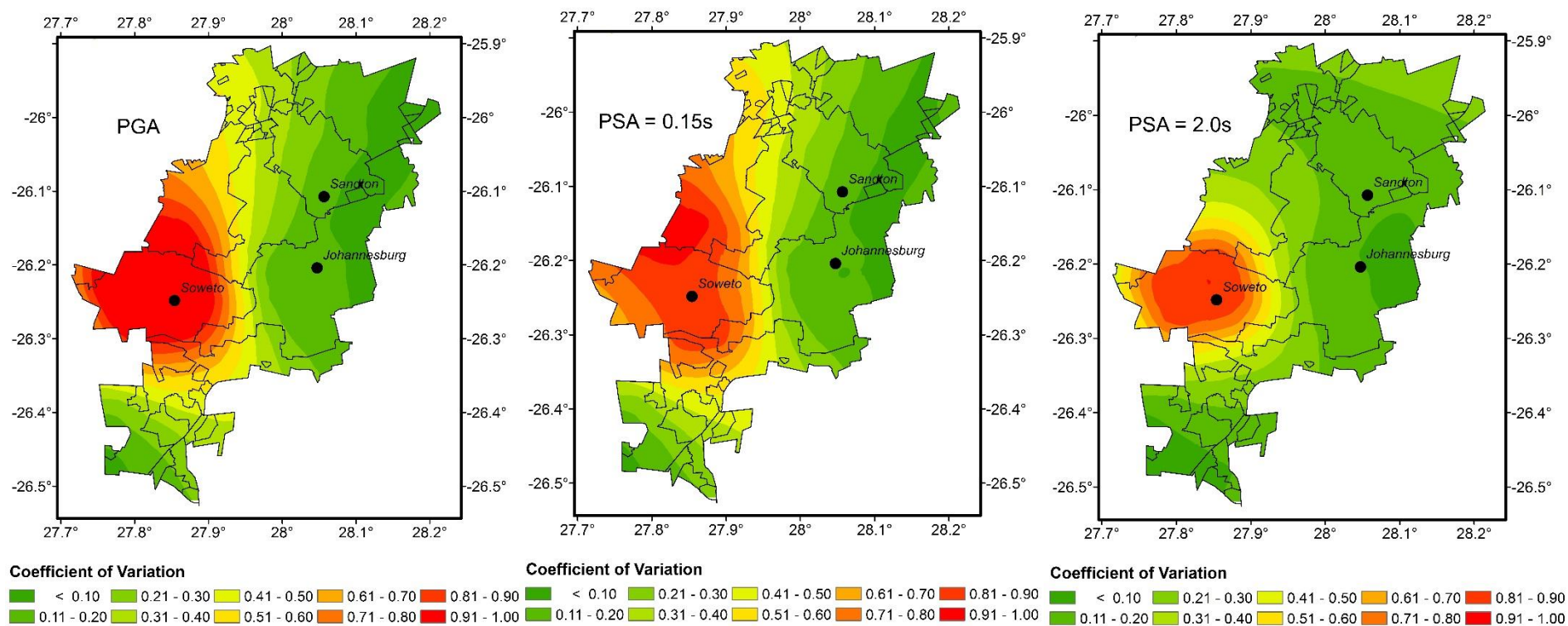
Figure 8-9: Results of different source models used in computing hazard for Johannesburg for the COV.
