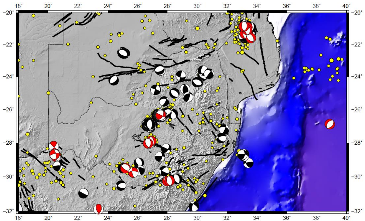
Figure 5-6: Focal mechanism solutions used in this study. Thick black lines represent faults located in the area and yellow circles represent earthquakes ( M > 4 ). Black beach balls represent new solutions (Table 5-2) while the red ones are the published solutions in Table 5-1 (Faults were extracted from Manzunzu et al., 2019; background topography was extracted from Amante et al., 2009).
