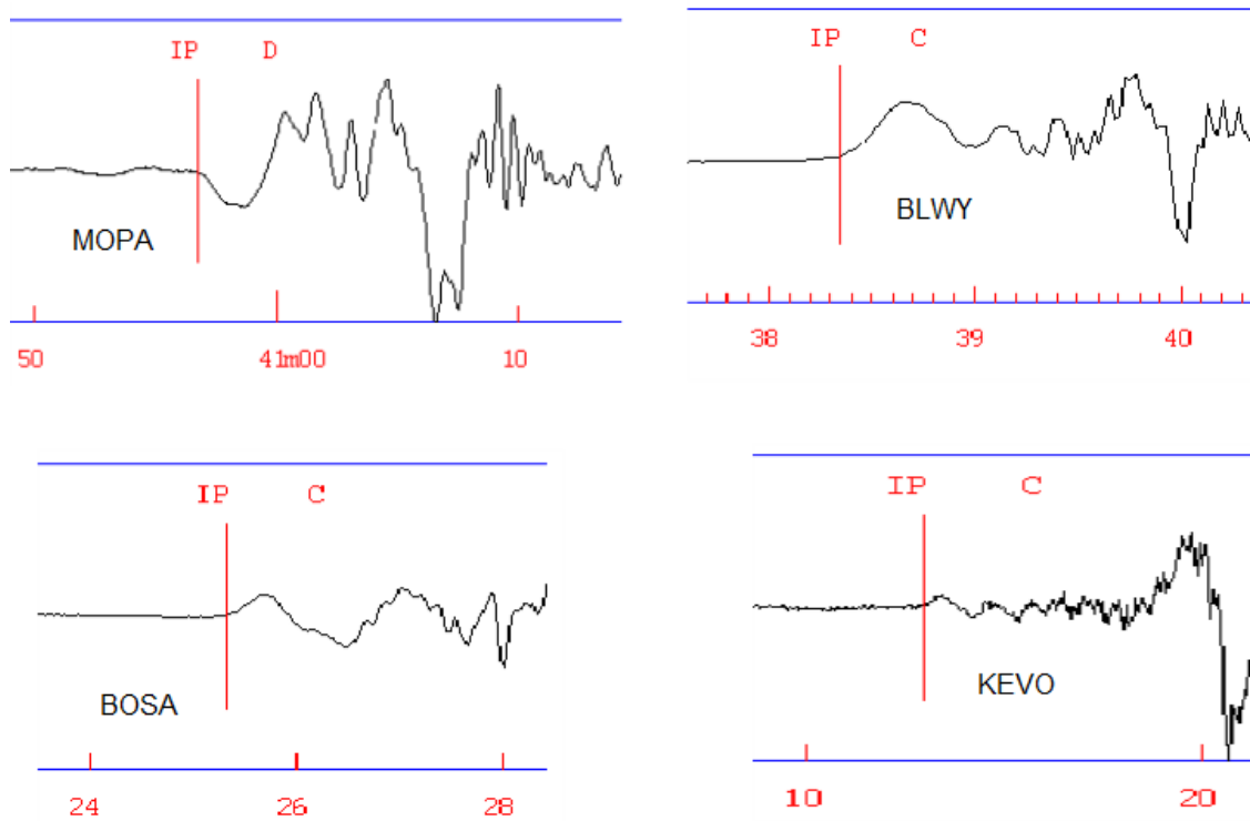
Figure 5-5: Examples of polarities picked. C is the upward first motion and D is the downward first motion. In this figure, station MOPA (BHZ channel) is at an epicentral distance of 210km: Polarity (Down). Station BLWY, (BHZ channel) is in Zimbabwe at 426 KM from the station : (Polarity (UP). BOSA, BHZ, is at epicentral distance of 136 km and station KEVO BHZ located at 221 km from the epicenter.
