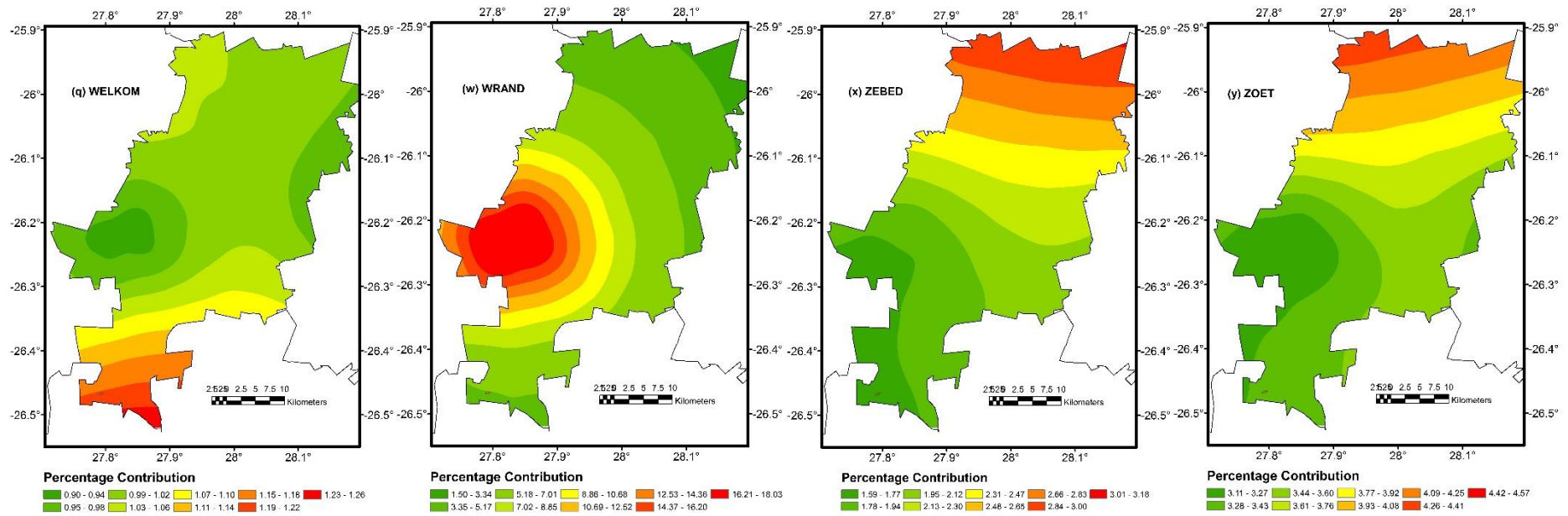
Figure 8-12: Maps showing the % contribution of the delineated zones to the total hazard for spectral period of 2.0s for Johannesburg. Note the variation in the percentage value. Each map is scaled according to its own range of values.
