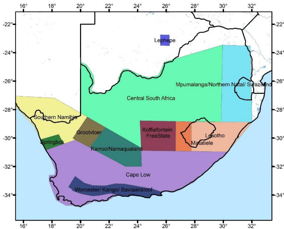
Figure 5-3: Modified seismotectonic zones defined by Du Plessis (1996).
