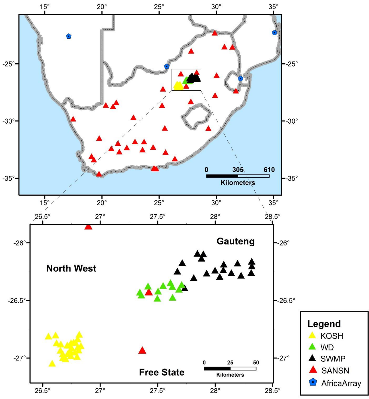
Figure 4-2: Map of the SANSN network. The three cluster networks also shown in the zoomed picture.
