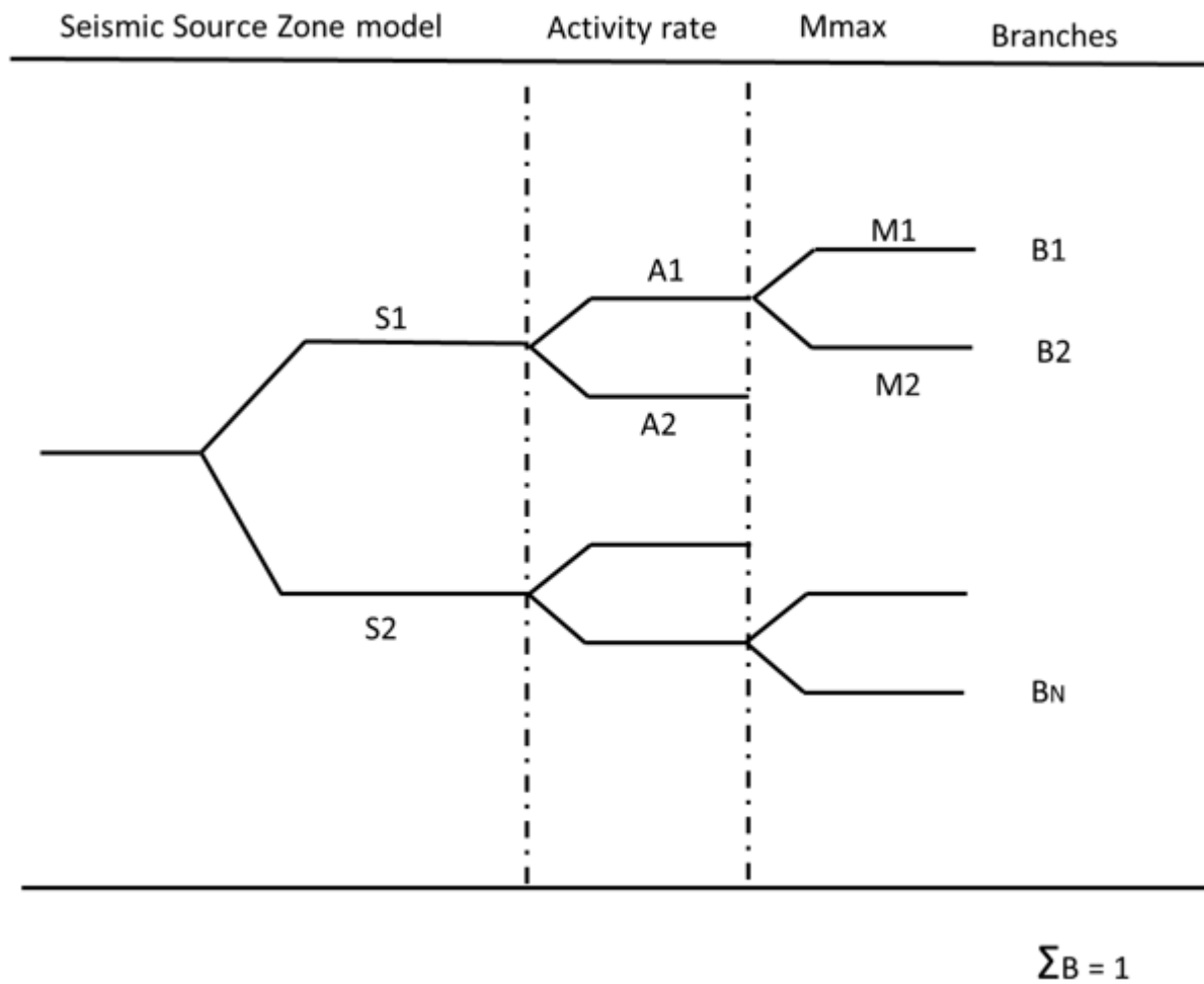
Figure 2-9: An example of a logic tree. The seismic source zone represents an independent node while the activity rate and Mmax are the dependent one.
