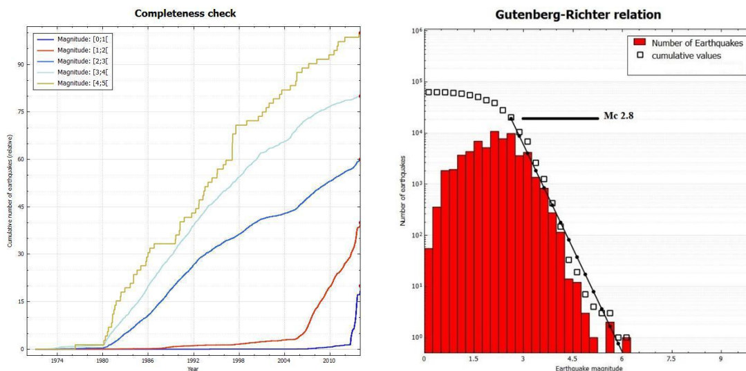
Figure 2-6: Different methods of estimating M_C . a) Stepp (1972) b) Cumulative distribution (Wiemer and Wyss, 200)
