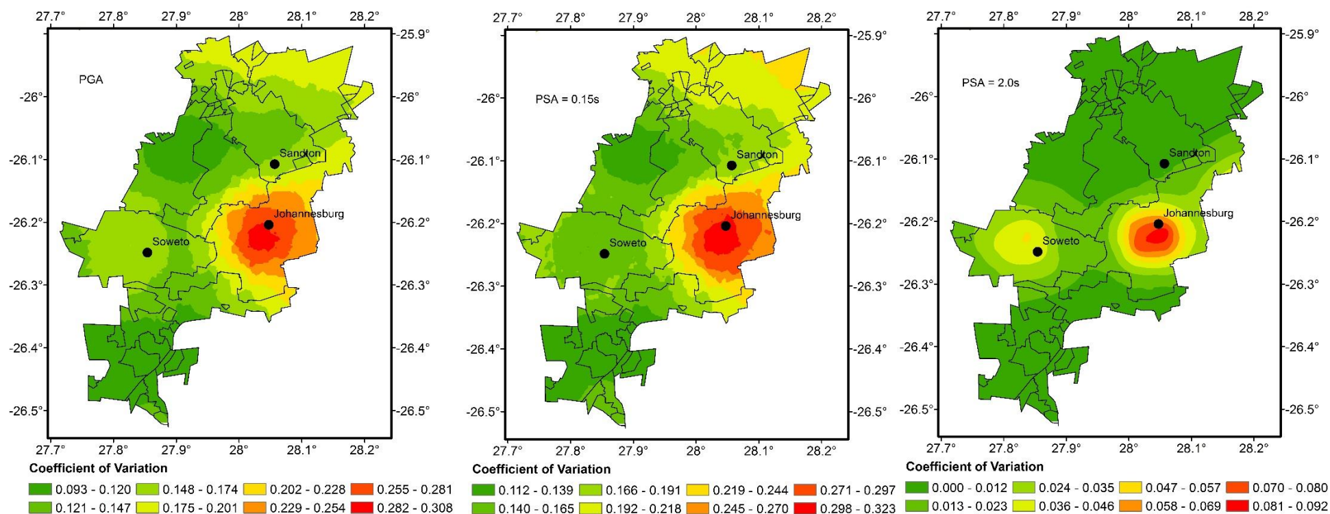
Figure 8-14: COV results for the sensitivity analysis for M_{min} .
