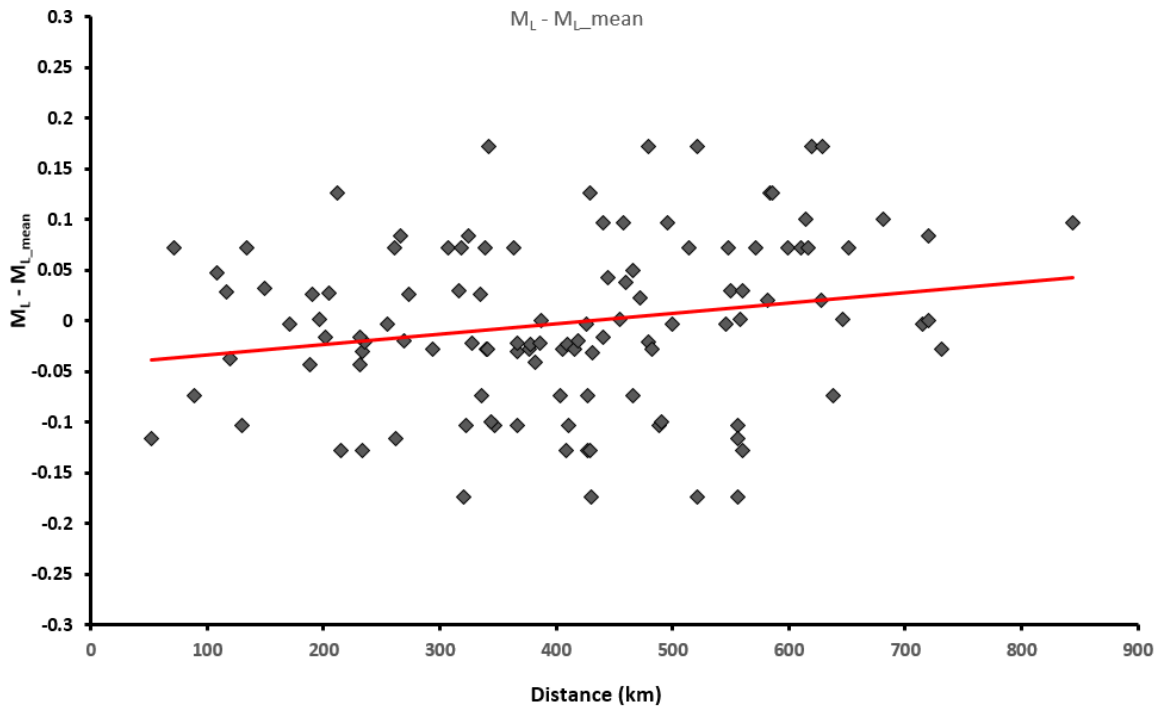
Figure 4-15: Mean magnitude residuals with distance local ( M_L ) magnitude values.
