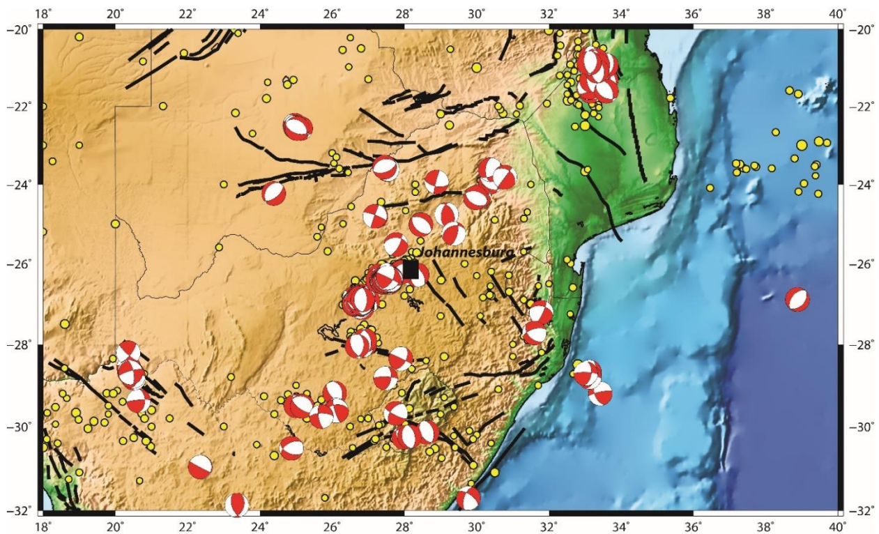
Figure 5-10: Seismotectonic map for Johannesburg and surrounding region used to delineate potential seismic sources (Faults were extracted from Manzunzu et al., 2019; background topography was extracted from Amante et al., 2009).
