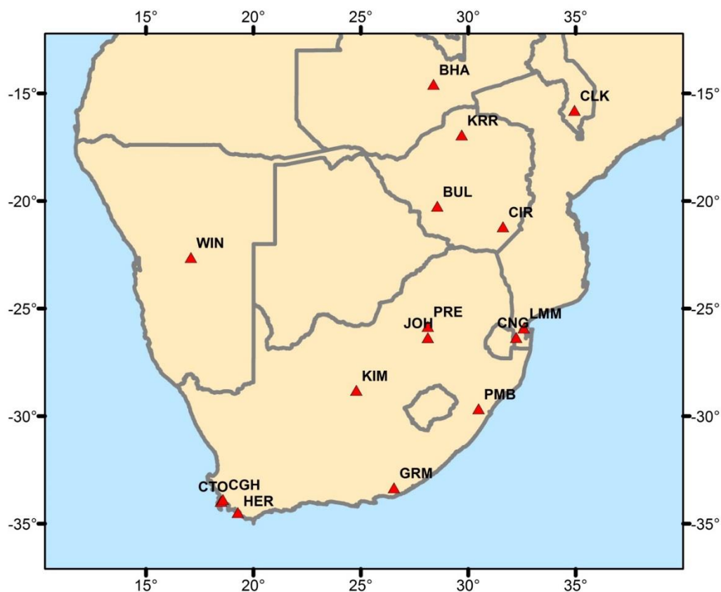
Figure 4-1: Location of early seismograph stations in Southern Africa region from 1899 to 1969.
