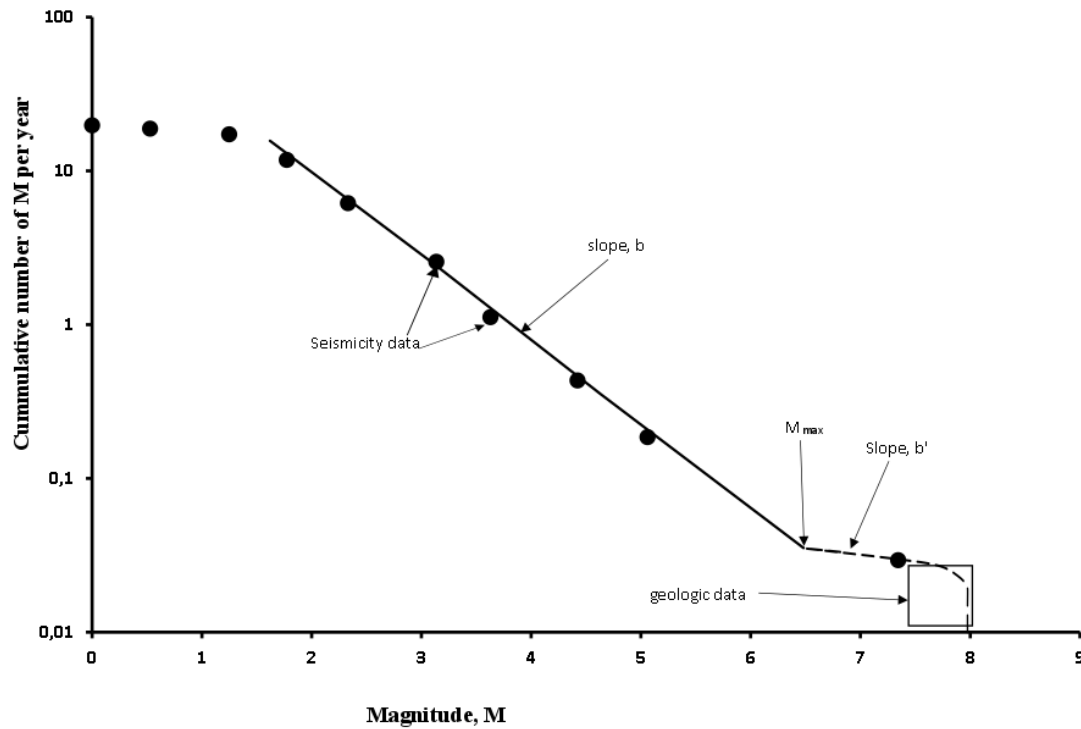
Figure 2-4: Characteristic earthquake model (modified from Youngs and Coppersmith, 1985).
