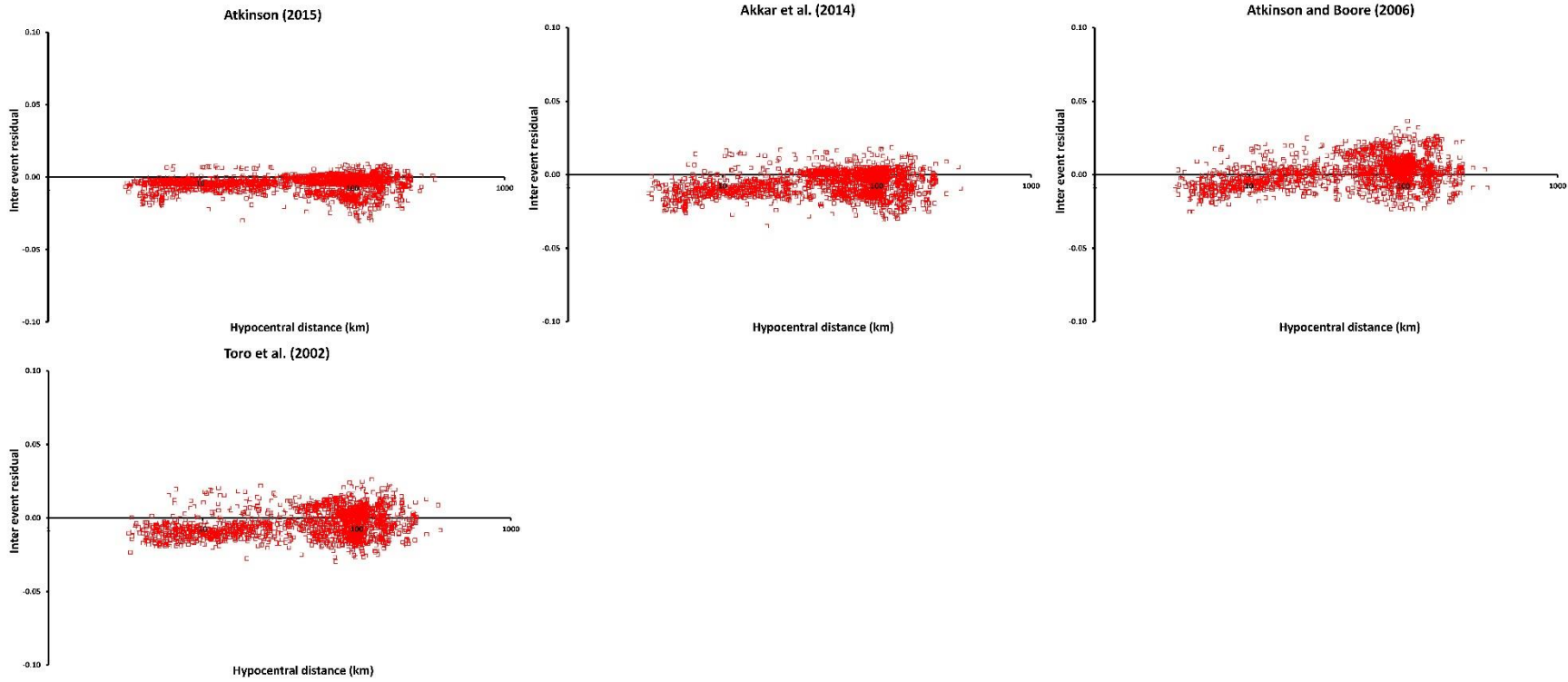
Figure 7-3: The inter-event residuals of all GMPEs for PGA ( T = 0.01s ) spectral acceleration versus hypocentral distance.
