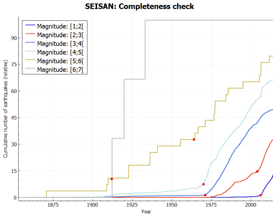
Figure 4-19: Results from the catalogue approach. The red dots represents the start of the completeness for each magnitude unit.
