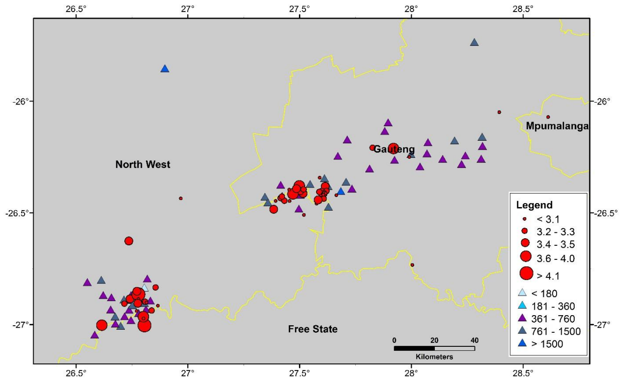
Figure 7-1: Location of earthquakes used in the testing of GMPEs. The figure shows the spatial distribution of the seismic events and the stations. Triangles represent the stations recording the events with each station having a V_{s30} value indicated with the color; circles are the seismic events.
