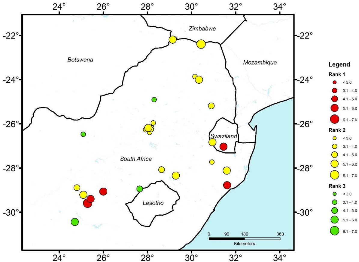
Figure 4-4: The location of the earthquakes with source parameters determined in this study. The earthquakes are shown with their ranking.
