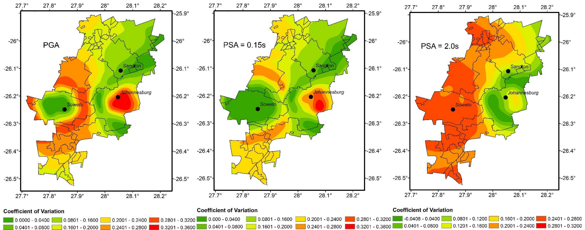
Figure 8-5: COV results for length of catalogue (full catalogue and post 1970 catalogue).
