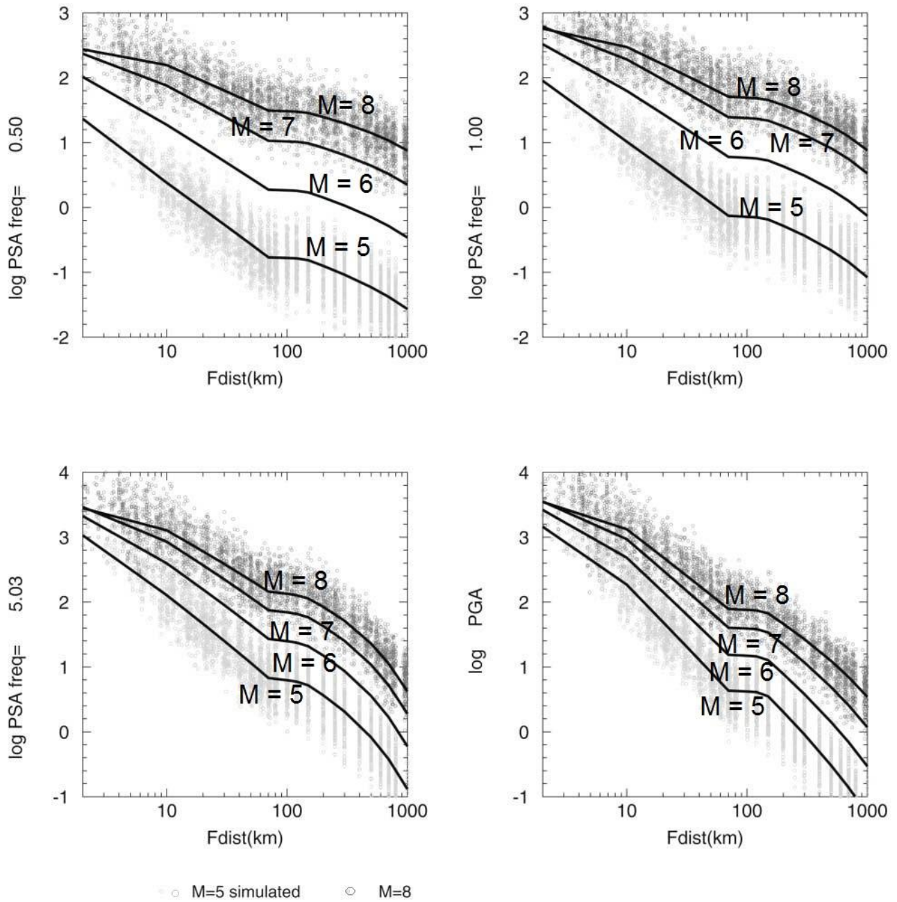
Figure 2-8: An example of a GMPE developed for Eastern and North America. Log 10 values of horizontal component 5% pseudo-spectral acceleration (PSA) at frequencies 0.5, 1, and 5.03 Hz, and the peak ground acceleration (PGA) is in units of m/s 2 . Dots show PSA from simulations, including aleatory uncertainty, for M 5 (light) and M 8 (dark); Fdist is the distance. Solid lines show predicted amplitudes from regression equations developed from simulated database, for M 5, 6, 7, and 8 (adapted from Atkinson and Boore, 2006).
