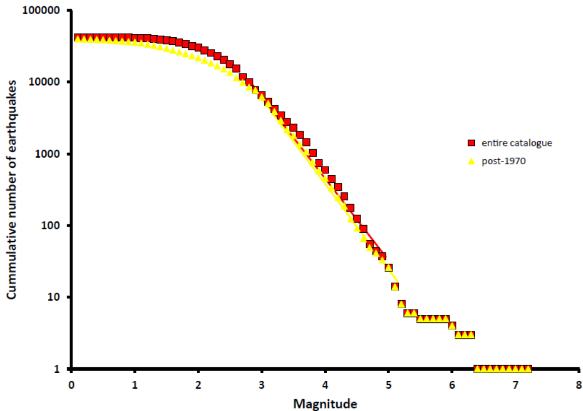
Figure 8-4: G-R curves for the two catalogues used in the assessment of the temporal stationarity of the catalogue. The entire catalogue starts from 1620 to 2016 while the post 1970 catalogue is from 1970 to 2016.
