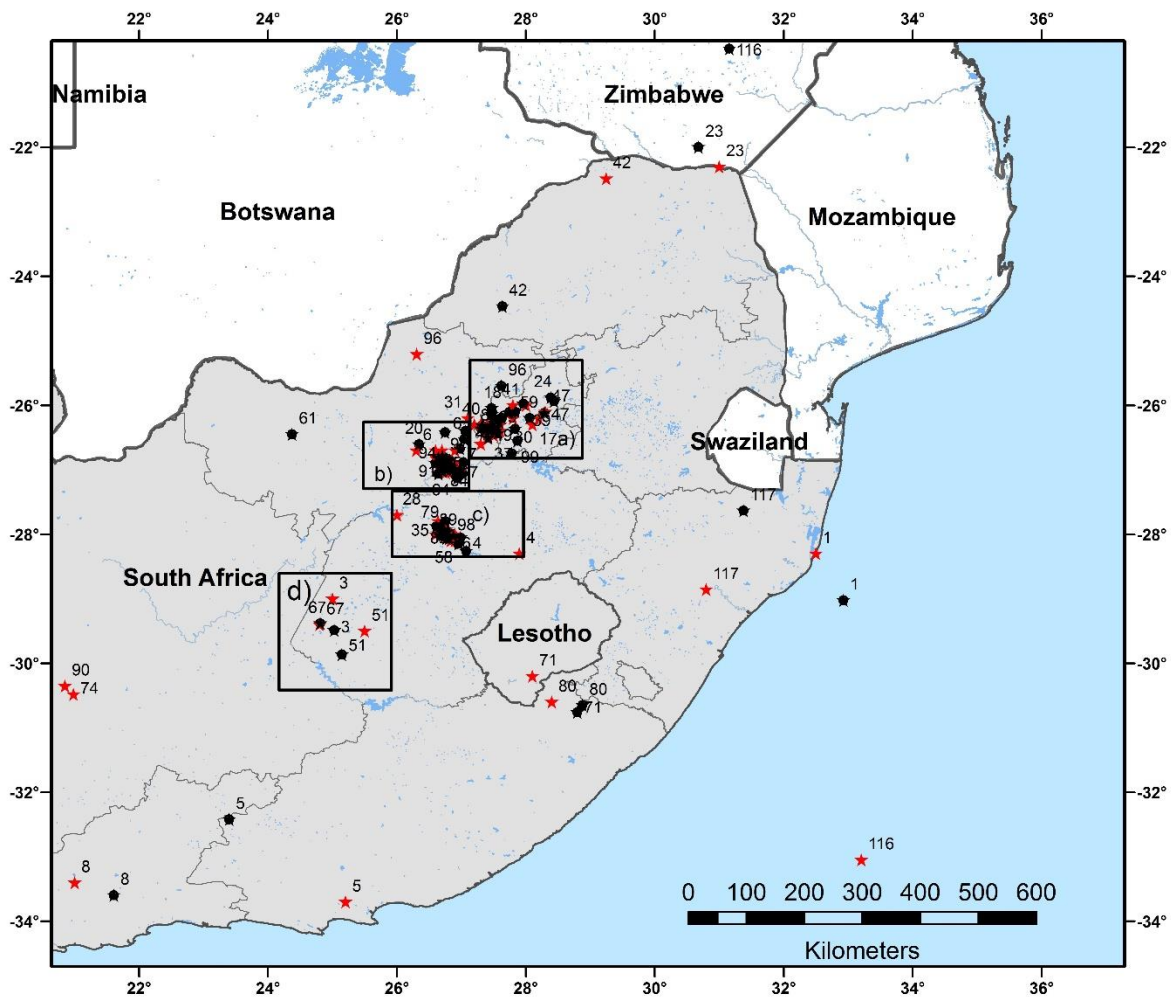
Figure 4-9. Comparison of new epicentral locations (black stars) to the published CGS locations (red stars). Black lined boxes represent clusters of seismicity zoomed as in Figure 4-10 for clarity (modified from Midzi et al., 2020).
