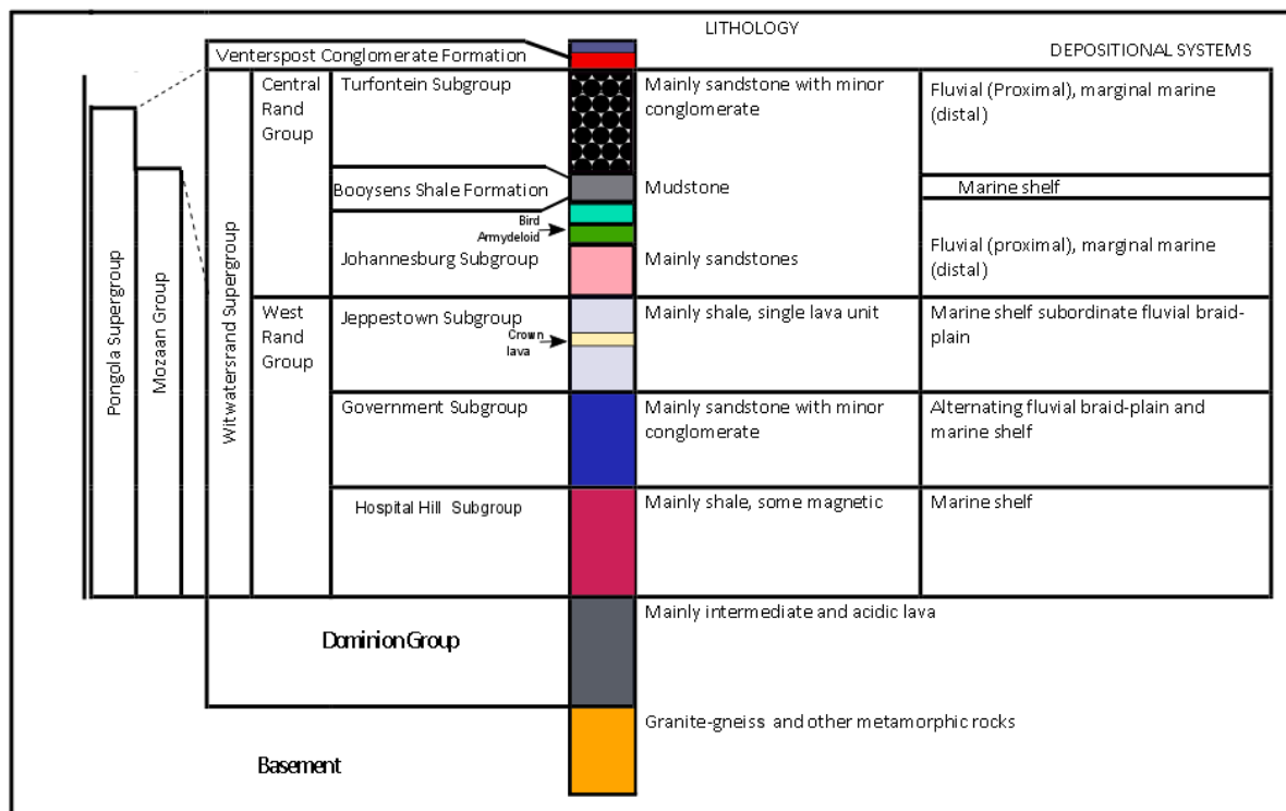
Figure 3-2: Detailed stratigraphic unit of the Witwatersrand Supergroup with the lithologies and depositional settings of the Central Rand and the West Rand Groups (modified from Catuneanu and Eriksson, 1999; McCarthy, 2006; Smith et al., 2013).
