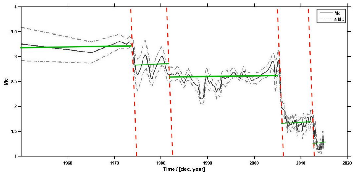
Figure 4-21: Variation of the magnitude of completeness ( M_C ) with time for our catalogue. The green line indicates the average M_C for the time period. The dashed line represents the uncertainty.
