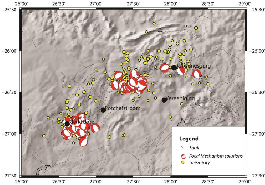
Figure 5-7: Zoomed in focal mechanism solution for the Witwatersrand basin. The seismicity is for magnitude 3.5 and above for the period 1602 to 2017 (Faults were extracted from Manzunzu et al., 2019; background topography was extracted from Amante et al., 2009).
