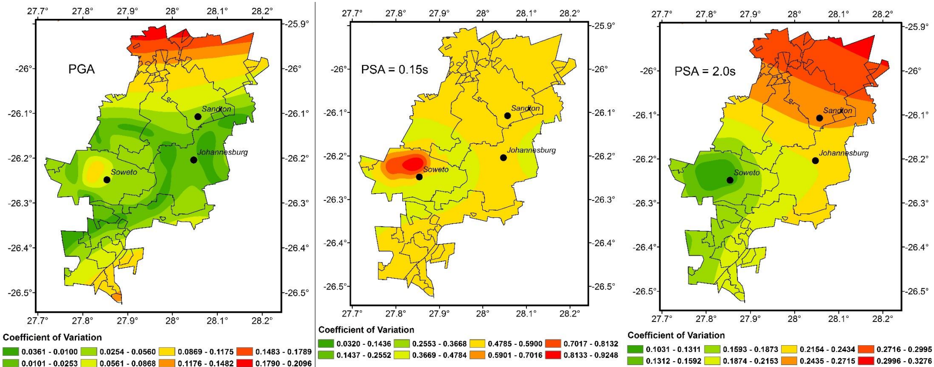
Figure 8-3: COV results for earthquake magnitude homogenisation process.
