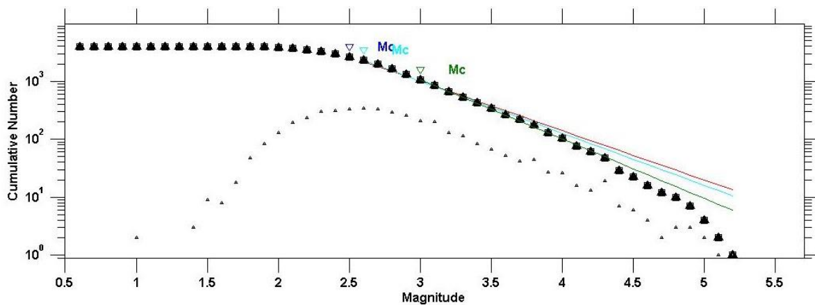
Figure 4-24: Different M_C calculation methods. Green is M_C by the Shi and Bolt method, blue is M_C by EMR and magenta is Maximum curvature method. Both methods were computed using the Gardner and Knoppoff catalogue.
