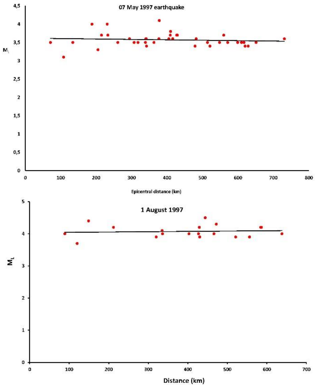
Figure 4-14: Variation of local magnitude with epicentral distance.
