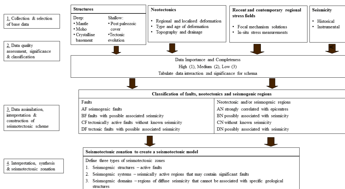
Figure 5-9: Flow chart of the construction of a seismotectonic model as suggested by Terrier et al. (2000).
