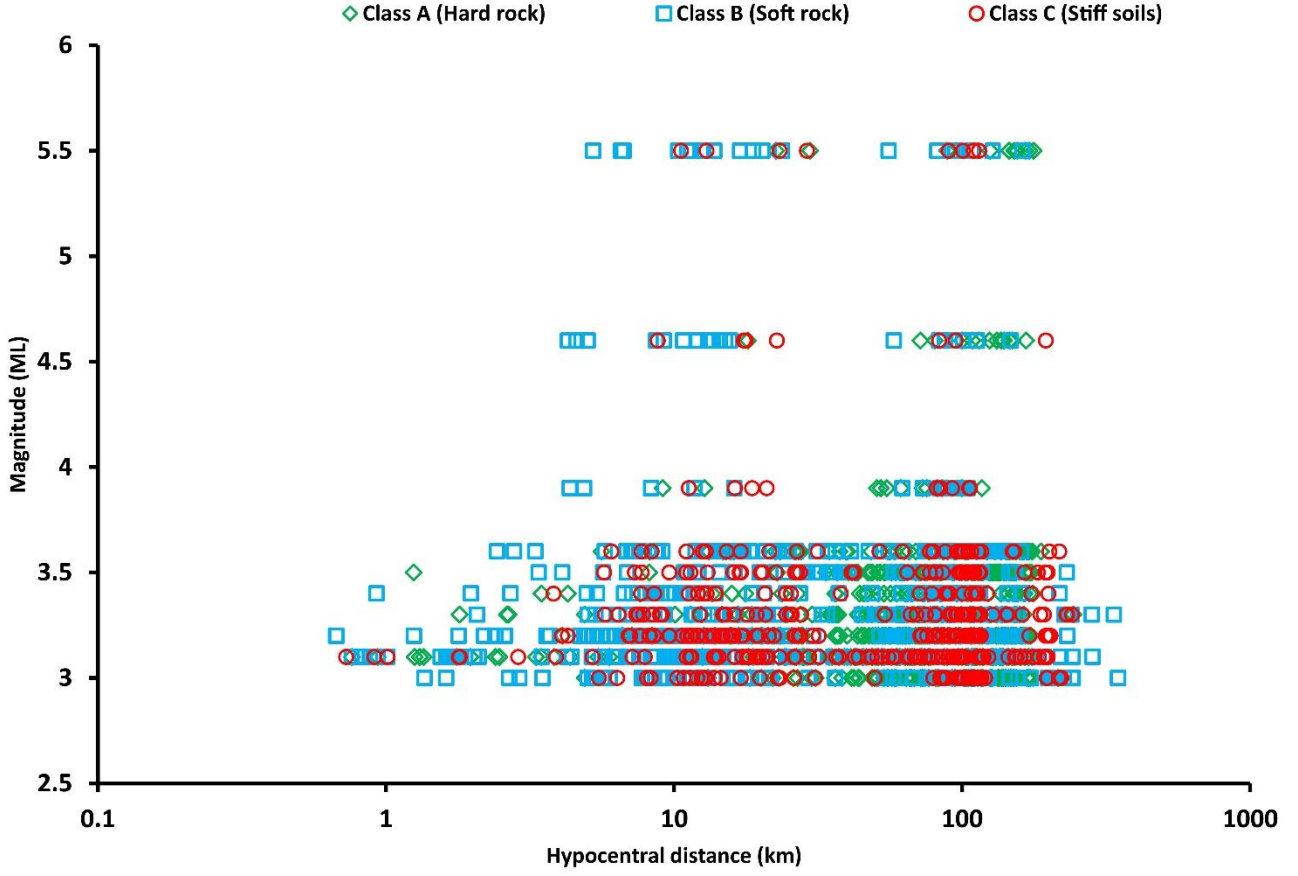
Figure 7-2: Illustration of site classification of the seismic station records representing different site classes based on NEHRP site classification.
