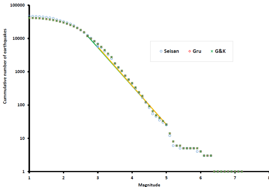
Figure 8-6: The G-R distribution for the three declustered catalogues used for sensitivity analysis. Seisan is from the CLUSTER program in SEISAN, Gru is the catalogue declustered with the Grunthal (1985) and G&K is from the Gardner and Knoppoff (1975) catalogue.
