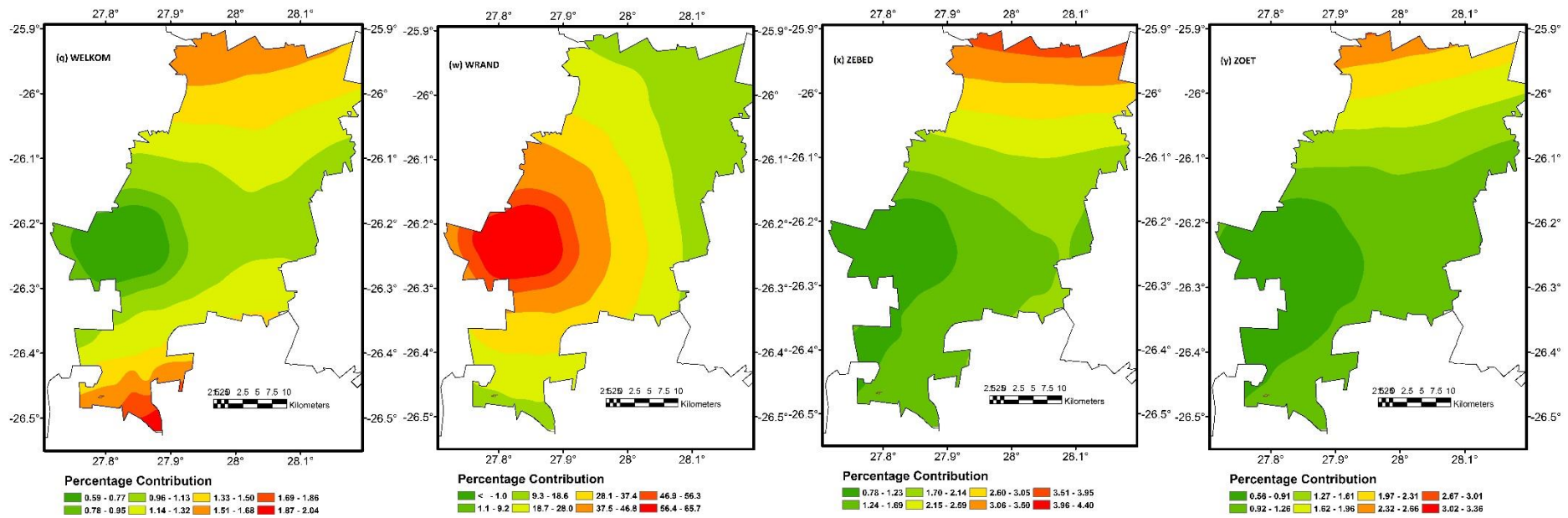
Figure 8-10: Maps showing the % contribution of the delineated zones to the total hazard for PGA for Johannesburg. Note the variation in the percentage value. Each map is scaled according to its own range of values.
