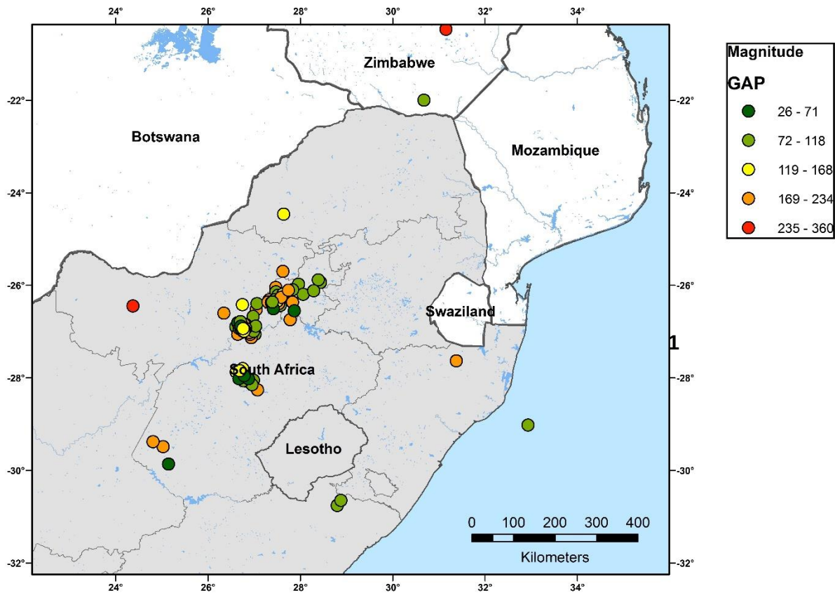
Figure 4-11. Map showing the typical GAP values obtained during the analysis and their distribution with epicentres.
