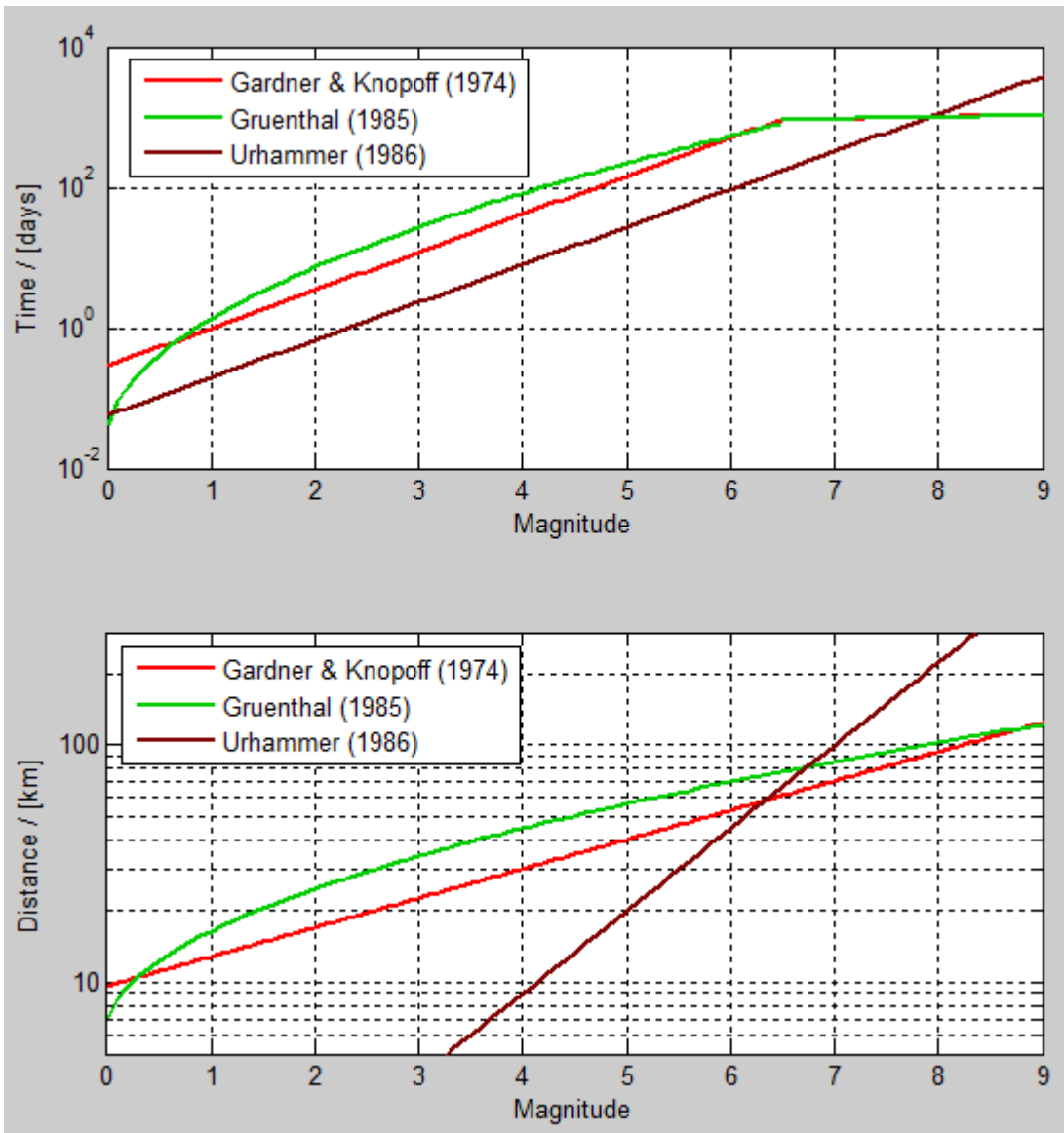
Figure 4-17: Spatial-temporal variation of the dependence windows for the three windows-based declustering techniques.
