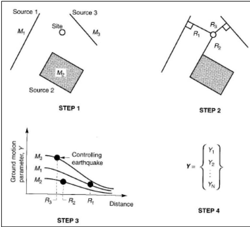
Figure 2-1: The four-step process of a deterministic seismic hazard assessment process (Reiter, 1990).
