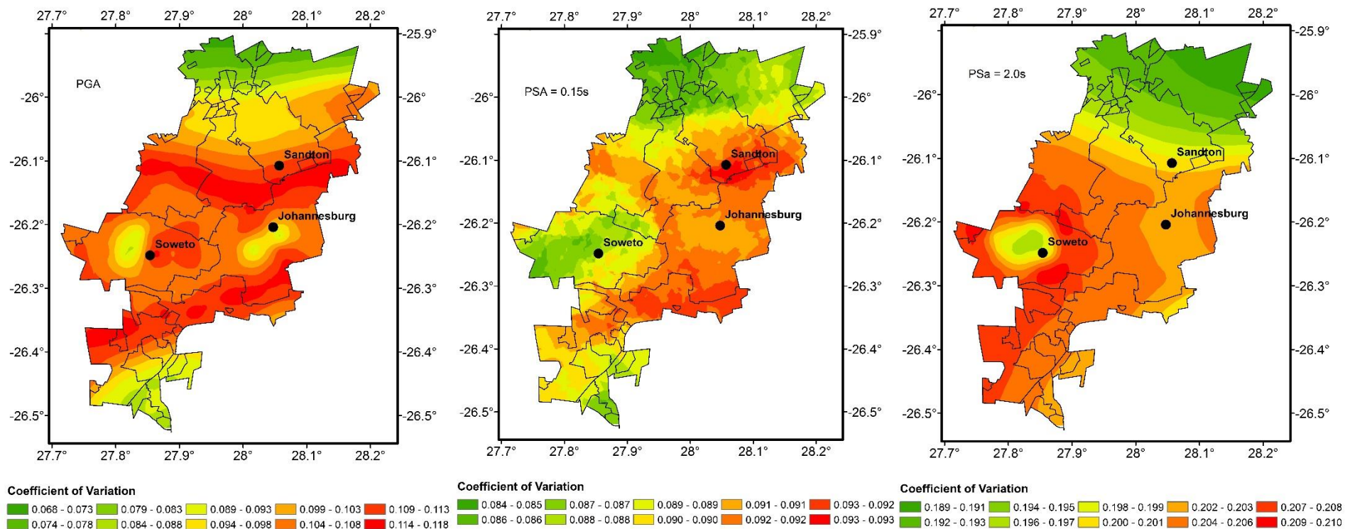
Figure 8-13: COV results for the sensitivity analysis for bedrock shearwave velocity V_s .
