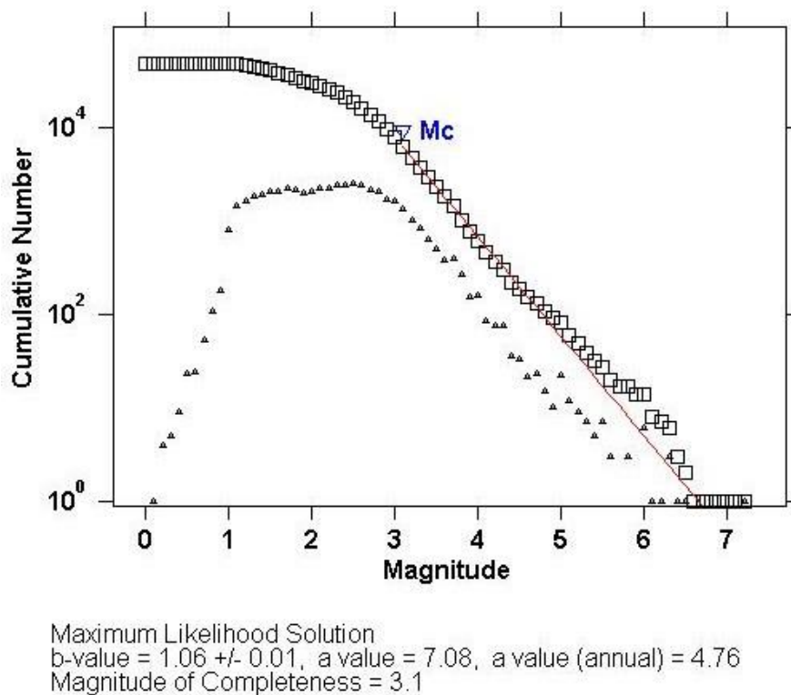
Figure 4-20: Estimation of the magnitude of completeness using Maximum-Curvature.
