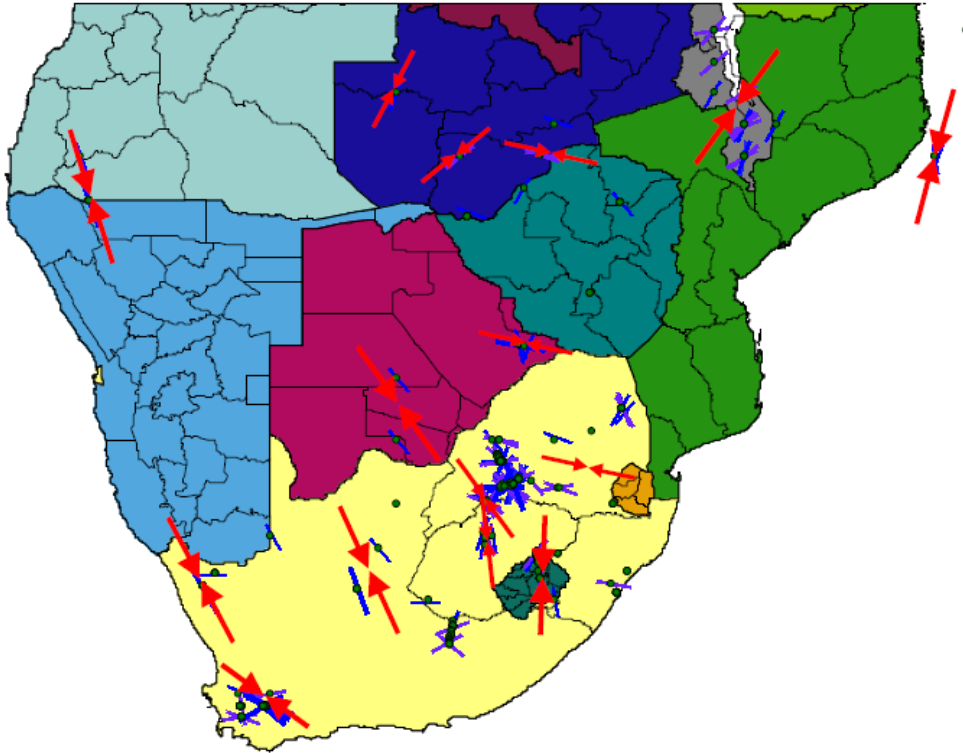
Figure 5-4: Orientations of the major horizontal stresses from in-situ measurements by Stacey and Wessloo (1998). Red arrow indicate compressive stress, blue lines shows extensional stress orientations.
