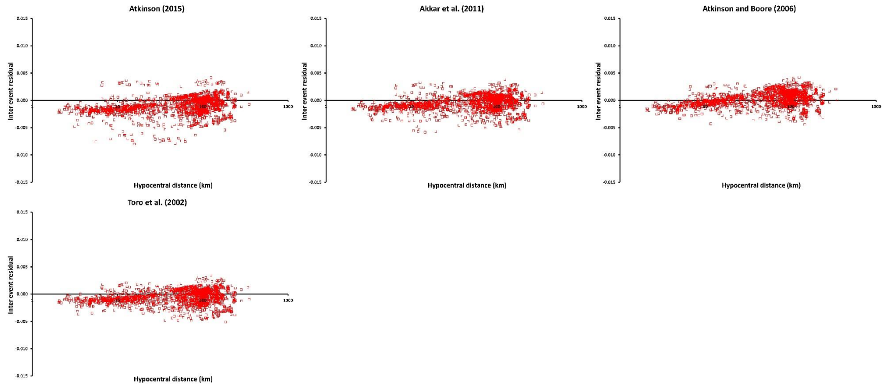
Figure 7-4: The inter-event residuals of all GMPEs for PSA ( T = 0.15s ) versus hypocentral distance.
