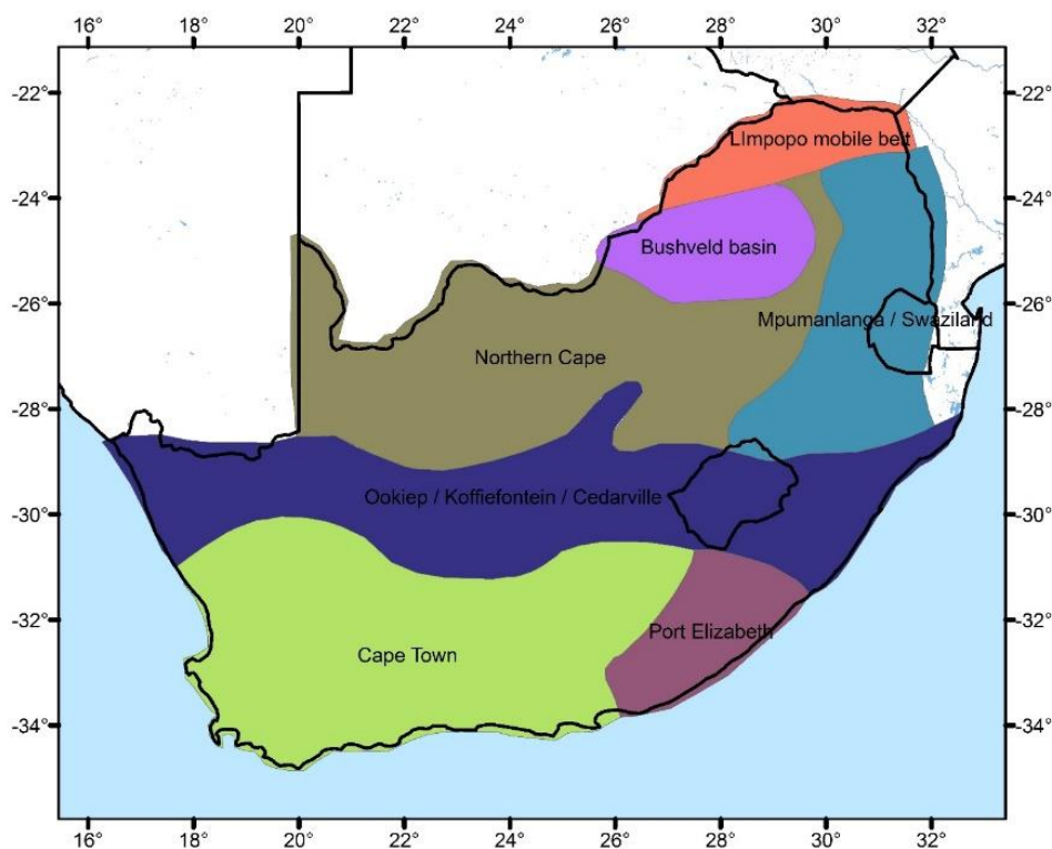
Figure 5-1: A seismotectonic model for South Africa proposed by Partridge (1995).
