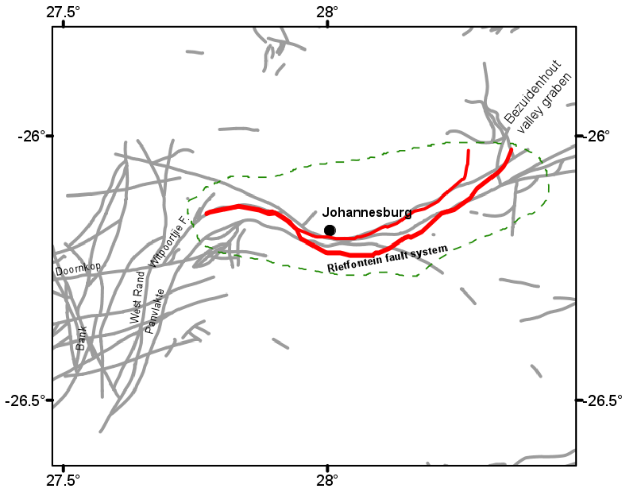
Figure 3-4: The Rietfontein Fault system and the related structural features of the Witwatersrand Basin (modified from Myers et al., 1990).
