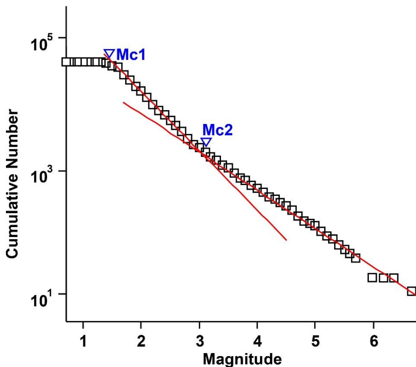
Figure 4-16: Frequency magnitude distribution of the current catalogue for seismicity in and around Johannesburg. Effect of mining related seismic events are illustrated by the 2 G-R lines (in red). The first cut-off magnitude M_{C1} shows the G-R distribution for small mining related events and the second M_{C2} shows the G-R distribution for tectonic events.
