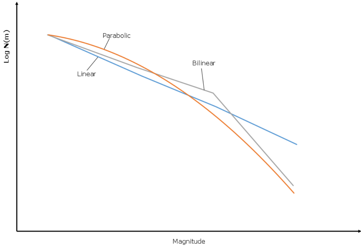
Figure 2-5: Linear, Bilinear and Parabolic recurrence relationships.
