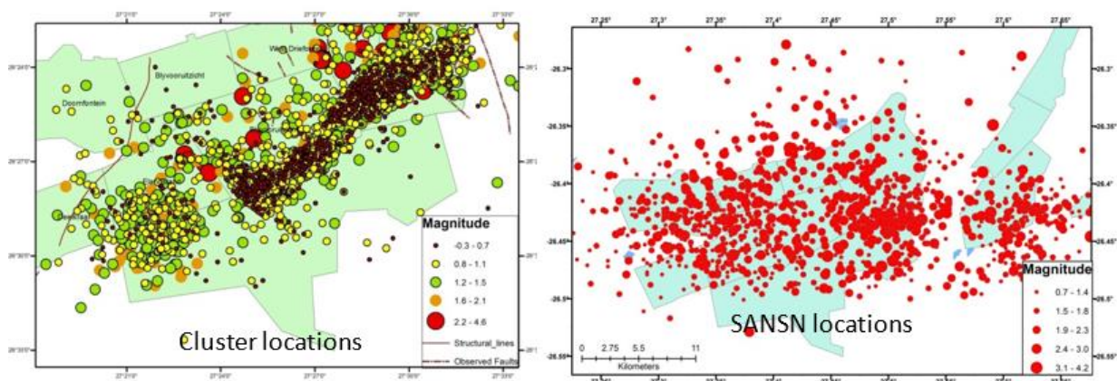
Figure 2-7: Illustration of possible influence of errors in earthquake locations in seismic source delineations in the West Rand region. Comparison of locations produced by a) cluster network and b) national network location.
