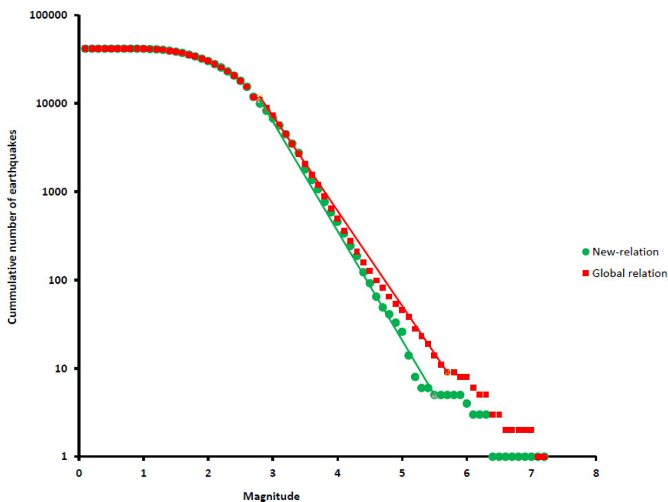
Figure 8-2: G-R curves for the two catalogues used for sensitivity analysis for the homogenisation process. New relation refers to the homogenisation relations developed by Manzunzu et al. (2020) as applied while Global relation refers to the Deichmann (2006) magnitude homogenisation relation.
