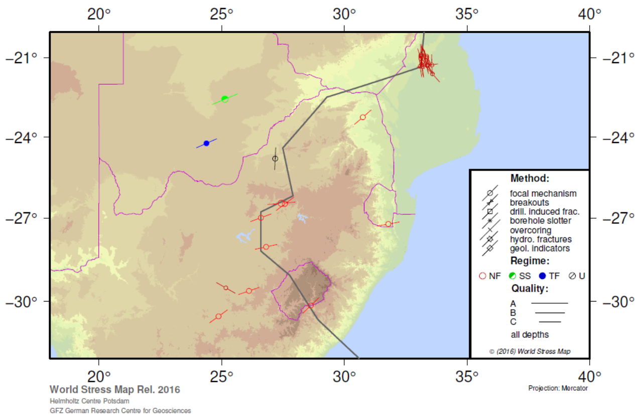
Figure 5-8: Stress inversion from focal mechanism orientation data plotted using the CASMO software (Heidbach et al., 2018) for the inverted focal mechanism solutions.
