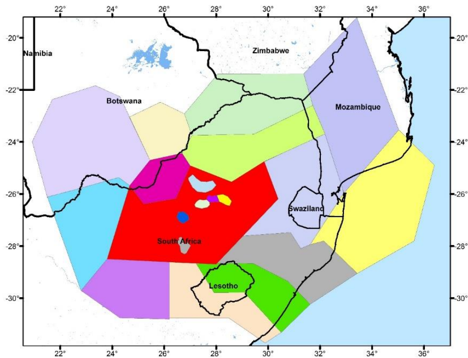
Figure 5-11: Seismic source zones identified for this study. The smaller zones found within the red zone are the mining-related zones.
