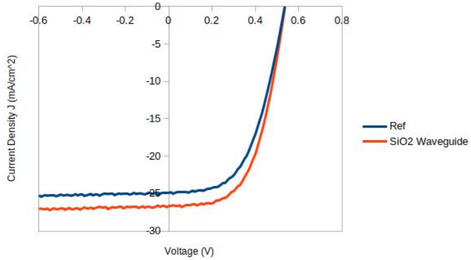
Figure 5.5: The J - V characteristics of commercial a - Si solar with silica waveguide
