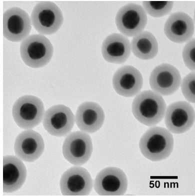
(a) Au@SiO_2 core shells
