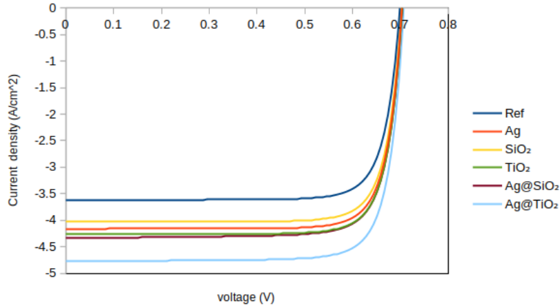
Figure 3.8: J - V curve of c - Si solar cell incorporated with Ag NPs, SiO_2 NPs, TiO_2 NPs, Ag@SiO_2 core-shell NPs and Ag@TiO_2 core-shell NPs.
