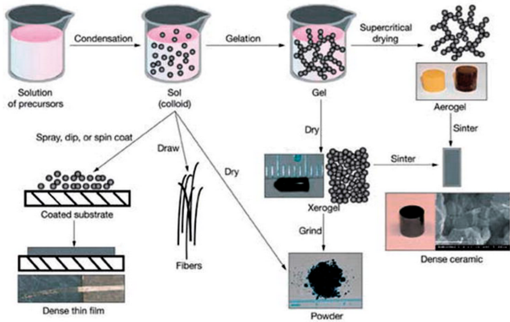
Figure A.1: Schematic representation of the different stages and routes of the sol–gel technology [198]
