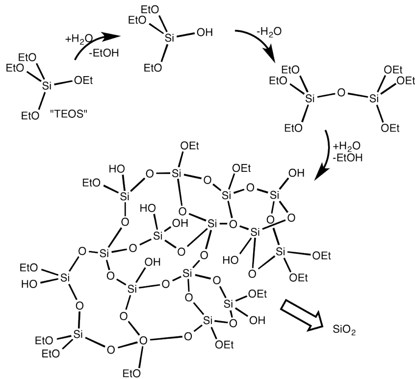
Figure 4.1: Hydrolysis and condensation of TEOS in the Stöber process [133].
