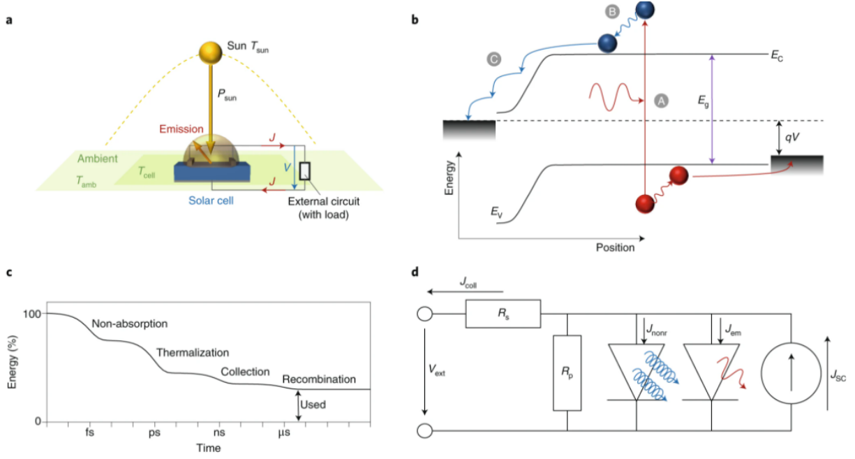
Figure 2.6: Schematic of the Shockley-Queisser model [59].
