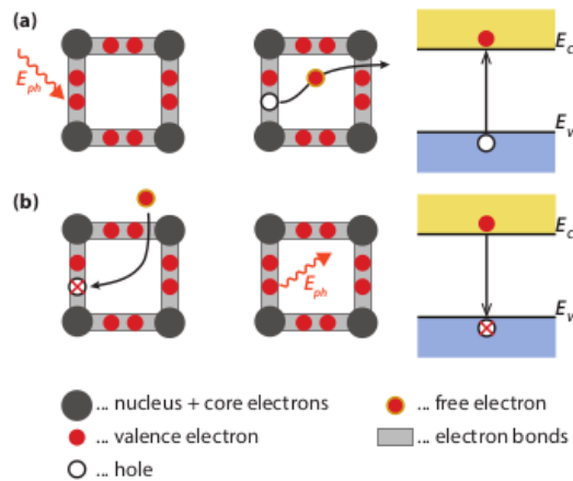
Figure 2.7: Visualisation of bandgap-to-bandgap (a) generation and (b) recombination processes using the bonding model and the energy band diagram [72].
