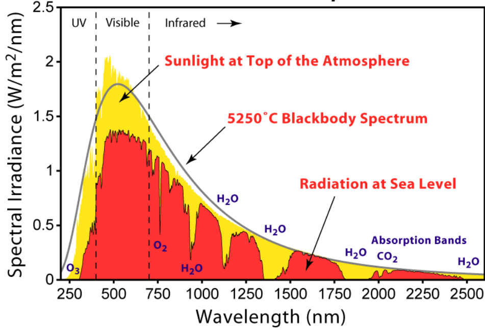
Figure 2.2: Solar cell spectrum (sourced from [40]).
