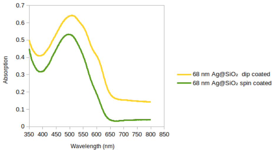
Figure 4.12: Absorption spectra of \text{Ag@SiO}_2 core-shell NPs deposited with two different methods (dip and spin coating).
