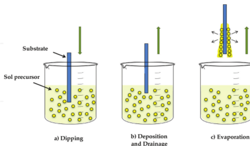
Figure A.2: Sequential stages of the dip-coating technique for thin film deposition: (a) the substrate is dipped and immersed in the sol precursor, (b) the substrate is withdrawn at constant speed rate, and (c) solvent evaporation yields to the gelation of the layer. [199]
