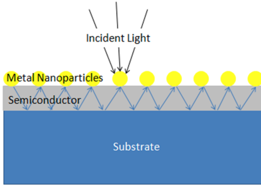
Figure 2.10: Basic solar cell structure with metallic NPs [44].
