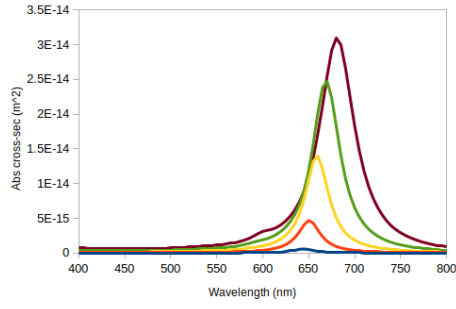
(a) Ag@TiO_2 core-shell NPs absorption cross-section
