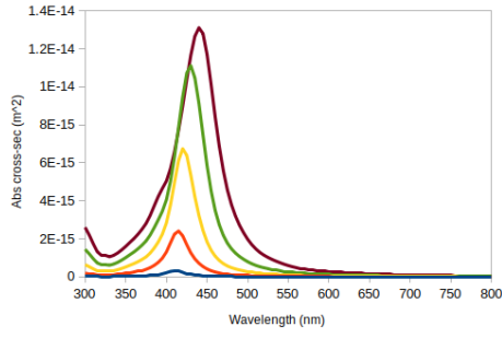
(a) Ag@SiO_2 core-shell NPs absorption cross-section
