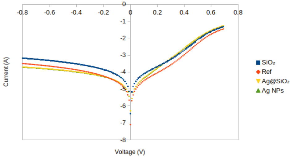
Figure 4.21: Semi-Log dark current of a commercial a - Si solar incorporated with Ag NPs, SiO_2 NPs and Ag@SiO_2 core-shell NPs.
