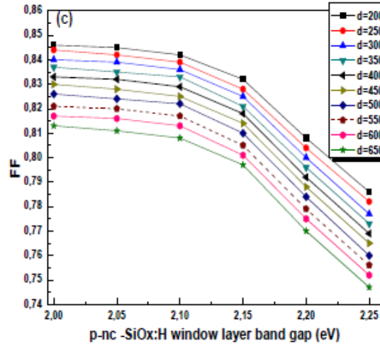
Figure 2.5: FF decrease with an increase of the band gap in the semiconductor and with an increase of the absorber layer thickness d [55].
