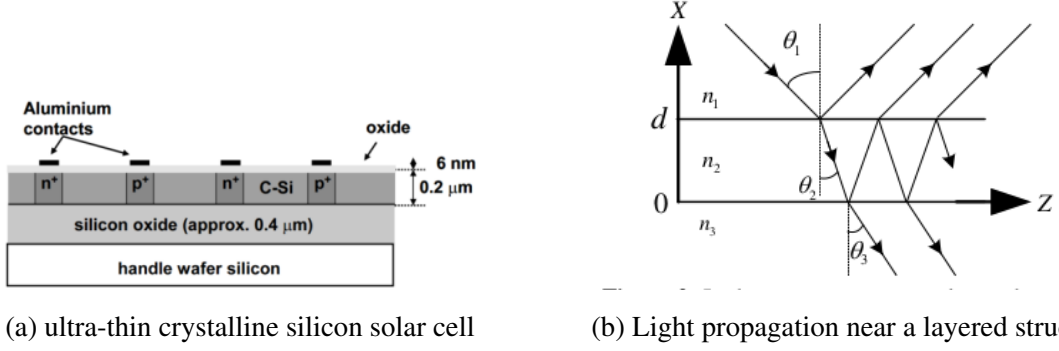
Figure 2.11: Basic structure for c-Si solar cell and refractive-index profile of the optical waveguide [51, 98].
