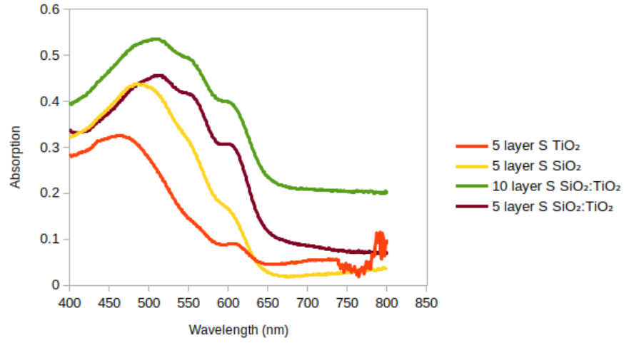
(a) Sintering after depositing every layer
