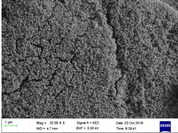
(a) 85.51 nm \text{SiO}_2 nanospheres
