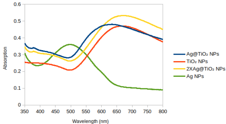
Figure 4.16: Absorption spectra of \text{Ag} NPs, \text{TiO}_2 NPs and \text{Ag@TiO}_2 core shells NPs.
