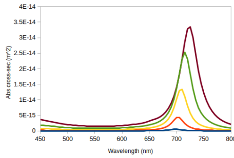
(c) Au@TiO_2 core-shell NPs absorption cross-section
