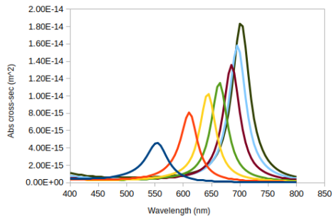
(c) Au@TiO_2 core-shell NPs absorption cross-section
