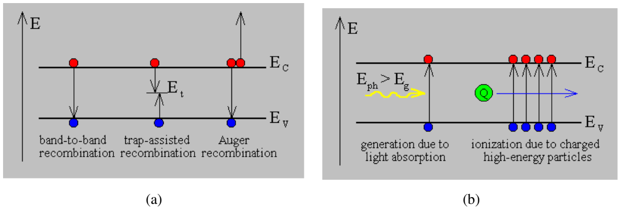
Figure 2.8: Carrier recombination mechanisms in semiconductors [75].
