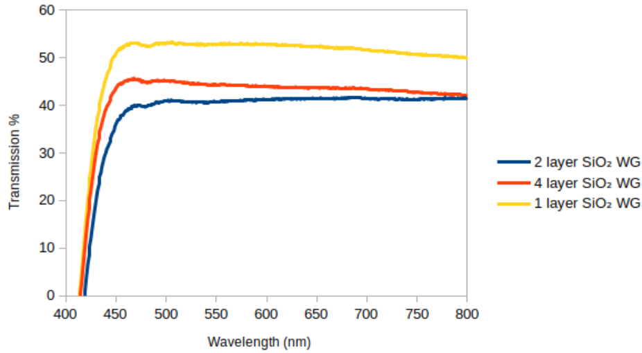
Figure 5.2: Transmission spectra of silica waveguides with different number of layers dip coated on a microscope glass slab, that were thermal treated after a layer or all layers were deposited.
