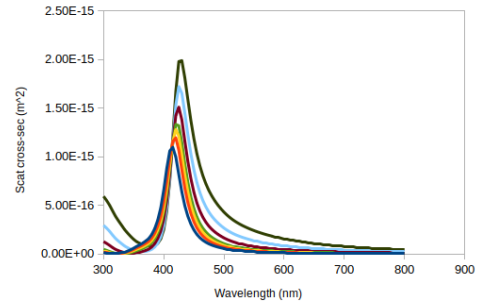
(b) \text{Ag}@/\text{SiO}_2 core-shell NPs scattering cross-section
