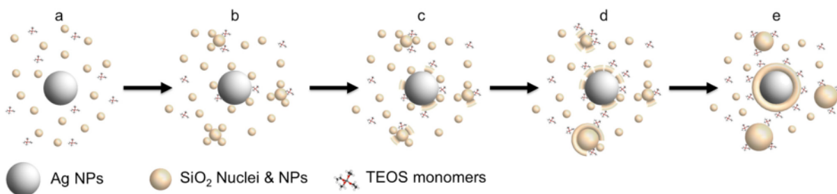
Figure 4.2: The \text{SiO}_2 shell development mechanism on the \text{Ag} core is depicted schematically. (a) \text{SiO}_2 primary nuclei arise in the initial stage and (b) slowly aggregate among themselves as well as onto \text{Ag NP} surfaces and (c) to form ravined structures. These ravines are gradually filled with fresh \text{SiO}_2 nuclei (d) until the \text{Ag NPs} are completely wrapped (e). \text{TEOS} monomers are also introduced to \text{NPs} at the same time and contribute to the surface smoothing [139].
