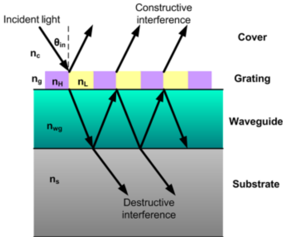
Figure 5.1: Schematic RWG coupling at resonance from the model provided by Rosenblatt et al [172]
