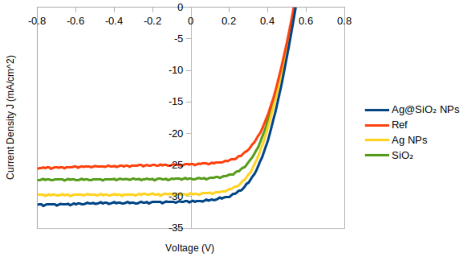
Figure 4.19: The J - V curve of a commercial a - Si solar cell incorporated with Ag NPs, SiO_2 and Ag@SiO_2 core-shell NPs.
