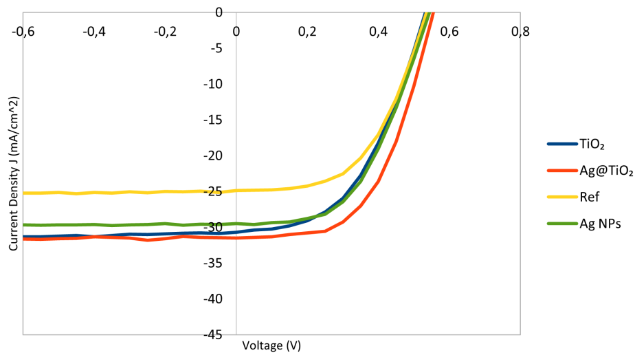
Figure 4.20: The J - V curve of a commercial a -Si solar incorporated with Ag NPs, Ag@TiO_2 and TiO_2 core-shell NPs
