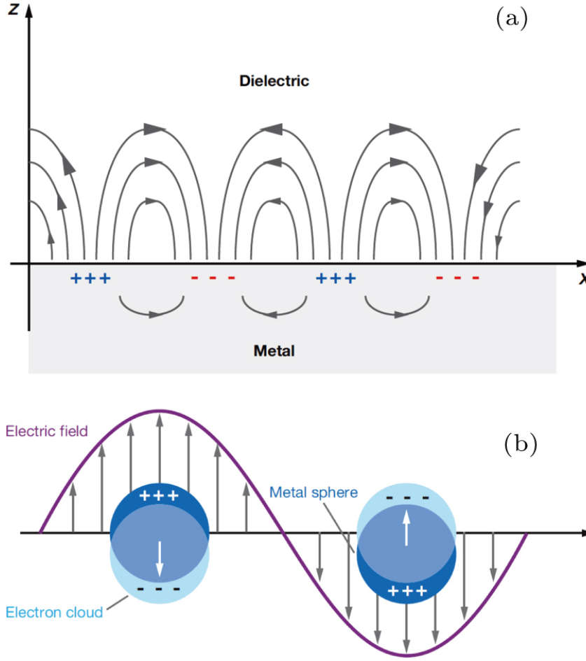
Figure 2.9: Incident light on a metallic NPs causes the conduction band electrons to oscillates and is known as the localized surface plasmon [83] .
