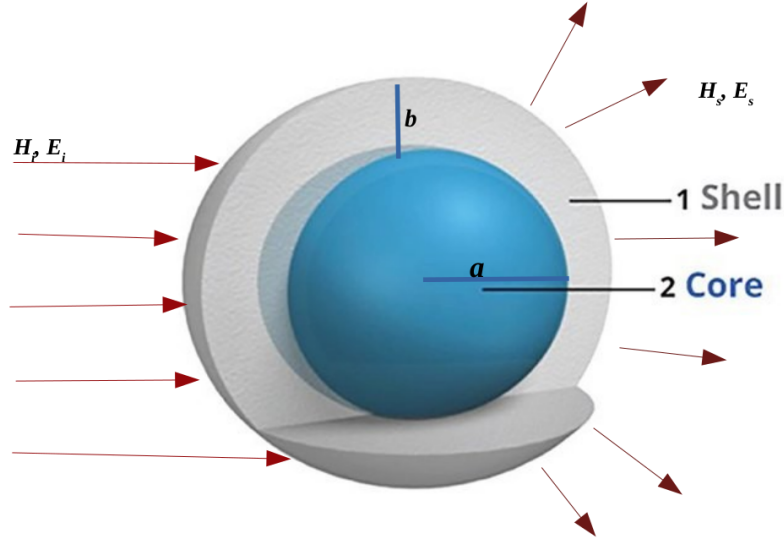
Figure 3.1: Scattering for non-interactive core-shell nano-sphere [103].
