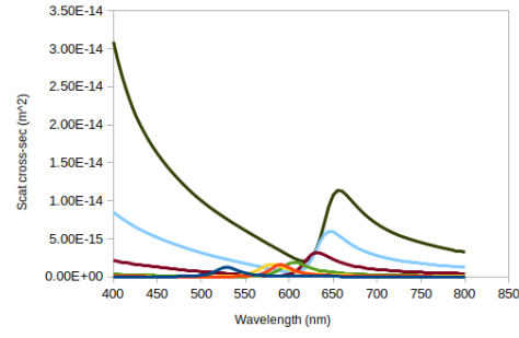
(b) Ag@TiO_2 core-shell NPs scattering cross-section
