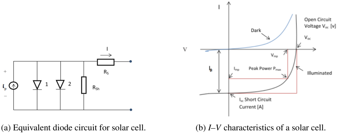
Figure 2.4: Circuit structure and I - V characteristics of a solar cell in the dark and under illumination [51].
