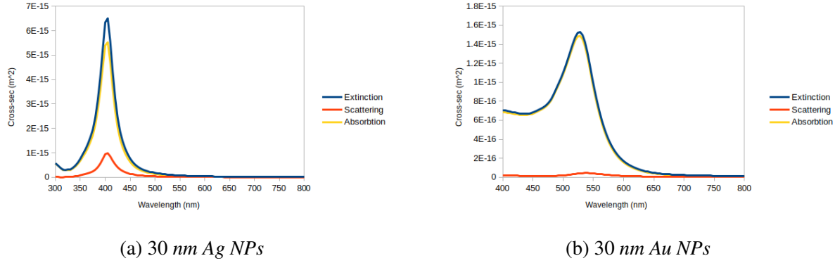
Figure 3.2: The absorption and scattering cross-section of 30 nm spherical Ag And Au NPs
