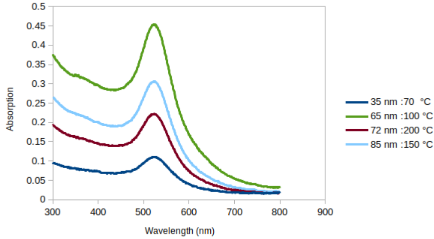
Figure 4.13: The absorption spectra of spherical like \text{SiO}_2 NPs synthesized at 70, 100, 150 and 200 °C respectively
