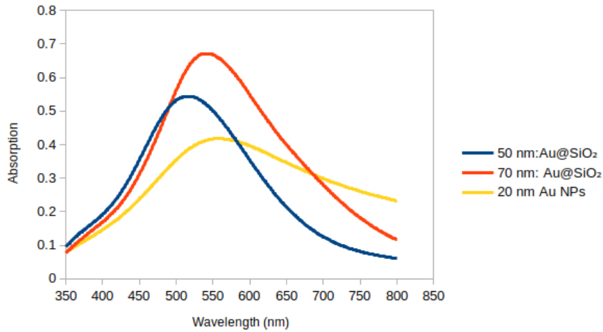
Figure 4.14: The absorption of Au NPs and Au@SiO 2 core-shell NPs having different Au NPs concentrations.
