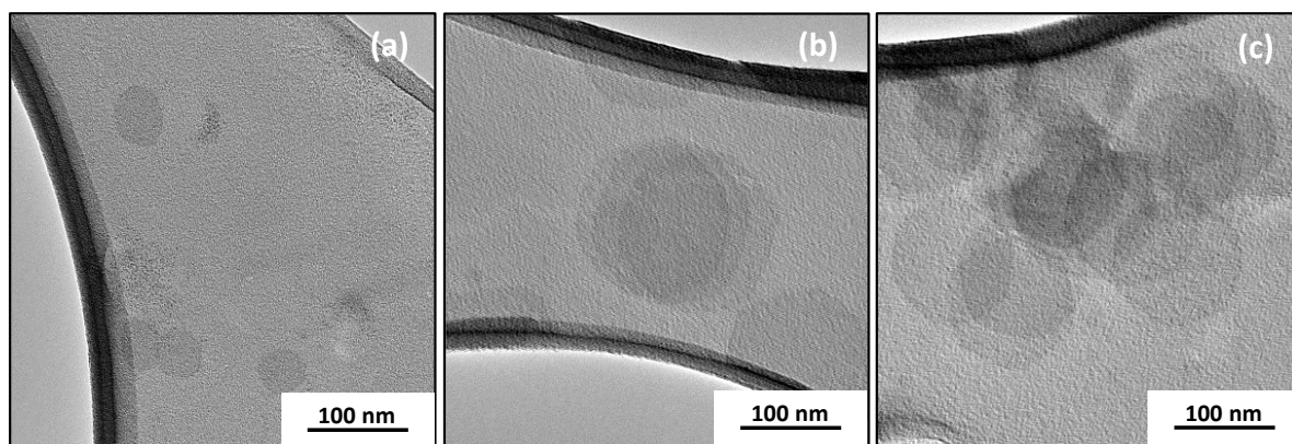
Figure 4.20: TEM images of OLA/ \beta -In 2 S 3 nanostructures synthesized for (a) 120 min, (b) 150 min, and (c) 180 min in OLA with 1-DDT as source of sulphur.
