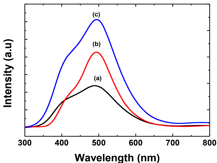
Figure 4.10: PL spectra of OLA/ \beta - \text{In}_2\text{S}_3 nanostructures synthesized for (a) 60 min, (b) 120 min, and (c) 150 min in the 1:1.5 (In:S) reaction system.
