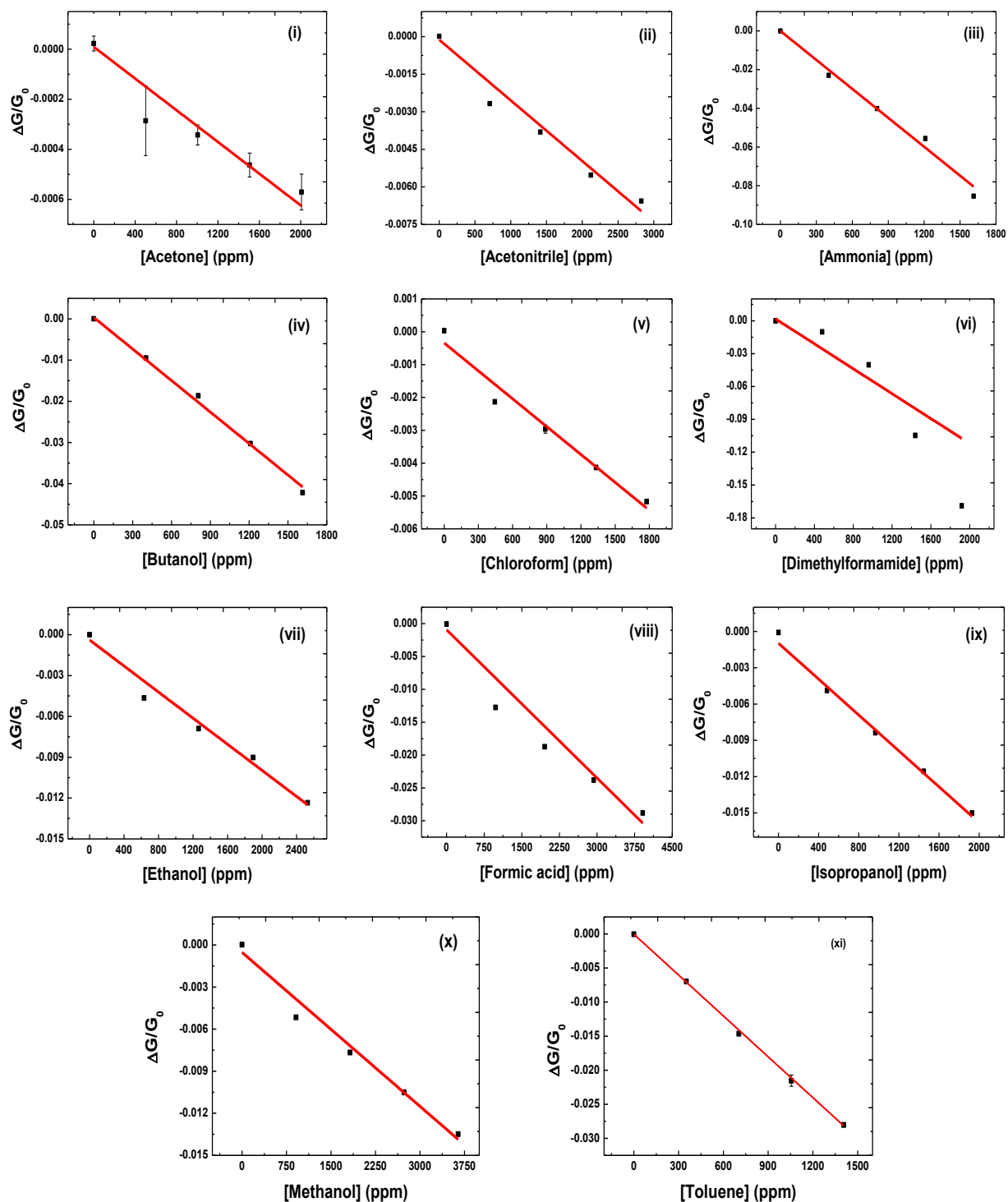
Figure 3.45: Response curves of OLA/WS 2 nanostructures (60 min).
