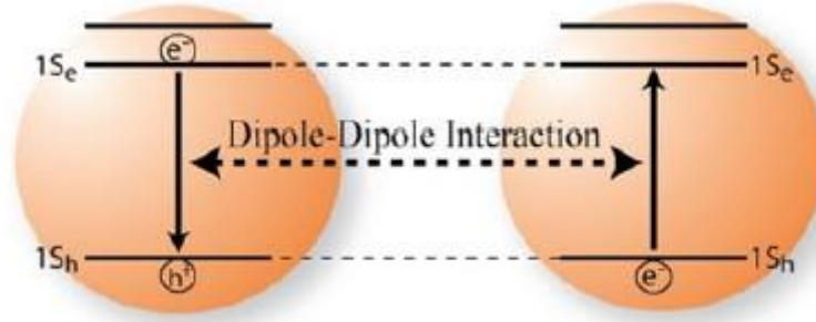
Figure 2.7: Schematic representation of resonant exciton energy transfer from the donor QD (left) to the acceptor QD [12].
