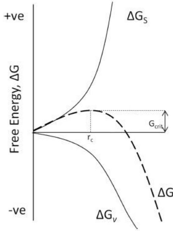
Figure 2.9: A maximum free energy \Delta G at a critical cluster size, r_c , which defines the first stable particles – the nuclei [78, 81].
