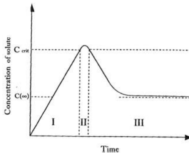
Figure 2.8: Schematic representation of the LaMer diagram [78].
