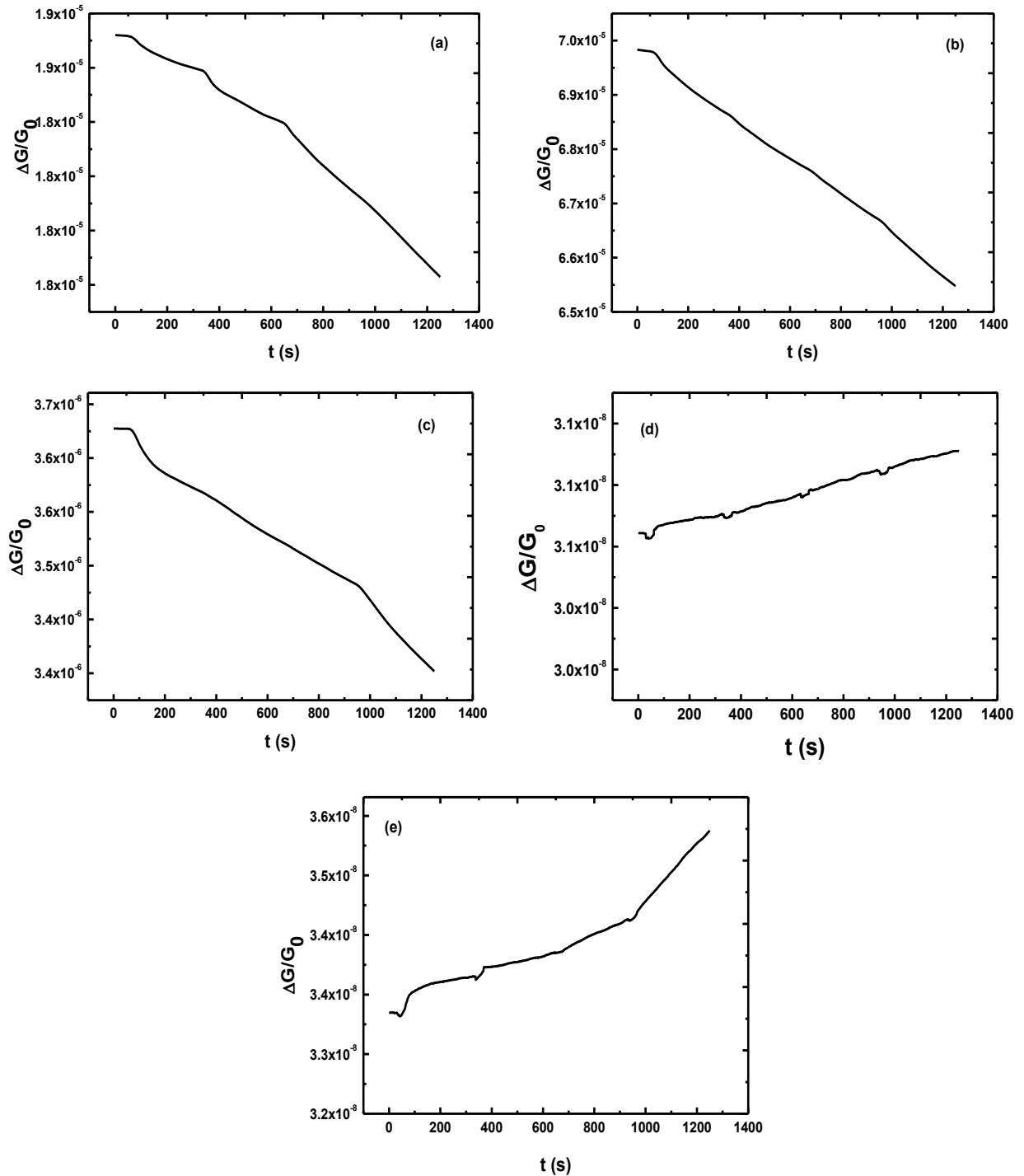
Figure 3.21: (a)-(e) Gas response of the OLA/ \text{WS}_2 based sensors (15, 45, 60, 180 and 240 min) to \text{NH}_3 vapour at different concentrations.
