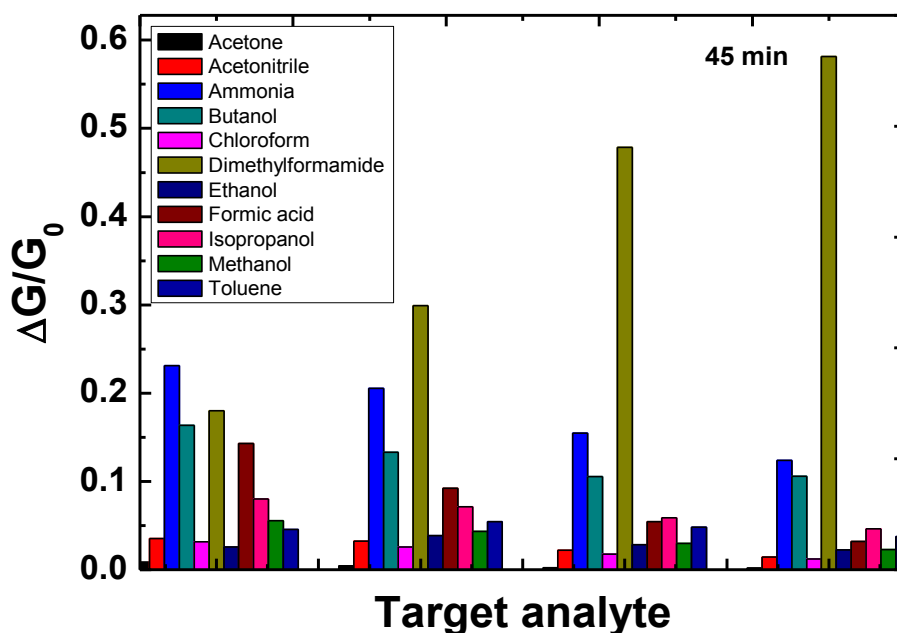
Figure 3.49: Selectivity tests of the OLA/WS 2 sensor (45 min) at 1.5, 3.0, 4.5 and 6.0 μL of NH 3 and various VOCs.
