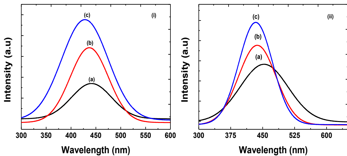
Figure 4.35: PL spectra of (i) HDA/ \beta - \text{In}_2\text{S}_3 at (a) 60 min, (b) 90 min, and (c) 150 min; (ii) HDA/1-DDT_ \beta - \text{In}_2\text{S}_3 at (a) 60 min, (b) 90 min, and (c) 150 min.
