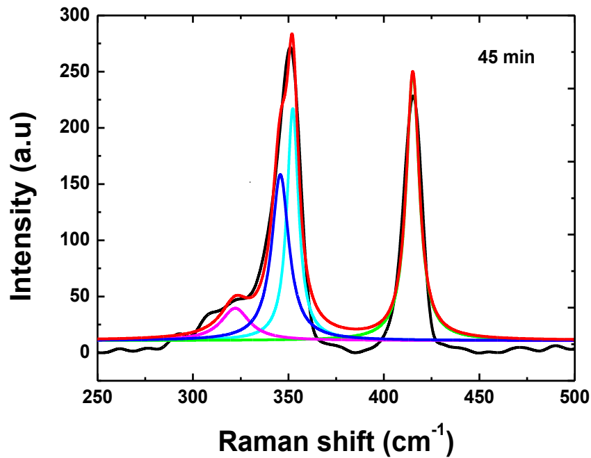
Figure 3.13: Lorentzian multi-peak fit of the Raman spectra of OLA/WS 2 nanostructures at 45 min. The black line represents the experimental data; the red, magenta, blue, cyan and green lines represent the combined peak fitting, the individual contributions of the most intense phonon modes.
