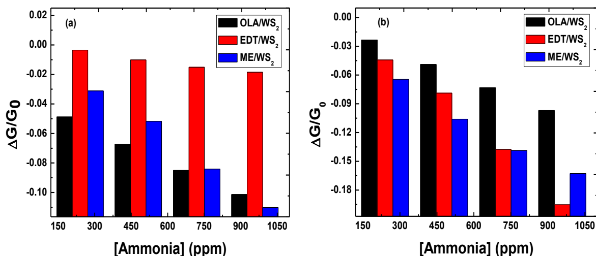
Figure 3.58: Histograms representing the response of OLA/WS 2 , EDT/WS 2 and ME/WS 2 sensors from the (a) 15 min and (b) 45 min towards 240, 479, 719 and 958 ppm of NH 3 under limited light and low humidity.
