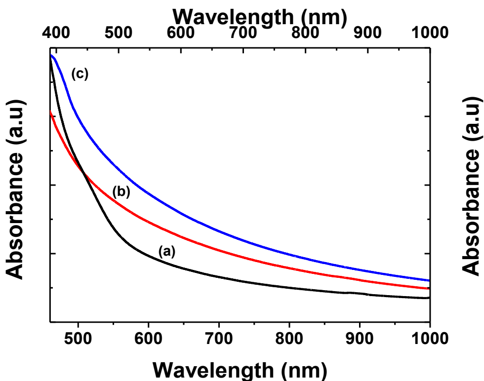
Figure 4.13: UV-vis spectra of OLA/ \beta - \text{In}_2\text{S}_3 nanostructures synthesized for (a) 60 min, (b) 120 min, and (c) 150 min in the 1:2 (In:S) reaction system.
