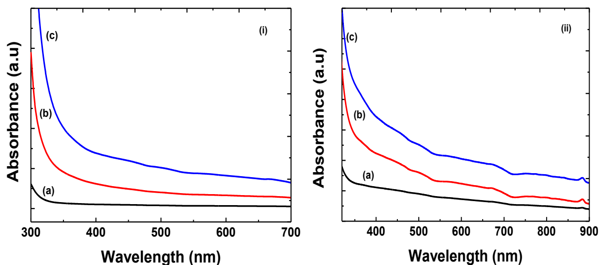
Figure 4.34: UV-vis spectra of (i) HDA/ \beta - \text{In}_2\text{S}_3 at (a) 60 min, (b) 90 min, and (c) 150 min; (ii) HDA/1-DDT_ \beta - \text{In}_2\text{S}_3 at (a) 60 min, (b) 90 min and (c) 150 min.
