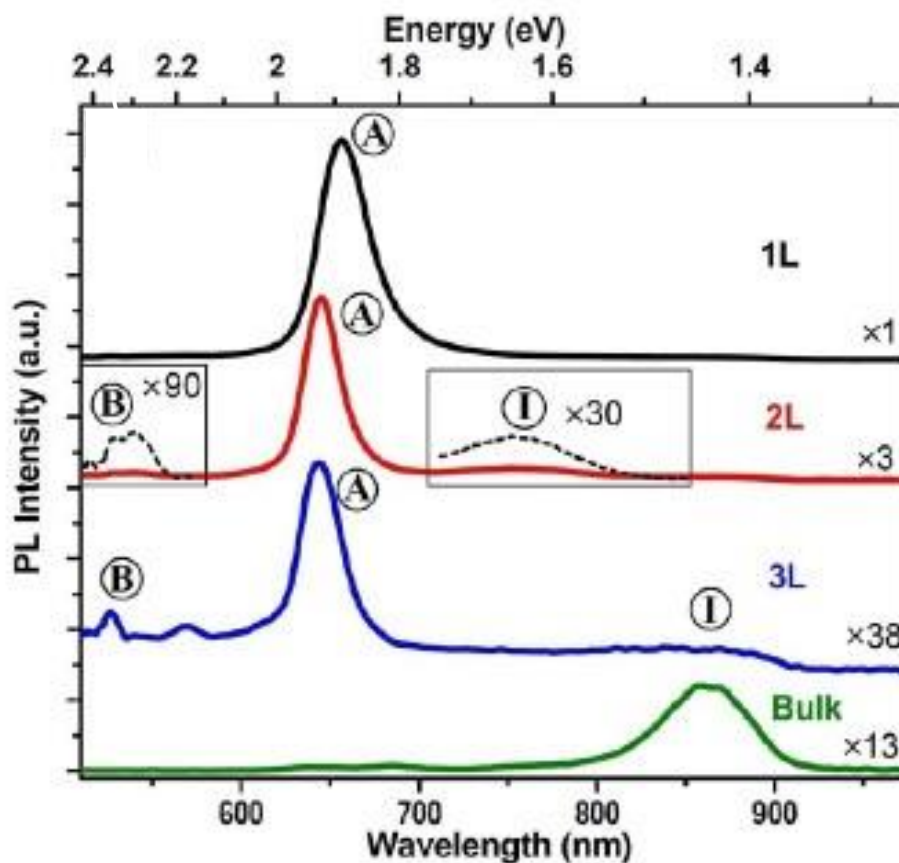
Figure 3.19: PL intensities for mono-, bi- and three-layered WS 2 nanostructures at 488 nm excitation wavelength with the positions for the excitons A and B as well as the indirect band gap (I) [8].
