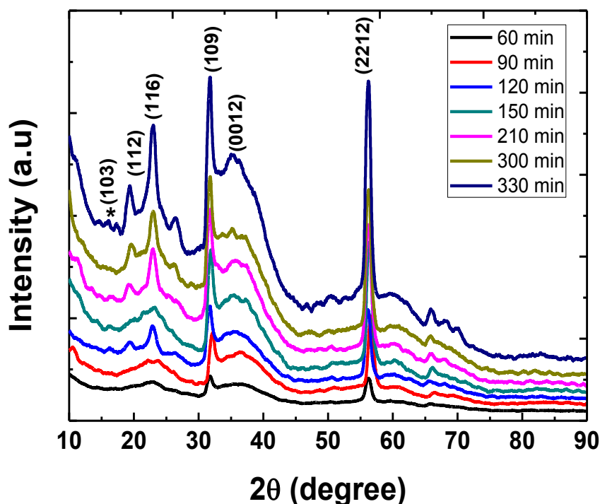
Figure 4.4: XRD patterns of OLA/ \beta - \text{In}_2\text{S}_3 nanostructures at different reaction times in the 1:1 (In:S) reaction system.
