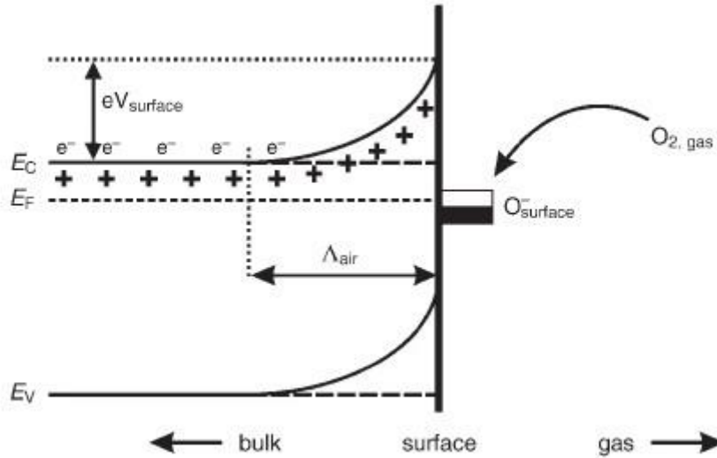
Figure 2.11: A schematic representation of a simplified model of band bending in a wide bandgap semiconductor after chemisorption of charged species ( e.g. ionosorption of oxygen) on surface sites. E_C , E_V , and E_F represent the energy of the conduction band, valence band, and the Fermi level, respectively, while \Lambda_{air} denotes the thickness of the space-charge layer, and eV_{surface} the potential barrier. The conducting electrons are represented by e^- and + represents the donor sites [94].
