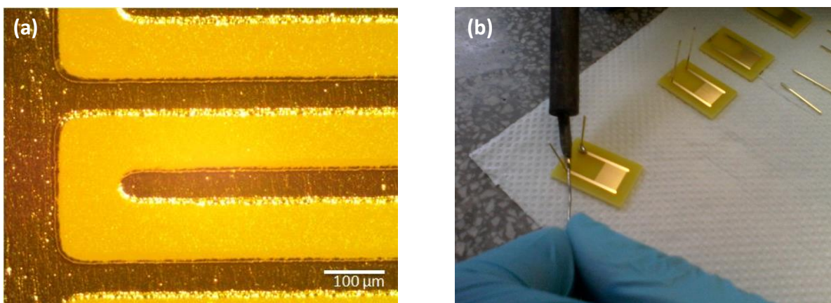
Figure 3.4: Optical image of the IDE is represented by (a) while (b) shows soldering of contacts onto IDEs.
