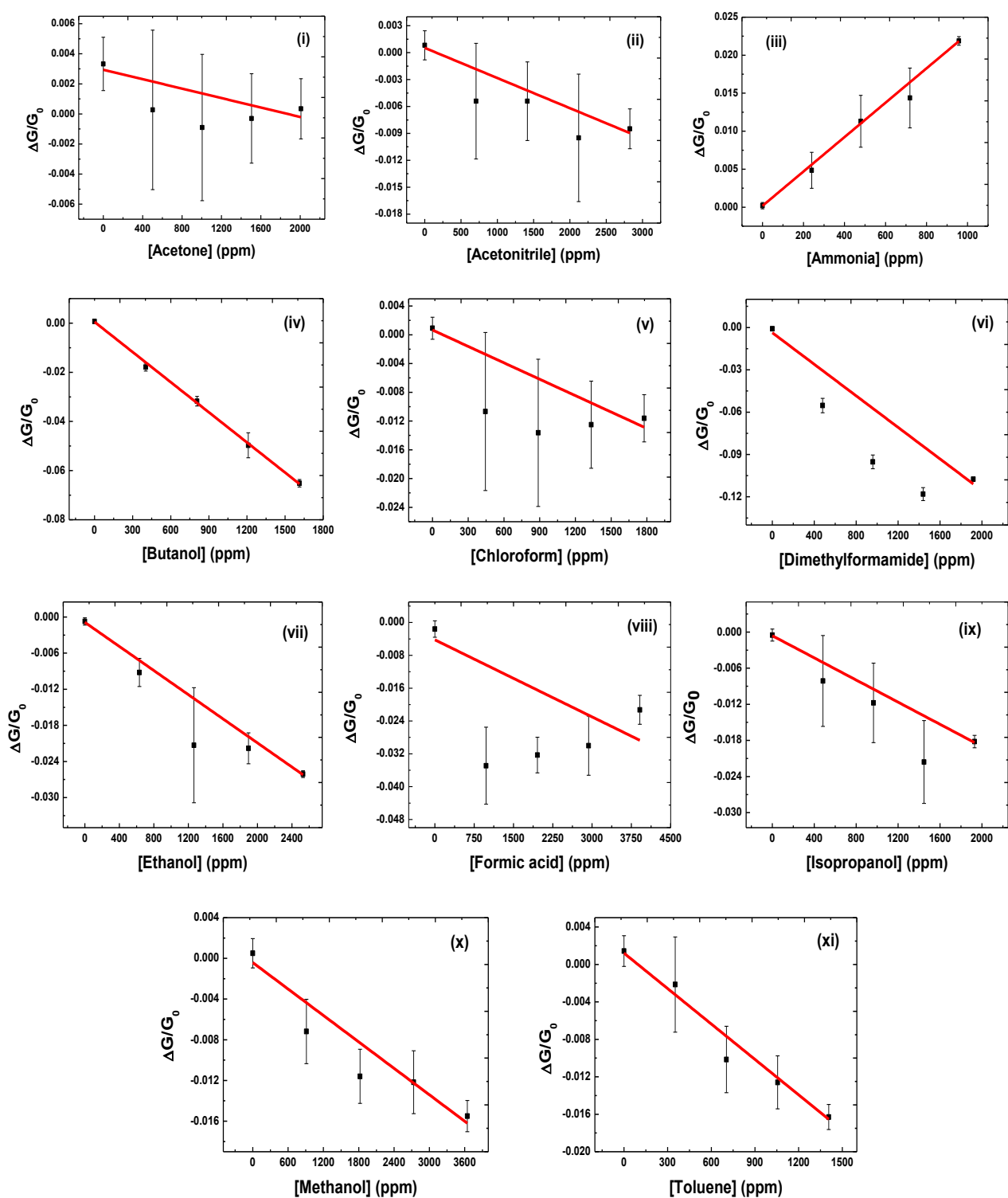
Figure 3.46: Response curves of OLA/WS 2 nanostructures (180 min).
