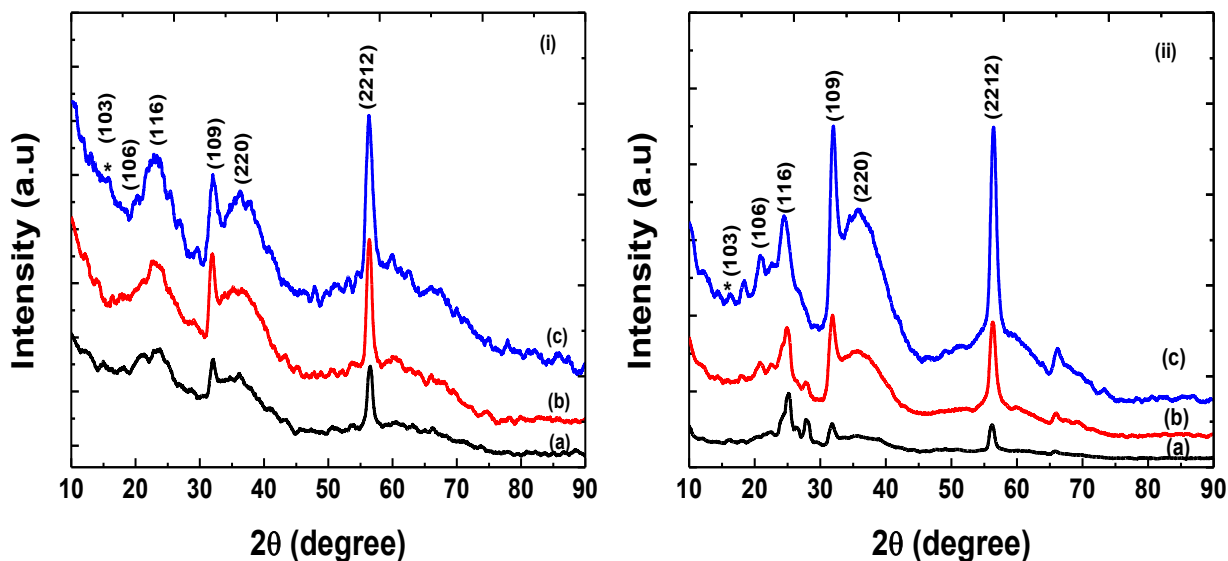
Figure 4.21: XRD patterns of OLA/ \beta - \text{In}_2\text{S}_3 nanostructures at (a) 60 min, (b) 90 min, and (c) 150 min; (i) OLA / 0.2 mL of 1-DDT and (ii) OLA / 0.4 mL 1-DDT.
