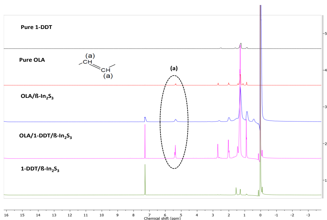
Figure 4.25: Solution 1 H NMR spectra obtained on CDCl 3 dispersions of the free capping agents and capped \beta -In 2 S 3 nanostructures.
