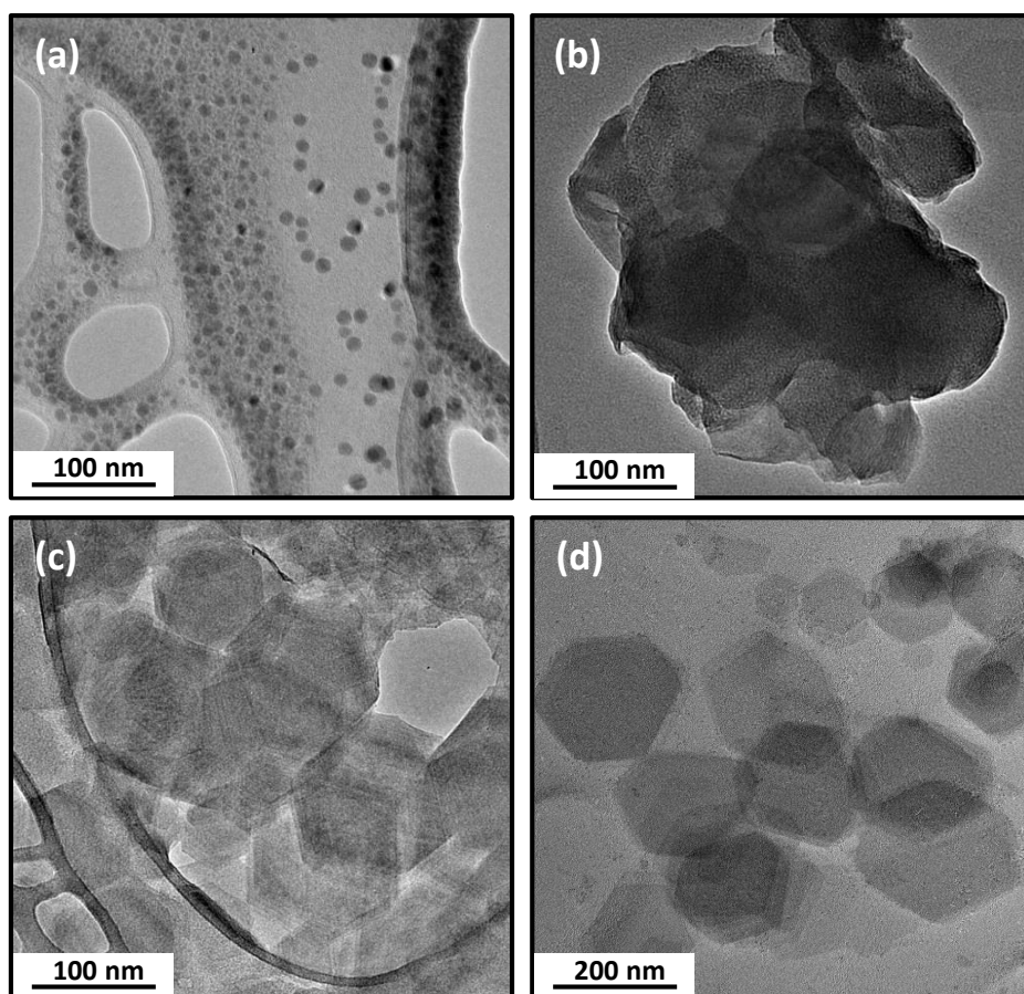
Figure 4.16: The TEM images of OLA/ \beta\text{-In}_2\text{S}_3 nanostructures in the 1:1 (In:S) reaction system: (a) 60 min, (b) 90 min, (c) 120 min and (d) 150 min.
