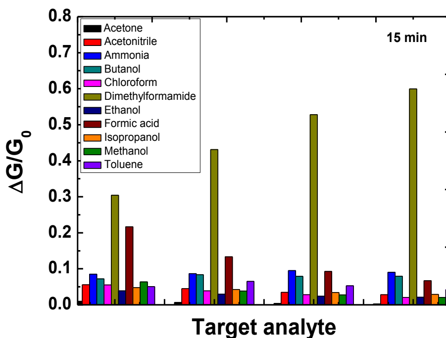
Figure 3.48: Selectivity tests of the OLA/WS 2 sensor (15 min) at 1.5, 3.0, 4.5 and 6.0 μL of NH 3 and various VOCs.
