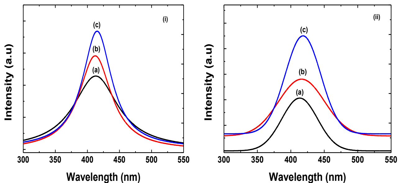
Figure 4.27: PL spectra of (i) OLA/0.2 mL 1 -DDT/ \beta -In 2 S 3 nanostructures and (ii) OLA/0.4 mL 1 -DDT/ \beta -In 2 S 3 nanostructures at (a) 60 min, (b) 90 min, and (c) 150 min.
