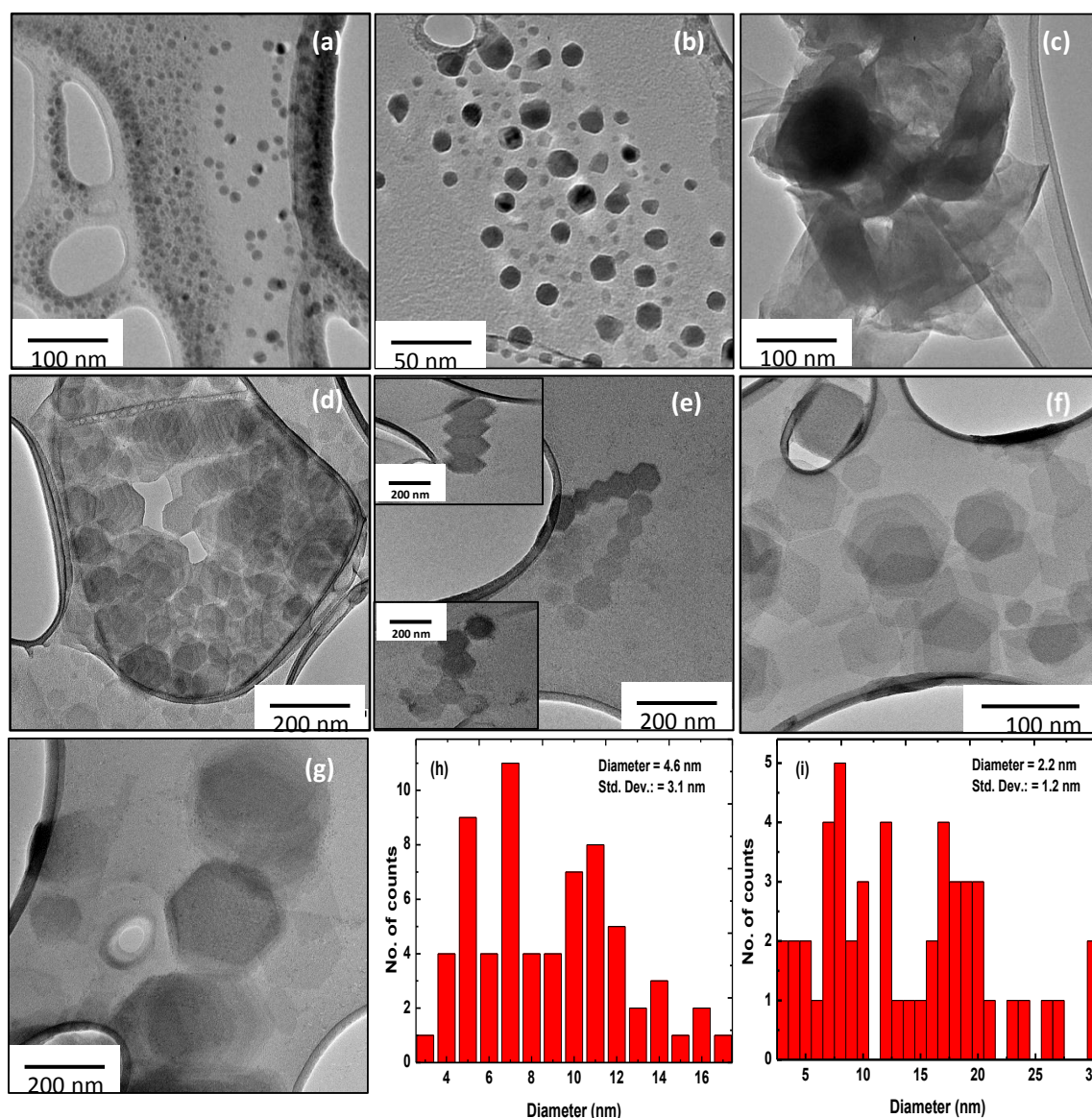
Figure 4.3: The TEM images of OLA/β-In 2 S 3 nanostructures in the 1:1 (In:S) reaction system at: (a) 60 min, (b) 90 min, (c) 120 min, (d) 150 min, (e) 210 min, (f) 300 min, (g) 330 min; (h) and (i) represent size distribution for 60 and 90 min nanostructures respectively.
