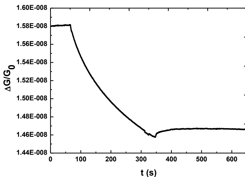
Figure 3.23: Response for 45 min OLA/WS 2 based sensor exposed to 1024 ppm of ammonia.
