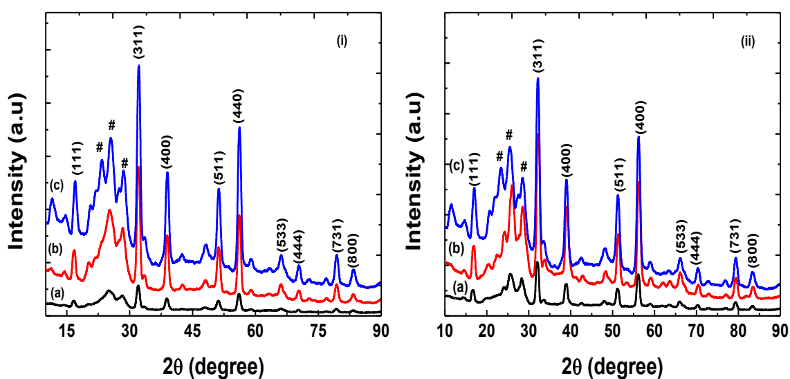
Figure 4.33: XRD patterns of (i) ODA/ \beta -In 2 S 3 at (a) 60 min, (b) 90 min, and (c) 150 min; (ii) ODA/1-DDT_ \beta -In 2 S 3 at (a) 60 min, (b) 90 min and (c) 150 min. The reflections marked with # represent ODA.
