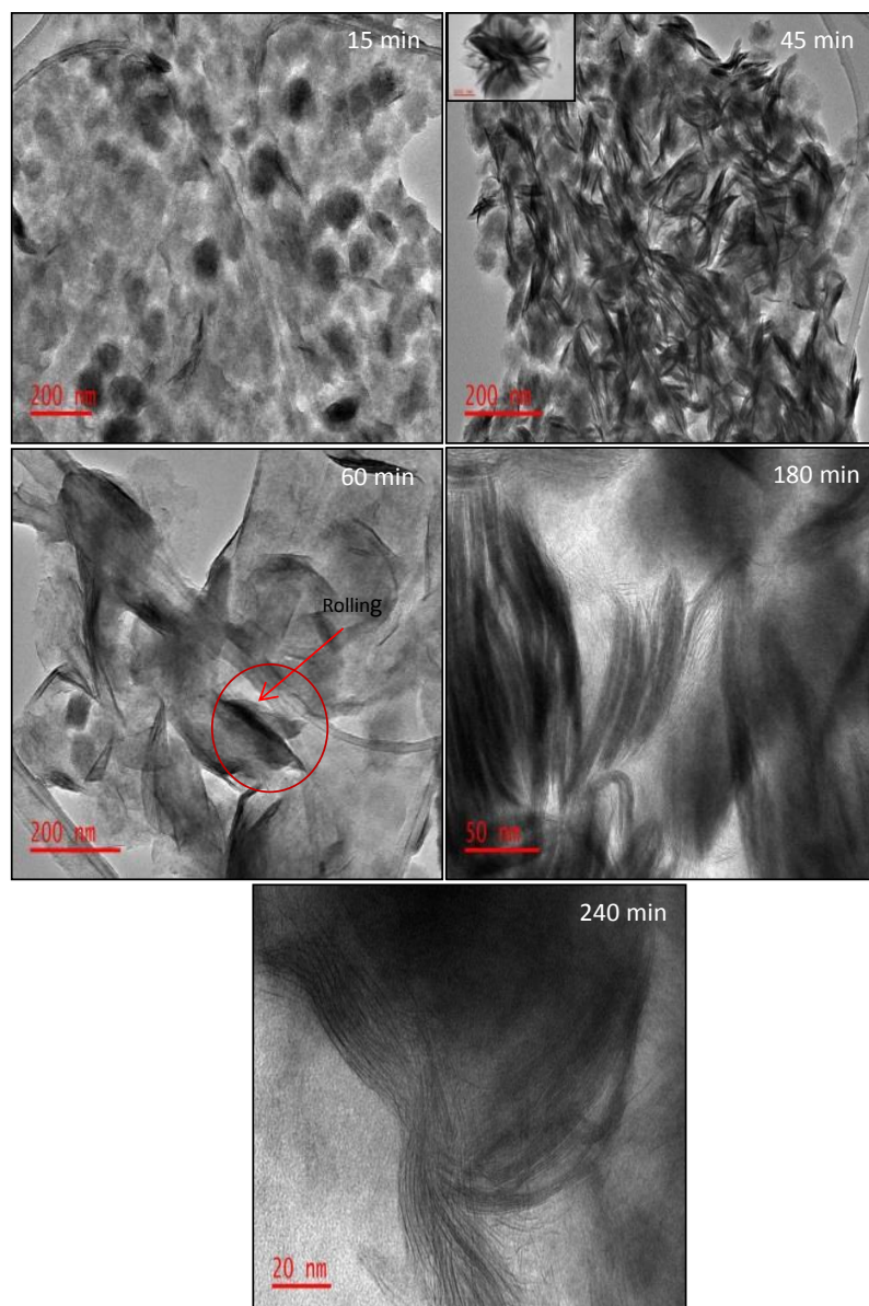
Figure 3.9: TEM micrographs of OLA/WS 2 nanostructures synthesized at different reaction times.
