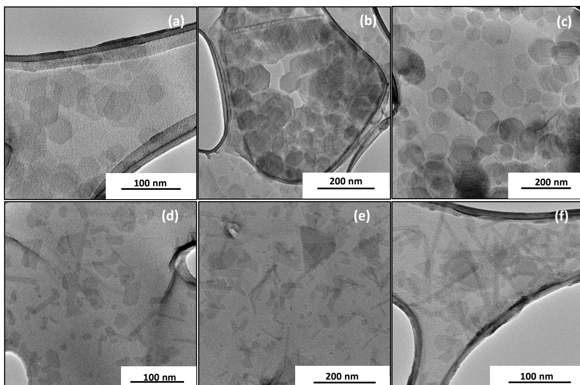
Figure 4.17: The TEM images of \beta - \text{In}_2\text{S}_3 nanostructures in: OLA_0.2 mL of 1-DDT at (a) 60 min, (b) 90 min, and (c) 150 min; OLA_0.4 mL of 1-DDT at (d) 60 min, (e) 90 min, and (f) 150 min in the 1:1 (In:S) reaction system.
