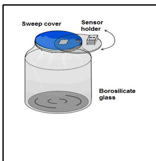
Figure 3.39: Schematic representation of the gas chamber with a sweep cover used under humid conditions.
