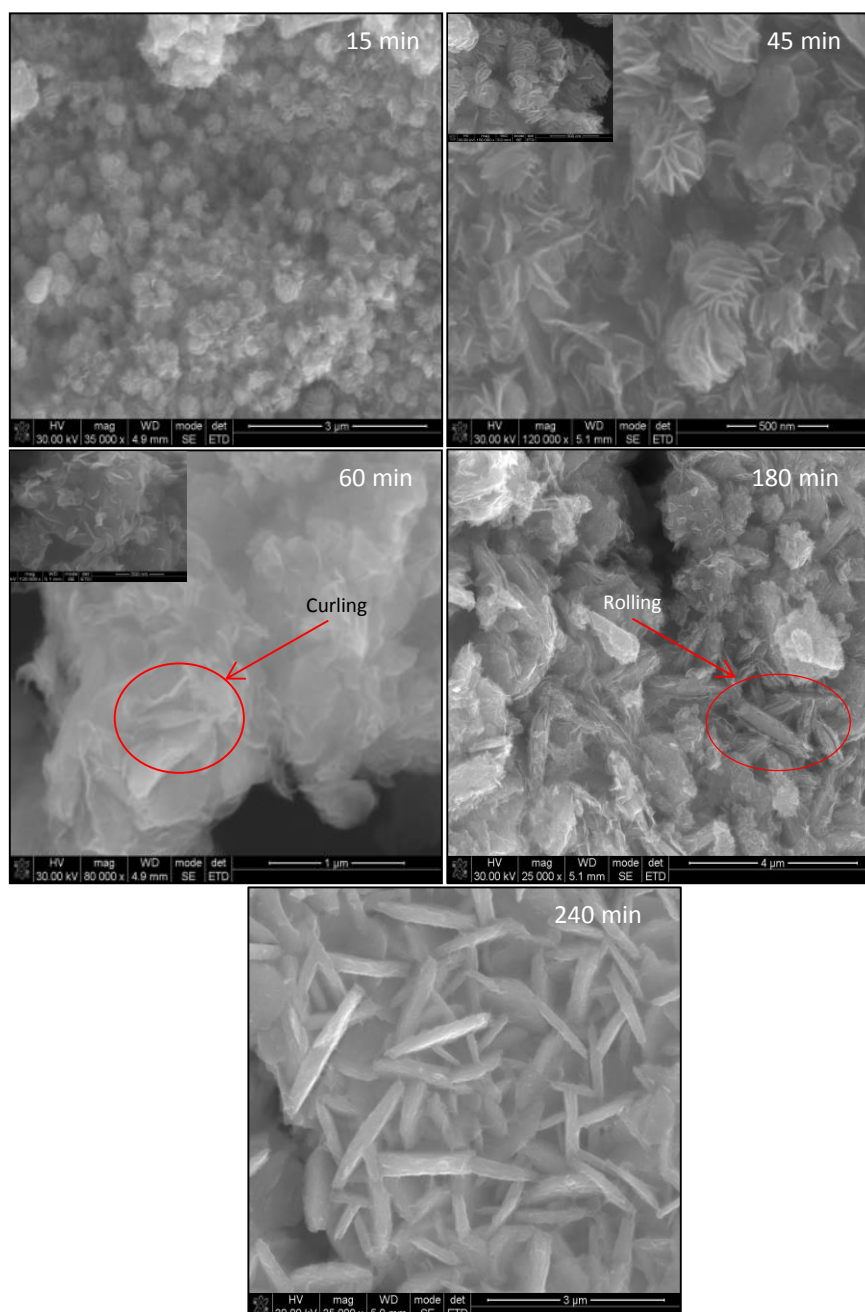
Figure 3.8: SEM images of OLA/ \text{WS}_2 synthesized at different reaction times.
