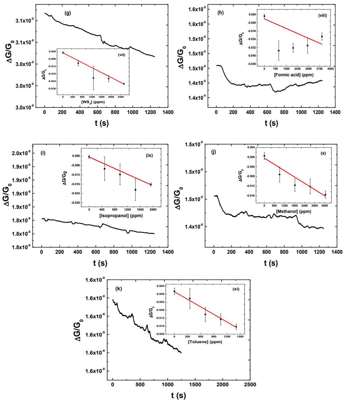
Figure 3.31: (a-k) Relative conductance of OLA/WS 2 sensors (180 min) vs time for NH 3 and several VOCs. Corresponding relative conductance vs concentration for each analyte (i-xi) [inset].
