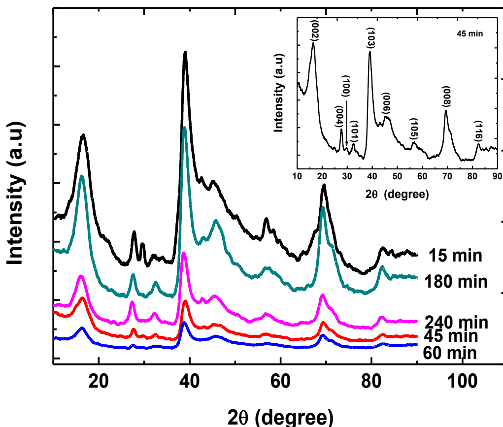
Figure 3.11: XRD patterns of OLA/WS 2 nanostructures synthesized at different reaction times. Insert shows the labelled peaks of the diffraction pattern of the 45 min sample.
