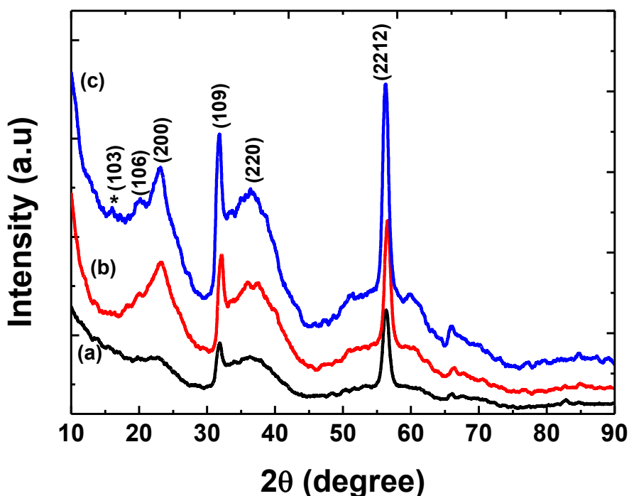
Figure 4.8: XRD patterns of OLA/ \beta - \text{In}_2\text{S}_3 nanostructures synthesized for (a) 60 min, (b) 120 min, and (c) 150 min in the 1:1.5 (In:S) reaction system.
