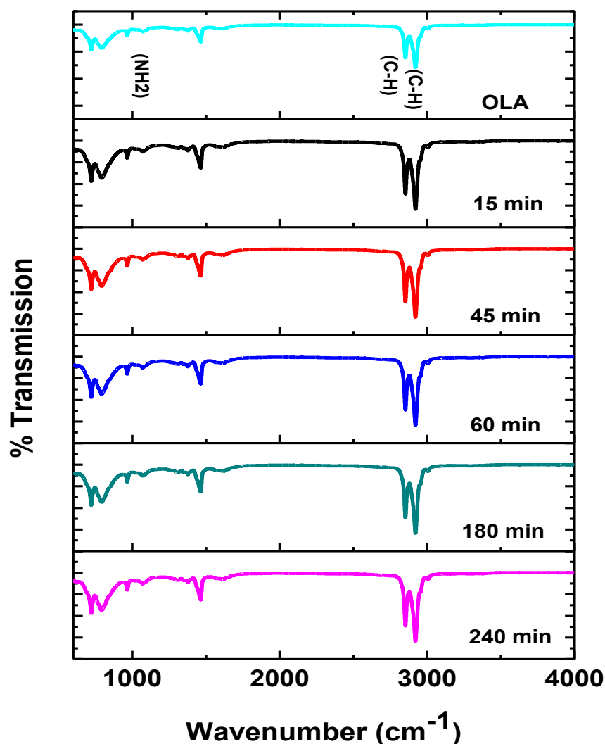
Figure 3.20: FTIR spectra of pure OLA and OLA/ \text{WS}_2 nanostructures synthesized at different reaction times.
