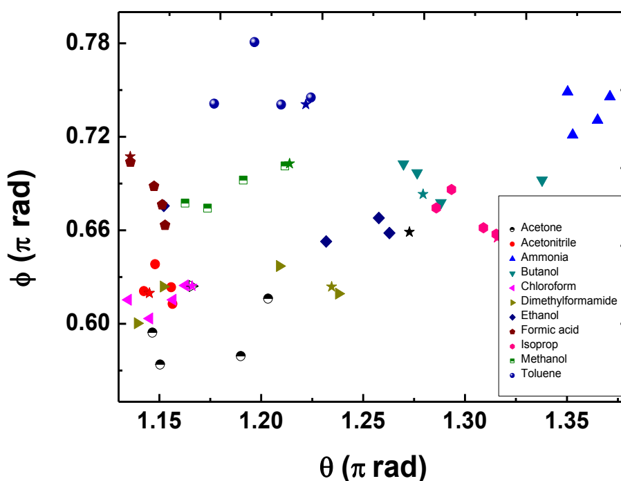
Figure 3.33: Bidimensional plot showing the separation between \text{NH}_3 and the various VOCs using an array of three OLA/ \text{WS}_2 chemiresistive sensors (15, 45 and 60 min) at different concentrations.
