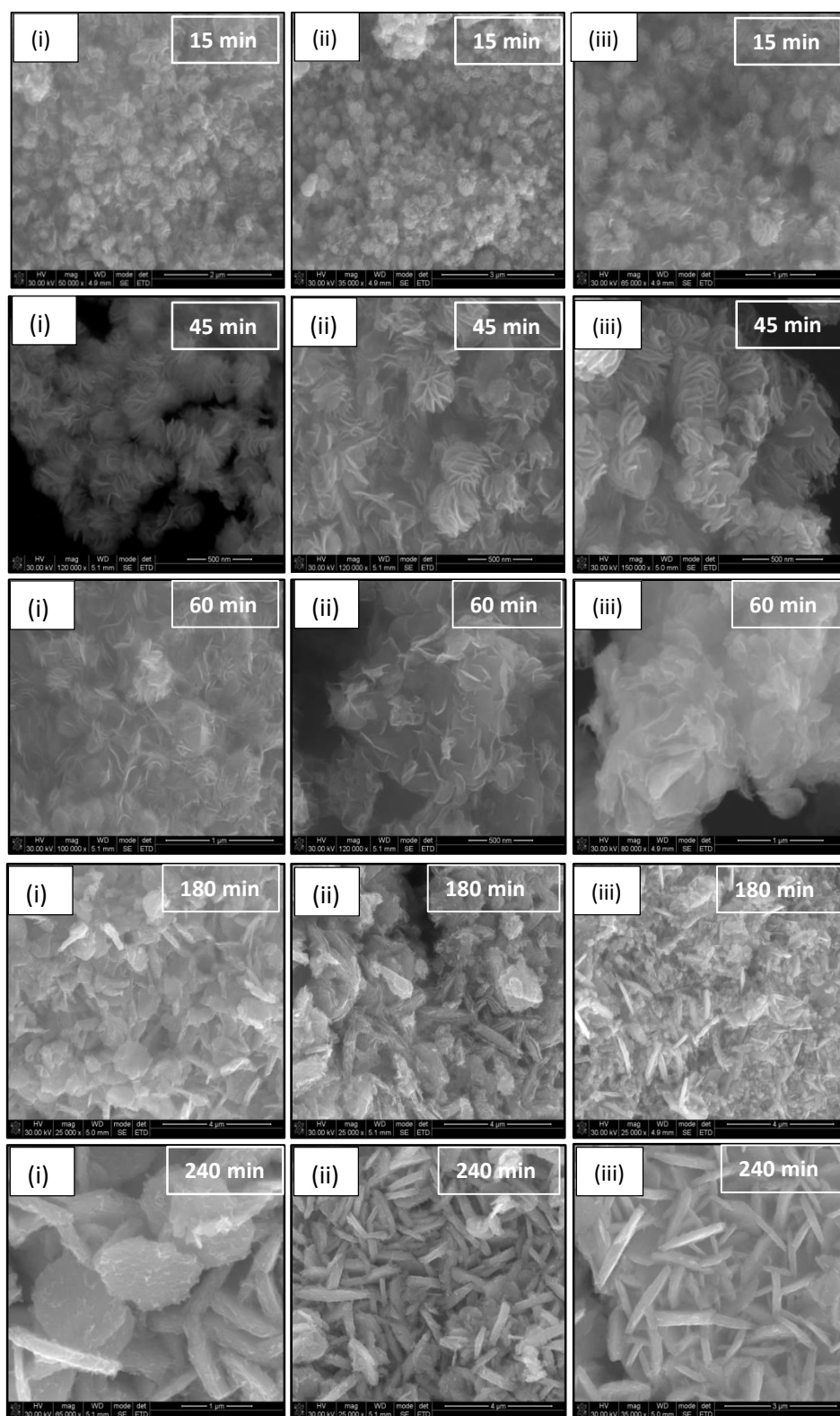
Figure 3.40: SEM micrographs of OLA/WS 2 nanostructures at 15, 45, 60, 180 and 240 min.
