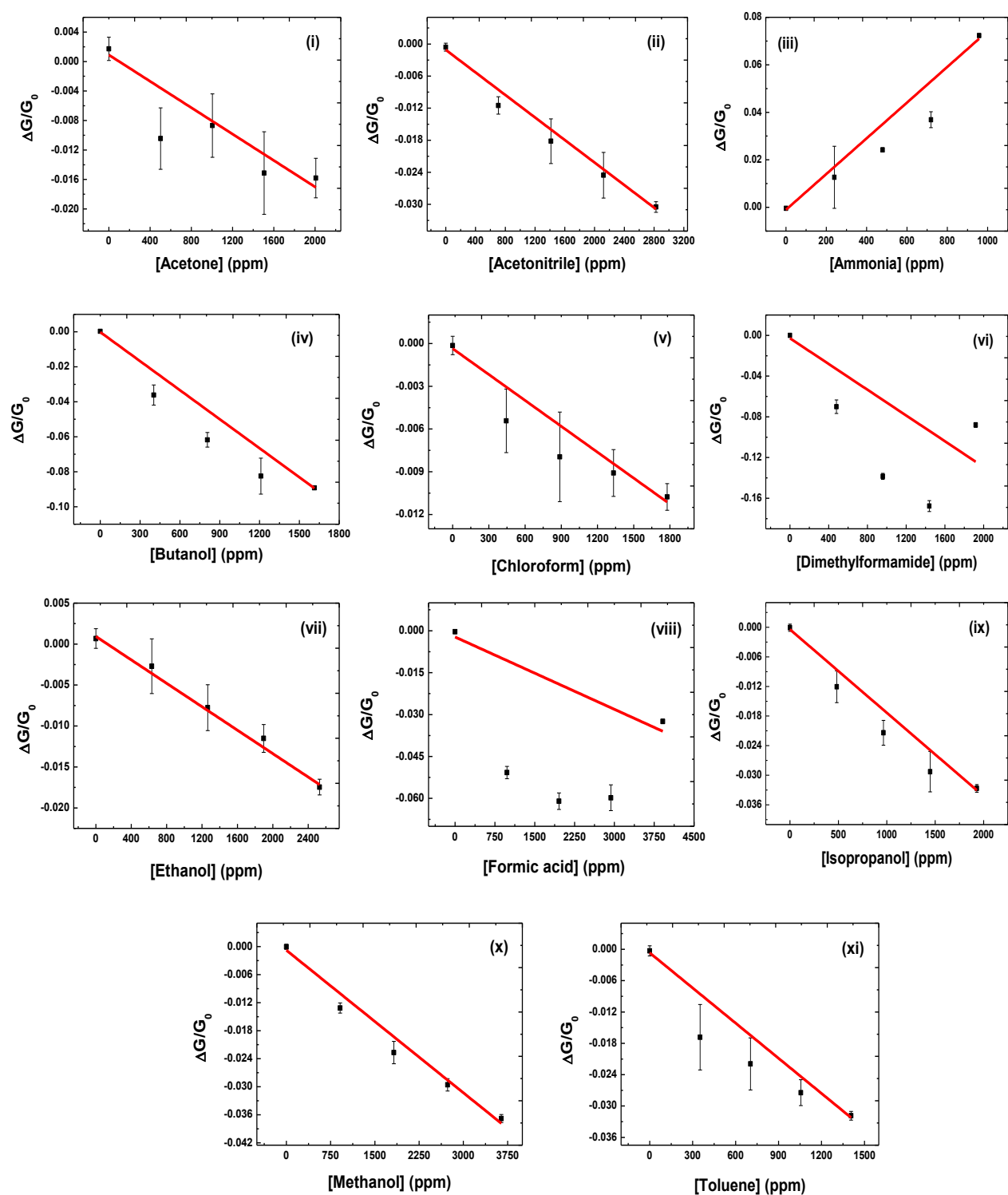
Figure 3.47: Response curves of OLA/WS 2 nanostructures (240 min).
