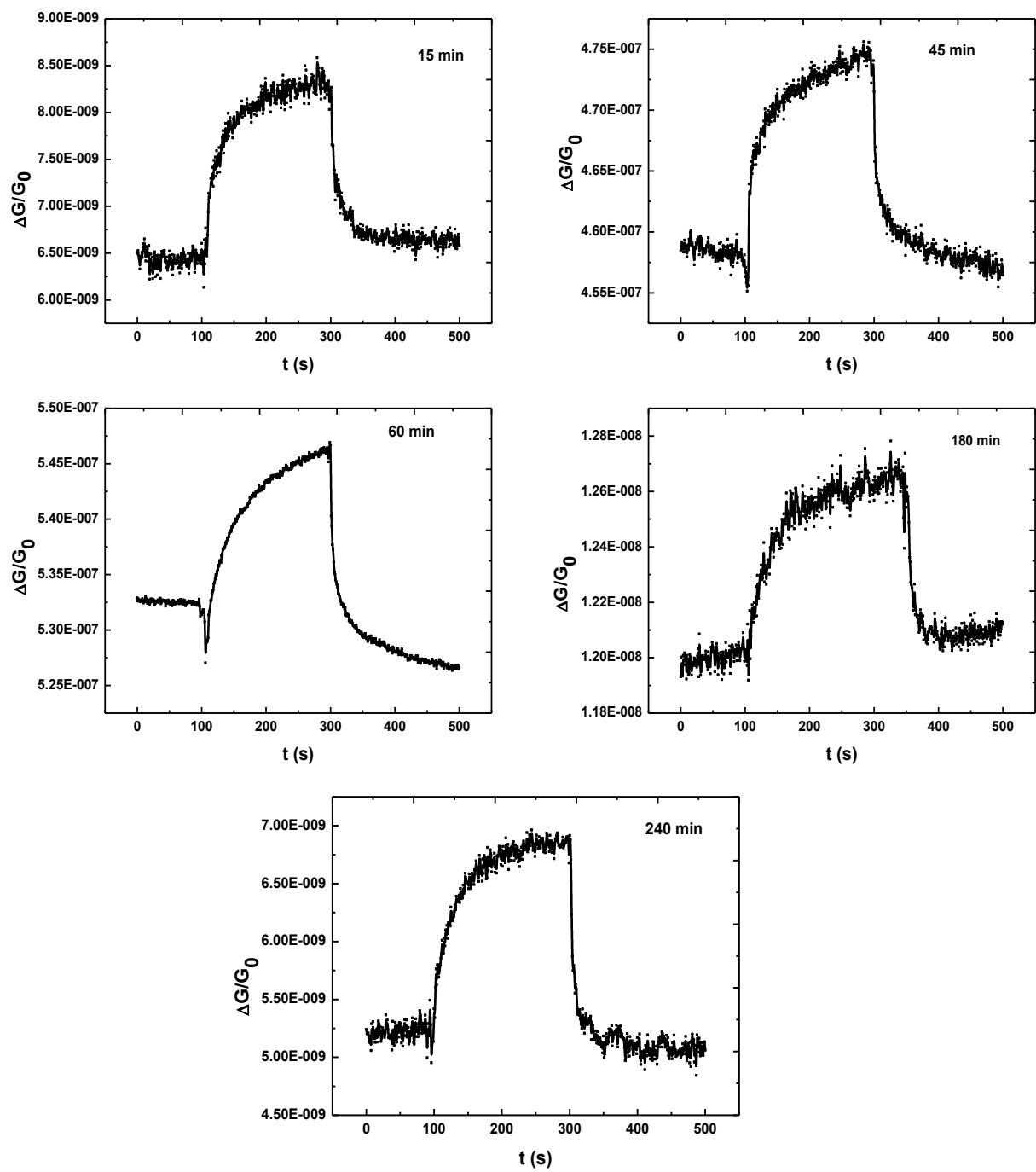
Figure 3.24: Response for OLA/WS 2 based sensors exposed to 240 ppm of ammonia.
