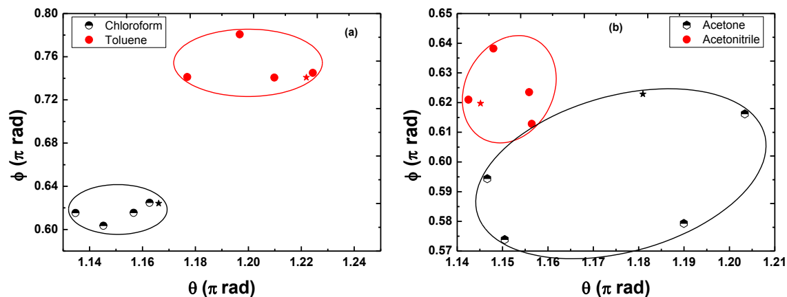
Figure 3.35: Discrimination between (a) non-polar solvents; (b) polar aprotic.
