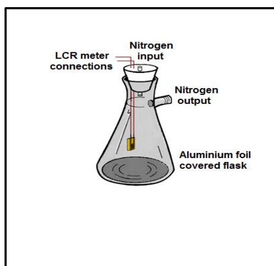
Figure 3.25: Schematic representation of the gas chamber used in sensor measurements.
