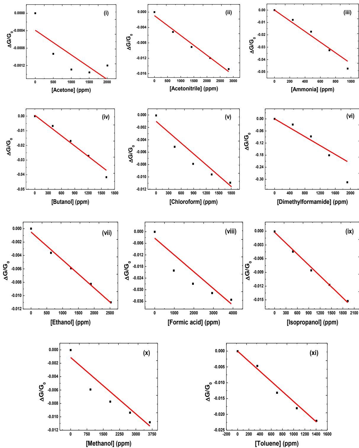
Figure 3.43: Response curves of OLA/WS 2 nanostructures (15 min).
