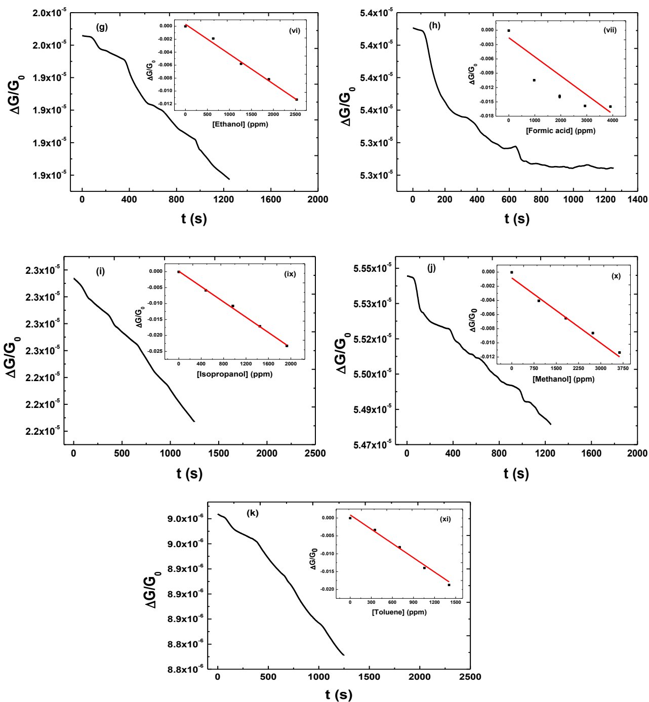
Figure 3.29: (a-k) Relative conductance of OLA/WS 2 sensors (45 min) vs time for NH 3 and several VOCs. Corresponding relative conductance vs concentration for each analyte (i-xi) [inset].
