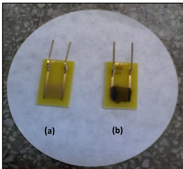
Figure 3.5: IDEs before (a) and after (b) deposition of OLA/WS 2 nanostructure film respectively.
