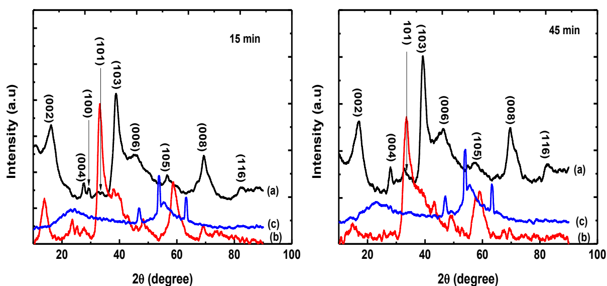
Figure 3.57: XRD patterns of WS 2 nanostructures synthesized at 15 and 45 min: (a) OLA/WS 2 before annealing; (b) OLA/WS 2 after annealing and (c) EDT/WS 2 after annealing. The annealing was performed for 3 h at 200 °C.
