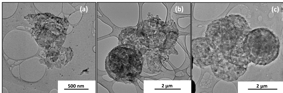
Figure 4.19: TEM images of 1-DDT/ \beta - \text{In}_2\text{S}_3 nanostructures synthesized for (a) 60 min, (b) 90 min, and (c) 150 min in the 1:1 (In:S) reaction system.
