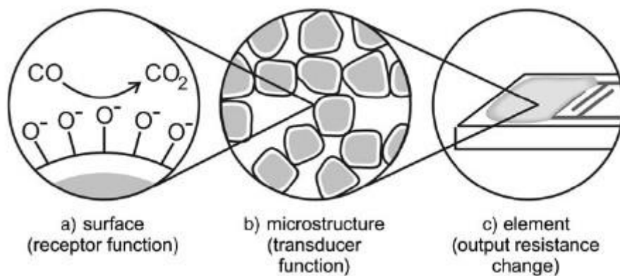
Figure 2.12: Receptor and transducer function of a semiconductor gas sensor: a) surface, providing the receptor function, b) microstructure of the sensing layer, providing the transducer function, and c) element, enabling the detection of the change in output resistance of the sensing layer, here deposited on an interdigital microelectrode [94].
