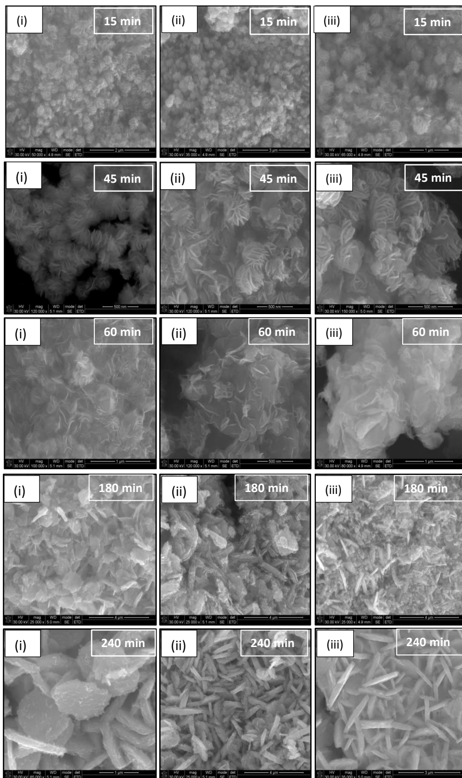
Figure 3.27: SEM micrographs of OLA/WS 2 nanostructures at 15, 45, 60, 180 and 240 min.
