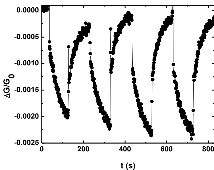
Figure 4.15: Response of \beta -In 2 S 3 sensor to successive introductions of formaldehyde vapour over time.
