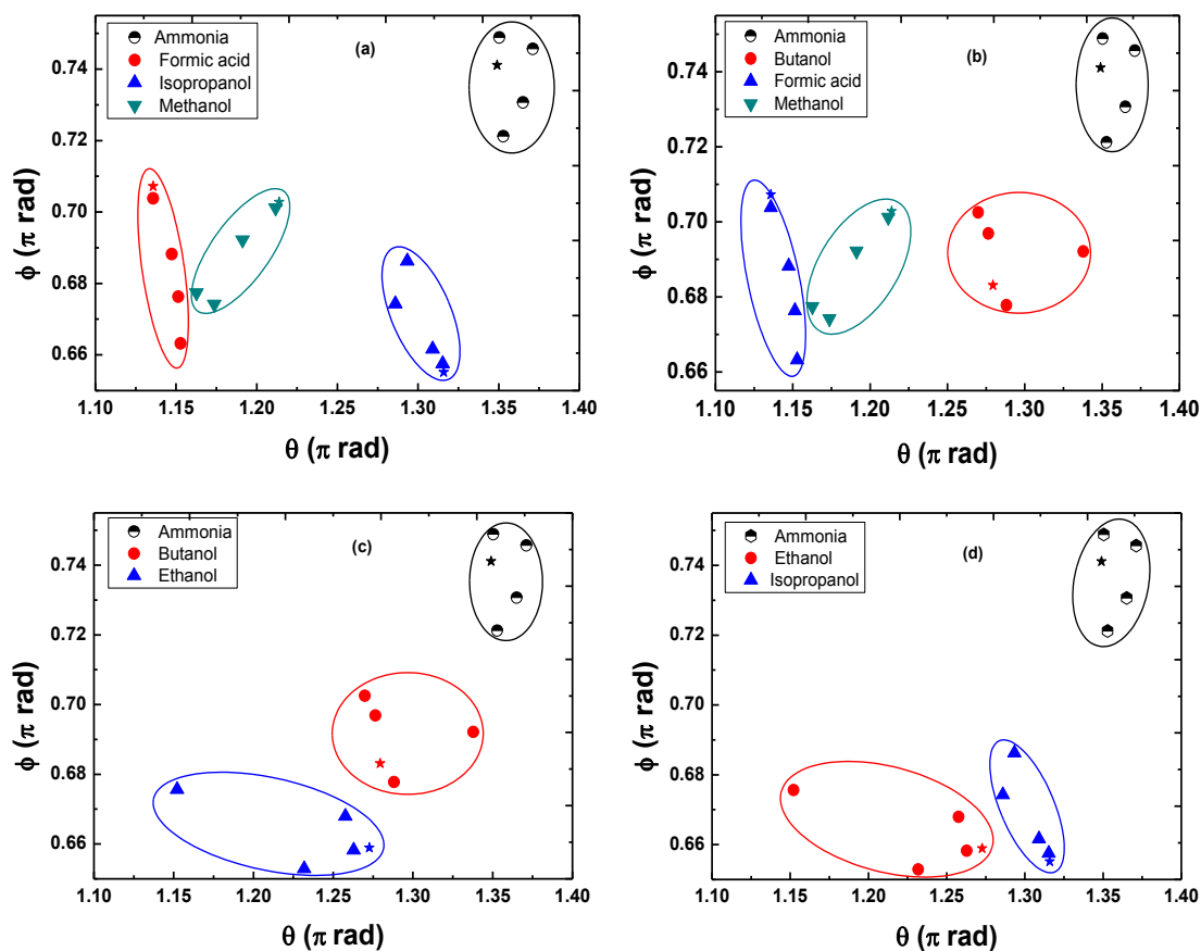
Figure 3.36: Discrimination between ammonia and other polar protic solvents.
