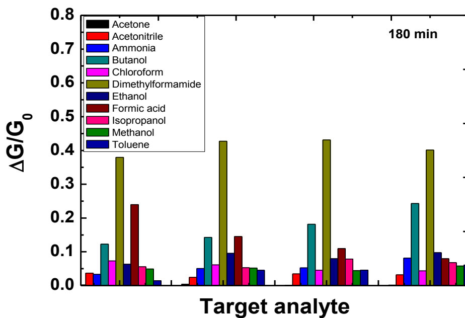
Figure 3.51: Selectivity tests of the OLA/WS 2 sensor (180 min) at 1.5, 3.0, 4.5 and 6.0 μL of NH 3 and various VOCs.
