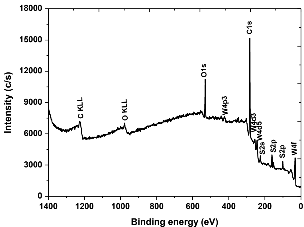
Figure 3.41: XPS survey spectrum of OLA/WS 2 nanostructures (45 min).
