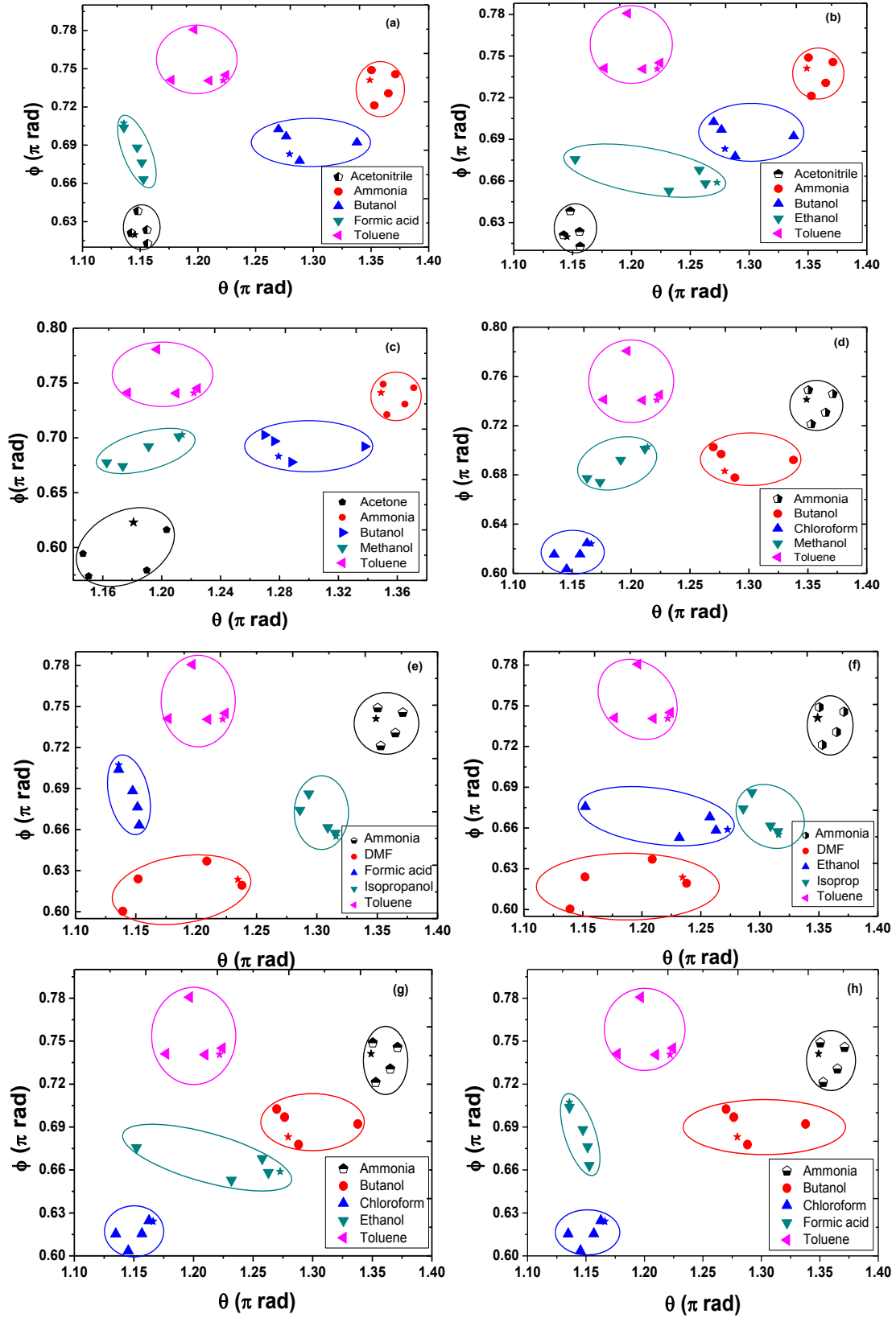
Figure 3.34: TA results differentiating \text{NH}_3 from polar and non-polar VOCs at different concentrations.
