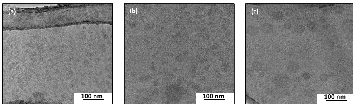
Figure 4.7: The TEM images of OLA/ \beta - \text{In}_2\text{S}_3 nanostructures for (a) 60 min, (b) 120 min, and (c) 150 min in 1:1.5 (In:S) reaction system.
