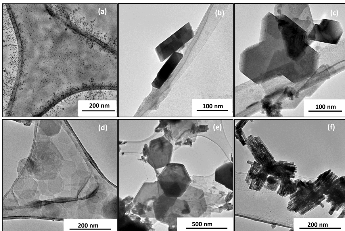
Figure 4.31: TEM images of ODA/ \beta -In 2 S 3 at (a) 60 min, (b) 90 min, and (c) 150 min; ODA/1-DDT_ \beta -In 2 S 3 (d) 60 min, (b) 90 min and (f) 150 min.
