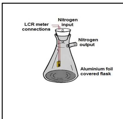
Figure 3.38: Schematic representation of the gas chambers used in sensor measurements.
