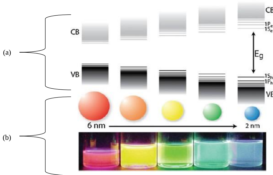
Figure 2.3: Illustration of the quantum confinement effects on: (a) the band gap and (b) fluorescence of dispersions of CdSe QDs with different sizes under excitation with a UV-lamp in the dark [12].
