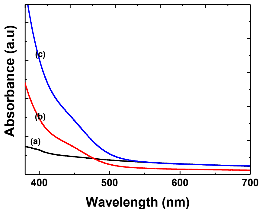
Figure 4.9: UV-vis spectra of OLA/ \beta - \text{In}_2\text{S}_3 nanostructures synthesized for (a) 60 min, (b) 120 min, and (c) 150 min in the 1:1.5 (In:S) reaction system.
