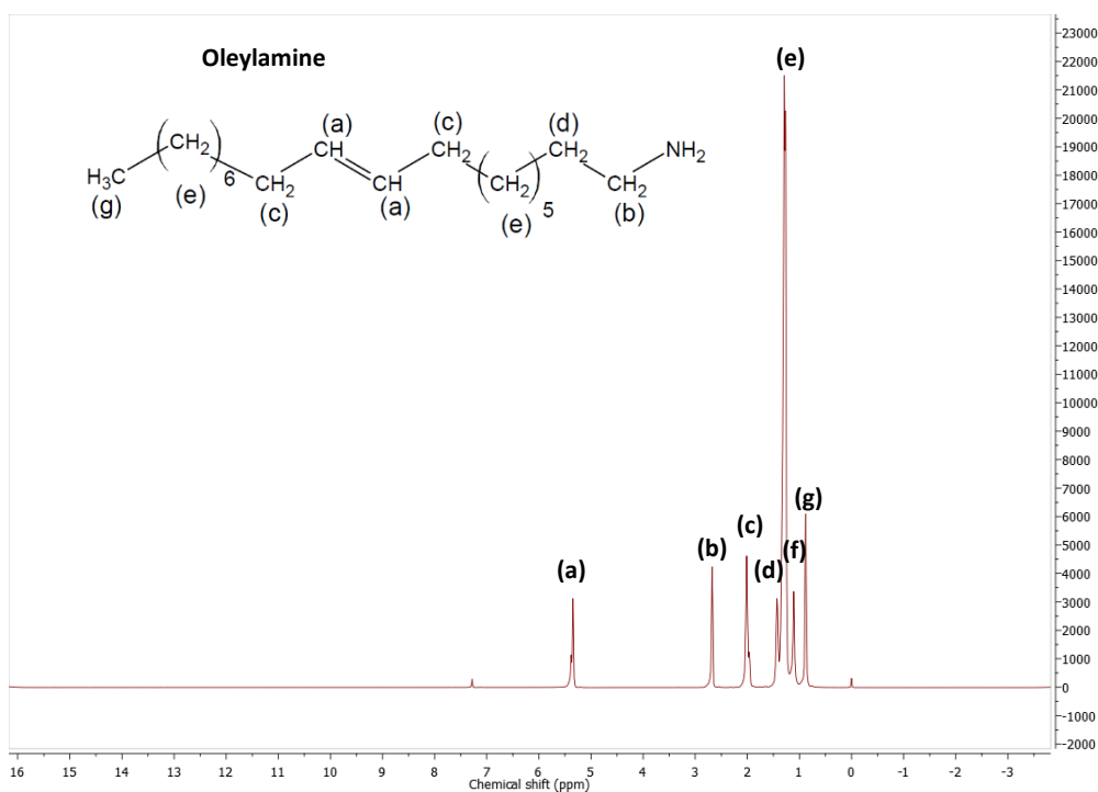
Figure 4.23: Solution 1 H NMR spectra obtained on CDCl 3 dispersions of pure OLA.
