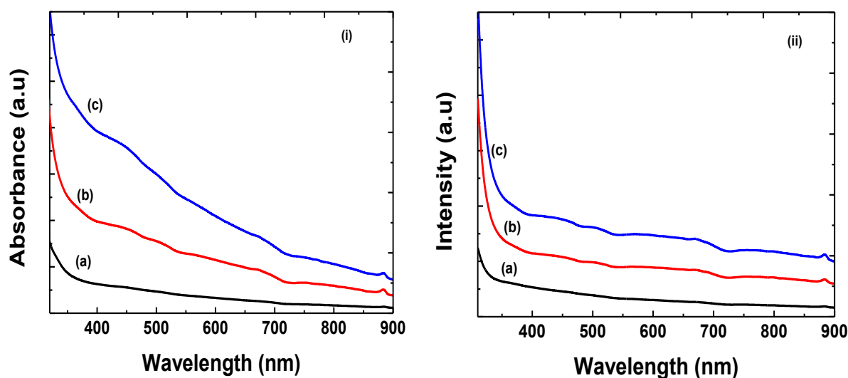
Figure 4.36: UV-vis spectra of (i) ODA/ \beta -In 2 S 3 at (a) 60 min, (b) 90 min, and (c) 150 min; (ii) ODA/1-DDT_ \beta -In 2 S 3 at (a) 60 min, (b) 90 min, and (c) 150 min.
