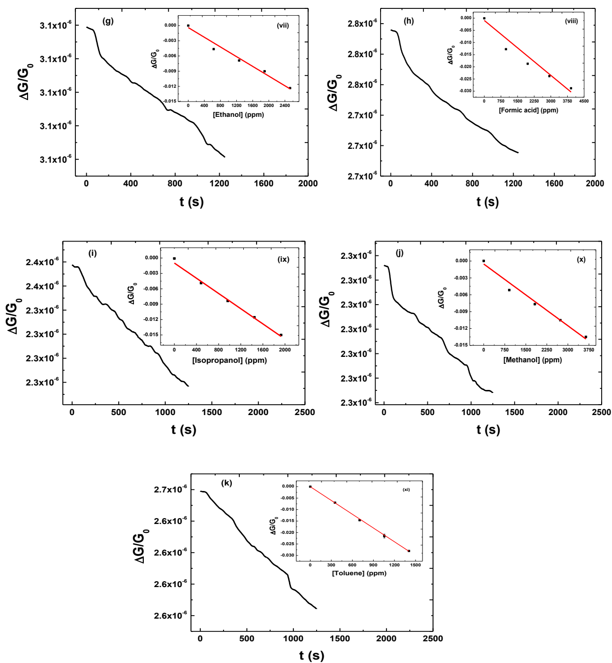
Figure 3.30: (a-k) Relative conductance of OLA/WS 2 sensors (60 min) vs time for NH 3 and several VOCs. Corresponding relative conductance vs concentration for each analyte (i-xi) [inset].
