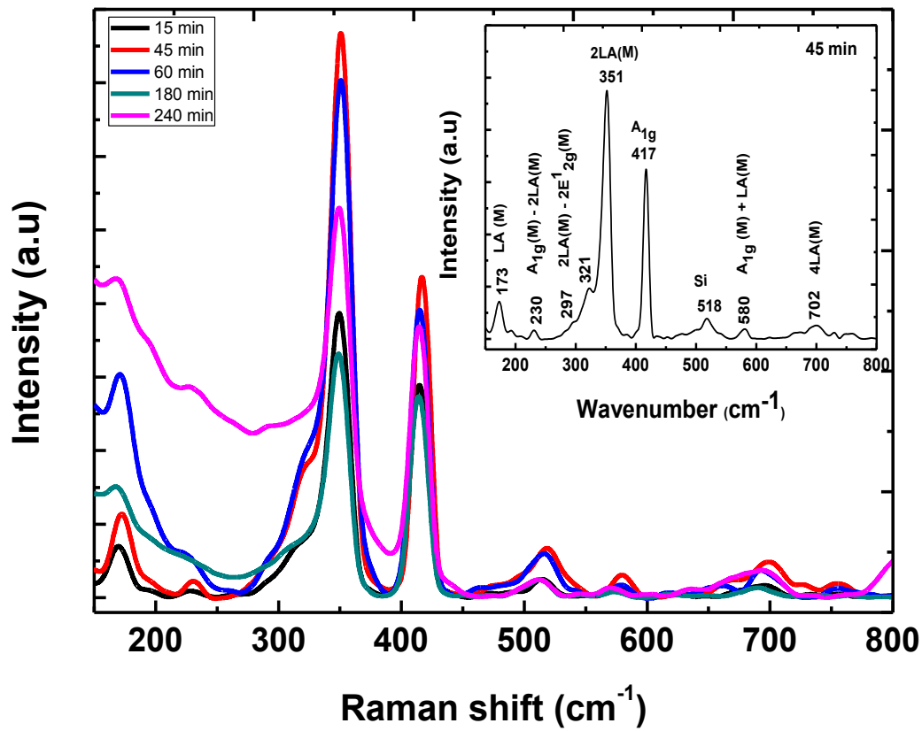
Figure 3.12: Raman spectra of OLA/WS 2 nanostructures from the different reaction times. Inset shows the first and second order peaks of the spectrum from the 45 min sample.
