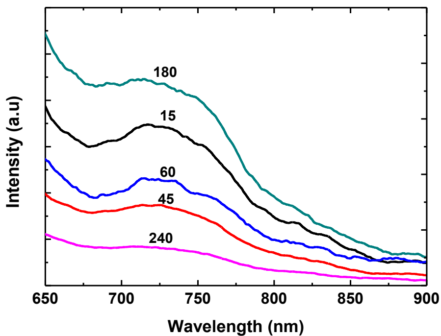
Figure 3.18: PL spectra of WS 2 nanostructures from the different reaction times.
