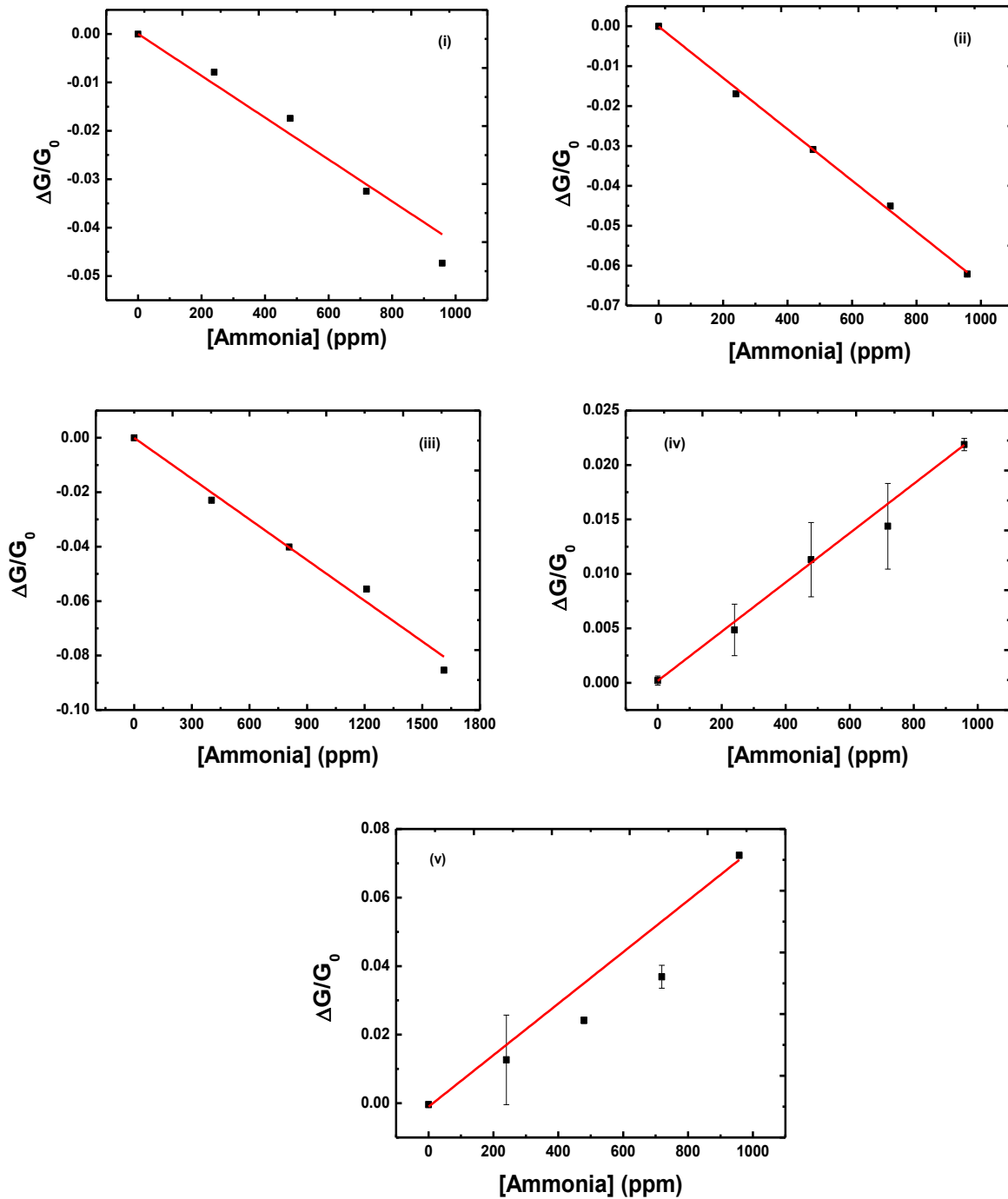
Figure 3.22: Sensitivities of the different reaction times towards \text{NH}_3 from (i) to (v).
