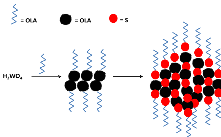
Figure 3.7: Passivation of WS 2 nanostructures by OLA.
