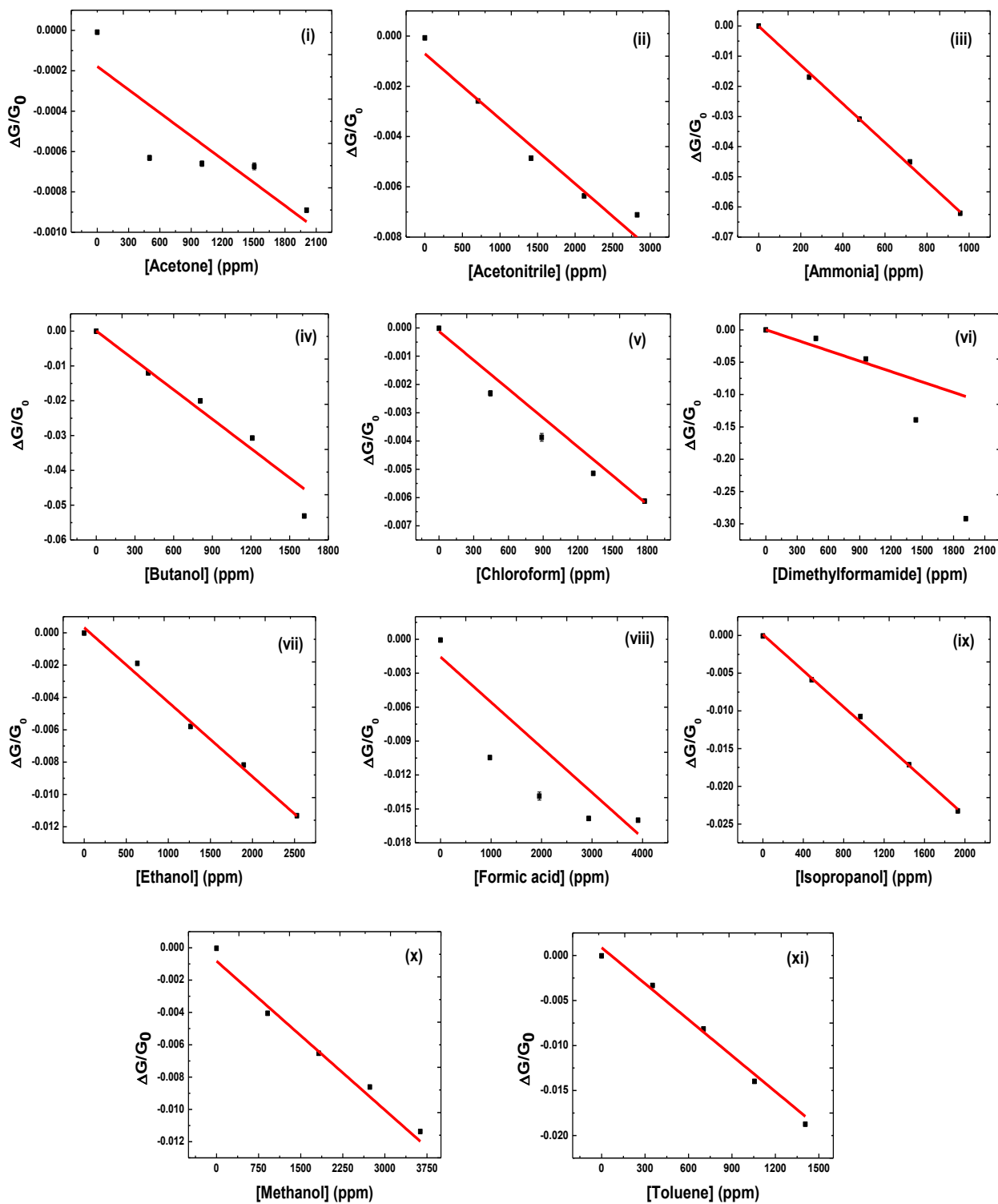
Figure 3.44: Response curves of OLA/WS 2 nanostructures (45 min).
