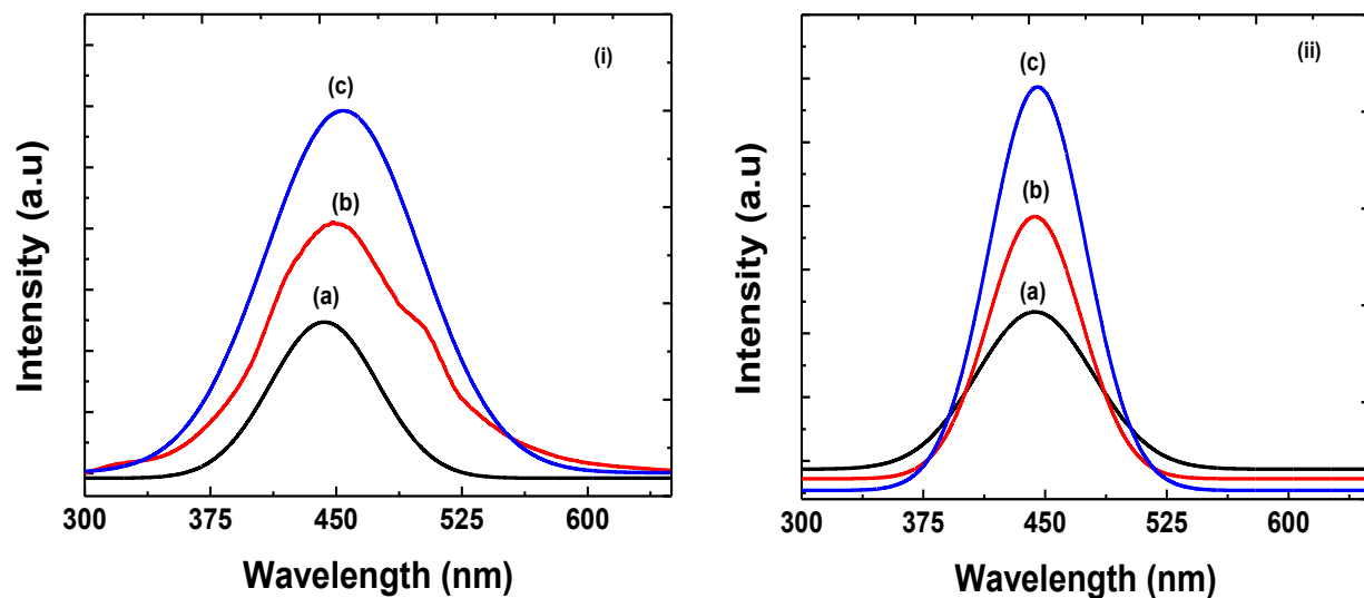
Figure 4.37: PL spectra of (i) ODA/ \beta - \text{In}_2\text{S}_3 at (a) 60 min, (b) 90 min, and (c) 150 min; (ii) ODA/1-DDT_ \beta - \text{In}_2\text{S}_3 at (a) 60 min, (b) 90 min, and (c) 150 min.
