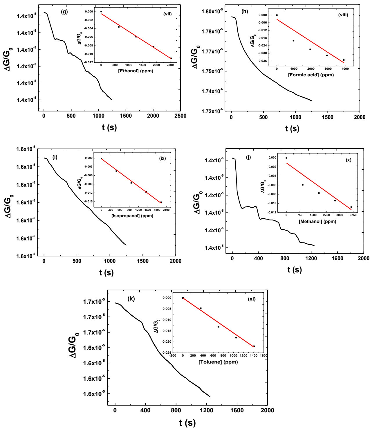
Figure 3.28 (a-k) Relative conductance of OLA/WS 2 sensors (15 min) vs time for \text{NH}_3 and several VOCs. Corresponding relative conductance vs concentration for each analyte (i-xi) [inset].
