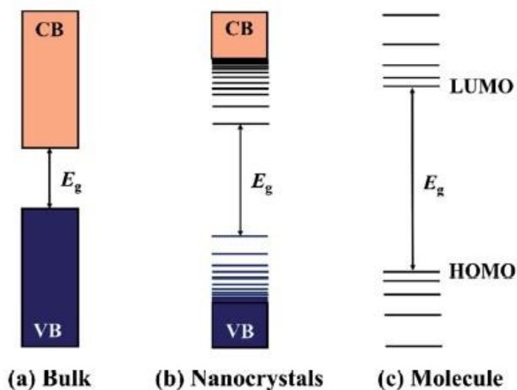
Figure 2.1: A depiction of the electronic energy states of: (a) bulk inorganic semiconductors, (b) inorganic semiconductor NCs, and (c) molecular semiconductors [3].
