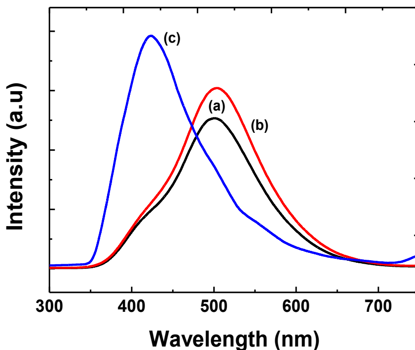
Figure 4.14: PL spectra of OLA/ \beta -In 2 S 3 nanostructures synthesized for (a) 60 min, (b) 120 min, and (c) 150 min in the 1:2 (In:S) reaction system.
