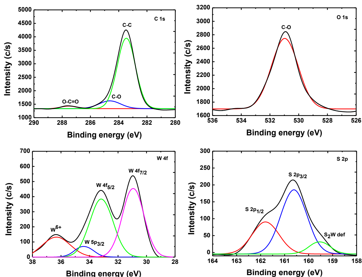
Figure 3.42: High resolution XPS spectrum of OLA/WS 2 nanostructures (45 min).
