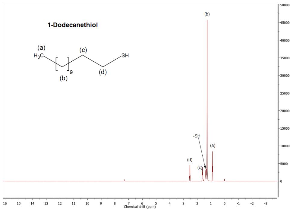
Figure 4.24: Solution 1 H NMR spectra obtained on CDCl 3 dispersions of pure 1-DDT.
