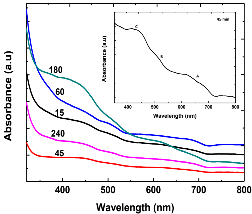
Figure 3.16: UV-vis spectra of OLA/ \text{WS}_2 nanostructures from the different reaction times. Insert shows the spectrum of the 45 min sample different peaks A, B and C.
