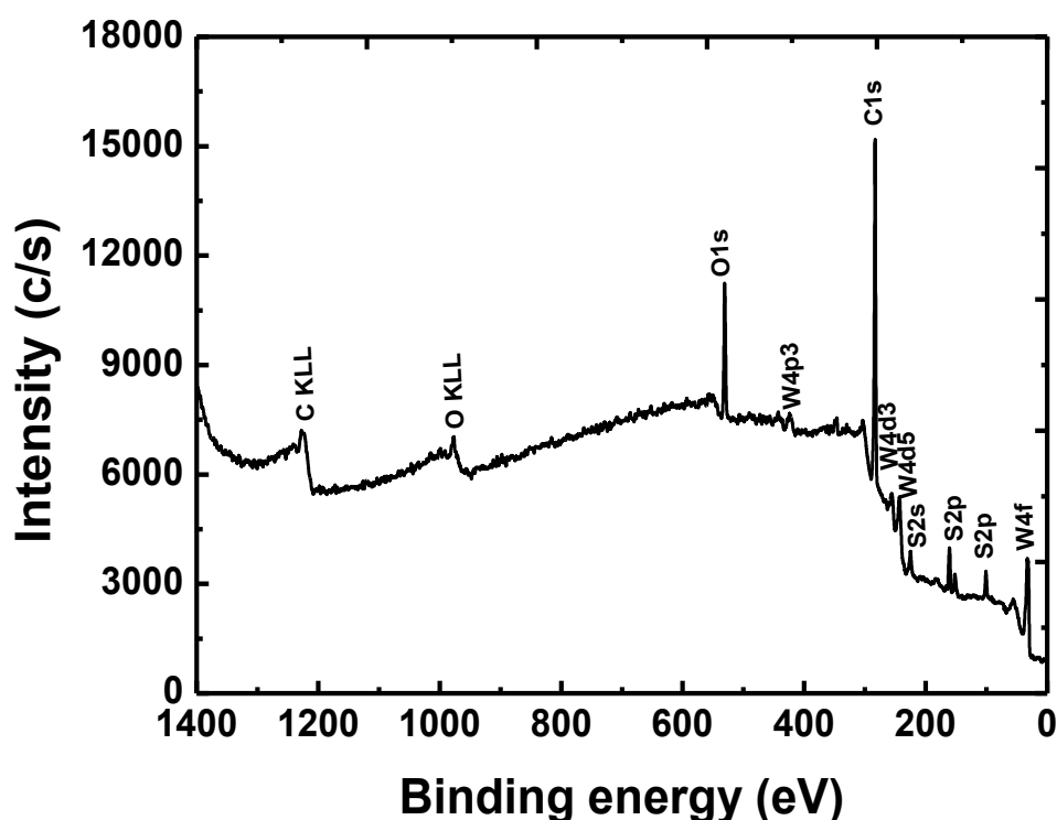
Figure 3.14: XPS survey spectrum of OLA/WS 2 nanostructures synthesized in 45 min.
