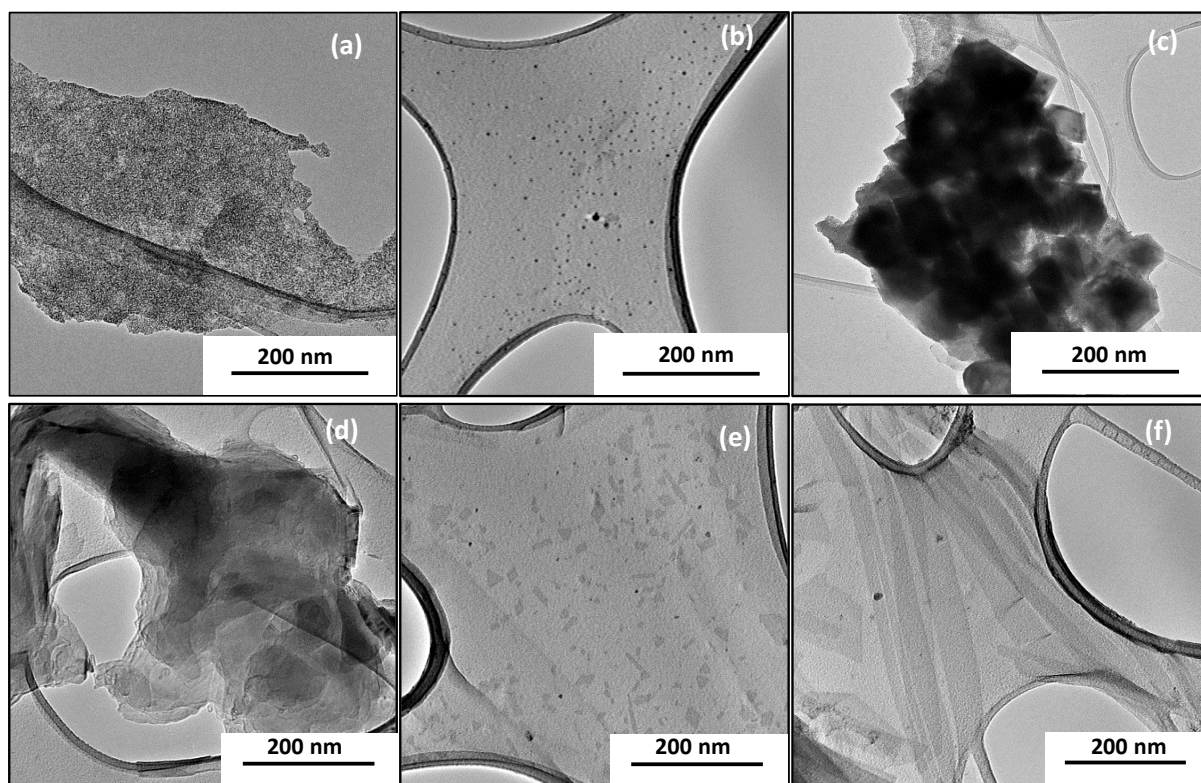
Figure 4.30: TEM images of HDA/ \beta -In 2 S 3 at (a) 60 min, (b) 90 min, and (c) 150 min; HDA/1-DDT_ \beta -In 2 S 3 at (d) 60 min, 90 min and (f) 150 min.
