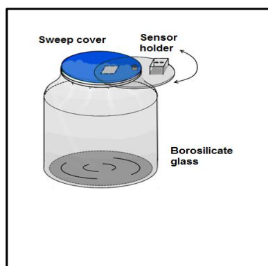
Figure 4.2: Schematic representation of the gas chamber (with a sweep cover).
