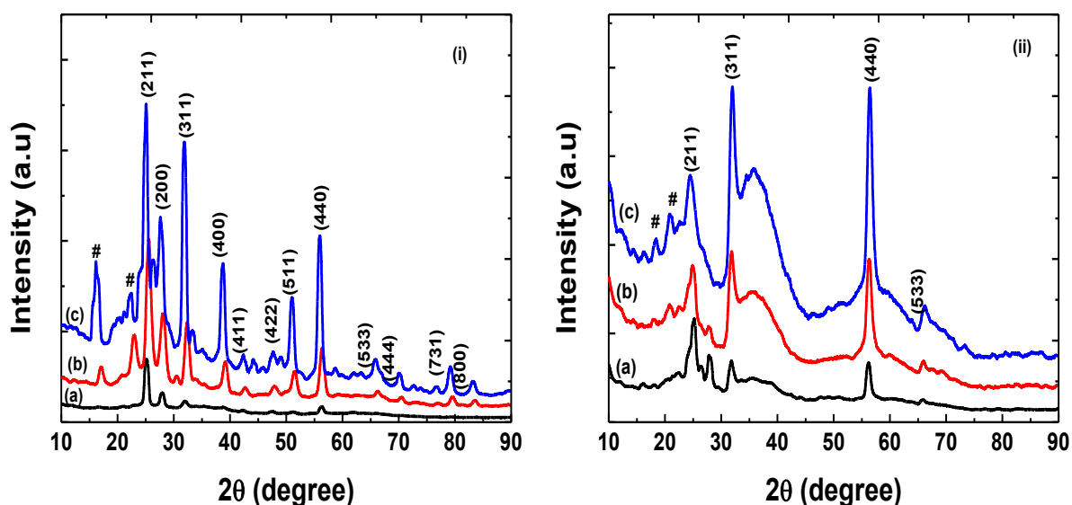
Figure 4.32: XRD patterns of (i) HDA/ \beta -In 2 S 3 at (a) 60 min, (b) 90 min, and (c) 150 min; (ii) HDA/1-DDT_ \beta -In 2 S 3 at (a) 60 min, (b) 90 min and (c) 150 min. The reflections marked with # represent InS.
