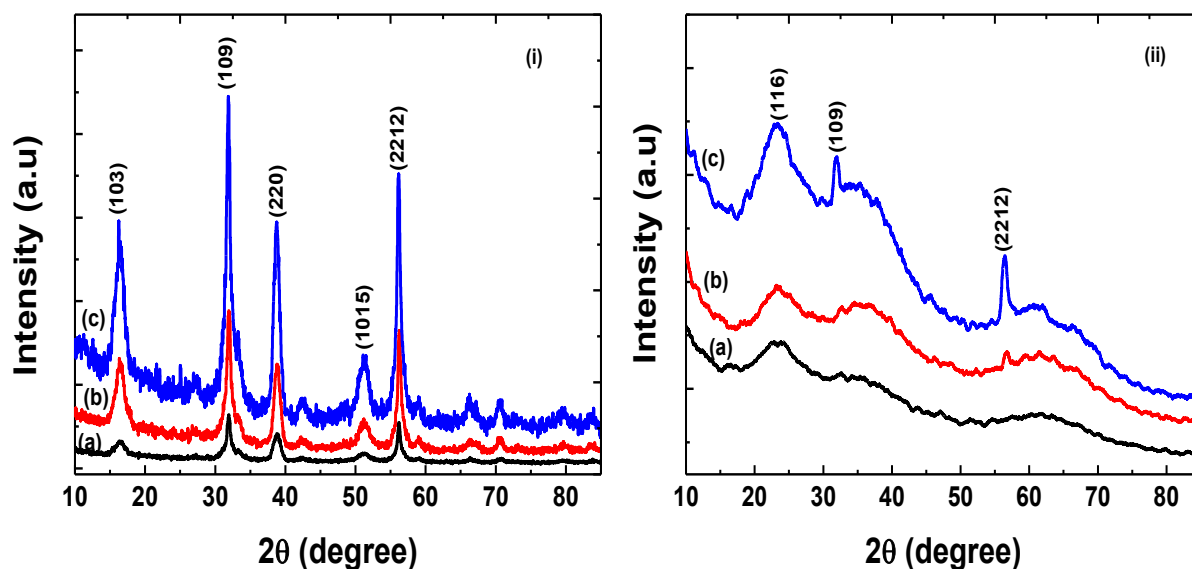
Figure 4.22: XRD patterns of (i) 1-DDT/ \beta - \text{In}_2\text{S}_3 nanostructures at (a) 60 min, (b) 90 min, and (c) 150 min; (ii) OLA/ \beta - \text{In}_2\text{S}_3 nanostructures at (a) 120 min, (b) 150 min, and (c) 180 min.
