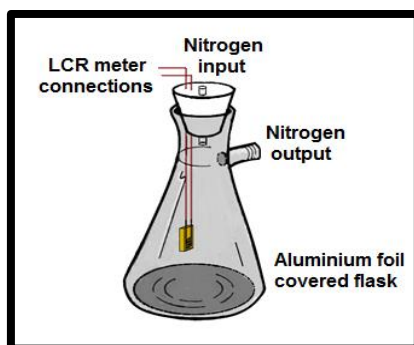
Figure 3.56: Schematic representation of the gas chambers used in sensor measurements.
