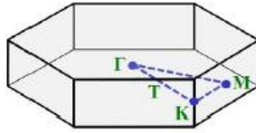
Figure 3.1: Brillouin zone for WS 2 monolayer [8].
