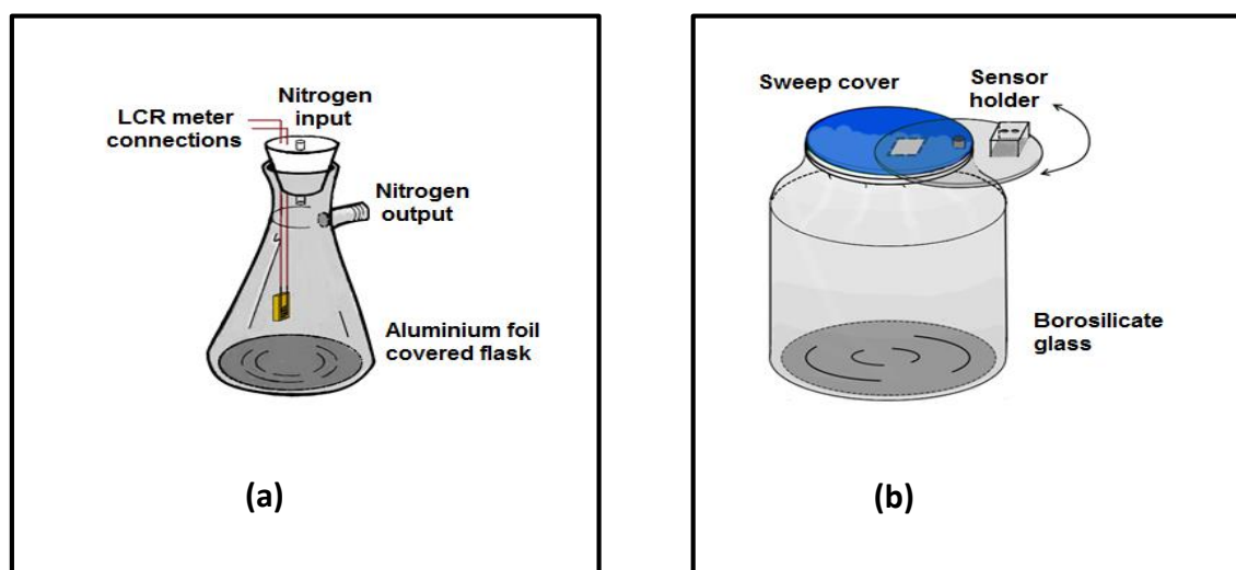
Figure 3.6: Schematic representation of gas chambers used in the gas sensing measurements: (a) the rubber stoppered filtering flask and (b) glass bottle with a sweep cover.
