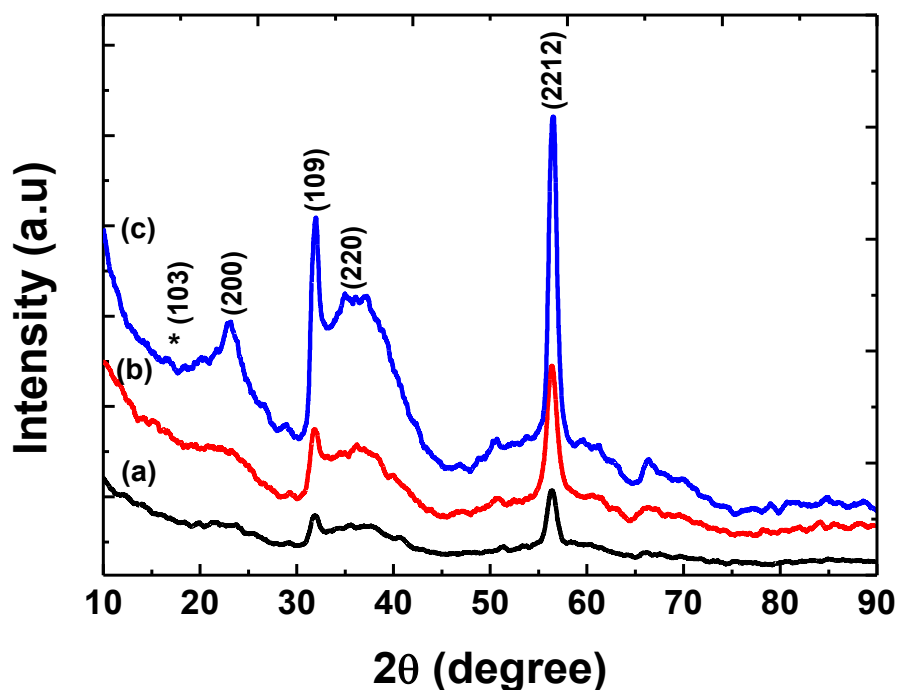
Figure 4.12: XRD patterns of OLA/ \beta - \text{In}_2\text{S}_3 nanostructures synthesized for (a) 60 min, (b) 120 min, and (c) 150 min in the 1:2 (In:S) reaction system.
