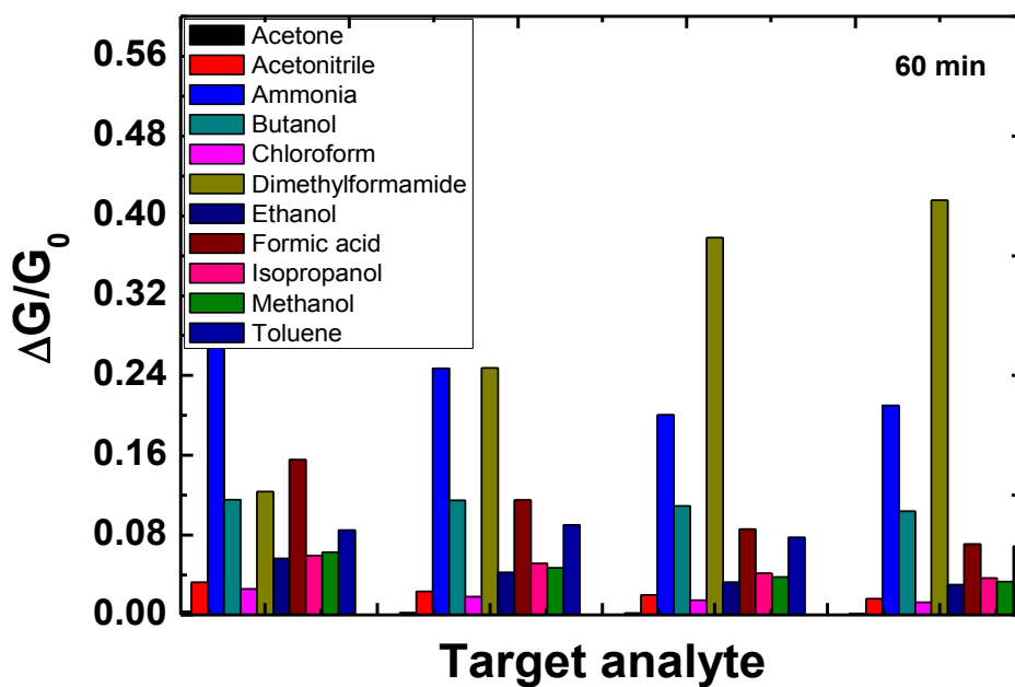
Figure 3.50: Selectivity tests of the OLA/WS 2 sensor (60 min) at 1.5, 3.0, 4.5 and 6.0 μL of NH 3 and various VOCs.
