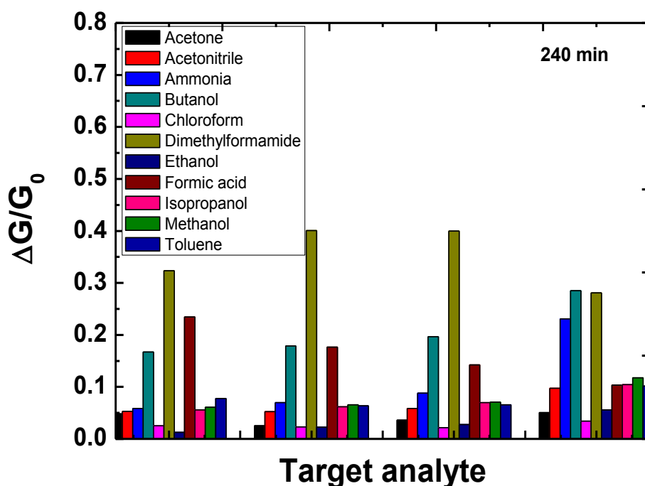
Figure 3.52: Selectivity tests of the OLA/WS 2 sensor (240 min) at 1.5, 3.0, 4.5 and 6.0 \mu\text{L} of NH 3 and various VOCs.
