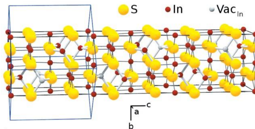
Figure 4.1: Structure model of \beta - \text{In}_2\text{S}_3 unit cell. The indium vacancies are marked as grey spheres. In the tetragonal \beta - \text{In}_2\text{S}_3 configuration, the vacancies are ordered on a 4_1 screw axis parallel to the c-axis of the crystal. In the \alpha - \text{In}_2\text{S}_3 configuration, the vacancies are randomly distributed over all tetrahedral indium sites. The edges of the unit cell of the tetragonal \beta - \text{In}_2\text{S}_3 structure (cubic \alpha - \text{In}_2\text{S}_3 ) structure are indicated by black (blue) lines [43].
