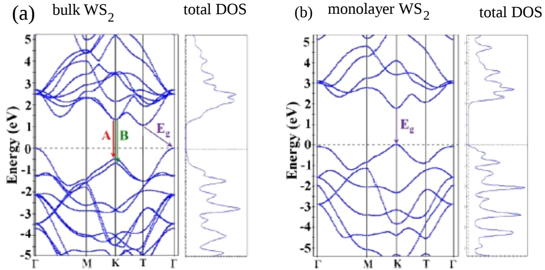
Figure 3.17: Electronic band structure (left) and total density of states (right) for (a) WS 2 bulk and (b) monolayer [8].
