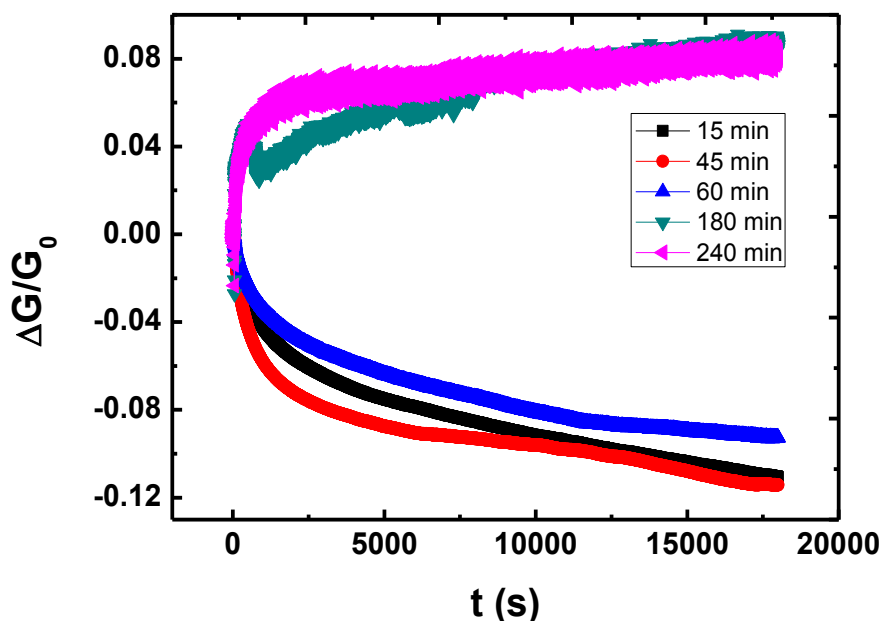
Figure 3.55: Response curves of OLA/WS 2 sensors (15, 45, 60, 180 and 240 min) towards at 240 ppm of NH 3 for five hours.
