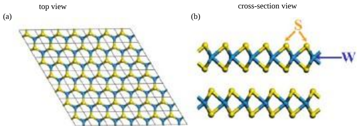
Figure 3.2: (a) top and (b) cross-section view of the WS 2 atomic structure [8].
