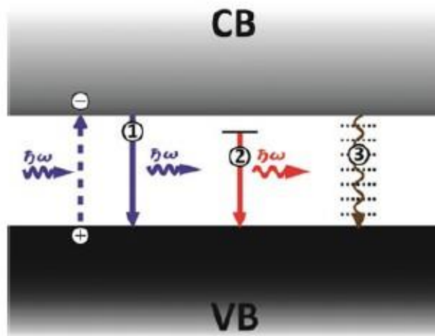
Figure 2.6: Possible exciton recombination pathways in semiconductors. (1) Radiative recombination, (2) defect assisted radiative recombination, and (3) non-radiative recombination [12].
