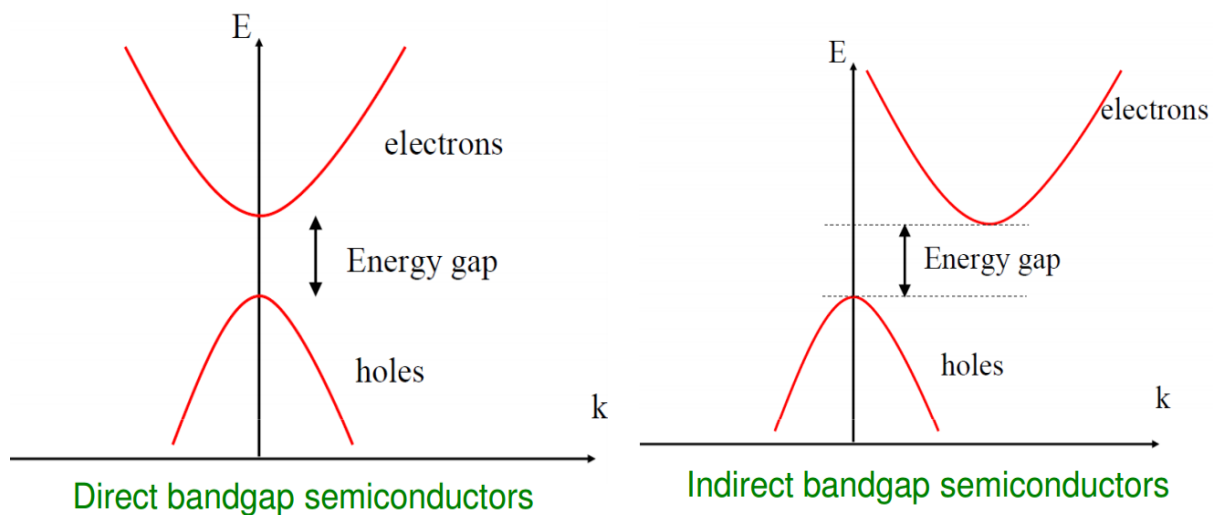
Figure 2.2: Schematic representation of (a) direct and (b) indirect electronic transitions [14].
