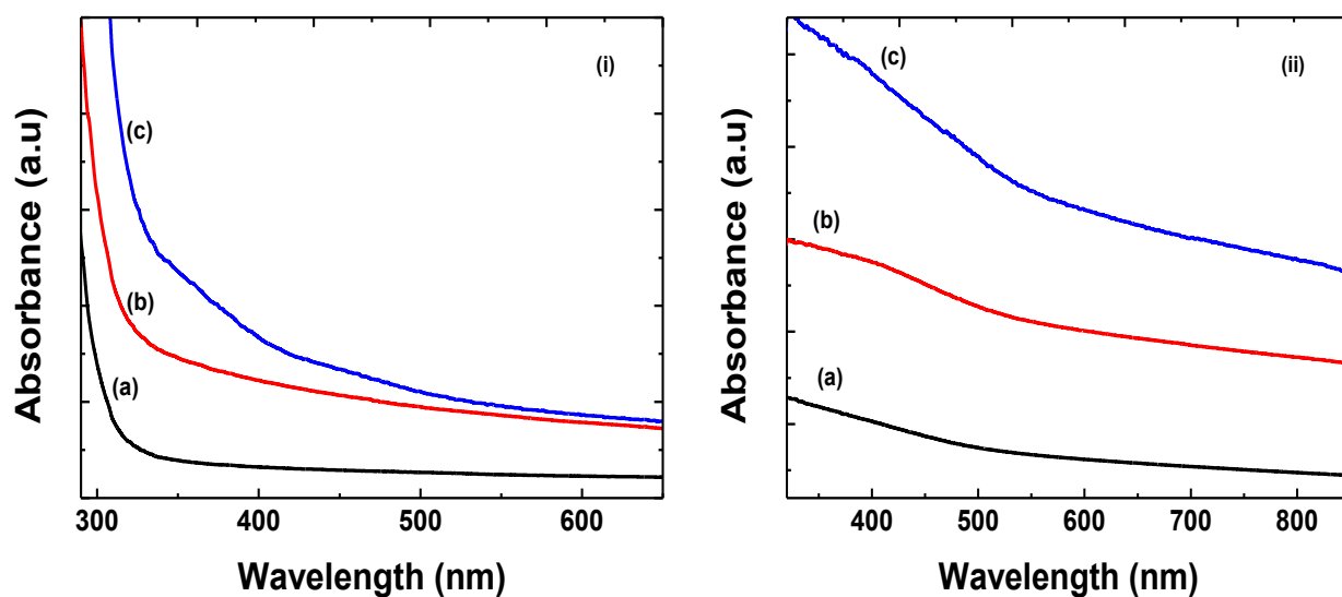
Figure 4.28: (i) UV-vis spectra of OLA/β-In 2 S 3 at (a) 120 min, (b) 150 min, and (c) 180 min with 1-DDT as sulphur source; (ii) 1-DDT/β-In 2 S 3 at (a) 60 min, (b) 90 min, and (c) 150 min.
