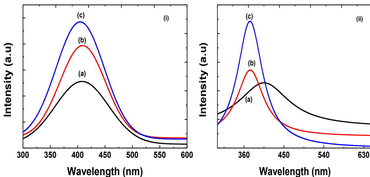
Figure 4.29: (i) PL spectra of OLA/ \beta - \text{In}_2\text{S}_3 at (a) 120 min, (b) 150 min, and (c) 180 min with 1-DDT as sulphur source; (ii) 1-DDT/ \beta - \text{In}_2\text{S}_3 at (a) 60 min, (b) 90 min, and (c) 150 min.
