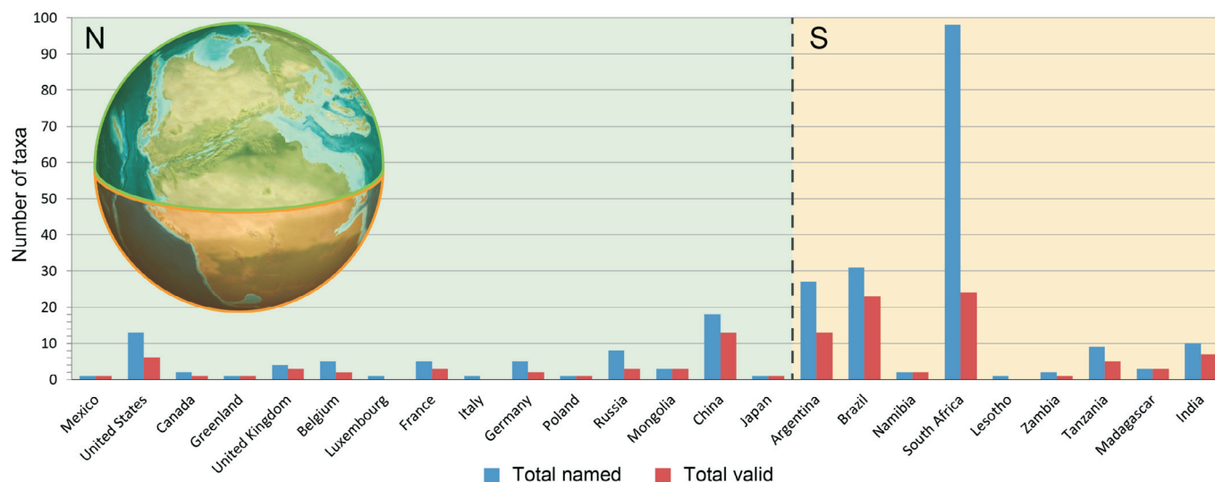
Figure 5. Non-mammaliaform cynodonts named and valid in the world. N, in green, is north Pangaea and S, in yellow, south Pangaea. Only places where species were nominated for the first time are presented.
