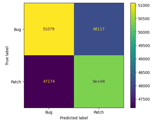
Figure 4.40: VGG16 Word2Vec Confusion matrix
