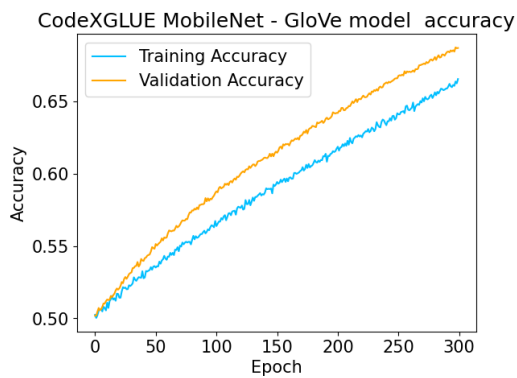
Figure 57: MobileNet GloVe Model Accuracy vs Epoch
