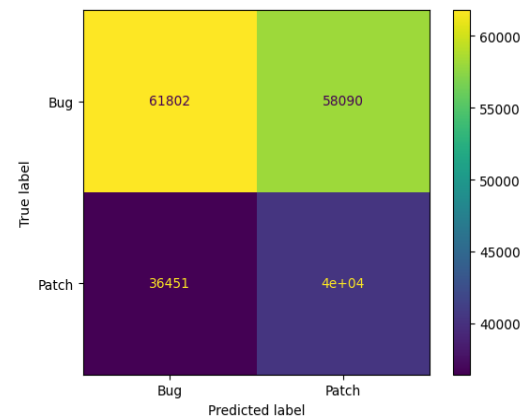
Figure 4.16: 2D Basemodel Word2Vec Confusion matrix
