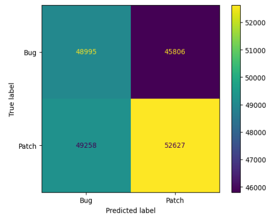
Figure 4.24: 2D Basemodel GloVe Confusion matrix
