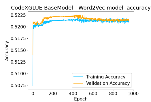
Figure 18: 2D Basemodel Word2Vec Model Accuracy vs Epoch
