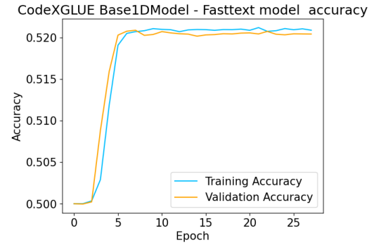
Figure 2: 1DBasemodel Fasttext Model Accuracy vs Epoch
