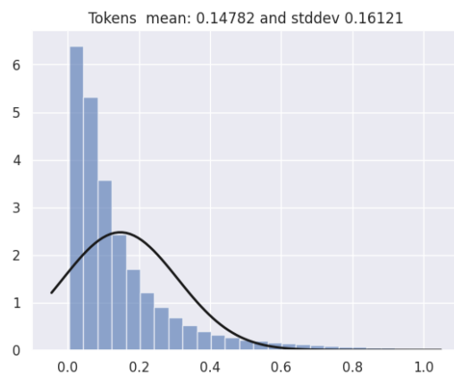
Figure 4.78: Represents a histogram of the normalized lengths of each method tokenized before padding it to length 1225
