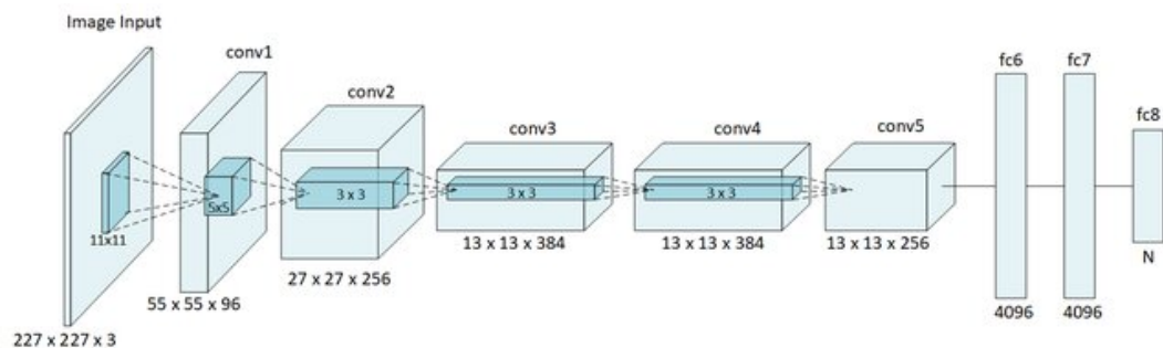
Figure 2.15: AlexNet architecture [7]
