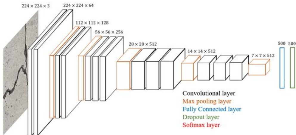
Figure 2.16: VGG16 architecture [8]
