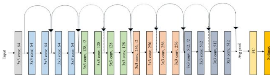
Figure 2.18: Resnet18 architecture [10]
