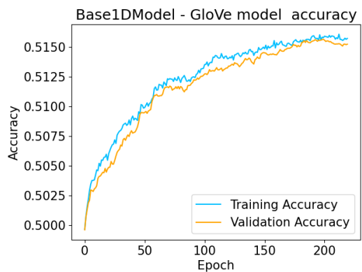
Figure 77: 1DBasemodel GloVe Model Accuracy vs Epoch
