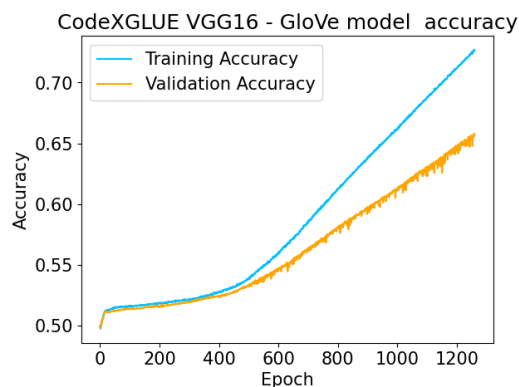
Figure 46: VGG16 GloVe earlystop Model Accuracy vs Epoch
