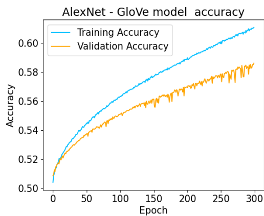
Figure 4.33: AlexNet GloVe Model Accuracy vs Epoch
