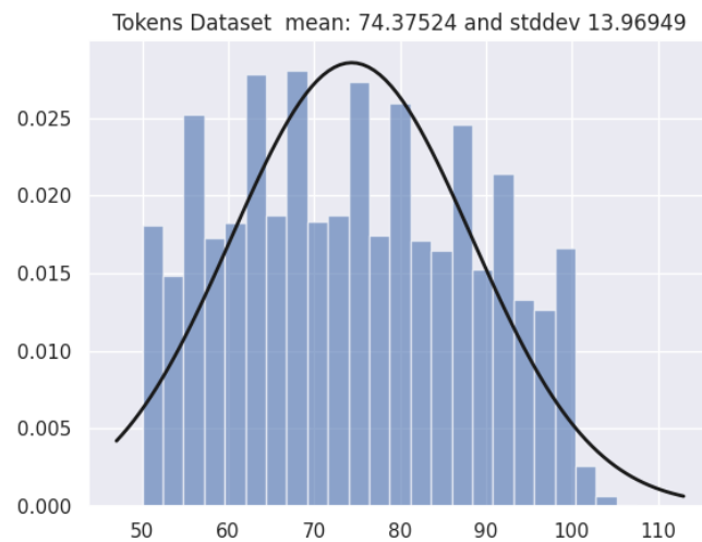
Figure 3.7: Represents a histogram of the token dataset lengths of each method from the processed CodeXGLUE dataset
