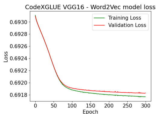
Figure 43: VGG16 Word2Vec Model Loss vs Epoch
