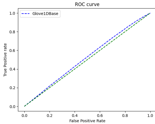
Figure 4.11: 1DBasemodel GloVe Model ROC, AUC score : 0.522
