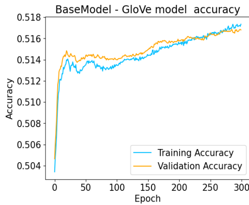
Figure 4.21: 2D Basemodel GloVe Model Accuracy vs Epoch
