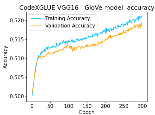
Figure 45: VGG16 GloVe Model Accuracy vs Epoch
