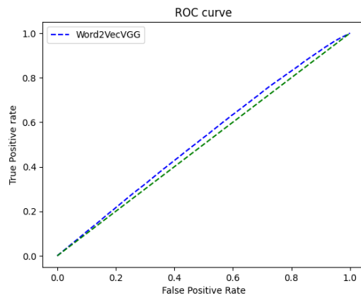
Figure 4.39: VGG16 Word2Vec Model ROC, AUC score :0.523
