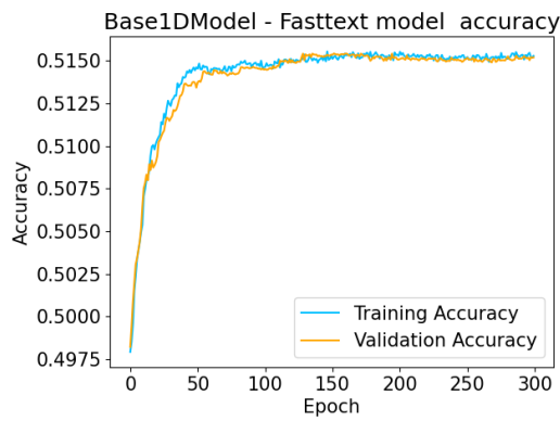
Figure 4.5: 1DBasemodel Fasttext Model Accuracy vs Epoch
