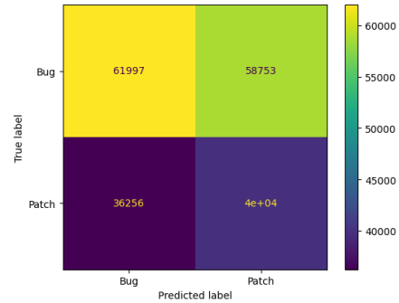
Figure 4.4: 1DBasemodel Word2Vec Confusion matrix
