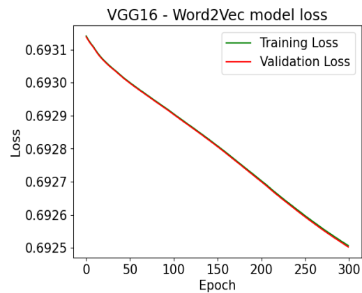
Figure 4.38: VGG16 Word2Vec Model Loss vs Epoch
