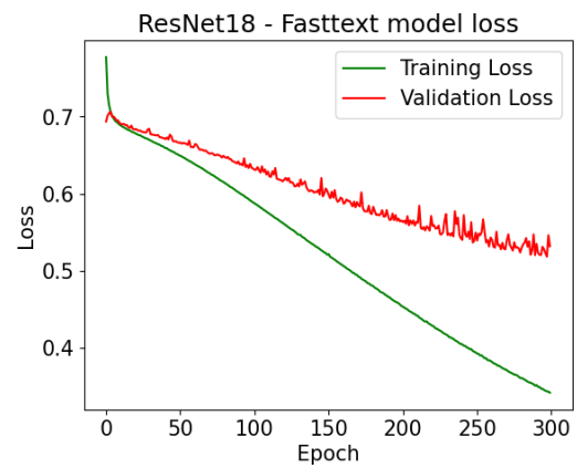
Figure 4.66: ResNet18 Fasttext Model Loss vs Epoch
