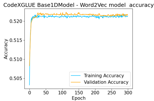
Figure 5: 1DBasemodel Word2Vec Model Accuracy vs Epoch
