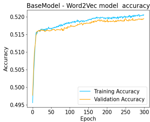
Figure 4.13: 2D Basemodel Word2Vec Model Accuracy vs Epoch
