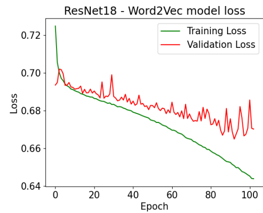
Figure 104: ResNet18 Word2Vec Model Loss vs Epoch
