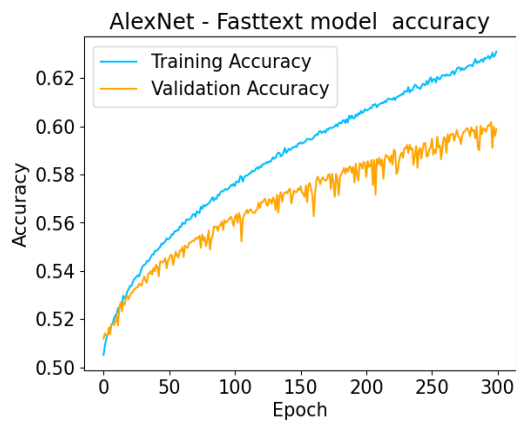
Figure 4.29: AlexNet Fasttext Model Accuracy vs Epoch
