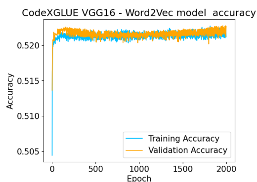
Figure 42: VGG16 Word2Vec Model Accuracy vs Epoch
