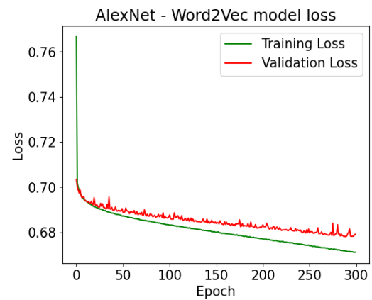
Figure 4.26: AlexNet Word2Vec Model Loss vs Epoch
