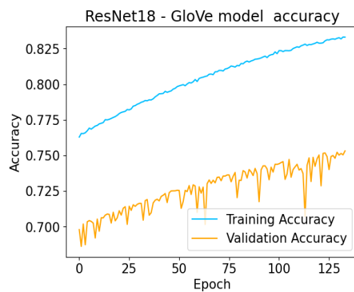
Figure 107: ResNet18 GloVe Model Accuracy vs Epoch
