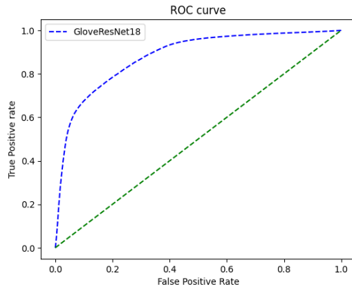
Figure 4.71: ResNet18 GloVe Model ROC, AUC score : 0.880
