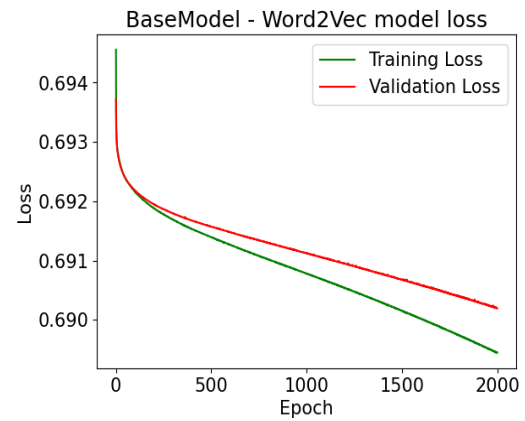
Figure 80: 2D Basemodel Word2Vec Model Loss vs Epoch
