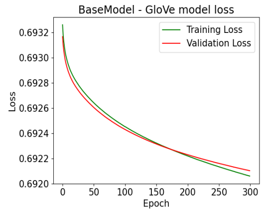
Figure 4.22: 2D Basemodel GloVe Model Loss vs Epoch
