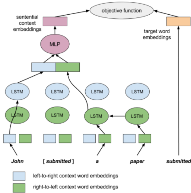
Figure 2.11: Context2Vec architecture takes input sentence words from both directions passed to a bidirectional LSTM to output embedding of the context word [6].
