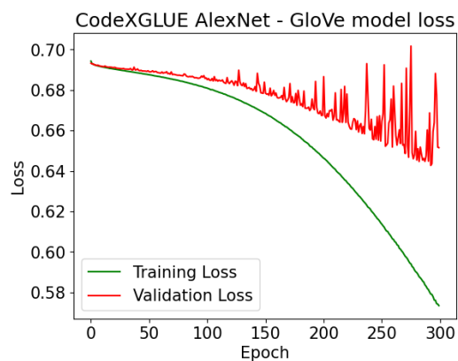
Figure 35: AlexNet GloVe Model Loss vs Epoch
