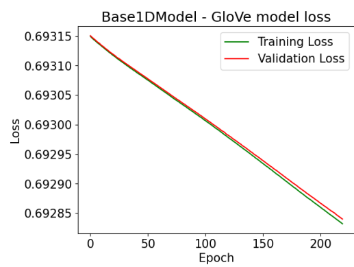
Figure 78: 1DBasemodel GloVe Model Loss vs Epoch
