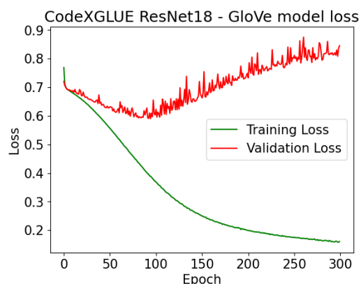
Figure 71: ResNet18 GloVe Model Loss vs Epoch
