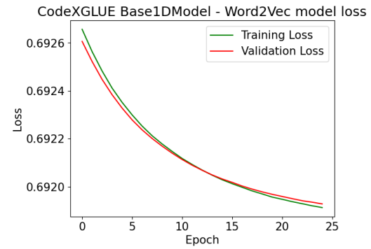
Figure 8: 1DBasemodel Word2Vec earlystop Model Loss vs Epoch
