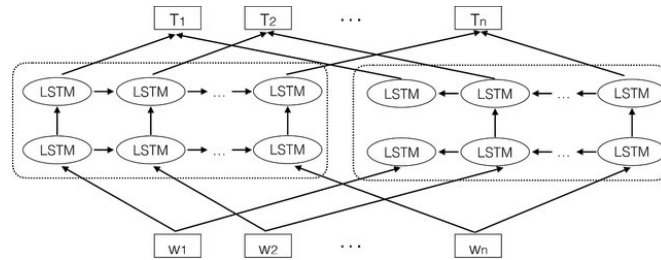
Figure 2.12: ELMo takes input of n-gram word vectors which are fed through bidirectional LSTM to output a sequence of corresponding embeddings[5].
