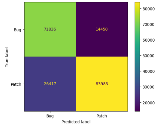
Figure 4.72: ResNet18 GloVe Confusion matrix
