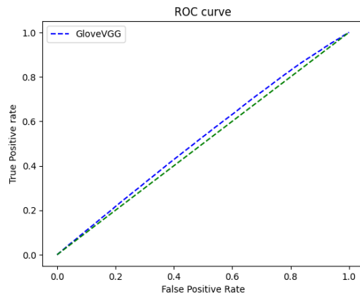
Figure 4.47: VGG16 GloVe Model ROC, AUC score : 0.521
