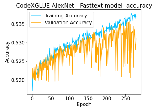
Figure 26: AlexNet Fasttext Model Accuracy vs Epoch
