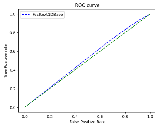
Figure 4.7: 1DBasemodel Fasttext Model ROC, AUC score : 0.520
