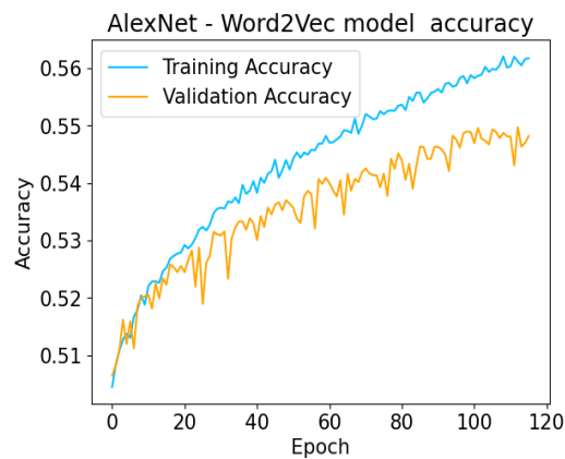
Figure 85: AlexNet Word2Vec Model Accuracy vs Epoch
