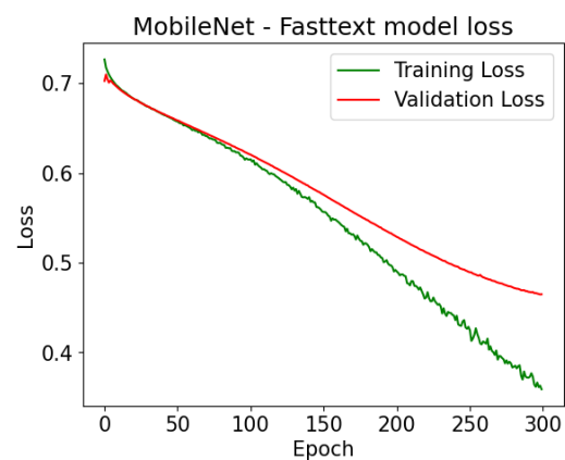
Figure 4.54: MobileNet Fasttext Model Loss vs Epoch
