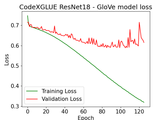
Figure 72: ResNet18 GloVe earlystop Model Loss vs Epoch
