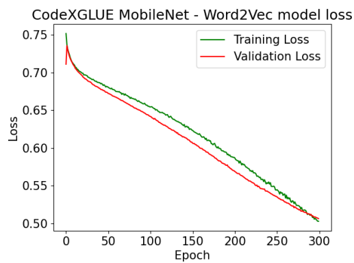
Figure 55: MobileNet Word2Vec Model Loss vs Epoch
