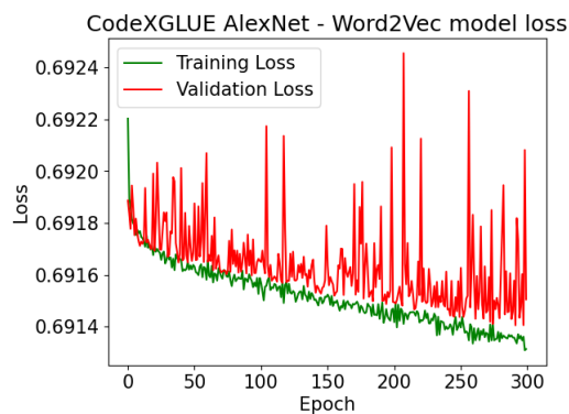
Figure 31: AlexNet Word2Vec Model Loss vs Epoch
