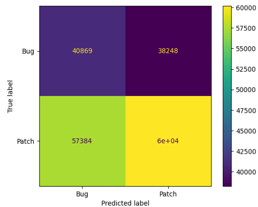
Figure 4.48: VGG16 GloVe Confusion matrix
