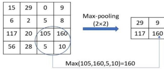
Figure 2.5: Max pooling computation [3]
