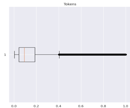
Figure 4.79: Represents a box and whisker plot of the normalized lengths of each method tokenized before padding it to length 1225
