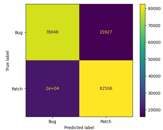
Figure 4.60: MobileNet GloVe Confusion matrix
