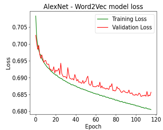
Figure 86: AlexNet Word2Vec Model Loss vs Epoch
