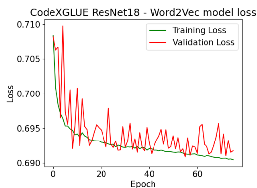
Figure 68: ResNet18 Word2Vec earlystop Model Loss vs Epoch
