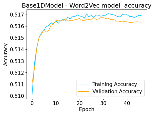
Figure 73: 1DBasemodel Word2Vec Model Accuracy vs Epoch
