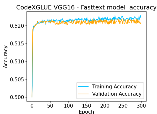
Figure 37: VGG16 Fasttext Model Accuracy vs Epoch
