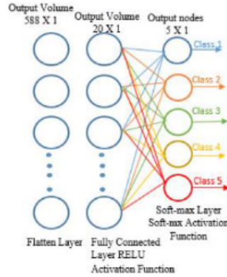
Figure 2.6: Illustration of a dense layer connected to a flattened output of a convolution layer [3]
