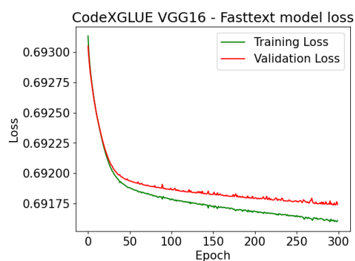
Figure 39: VGG16 Fasttext Model Loss vs Epoch
