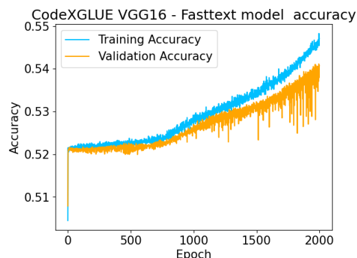
Figure 38: VGG16 Fasttext Model Accuracy vs Epoch
