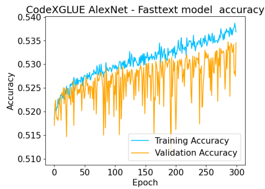
Figure 25: AlexNet Fasttext Model Accuracy vs Epoch
