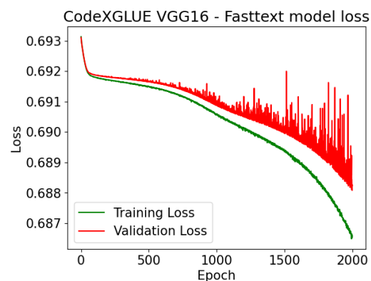
Figure 40: VGG16 Fasttext Model Loss vs Epoch
