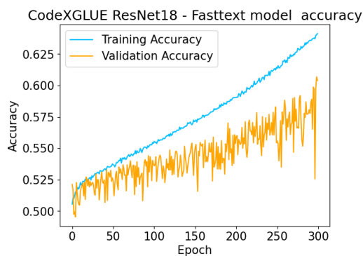
Figure 61: ResNet18 Fasttext Model Accuracy vs Epoch
