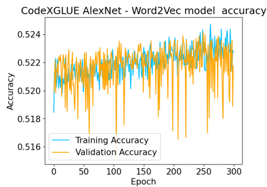
Figure 29: AlexNet Word2Vec Model Accuracy vs Epoch
