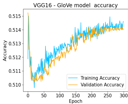
Figure 4.45: VGG16 GloVe Model Accuracy vs Epoch
