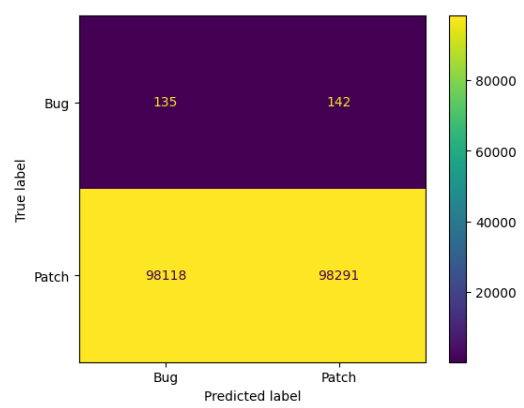
Figure 4.8: 1DBasemodel Fasttext Confusion matrix
