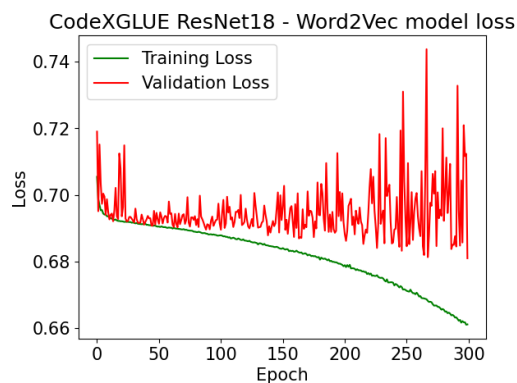
Figure 67: ResNet18 Word2Vec Model Loss vs Epoch
