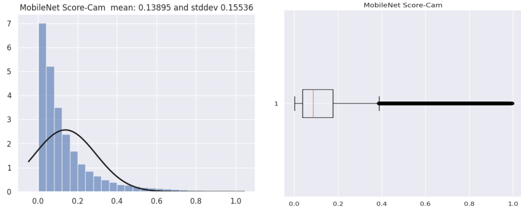
Figure 4.80: Represents a histogram of the MobileNet Fraction of Elements above threshold 0.4 using Score-CAM and Word2Vec embedding Figure 4.81: Represents a box and whisker plot of the MobileNet Fraction of Elements above threshold 0.4 using Score-CAM and Word2Vec embedding
