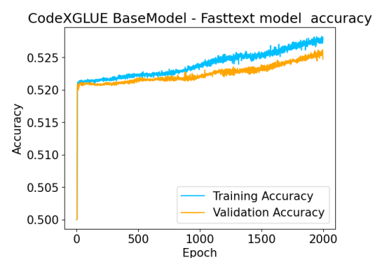
Figure 14: 2D Basemodel Fasttext Model Accuracy vs Epoch
