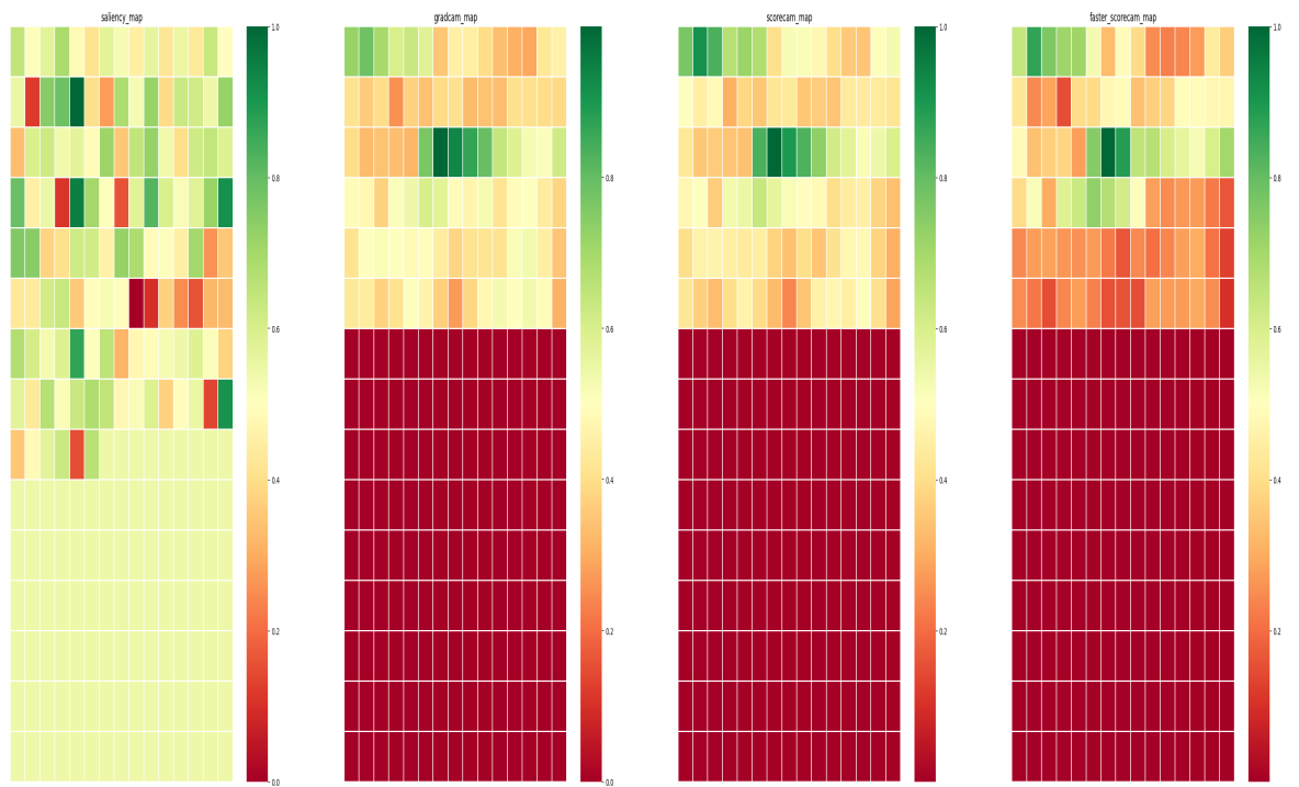
Figure 3.8: Explainable AI Visualization methods for code snippet 3.3 generated by MobileNet with Word2Vec embedding, From left to right is Saliency map ,Grad-CAM, Score-CAM, FIMF score-CAM with a heatmap scale of 0 to 1.0 of intensities
