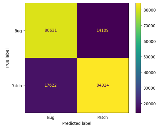
Figure 4.56: MobileNet Fasttext Confusion matrix
