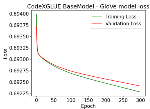
Figure 23: 2D Basemodel GloVe Model Loss vs Epoch
