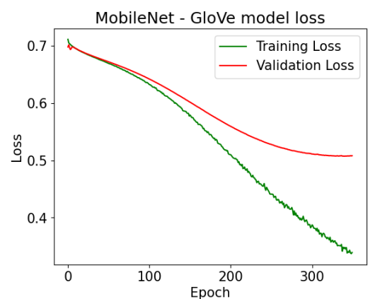
Figure 102: MobileNet GloVe Model Loss vs Epoch
