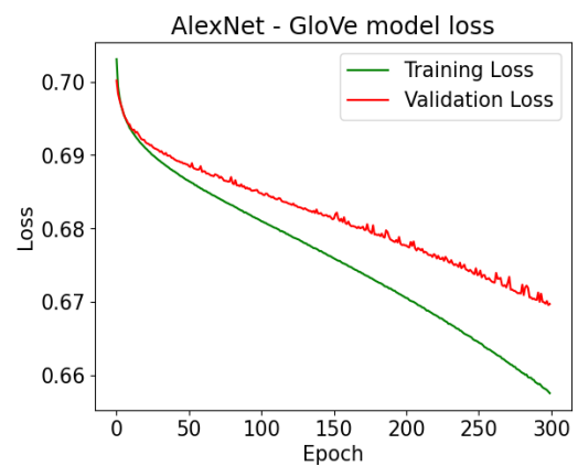
Figure 4.34: AlexNet GloVe Model Loss vs Epoch
