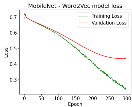
Figure 98: MobileNet Word2Vec Model Loss vs Epoch
