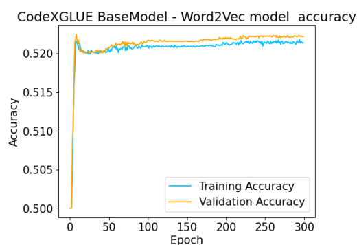
Figure 17: 2D Basemodel Word2Vec Model Accuracy vs Epoch
