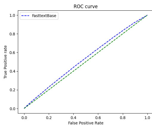
Figure 4.19: 2D Basemodel Fasttext Model ROC, AUC score : 0.530
