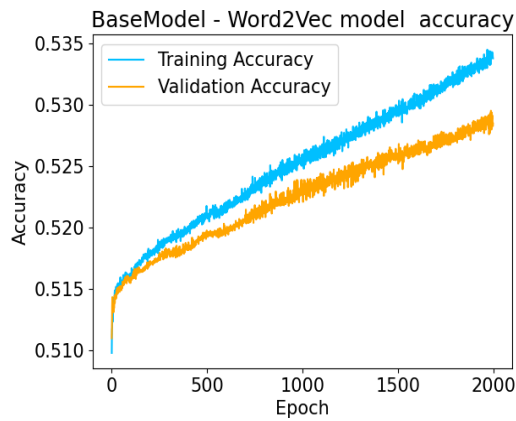
Figure 79: 2D Basemodel Word2Vec Model Accuracy vs Epoch
