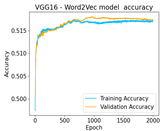
Figure 91: VGG16 Word2Vec Model Accuracy vs Epoch
