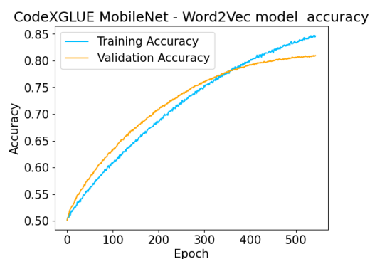
Figure 54: MobileNet Word2Vec earlystop Model Accuracy vs Epoch
