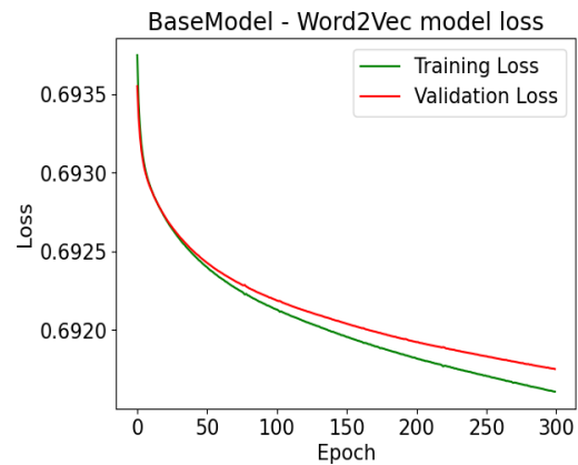
Figure 4.14: 2D Basemodel Word2Vec Model Loss vs Epoch
