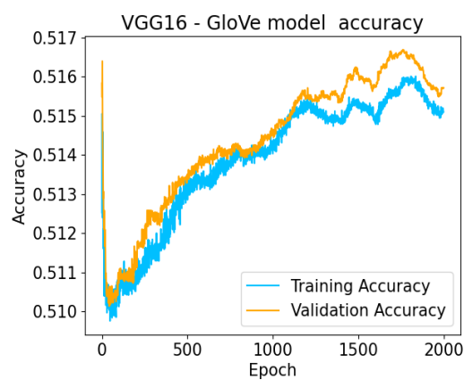
Figure 95: VGG16 Glove Model Accuracy vs Epoch
