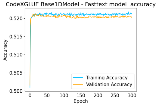
Figure 1: 1DBasemodel Fasttext Model Accuracy vs Epoch
