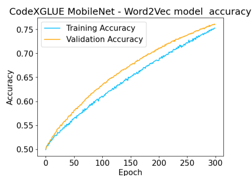
Figure 53: MobileNet Word2Vec Model Accuracy vs Epoch
