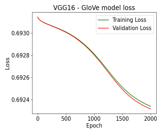
Figure 96: VGG16 GloVe Model Loss vs Epoch
