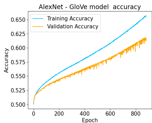
Figure 89: AlexNet GloVe Model Accuracy vs Epoch
