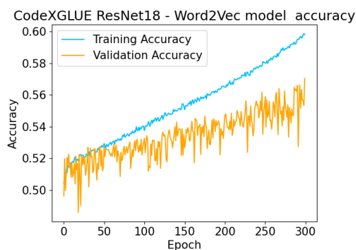
Figure 65: ResNet18 Word2Vec Model Accuracy vs Epoch
