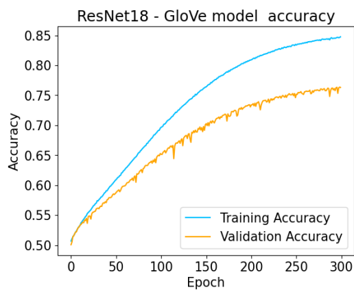
Figure 4.69: ResNet18 GloVe Model Accuracy vs Epoch
