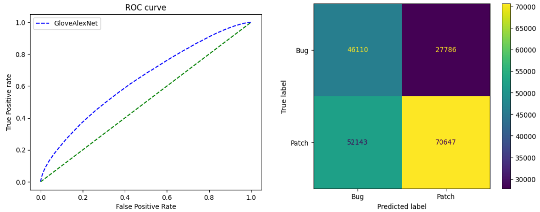
Figure 4.35: AlexNet GloVe Model ROC, Figure 4.36: AlexNet GloVe Confusion matrix AUC score : 0.637
