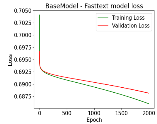
Figure 82: 2D Basemodel Fasttext Model Loss vs Epoch
