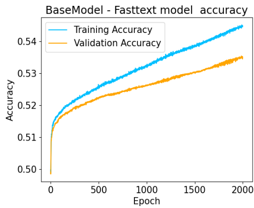
Figure 81: 2D Basemodel Fasttext Model Accuracy vs Epoch
