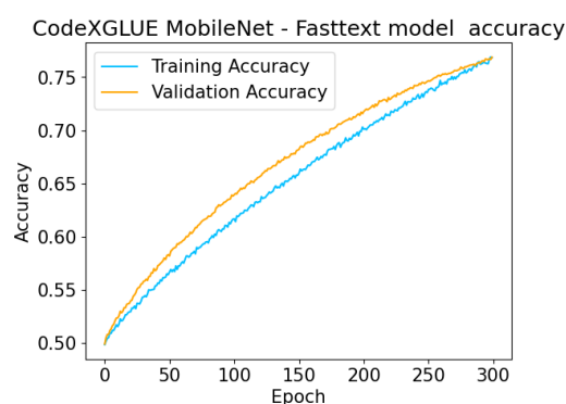
Figure 49: MobileNet Fasttext Model Accuracy vs Epoch
