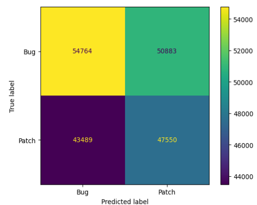
Figure 4.20: 2D Basemodel Fasttext Confusion matrix
