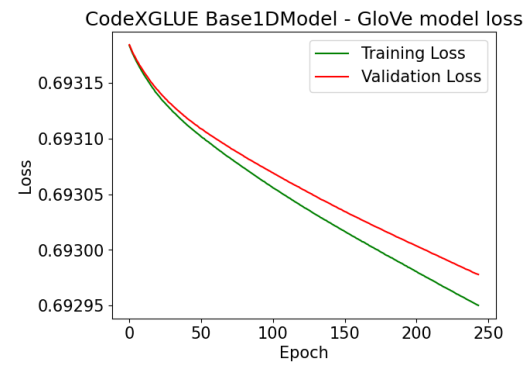
Figure 12: 1DBasemodel GloVe earlystop Model Loss vs Epoch
