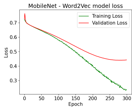
Figure 4.50: MobileNet Word2Vec Model Loss vs Epoch
