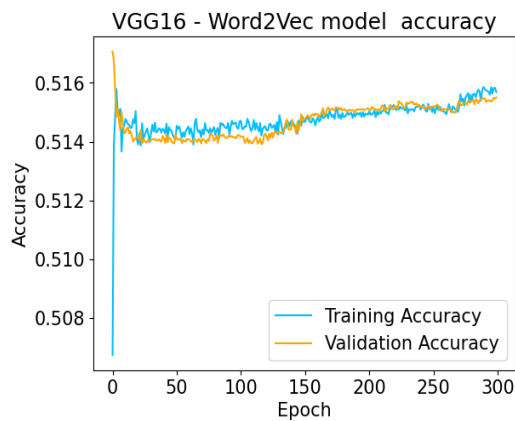
Figure 4.37: VGG16 Word2Vec Model Accuracy vs Epoch
