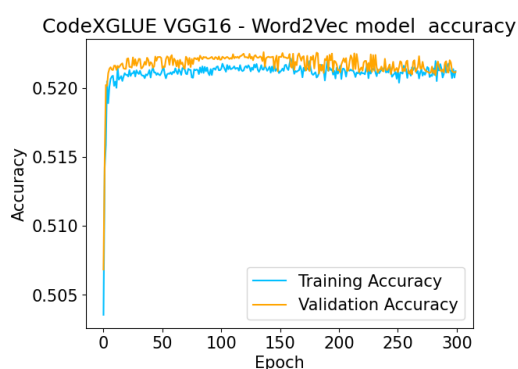
Figure 41: VGG16 Word2Vec Model Accuracy vs Epoch
