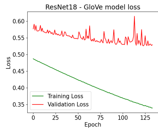
Figure 108: ResNet18 GloVe Model Loss vs Epoch
