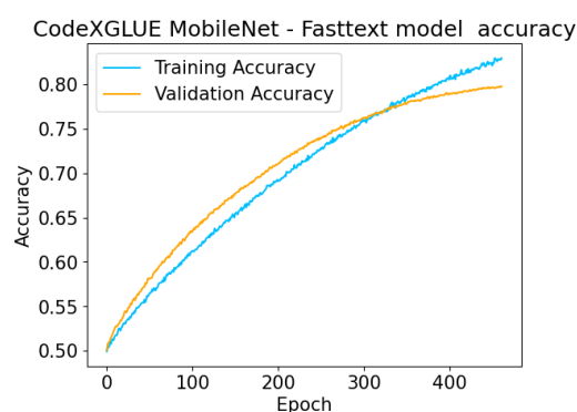
Figure 50: MobileNet Fasttext earlystop Model Accuracy vs Epoch
