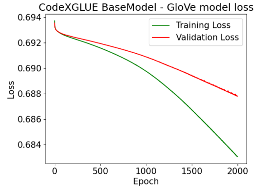
Figure 24: 2D Basemodel GloVe earlystop Model Loss vs Epoch
