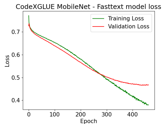
Figure 52: MobileNet Fasttext earlystop Model Loss vs Epoch
