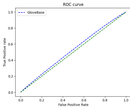
Figure 4.23: 2D Basemodel GloVe Model ROC, AUC score : 0.525
