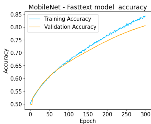
Figure 4.53: MobileNet Fasttext Model Accuracy vs Epoch
