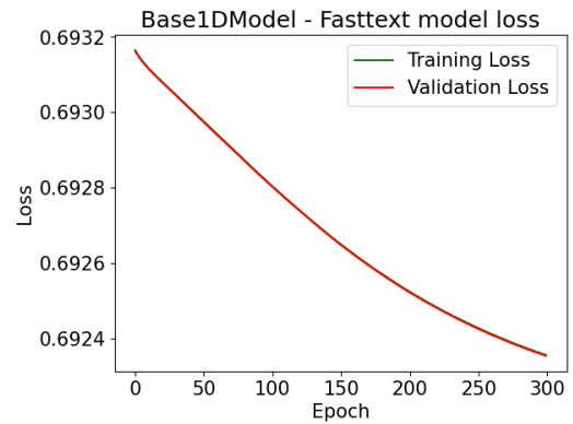
Figure 4.6: 1DBasemodel Fasttext Model Loss vs Epoch
