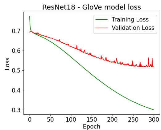
Figure 4.70: ResNet18 GloVe Model Loss vs Epoch
