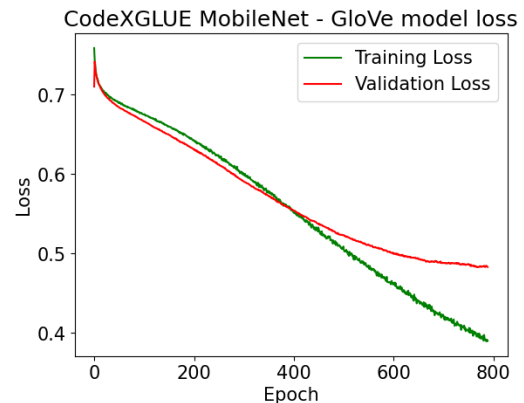
Figure 60: MobileNet GloVe earlystop Model Loss vs Epoch
