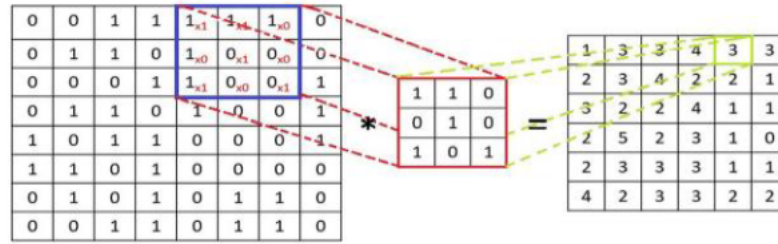
Figure 2.4: Convolution layer computation with a kernel of size 3x3 [3]
