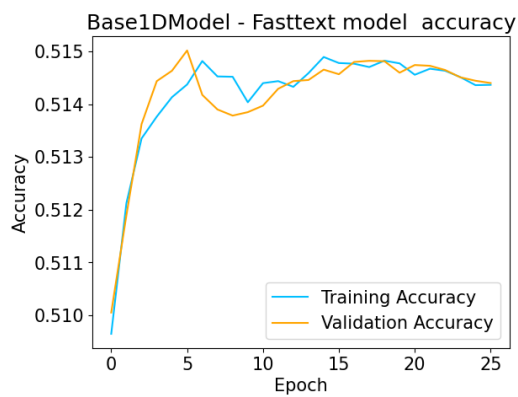
Figure 75: 1DBasemodel Fasttext Model Accuracy vs Epoch
