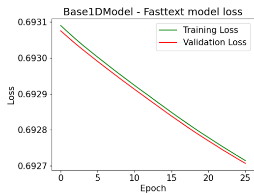
Figure 76: 1DBasemodel Fasttext Model Loss vs Epoch
