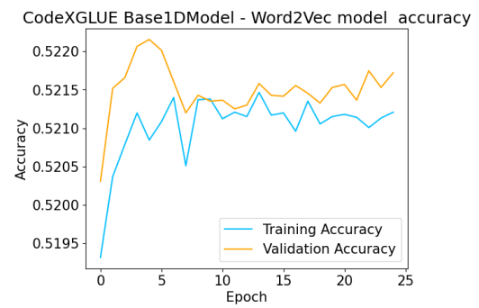
Figure 6: 1DBasemodel Word2Vec Model Accuracy vs Epoch
