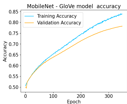
Figure 101: MobileNet GloVe Model Accuracy vs Epoch
