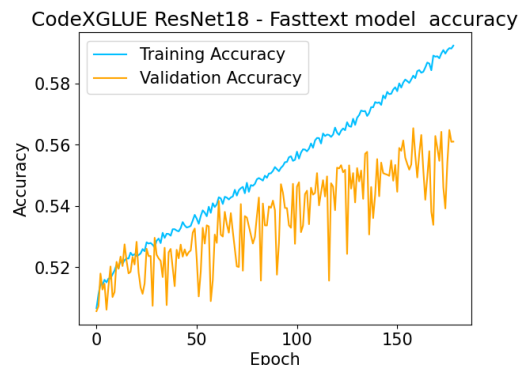
Figure 62: ResNet18 Fasttext Model Accuracy vs Epoch
