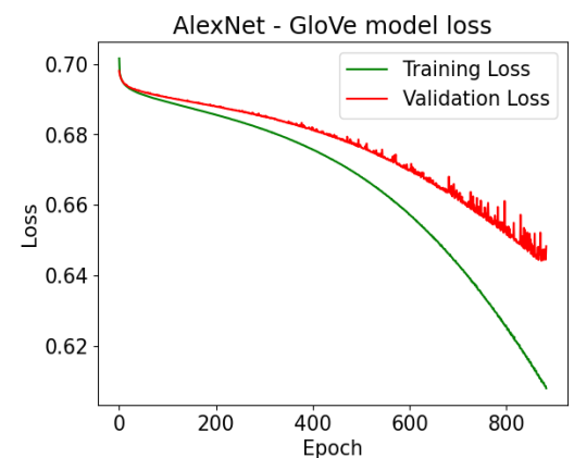
Figure 90: AlexNet GloVe Model Loss vs Epoch
