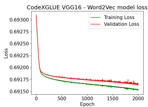
Figure 44: VGG16 Word2Vec earlystop Model Loss vs Epoch
