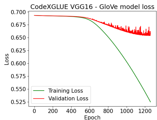
Figure 48: VGG16 GloVe earlystop Model Loss vs Epoch
