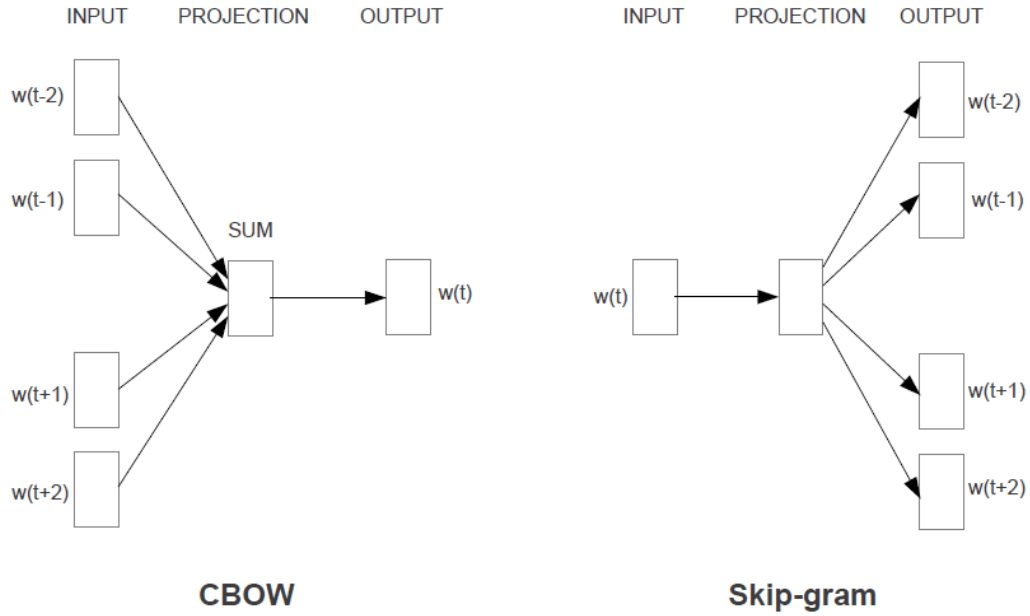
Figure 2.9: CBOW and Skip-gram model architecture [4]. CBOW takes input of a one-hot encoded aggregated context vector passed to a neural network with one hidden layer to predict the target word, while Skip-gram takes a target word as input passed through a neural network with a single hidden layer to predict neighboring context words.
