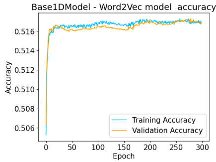
Figure 4.1: 1DBasemodel Word2Vec Model Accuracy vs Epoch
