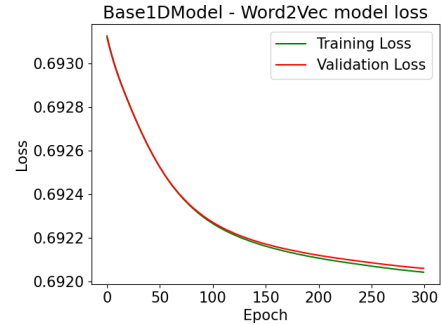
Figure 4.2: 1DBasemodel Word2Vec Model Loss vs Epoch
