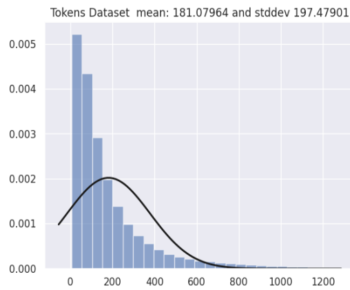
Figure 4.76: Represents a histogram of the lengths of each method tokenized before padding it to length 1225
