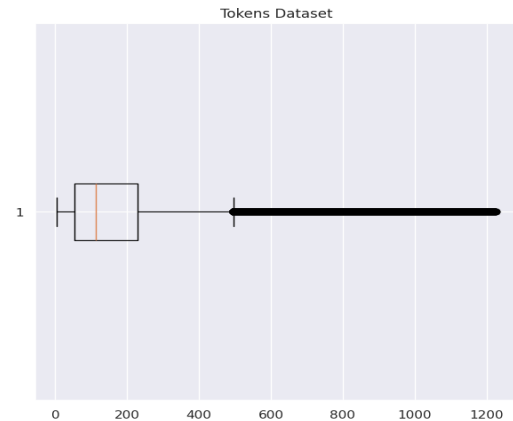
Figure 4.77: Represents a box and whisker plot of the lengths of each method tokenized before padding it to length 1225
