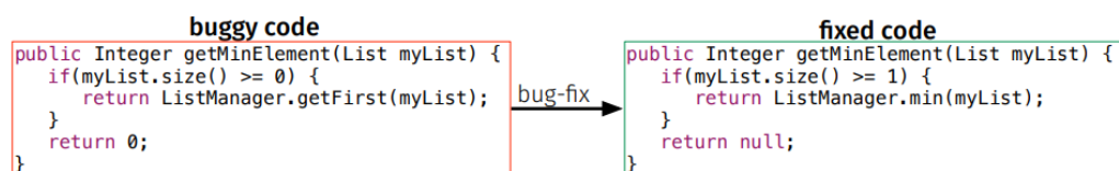
Figure 3.1: Example code snippets in the DataSet [11] showing buggy code snipped along with a fix of the code snipped
