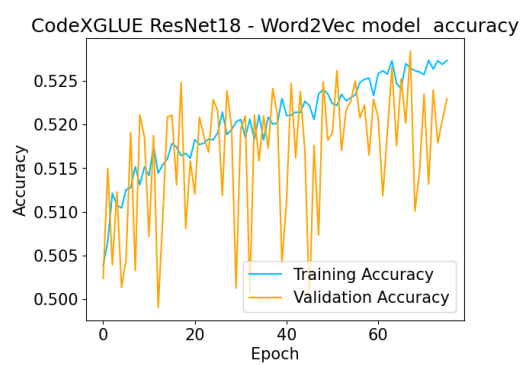
Figure 66: ResNet18 Word2Vec Model Accuracy vs Epoch
