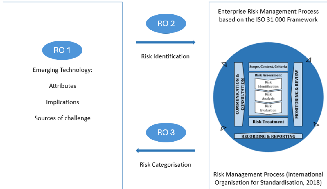
Figure 2: Conceptual framework
