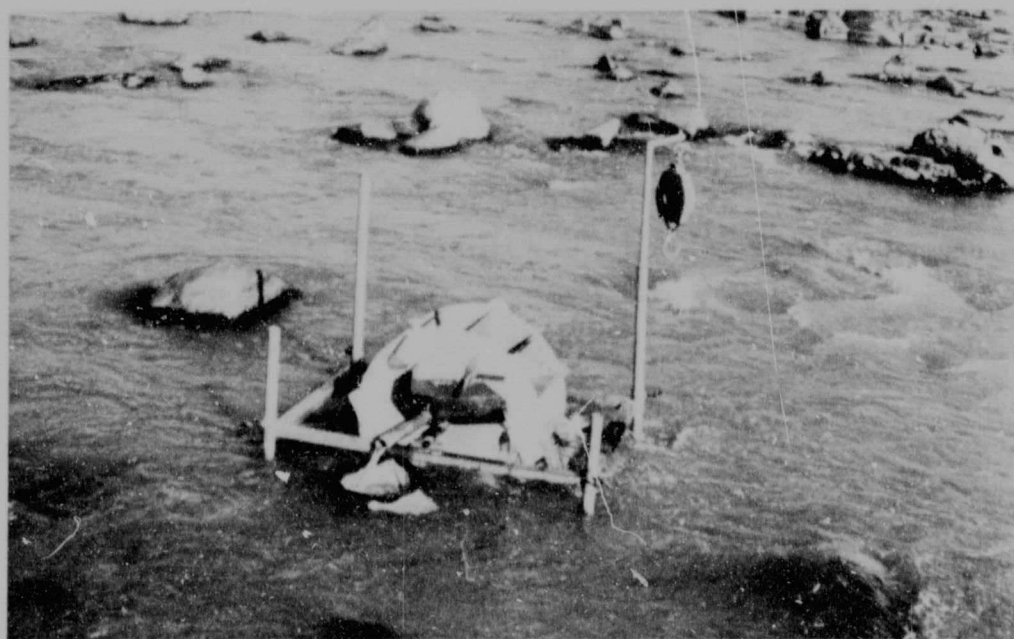
PLATE 4: The paddle-wheel sampler collecting drifting organisms from the Vaal River ca. 35 m upstream of the top end of the study rapid. Note star shaped revolution counter, net, and scale used to calibrate sampler.
