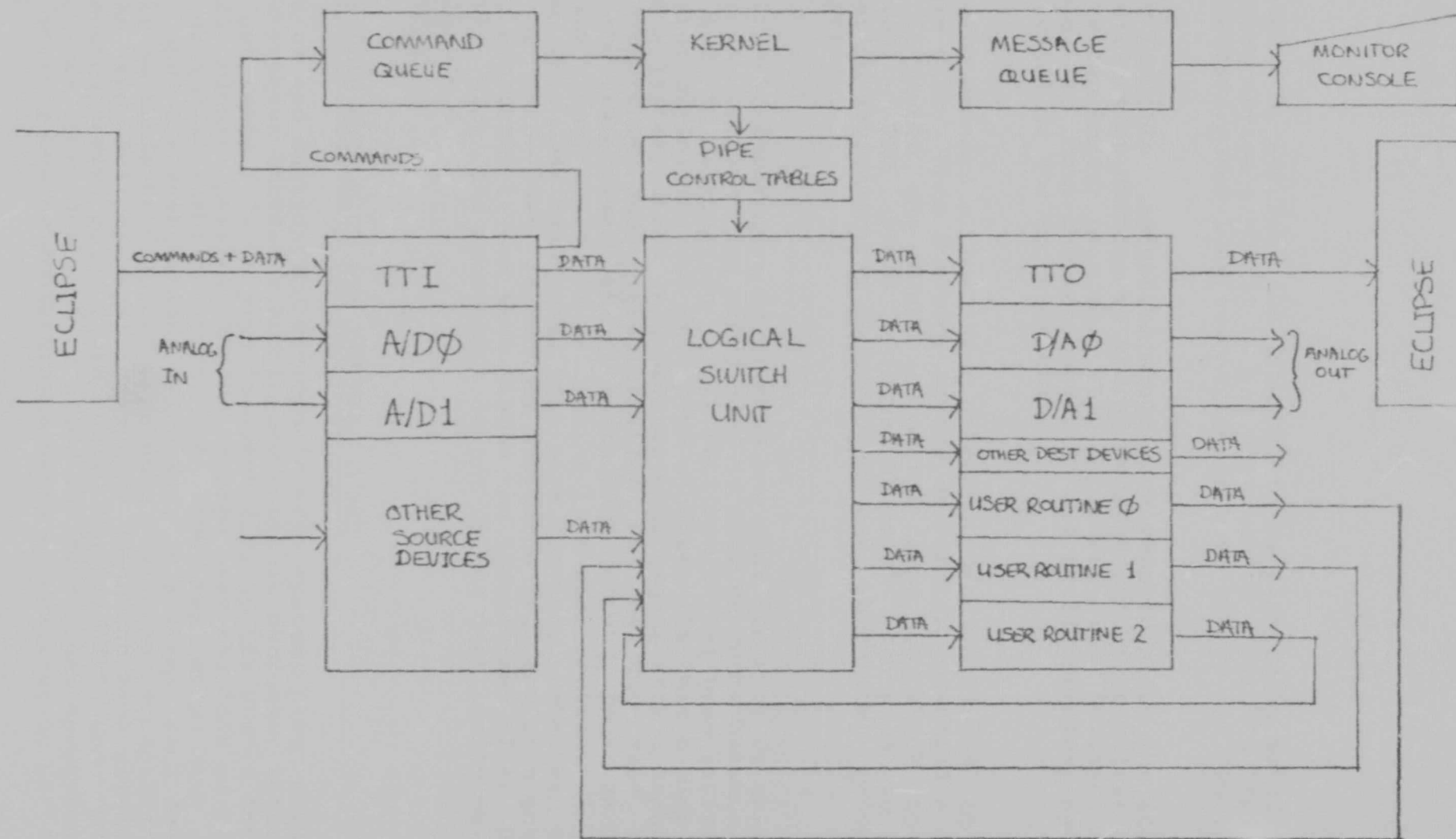
FIGURE 3: BAEDAS CONCEPTUAL MODEL
