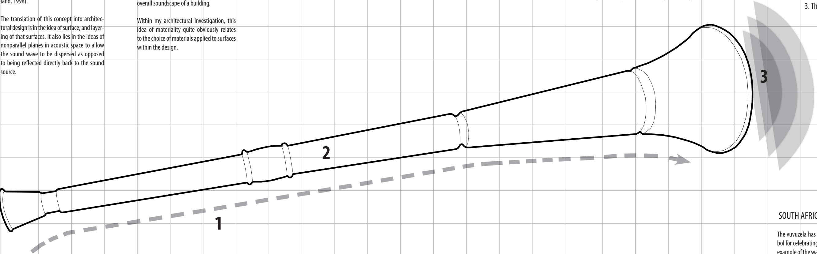
Graph showing the sound waves produced by a vuvuzela
