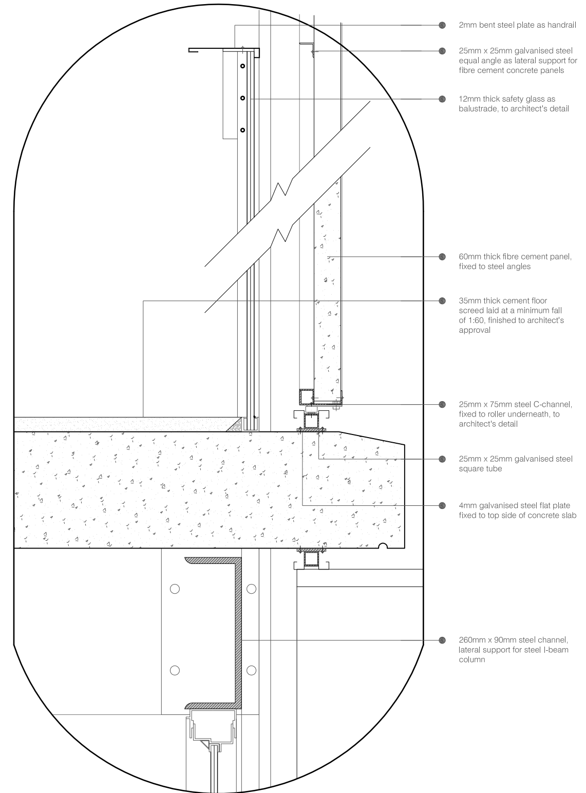
DETAIL A
