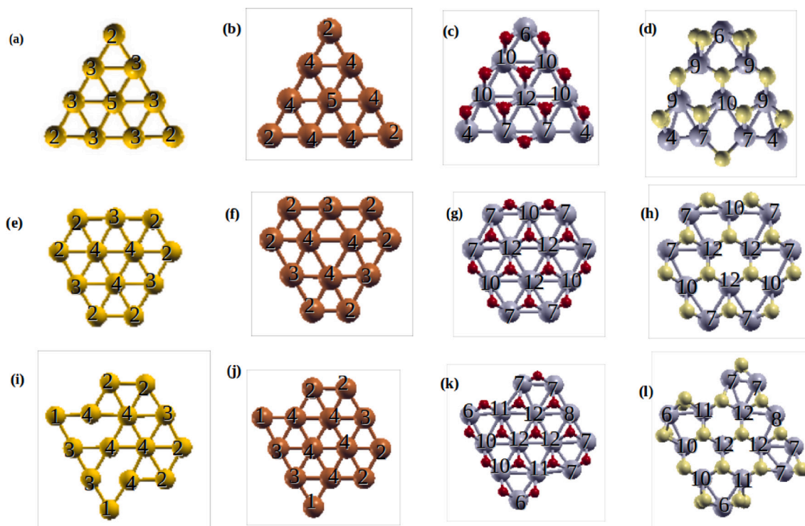
Fig. 1. First, second and third rows represent the optimized nanostructures for Au, Cu, MoO 2 , MoS 2 ; in (a–d) triangular, (e–h) irregular hexagonal, (i–l) octagonal shapes. These shapes correspond to a number of atom x = 10, 12 and 14 , respectively. The coordination number of each probable site of fixation are indicated in each figure. With atom colors: Au (gold), Cu (brown), Mo (gray), O (red) and S (yellow).
