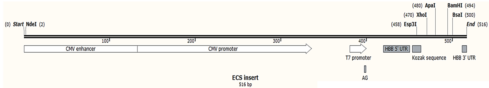
Figure 2.4: Design of the ECS-Fragment for pT7-(AG) Cloning. The ECS-fragment was engineered with several key features: A 5' UTR and an NdeI site for easy insertion into the pT7-(AG) backbone, multiple restriction sites ( XhoI , ApaI , BamHI ) for integrating DEM-encoding sequences, 4 consecutive stop codons and a BsaI site downstream of BamHI to generate an overhang complementary to the Esp3I overhang in the pT7-(AG) vector.
