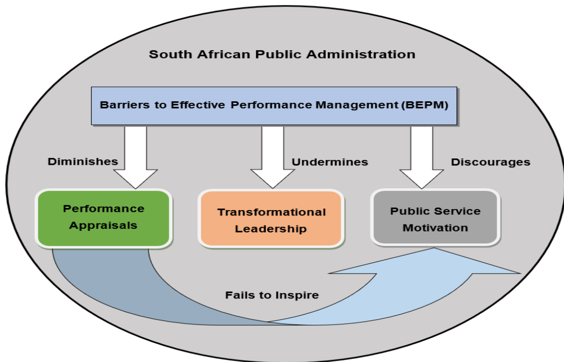
Figure 3: Problem statement
