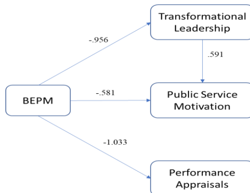
Figure 14: Mediation Analysis
