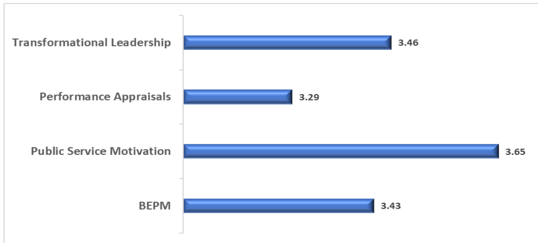
Figure 7: Constructs and their mean values
