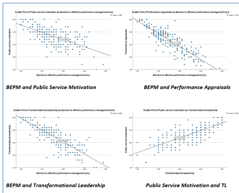
Figure 9: Scatter Plot Diagram
