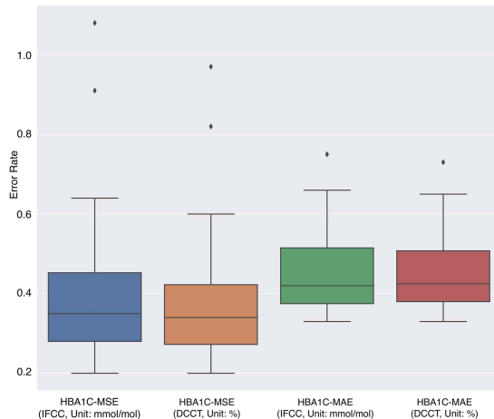
Fig. 6. Error rates in the prediction of IFCC and DCTT units of HbA1c biomarker values.
