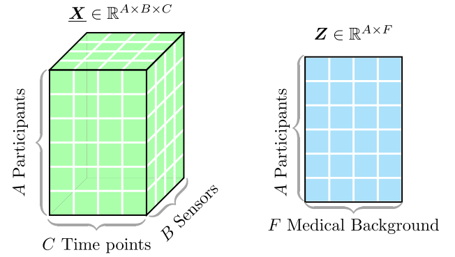
Fig. 3. Coupled matrix - tensor example: Tensors often share one or more modes (i.e. A, participants): \underline{\mathbf{X}} is the activity monitoring sensor recording tensor and \mathbf{Z} is the medical background matrix. As the vertical line indicates, these two datasets are coupled in the “participants” dimension.
