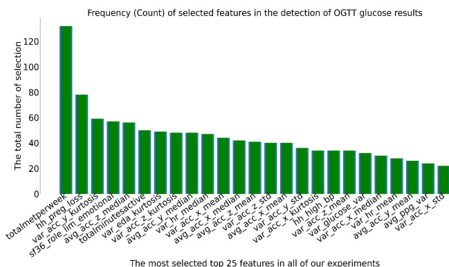
Fig. 8. Most frequently selected features in the feature selection process.
