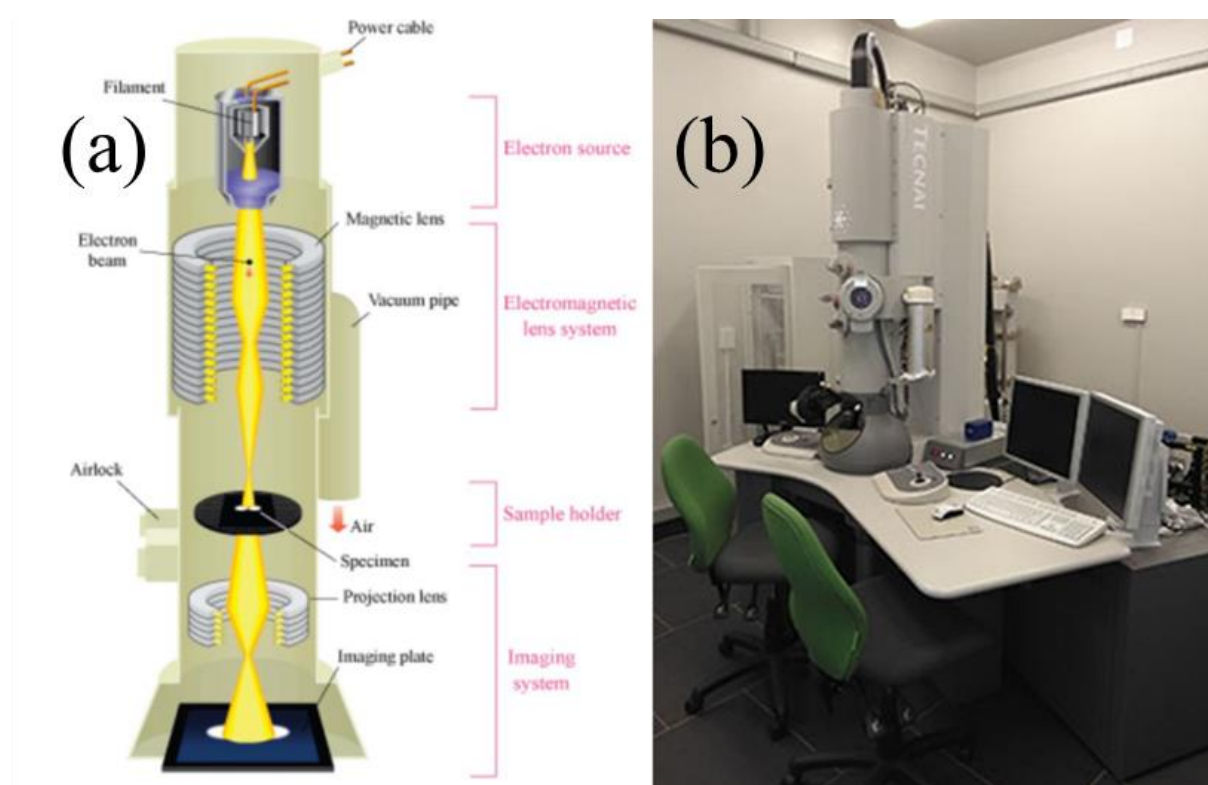
Figure 2.8: (a) Schematic of a TEM and (b) F20 Tecnai transmission electron microscope. 22
