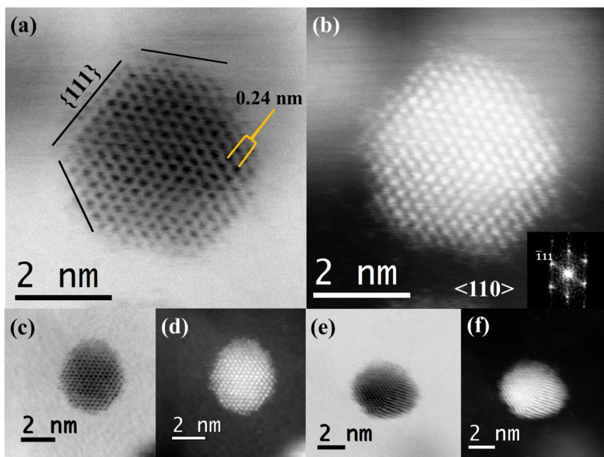
Figure 5.7: High resolution ADF-BF STEM images of (a-b) Pt/BHCSs and (c-f) Pt/BNHCSs. The insert in (b) is the power spectrum of a <110> projection of the fcc Pt.
