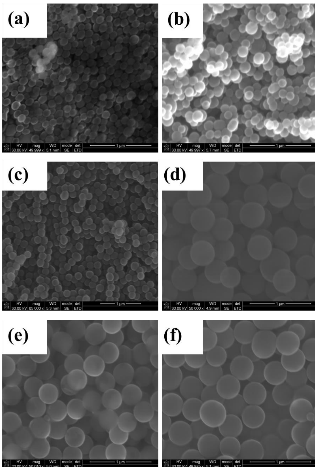
Figure 3.8: SEM images as the deionized water concentration is varied from (a) 5 M, (b) 10 M, (c) 15 M, (d) 20 M, (e) 25 M, (f) 30 M and optimum concentration of the other reagents \text{NH}_4\text{OH} (2 M), TEOS (2 M) and EtOH (8 M).
