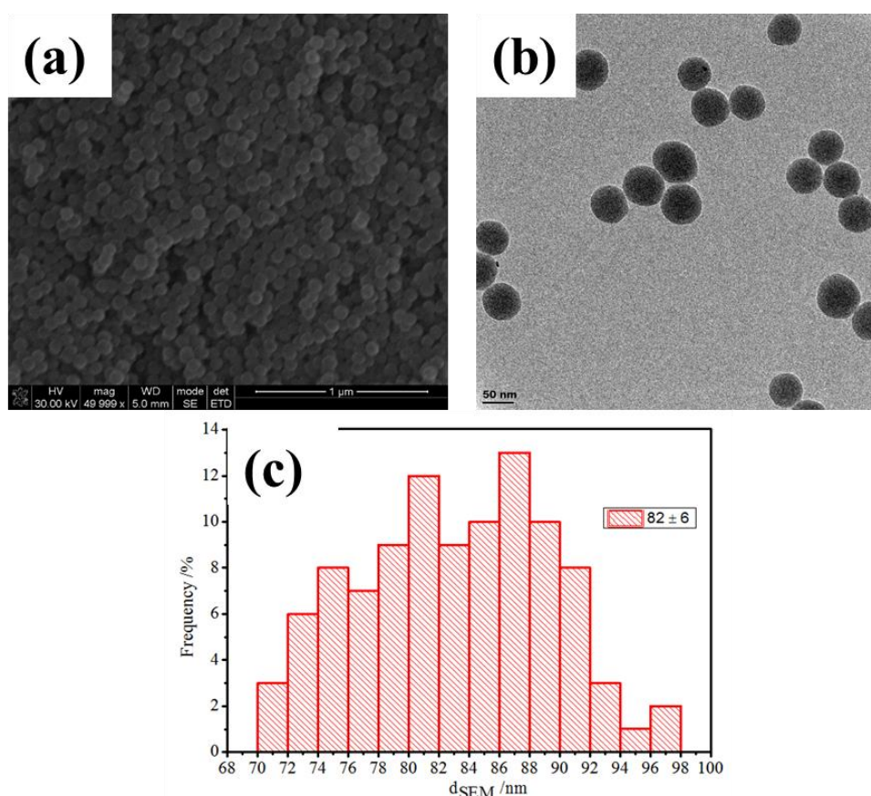
Figure 3.13: SEM(a), TEM(b) images and particle size distribution (c) of the small silica particle ( d < 100 nm) formed at low concentrations of TEOS (2 M), \text{NH}_4\text{OH} (2 M) and DI (5 M) and EtOH (15 M).
