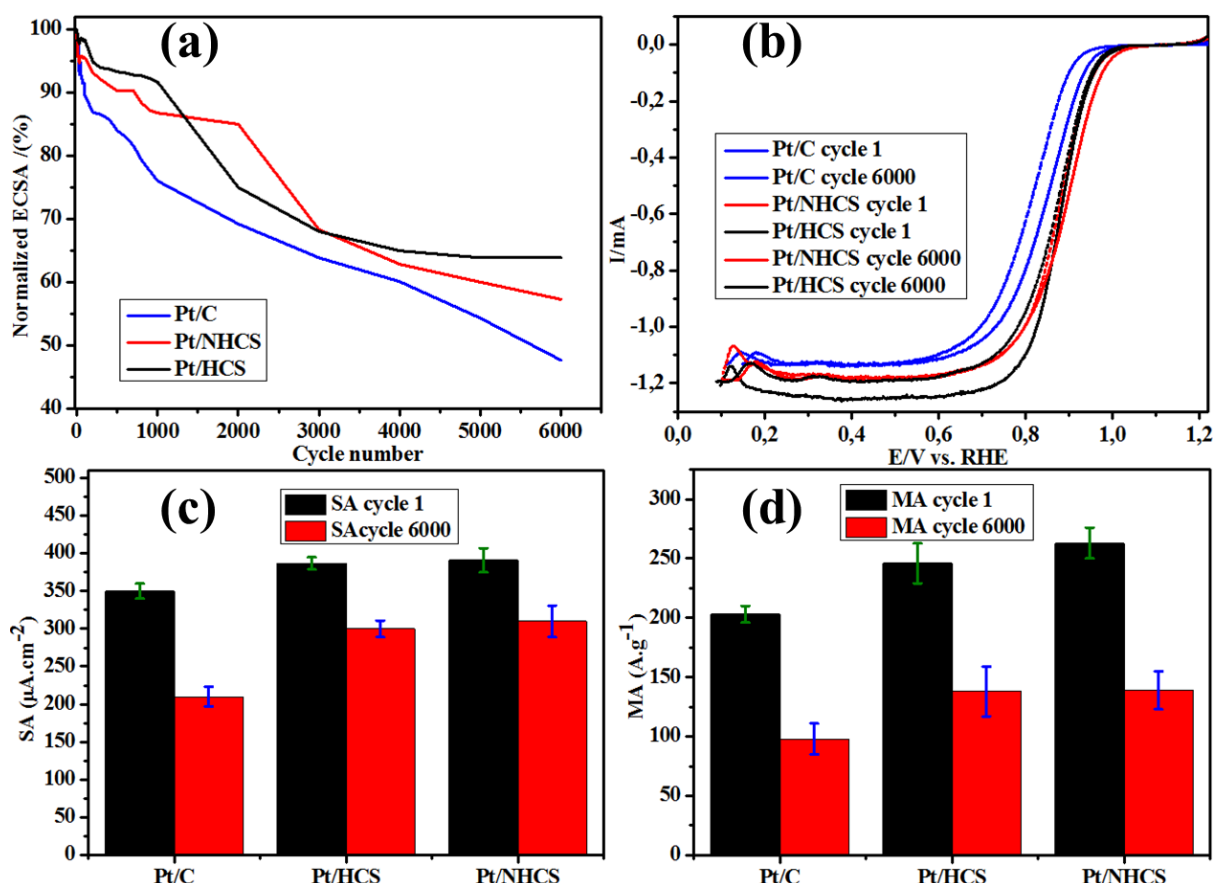
Figure 7. 11: (a) Normalized ECSA% degradation of the catalysts, (b) catalyst LSVs before and after durability studies for the Pt/HCSs, Pt/NHCSs and the commercial benchmark Pt/C catalysts (c) SA data before and after durability studies (d) MA data before and after durability studies.
