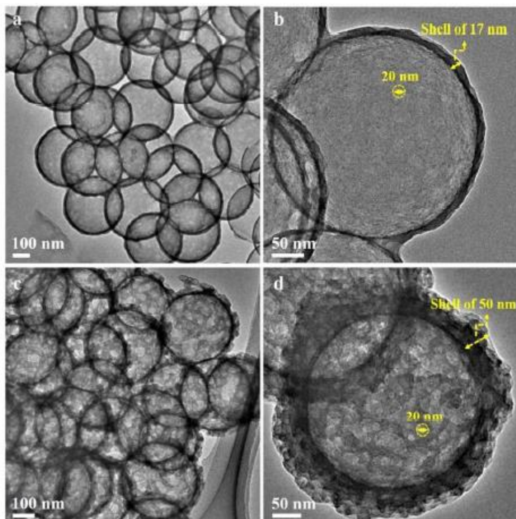
Figure 1.14: TEM images of NHCSs with identical internal diameter and various shell thickness. 137
