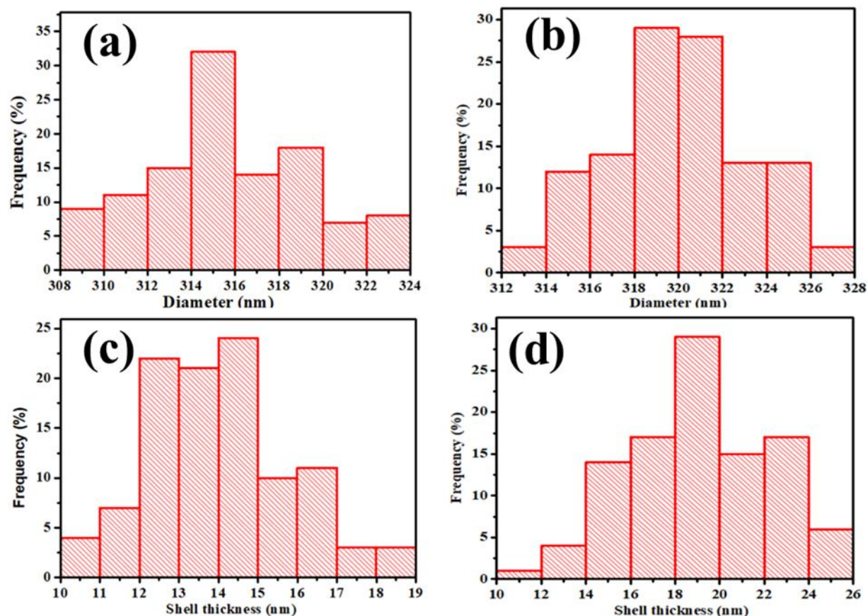
Figure 4.4: Diameter distribution of HCSs (a) and NHCSs (b), shell thickness distribution of HCSs (c) and NHCSs (d)
