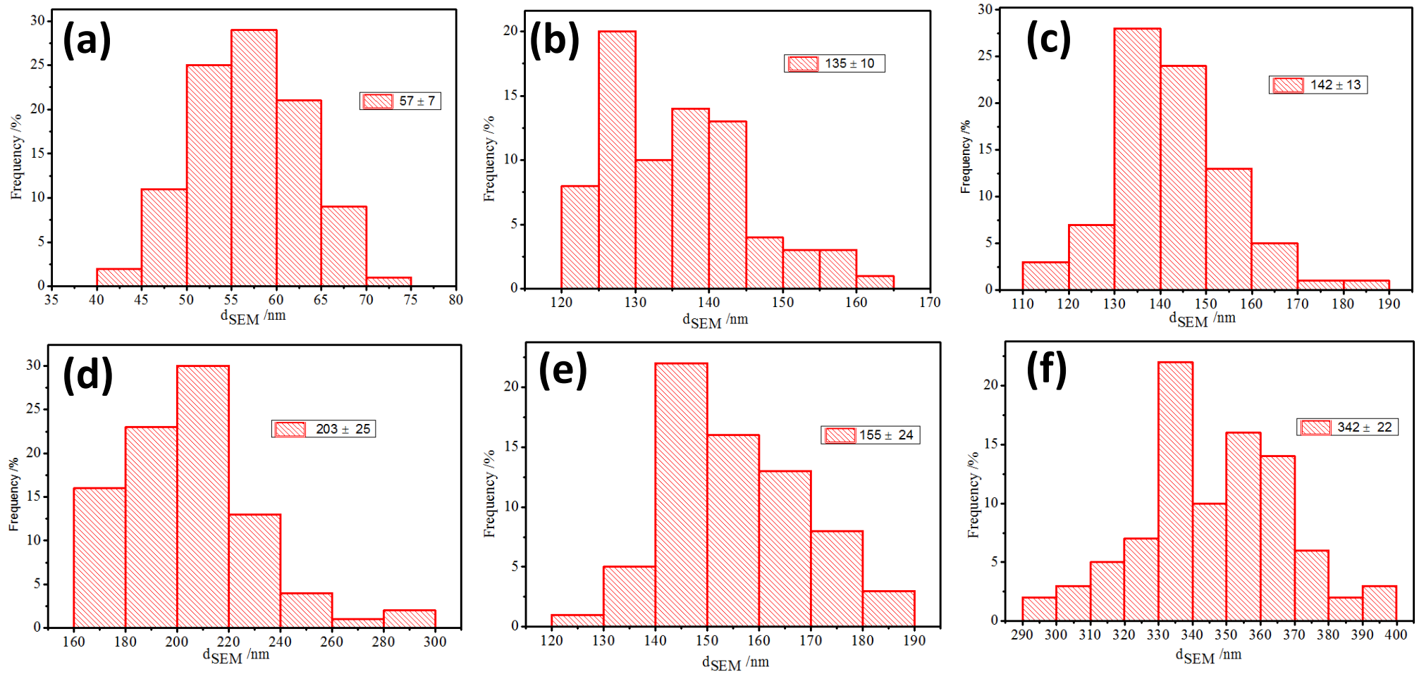
Figure 3. 2: Particle size distributions of silica particles synthesized with \text{NH}_4\text{OH} (2 M), DIW (5 M), EtOH (8 M) and increasing concentrations of TEOS (a) 0.1 M, (b) 0.2 M, (c) 0.4 M, (d) 0.8 M, (e) 1.6 M, (f) 3.2 M.
