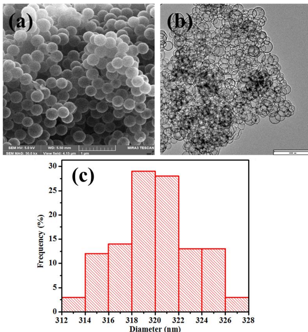
Figure 4.1: SEM micrograph of silica particles (a), TEM micrographs of HCSs (b) and particle size distribution of the HCSs (c).
