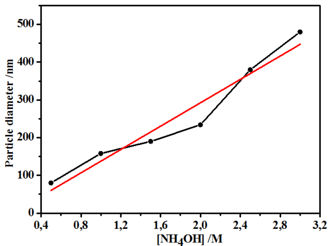
Figure 3.7: Dependence of Silica particle sizes on the concentration of NH 4 OH and at an optimum of the other reagents with TEOS (2 M), DIW (5 M) and EtOH (8 M).
