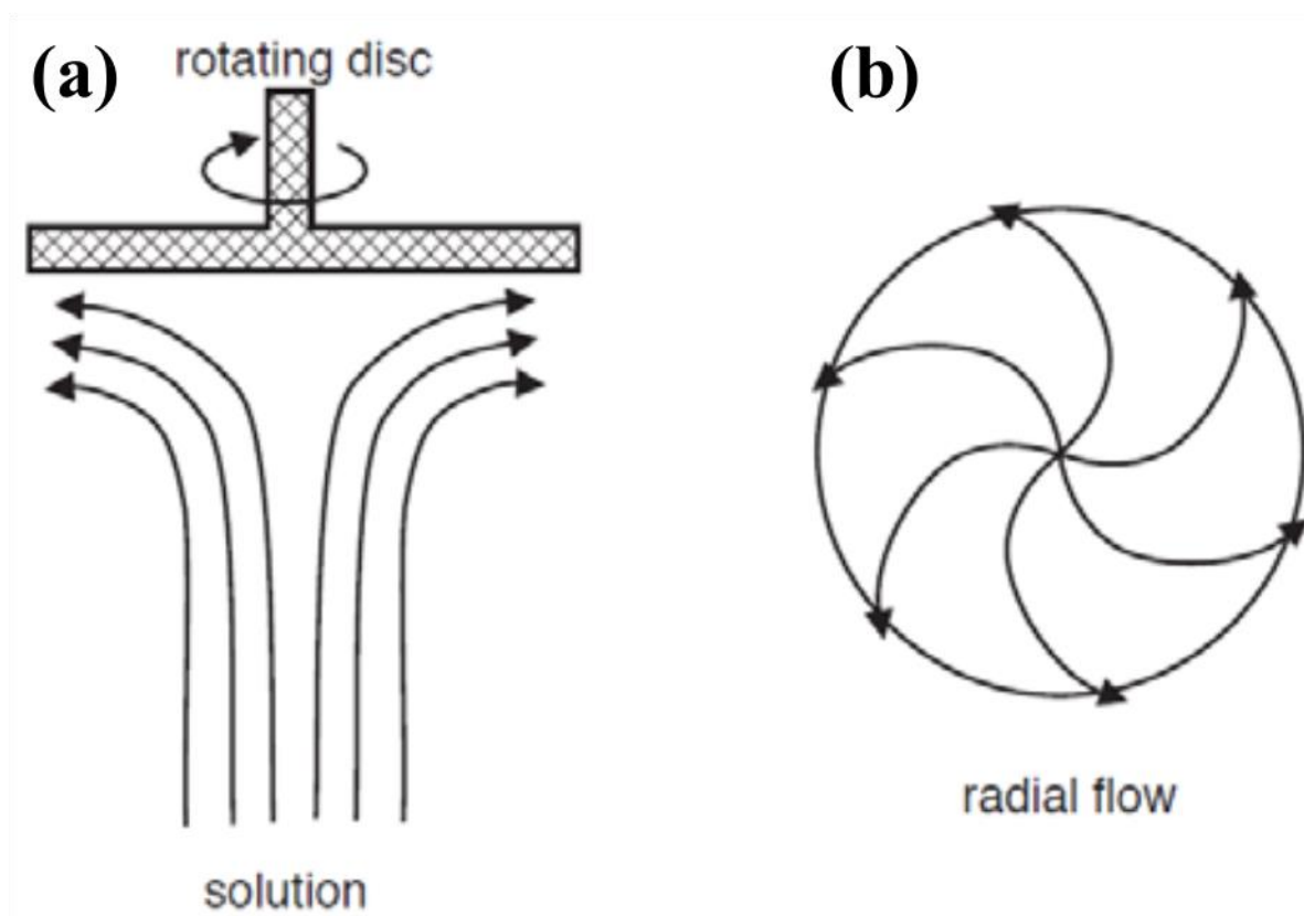
Figure 2.3: (a) Schematic of electrolyte flow towards a RDE surface and (b) electrolyte flow near its surface.
