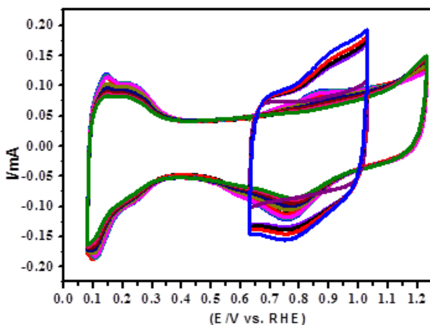
Figure 6. 1: Cyclic voltammograms for ECSA and load cycling (catalyst durability cycle) recorded in 0.1 M HClO 4 (room temperature and in argon saturated electrolyte) for Pt/BHCSs.
