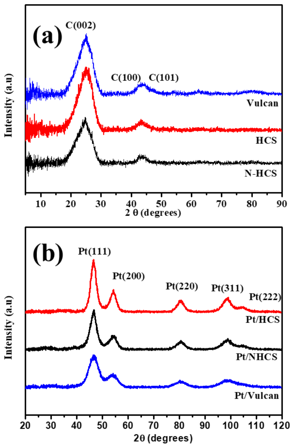
Figure 4.7: (a) PXRD diffractograms for HCSs, NHCSs, Vulcan and (b) for Pt/HCSs, Pt/NHCSs, Pt/Vulcan.
