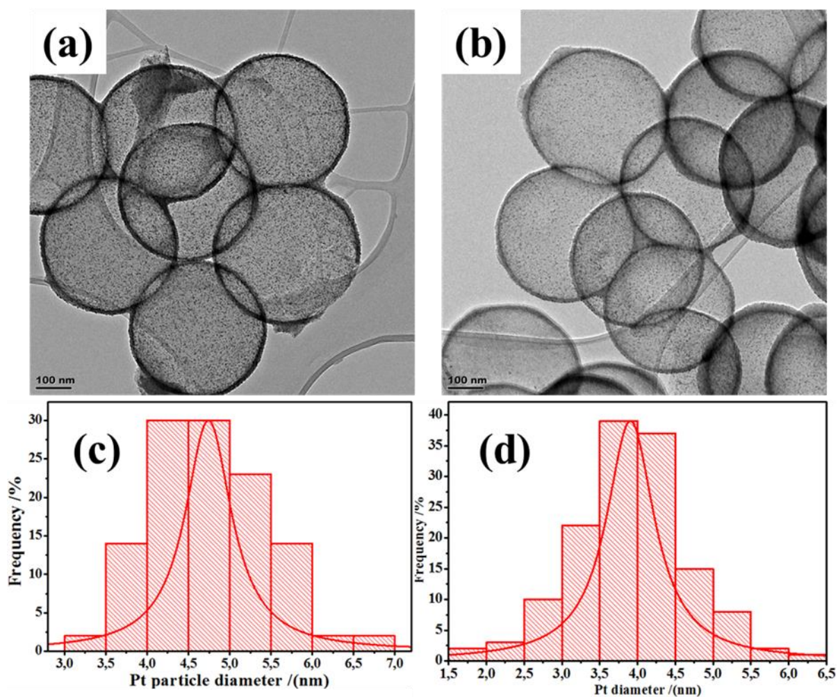
Figure 7.3: TEM image of (a) Pt/HCSs, (b) Pt/NHCSs, (c) particle size distribution of Pt on Pt/HCSs and (d) particle size distribution of Pt on Pt/NHCSs.
