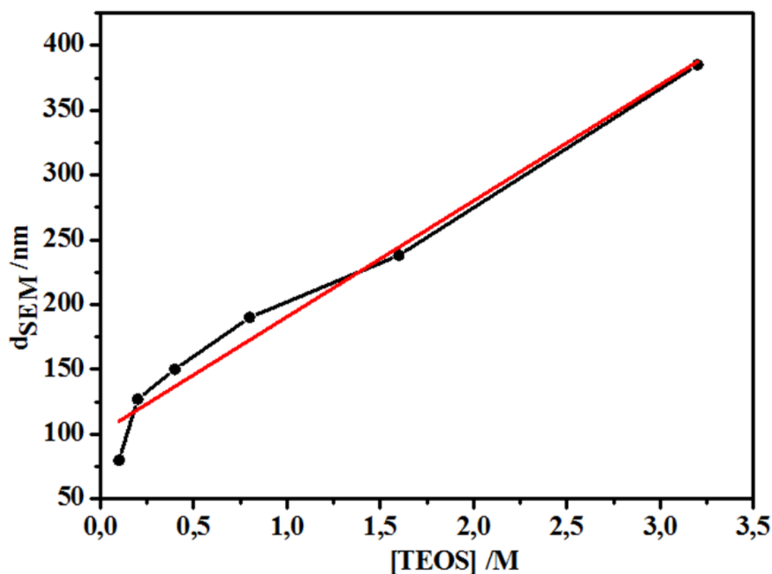
Figure 3.3: Particle size changes of silica particles synthesized with \text{NH}_4\text{OH} (2 M), DIW (5 M), EtOH (8 M) and increasing concentrations of TEOS (a) 0.1 M, (b) 0.2 M, (c) 0.4 M, (d) 0.8 M, (e) 1.6 M, (f) 3.2 M.
