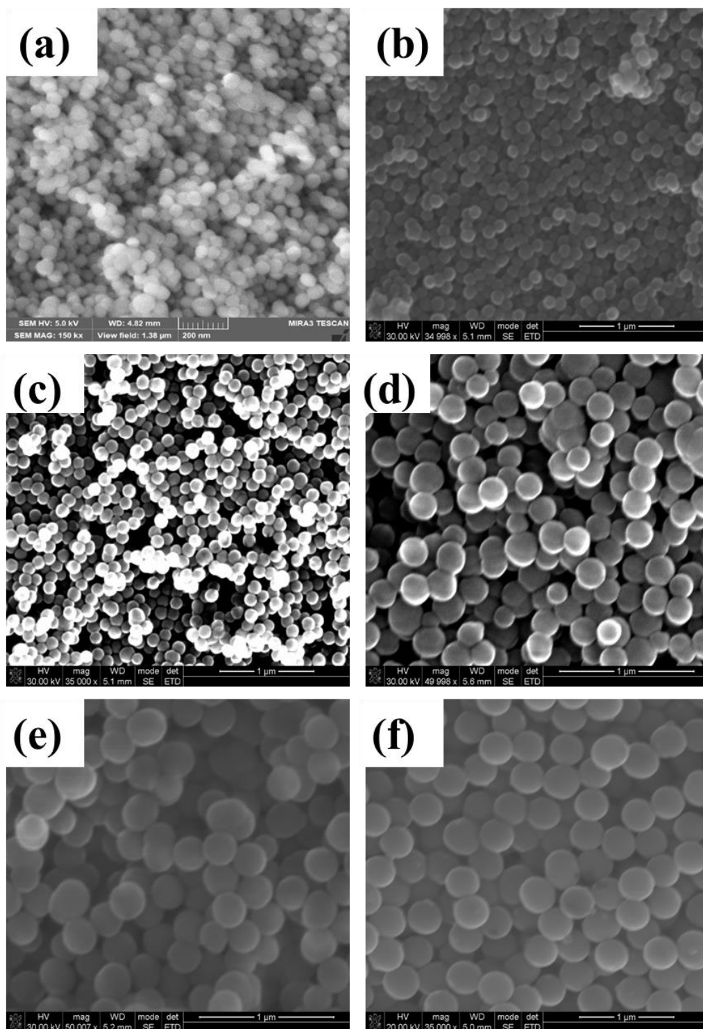
Figure 3.1: SEM images of silica particles synthesized with \text{NH}_4\text{OH} (2 M), DIW (5 M), EtOH (8 M) and increasing concentrations of TEOS (a) 0.1 M, (b) 0.2 M, (c) 0.4 M, (d) 0.8 M, (e) 1.6 M, (f) 3.2 M
