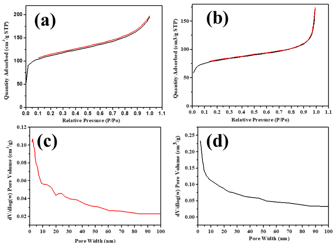
Figure 4. 6: Type II BET isotherm for HCSs (a) and NHCSs (b), Pore size distribution for HCSs (c) and for NHCSs (d)
