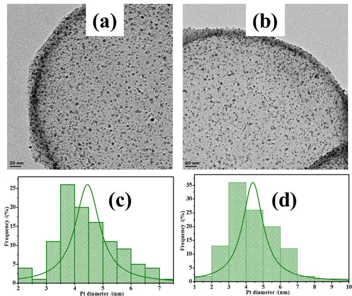
Figure 7.5: After durability study TEM image of (a) Pt/HCSs (b) Pt/NHCSs (c) particle size distribution of Pt on Pt/HCSs (d) particle size distribution of Pt on Pt/NHCSs.
