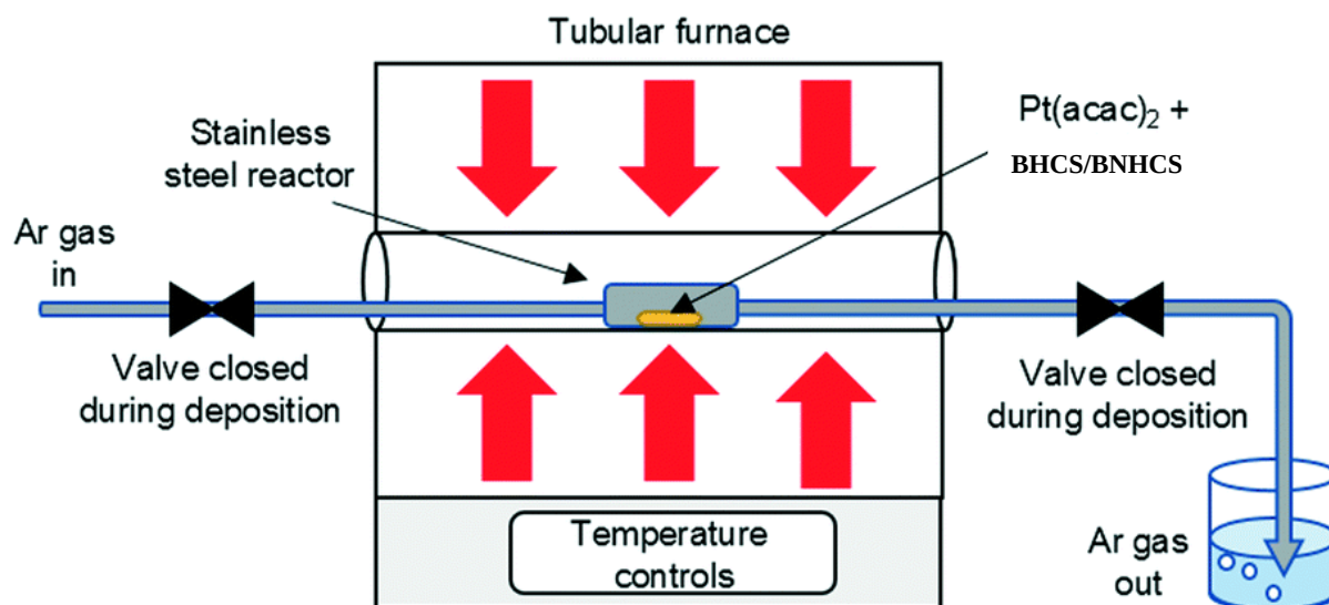
Figure 5.5: Schematic diagram of the metal-organic deposition equipment. 21
