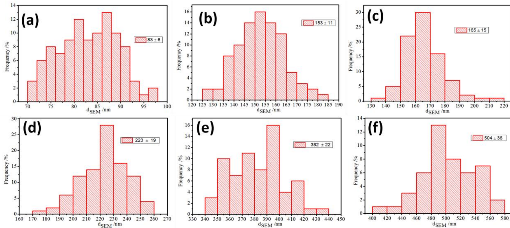
Figure 3.6: Particle size distribution showing variation due to changes in the concentration of NH 4 OH (a) 0.5 M, (b) 1.0 M, (c) 1.5 M, (d) 2.0 M, (e) 2.5 M and 3.0 M and at an optimum of the other reagents with TEOS (2 M), DIW (5 M), EtOH (8 M).
