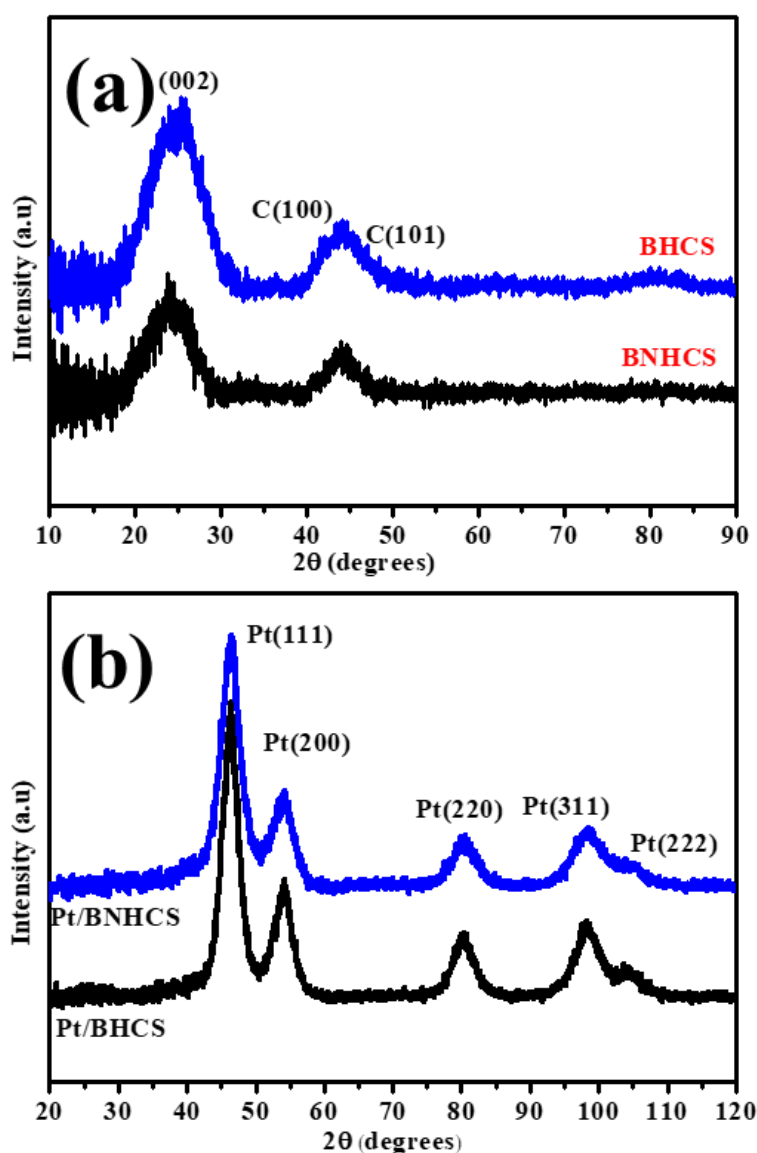
Figure 5.12: PXRD diffractograms of BHCSs and BNHCSs (a), Pt/BHCSs and Pt/BNHCSs (b).
