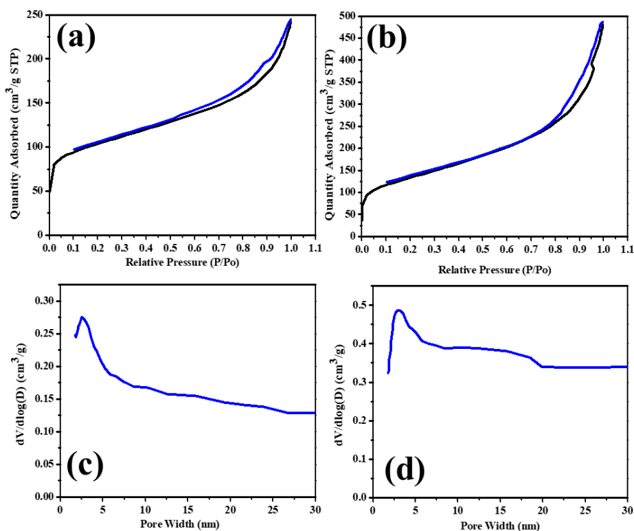
Figure 5.10: BET Isotherms for (a) Pt/BHCSs and (b) Pt/BNHCSs. Pore size distribution for (c) Pt/BHCSs and (d) Pt/BNHCS.
