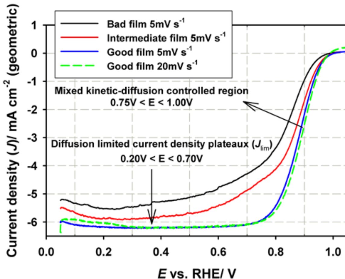
Figure 2.5: ORR polarization profiles for a Pt/C catalyst of different catalyst film quality. 10
