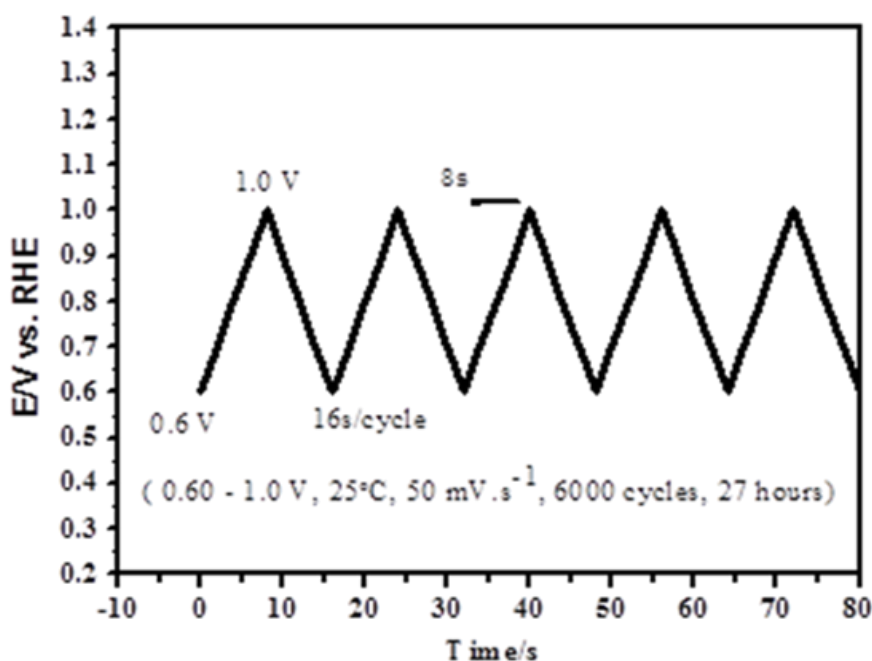
Figure 6.2: Load cycle durability test protocol for the Pt corrosion test.
