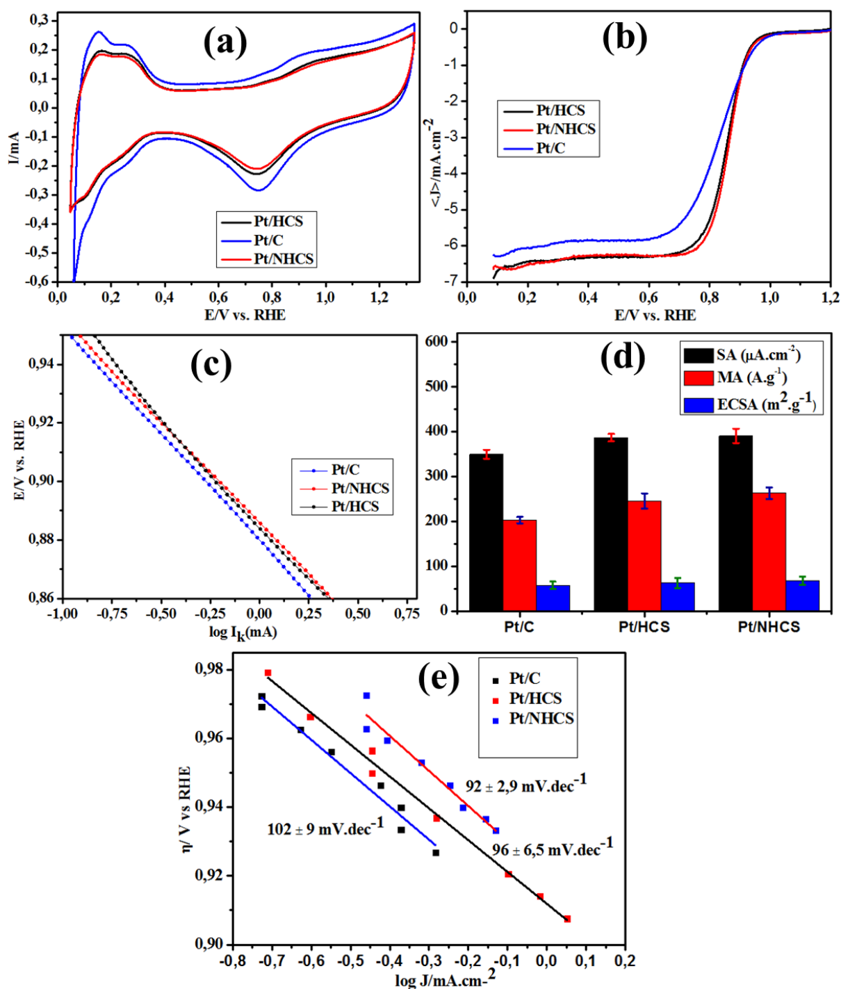
Figure 7.10: The (a) cyclic voltammograms, (b) ORR polarization I-V curves, (c) \log(I_k) Tafel plots and (d) ORR activity and ECSA data for the Pt/HCSs, Pt/NHCSs and the commercial benchmark Pt/C (e) Tafel plots for the three catalysts.
