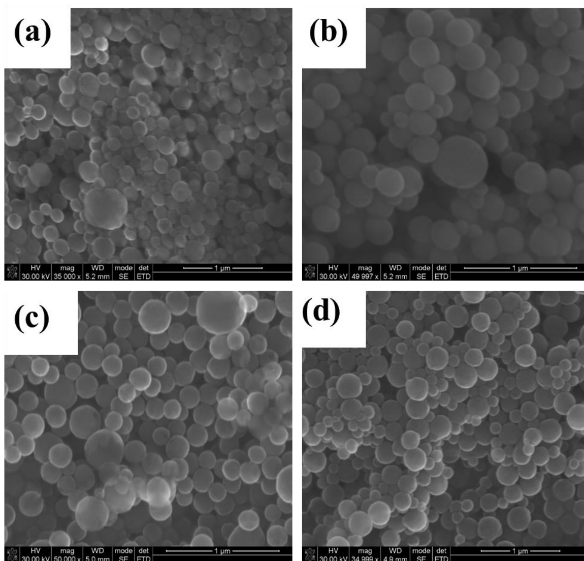
Figure 3. 11: SEM images of polydisperse silica spheres formed with slow addition of TEOS (a) 20 ml.min -1 (b) 30 mil. min -1 (c) 40 mil.min -1 (d) 50 mil.min -1 using a syringe pump.
