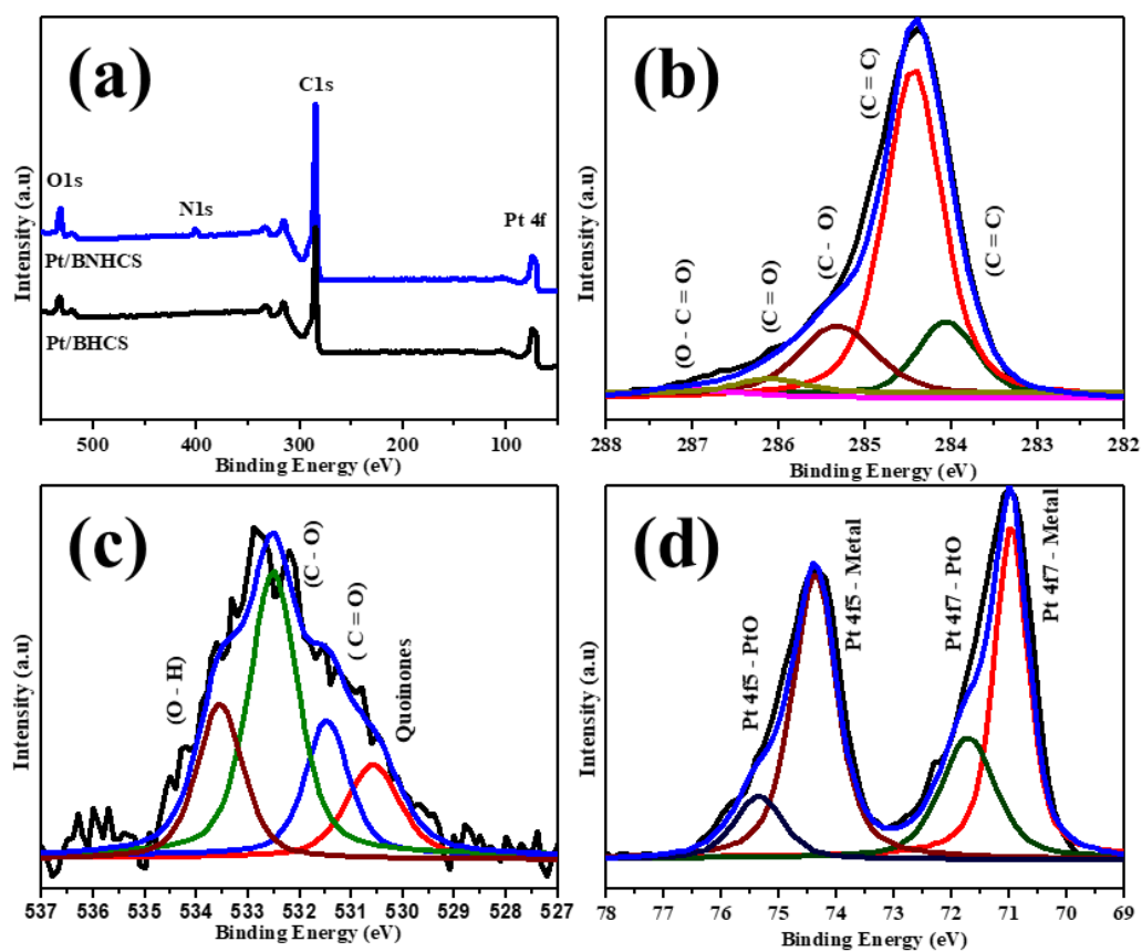
Figure 5.13: XPS surveys for (a) Pt/BHCSs and Pt/BNHCSs. High resolution (b) C1s, (c) O1s and (d) Pt4f spectra for Pt/BHCSs.
