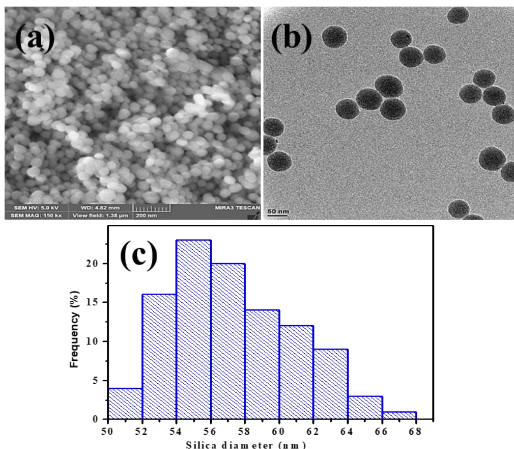
Figure 5.1: (a) SEM micrograph, (b) TEM micrograph of SiO 2 and (c) particle size distribution of the small silica particles.
