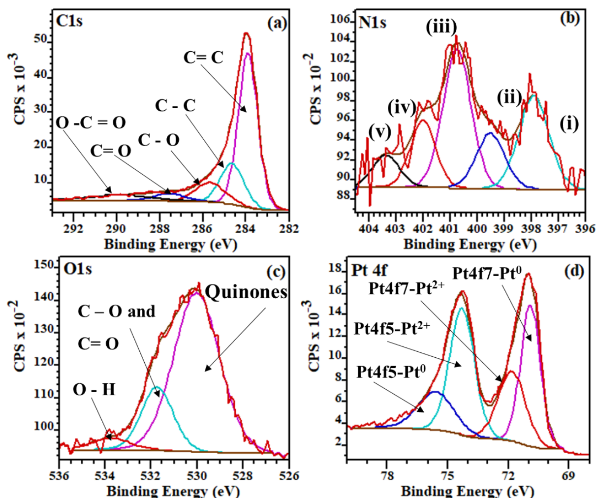
Figure 7. 9: Deconvoluted high resolution XPS spectra for Pt/NHCSs (a) C1s, (b) N1s (c) O1s and (d) Pt 4f.
