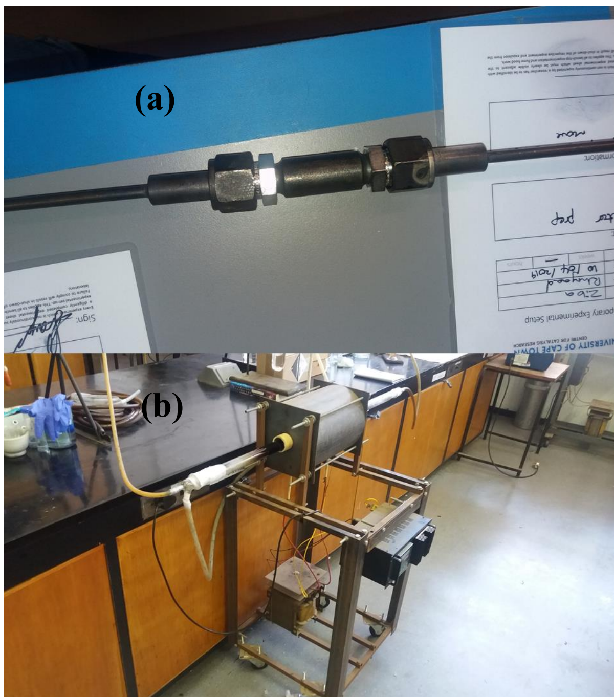
Figure 2.1: Steel cylindrical reactor (a), Horizontal tubular furnace used for Pt deposition, carbonization of \text{SiO}_2\text{@RF} and annealing of HCSs and NHCSs (b).
