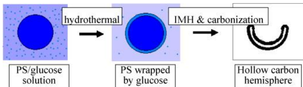
Figure 1.15: Schematic illustration of the synthesis procedure of the HCHs. 138
