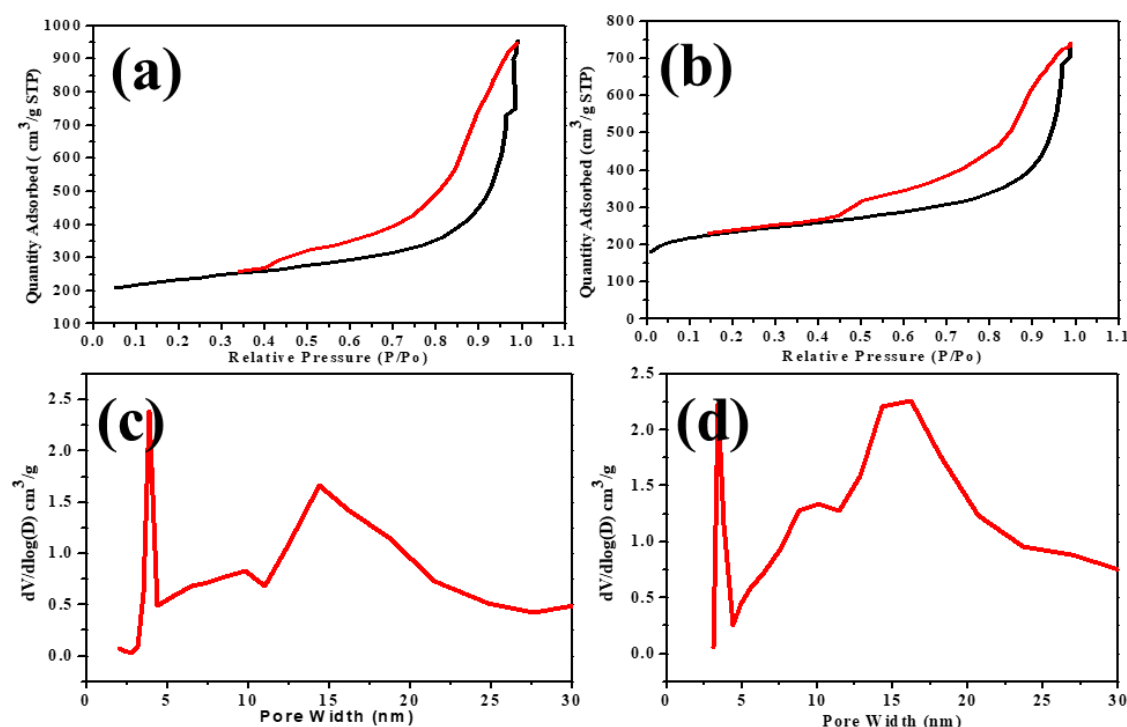
Figure 5.9: BET Isotherms for (a) BHCSs and (b) BNHCSs. Pore size distribution for (c) BHCSs and (d) BNHCSs.
