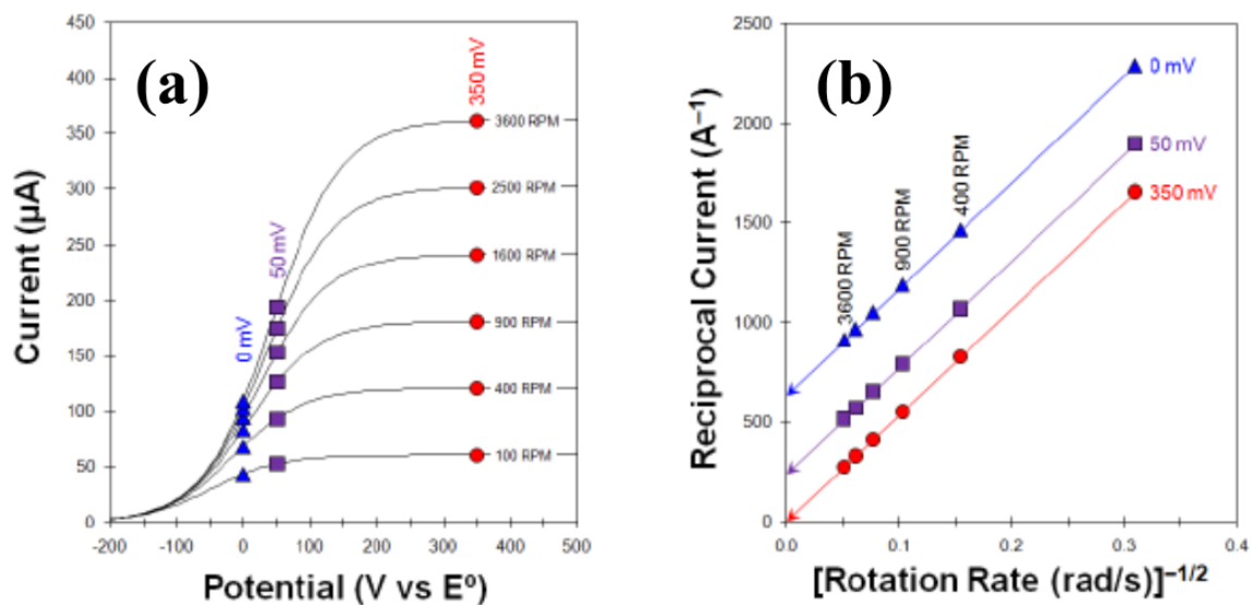
Figure 2.4: (a) Linear sweep voltammograms at various rpm and (b) Koutecky-Levich plot for three different overpotentials. 17
