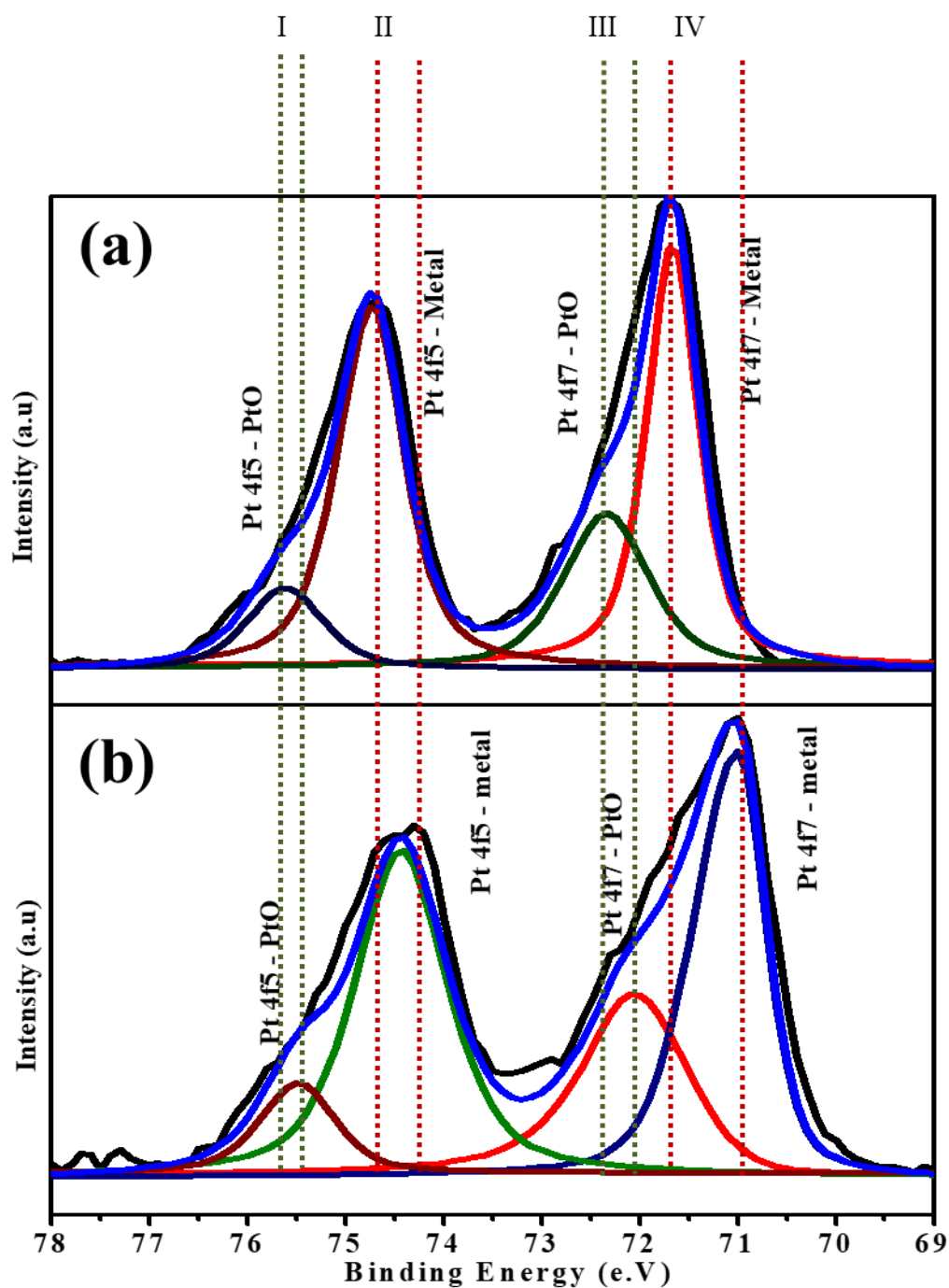
Figure 5.15: Stacked deconvoluted Pt4f XPS spectra for (a) Pt/BHCSs and (b) Pt/BNHCSs showing binding energy shifts.
