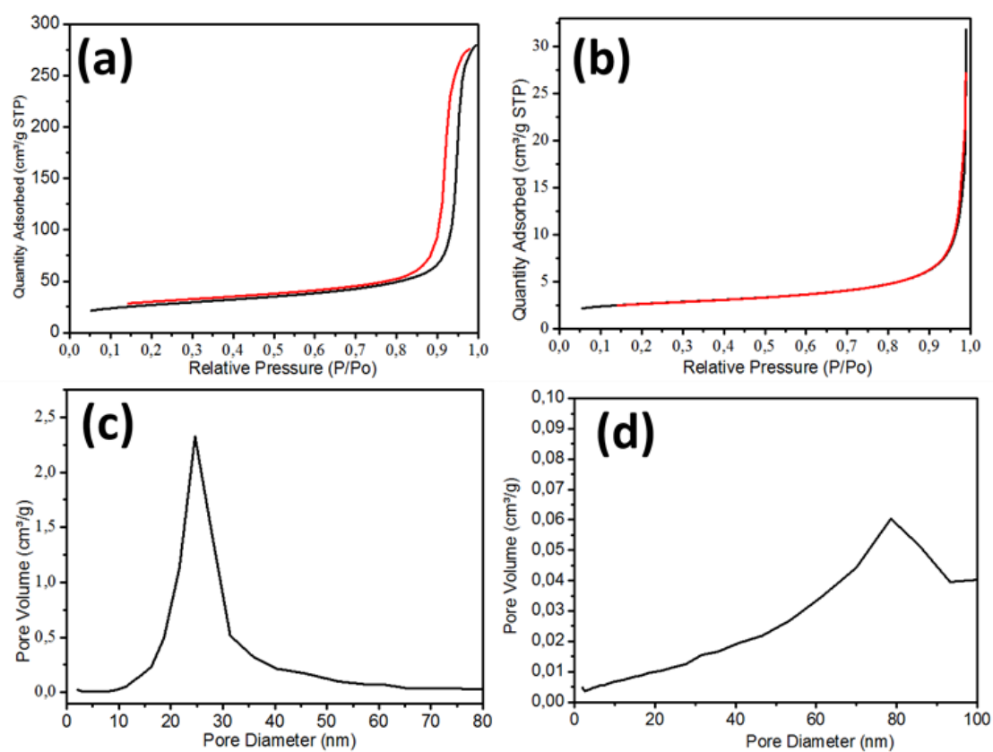
Figure 3. 14: BET properties of the formed silica at varying DI concentrations.
