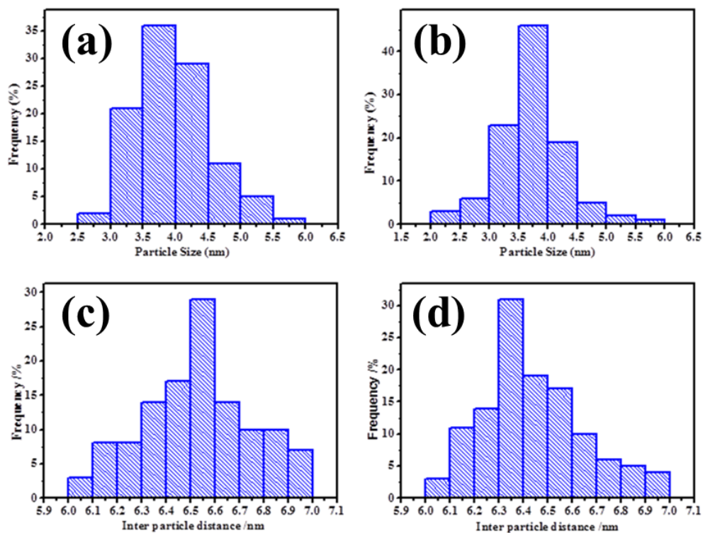
Figure 5.8: Pt particle size distribution of (a) Pt/BHCSs and (b) Pt/BNHCSs. Pt – Pt interparticle distance of (c) Pt/BHCSs and (d) Pt/BNHCSs.
