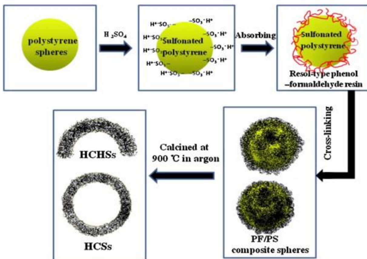
Figure 1.17 : Schematic of the preparation of hollow carbon hemispheres (HCHS). 139
