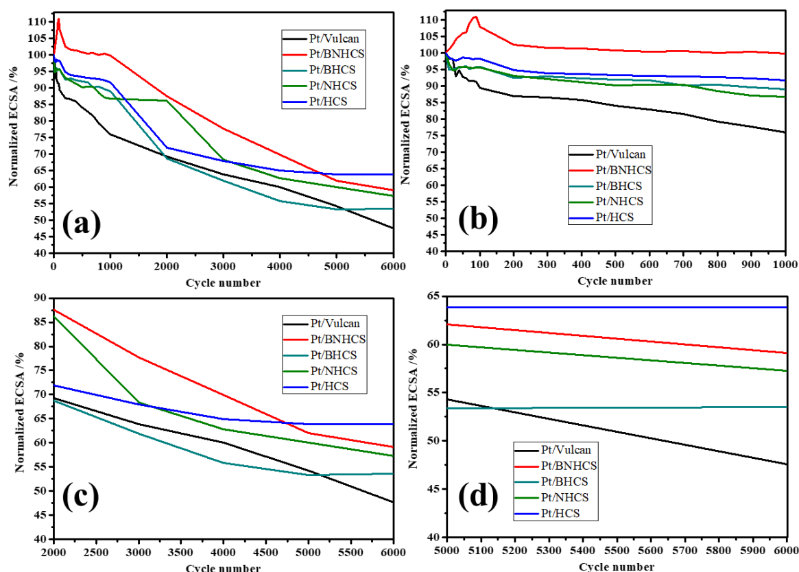
Figure 6.7: Catalyst durability study showing the change in normalized ECSA (a) from BOL to 6000 cycles, (b) From BOL to 1000 cycles, (c) from 2000 to EOL (end of life – 6000 cycles) and (d) from the 5000 th to the end of life (EOL) 6000 th cycle.
