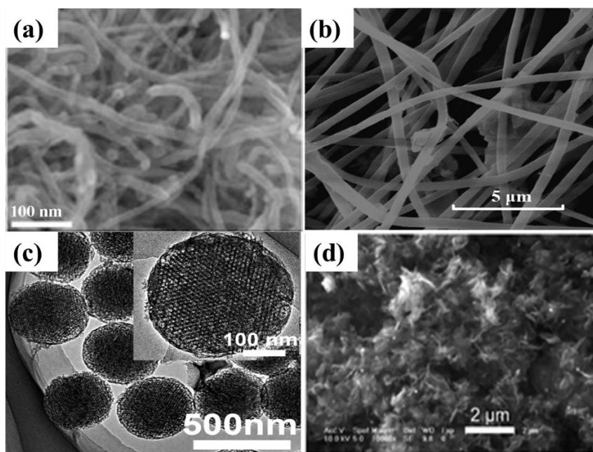
Figure 1.8: SEM images of some of the carbon materials that have been used in catalysis either as supports or as catalysts themselves: (a) carbon nanotubes, (b) carbon nanofibers, (c) solid carbon spheres and (d) graphene sheets. 119-122
