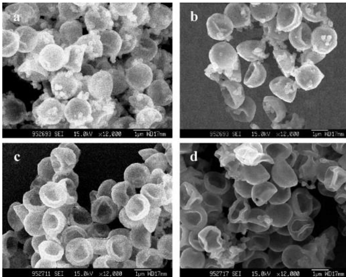
Figure 1.16: SEM micrograms of the HCHs with the mass ratios of PSs to glucose were (a) 1:4, (b) 1:3, (c) 1:2 and (d) 1:1. 138
