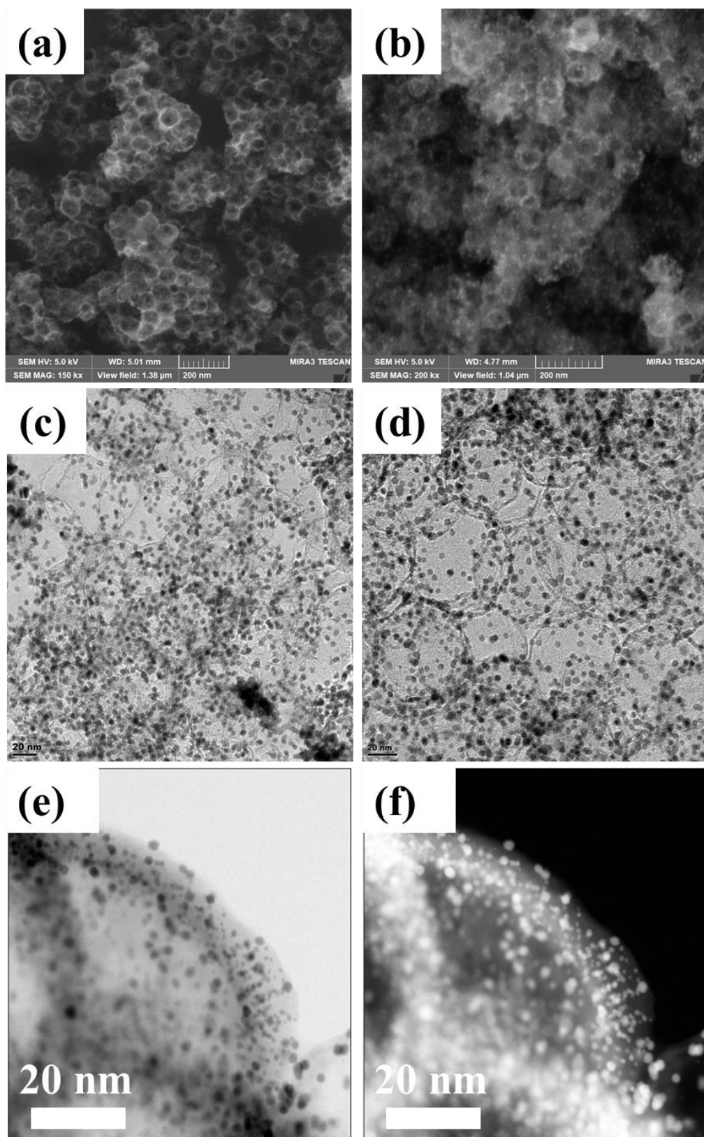
Figure 5.6: SEM micrographs of (a) Pt/BHCSs, (b) Pt/BNHCSs, TEM micrographs of (c) Pt/BHCSs, (d) Pt/BNHCSs, ADF-BF STEM images of (e-f) Pt/BNHCSs.
