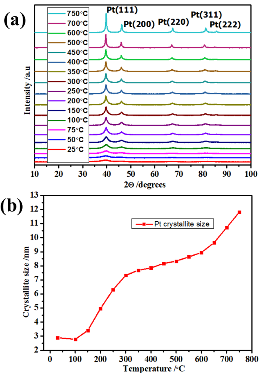
Figure 6.12: Variable temperature PXRD diffractograms for commercial Pt/C (a) and the corresponding variable temperature dependent Pt crystallite growth (b). See Table 6.8: In-situ PXRD Pt crystallite size change due to the variable temperature for Pt/BHCSs.
