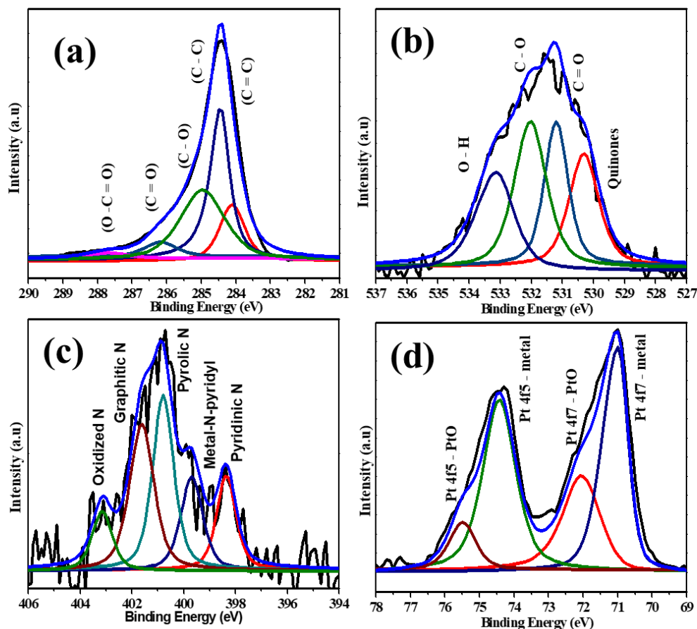
Figure 5.14: Deconvoluted high resolution (a) C1s, (b) O1s, (c) N1s and (d) Pt4f spectra for Pt/BNHCSs.
