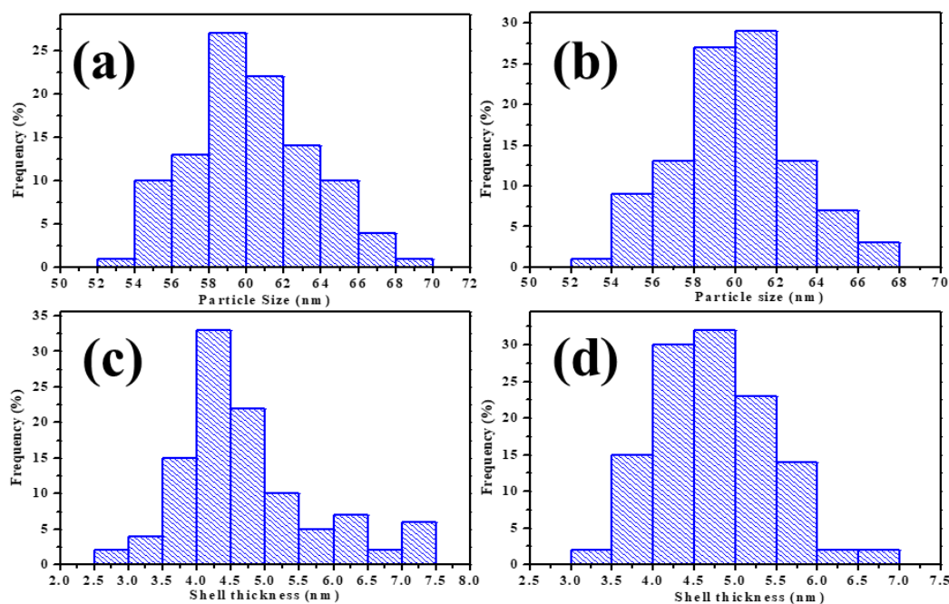
Figure 5.3: (a) Particle size distribution of BHCSs and (b) BNHCSs. Shell thickness of (c) BHCSs and (d) BNHCSs.
