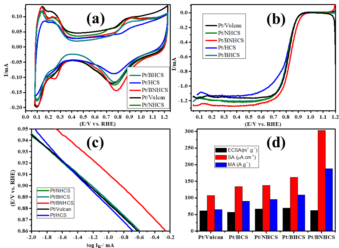
Figure 6.5: Electrocatalysis characterization data for the 40 wt% catalysts showing (a) Cyclic voltammograms, (b) ORR polarization I-V curves, (c) Tafel plots and (d) Mass specific (MA), area specific (SA) activities and electrochemical surface area (ECSA).
