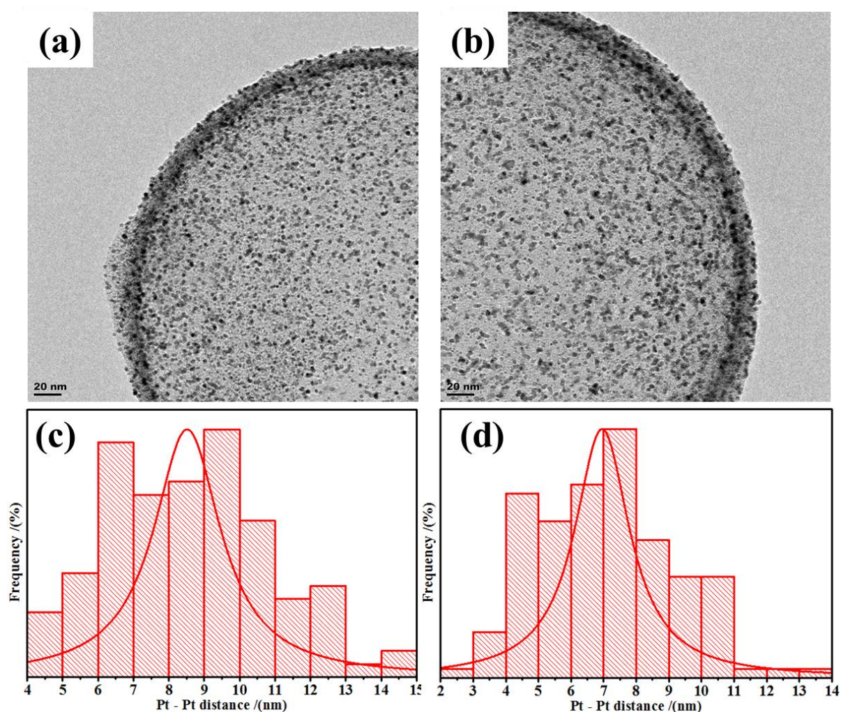
Figure 7.4: TEM image of (a) Pt/HCSs (b) Pt/NHCSs (c) Pt – Pt interparticle distance of Pt/HCSs (d) Pt – Pt interparticle distance of Pt/NHCSs.
