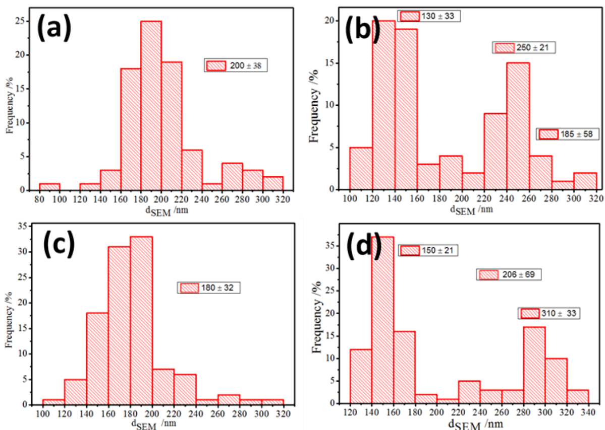
Figure 3.12: Particle size distributions of polydisperse silica spheres formed with slow addition of TEOS (a) 20 ml.min -1 (b) 30 ml.min -1 (c) 40 ml.min -1 (d) 50 ml.min -1 using a syringe pump.
