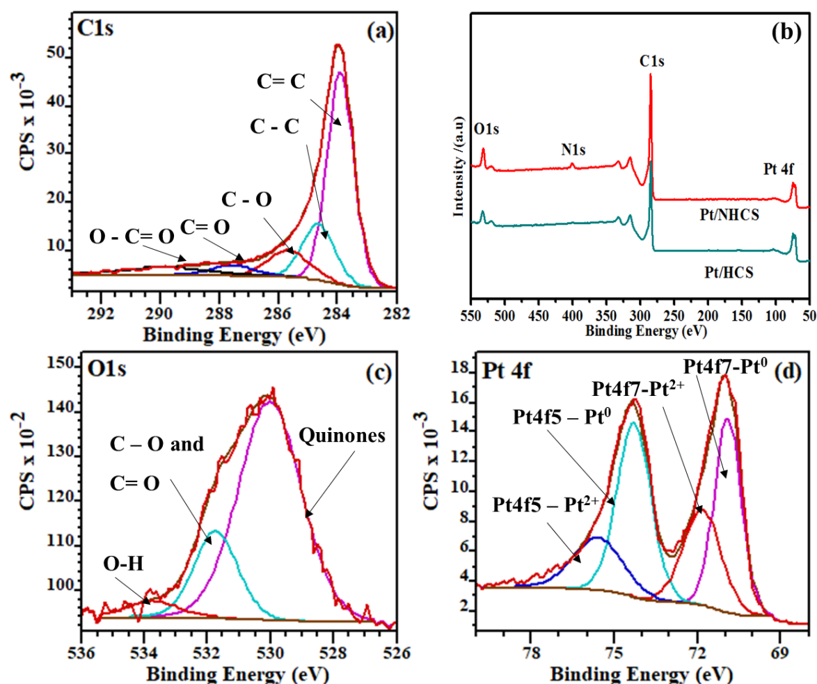
Figure 7.8: Deconvoluted high resolution XPS spectra for Pt/HCSs (a) C1s, (b) low resolution surveys of Pt/HCS and Pt/NHCS (c) O1s and (d) Pt 4f.
