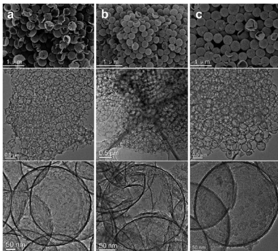
Figure 1.12: SEM and TEM images of NHCS synthesized using different ratios of silica and ionic liquid [\text{C}_{16}\text{Mim}]\text{Br} (a – c) 136
