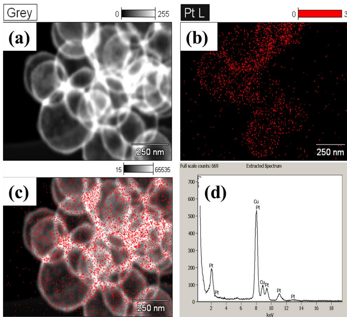
Figure 6.11: (a) DF-STEM images of Pt/HCSs showing the bright edges of the HCSs support due to Pt. (b) and (c) Pt map showing location of Pt in the shell region of the support. (d) EDX showing the presence of Pt on the supports, the copper is due to the copper grid used for analysis.
