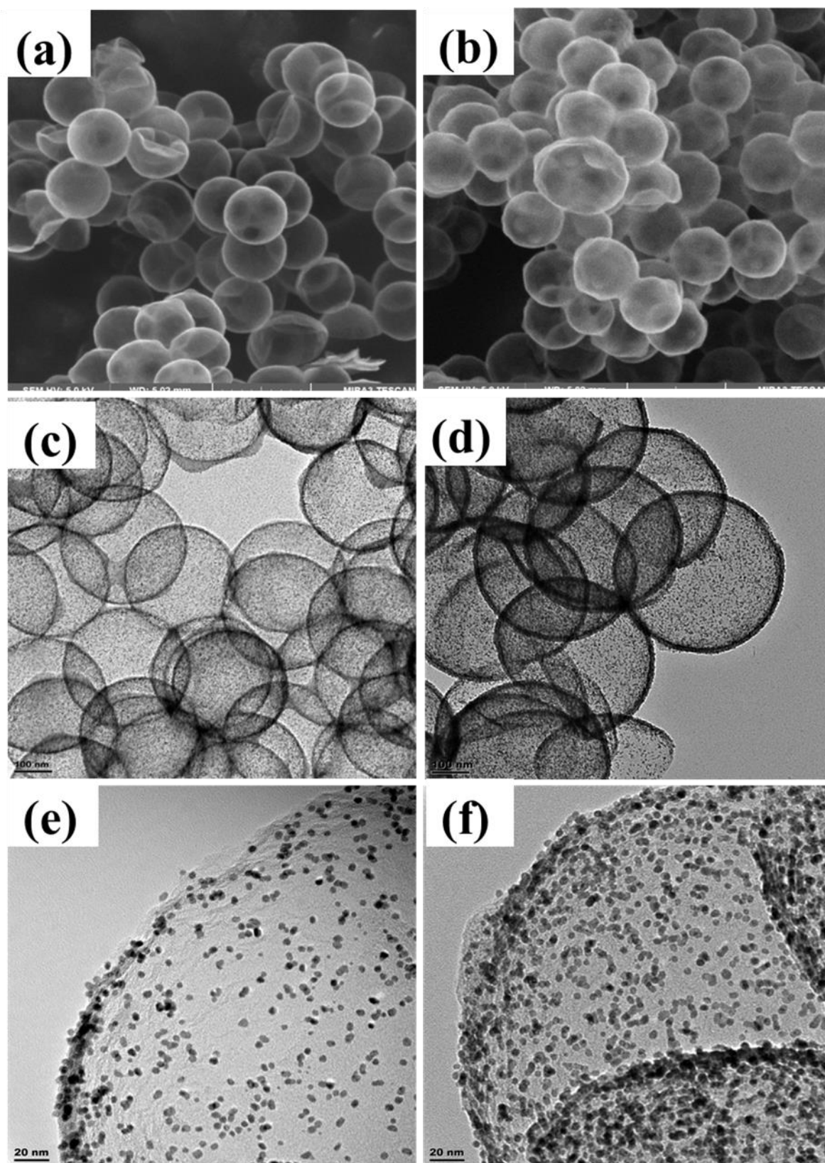
Figure 4.3: SEM image of Pt/HCSs (a), SEM image of Pt/NHCSs (b), TEM image of Pt/HCSs (c), TEM image of Pt/NHCSs (d), higher magnification TEM image of Pt/HCSs (e) and higher magnification TEM image of Pt/NHCSs (f).
