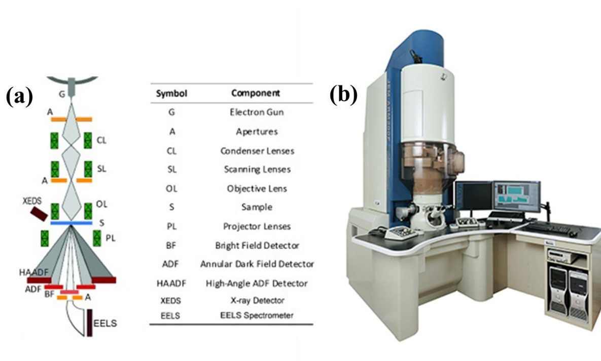
Figure 2.14: The schematic of the mode of operation of a STEM microscope (a) 34 and A JEOL ARM200F scanning transmission electron microscope (b).
