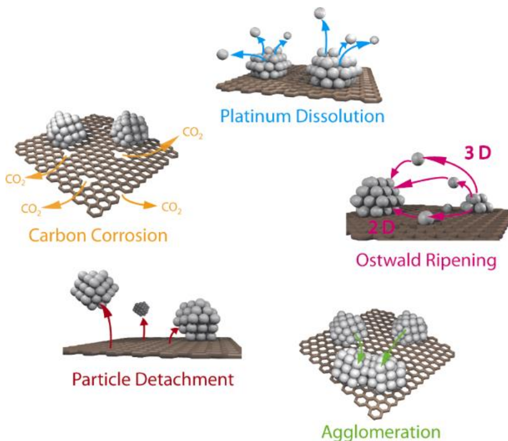
Figure 1.7: Schematic illustrations of the proposed mechanisms of degradation of Pt/C catalysts. 102
