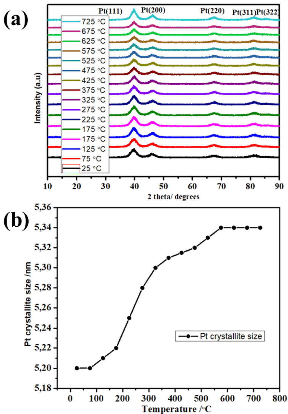
Figure 6.8: Variable temperature PXRD diffractograms for Pt/BHCSs (a) and the corresponding variable temperature dependent Pt crystallite growth (b). See Table 6.7: In-situ PXRD Pt crystallite size changes due to the variable temperature for Pt/BHCSs.
