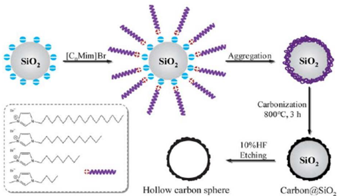
Figure 1.11: Schematic illustration of the formation of NHCSs using silica and ionic liquids. 136
