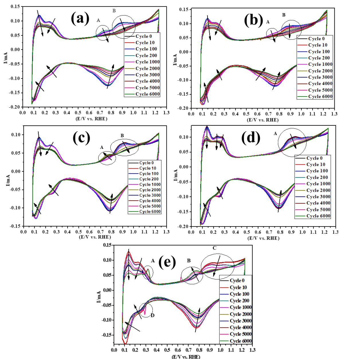
Figure 6.6: Durability cyclic voltammograms from beginning of life (BOL) to 6000 cycles showing the change in the structure due to the accelerated degradation for (a) Pt/HCS, (b) Pt/NHCS and (c) Pt/BHCSs, (d) Pt/BNHCSs and (e) the commercial benchmark Pt/Vulcan catalyst. Cycling was done between 0.6 – 1.0 V vs RHE at 20 \text{ mV.s}^{-1} and at room temperature ( 25^\circ\text{C} ).
