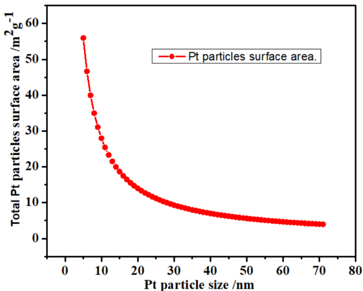
Figure 6.3: Theoretical total Pt surface area (MSA) as calculated using the density of Pt, assuming uniform spherical morphology and a given particle diameter.
