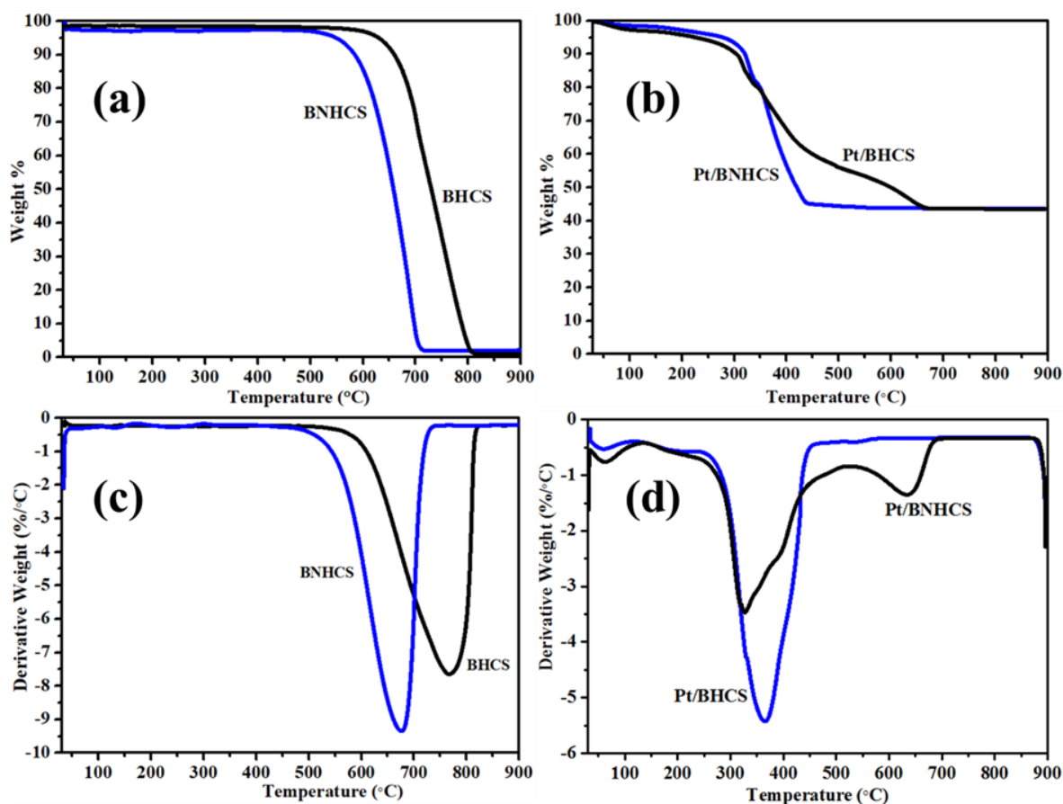
Figure 5.11: TGA profile for (a) BHCSs and BNHCSs, (b) Pt/BHCSs and Pt/BNHCSs. DTA profiles for (c) BHCSs and BNHCSs, (d) Pt/BHCSs and Pt/BNHCSs.
