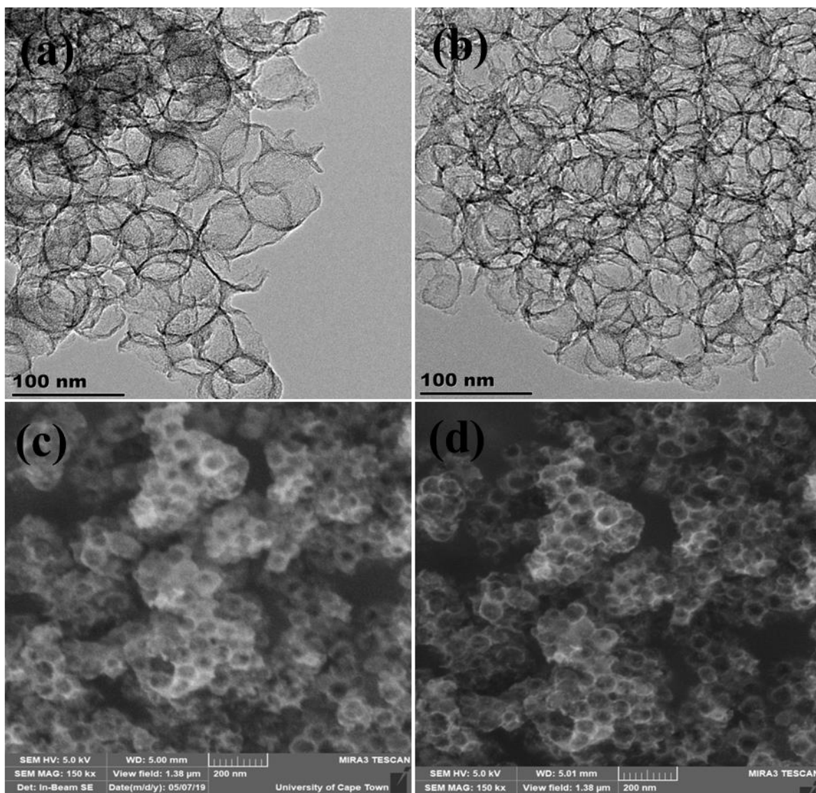
Figure 5.2: (a) TEM micrograph for BHCSs and (b) BNHCSs. (c) SEM micrograph of BHCSs and (d) BNHCSs.
