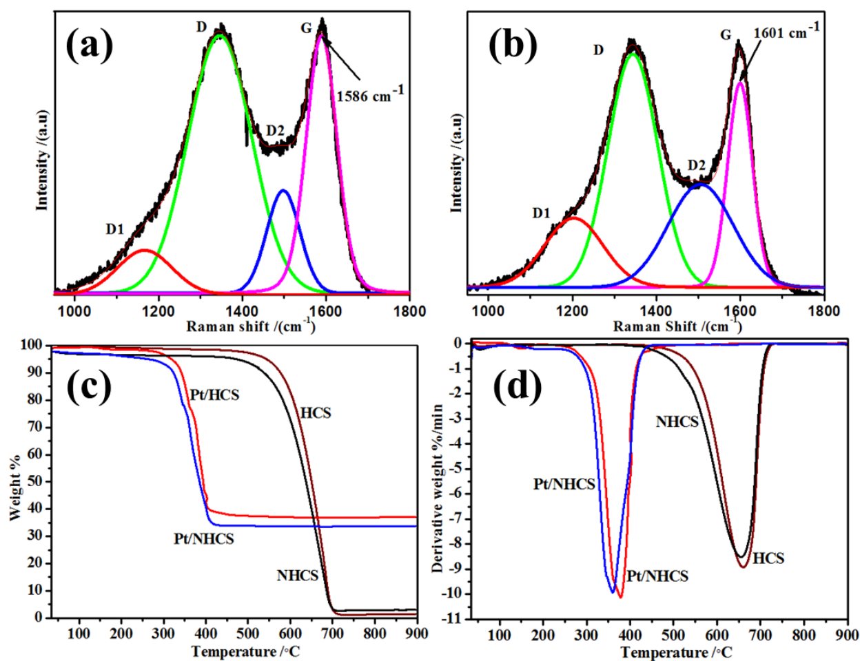
Figure 7.2: Raman spectra of HCSs (a) Raman spectra of NHCSs (b) TGA profiles of HCSs, NHCSs, Pt/HCSs and Pt/NHCSs (c) TGA derivative profiles of HCSs, NHCSs, Pt/HCSs and Pt/NHCSs.
