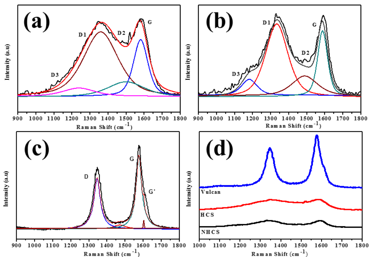
Figure 4.2: Deconvoluted Raman spectra of (a) HCSs, (b) NHCSs, (c) Vulcan carbon and (d) stacked Raman spectra for all supports showing the different G peak positions.
