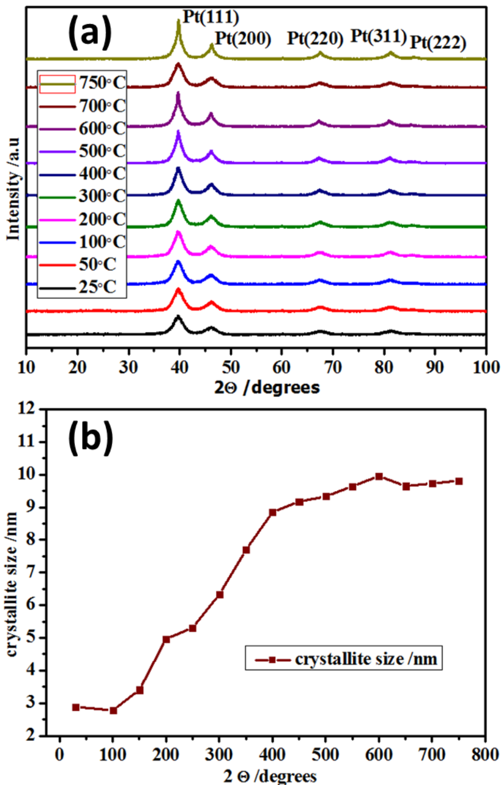
Figure 6.10: Variable temperature PXRD diffractograms for commercial Pt/HCS (a) and the corresponding variable temperature dependent Pt crystallite growth (b). See Table 6.8: In-situ PXRD Pt crystallite size change due to the variable temperature for Pt/BHCSs.
