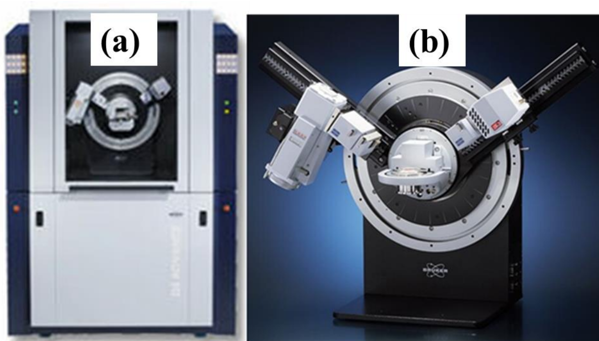
Figure 2.7: D8 Advanced diffractometer (a), Internal components of an X-ray diffractometer (b)
