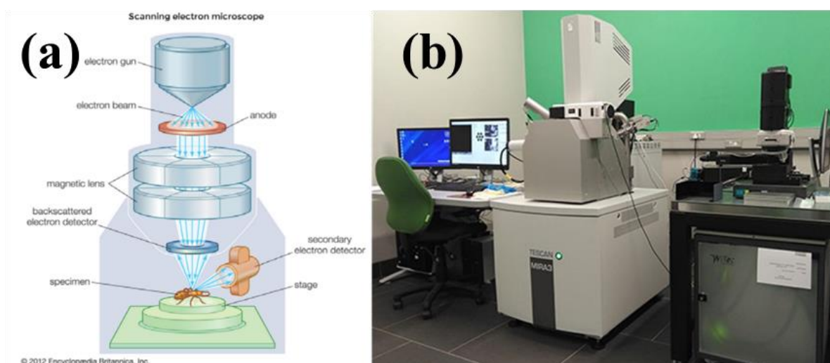
Figure 2.9: (a) Schematic of a SEM and (b)Tescan MIRA3 RISE scanning electron microscope. 23
