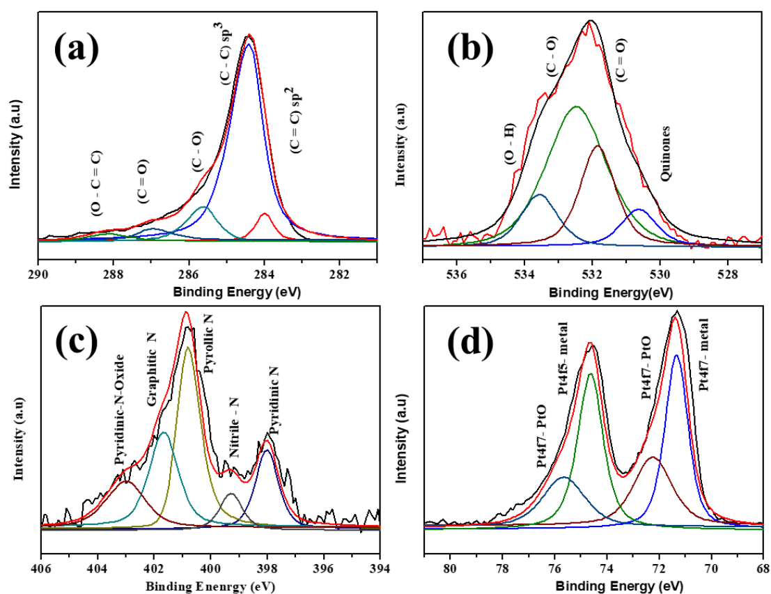
Figure 4.9: High resolution (a) C1s, (b) O1s, (c) N1s and (d) Pt4f spectra for Pt/NHCSs.
