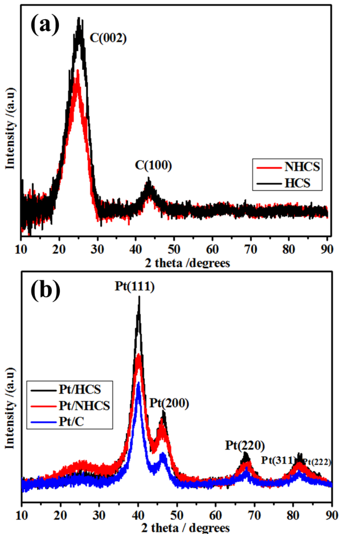
Figure 7.7: PXRD diffractograms of (a) HCSs and NHCSs, (b) Pt/HCSs and Pt/NHCSs.
