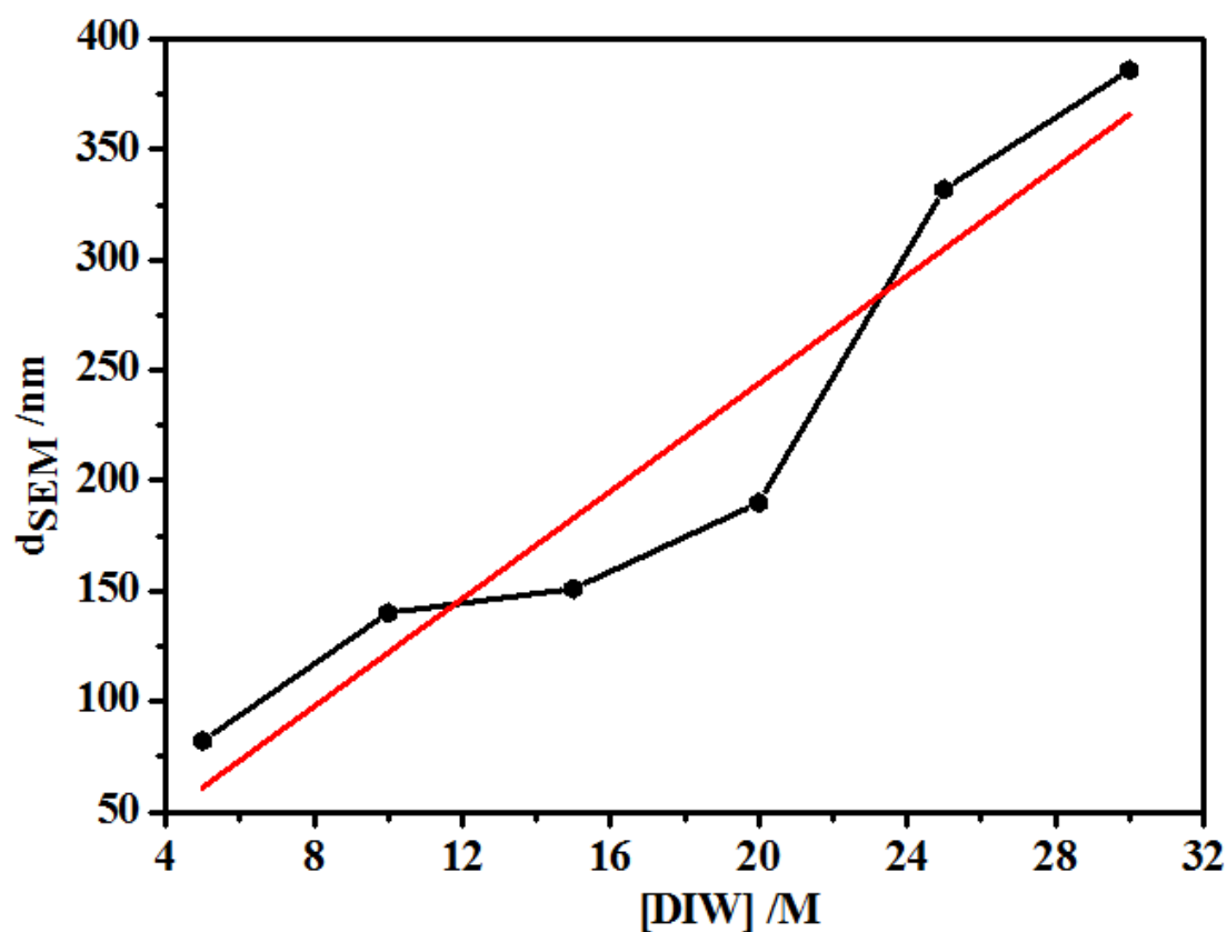
Figure 3.10: Changes in the silica particle size due to the variation of the deionized water concentration was varied from 5 - 30 M at optimum concentration of NH_4OH (2 M), TEOS (2 M), EtOH (8M).
