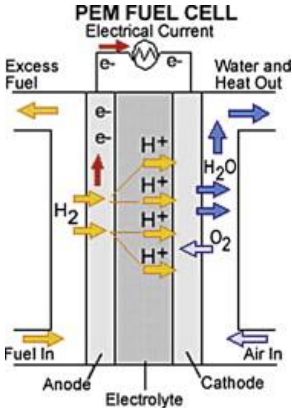
Figure 1.5: Schematic illustration of a PEMFC. 54
