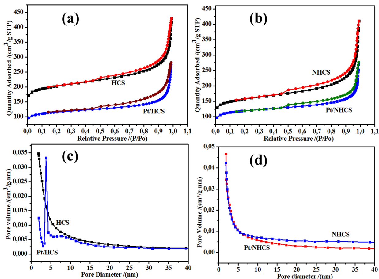
Figure 7.6: BET isotherms for (a) HCSs and Pt/HCSs and (b) NHCSs and Pt/NHCSs. Pore size distribution plots for (c) HCSs and Pt/HCSs and (d) NHCSs and Pt/NHCSs.
