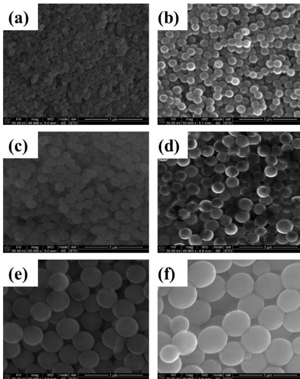
Figure 3.5: SEM images of the silica spheres formed at an optimum of the other reagents with TEOS (2 M), DIW (5 M), EtOH (8 M) and various ammonia concentrations of \text{NH}_4\text{OH} (a) 0.5 M, (b) 1.0 M, (c) 1.5 M, (d) 2.0 M, (e) 2.5 M and 3.0 M.
