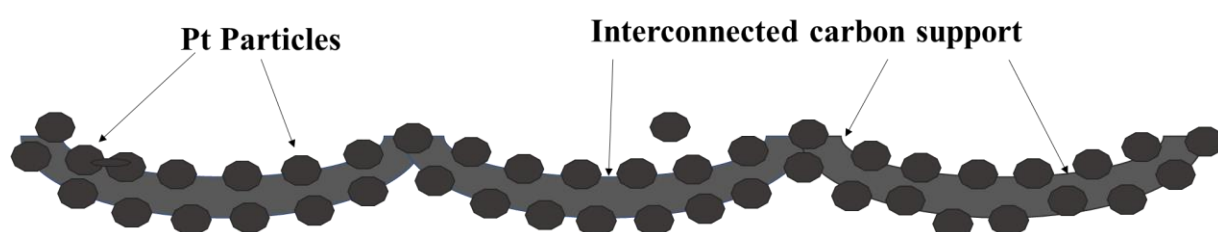
Figure 6.4: Schematic illustration of the Pt nanoparticles supported on top and inside pores of interconnected broken bowl like and broken bowl like nitrogen doped hollow carbon spheres.
