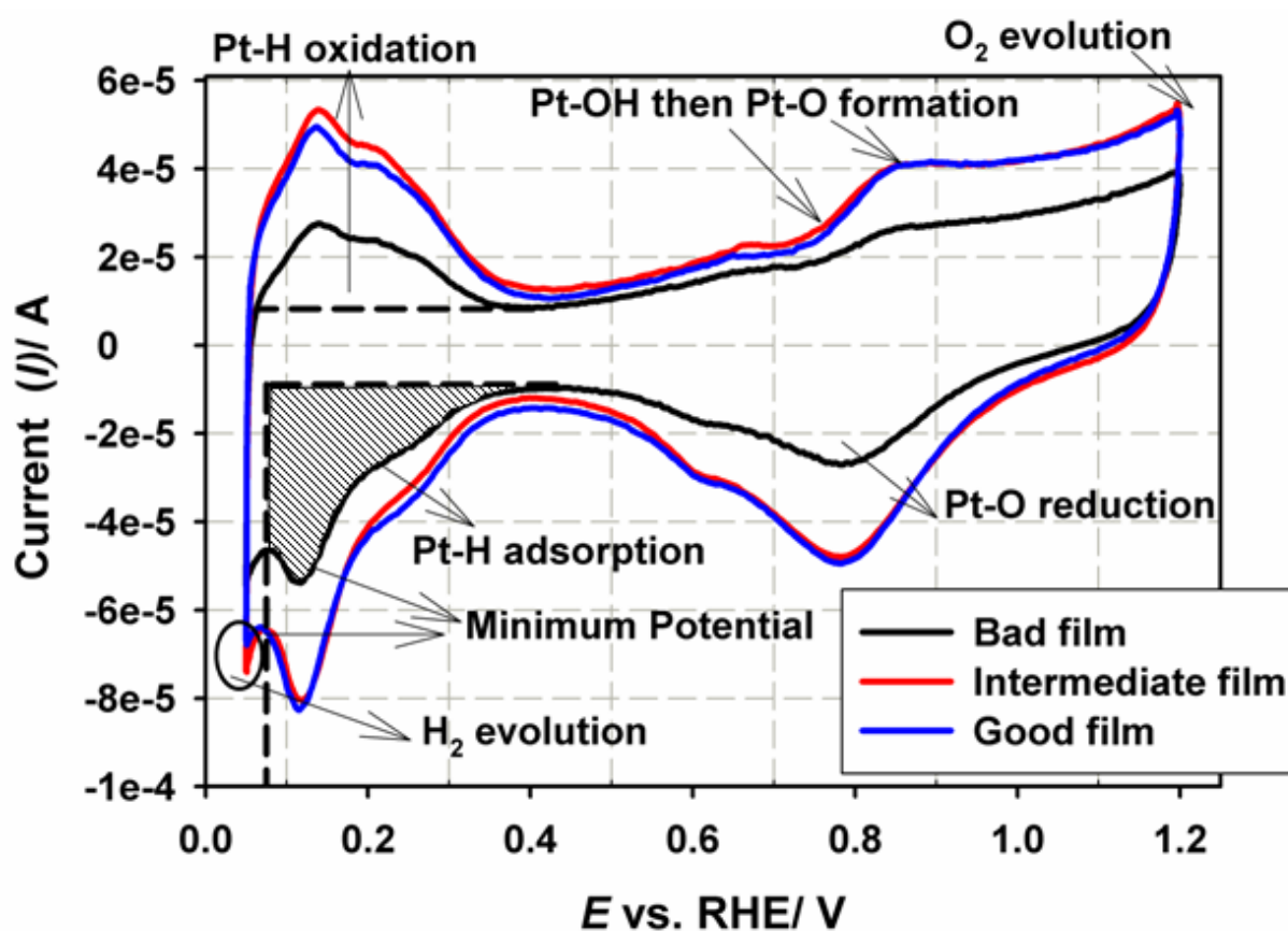
Figure 2.2: Cyclic voltammograms of a Pt/C catalyst of various catalyst film quality. 10
