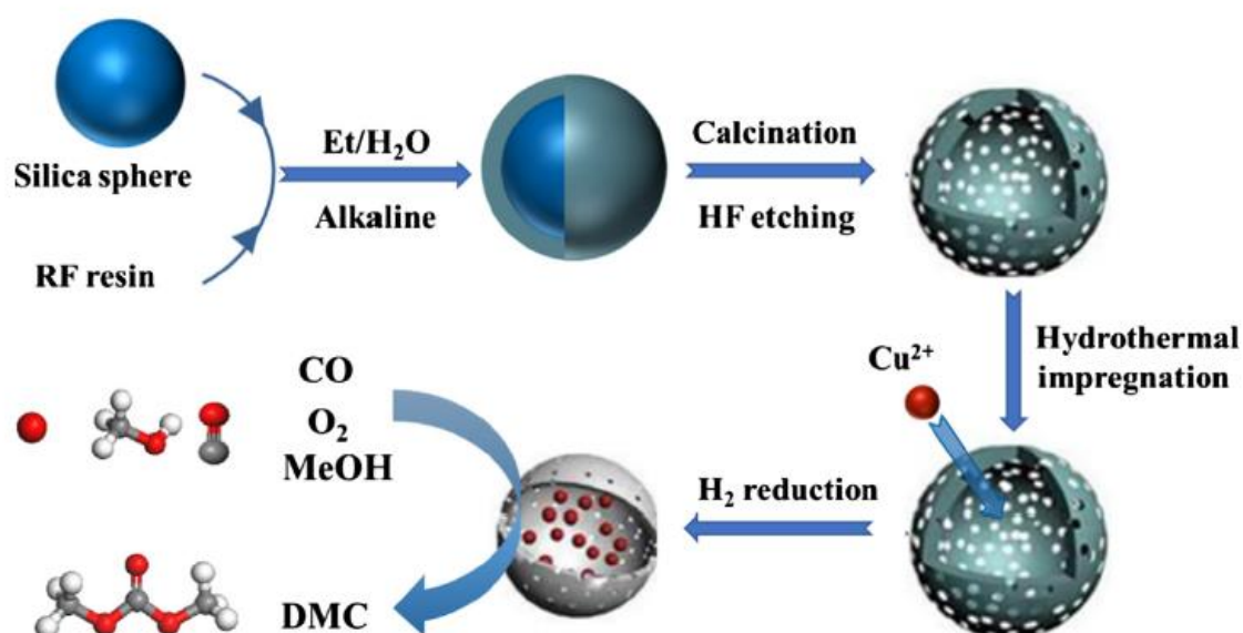
Figure 1.9: Schematic illustration of the encapsulation of Cu inside HCSs to form Cu@HCS. 126
