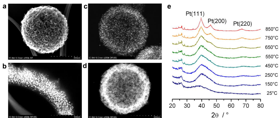
Figure 1.6: (a) to (d) are DF-STEM images showing pore confined Pt in the hollow carbon supports and (e) variable temperature in-situ PXRD diffractograms for a Pt/C catalyst confirming pore confinement. 72
