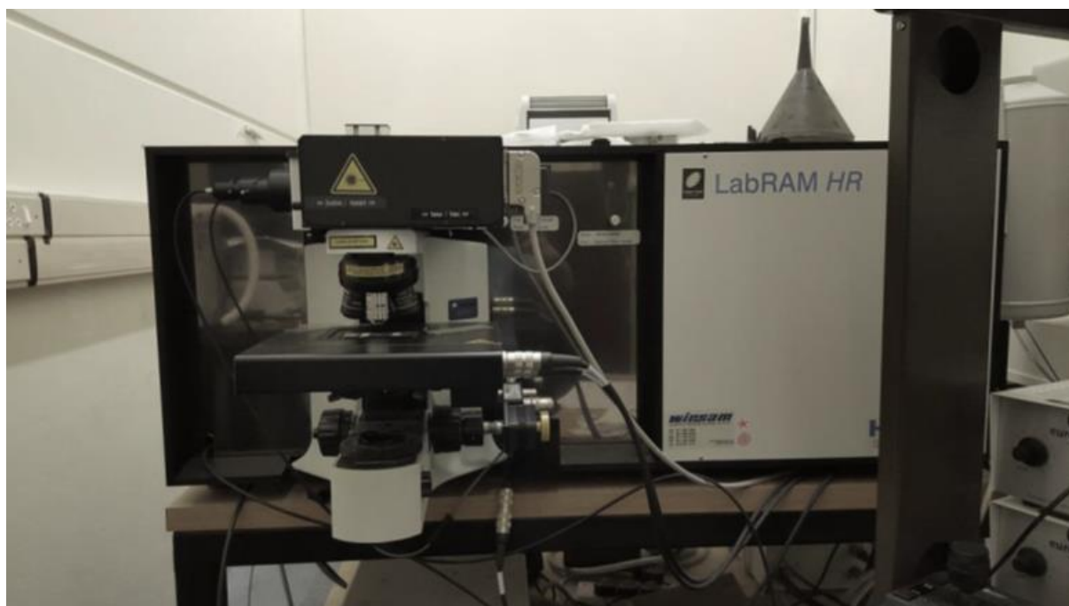
Figure 2.12: A Horiba Jobin-Yvon Raman spectrometer.
