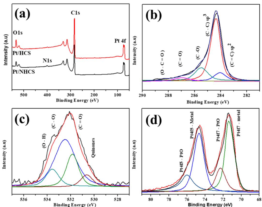
Figure 4.8: (a) XPS low resolution survey spectra for Pt/HCSs, Pt/NHCSs and high resolution (b) C1s, (c) O1s, and (d) Pt4f spectra for Pt/HCSs.
