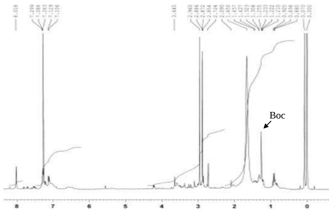
Figure A9 HNMR of MWCNT-DEA-Boc.peak at 1.2 represents the Boc group
