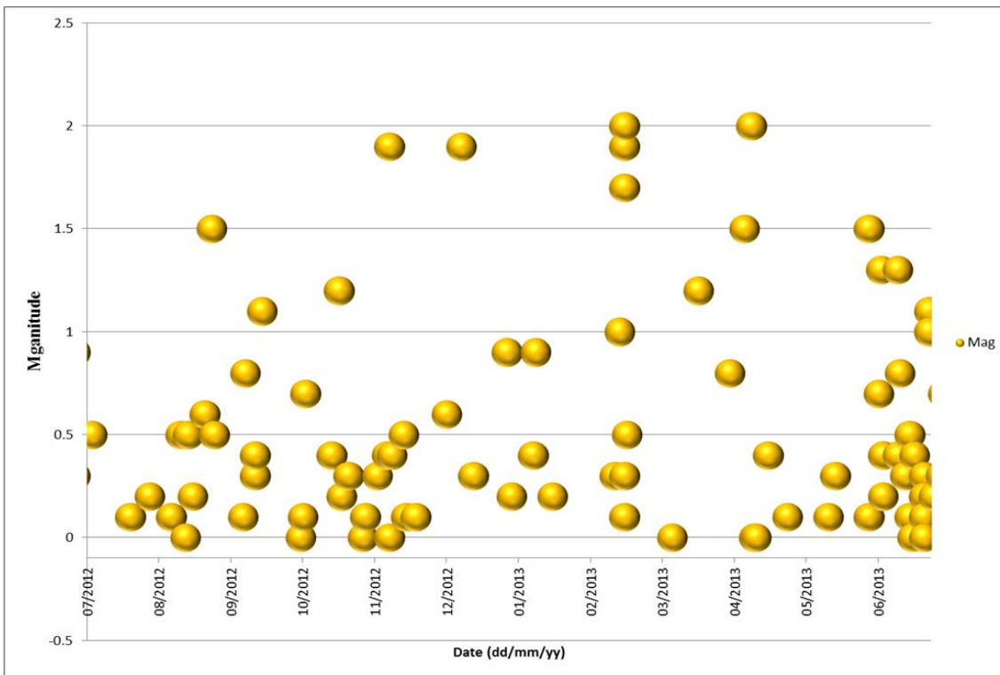
Figure 5: 7 Summary of seismic events ( M \geq 0 ) from July 2012 to June 2013
