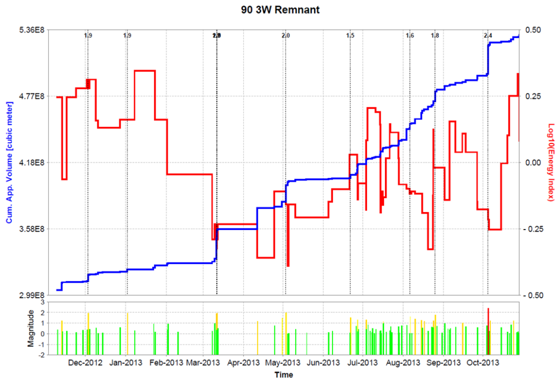
Figure 6: 3: 12 Cum apparent volume against Energy Index
