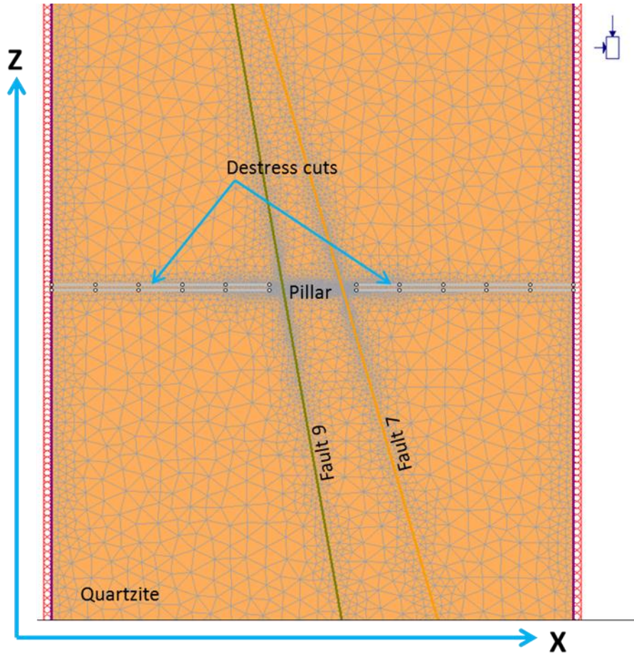
Figure 5: 5: Phase 2 inelastic model displaying the cross sectional view of the regional pillar.
