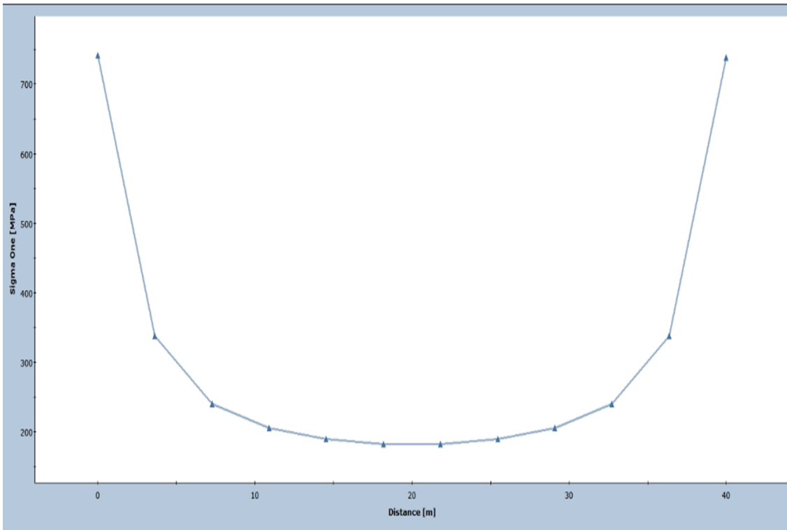
Figure 6: 2: 10 Major Principal Stress across the pillar in an elastic model
