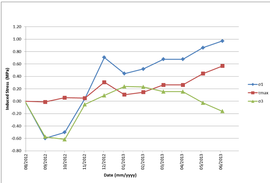
Figure 6: 3: 1 Induced principal stress changes from strain readings
