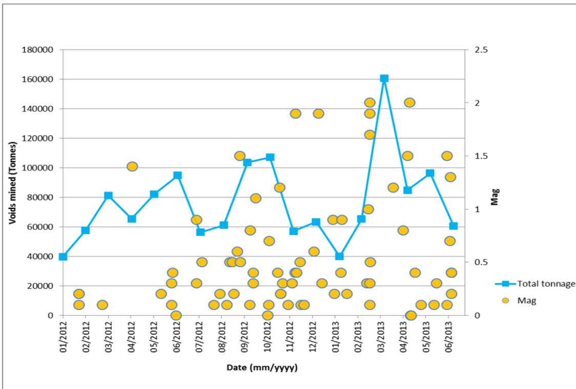
Figure 6: 3: 5 Correlation between seismic events ( M \geq 0 ) and mined tonnages from Aug 2012 to June 2013
