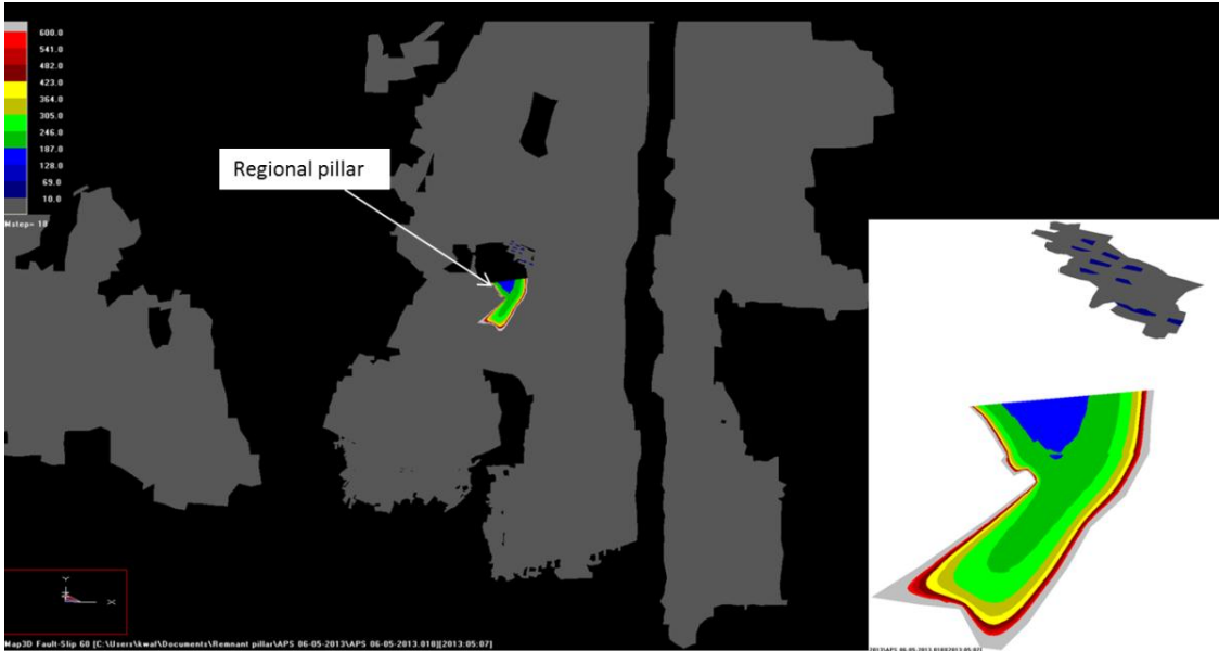
Figure 6: 2: 6 Normal stresses in the remnant pillar at mining step 18 of 90 3W
