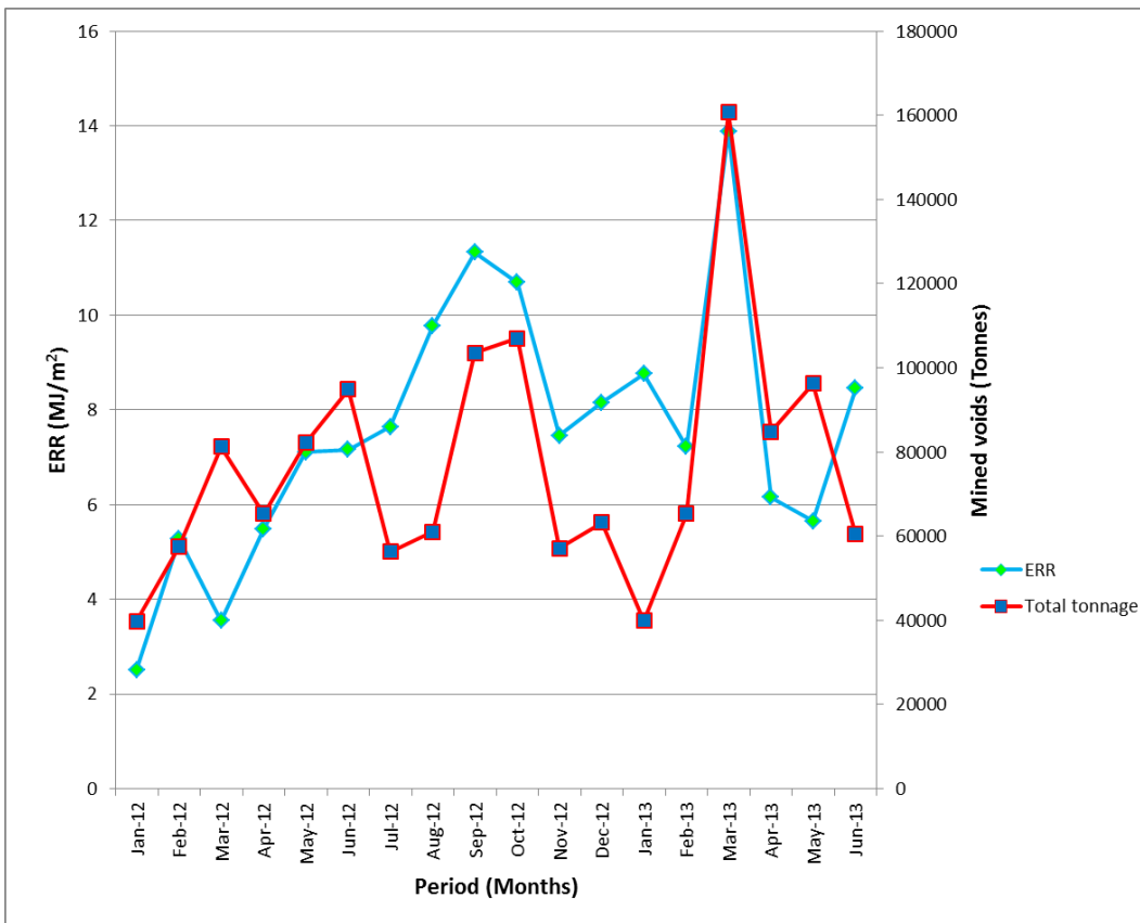
Figure 6: 2: 8 Association between energy release rate (ERR) and mined tonnages
