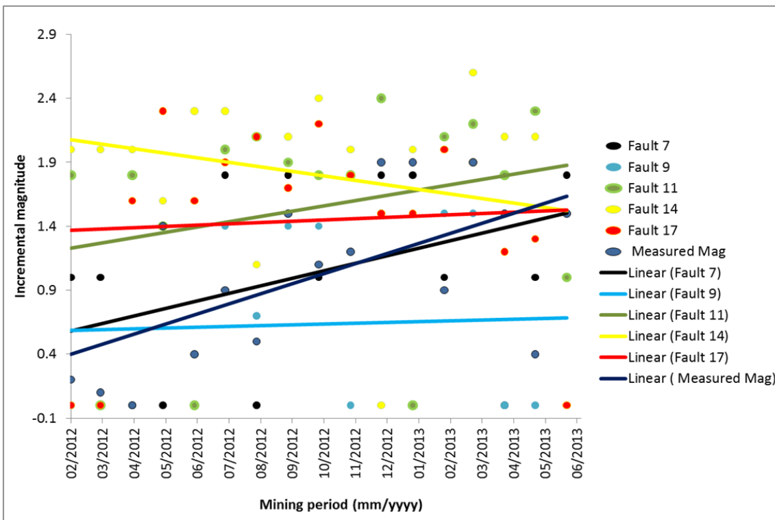
Figure 6: 2: 5 Expected event incremental magnitudes for actual mining sequence capping maximum ESS value at 15 MPa
