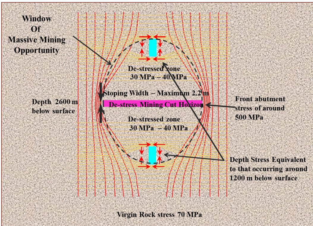
Figure 1: 6 De-stress Mechanism, after Watson (2012)
