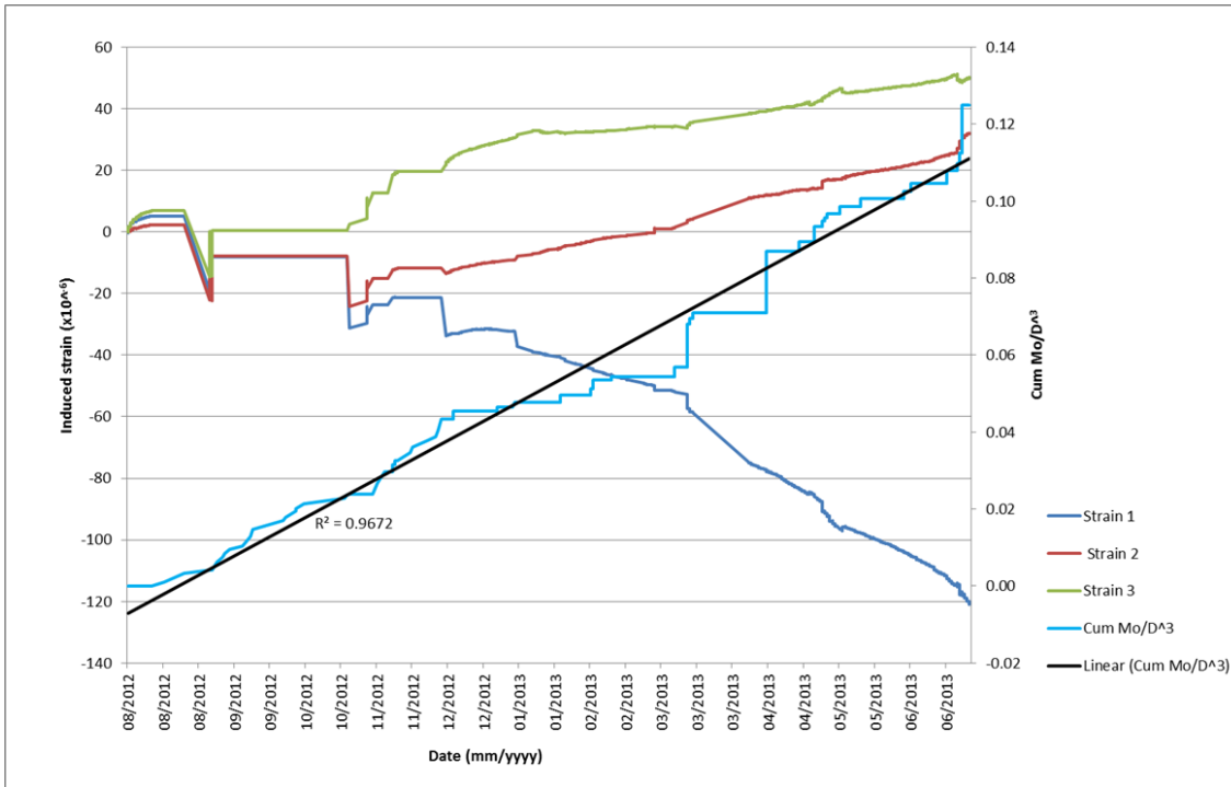
Figure 6: 3: 7 Correlating strain with \frac{M_o}{D^3}
