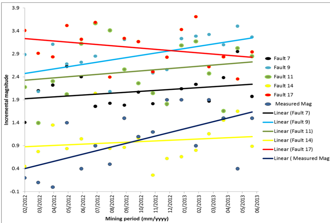
Figure 6: 2: 4 Expected event incremental magnitudes for actual mining sequence averaging 10 maximum ESS values
