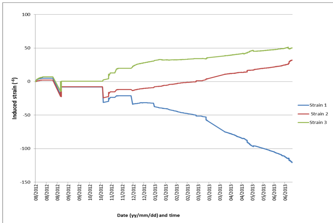
Figure 5: 6 Summary of measured strain data
