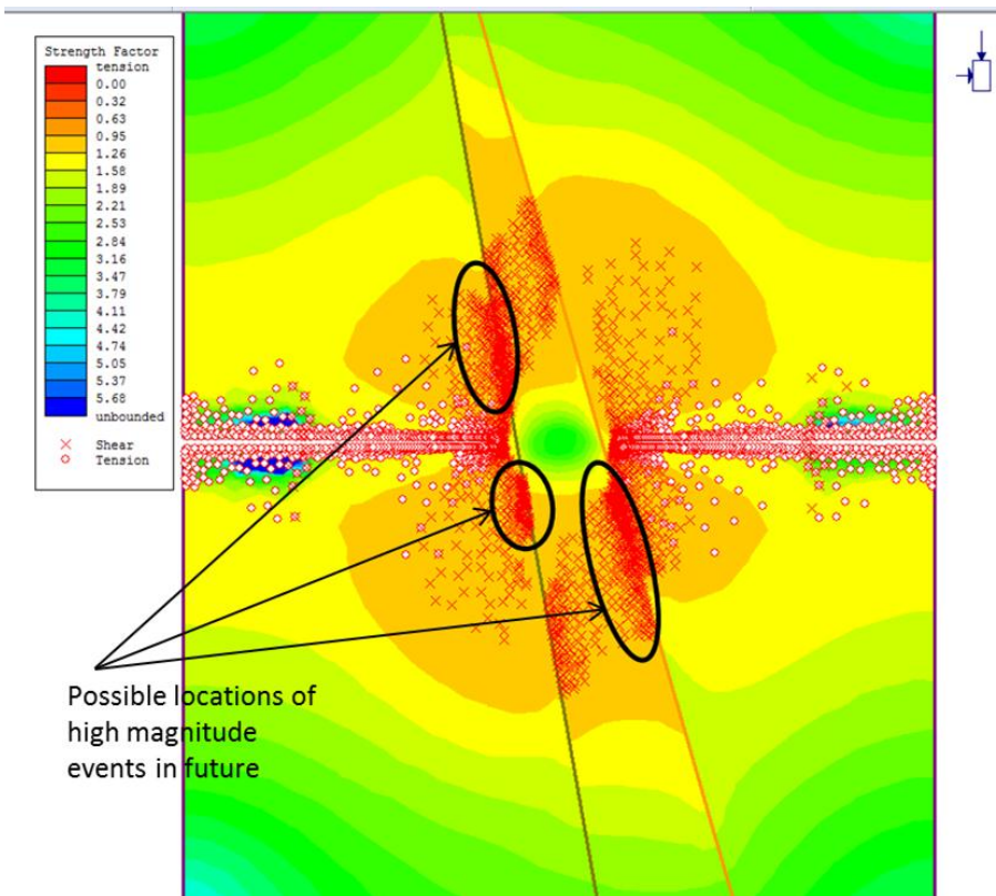
Figure 6: 2: 11 Strength factor across the pillar from Phase 2 model
