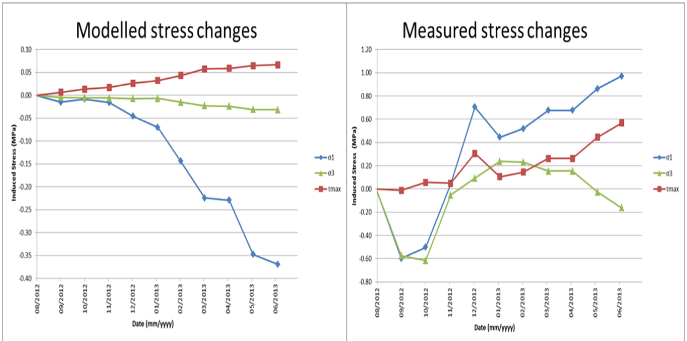
Figure 6: 3: 2 Comparison between modelled and calculated stress changes
