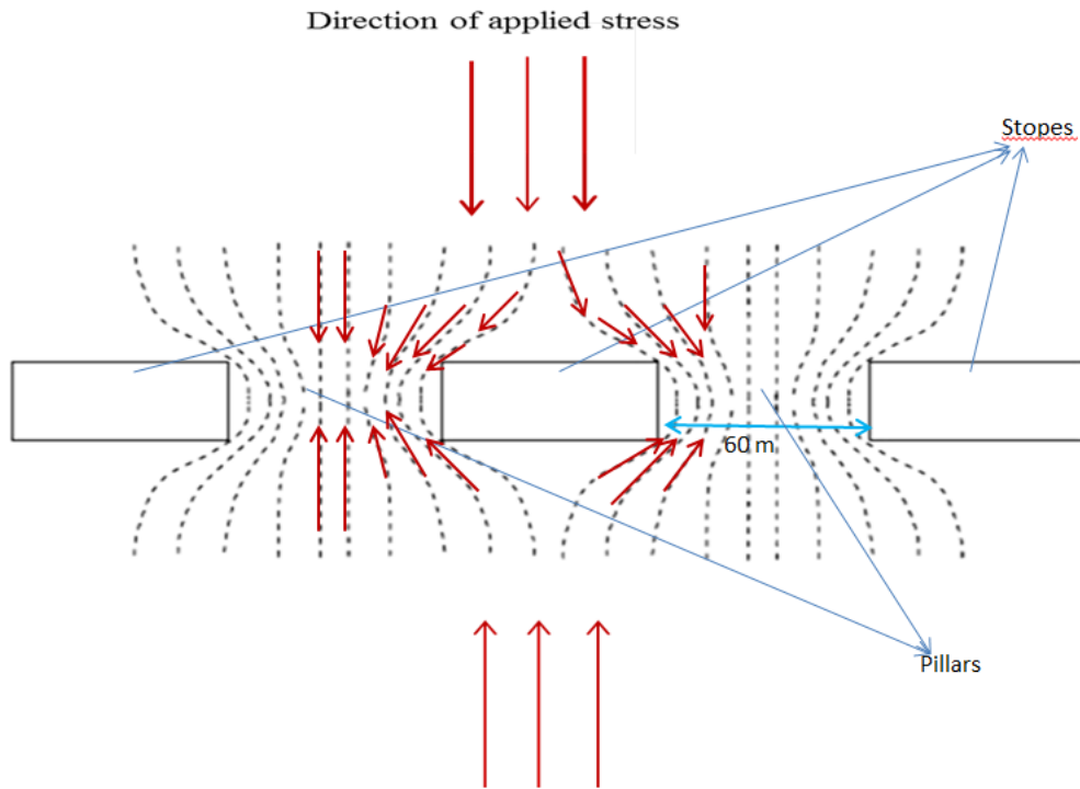
Figure 2: 2 Stress flow lines around stopes separated by typical regional pillars, Hoek and Brown (1982)
