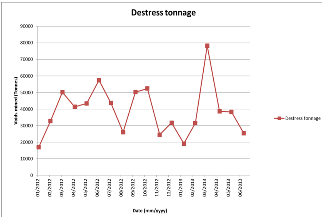
Figure 6: 1: 2 Total de-stressed tonnages
