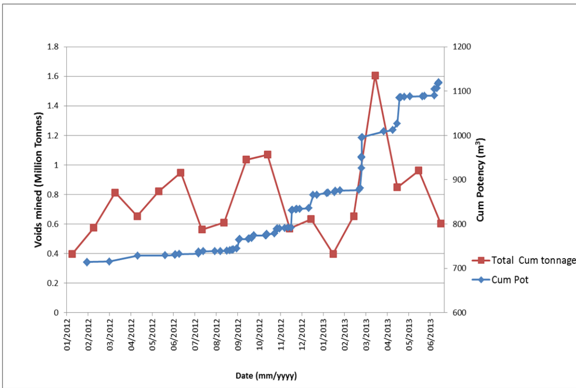
Figure 6: 3: 6 Correlation between cumulative potency and mining tonnages from Aug 2012 to June 2013
