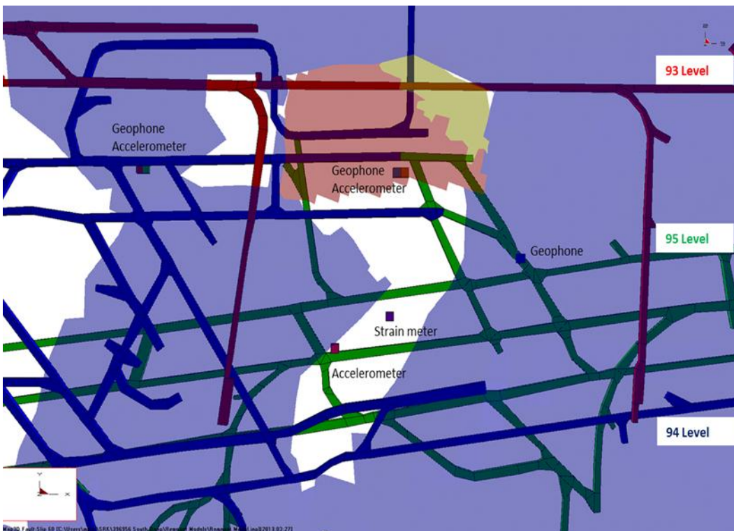
Figure 4: 2 Position of instrumentation in relation to the regional pillar (Plan view)
