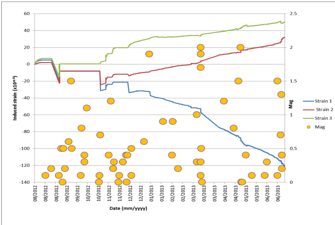
Figure 6: 3: 4 Correlation between seismic events ( M \geq 0 ) and strain data from Aug 2012 to June 2013
