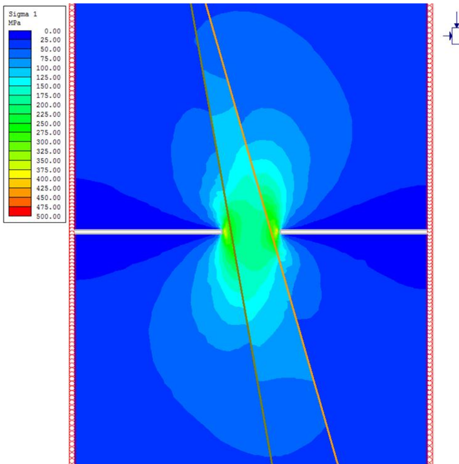
Figure 6: 2: 12 Major principal stress across the pillar from Phase 2 model
