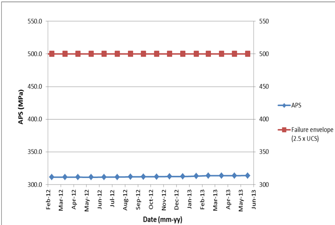
Figure 6: 2: 7 Average pillar stresses of the remnant during mining on 90 3W
