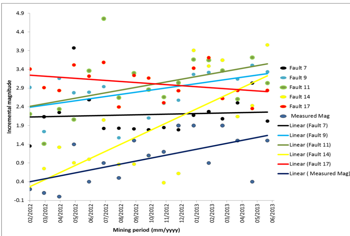
Figure 6: 2: 3 Expected event incremental magnitude for actual mining sequence from maximum ESS values
