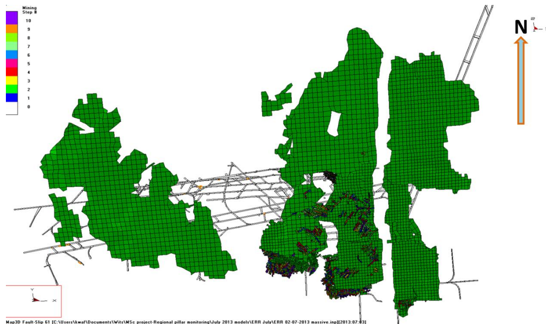
Figure 5: 1 Overall model showing de-stress mining (green) and massive mining (blue, red and yellow) on top
