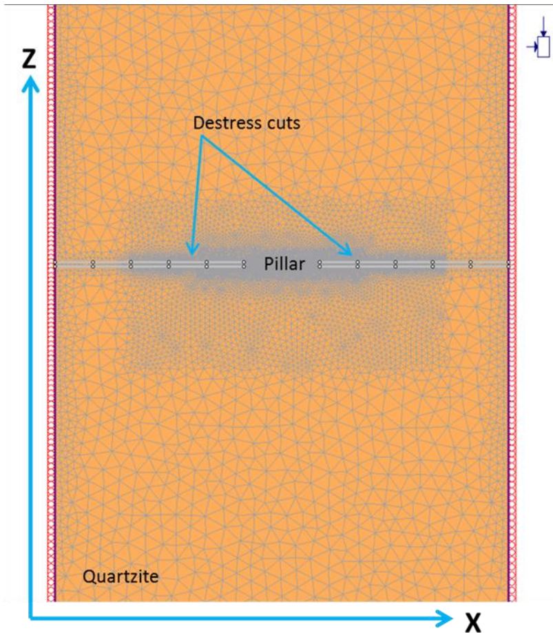
Figure 5: 4 Phase 2 elastic model
