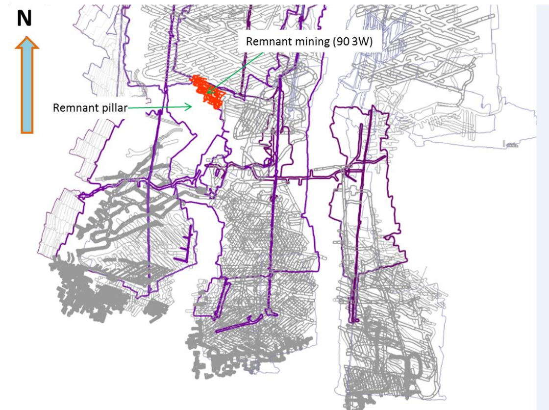
Figure 4: 1 Location of the Regional (Remnant) pillar
