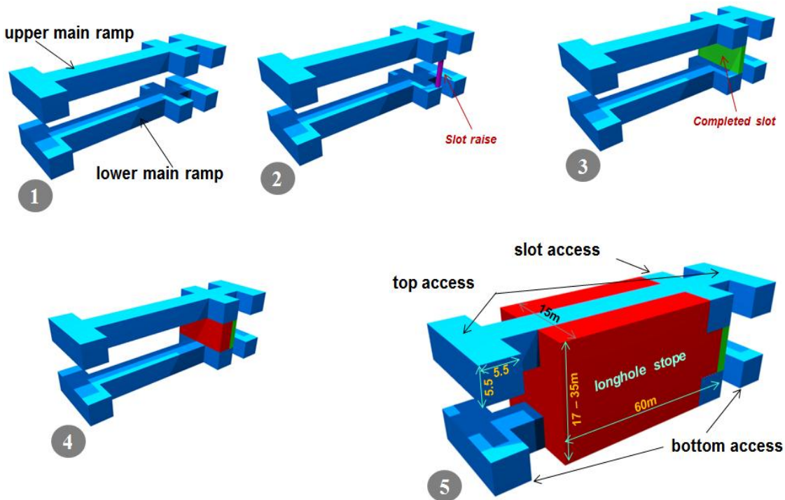
Figure 1: 8 Long hole stoping method (South Deep, 2012)
