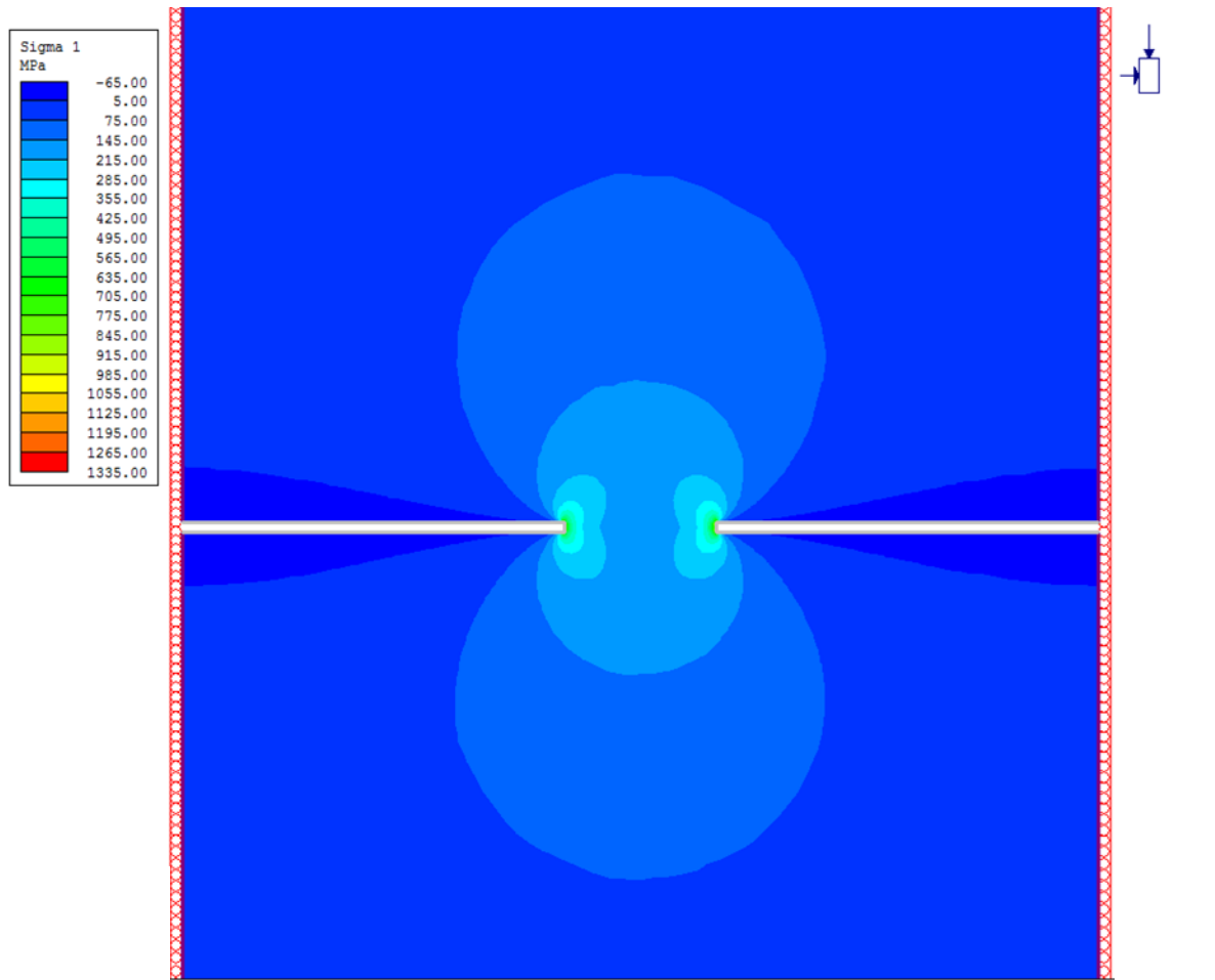
Figure 6: 2: 9 Major Principal Stresses across the pillar
