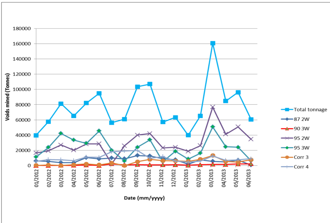
Figure 6: 1: 1 Mined tonnages for areas around the remnant pillar
