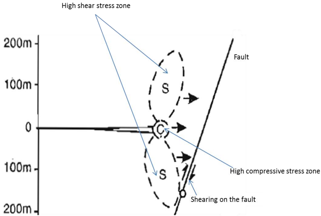
Figure 6: 2: 2 ESS lobes in front in excavation face, (after Jager and Ryder, 1999)
