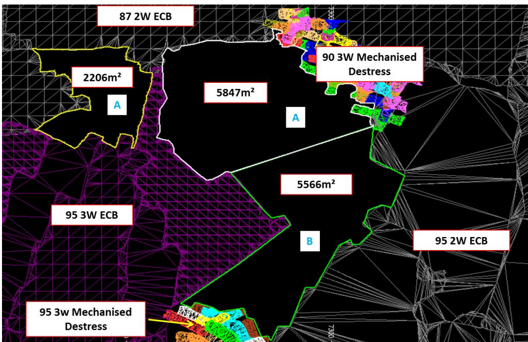
Figure 4: 4 Proposed final pillar layout and size
