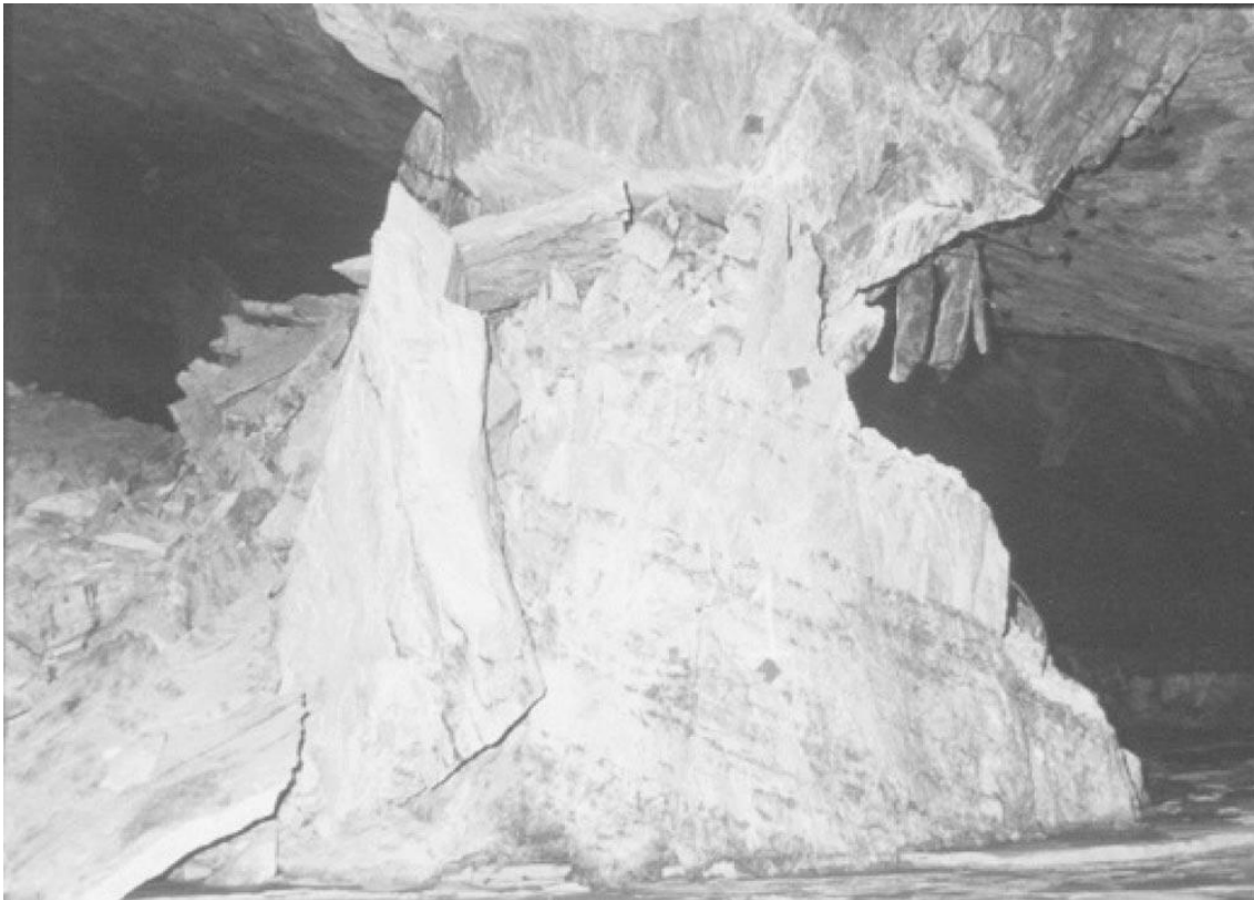
Figure 1: 1 Crushed pillar in massive quartzite (after Martin and Maybee, 2000)
