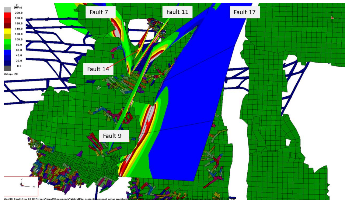
Figure 6: 2: 1 Location of faults and sigma 1 plot
