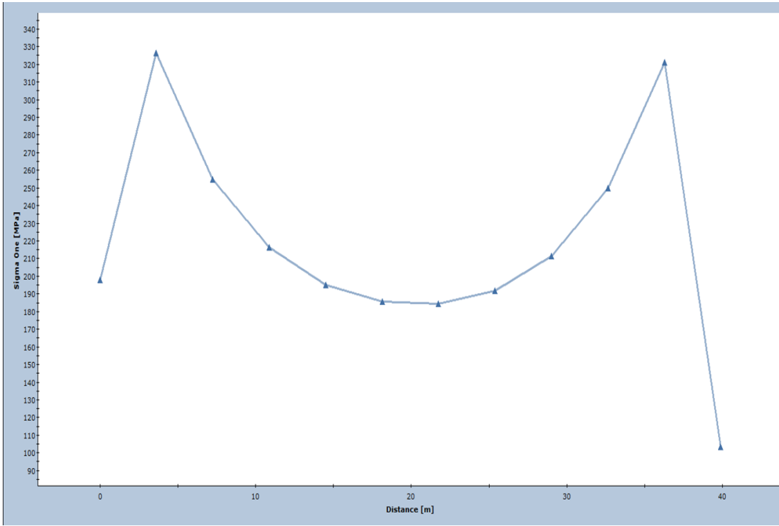
Figure 6: 2: 13 Distribution of major principal stress across the pillar
