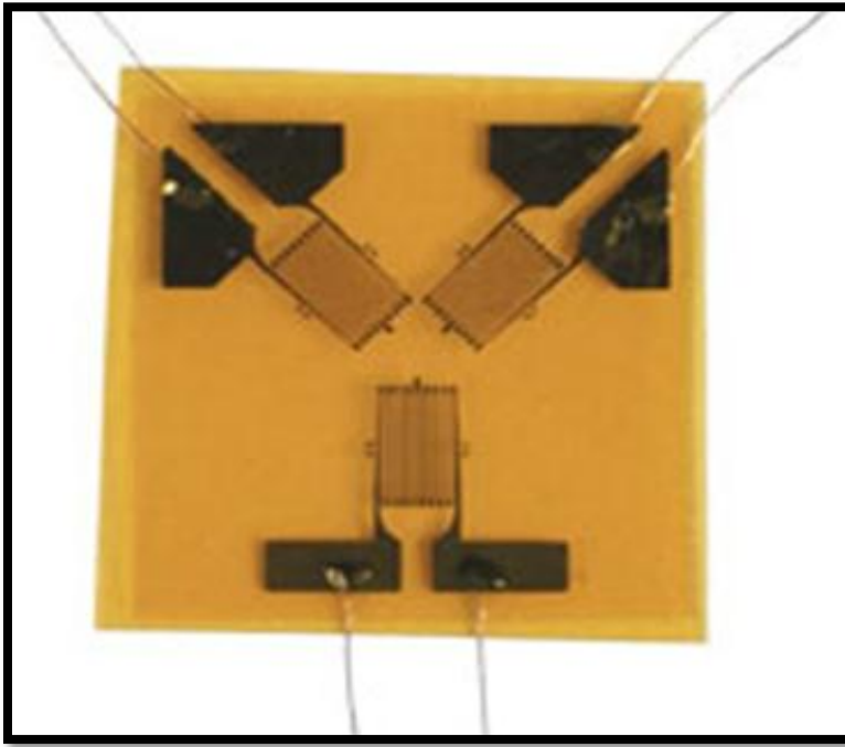
Figure 3: 2 0^{\circ} - 120^{\circ} - 240^{\circ} strain gauge rosette orientation
