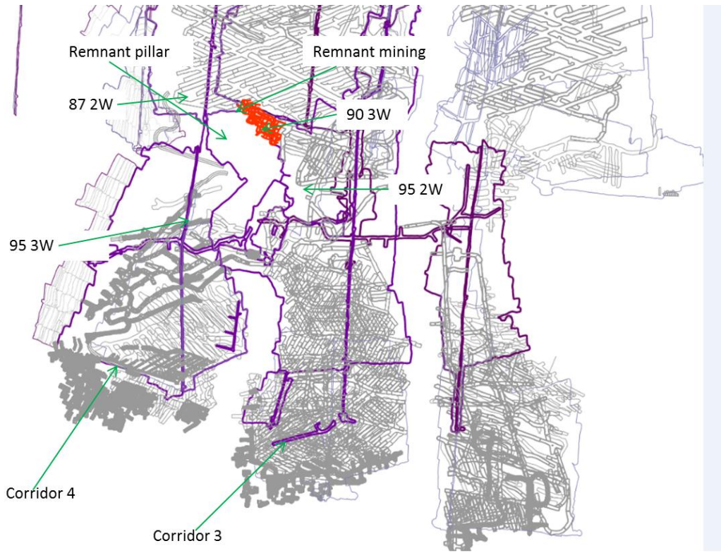
Figure 5: 9 Production areas considered for pillar monitoring
