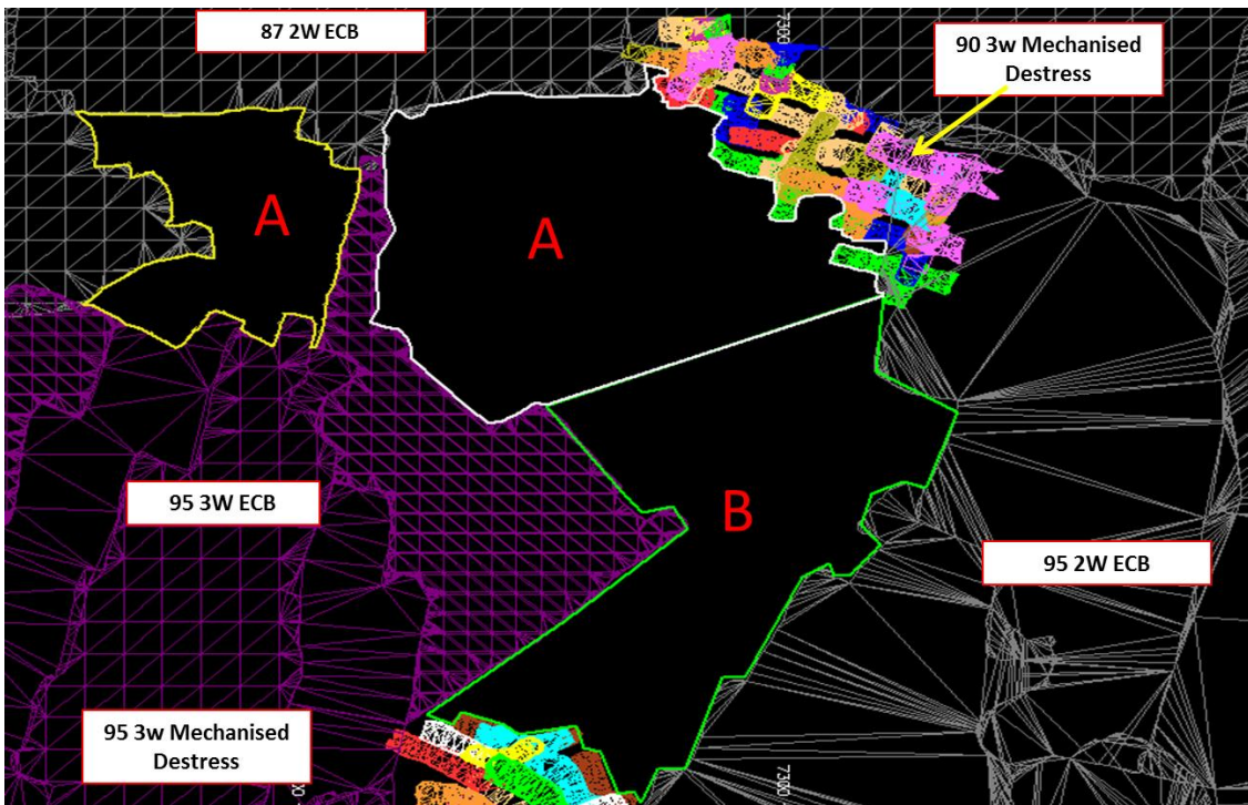
Figure 5: 2 Remnant pillar layout
