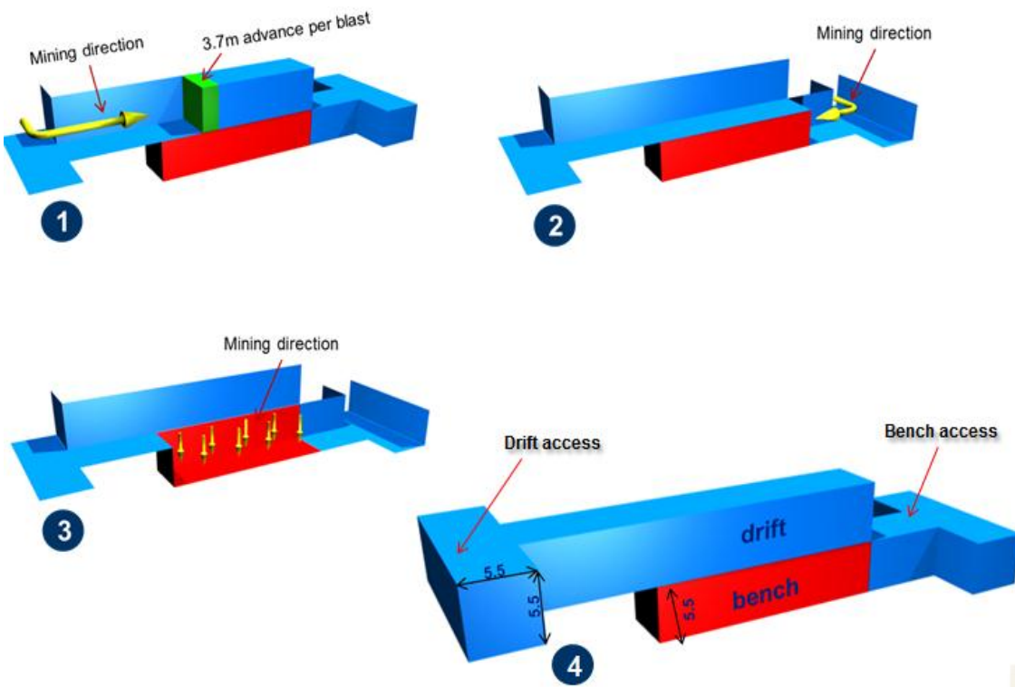
Figure 1: 9 Drift and bench mining (South Deep, 2012)
