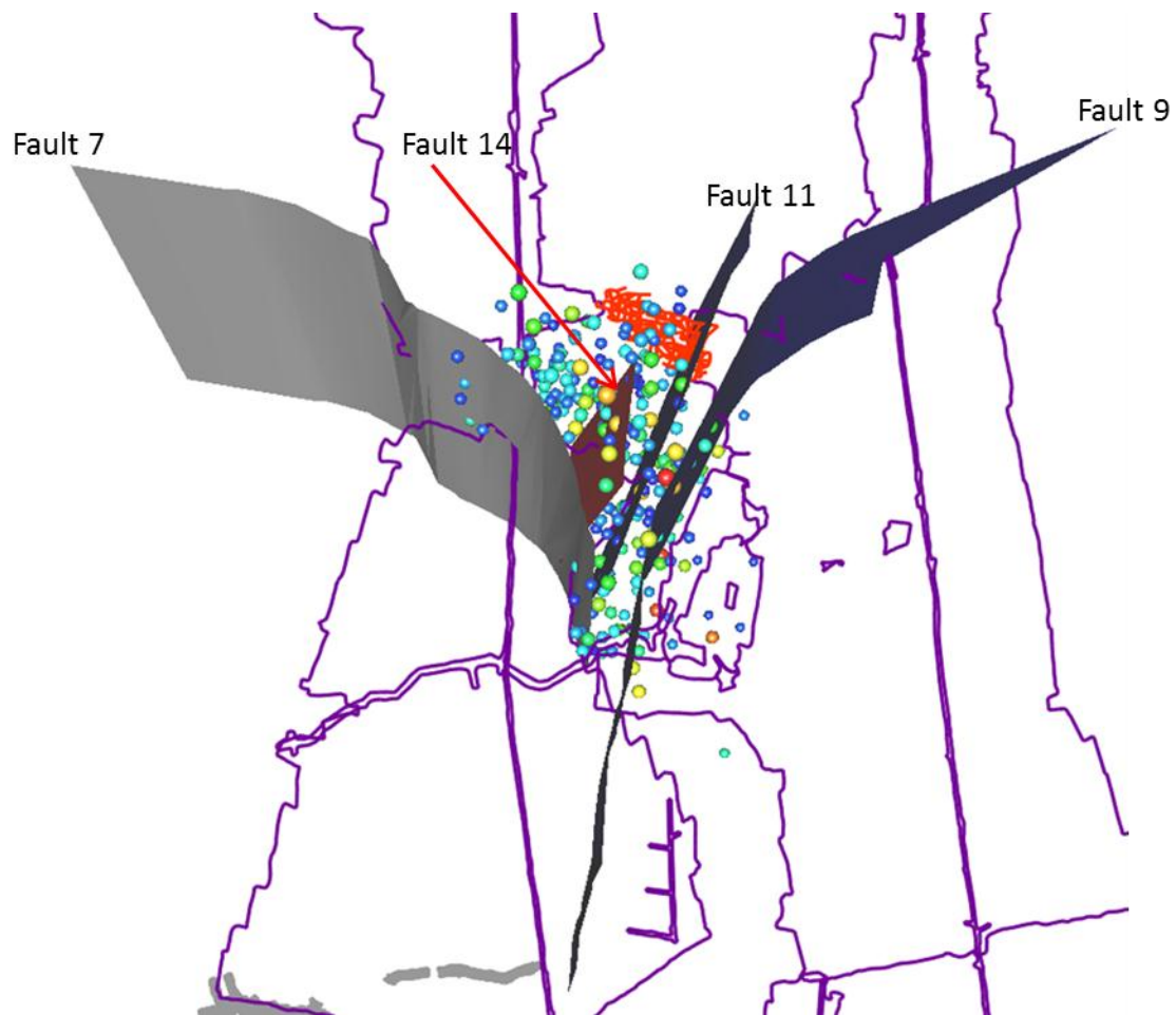
Figure 5: 8 Seismic events inside the pillar and geological structures
