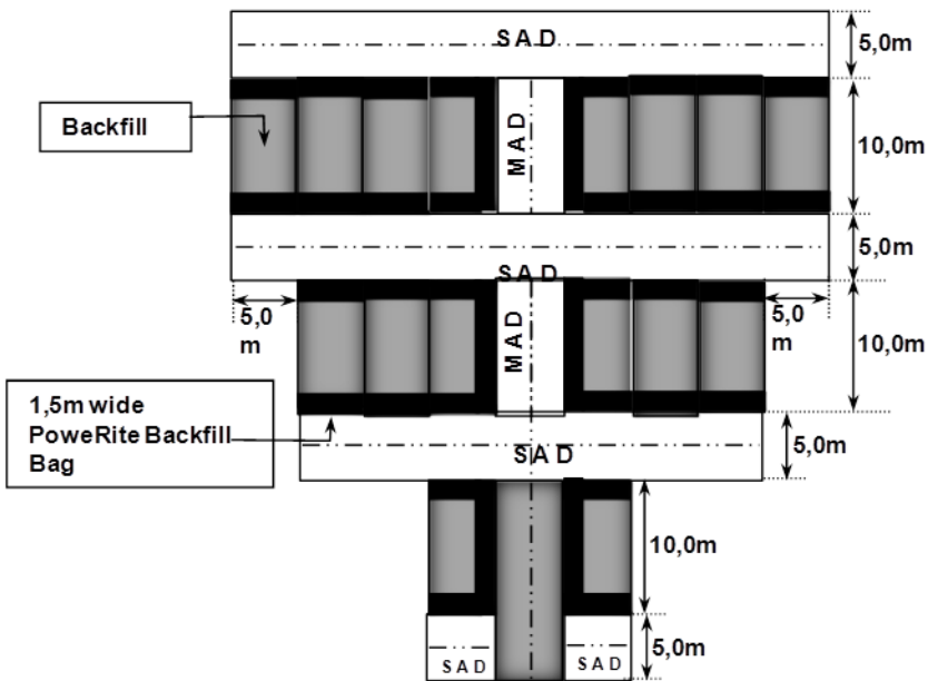
Figure 1: 7 Mining and backfill sequence for mechanized de-stress method (Plan view), South Deep gold mine (2012)
