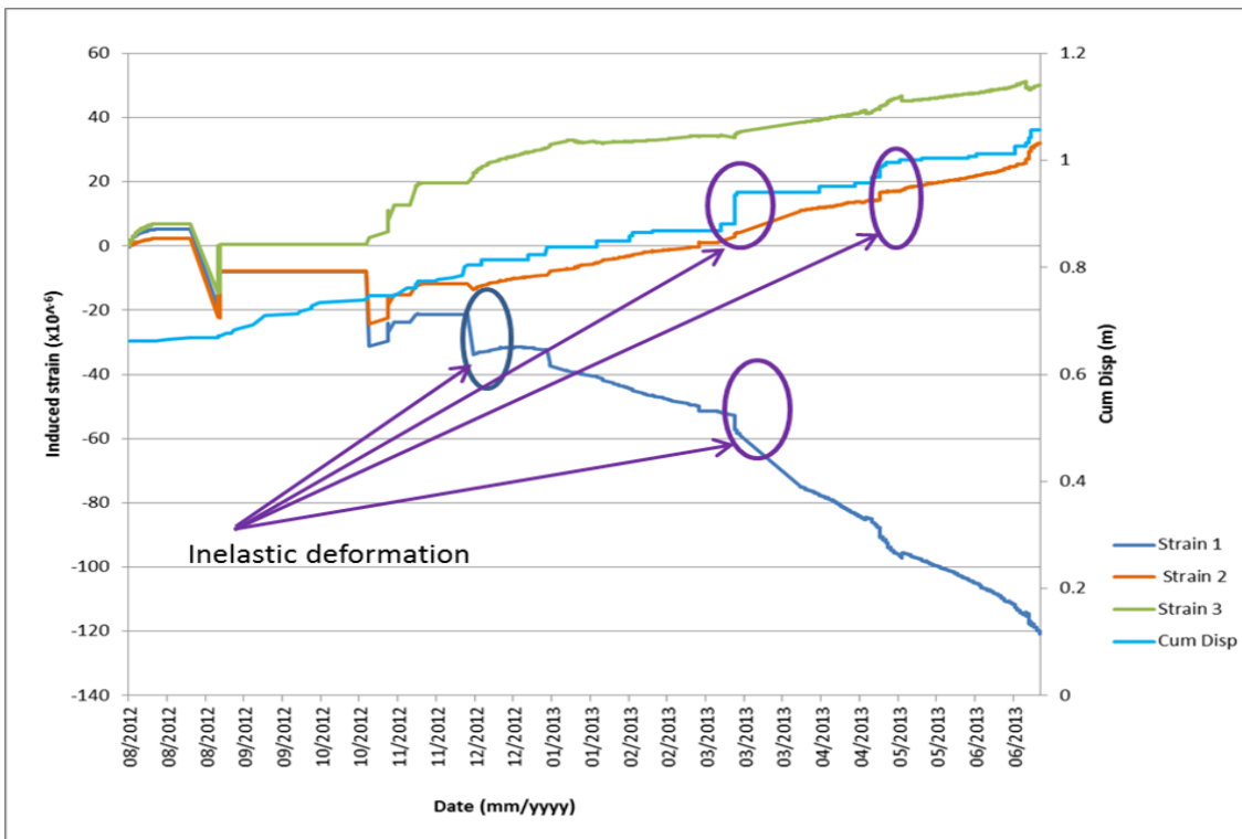
Figure 6: 3: 8 Co-seismic cumulative displacement and strain analysis from August 2012 to June 2013
