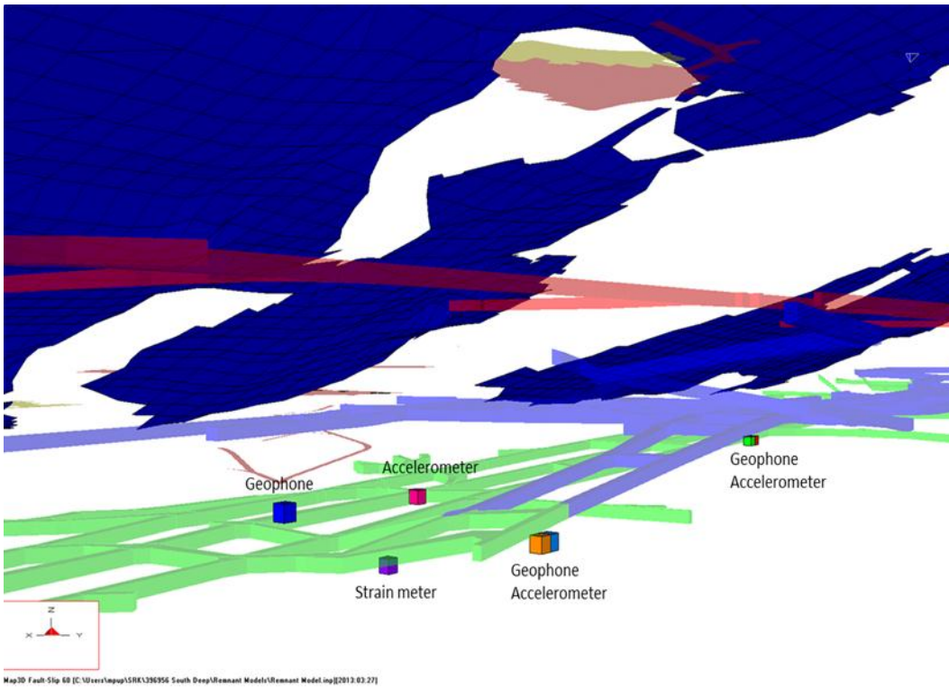
Figure 4: 3 Location of instrumentation looking west from below
