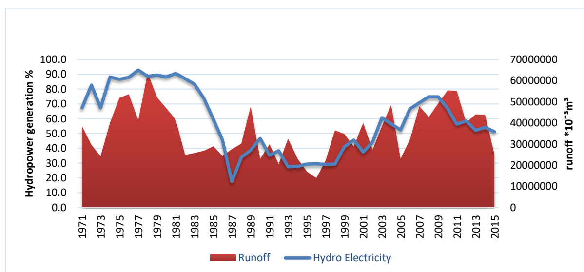
Figure 4.3.1 Hydropower and runoff trends in Victoria Falls
