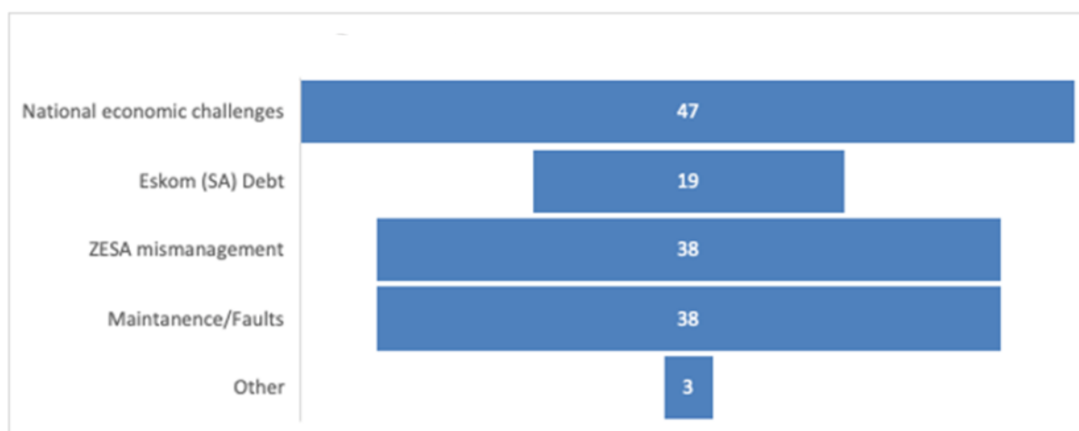
Figure 4.5.9 Reasons behind load shedding Source: Field survey (2018)
