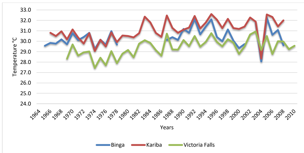
Figure 4.2.1 Long-term average annual maximum temperature patterns over the Kariba sub-basin
