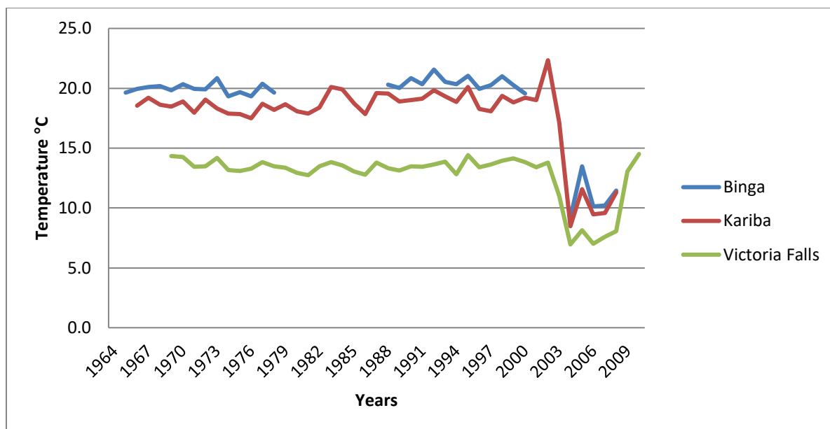
Figure 4.2.5 Long-term average annual minimum temperature patterns over the Kariba sub-basin
