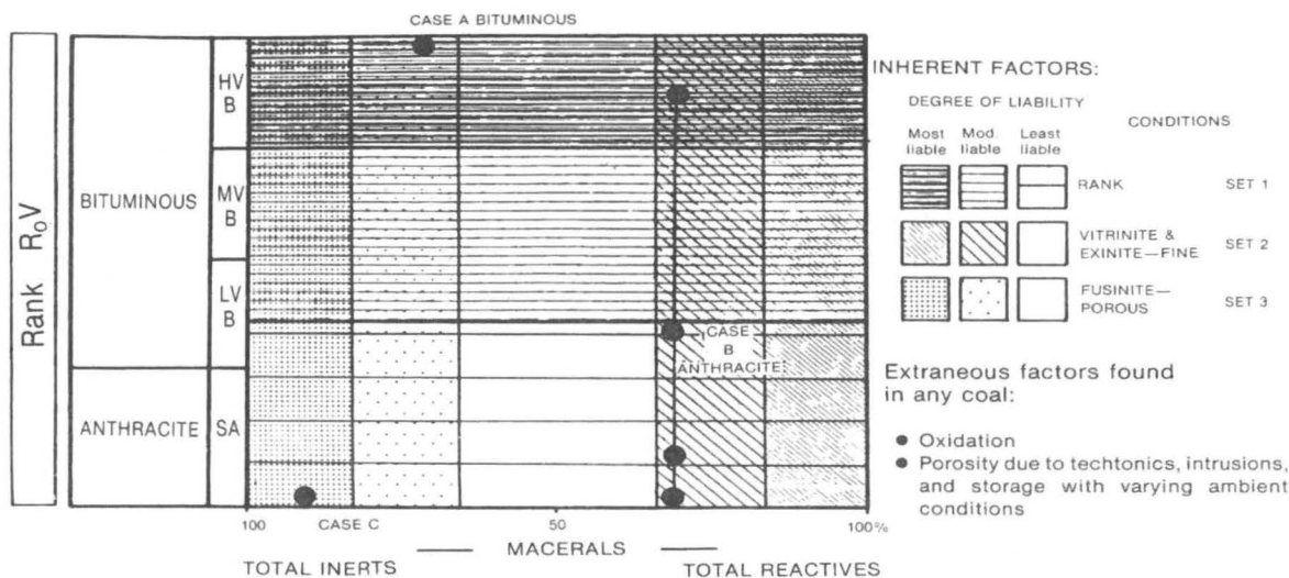
Figure 17: Liability of coals to spontaneously combustion as determined by inherent petrographic characteristics. Cases A, B and C are coals that have undergone rapid spontaneous combustion (Falcon, 1986)
