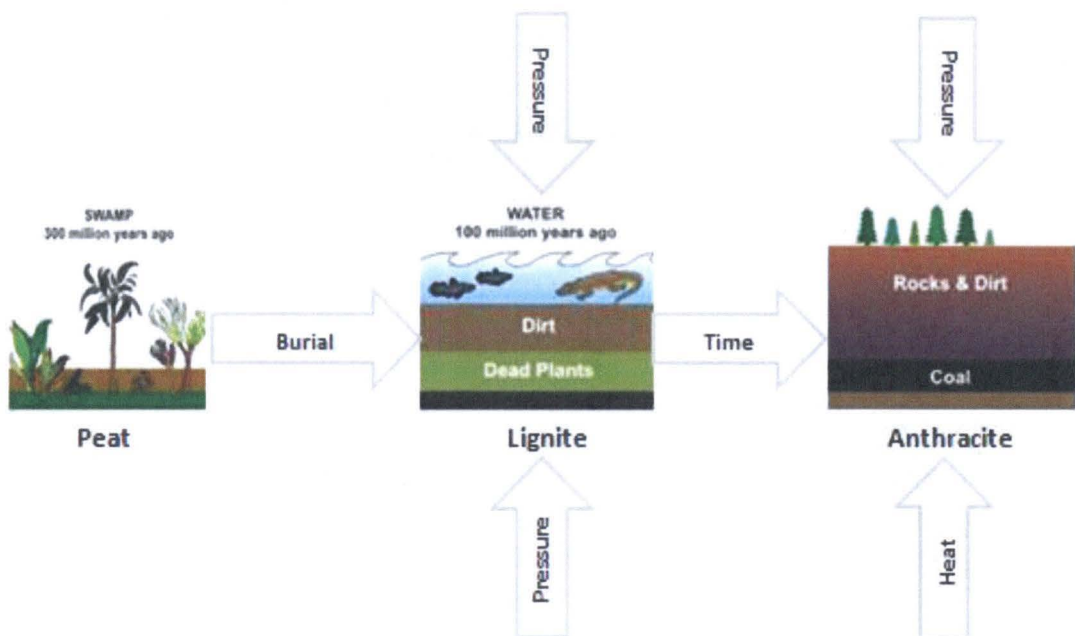
Figure 1: Coal Formation (EIA, 2013)
