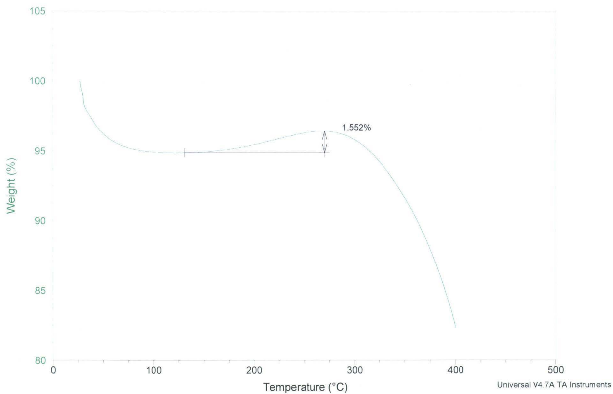
Figure 91: ZM26 O 2 Adsorption
