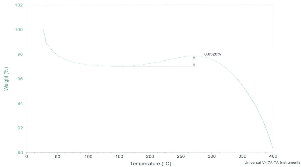
Figure 83: ZM18 O 2 Adsorption
