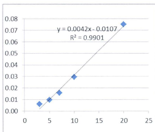
Figure 123: ZM10 R 2 graph
