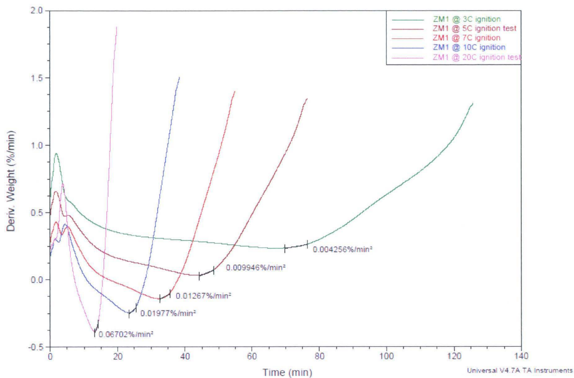
Figure 95: ZM1 Derivative curves and their slopes
