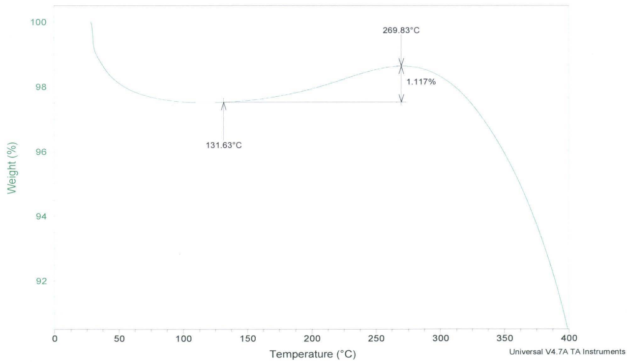
Figure 89: ZM24 O 2 Adsorption
