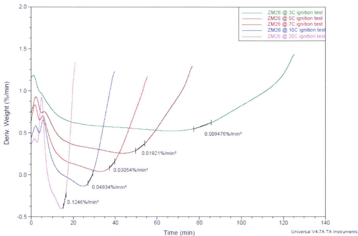
Figure 170: ZM26 Derivative curves and their slopes
