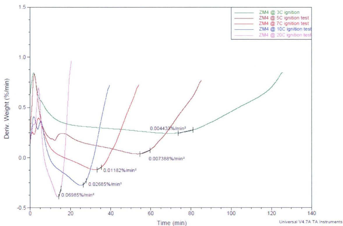
Figure 104: ZM4 Derivative curves and their slopes
