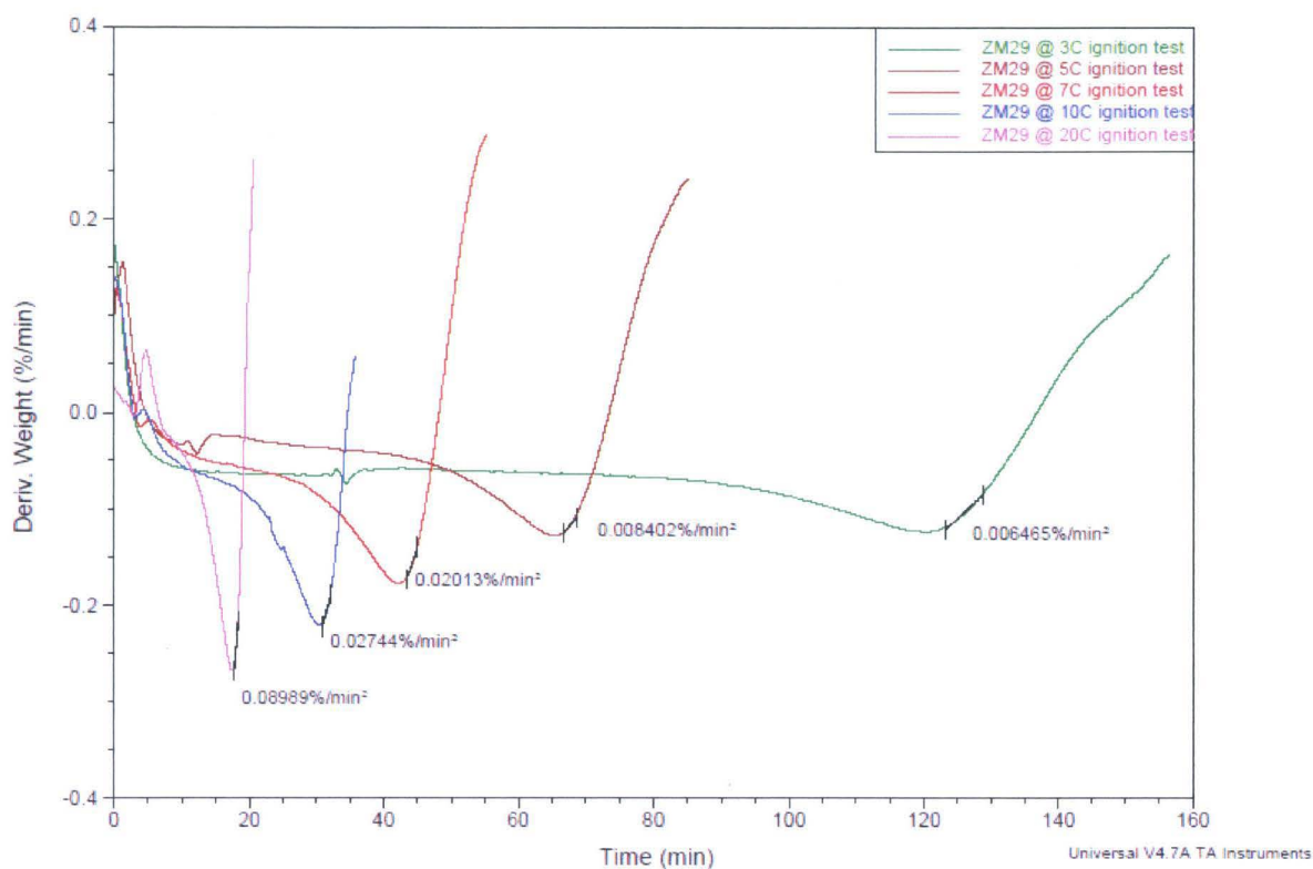
Figure 179: ZM29 Derivative curves and their slopes
