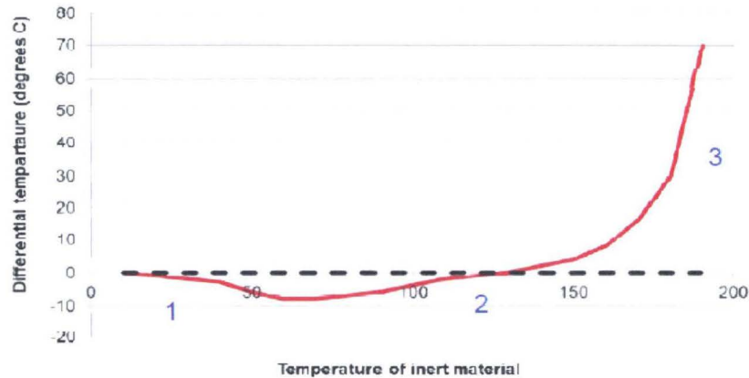
Figure 11: Differential thermograms (de Korte, 2014)
