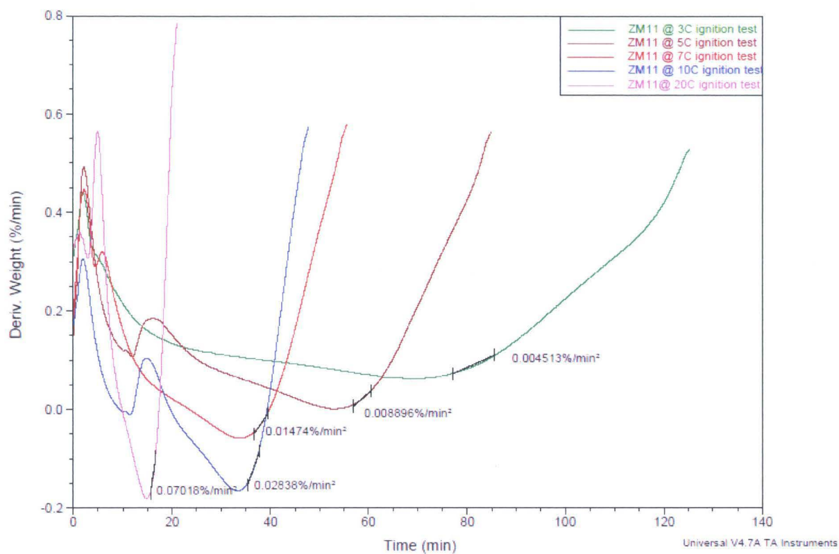
Figure 125: ZM11 Derivative curves and their slopes
