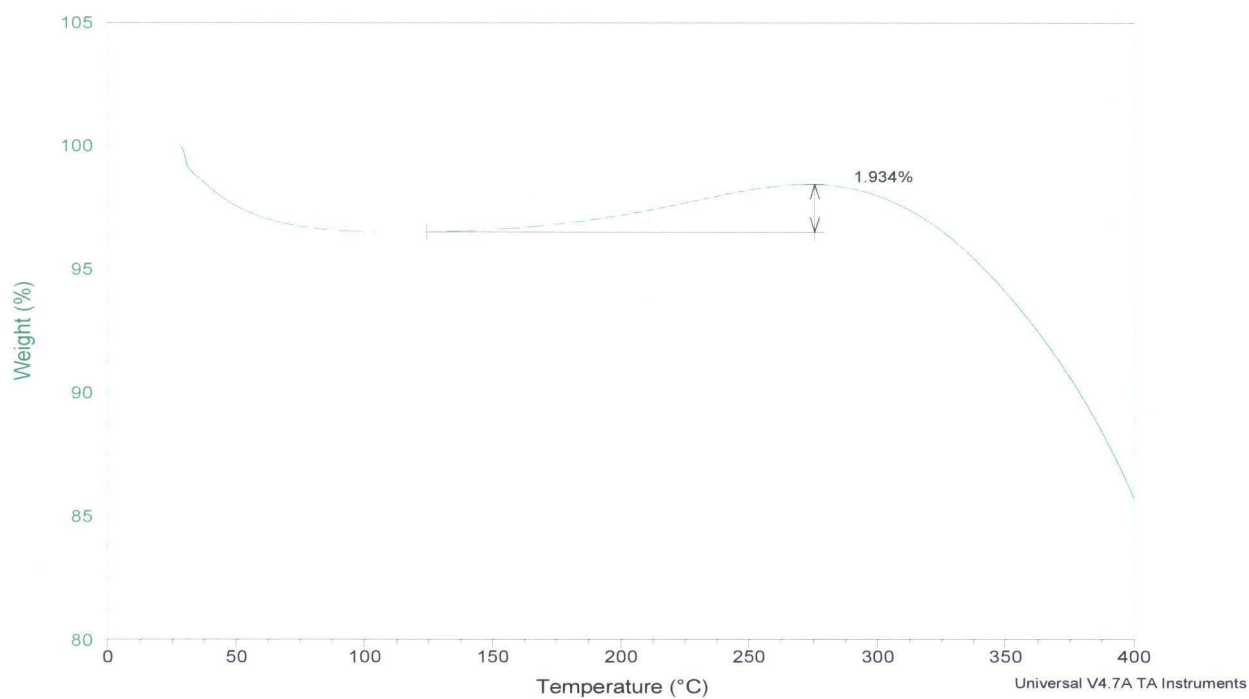
Figure 90: ZM25 O 2 Adsorption
