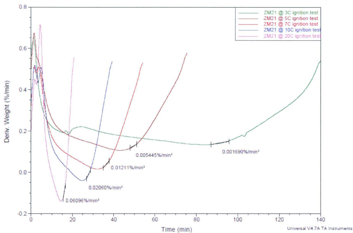
Figure 155: ZM21 Derivative curves and their slopes
