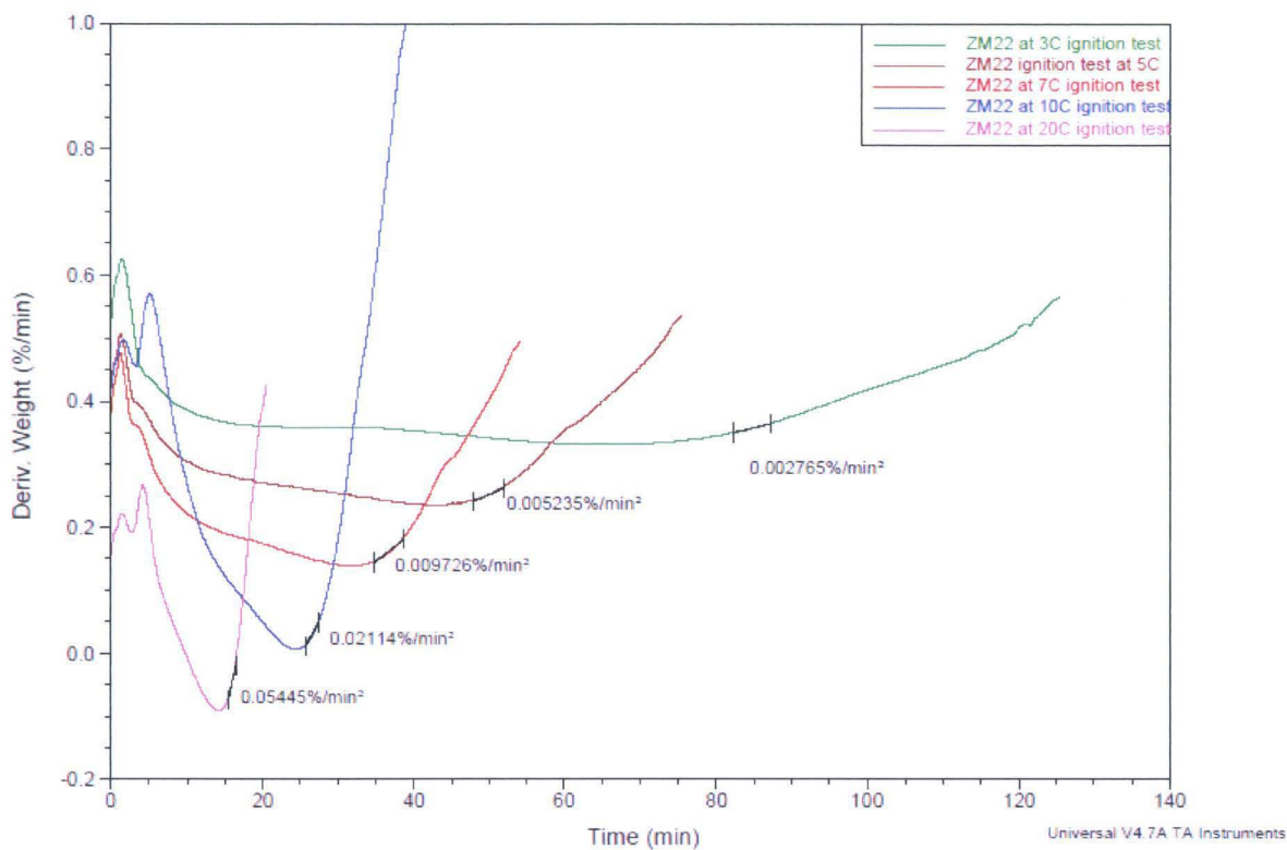
Figure 158: ZM22 Derivative curves and their slopes
