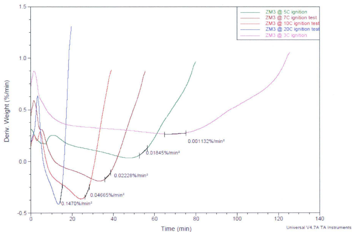
Figure 101: ZM3 Derivative curves and their slopes
