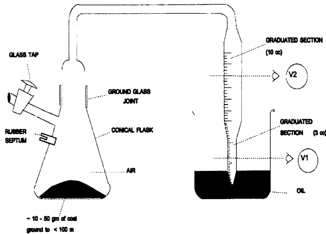
Figure 9: The Smith-Glasser Apparatus (Adamski, 2003)
