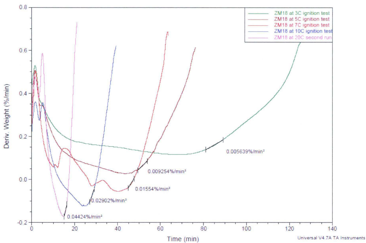
Figure 146: ZM18 Derivative curves and their slopes
