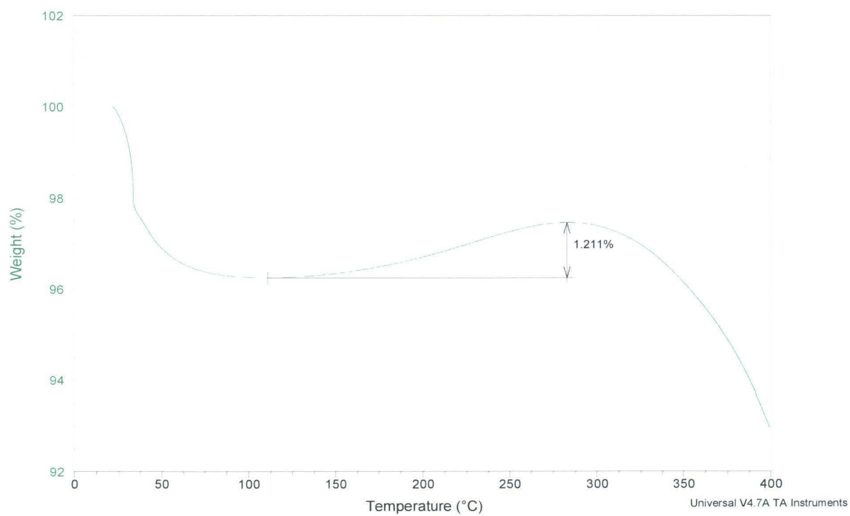
Figure 85: ZM20 O 2 Adsorption
