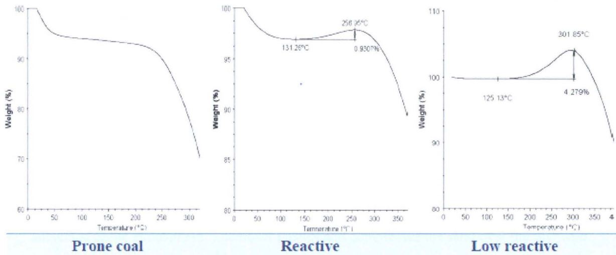
Figure 13: Oxygen adsorption curves illustrating the weight gain (Avila, 2012)
