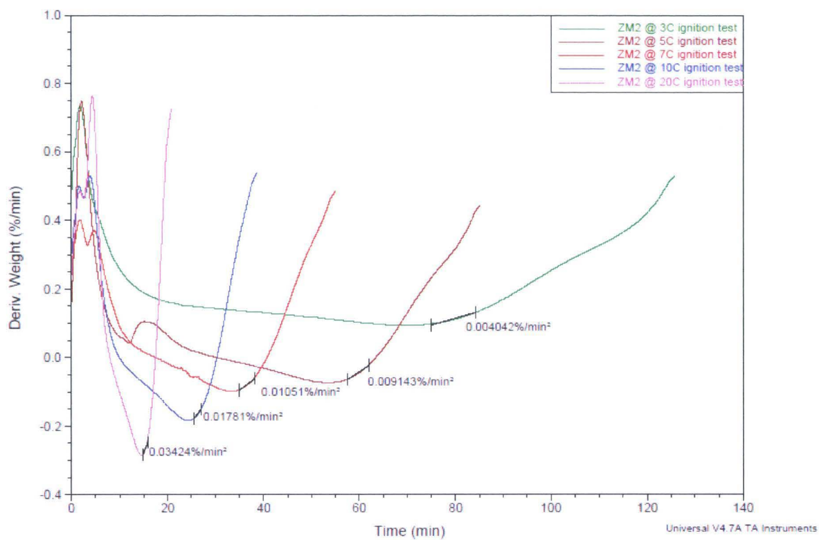
Figure 98: ZM2 Derivative curves and their slopes
