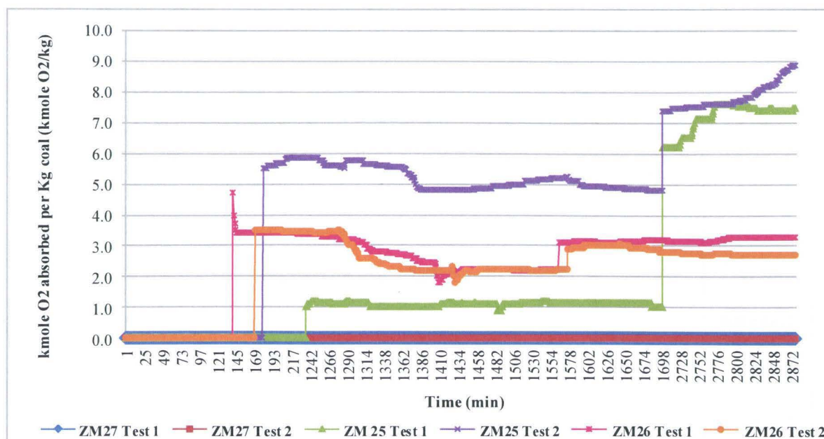
Figure 194: Smith-Glasser Repeatability Test (ZM 27, ZM25, ZM26)
