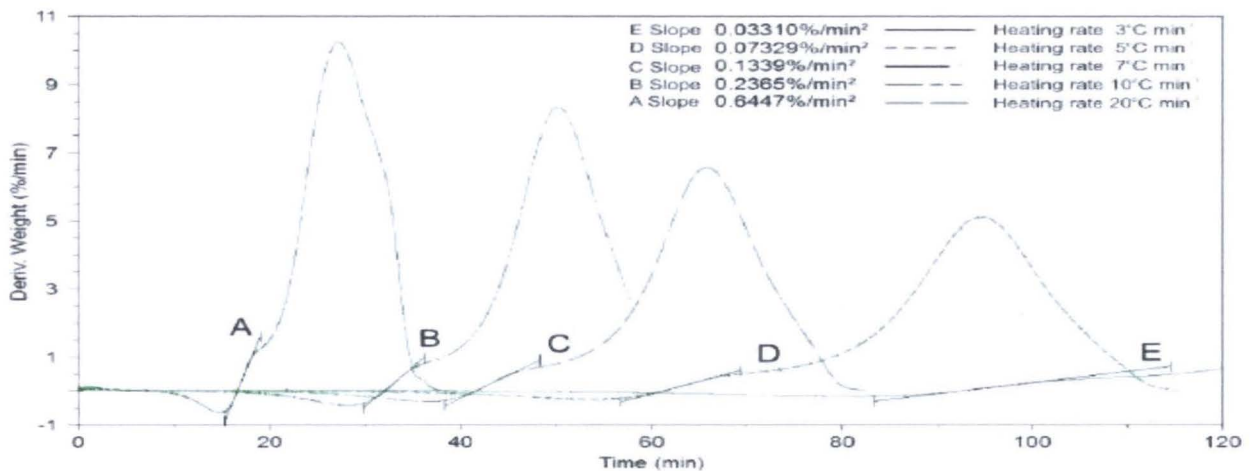
Figure 12: Derivative profiles used to obtain the TG_{spc} index (Avila, 2012)
