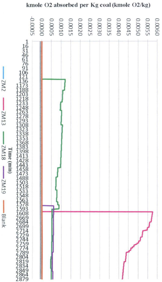
Figure 187: Smith-Glasser Oxygen absorption (ZM12, ZM13, ZM18, ZM19)
