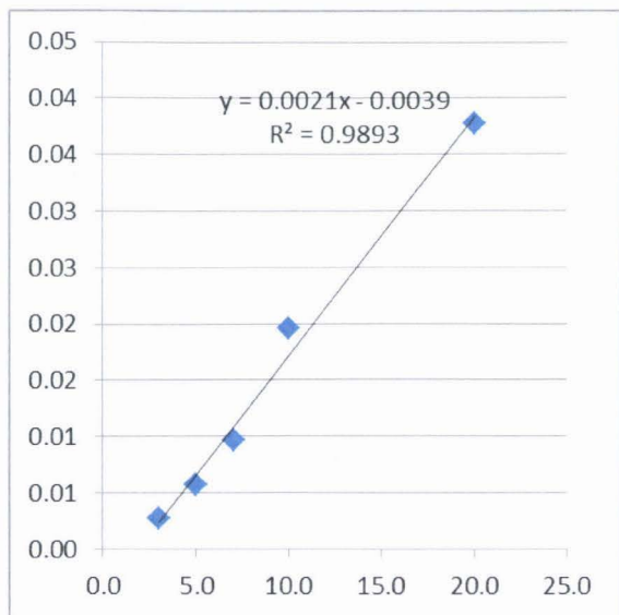
Figure 190: ZM28 R^2_{\text{graph}} Repeat
