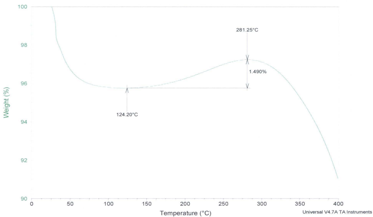
Figure 80: ZM15 O_2 Adsorption
