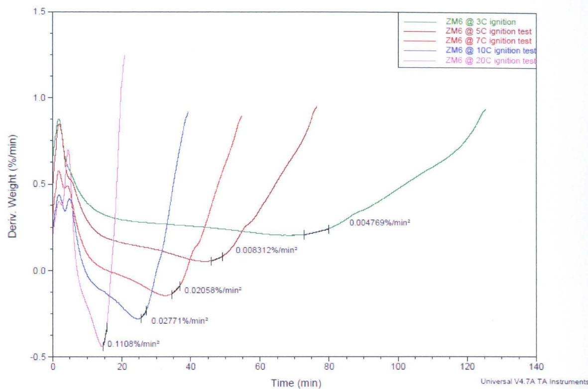
Figure 110: ZM6 Derivative curves and their slopes
