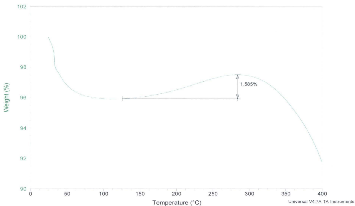
Figure 84: ZM19 O 2 Adsorption
