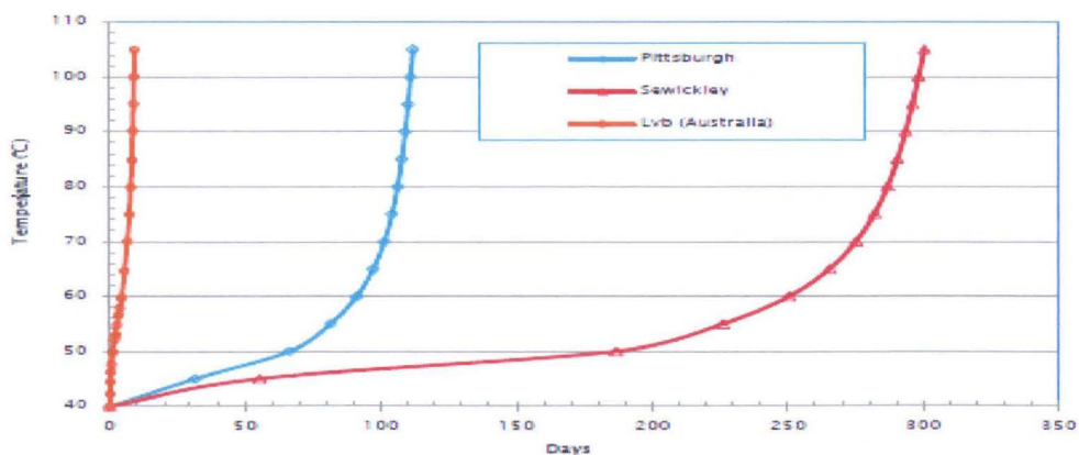
Figure 10: R70 Predicted self-heating curves of samples from the Pittsburgh and Sewickley Coal seams illustrating the duration of R70 tests (Luo and Wang, 2012).
