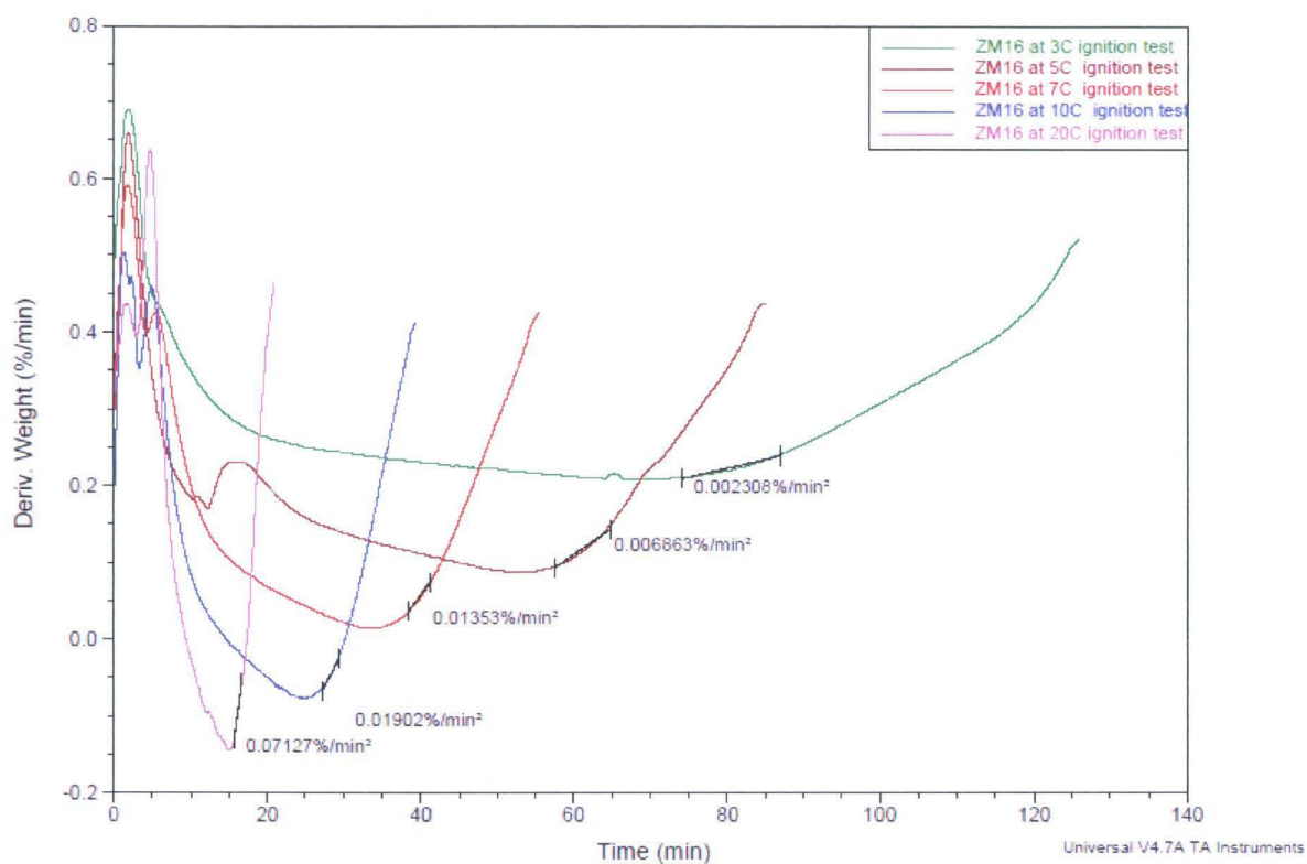
Figure 140: ZM16 Derivative curves and their slopes
