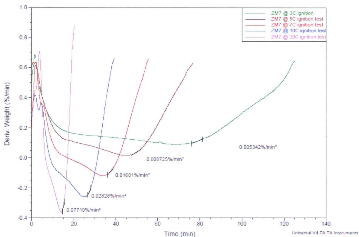
Figure 113: ZM7 Derivative curves and their slopes
