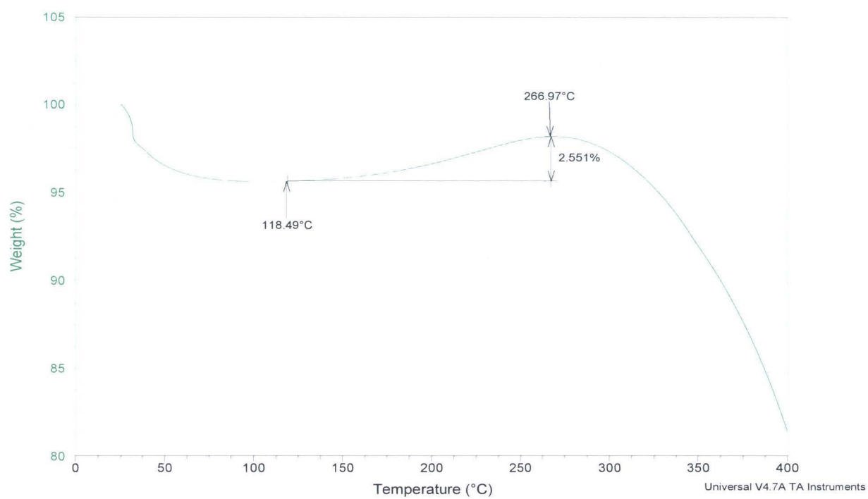
Figure 70: ZM5 O 2 Adsorption
