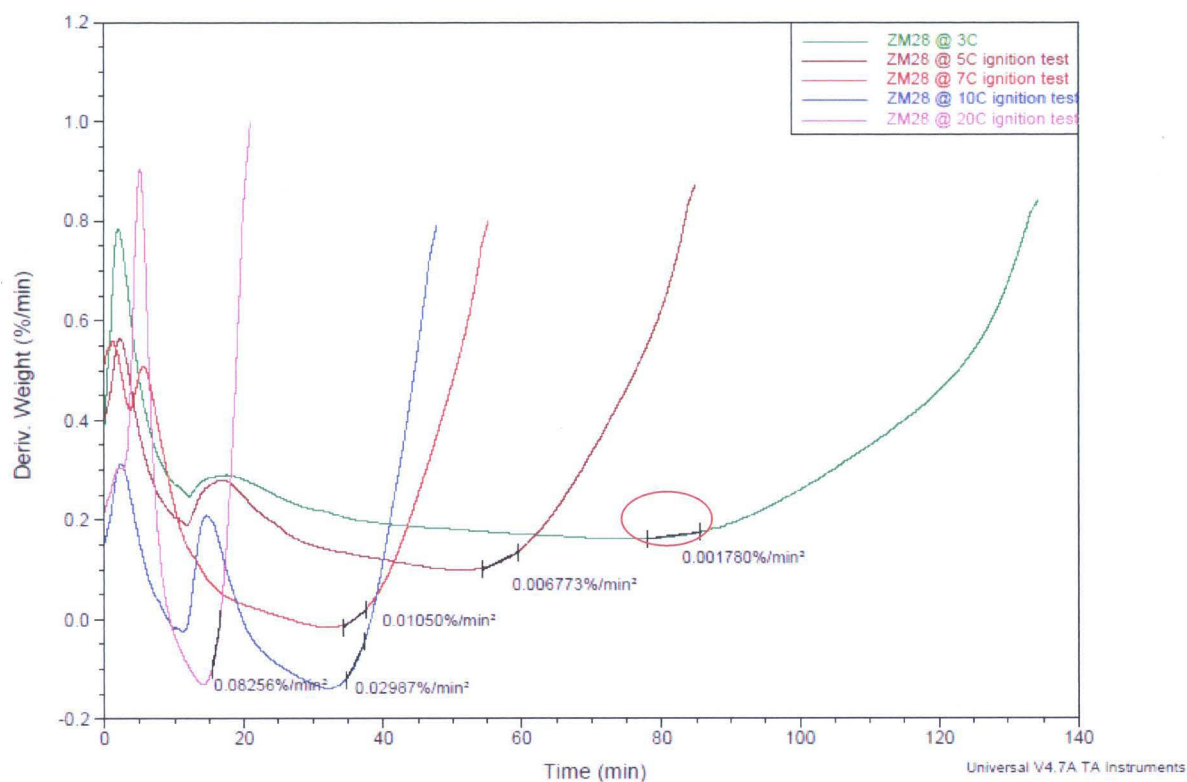
Figure 23: ZM28 Derivative weight curve at different temperature ramps (%/min)
