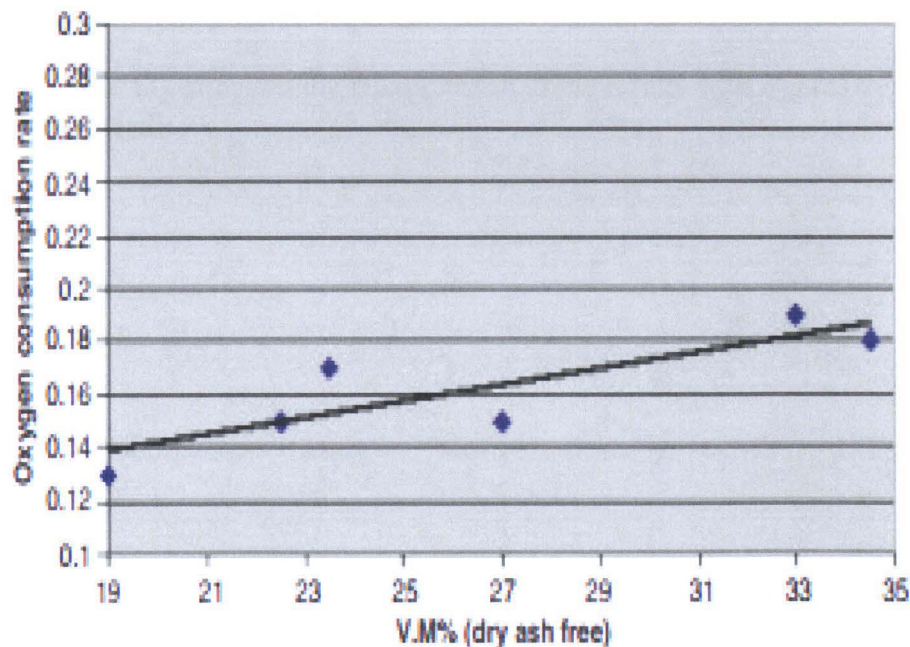
Figure 22: Rate of oxidation and volatile matter content (Uludag, 2007)
