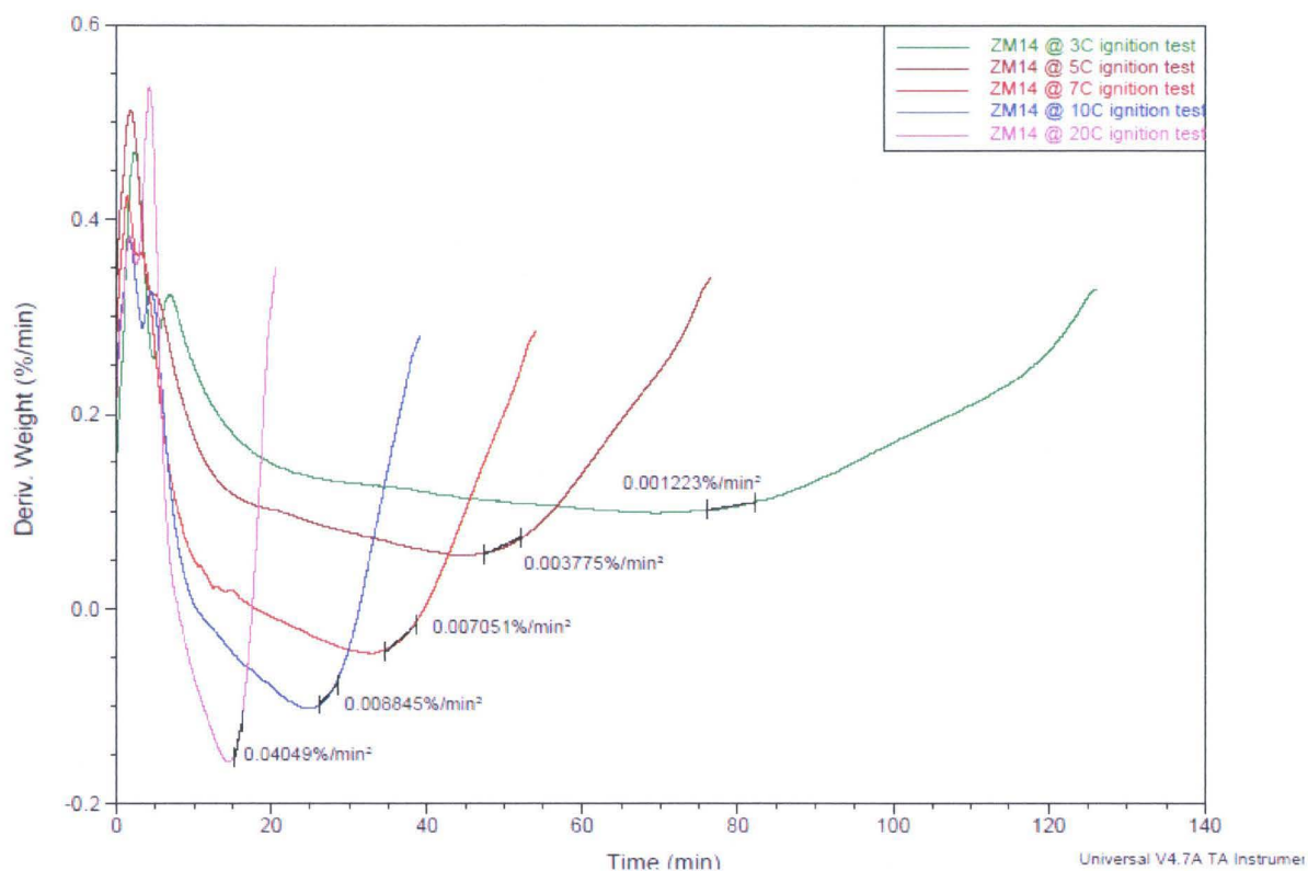
Figure 134: ZM14 Derivative curves and their slopes
