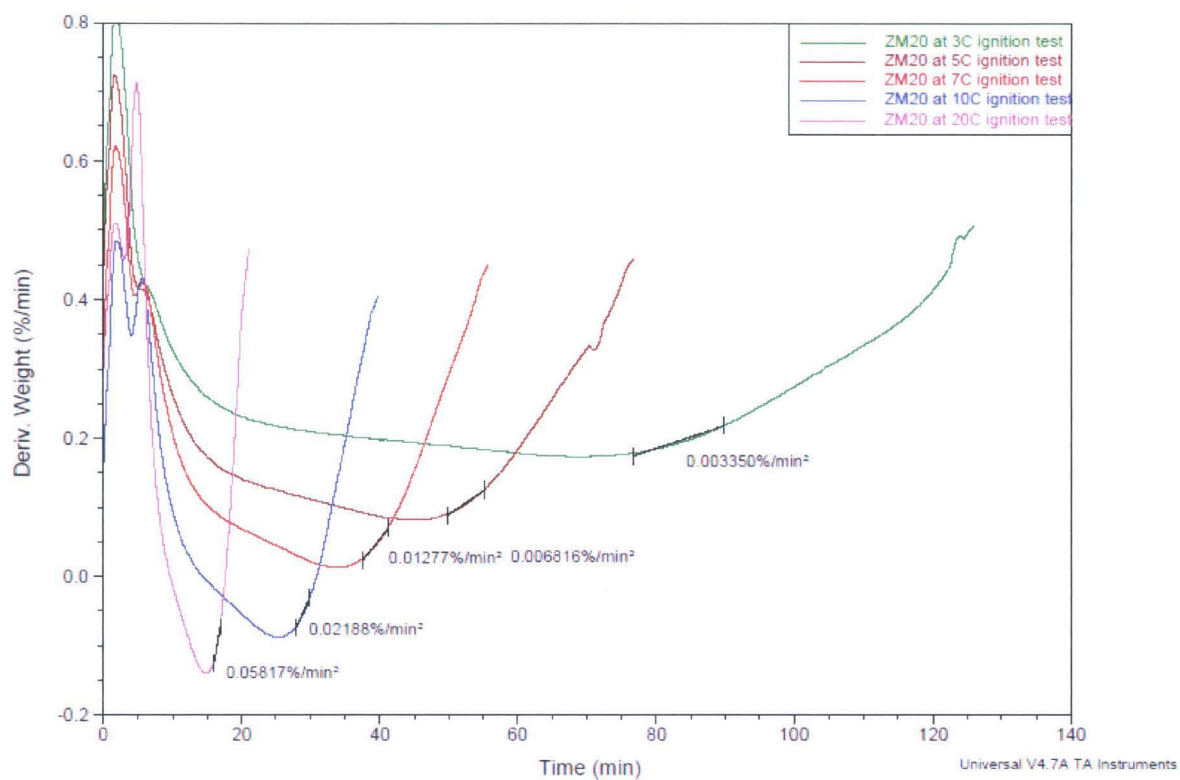
Figure 152: ZM20 Derivative curves and their slopes
