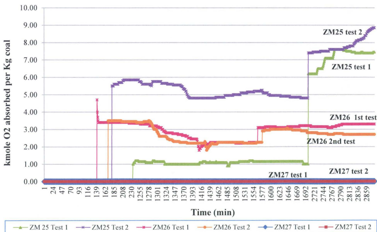
Figure 37: (ZM25, 26, &27) Smith Glasser test Repeatability Tests
