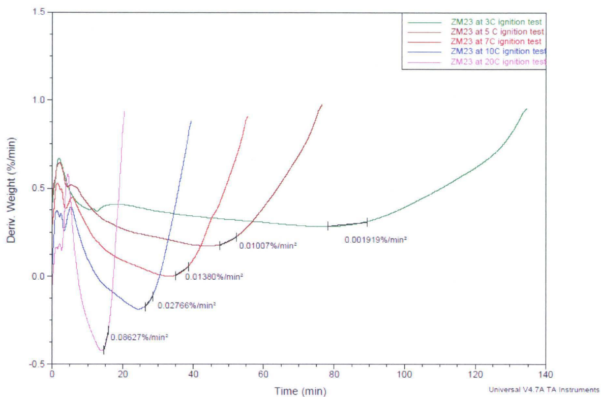
Figure 161: ZM23 Derivative curves and their slopes
