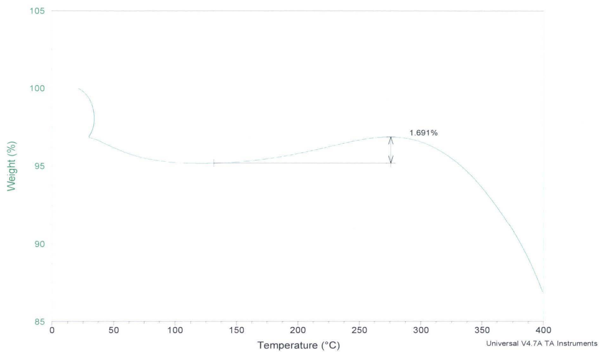
Figure 82: ZM17 O 2 Adsorption
