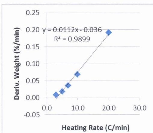
Figure 31: ZM9 Slope of derivative curves used to obtain R^2_{\text{graph}}
