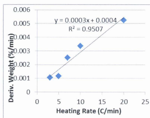
Figure 32: ZM9 Calculated Slope of derivative curves used R^2_{\text{calculated}}
