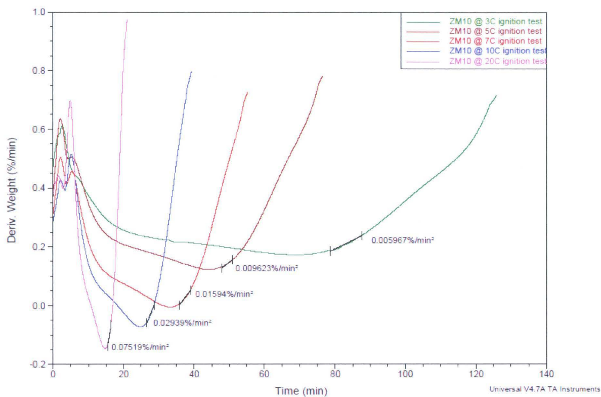
Figure 122: ZM10 Derivative curves and their slopes
