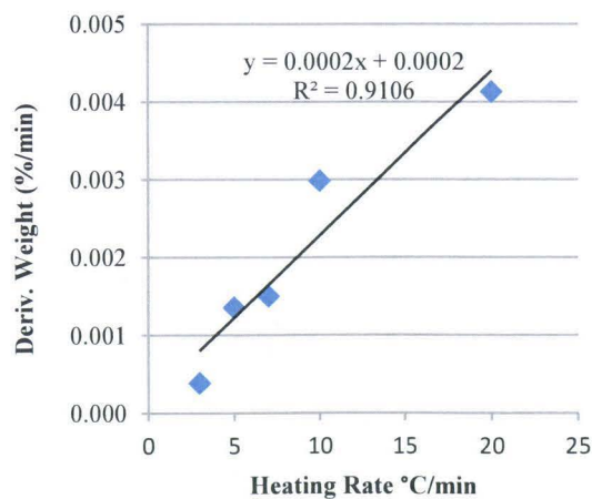
Figure 25: ZM 28 Calculated slope of derivative weight curves used to obtain R^2_{\text{calculated}}
