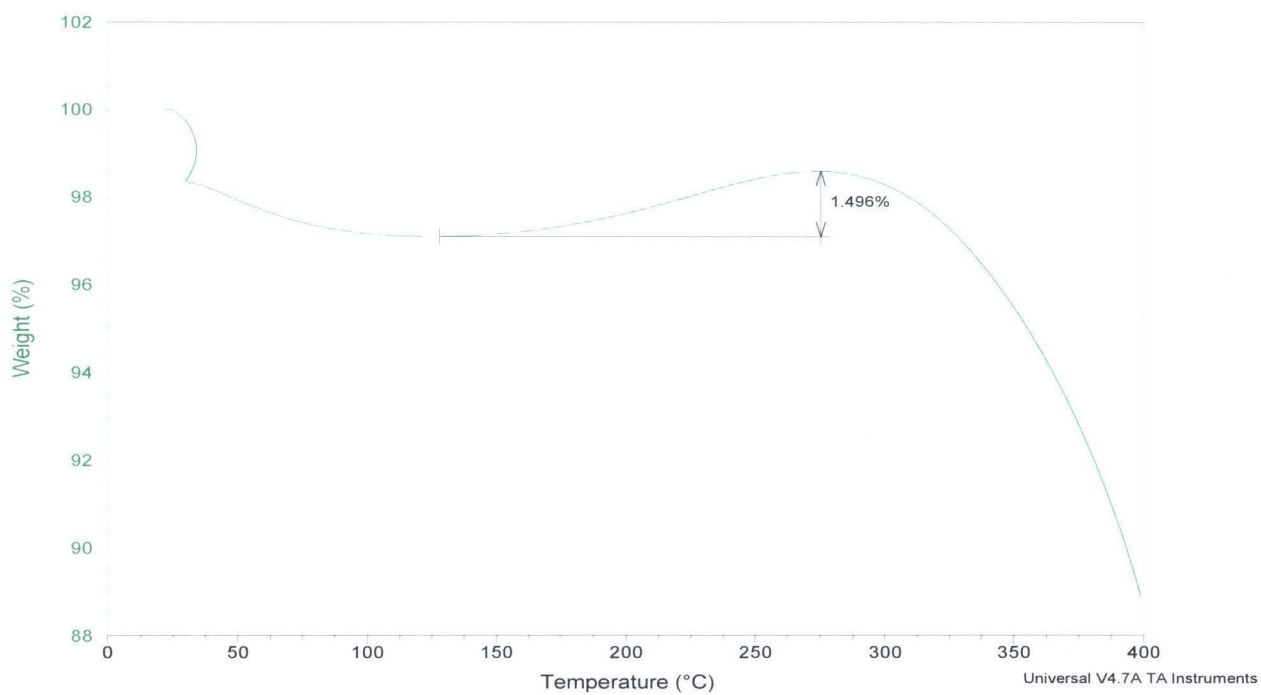
Figure 88: ZM23 O 2 Adsorption
