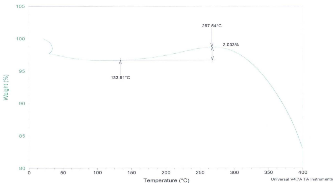
Figure 35: ZM9 O 2 Adsorption 1st test
