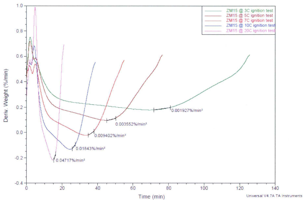
Figure 137: ZM15 Derivative curves and their slopes
