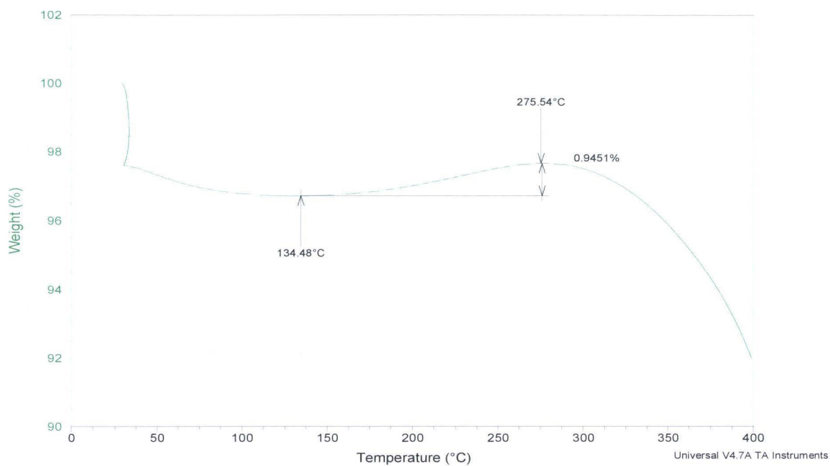
Figure 86: ZM21 O 2 Adsorption
