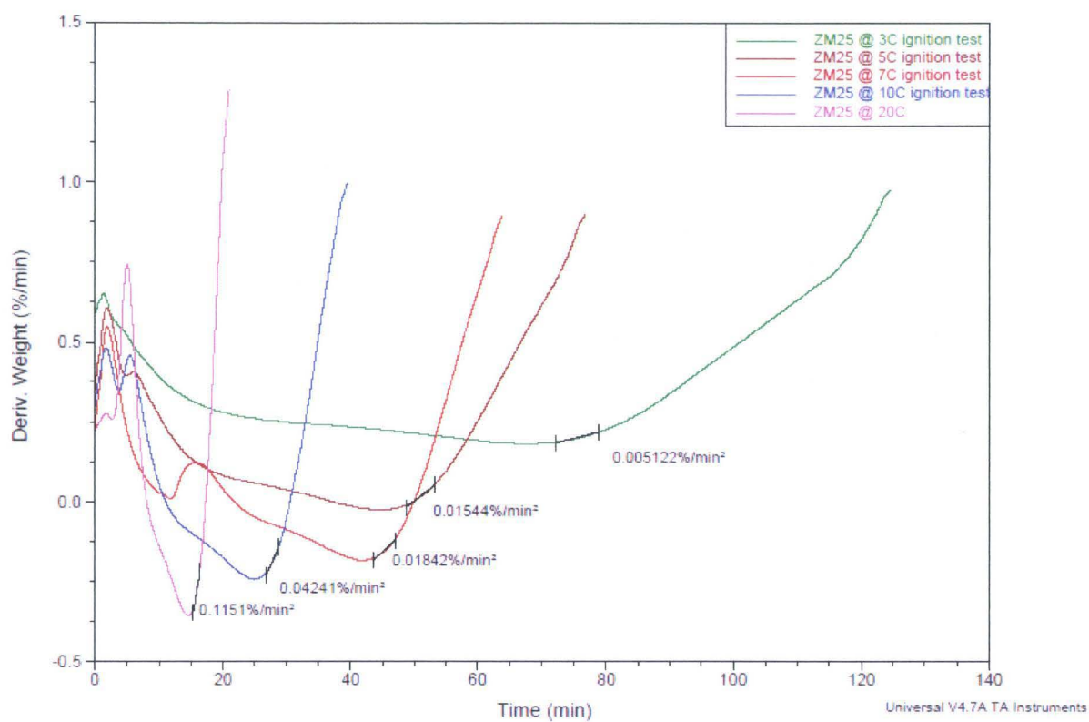
Figure 167: ZM25 Derivative curves and their slopes
