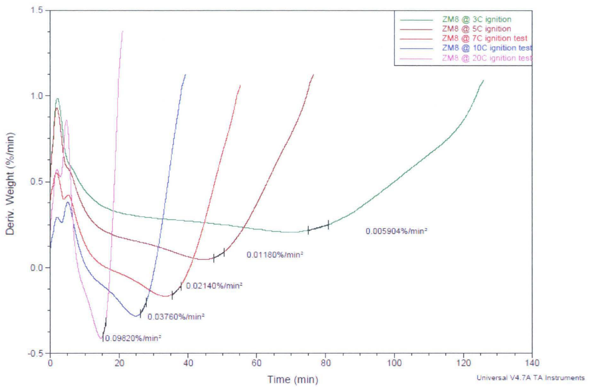
Figure 116: ZM8 Derivative curves and their slopes
