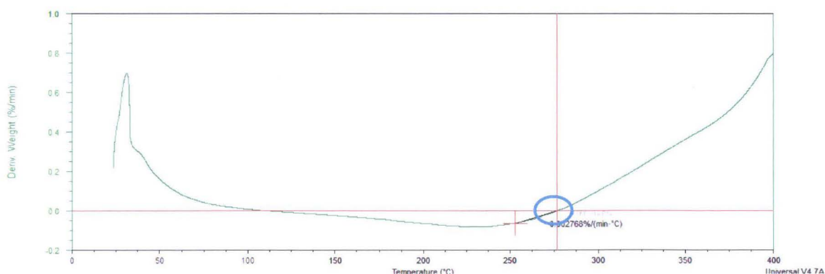
Figure 19: Derivative weight curve showing Ignition point
