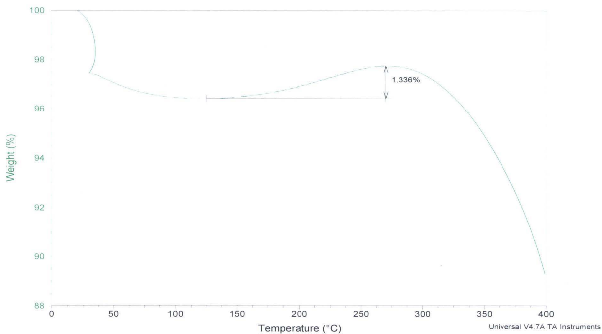
Figure 78: 13 O 2 Adsorption
