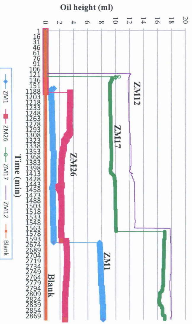
Figure 30: Smith-Glasser Oxidation Test – oil height
