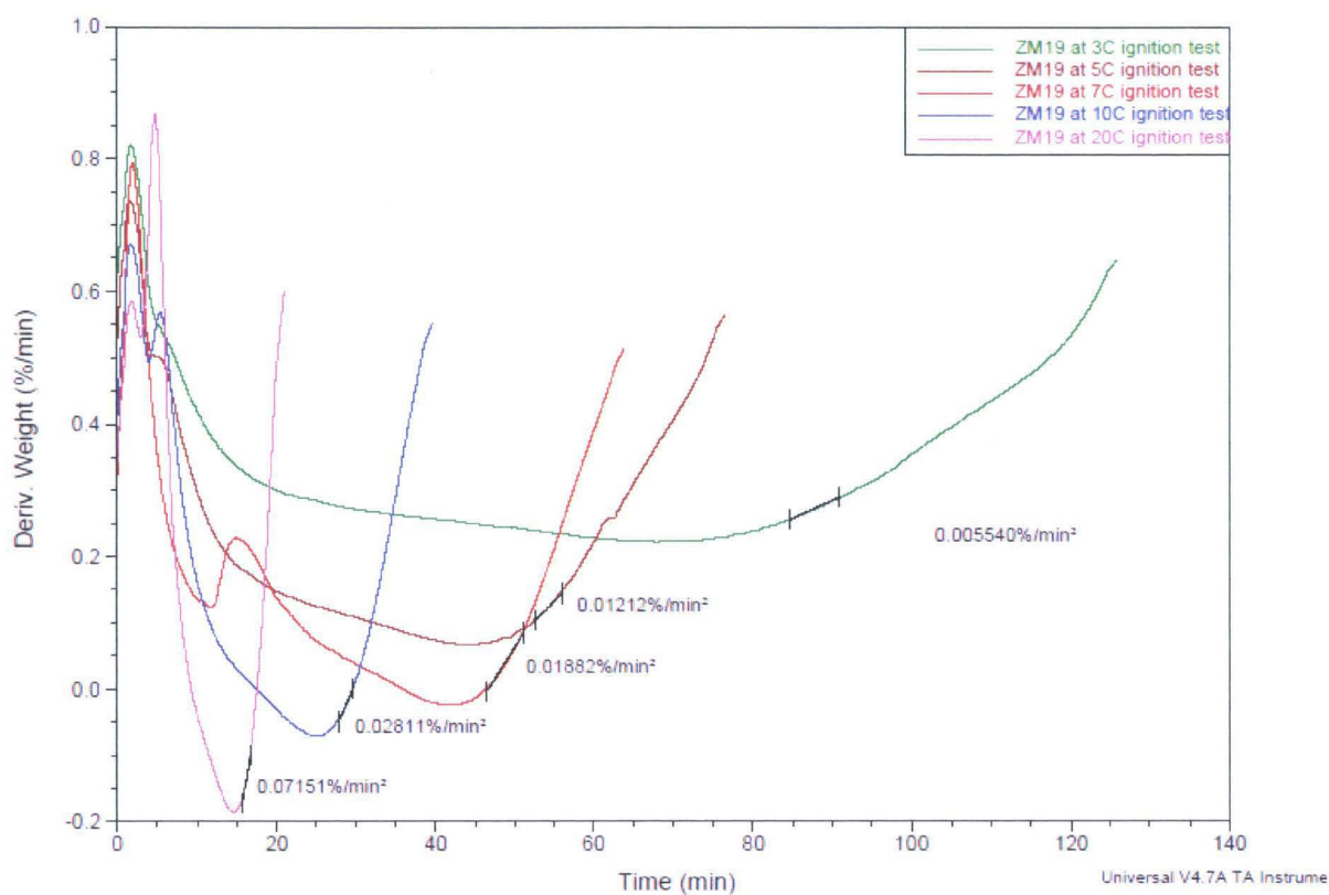
Figure 149: ZM19 Derivative curves and their slopes
