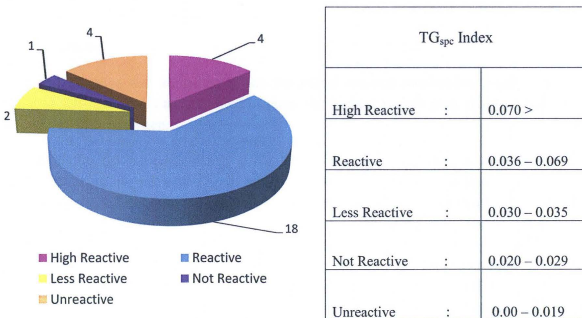
Figure 26: Coal Sample Reactivity using the TG_{spc} Index as a guideline set by Avila (2012)
