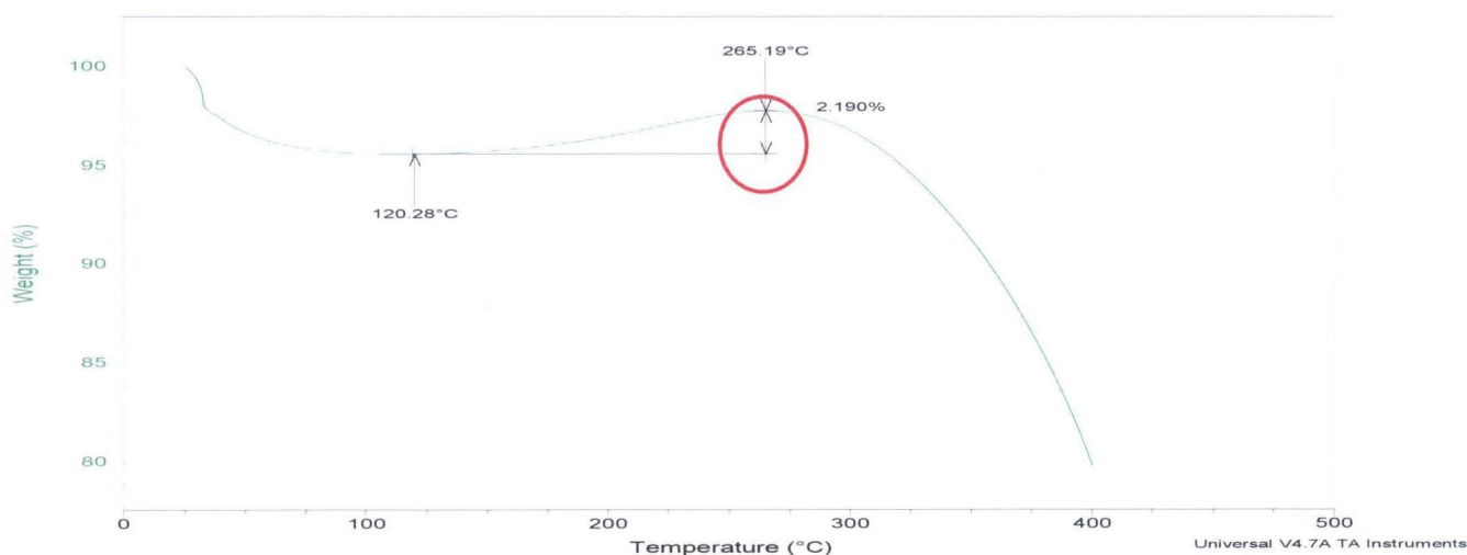
Figure 27: Sample ZM1 - O 2 Adsorption graph illustrating the weight increase at 3°C/min
