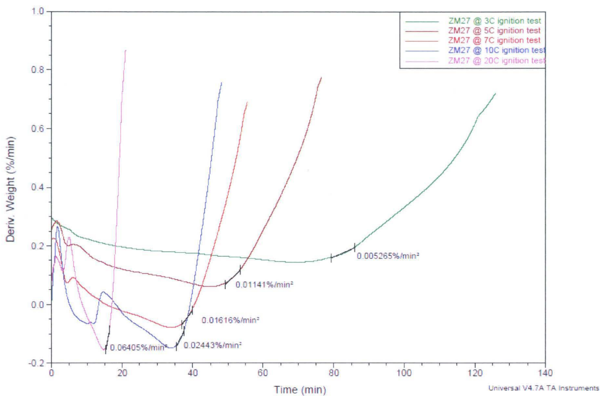
Figure 173: ZM27 Derivative curves and their slopes
