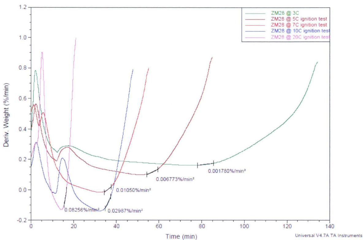
Figure 176: ZM28 Derivative curves and their slopes
