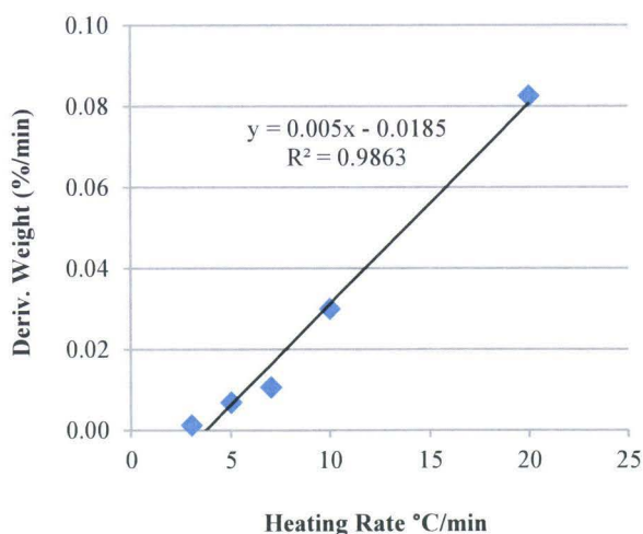
Figure 24: ZM 28 Slope of derivative weight curves (Linear segment) used to obtain used R^2 graph
