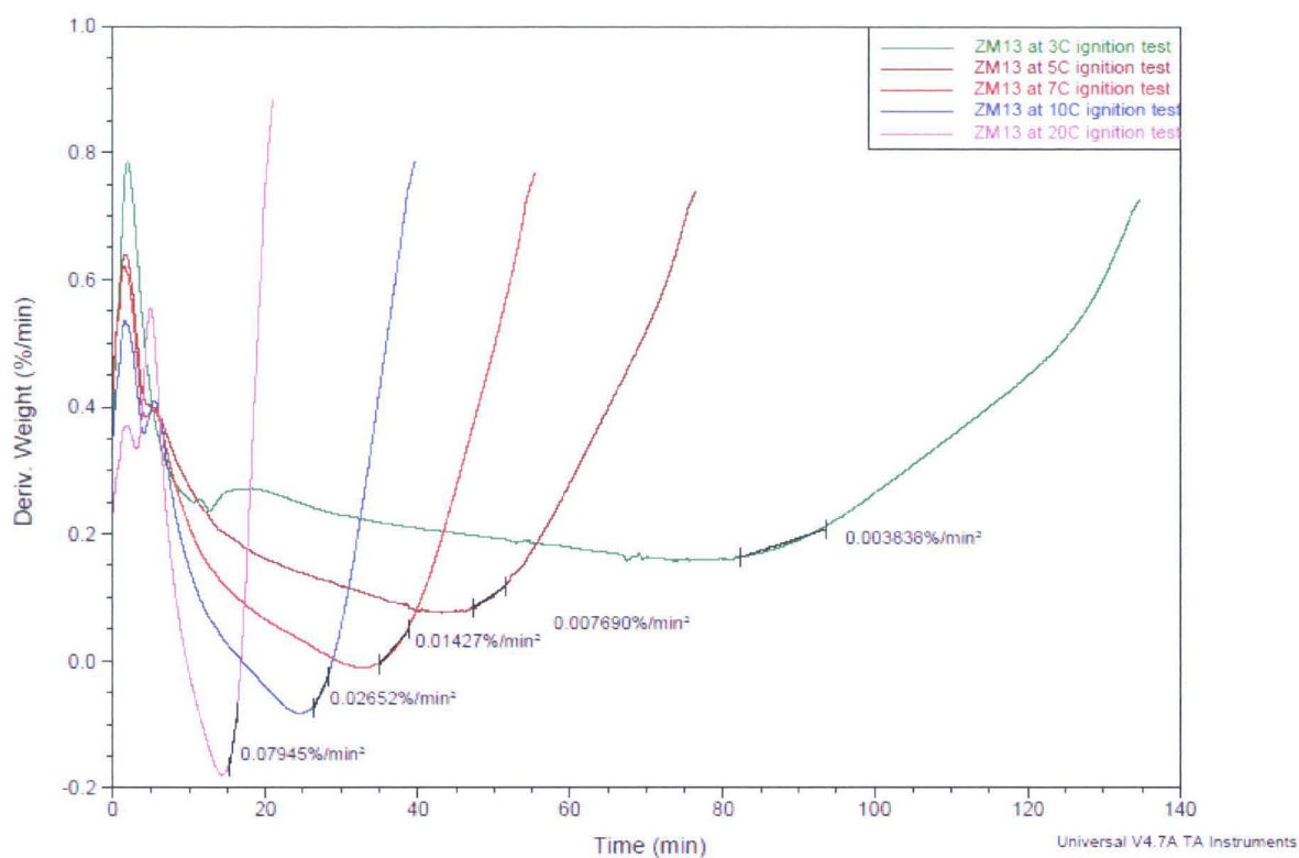
Figure 131: ZM13 Derivative curves and their slopes
