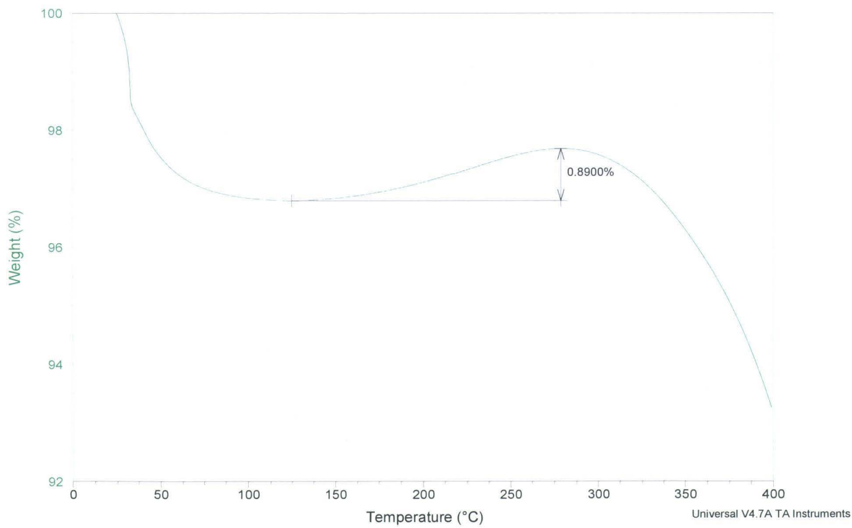
Figure 81: ZM16 O_2 Adsorption
