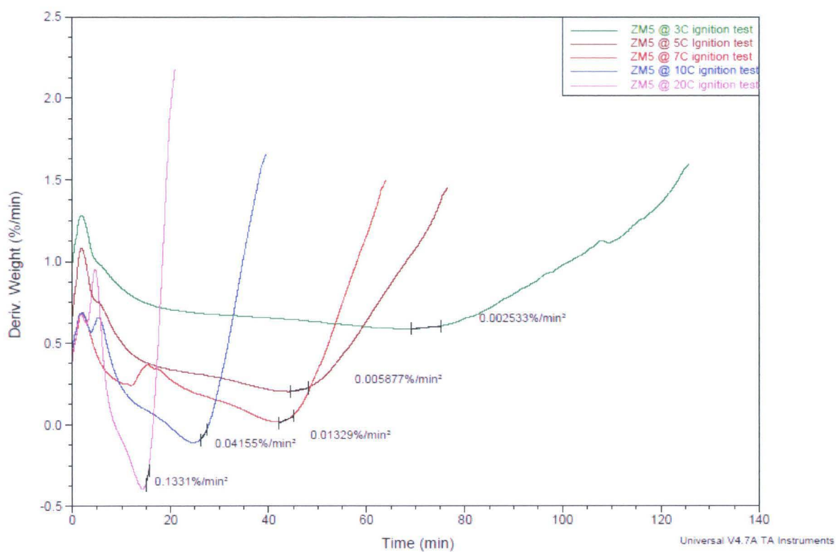
Figure 107: ZM5 Derivative curves and their slopes
