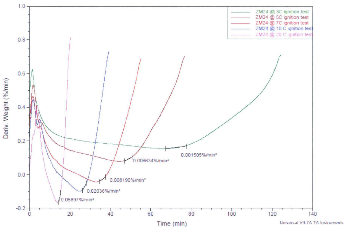
Figure 164: ZM24 Derivative curves and their slopes
