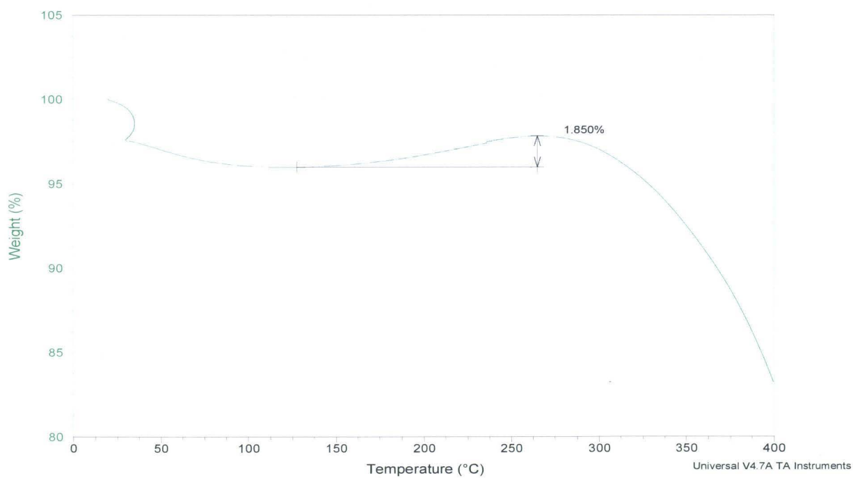
Figure 77: ZM12 O 2 Adsorption
