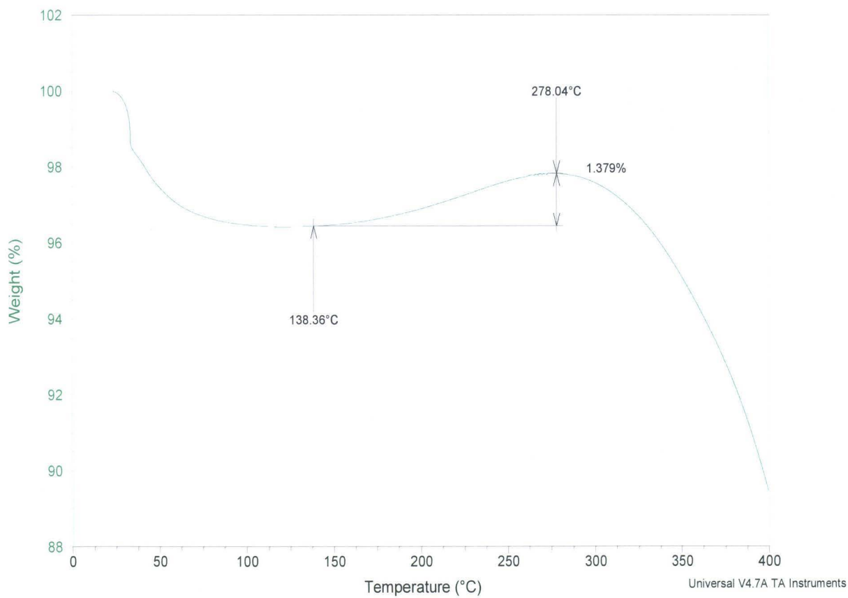
Figure 75: ZM10 O 2 Adsorption
