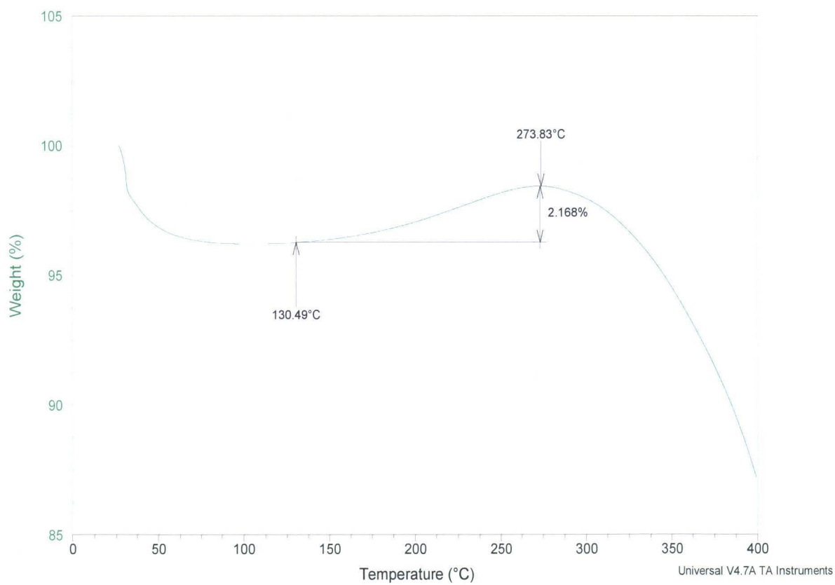
Figure 71: ZM6 O 2 Adsorption
