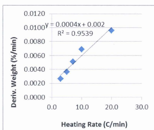
Figure 32: ZM9 Calculated Slope of derivative curves used R^2_{\text{calculated}}
