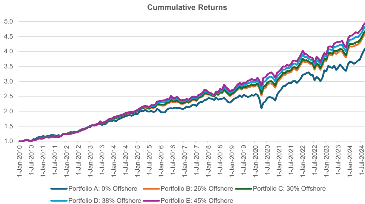
Figure 2: Cumulative Returns
