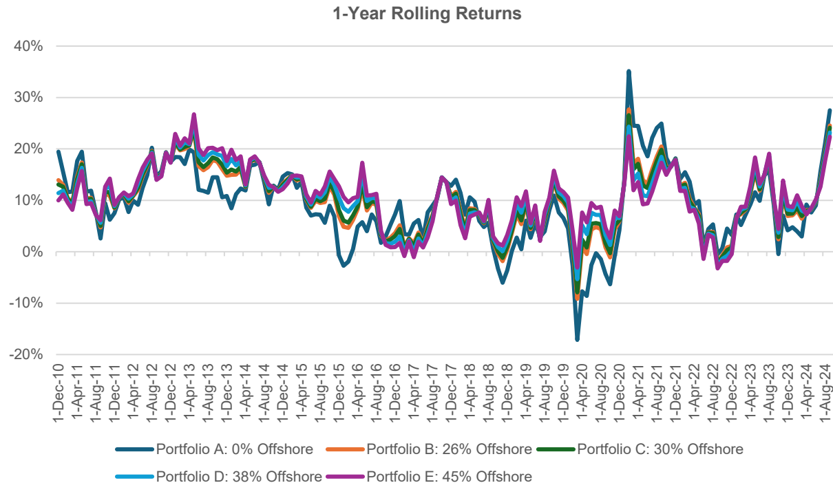
Figure 3: Rolling Returns
