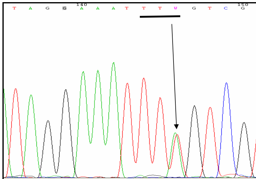
Figure 5.3: Chromatogram obtained by sequencing PCR products from A) Homozygous susceptible (SS), B) Homozygous resistant (RR) and C) Heterozygous resistant (RS) individual. The underlined nucleotide sequences indicate kdr region. The letter W in the underlined kdr nucleotide sequence of the heterozygote is the IUB code for A/T nucleotide. The arrow on the chromatogram indicates heterozygote situation (A and T peaks).
