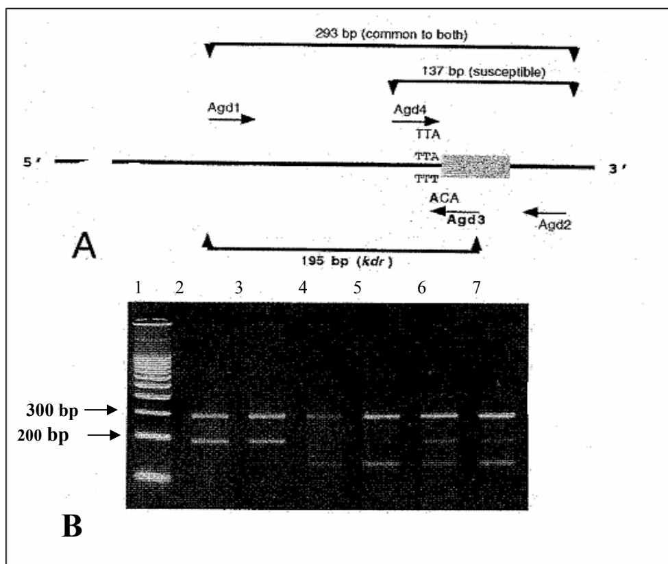
Figure 2.3 (A): Schematic representation of PCR-based diagnostic test for kdr detection. (B): PCR products separated on a 1.5% agarose gel (Martinez-Torres et al. 1998). Lane 1: molecular marker, Lane 2-3: homozygous RR, Lane 4-5: homozygous SS, Lane 6-7: heterozygous RS.
