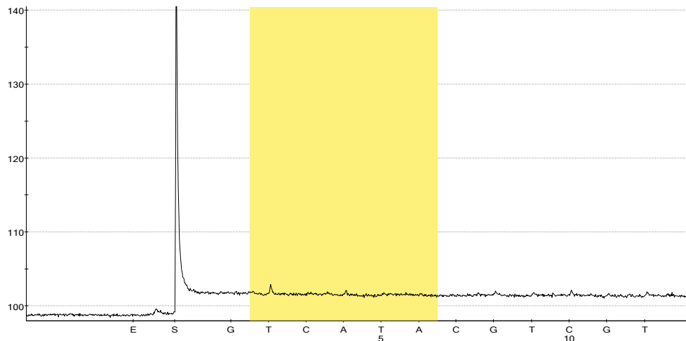
Figure 5.7: Pyrogram of PCR negative control generated from pyrosequencing reaction in one well of a 96 well plate. Initial addition of enzyme (E), substrate mixture (S) and sequential addition of nucleotides are shown on the x axis. The y axis (peak height) represents the number of nucleotide incorporated.
