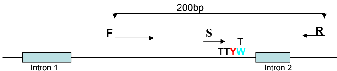
Figure 3.2: Schematic representation of a partial para sodium channel gene showing the kdr mutation and annealing sites of primers. F = forward primer, S = sequencing primer and R = Biotin labelled reverse primer. The Y is where the East African kdr mutation occurs and the W is where the West African kdr mutation occurs. Y can either be a T/C and W a T/A. This implies that for West Africa, the mutation is TTA to TTT and for East Africa from TCA or TTA. Y and W are International Union of Biochemistry (IUB) codes. The 200bp PCR product to be used for pyrosequencing reaction is biotin labelled.
