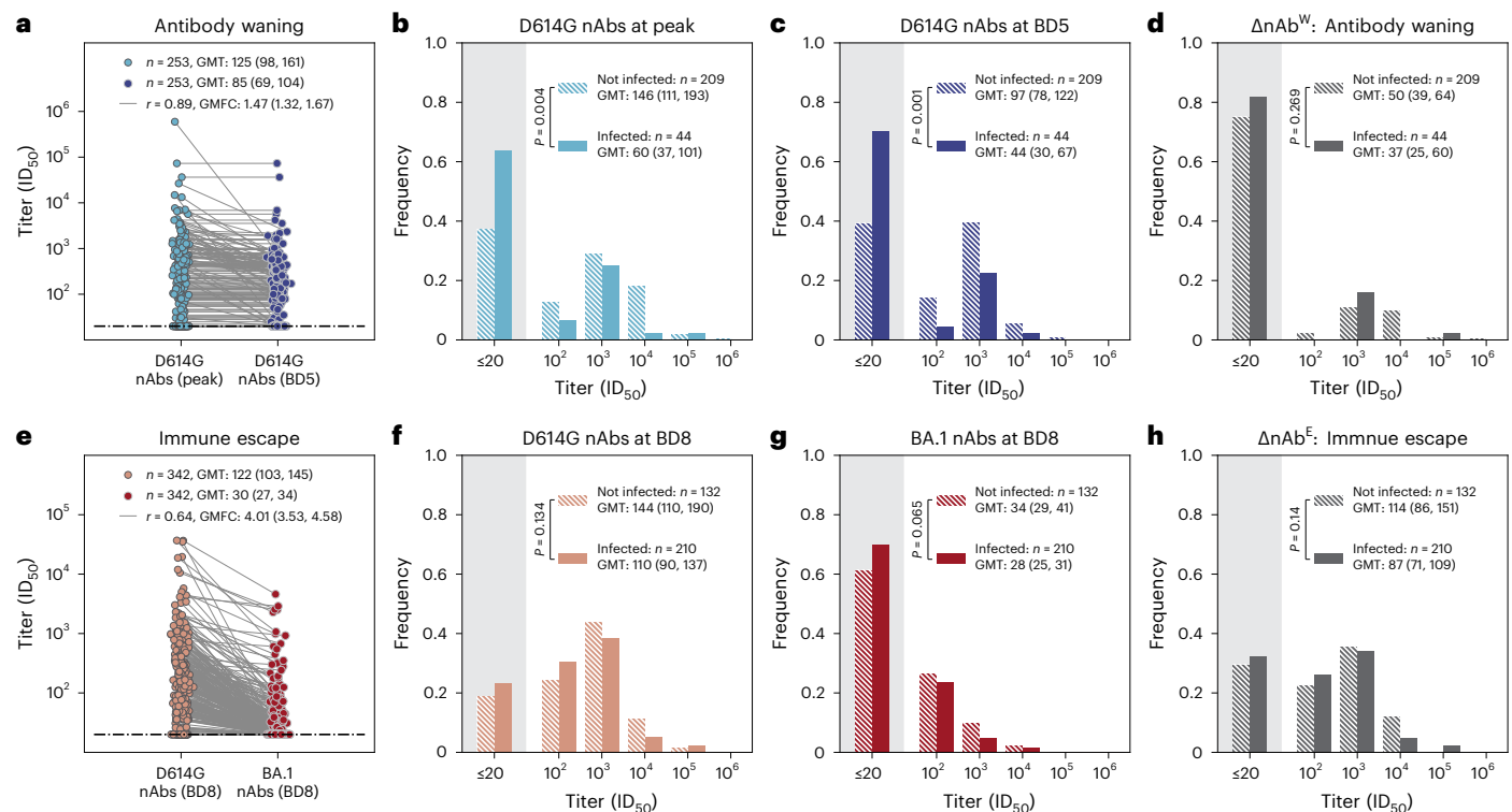
Fig. 2 | D614G and BA.1 nAb titers for the Delta wave and the Omicron wave analysis. a , For the Delta wave subgroup, the distribution of the peak D614G nAb titer up to BD5 (light blue dots) and the D614G nAb titer at BD5 (dark blue dots), among individuals who had one prior SARS-CoV-2 infection before BD5. Each dot represents one individual, with two measurements of the same individual connected through a gray line. GMFC, geometric mean fold change from peak D614G titer to that at BD5; r , Pearson correlation coefficient. b , For the Delta wave subgroup, the distribution of the peak D614G nAb titer up to BD5, stratified by individuals who were infected during the Delta wave (solid bar) versus those who were not infected (dashed bar). The independent-samples t -test (two-sided) was used to determine the statistical significance ( P value reported in the legend) of the difference between the GMTs of the two groups. c , Same as b but for
