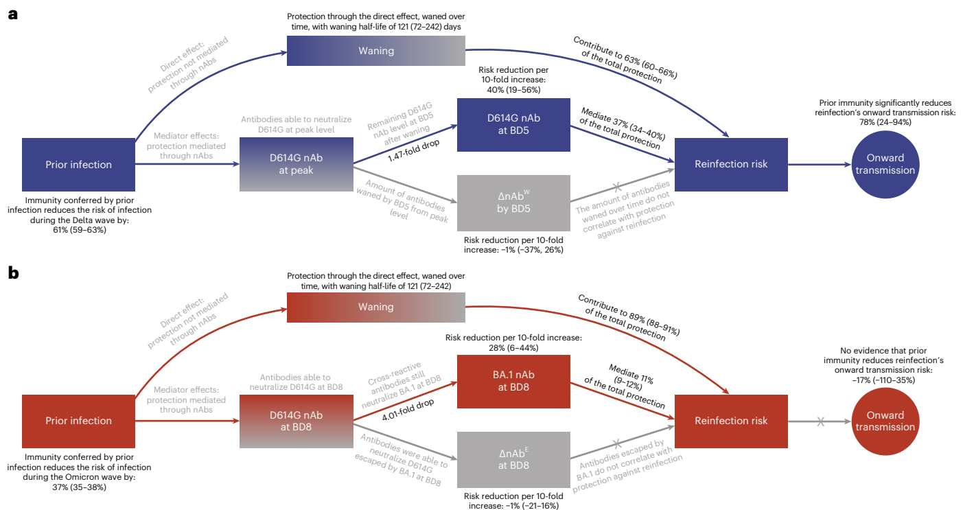
Fig. 3 | Causal diagrams for the mediation analyses. a , Causal diagram of the Delta wave mediation analysis showing the hypothesized relationship between prior immunity (induced by prior SARS-CoV-2 infection) and SARS-CoV-2 infection (outcome of interest) during the Delta wave. The mediators of interest are D614G nAbs at BD5 and \Delta nAb W (the quantity of D614G nAbs waned from peak level to that at BD5). The direct effect represents protection operating through immune mechanisms other than the mediators of interest. We hypothesized that the direct effect could wane over time since the initial immune exposure. For the prospective cohort data, both mediator–outcome confounding and exposure–outcome confounding factors need to be adjusted for the mediation analysis, as the immune exposure (prior SARS-CoV-2 infection) was not randomly assigned (unlike SARS-CoV-2 randomized control vaccine trials where vaccination was
