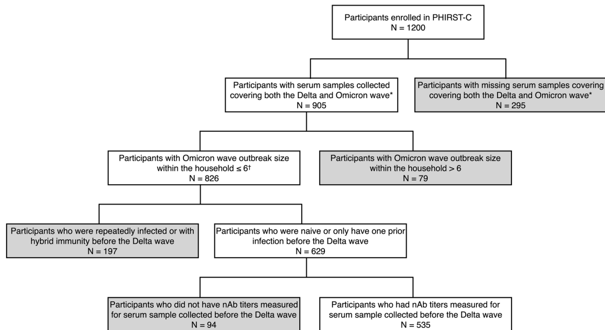
Extended Data Fig. 2 | Flowchart of participants included in the Omicron-wave subgroup analysis. Grey boxes represent participants excluded from the Omicron-wave subgroup analysis. *Based on a previously published study 31 .
