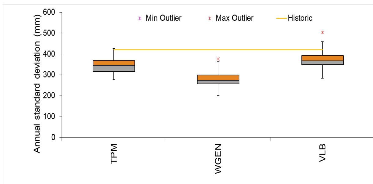
Figure 5.1-11: Comparison of the annual standard deviation values generated from the methods for the Hebron station
