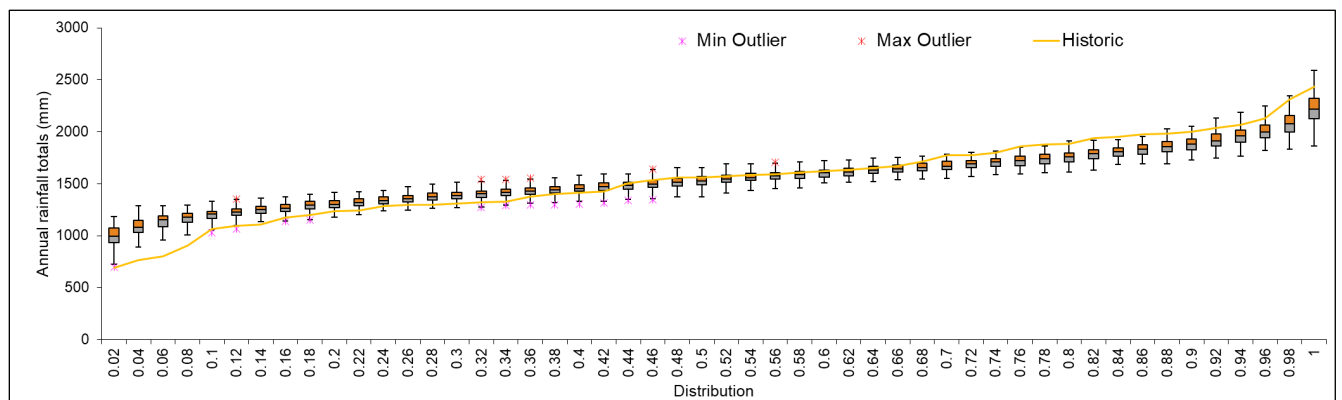
Figure 4.2-7: Rainfall distribution curve of the annual totals for data generated using WGEN Method for Hebron station
