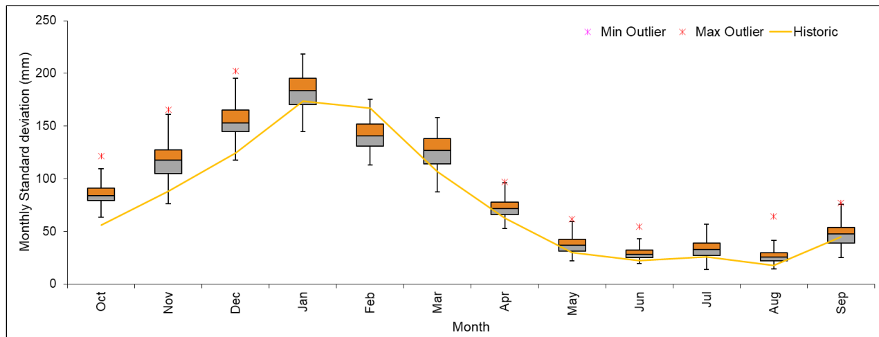
Figure 4.3-5: Standard deviation values of monthly data generated using VLB Method for Hebron station
