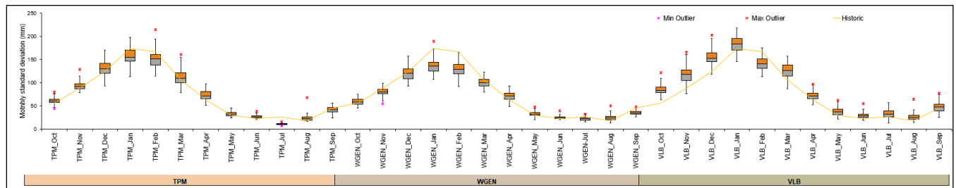
Figure 5.1-7: Comparison of the monthly standard deviation for the methods for the Hebron station
