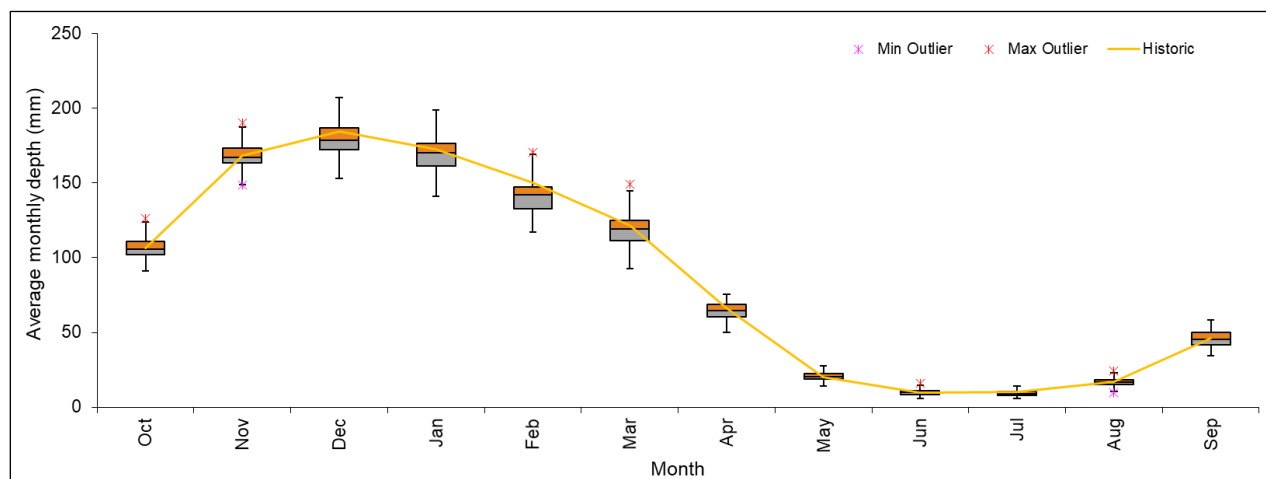
Figure 4.1-22: Averages of monthly data generated using TPM Method for Nelshoogte station
