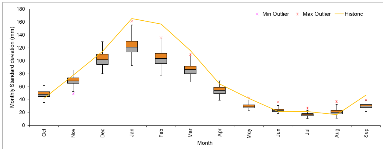
Figure 4.2-13: Standard deviation values of monthly data generated using WGEN Method for Welgevonden station
