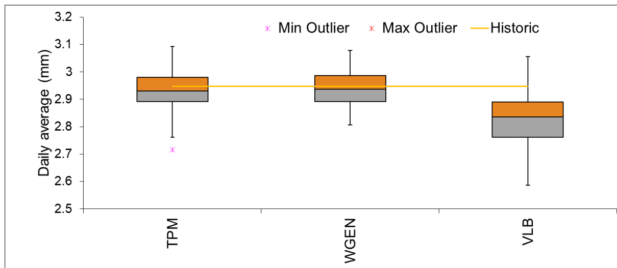
Figure 5.3-2: Comparison for the daily average values generated from the methods for Nelshoogte station
