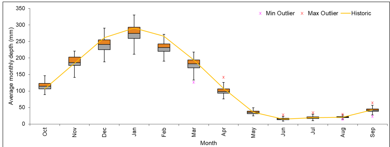
Figure 4.3-3: Averages of monthly data generated using VLB Method for Hebron station
