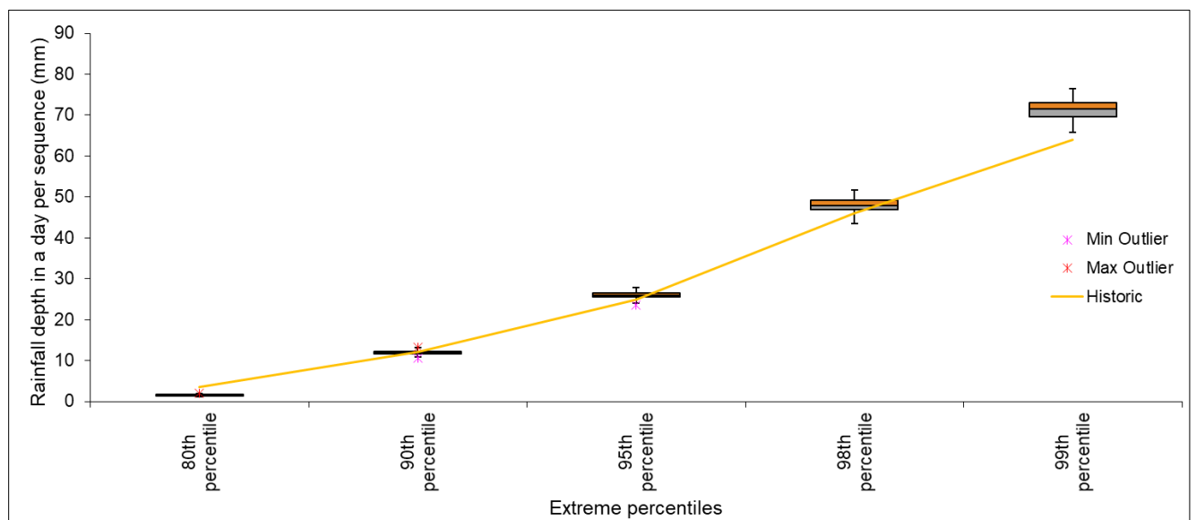
Figure 4.1-3: Percentiles of daily data generated using TPM Method for Hebron station
