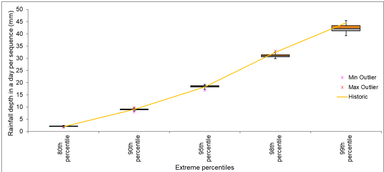
Figure 4.1-21: Percentiles of daily data generated using TPM Method for Nelshoogte station
