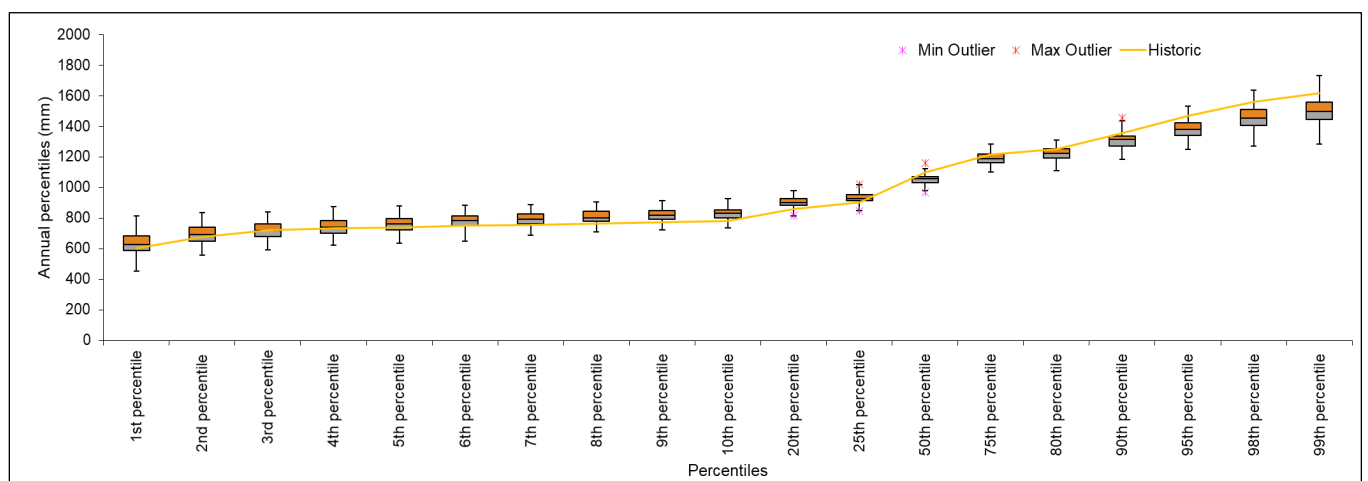
Figure 4.1-27: Annual percentiles of data generated using TPM Method for Nelshoogte station
