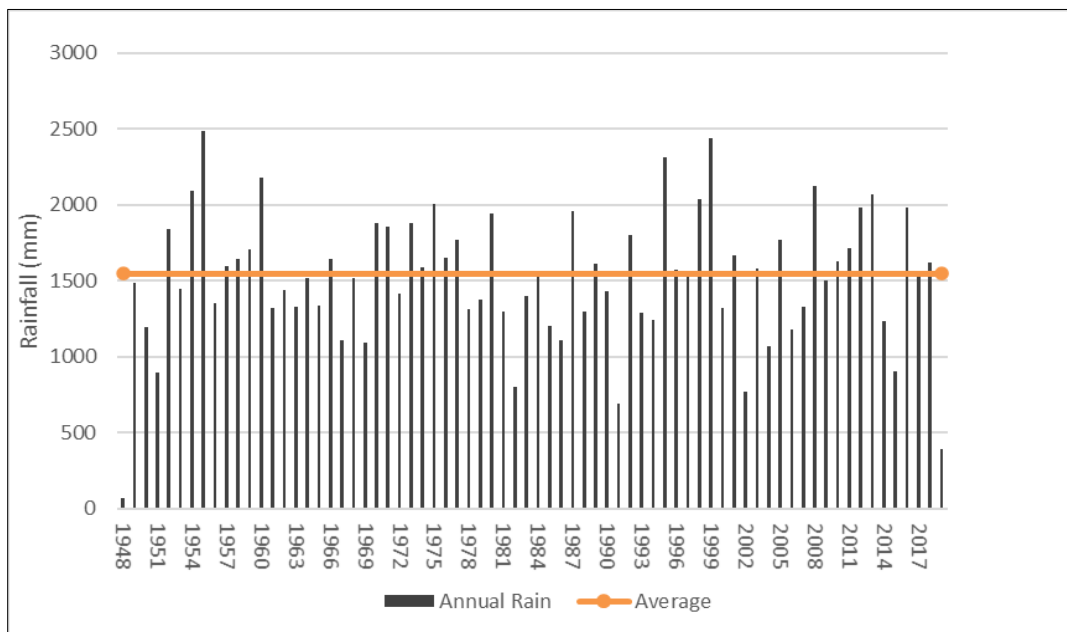
Figure 3-4: Annual rainfall depths measured at Hebron (0594760 W) rainfall station
