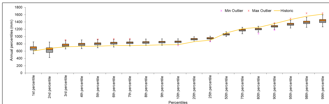
Figure 4.3-24: Annual percentiles of data generated using VLB Method for Nelshoogte station
