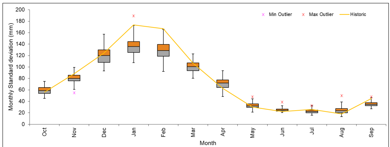
Figure 4.2-5: Standard deviation values of monthly data generated using WGEN Method for Hebron station
