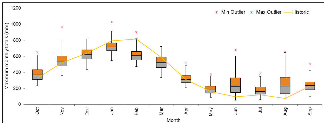
Figure 4.3-4: Maximum values of monthly data generated using VLB Method for Hebron station
