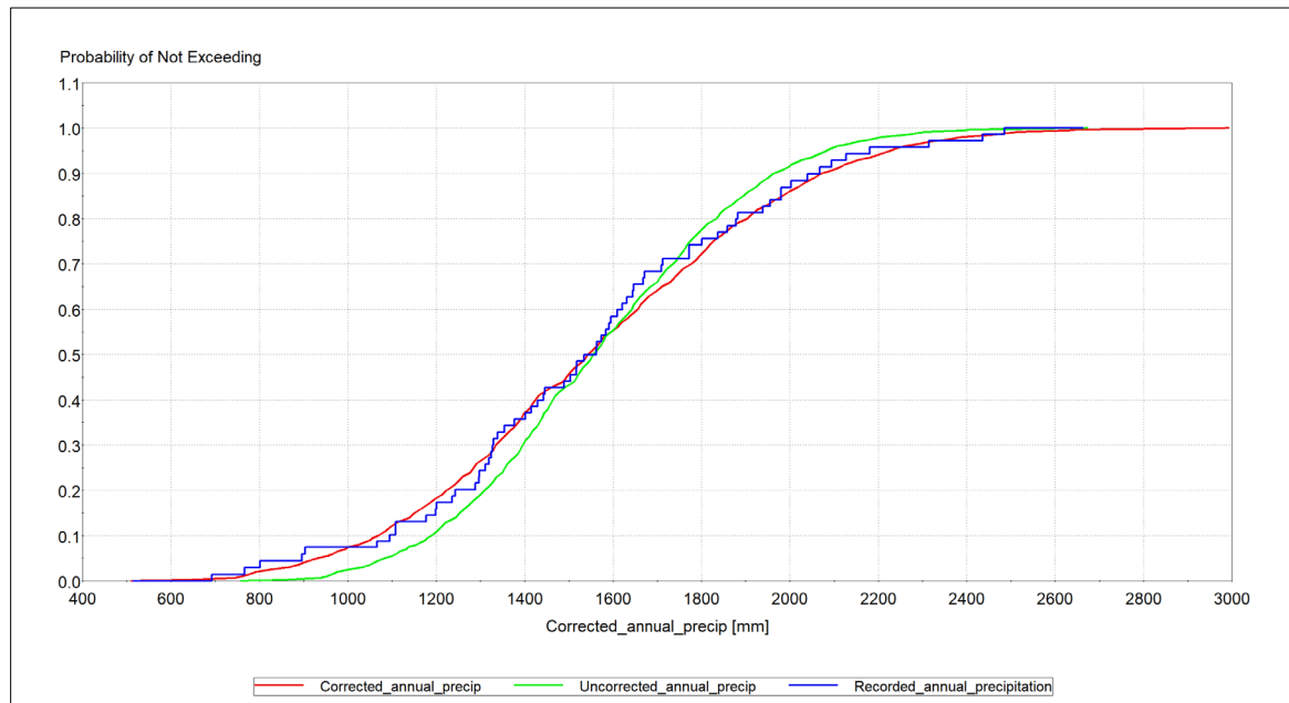
Figure 4.1-1: Comparison of the annual probability of exceedance for the generated annual precipitations to the recorded data for Hebron rainfall station
