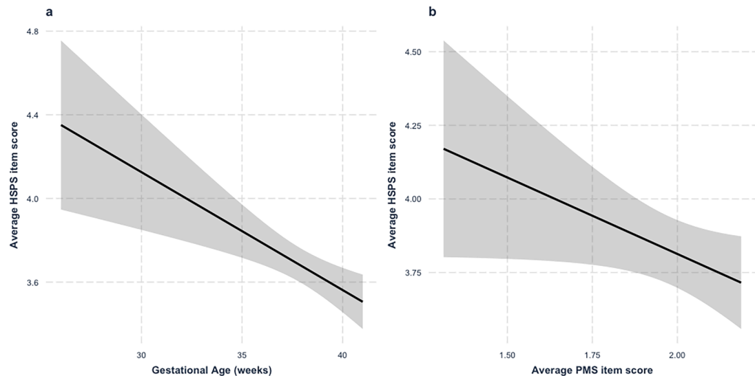
Fig. 1. Early predictors of adult SPS levels. While controlling for the effects of other variables, including sex, birthweight, maternal education, socioeconomic status, and internalising and external-ising behaviour (at age 7), (a) gestational age significantly ( p < .001 ) predicted SPS levels assessed at ages 28–29 amongst members of the Birth to Twenty Plus cohort ( n = 858 ). A longer gestational period correlated with a lower average item score on the Highly Sensitive Person scale. (b) In a smaller subset of participants with available data ( n = 357 ), prenatal maternal stress (PMS) emerged as a marginal predictor of SPS ( p = .05 ), suggesting that highly sensitive adults were more likely to be born to mothers experiencing stressful pregnancies. The grey shaded area represents the 95% confidence interval.
