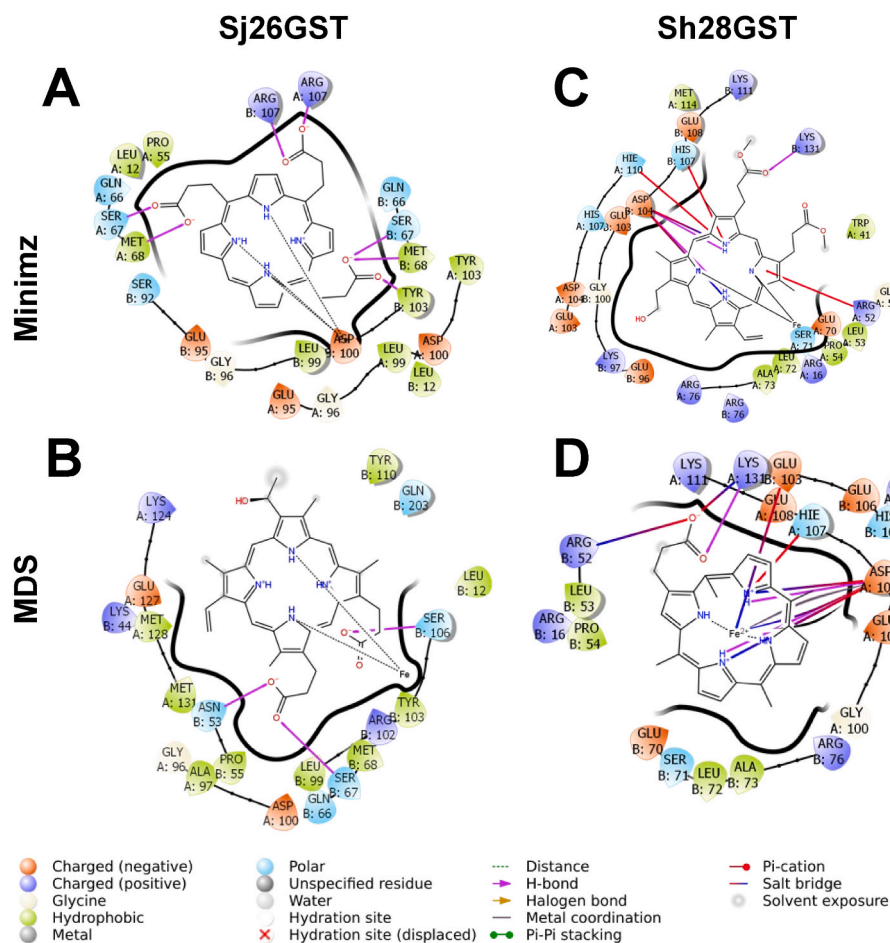
Fig. 7. 2D interaction plot of top poses of Sj26GST Minimized (A) and MD-simulated (C), respectively in complex with ligands. Similarly, the same information was captured for Sh28GST Minimized (B) and MD-simulated (D). The residues are within 4 Å from the ligand. The image was generated using the Maestro 2D interaction diagram implemented in Schrödinger Maestro v13.
