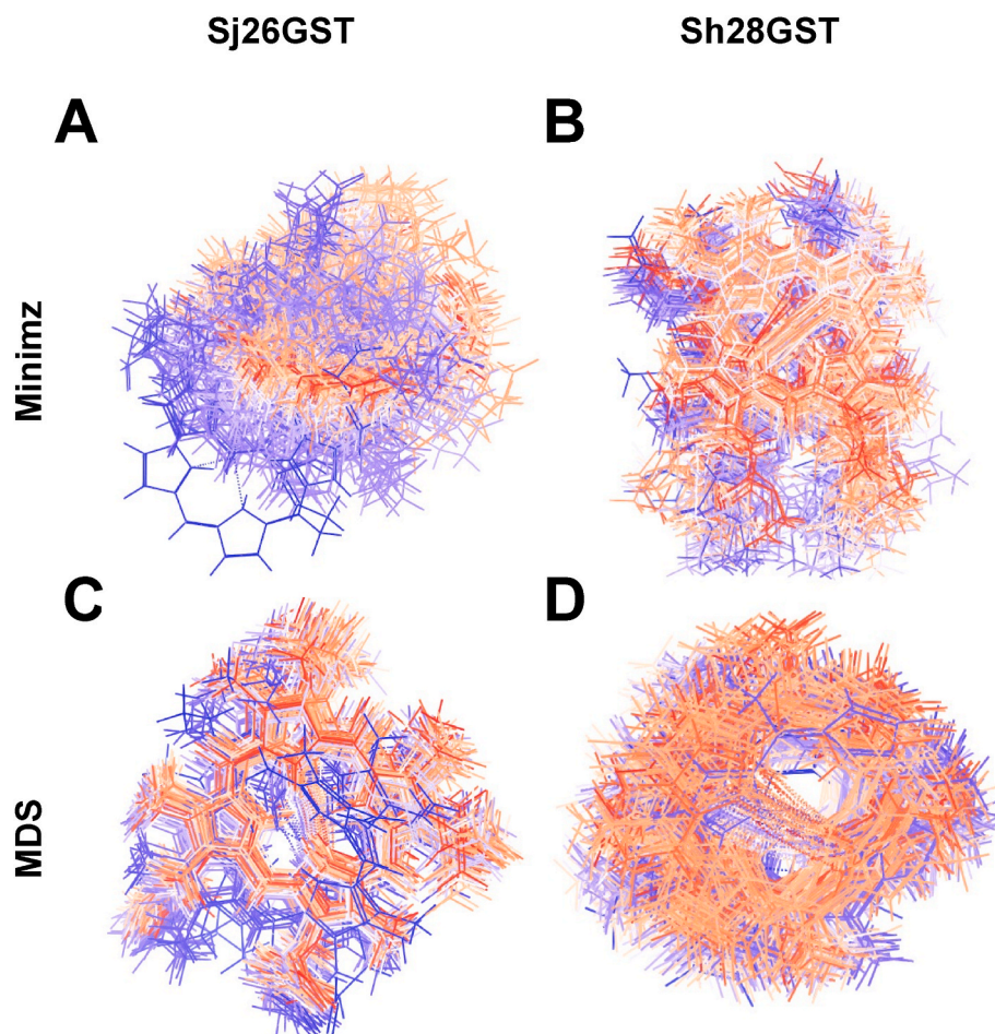
Fig. 6. The superimposed images of the top ligands' poses over the 500 ns simulation in the respective binding pocket. The Minimized systems, A CID: 122690402 and B CID: 70415734 show greater fluctuations than the MD-simulated ligands, C CID: 137797052 and D CID: 69301914.
