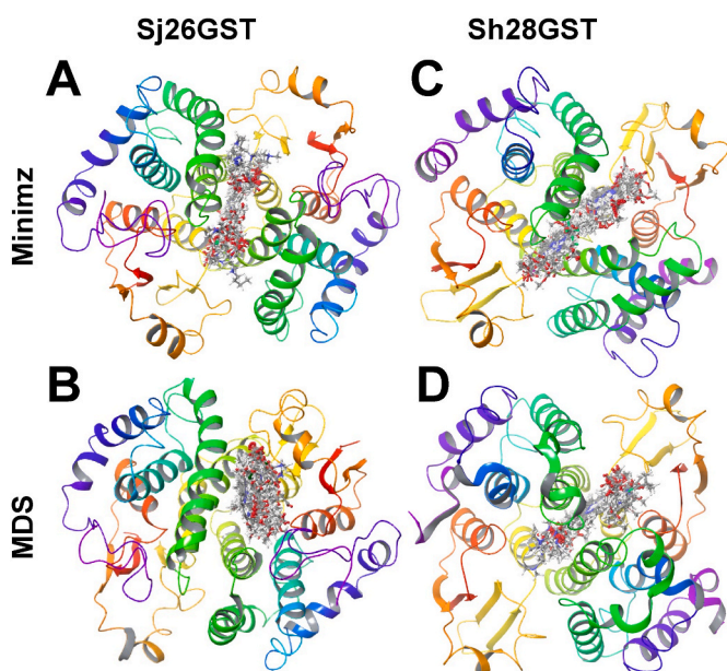
Fig. 3. The preferred binding site for protoporphyrin IX-like compounds in Schistosoma GSTs. Sj26GST Minimized ( A ), Sh28GST Minimized ( C ) and Sh28GST MD-simulated ( D ) tend to lean towards the L-site at the dimer interface and some ligands projections towards the H-site, whereas Sj26GST MD-simulated ( B ) on the other hand is towards the H-site.
