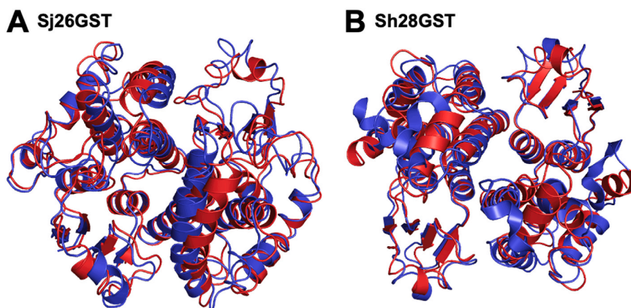
Fig. 2. Superimposed ribbon structures of energy-minimized protein structure (red) and average molecular dynamic simulated structure (blue) of A. Schistosoma japonicum 26-kDa glutathione transferase (Sj26GST) and B. Schistosoma haematobium 28-kDa glutathione transferase (Sh28GST). The structures were aligned using the Align tool in PyMol, whereby the RMSD for Sj26GST (PDB 6RWD) was 1.47 Å; then for Sh28GST (PDB 1OE8), it was 1.53 Å. (For interpretation of the references to colour in this figure legend, the reader is referred to the Web version of this article.)
