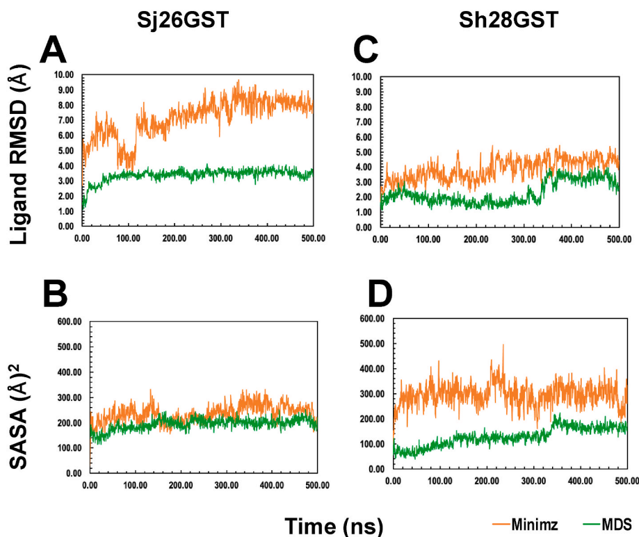
Fig. 5. The root mean square deviation of the ligand with respect to the receptor ( A and C ) and corresponding solvent-accessible surface area ( B and D ). A single protein structure in different models chose different ligands that have variable stability and solvent exposure.
