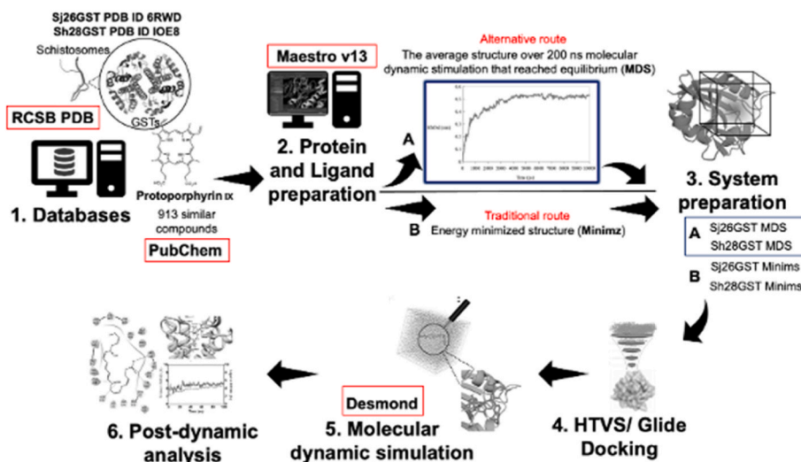
Fig. 1. Schematic representation of the computational workflow for identifying porphyrin-based antihelminthic compounds targeting schistosomiasis. The workflow incorporates an additional molecular dynamic (MD) simulation step following protein preparation to yield equilibrated structures. This approach enhances structural accuracy compared to traditional energy-minimized structures used in computational modelling.
