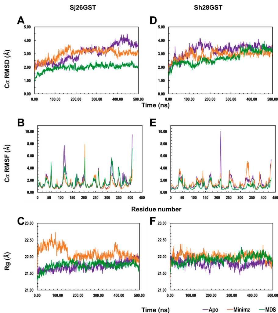
Fig. 4. Trajectory of 500 ns simulation showing the root mean square deviation (RMSD) of A/D C \alpha atoms and B/E root mean square fluctuation per residue side chain as well as C/F radius of gyration (Rg) for the Apo-proteins, Sj26GST and Sh28GST, respectively and ligand-bound complex of the various models.
