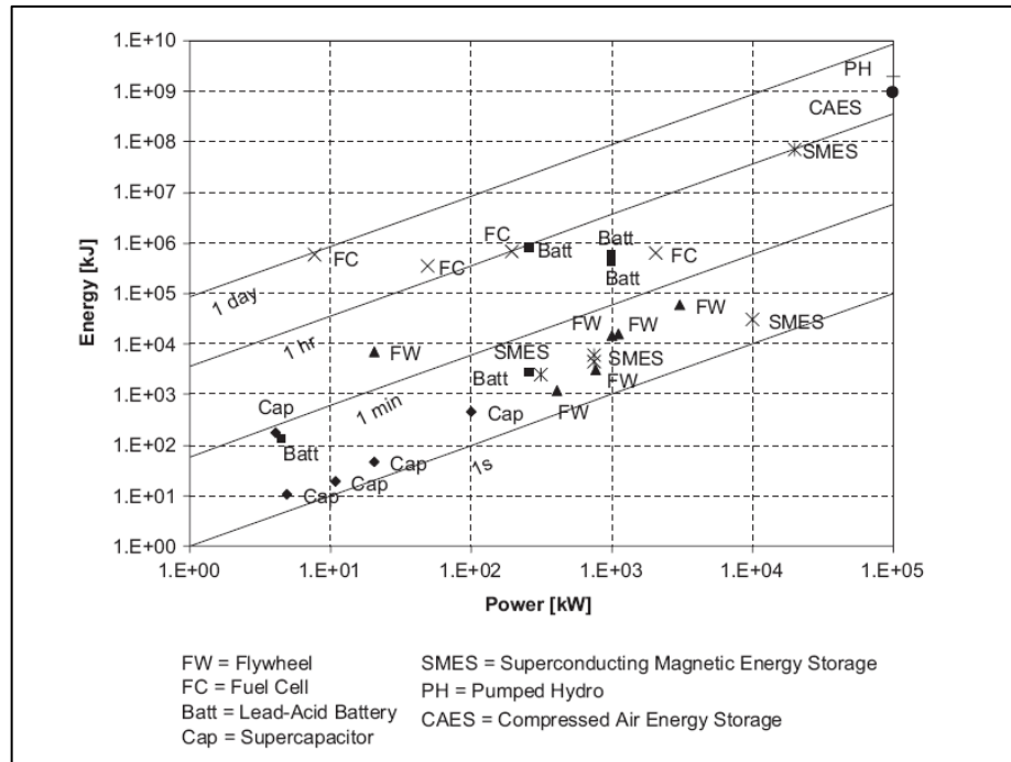
Figure 1 - Performance of Various Energy Storage Technologies (Grazzini and Milazzo, 2007)
