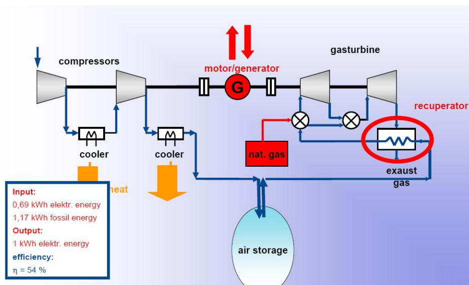
Figure 23 - Process Flow Diagram of McIntosh CAES System
