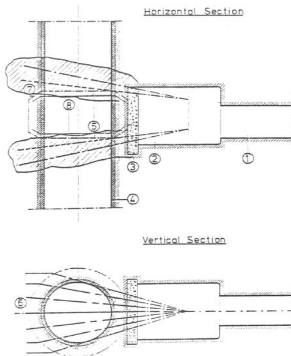
Fig.1. Description variant (a). 1 = Work gallery; 2 = Drilling chamber; 3 = Concrete wall; 4 = Shaft lining; 5 = Shaft-plug; 6 = Freeze tubes; 7 = Plug seats; 8 = Concrete reinforcement
