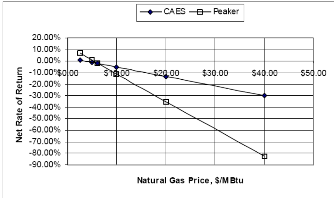
Figure 6 - NRR Plots for Scenario 1 (DeCorso et al, 2006)
