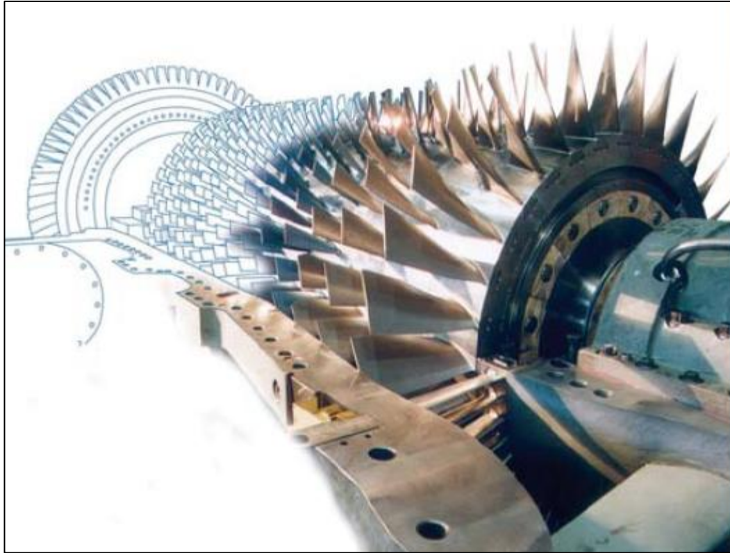
Figure 13 - GE CAES Turbine for ADELE (RWE Power, 2010)
