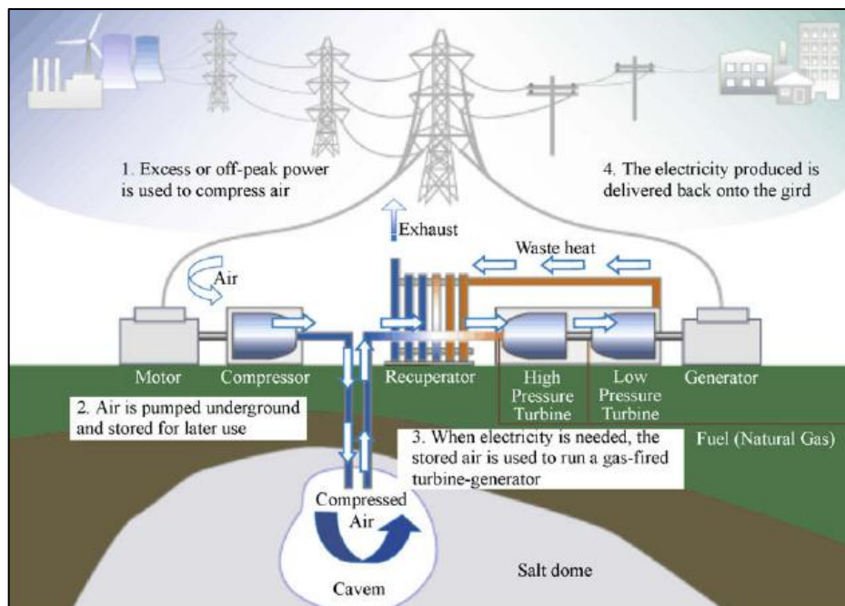
Figure 5 - Diagram of CAES principle (Chen et al, 2009)
