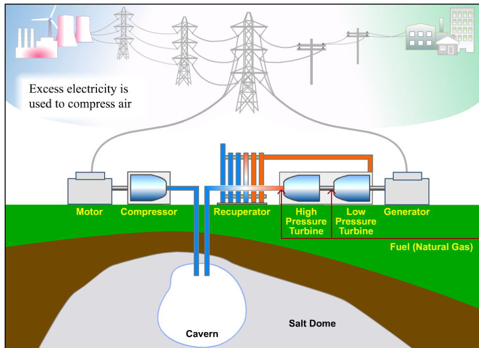
Figure 12 - Typical CAES equipment arrangement (Ridge Energy Storage, 2006)
