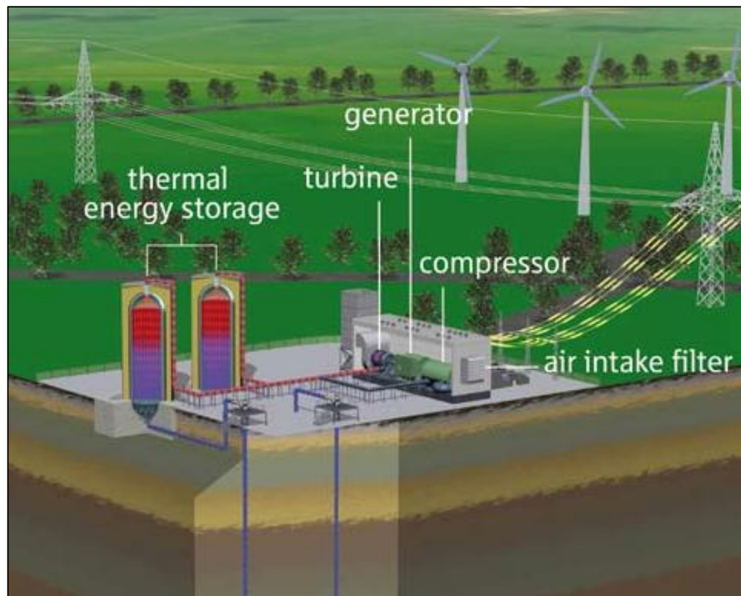
Figure 14 - Proposed ADELE CAES Plant in Germany (RWE Power, 2010)
