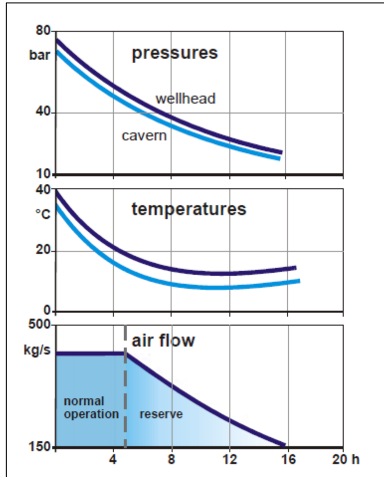
Figure 17 - Huntorf Cavern Operating Characteristics During Expansion (Crotagino, 2001)
