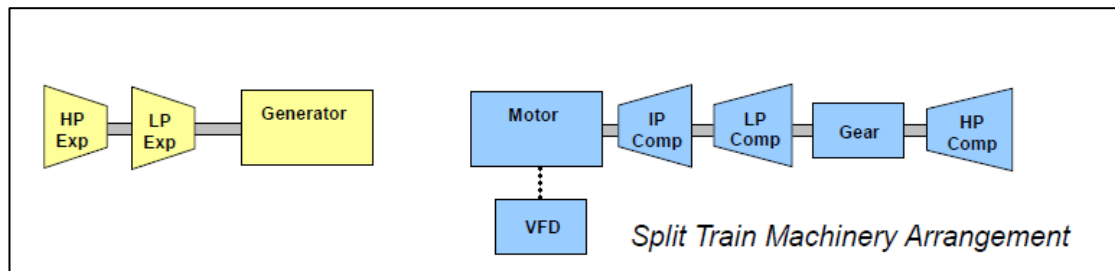
Figure 24 - McIntosh Split Train Equipment Configuration (HEID, 2010)
