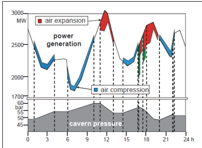
Figure 15 - Compression and expansion cycles for a CAES plant during a typical day (Crotagino, 2001)
