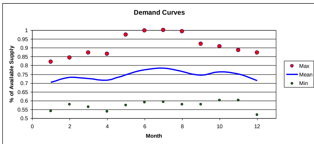
Figure 43 - Annual Demand Curve
