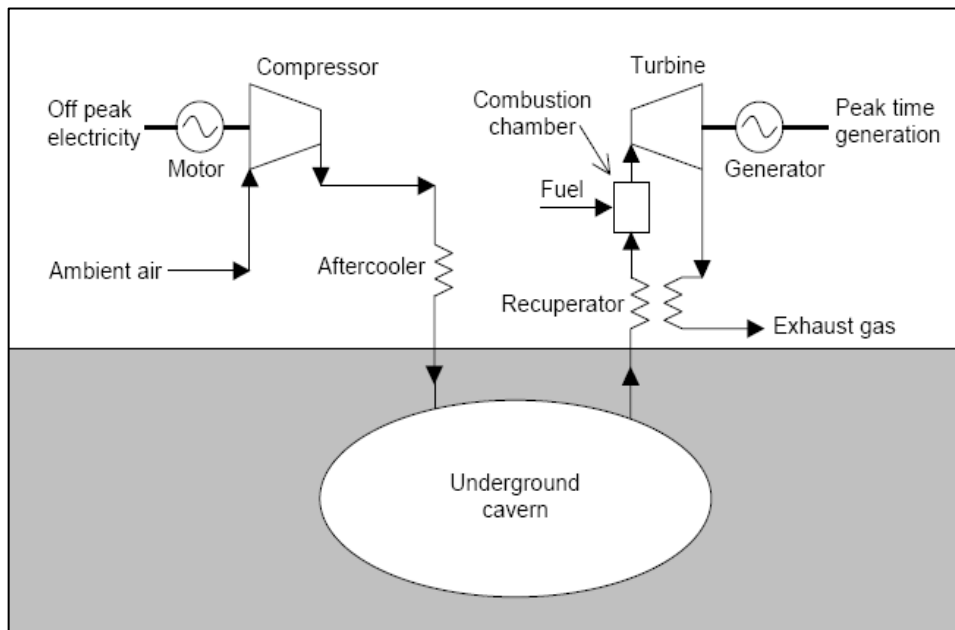
Figure 11 - Process Flow of a Compressed Air Energy Storage System (Valenti, 2010)
