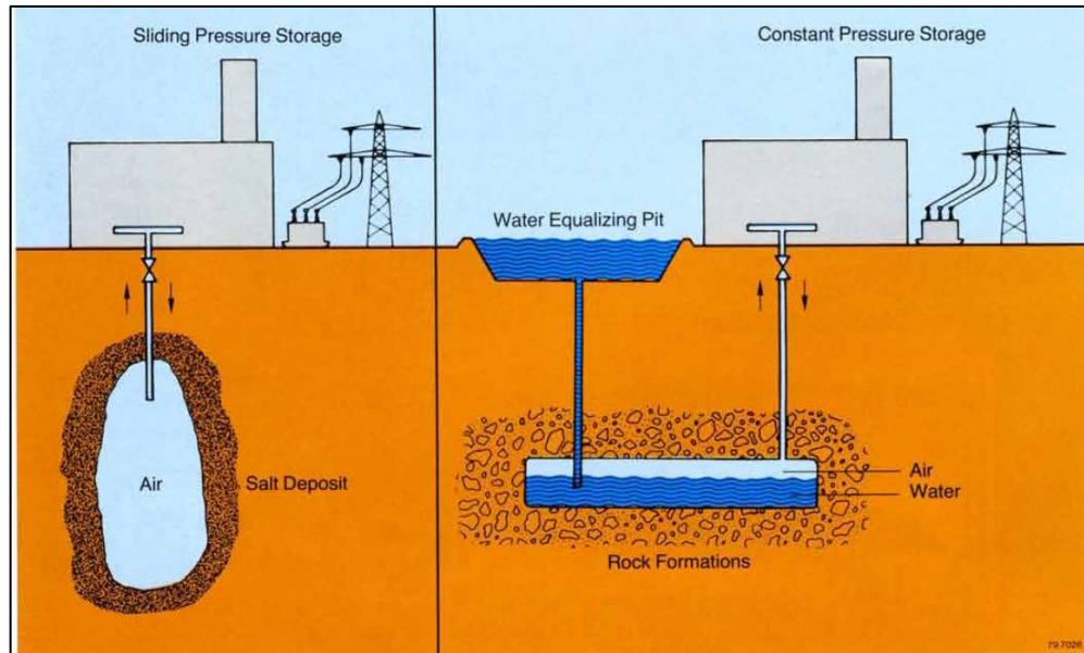
Figure 16 - Constant Pressure vs. Constant Volume Air Storage (BBC, 1990)
