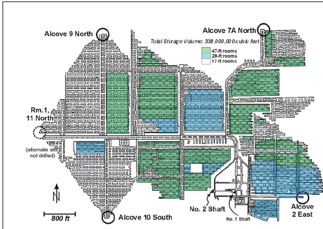
Figure 28 - Footprint of Norton Mine, showing location and distribution of room sizes
