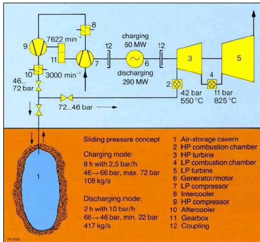
Figure 20 - Process Flow diagram of Huntorf CAES Plant (BBC, 1990)
