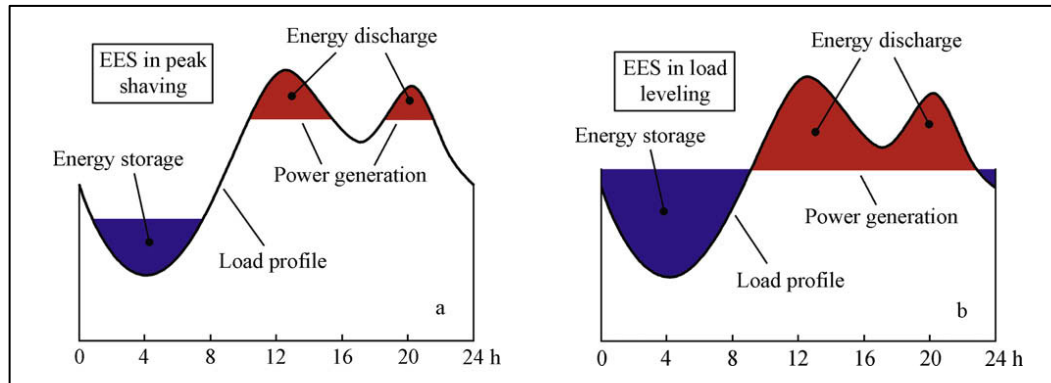
Figure 4 - Load profile of a large-scale electricity storage system. (a) EES in peak shaving (b) EES in Load Levelling (Chen et al, 2009)
