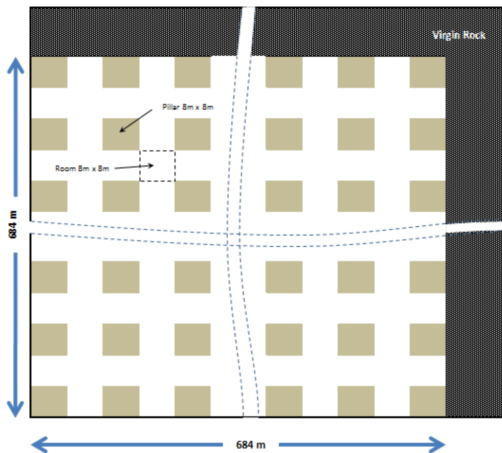
Figure 57 - Sealing Requirements for Room and Pillar Hard Rock Mine
