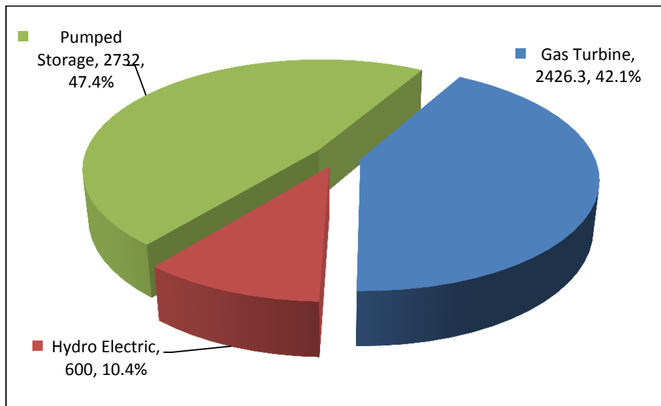
Figure 38 - Future Composition of Eskom Peaking Plant Types
