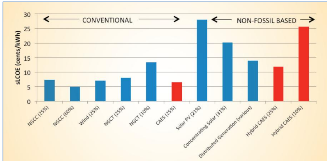
Figure 56 – Levelised Cost of Energy for Various Technologies (McGrail B et al, 2013).
