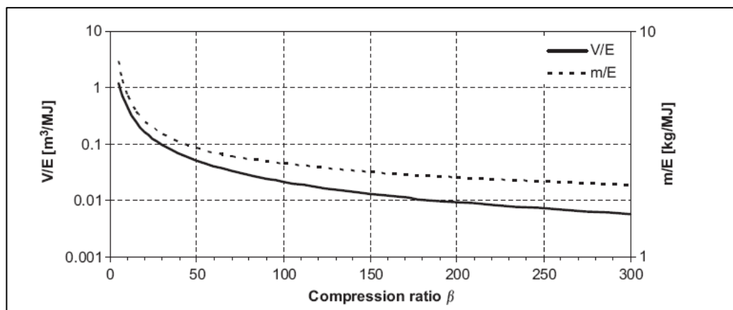
Figure 2 - Specific Air Volume and Mass for constant temperature energy storage (Grazzini and Milazzo, 2007)
