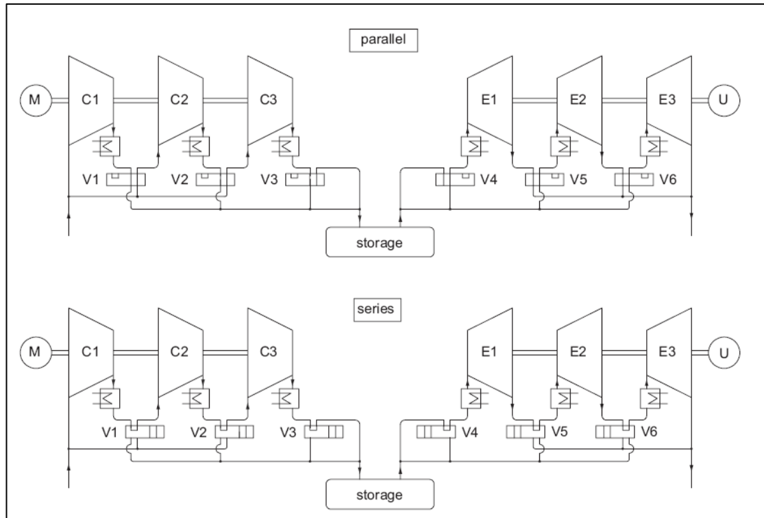
Figure 3 - CAES system with thermal storage (Grazzini and Milazzo, 2007)
