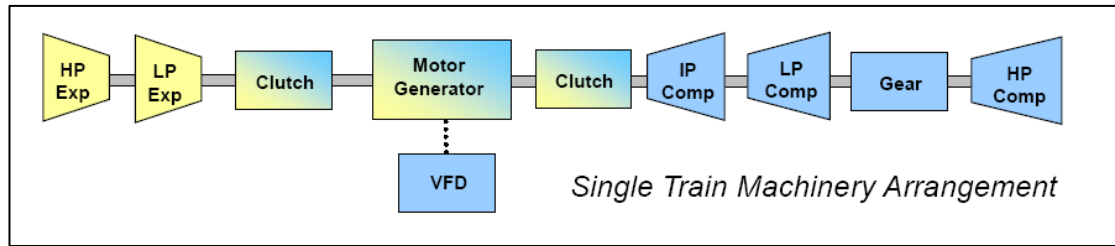
Figure 21 - Huntorf Single Train Equipment Configuration (HEID, 2010)
