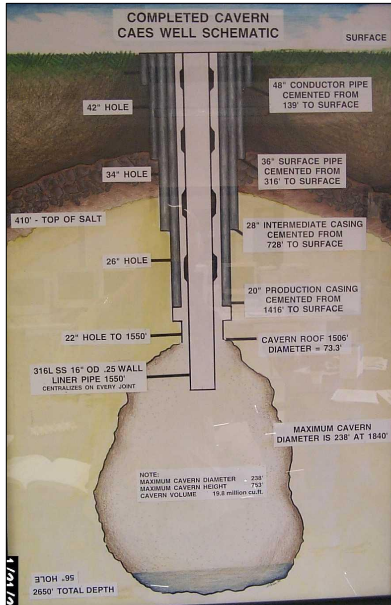
Figure 26 - Schematic of McIntosh Cavern (Email from Alabama Electric Cooperative)
