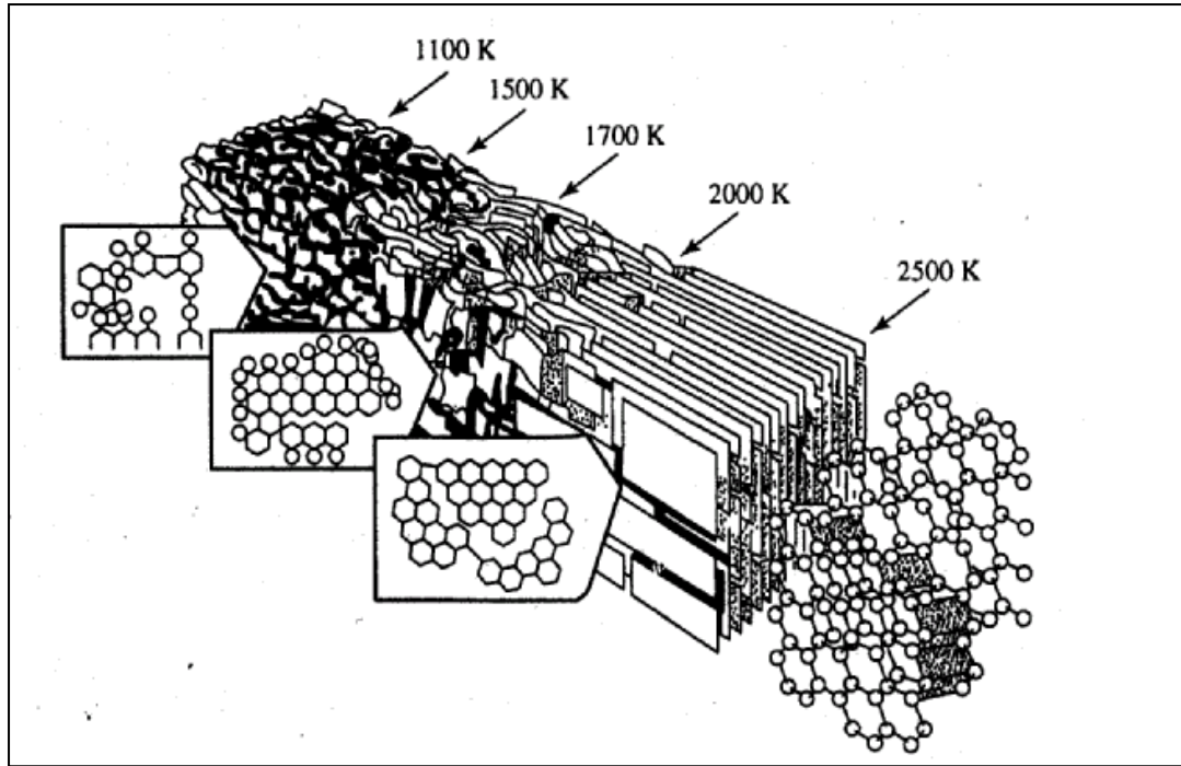
Figure 2-16 Diagram showing molecular re-organisation in anisotropic carbon heat treated from approx 900 - 2220°C (Marsh, 1997)
