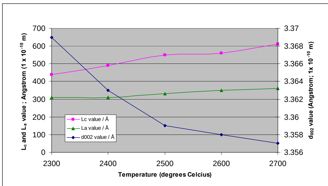
Figure 2-21 Crystalline development as a function of heat treatment temperature for a highly ordered carbon (Burchell, 1999)
