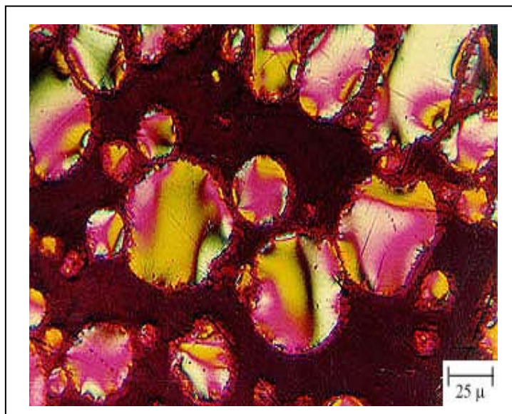
Figure 2-8 Polarised light micrograph showing coalescence of mesophase spherules (Magnification x 25 in oil) (Crelling, 1990)
