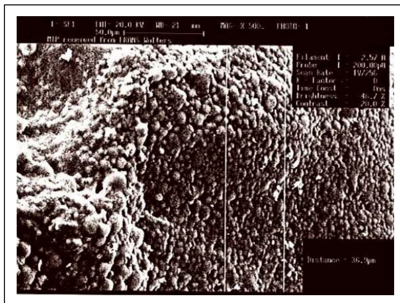
Figure 2-11 Scanning Electron Micrograph (SEM, Magnification x 3000) of an Isotropic coke showing fine mosaic “ball” structures (Clark, 1996)
