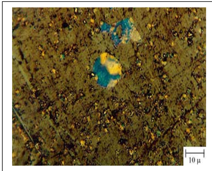
Figure 2-7 Polarised light micrograph showing development of embryonic mesophase spherules (Magnification x 50 in oil) (Crelling, 1990)
