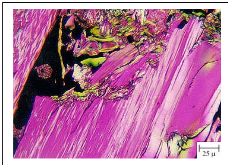
Figure 2-12 Polarised light micrograph of needle coke in a binder matrix showing elongated flow patterns (Magnification x 25 in oil) (Crelling, 1990)
