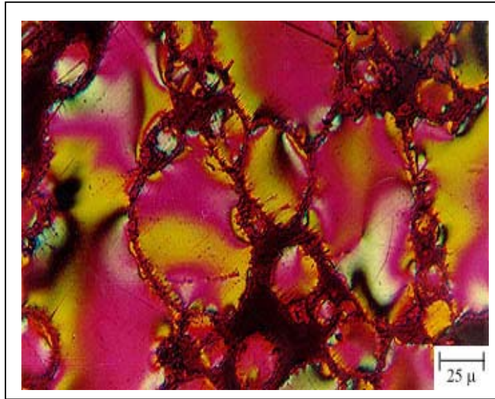
Figure 2-9 Polarised light micrograph of fully coalesced mesophase showing ash concentration at the grain boundaries (Magnification x25 in oil) (Crelling , 1990)
