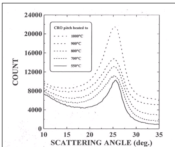
Figure 2-22 X-ray powder diffraction pattern showing the development of the d 002 peak for an anisotropic pitch treated between 550 and 1000°C (Burchell, 1999)
