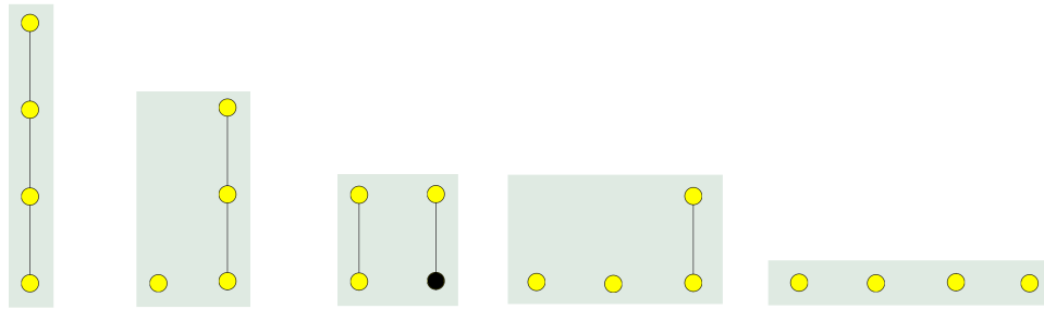
Figure 5: 19 lit nodes in the 5 partitions of 4.
