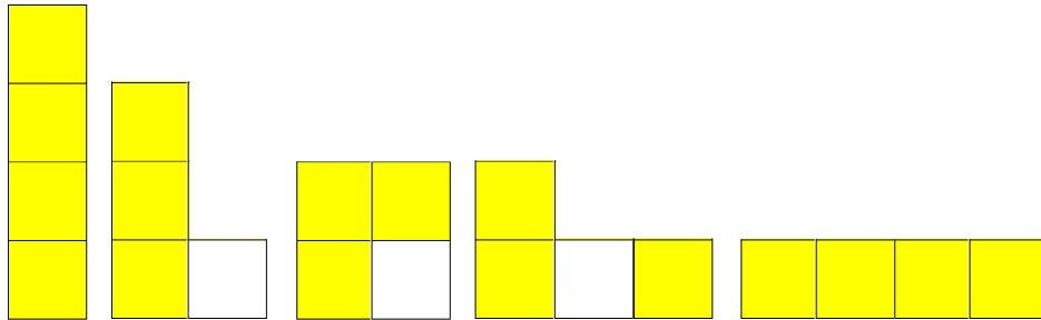
Figure 9: 17 lit cells in weakly decreasing partitions of 4.
