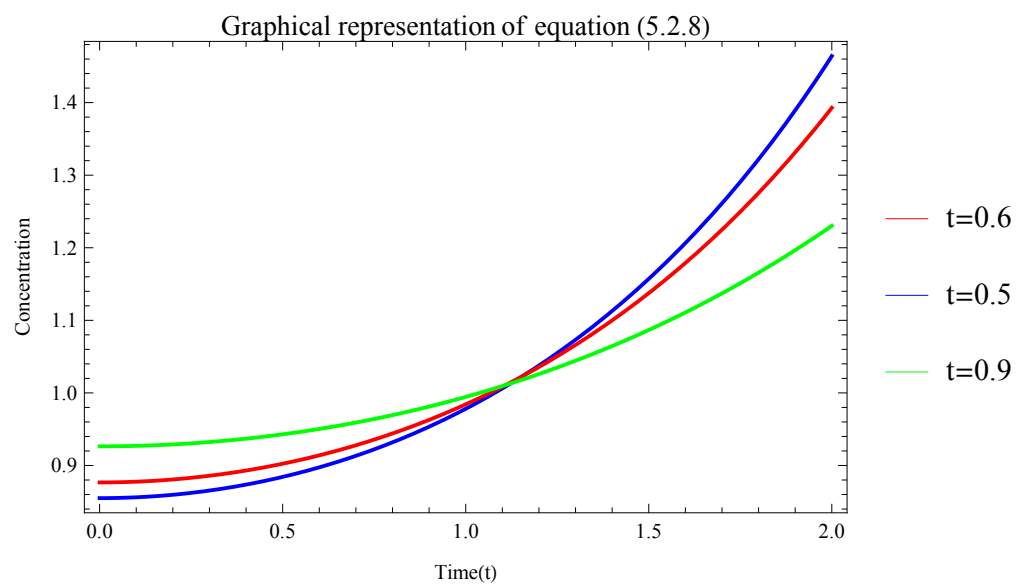
Figure 5.2: Concentration of oil over time.
