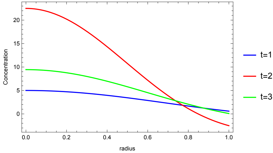
Figure 8.3: Concentration of oil along the sea from equation (8.3.19).
