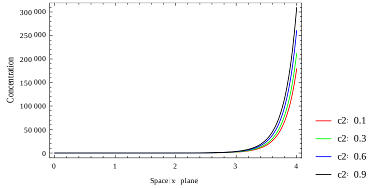
Figure 7.5: Graphical representation of equation (7.3.6), a_1=a_2=c_1=1 .
