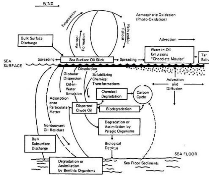
Figure 1.1: Weathering processes after oil spill. Image from https://ars.elsa-cdn.com/content/image/1-s2 .
