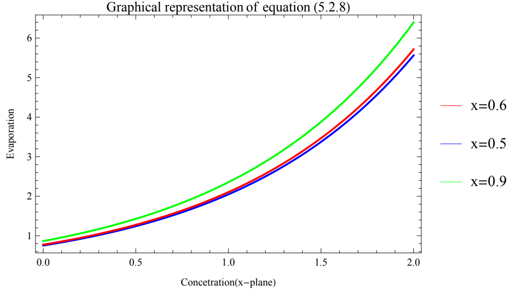
Figure 5.4: The effects of evaporation on the concentration of oil.
