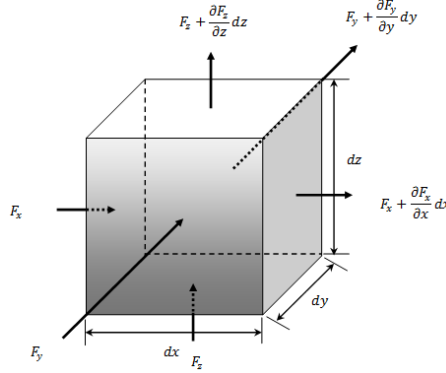
Figure 2.1: Convection-diffusion in a three-dimensional space. Image from www.nap.ed
