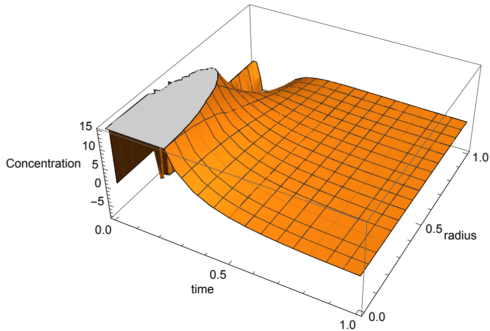
Figure 8.1: Concentration of oil over the surface from equation (8.3.19).
