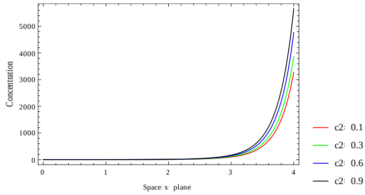
Figure 7.4: Graphical representation of equation (7.3.5), c_1=1 .
