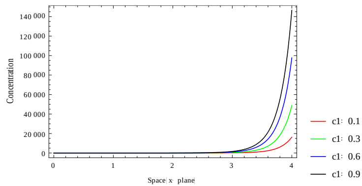
Figure 7.6: Graphical representation of equation (7.3.6), a_1=a_2=1, c_2=0 .
