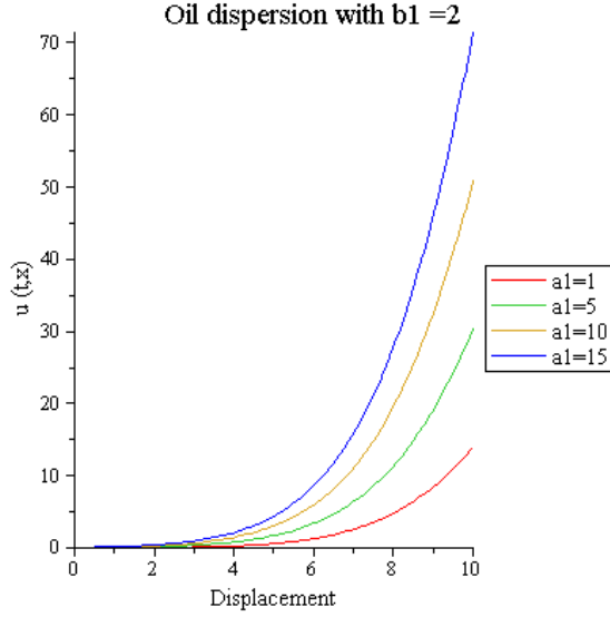
Figure 7.1: Oil dispersion for equation (7.2.21) after t = 10
