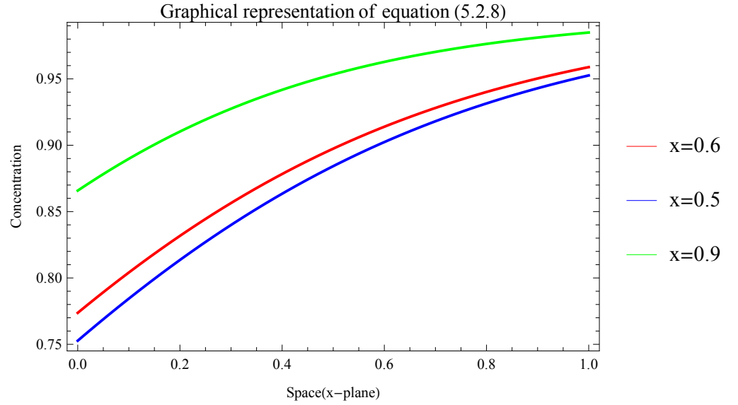
Figure 5.1: Concentration of oil over the x -plane.
