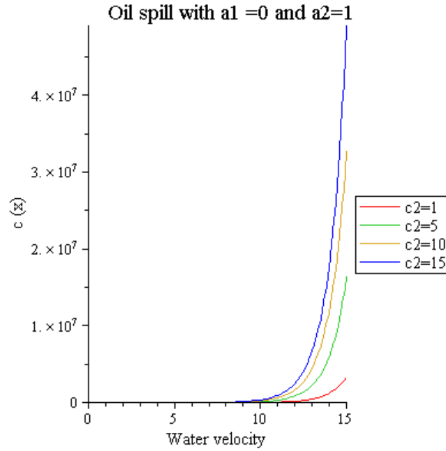
Figure 7.2: Steady state oil dispersion for equation (7.3.2).
