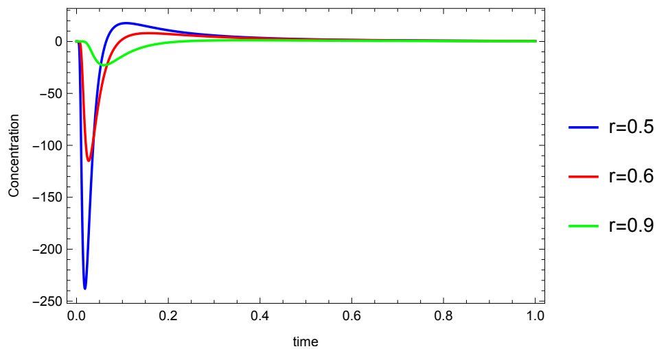
Figure 8.2: Concentration of oil over time from equation (8.3.19).
