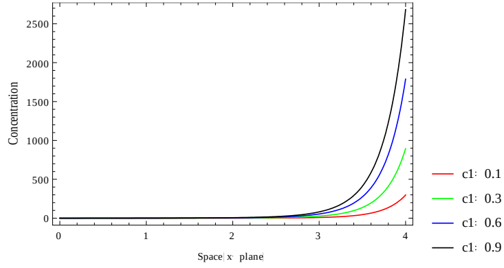
Figure 7.3: Graphical representation of equation (7.3.5), c_2=0 .
