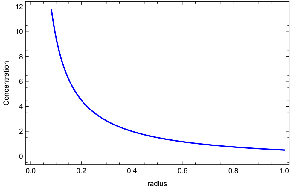
Figure 8.3: Concentration of oil along the sea from equation (8.3.19).
