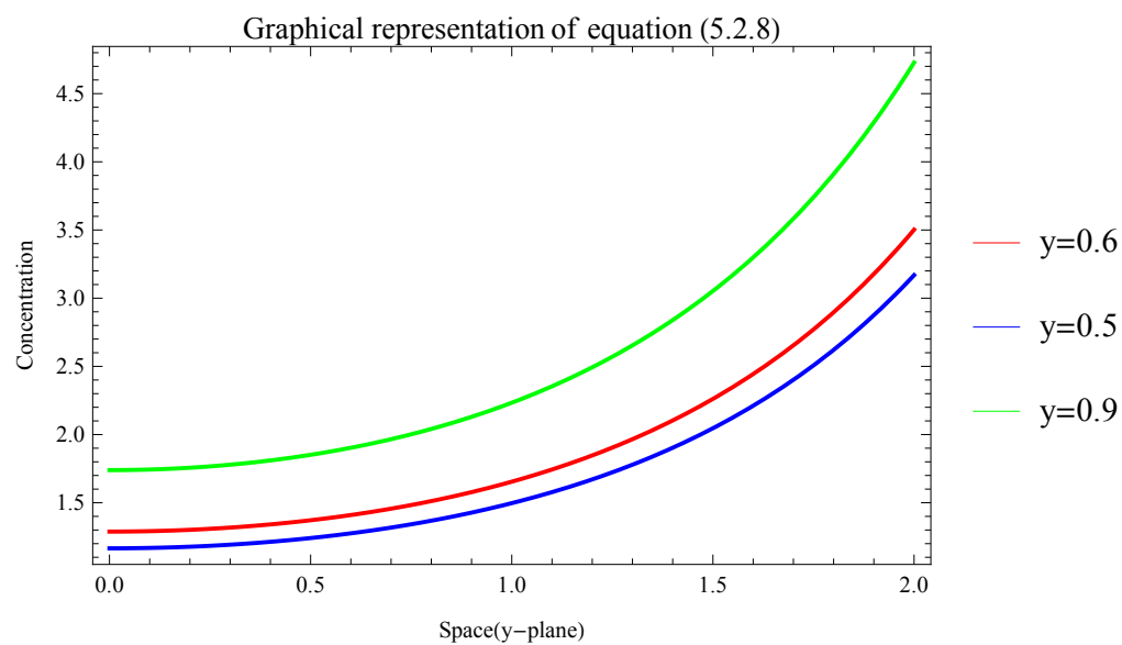
Figure 5.3: Concentration of oil over the y -space.
