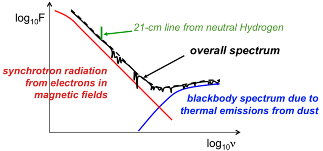
FIGURE 1.7: A log-log scale plot of a composite spectrum for a typical galaxy observed over a wide range of frequencies, from radio to visible [71].
