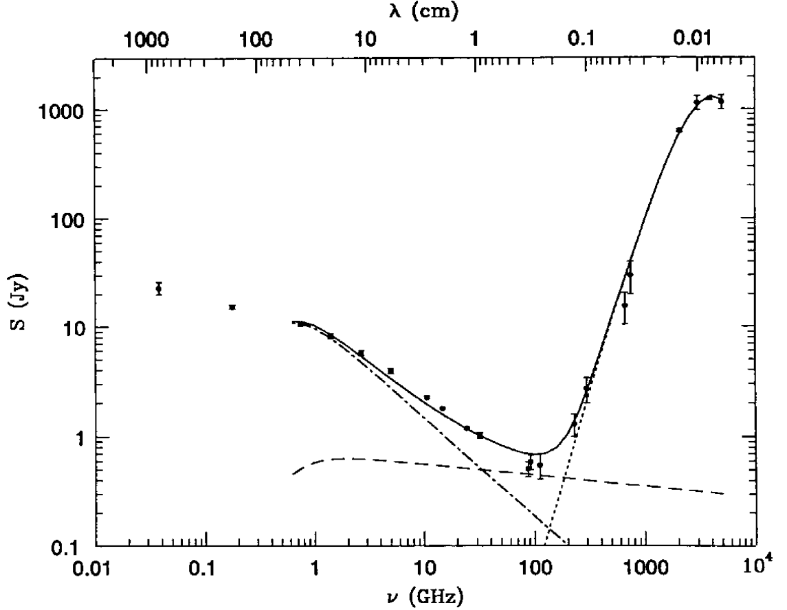
FIGURE 1.8: The radio and far-infrared spectrum of the nearby starburst galaxy M82 [18]. The contribution of free-free emission is indicated by the nearly horizontal dashed line. Synchrotron radiation (dot-dash line) and thermal dust emission (dots) dominate at low and high frequencies, respectively. Free-free absorption from H II regions distributed throughout the galaxy absorbs some of the synchrotron radiation and flattens the overall spectrum at the lowest frequencies [59].
