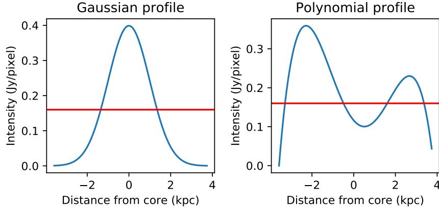
FIGURE 3.1: Source profile plots showing two possible source profiles. We display the red line to highlight the possible downside of using thresholds on sources with non-Gaussian profiles. The pixel masking and conversion procedure provides estimates to excluded sources since it simply cuts off pixel intensities and does not perform flux integration over the area above the threshold. This requires some human intervention to double check the excluded sources making it a less rigorous approach than using the dynamic flux per beam area procedure.
