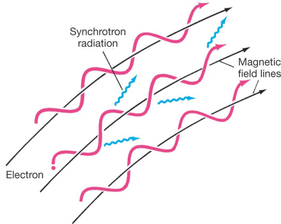
FIGURE 1.6: A simple illustration of a relativistic electron being accelerated by a magnetic field and the synchrotron radiation that is emitted as the charged particle gets boosted by the magnetic field [11]. This is the source of the diffuse emission we wish to study from the extended radio sources we looked at in this study.
