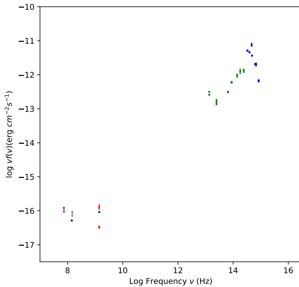
FIGURE 3.11: The SED of the core of the radio galaxy PGC2285791 with previously known optical (blue), infrared (green) and radio (red) data points plotted with the addition of the VLSSr (magenta), LoTSS (black), TGSS (grey) and NVSS (navy) data points, integrated over the VLSSr beam size.
