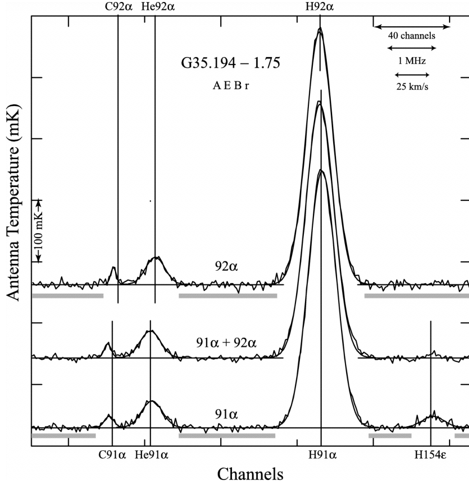
FIGURE 1.4: An example of observed recombination-line spectra from the 91\alpha and 92\alpha transitions of hydrogen, helium, and carbon observed in an \text{H II} region [60].
