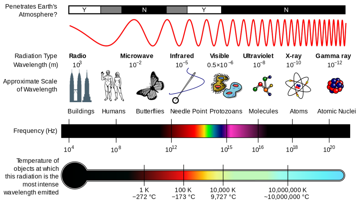
FIGURE 1.1: An illustration of the large variance in frequency and wavelengths found in the electromagnetic spectrum, along with intuitive scales of the different wavelengths, the temperature in these bands and the possibility of observing these signal from Earth's surface [33].
