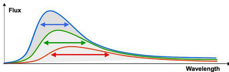
FIGURE 1.5: A plot of the flux against wavelength of a blackbody emitter, showing that such an object will emit a spectrum of radiation which peaks at a wavelength (or frequency) dependent only on the objects temperature. As the source temperature increases the peak wavelength decreases. This is why hot stars appear blue and cool stars appear red [71].
