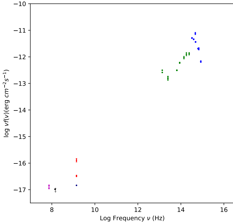
FIGURE 4.6: The SED of the core of the radio galaxy PGC2285791 with previously known optical (blue), infrared (green) and radio (red) data points plotted with the addition of the VLSSr (magenta), LoTSS (black), TGSS (grey overlaps with black) and NVSS (navy) data points.
