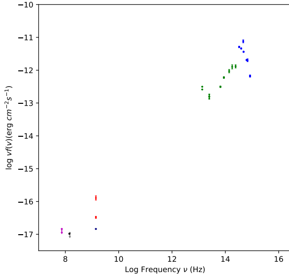
FIGURE 3.9: The SED of the core of the radio galaxy PGC2285791 with previously known optical (blue), infrared (green) and radio (red) data points plotted with the addition of the VLSSr (magenta), LoTSS (black), TGSS (grey overlaps with black) and NVSS (navy) data points, integrated over the LoTSS beam size.
