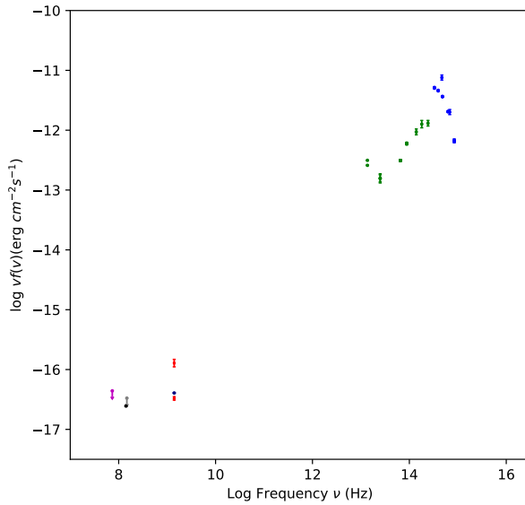
FIGURE 3.10: The SED of the core of the radio galaxy PGC2285791 with previously known optical (blue), infrared (green) and radio (red) data points plotted with the addition of the VLSSr (magenta), LoTSS (black), TGSS (grey) and NVSS (navy) data points, integrated over the TGSS beam size.
