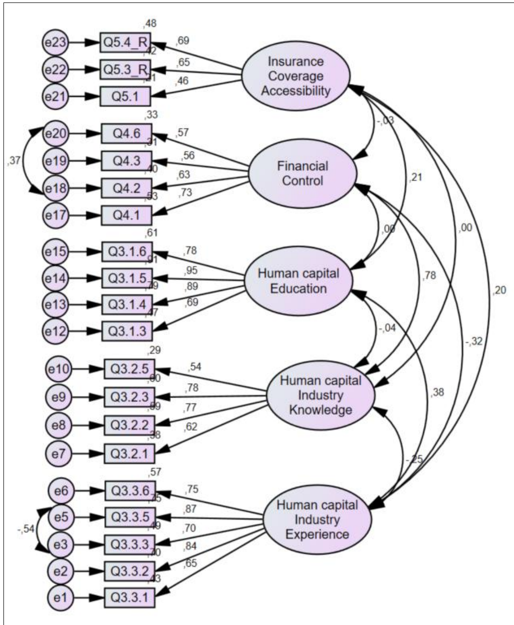
Figure 14: CFA Pruned Model
