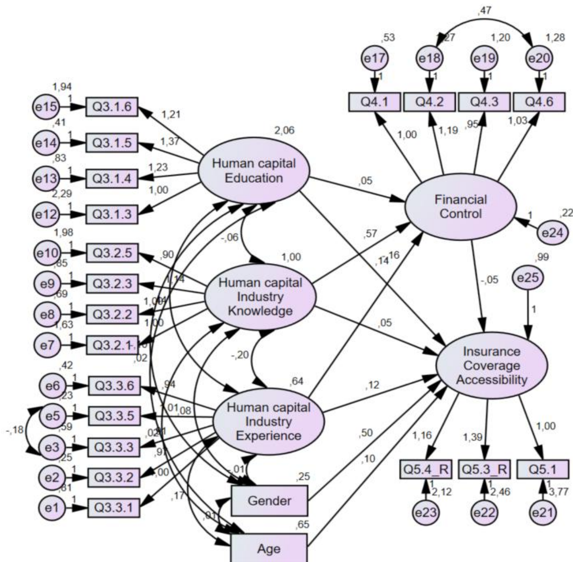
Figure 16: Figure 13: SEM Model using demographics as control variables
