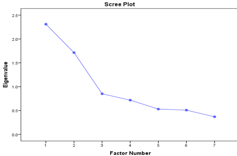
Figure 12: Scree plot - Dependent variable
