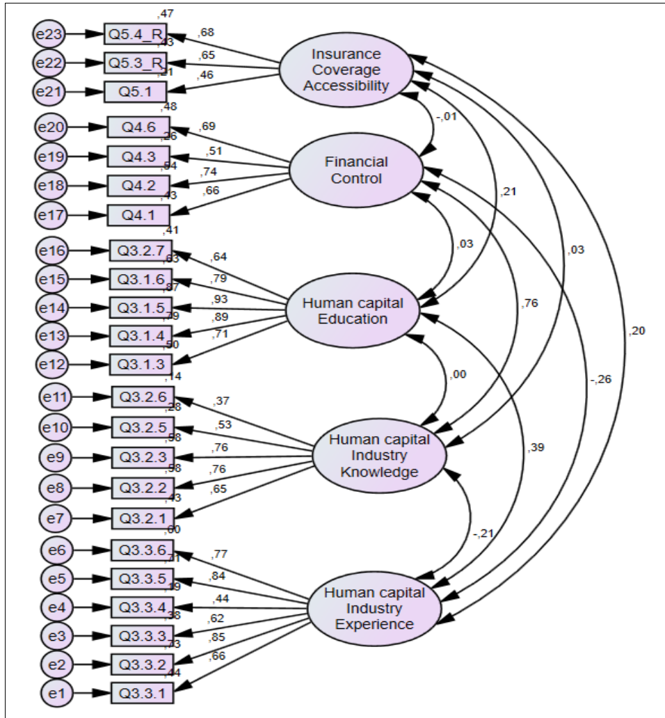
Figure 13: CFA Hypothesised Model
