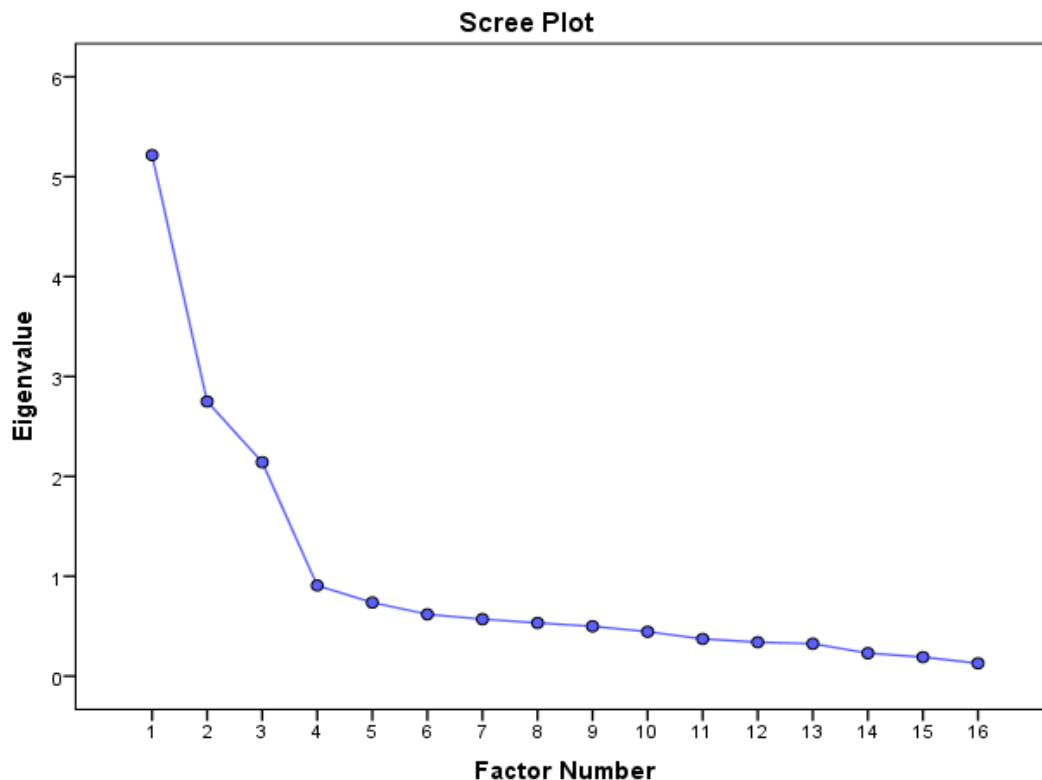
Figure 11: Scree plot – Independent variables
