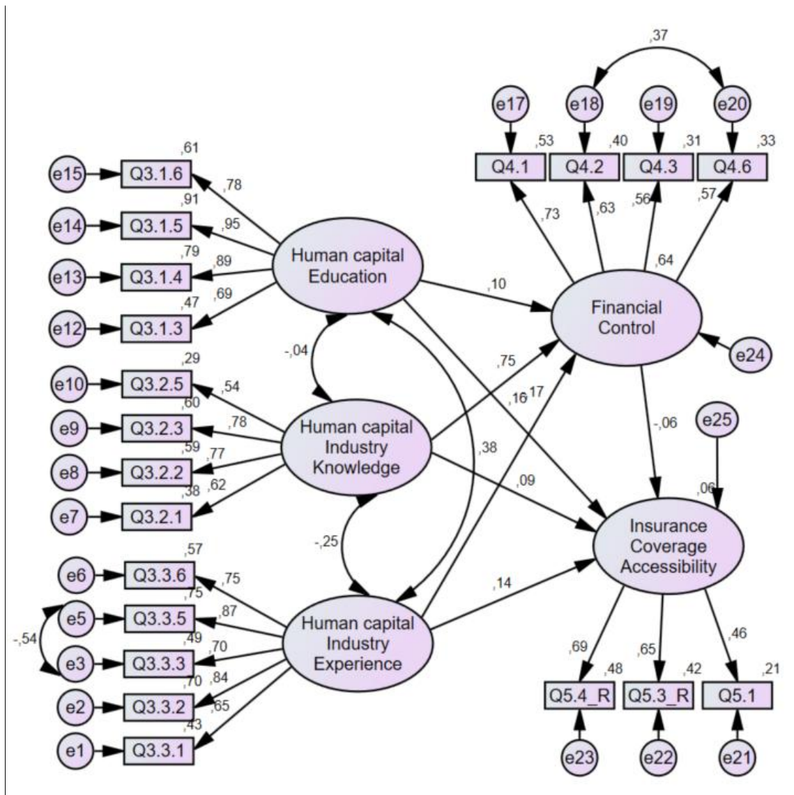
Figure 15: SEM Model
