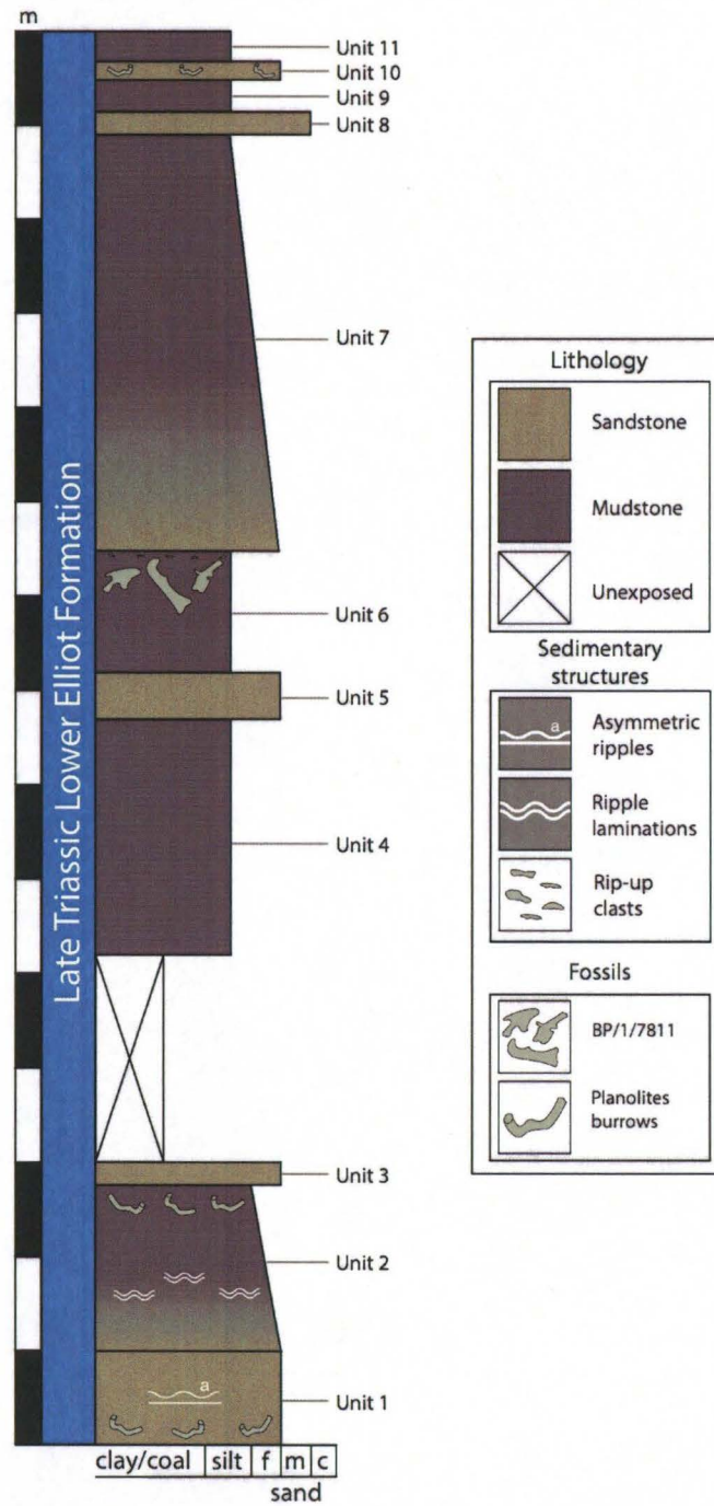
Figure 3: Stratigraphic column (15 m) depicting the lithostratigraphy of the H5 Quarry, Dreifontein Farm, Eastern Cape, South Africa.
