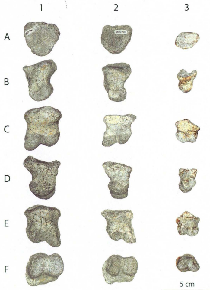
Figure 29: BP/1/7811 non-terminal ?manual phalanges. Proximal (A) lateral (B) anterior (C) medial (D) posterior (E) distal (F). Scale bar = 5cm.
