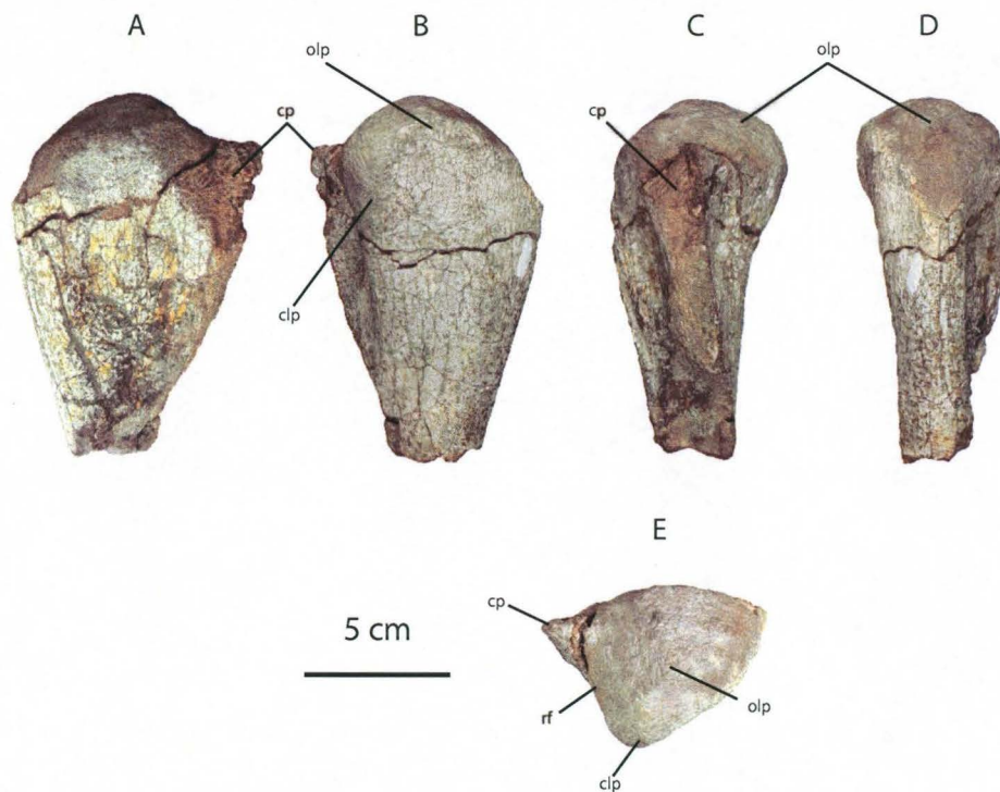
Figure 26: BP/1/7811, left proximal ulna. Medial (A) lateral (B) anterior (C) posterior (D) proximal (E). Abbreviations: clp, craniolateral process; cp, coronoid process; olp, olecranon process; rf, radial fossa. Scale bar = 5 cm
