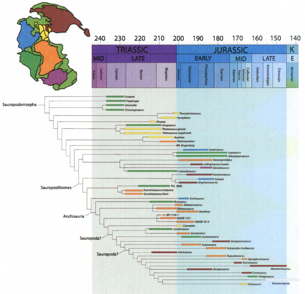
Figure 37: Time-calibrated strict consensus including the position of BP/1/7811. Colors from Triassic world map show modern continents and correlate with each bar adjacent to taxa.
