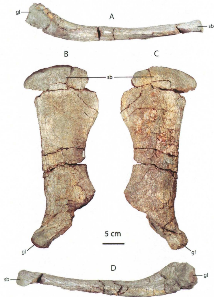
Figure 23: BP/1/7811, left scapula. Anterior (A) medial (B) lateral (C) posterior (D). Abbreviations: gl, glenoid; sb, scapular blade. Scale bar = 5 cm
