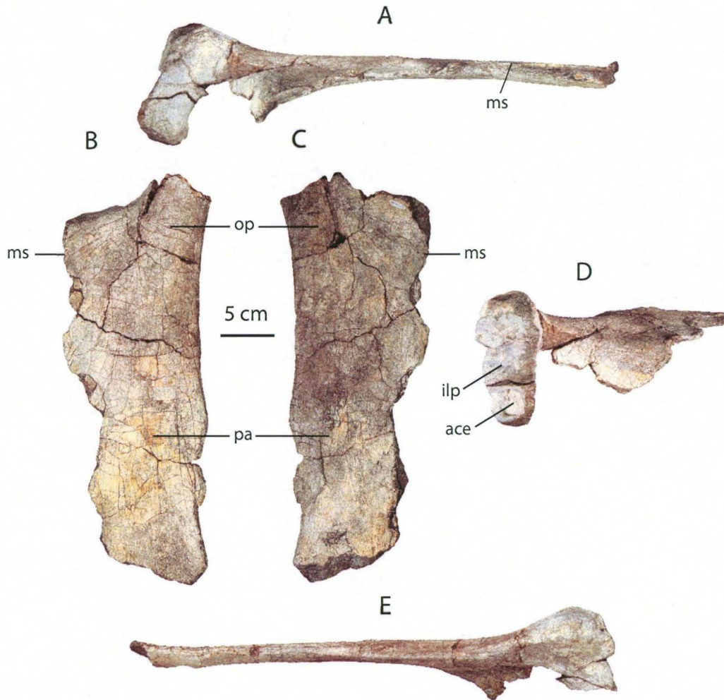
Figure 32: BP/1/7811, left pubis. Posterior (A) medial (B) lateral (C) proximal (D) anterior (E). Abbreviations: ace, acetabulum; ilp, iliac peduncle; ms, medial symphysis; op, obturator plate; pa, pubic apron. Scale bar = 5 cm
