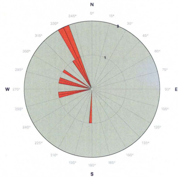
Figure 8: Rose diagram depicting BP/1/7811 long bone distribution within the H5 Quarry. Image generated by GeoRose 0.5.0 software.
