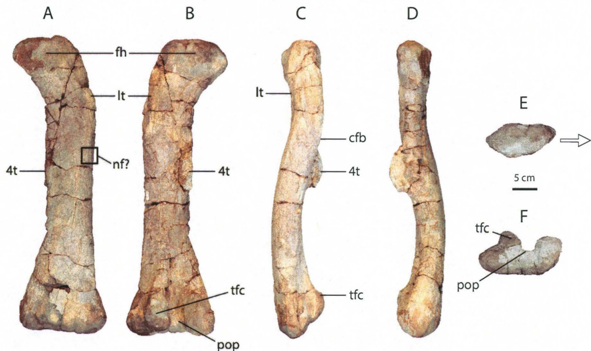
Figure 33: BP/1/7811, left femur. Anterior (A) posterior (B) lateral (C) medial (D) proximal (E) distal (F). Abbreviations: 4t, fourth trochanter; cfb, M. caudofemoralis; fh, femoral head; lt, lesser trochanter; nf, nutrient foramina; pop, popliteal fossa; tfc, tibiofibular crest. Arrow points medially. Scale bar = 5 cm
