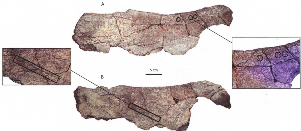
Figure 11: A) Left pubis showing tooth punctures B) Right pubis with drag marks. Circles show tooth punctures, rectangle shows tooth score. Scale bar = 5 cm.
