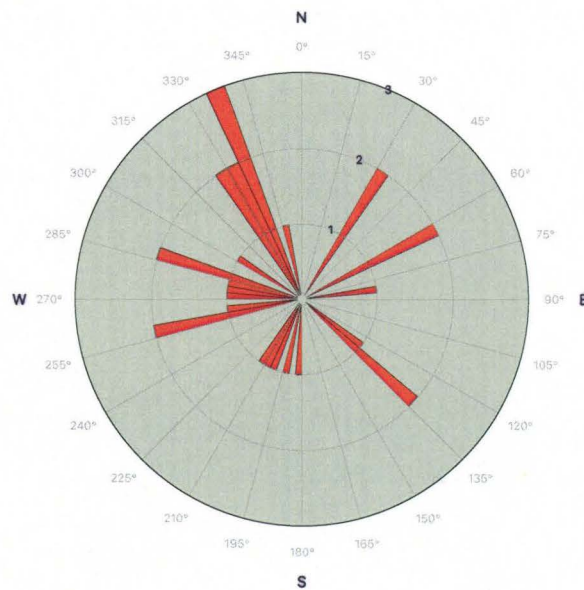
Figure 9: Rose diagram depicting BP/1/7811 all bone excluding rib distribution within the H5 Quarry. Image generated by GeoRose 0.5.0 software.
