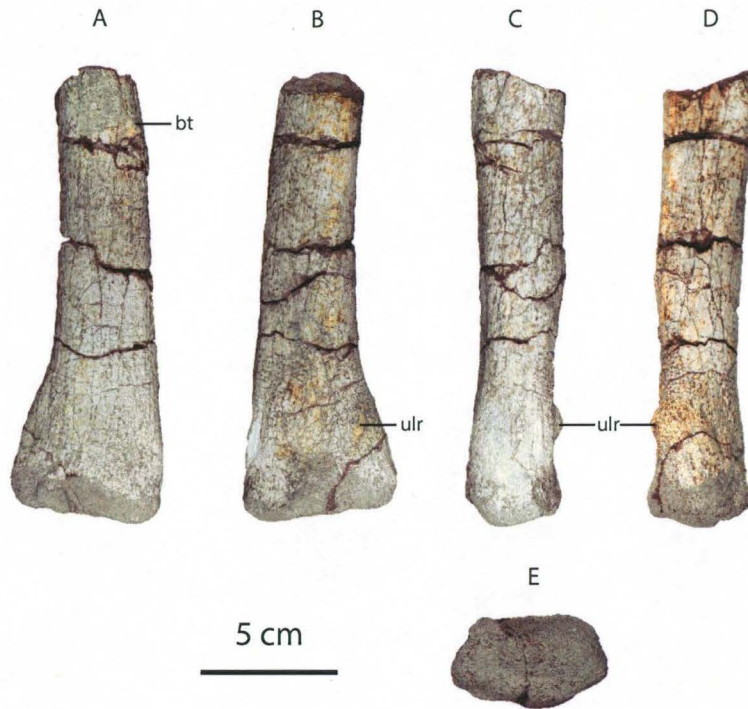
Figure 25: BP/1/7811, distal right radius. Lateral (A) medial (B) anterior (C) posterior (D) distal (E). Abbreviations: bt, biceps tubercle; ul, ulnar ligament of the radius. Scale bar = 5 cm
