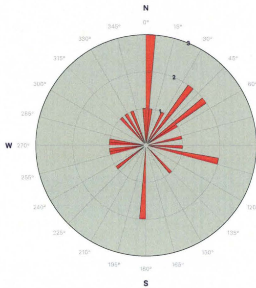
Figure 7: Rose diagram depicting BP/1/7811 rib distribution within the H5 Quarry. Image generated by GeoRose 0.5.0 software.
