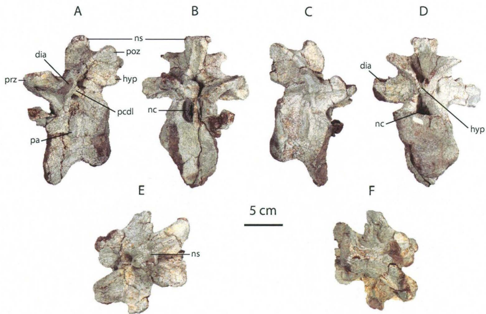
Figure 15: BP/1/7811, D2?. Left lateral (A) anterior (B) posterior (C) right lateral (D) dorsal (E) ventral (F). Abbreviations: di, diapophyses; hyp, hyposphene; nc, neural canal; ns, neural spine; pa, parapophyses; pcdl, posterior centrodiapophyseal lamina; poz, postzygapophyses; prz, prezygapophyses. Scale bar = 5 cm
