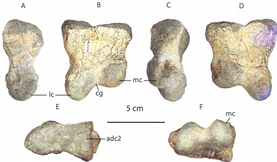
Figure 27: BP/1/7811, left MC1. Lateral (A) anterior (B) medial (C) posterior (D) proximal (E) distal (F). Abbreviations: adc2, articular surface for distal carpal; cg, central ginglymus; lc, lateral condyle; mc, medial condyle. Scale bar = 5 cm
