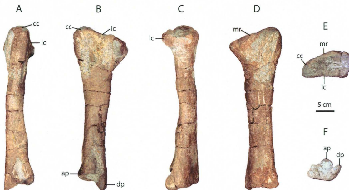
Figure 34: BP/1/7811, left tibia. Anterior (A) lateral (B) posterior (C) medial (D) proximal (E) distal (F). Abbreviations: ap, ascending process; cc, cnemial crest; dp, descending process; lc, lateral condyle; mr, medial ridge. Scale bar = 5 cm
