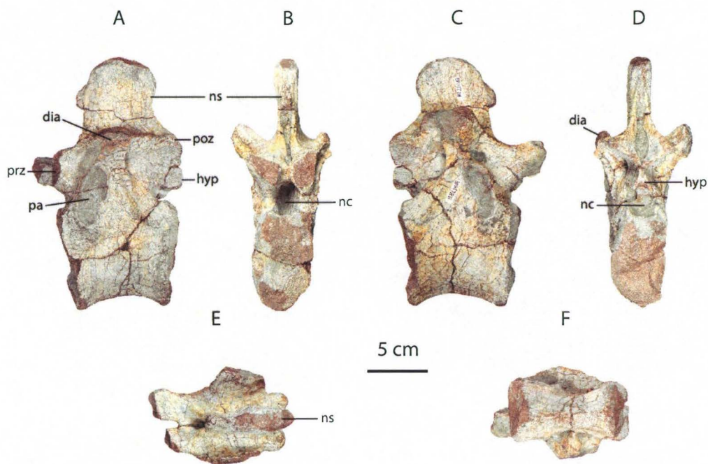
Figure 17: BP/1/7811, D5?. Left lateral (A) anterior (B) posterior (C) right lateral (D) dorsal (E) ventral (F). Abbreviations: di, diapophyses; hyp, hyposphene; nc, neural canal; ns, neural spine; pa, parapophyses; poz, postzygapophyses; prz, prezygapophyses. Scale bar = 5 cm
