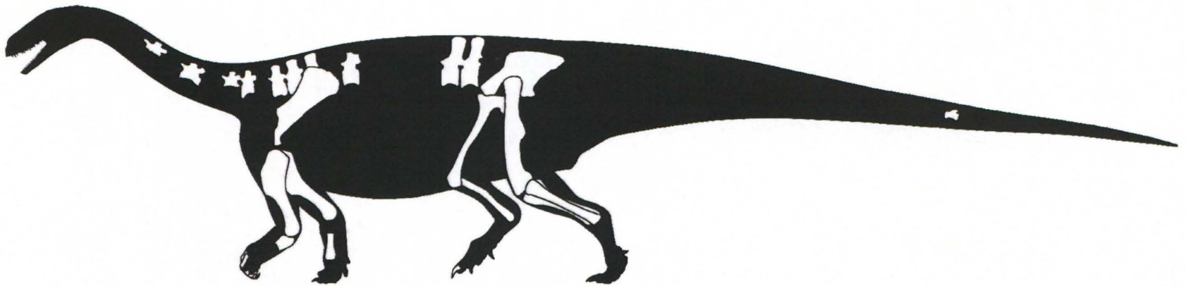
Figure 4: Silhouette showing the preserved skeletal remains of BP/1/7811 modified from Scott Hartman.
