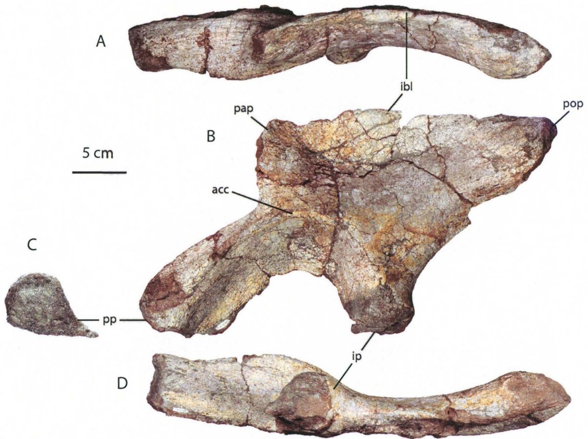
Figure 31: BP/1/7811, left ilium. Anterior (A) lateral (B) posterior pubic peduncle (C) posterior (D). Abbreviations: acc, acetabular crest; ip, ischial peduncle; ibl, iliac blade; pap, preacetabular process; pop, postacetabular process; pp, pubic peduncle. Scale bar = 5 cm
