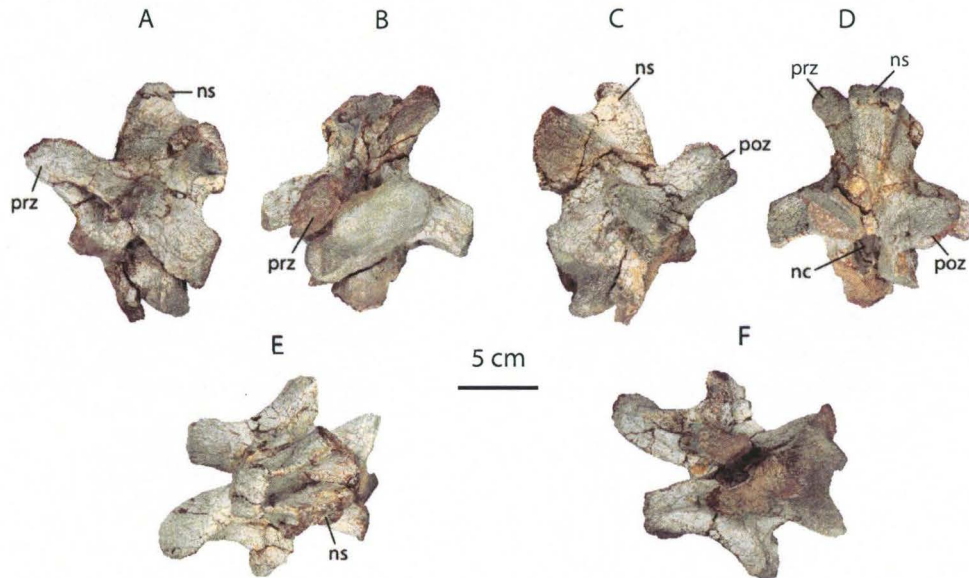
Figure 14: BP/1/7811, D1?. Left lateral (A) anterior (B) posterior (C) right lateral (D) dorsal (E) ventral (F). Abbreviations: epi, nc, neural canal; ns, neural spine; poz, postzygapophyses; prz, prezygapophyses. Scale bar = 5 cm
