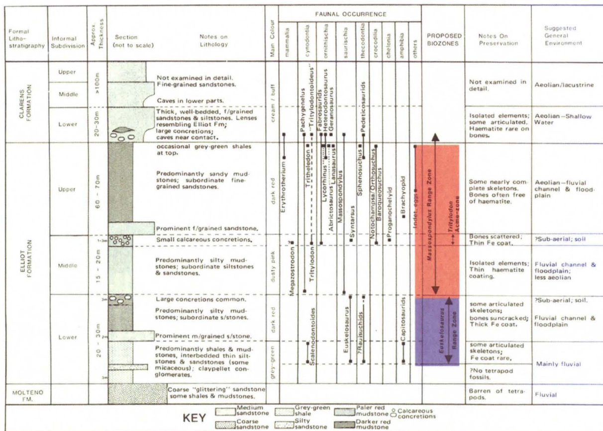
Figure 2: Kitching & Raath's (1984) Massospondylus (red) and "Euskelosaurus" (purple) Range Zones.
