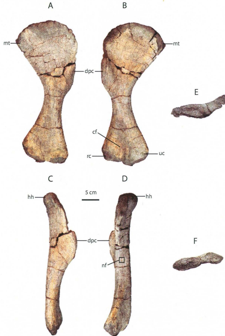
Figure 24: BP/1/7811, right humerus. Anterior (A) posterior (B) medial (C) lateral (D) proximal (E) distal (F). Abbreviations: cf, cuboid fossa; dpc, deltopectoral crest; hh, humeral head; mt, medial tuberosity, nf, nutrient foramina; rc, radial condyle; uc, ulnar condyle. Scale bar = 5 cm
