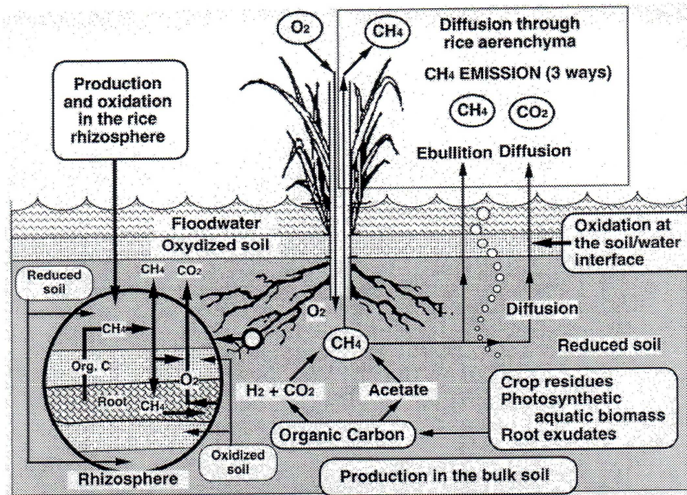
Figure 3.3 Methane production and oxidation in rice puddies (Danier et al. , 1996)
