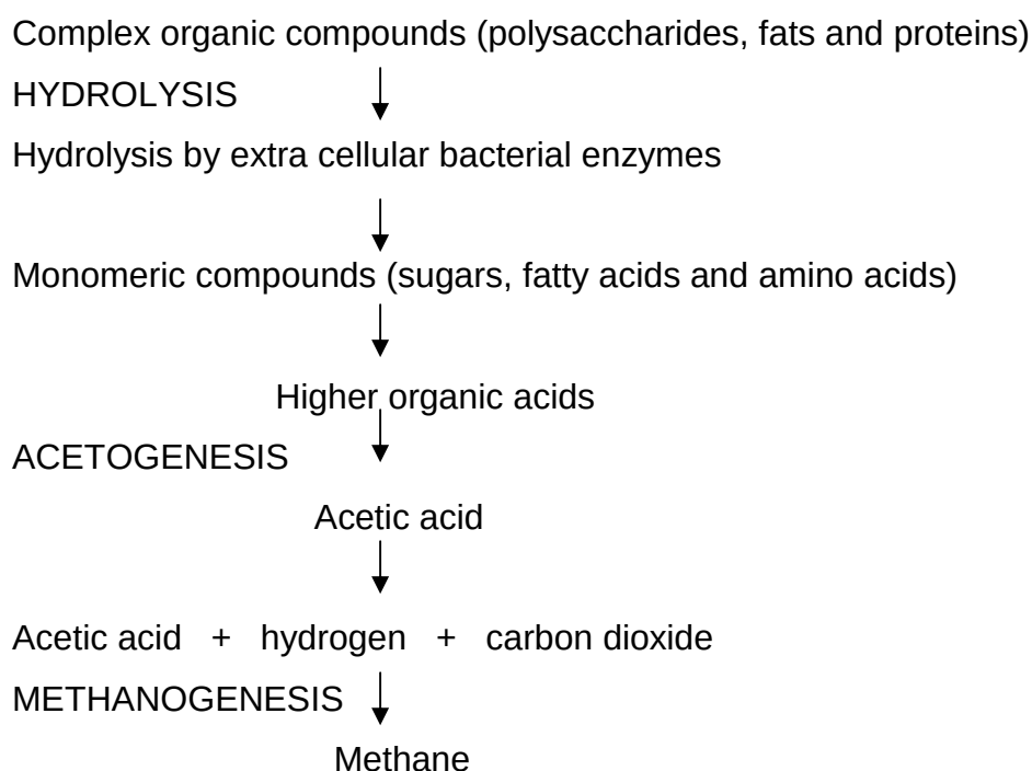
Figure 1.2 Degradation of organic matter to methane production
