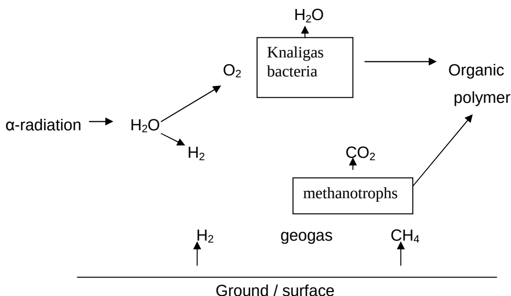
Figure 3.4 Methanotrophs in work fields and natural gas effluents (Daniel et.al., 1996)
