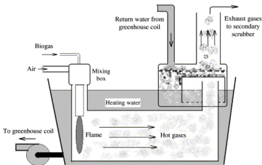
Figure 1.4: Harvesting biogas from landfill to be used in greenhouse (Jaffrin et al. , 2003)
