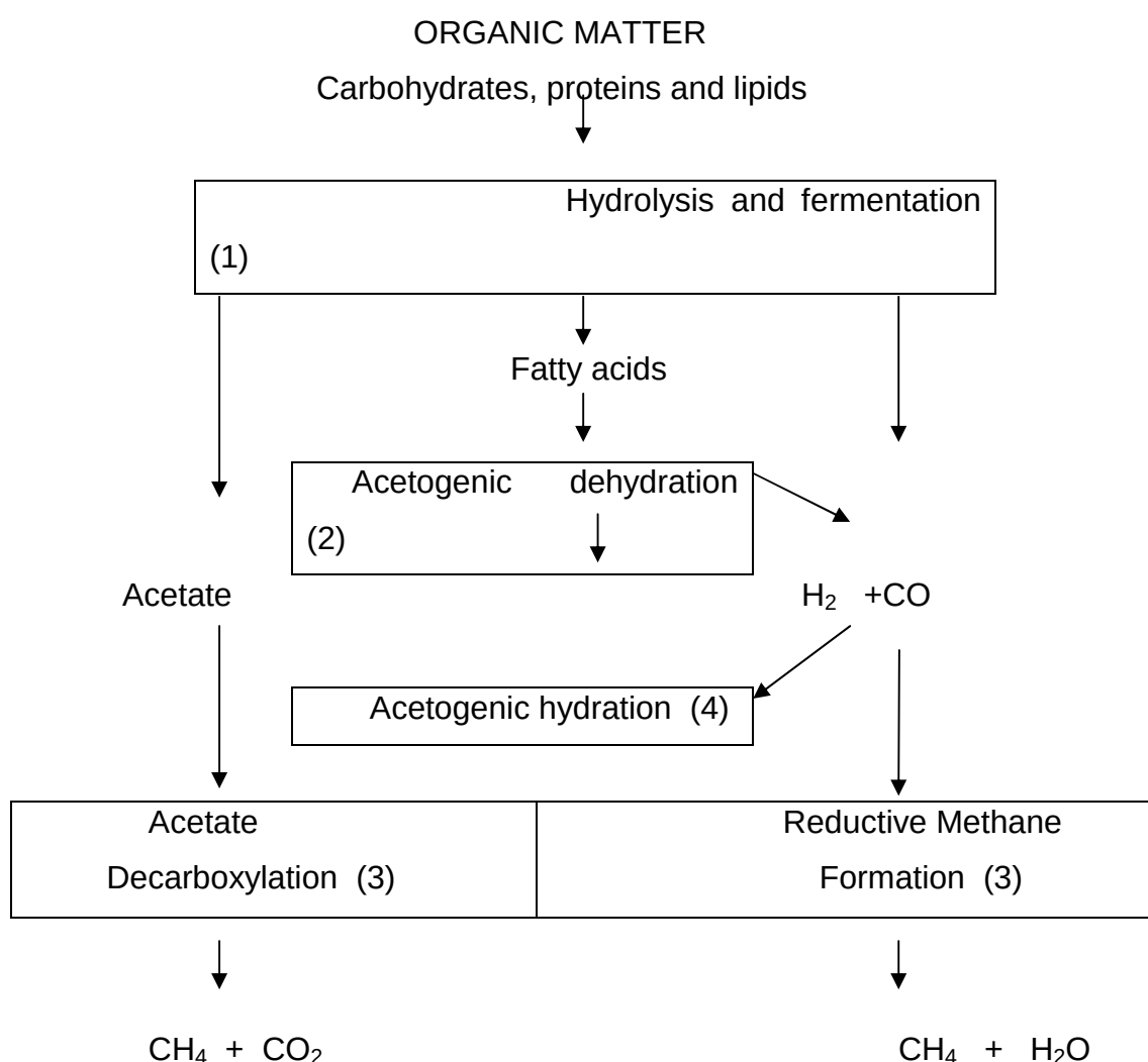
Figure 2.1: Some the pathways used by microbes in methane generation
