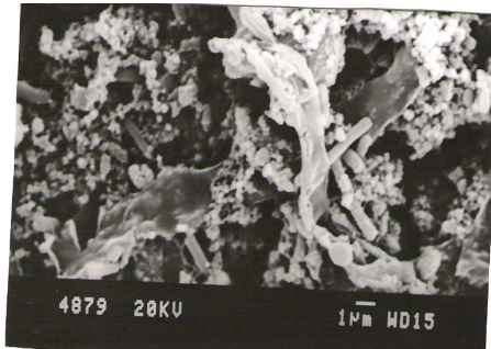
Figure 3.8 Mucus (ESP) produced by soil bacteria
