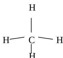
Figure 1.3 Methane structure
