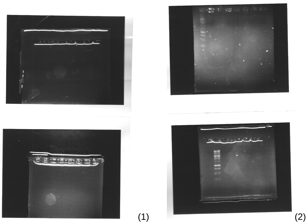
Figure 2.8 Molecular identification of the isolated cultures.
