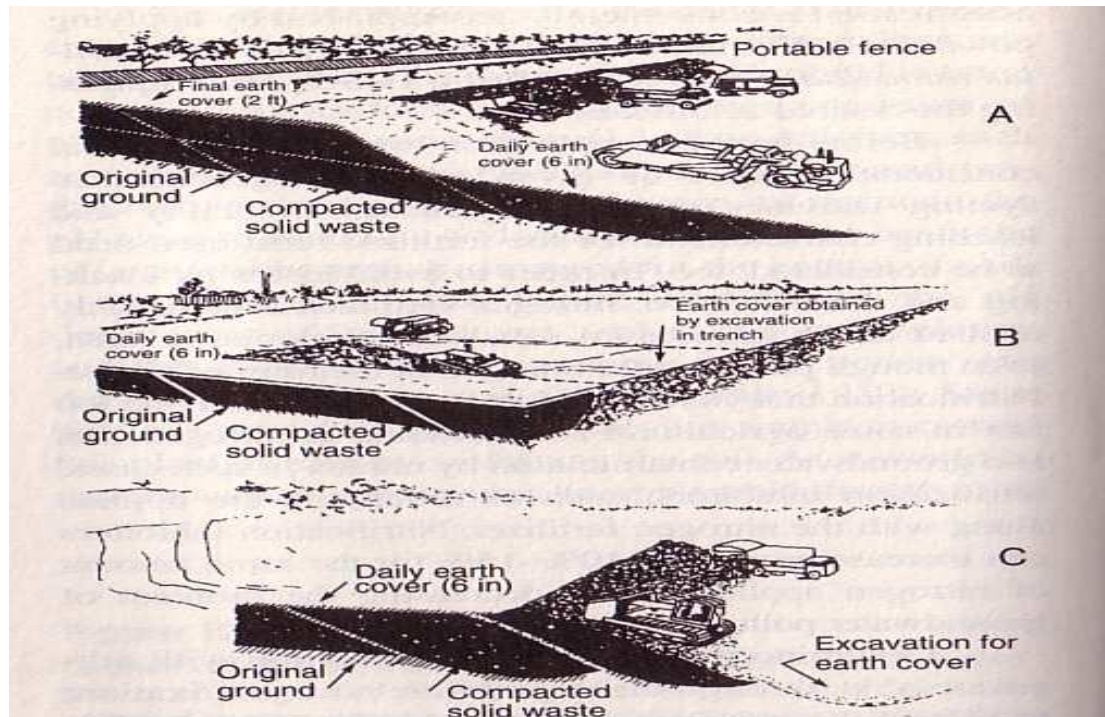
Figure 1.1 Landfill operation
