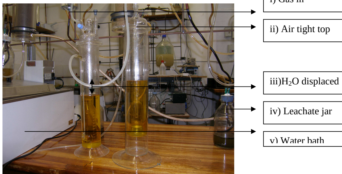
Figure 2.5: Gas displacement unit
