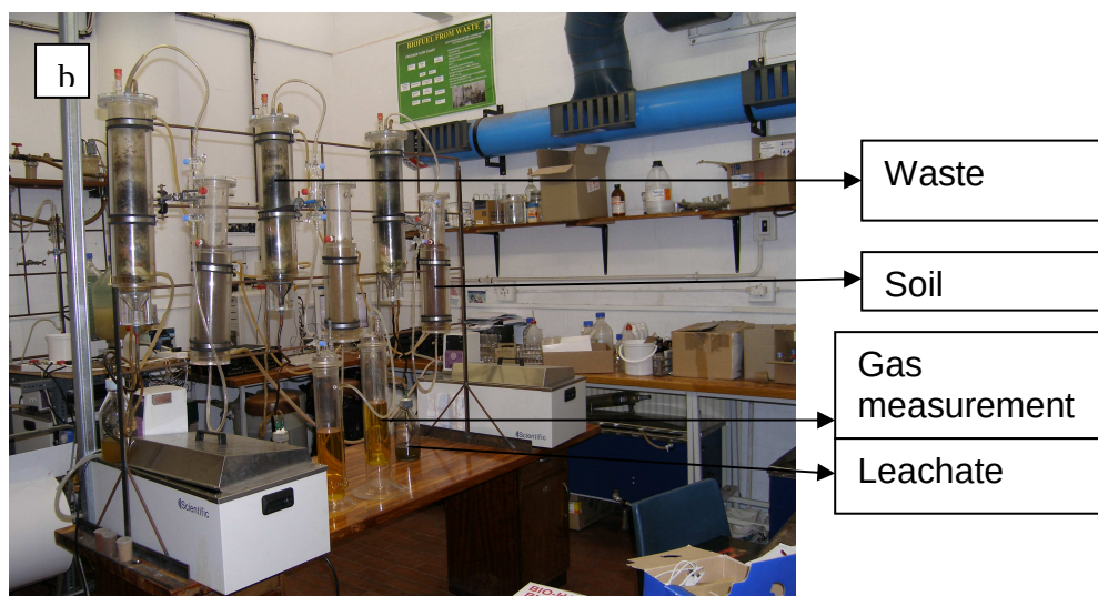
Figure 4.6 Apparatus set for this study (a) as set for the experiment, (b) experiment running
