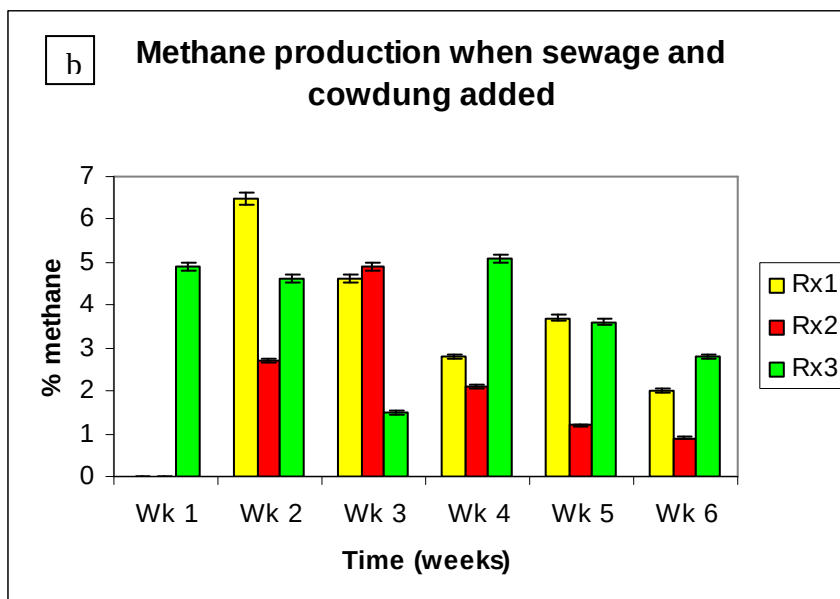
Graph 4.2b Methane production
