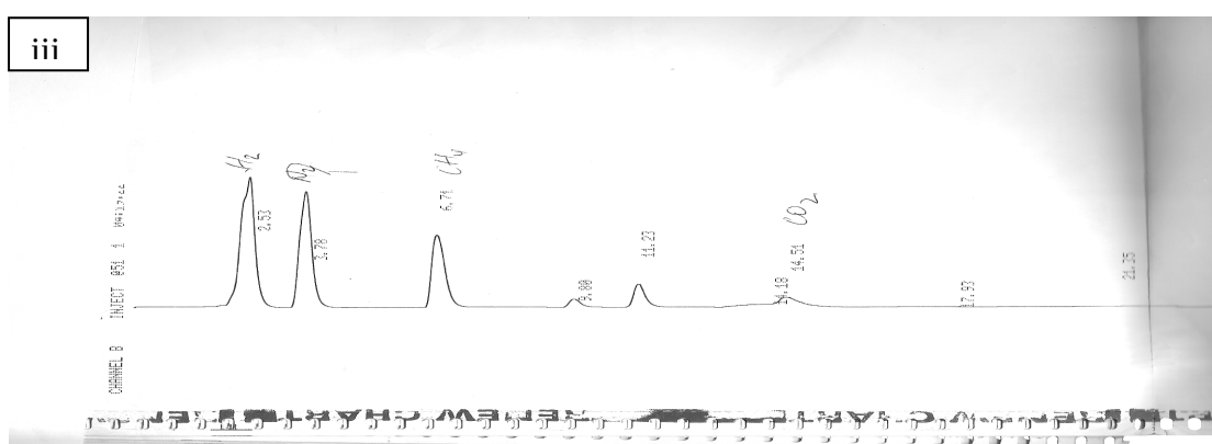
Figure 4.9 Gas analysis electrographs (i) Calibration curve; (ii) Gas from waste reactor; (iii) Gas after passing through soil
