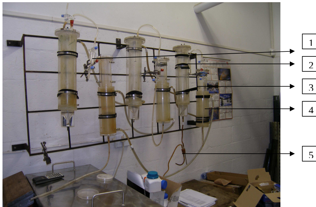
Figure 2.2: Bioreactors set-up (anaerobic reactor, aerobic reactor, gas sampling and effluent collection).
