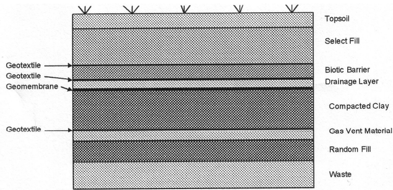
Figure B-1. Landfill cover with all optional layers.
