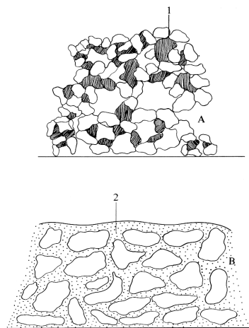
Figure 4.1 Soil structure as a function of colloid state
