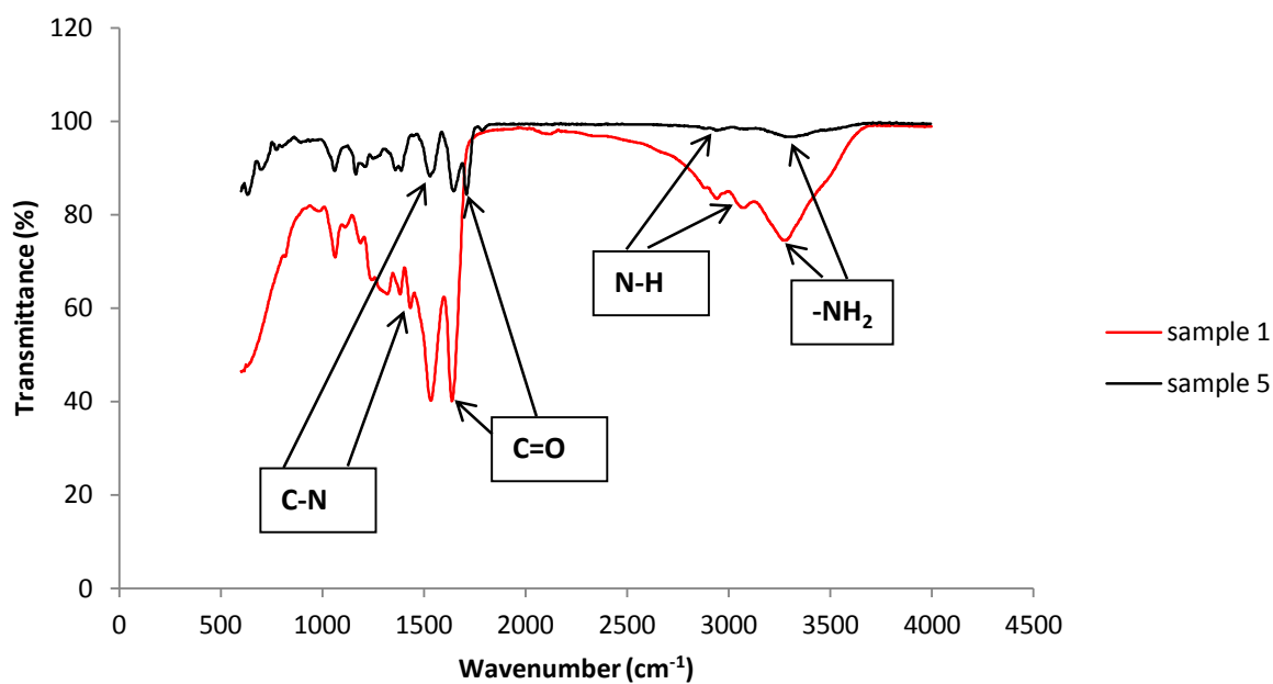
Fig. 7. FTIR analysis showing relevant peaks in the chemical structure of PSI-MA-EDA.
