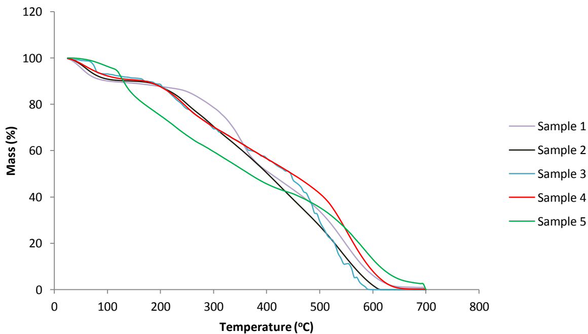
Fig. 9. Thermal stability analysis of PSI-MA-EDA samples showing variation of mass loss with temperature.
