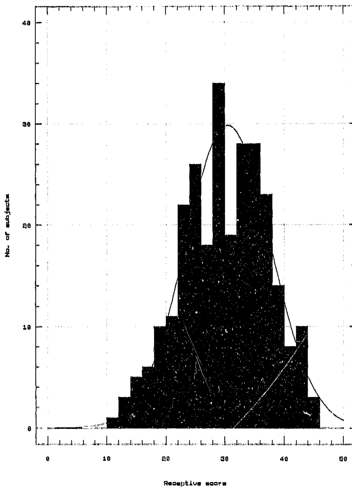
Frequency histogram of receptive scores
