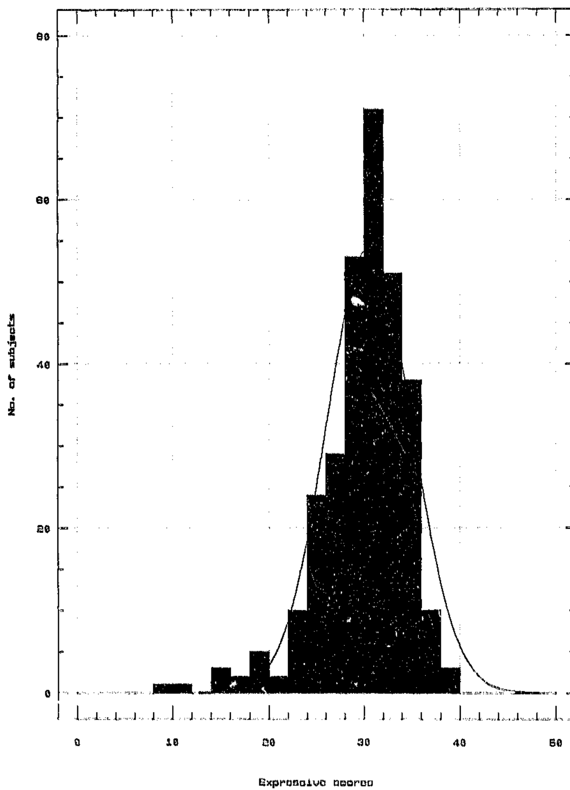
Frequency histogram of expressive scores
