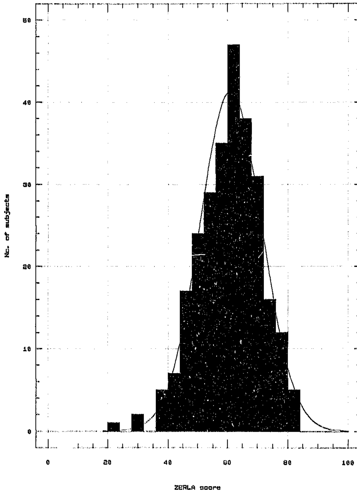
Frequency histogram of ZERLA scores
