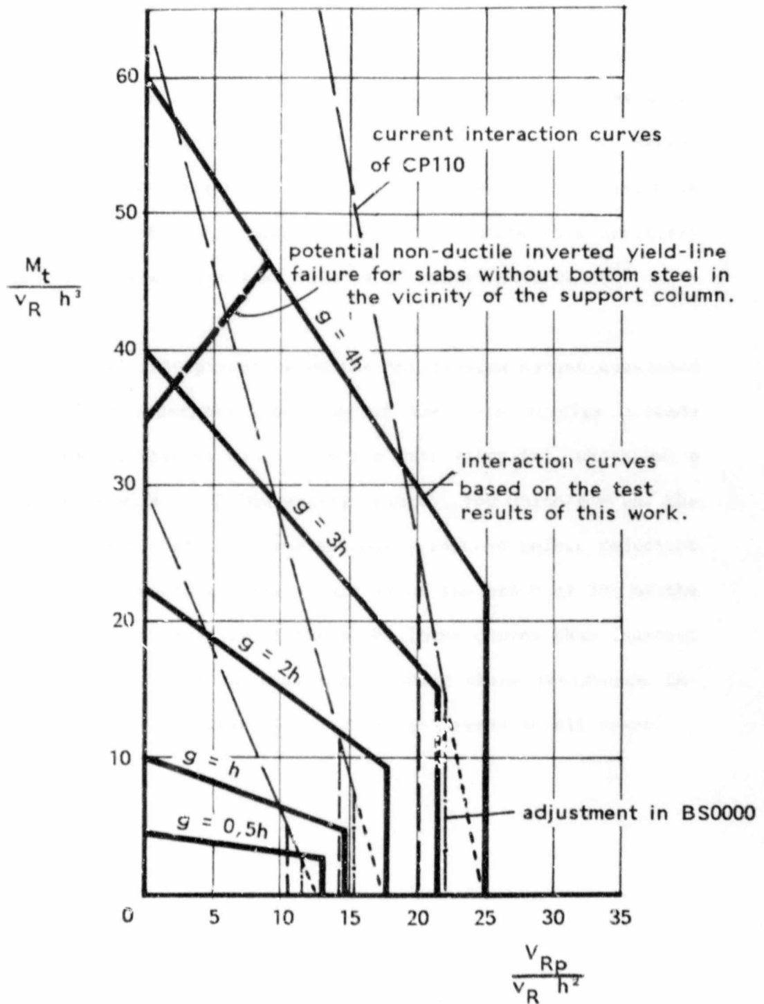
FIGURE 4.12 ULTIMATE PUNCHING SHEAR-TRANSFER MOMENT INTERACTION CURVES FOR TYPICAL FLAT PLATE REINFORCED CONCRETE STRUCTURES.
