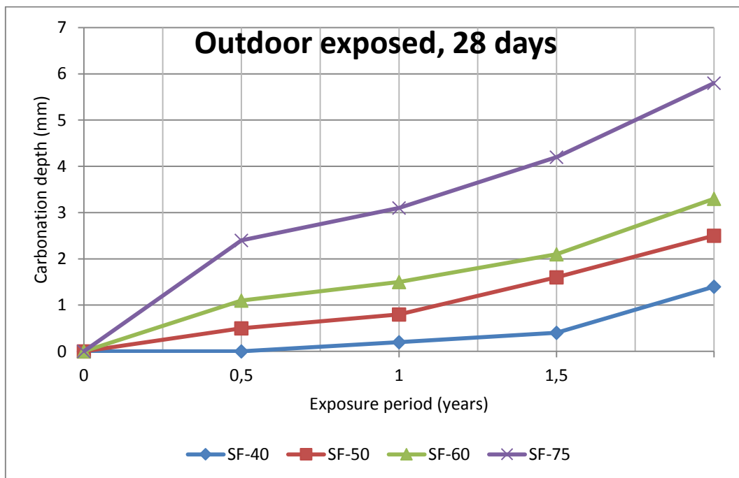
Figure 44 Carbonation depth Vs. Exposure period
