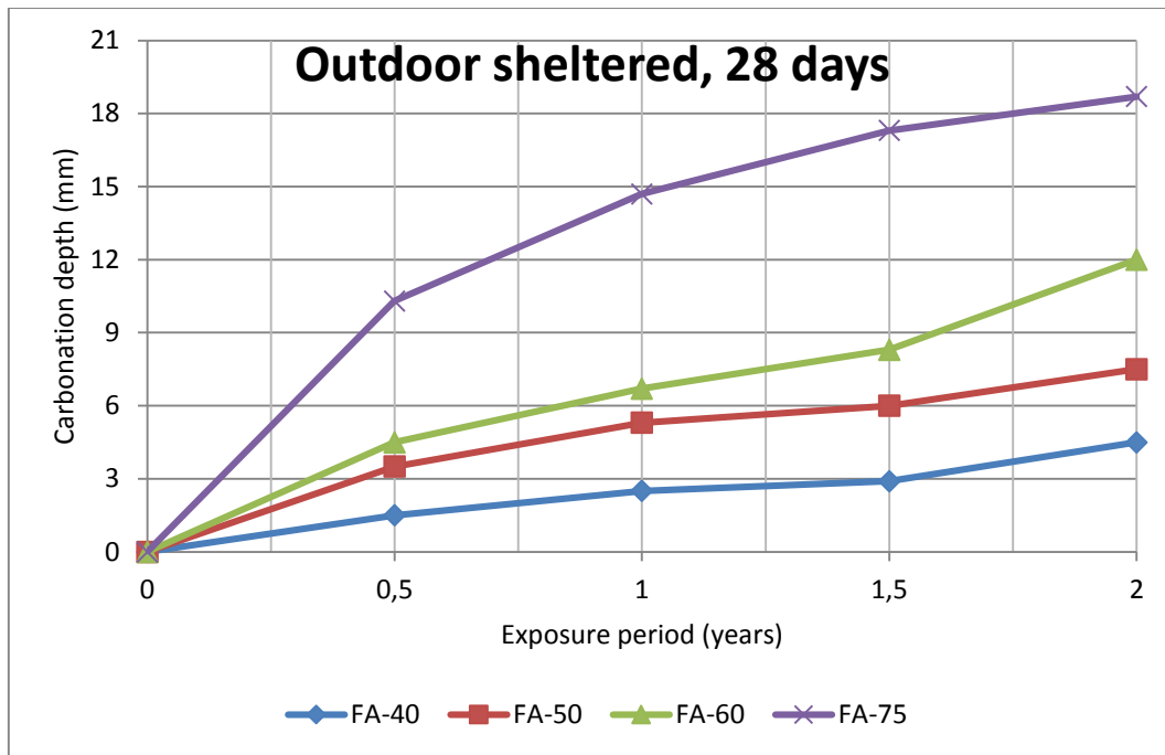
Figure 27 Carbonation depth Vs. Exposure period
