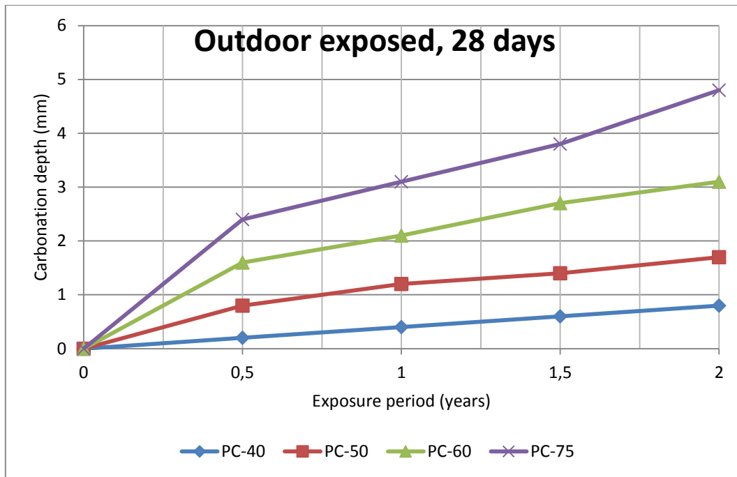
Figure 41 Carbonation depth Vs. Exposure period
