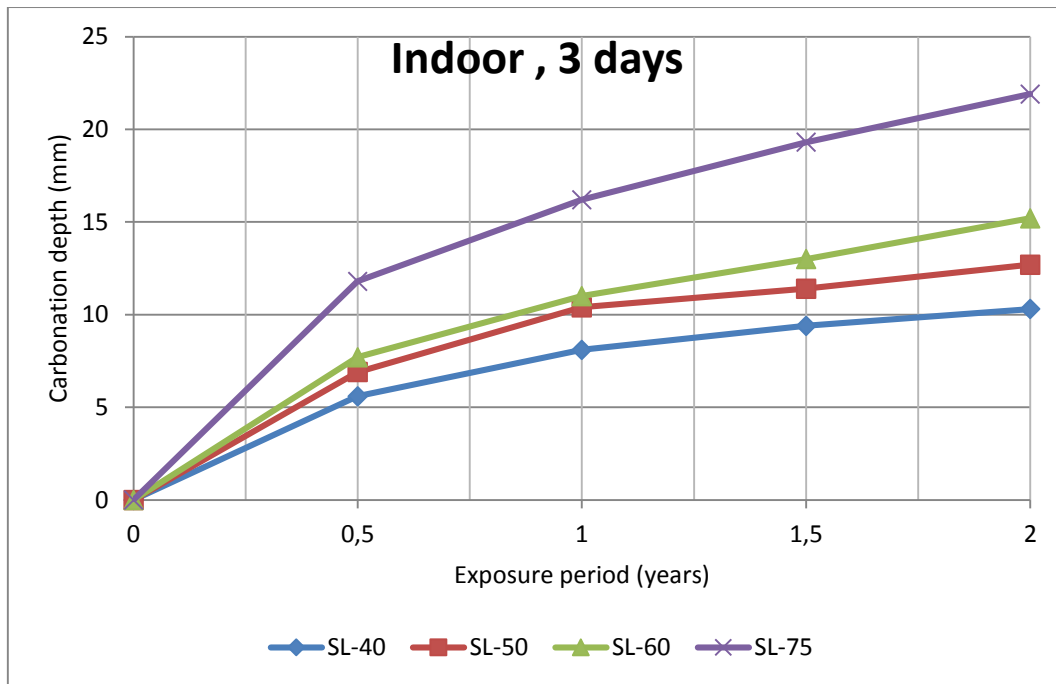
Figure 3 Carbonation depth Vs. Exposure period
