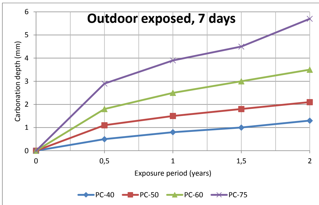
Figure 36 Carbonation depth Vs. Exposure period
