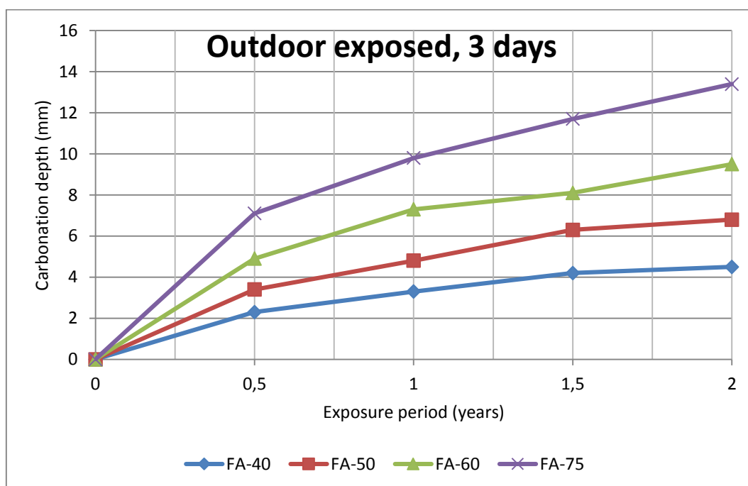
Figure 32 Carbonation depth Vs. Exposure period
