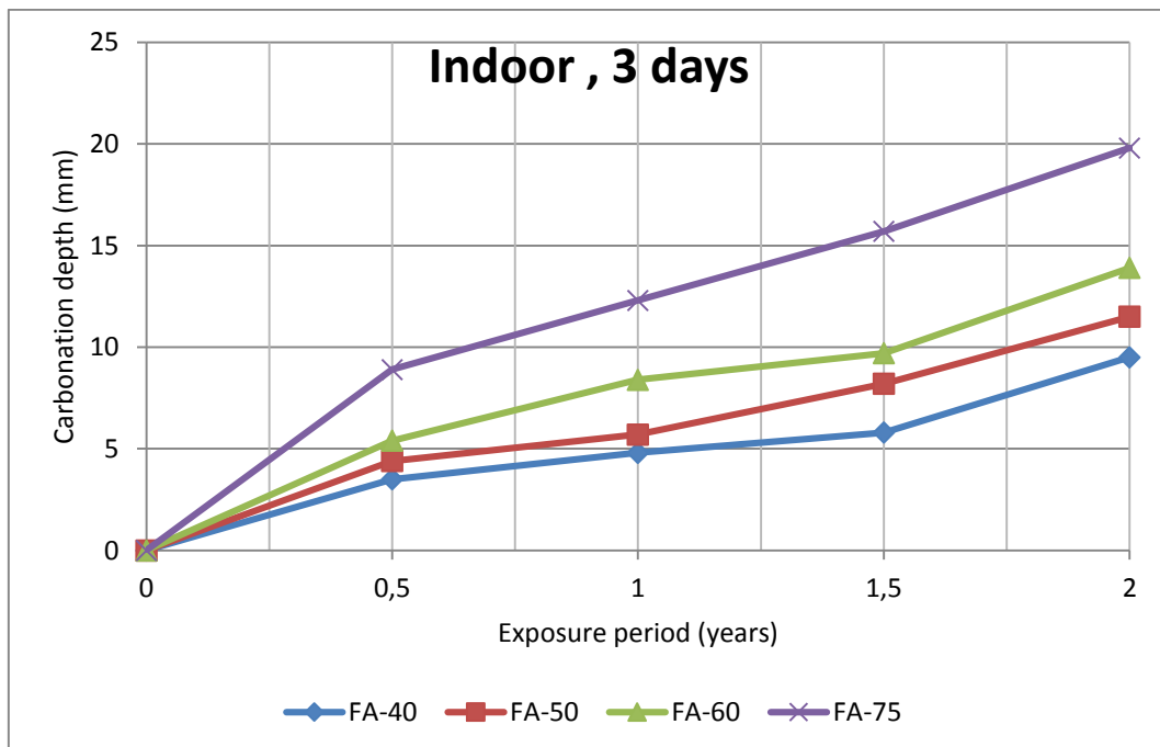
Figure 2 Carbonation depth Vs. Exposure period
