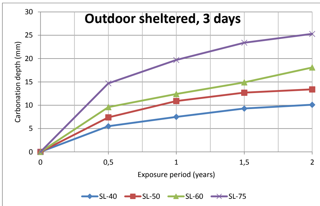
Figure 18 Carbonation depth Vs. Exposure period
