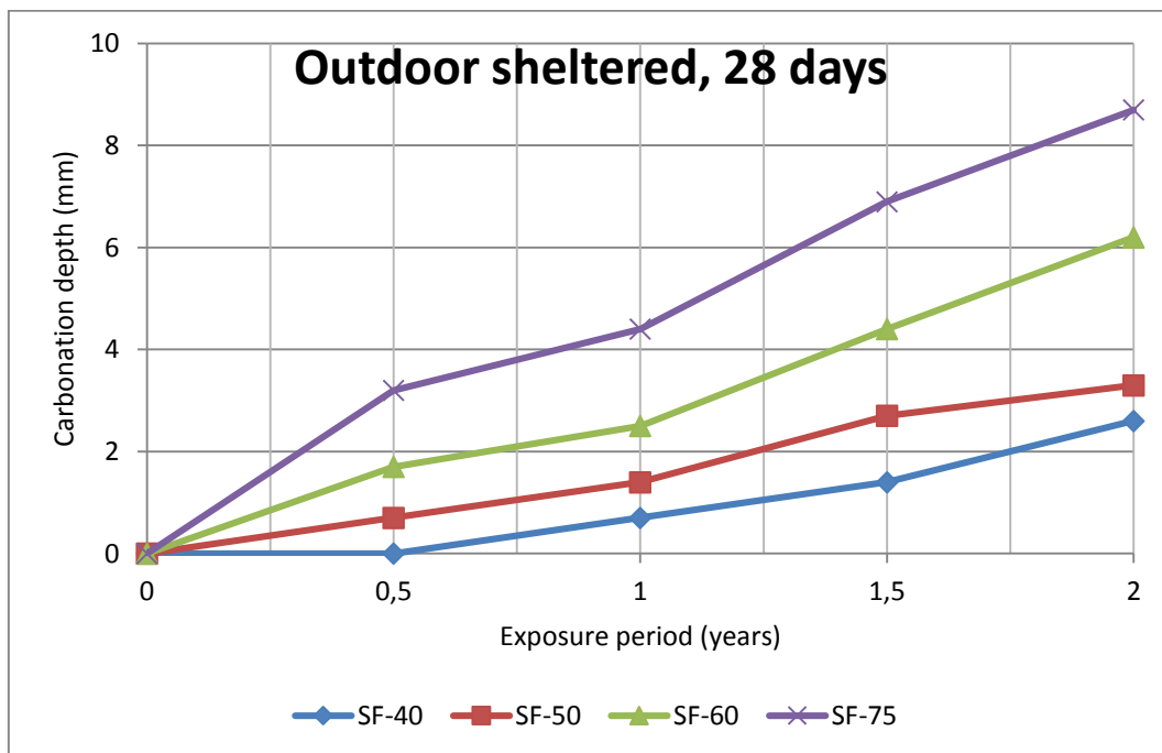
Figure 30 Carbonation depth Vs. Exposure period
