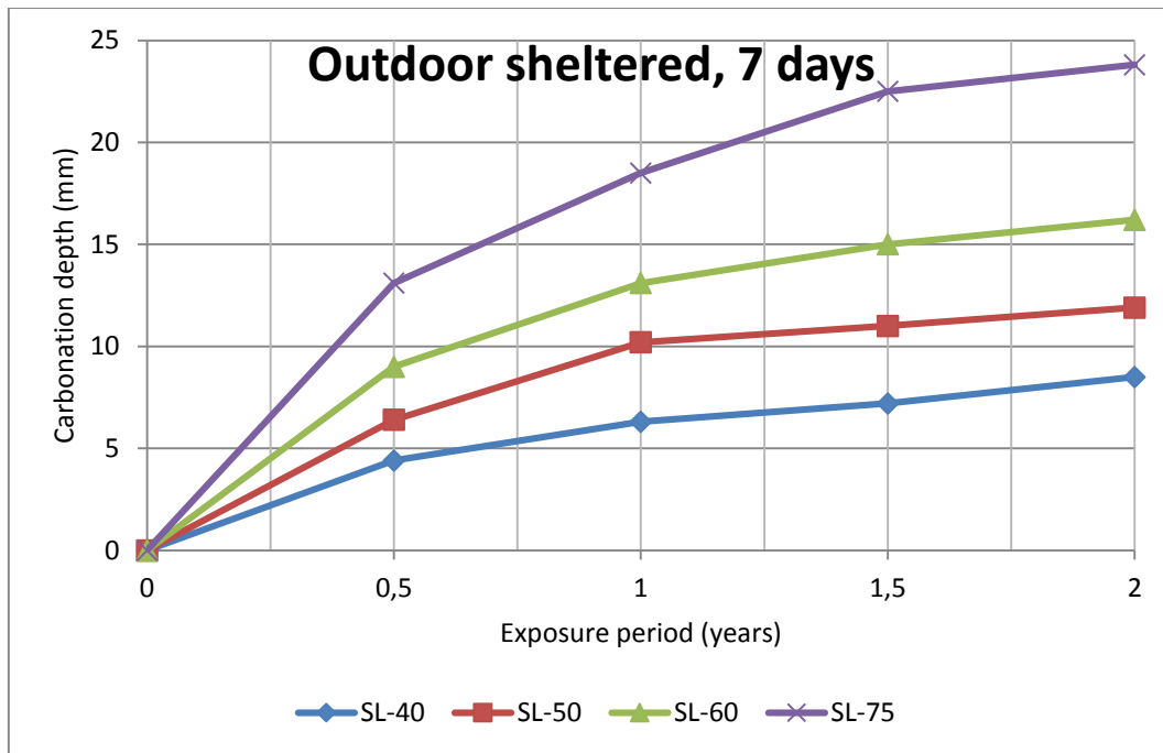
Figure 23 Carbonation depth Vs. Exposure period
