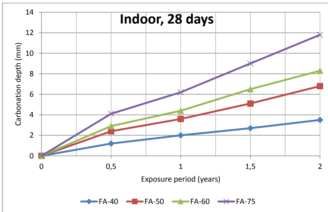
Figure 12 Carbonation depth Vs. Exposure period
