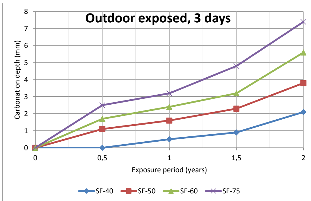
Figure 34 Carbonation depth Vs. Exposure period
