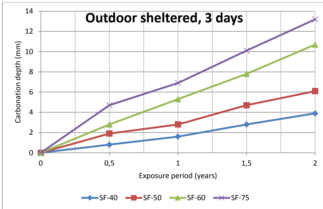
Figure 19 Carbonation depth Vs. Exposure period
