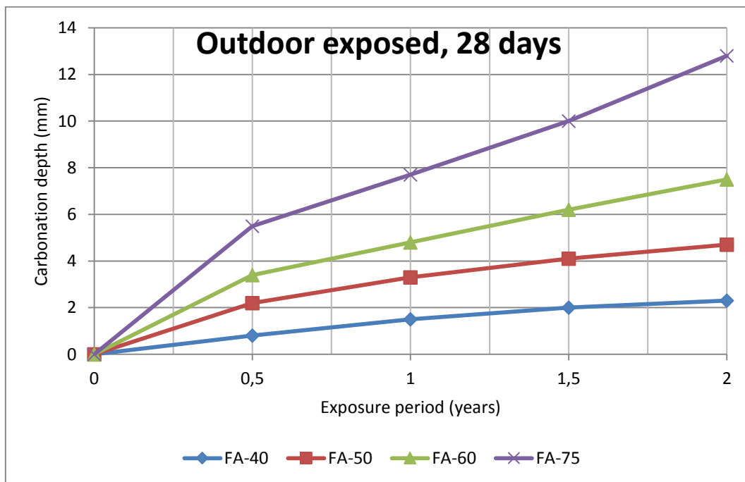
Figure 42 Carbonation depth Vs. Exposure period
