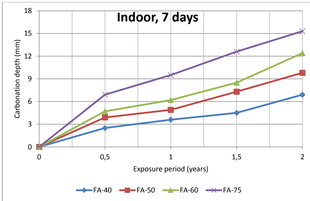
Figure 7 Carbonation depth Vs. Exposure period
