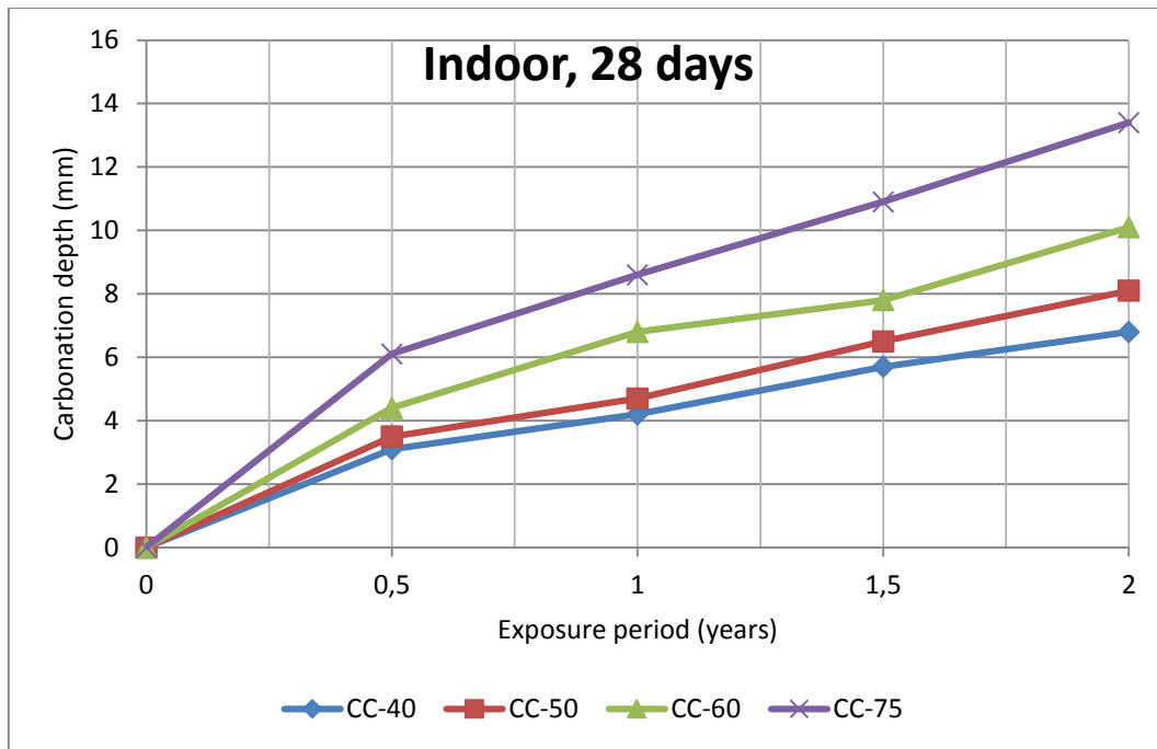
Figure 15 Carbonation depth Vs. Exposure period
