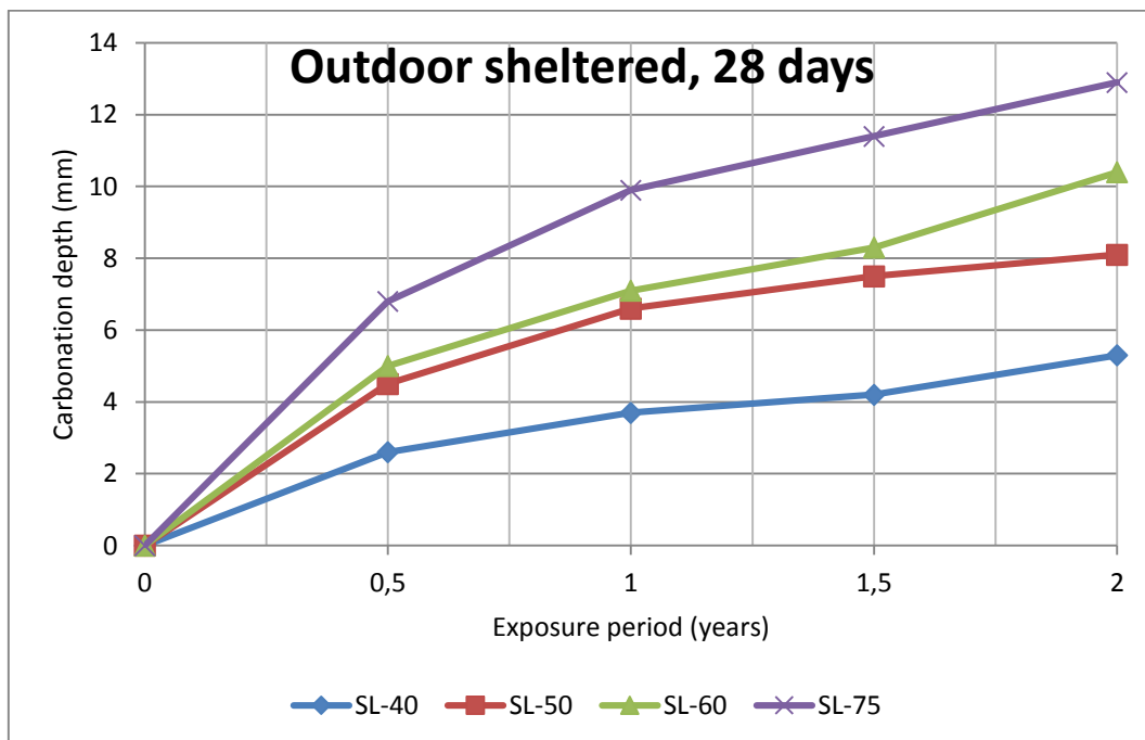
Figure 28 Carbonation depth Vs. Exposure period
