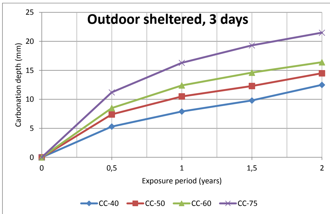
Figure 20 Carbonation depth Vs. Exposure period
