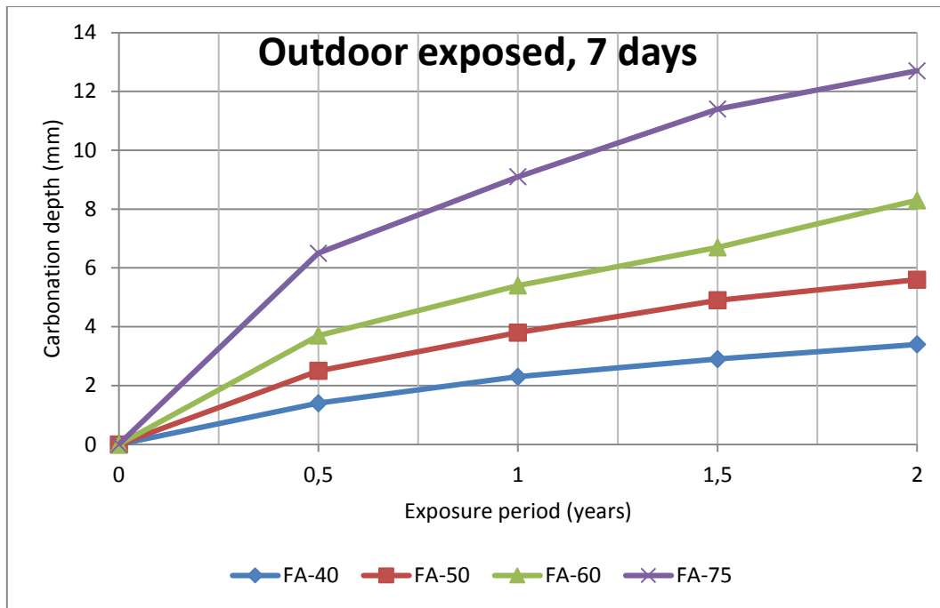
Figure 37 Carbonation depth Vs. Exposure period
