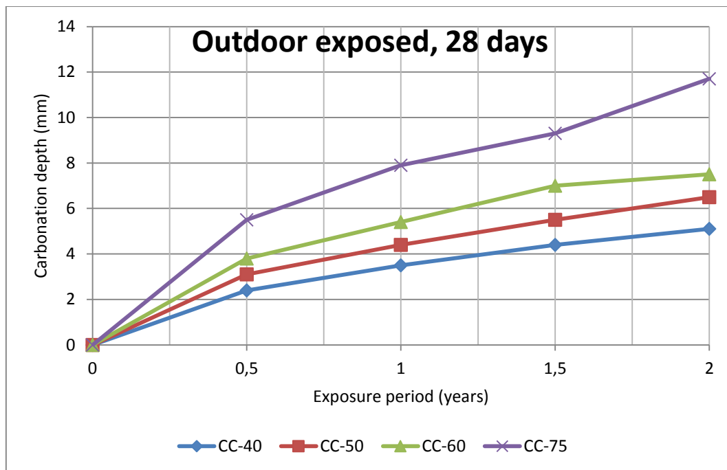
Figure 45 Carbonation depth Vs. Exposure period
