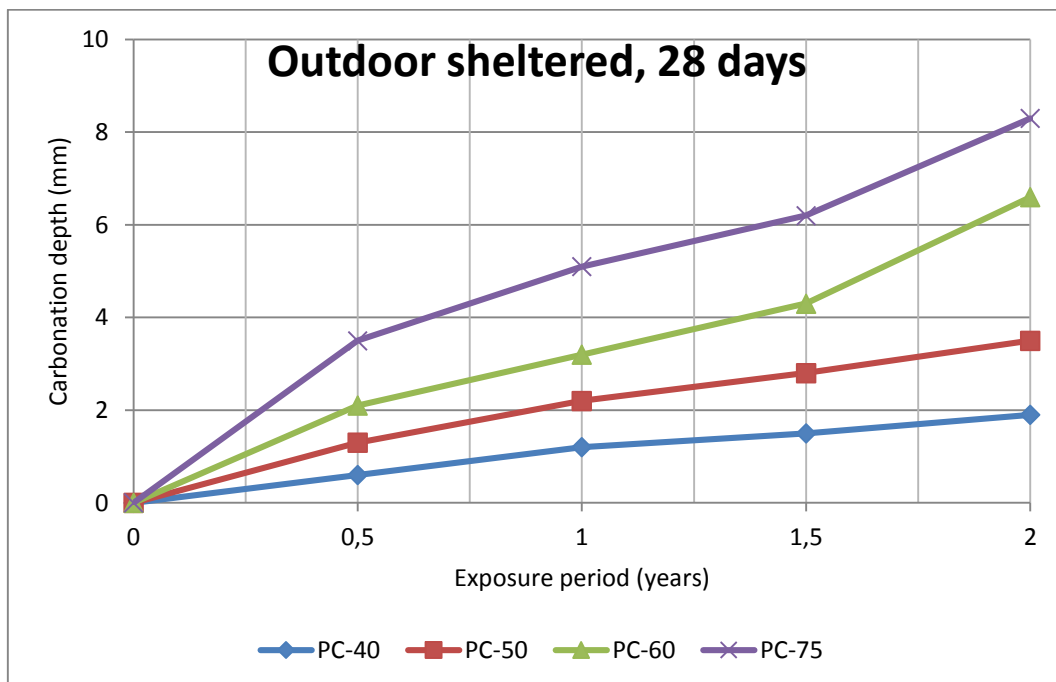
Figure 26 Carbonation depth Vs. Exposure period
