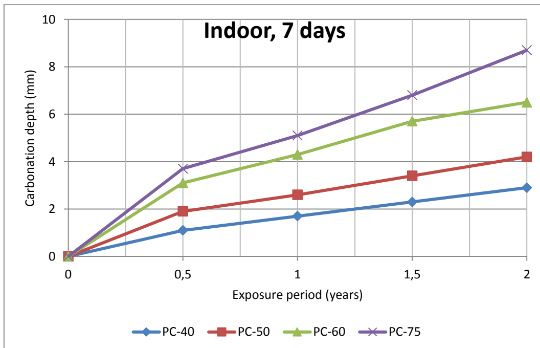
Figure 6 Carbonation depth Vs. Exposure period
