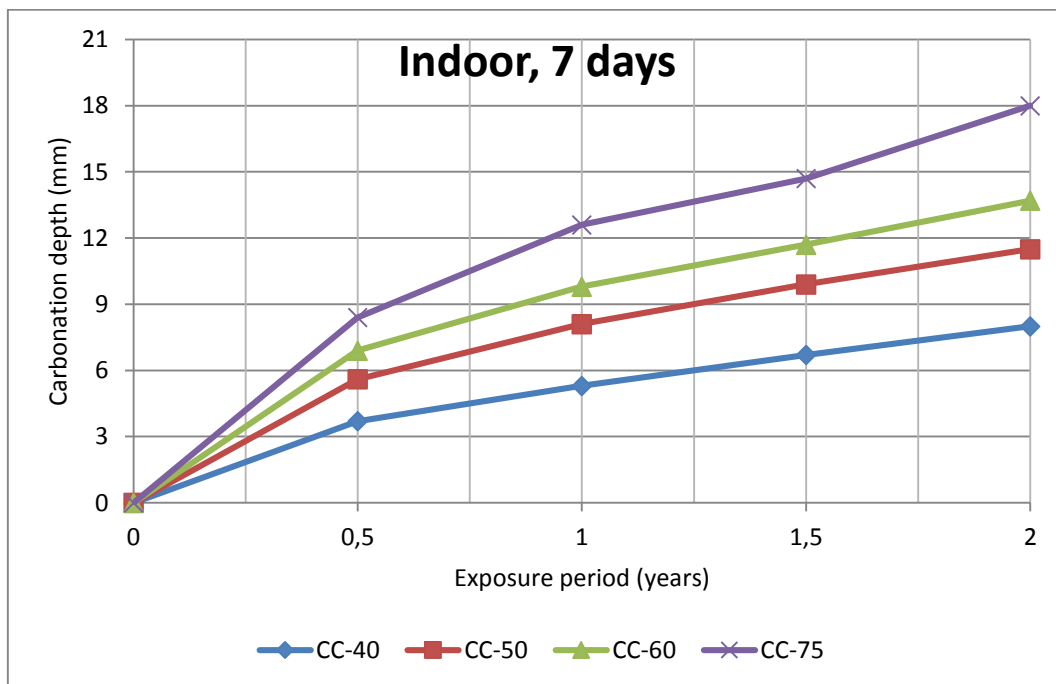
Figure 10 Carbonation depth Vs. Exposure period
