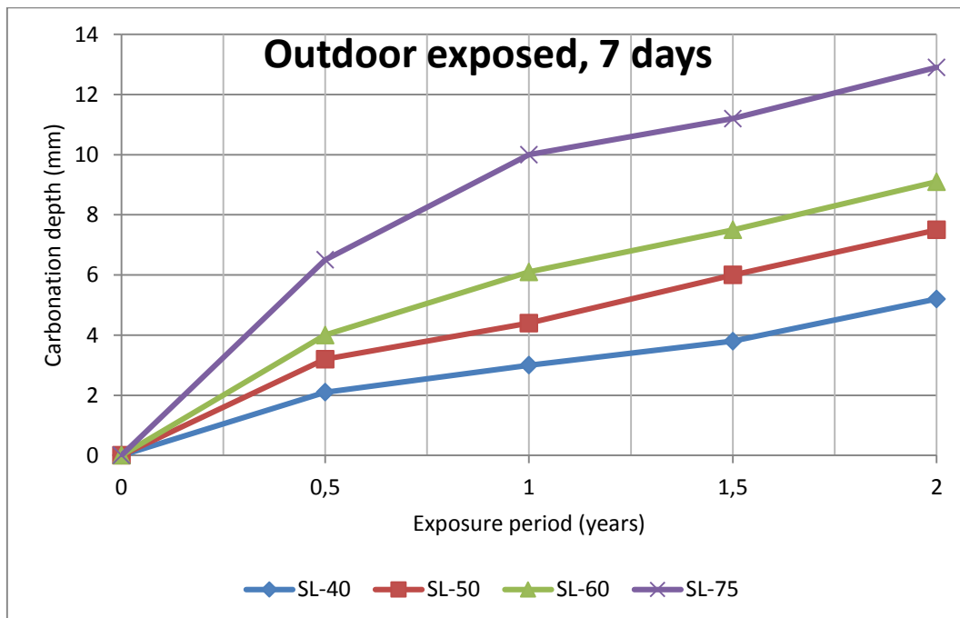
Figure 38 Carbonation depth Vs. Exposure period
