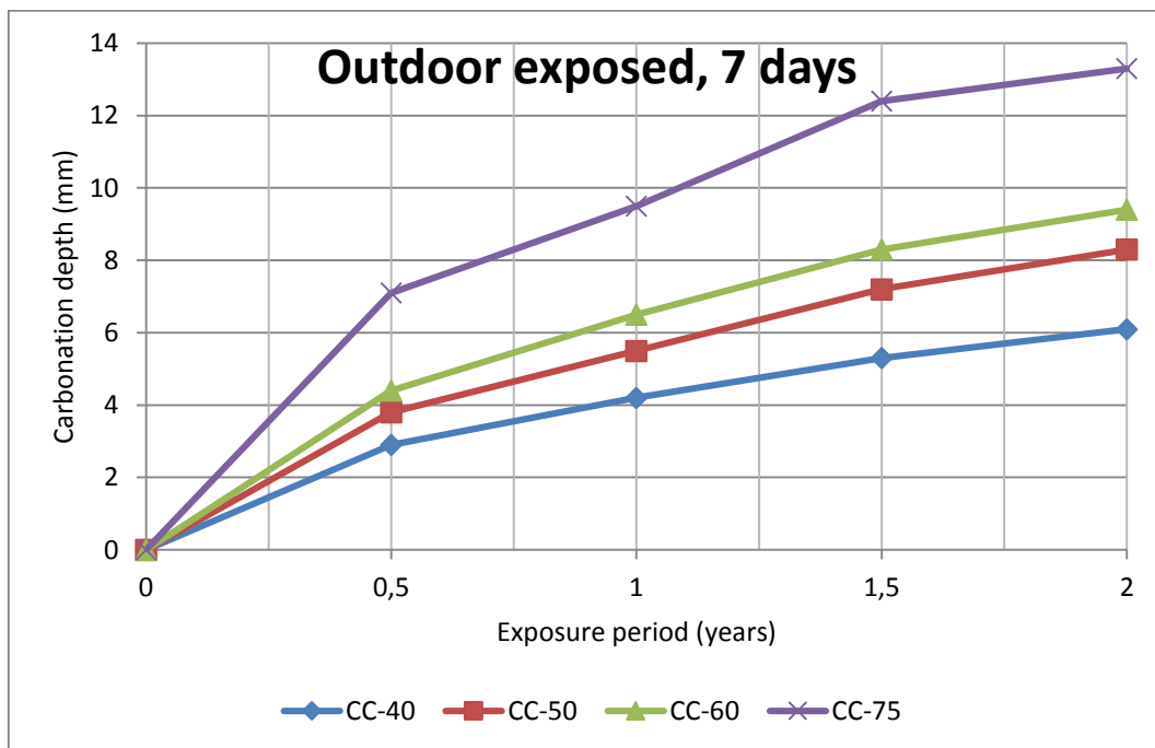
Figure 40 Carbonation depth Vs. Exposure period
