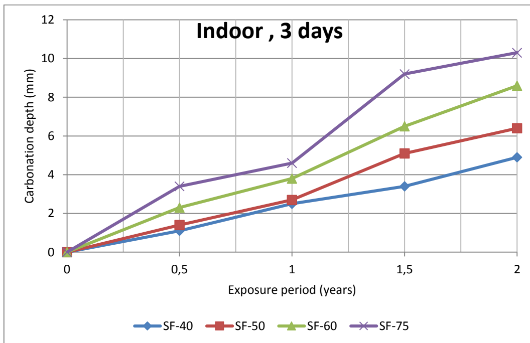
Figure 4 Carbonation depth Vs. Exposure period
