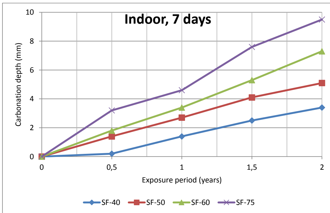
Figure 8 Carbonation depth Vs. Exposure period
