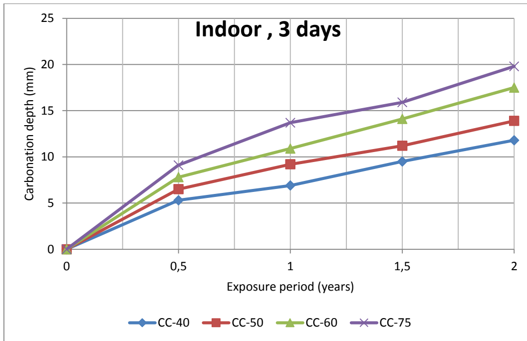
Figure 5 Carbonation depth Vs. Exposure period
