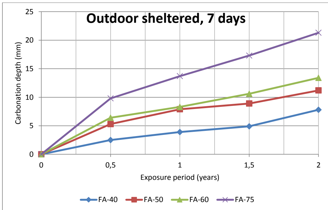
Figure 22 Carbonation depth Vs. Exposure period
