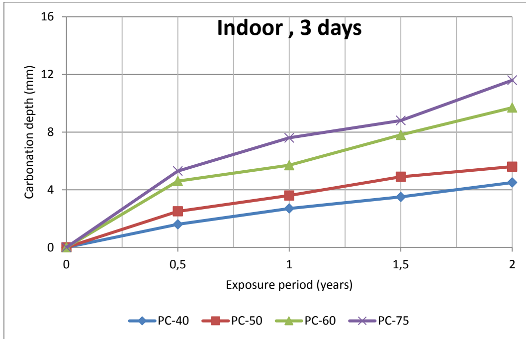
Figure 1 Carbonation depth Vs. Exposure period
