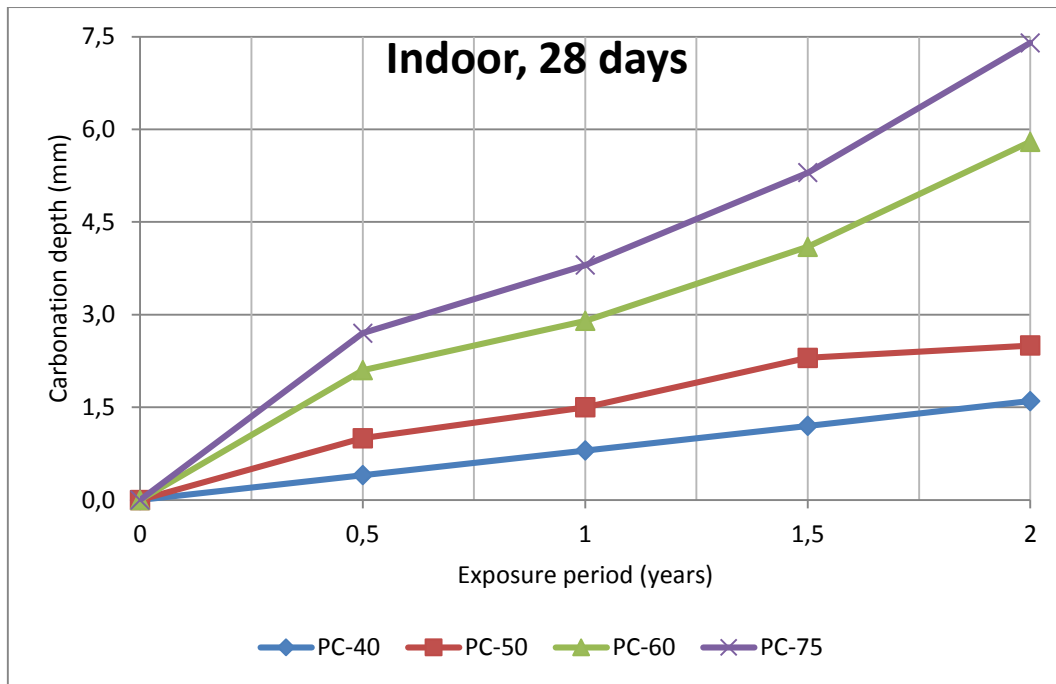
Figure 11 Carbonation depth Vs. Exposure period
