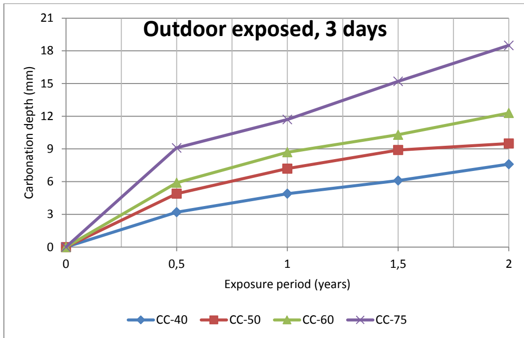
Figure35 Carbonation depth Vs. Exposure period
