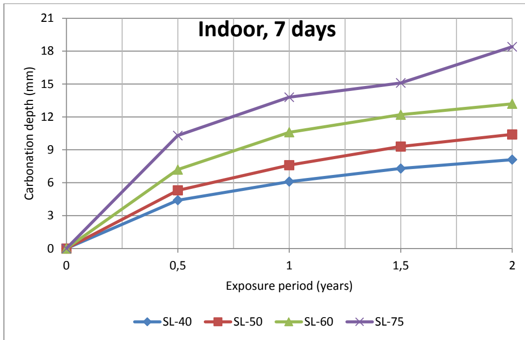
Figure 9 Carbonation depth Vs. Exposure period
