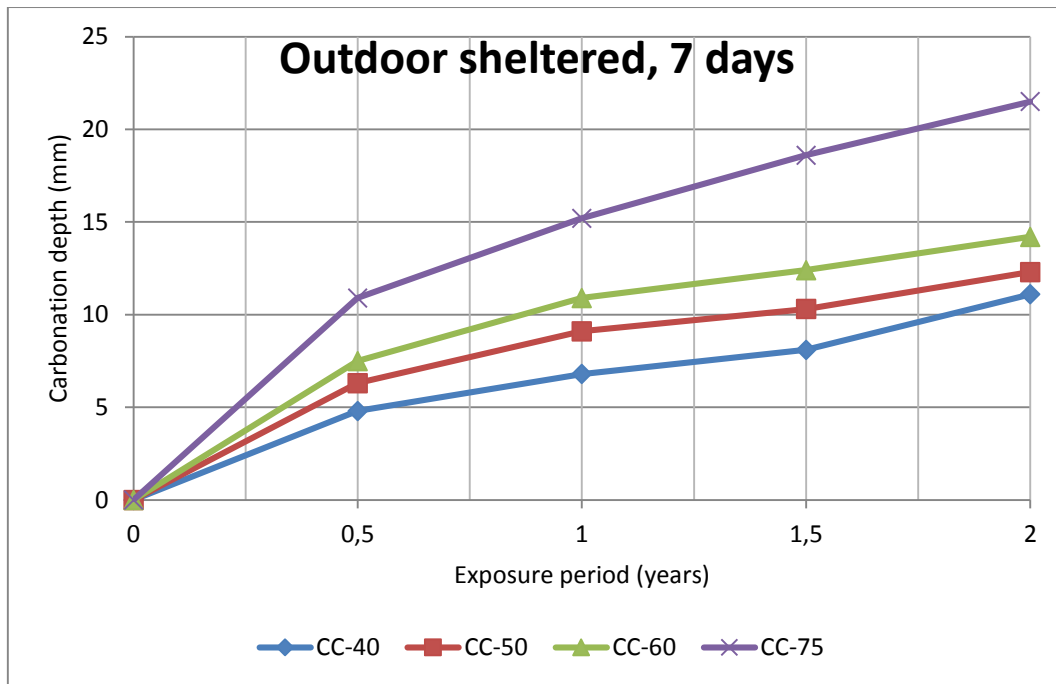
Figure 25 Carbonation depth Vs. Exposure period
