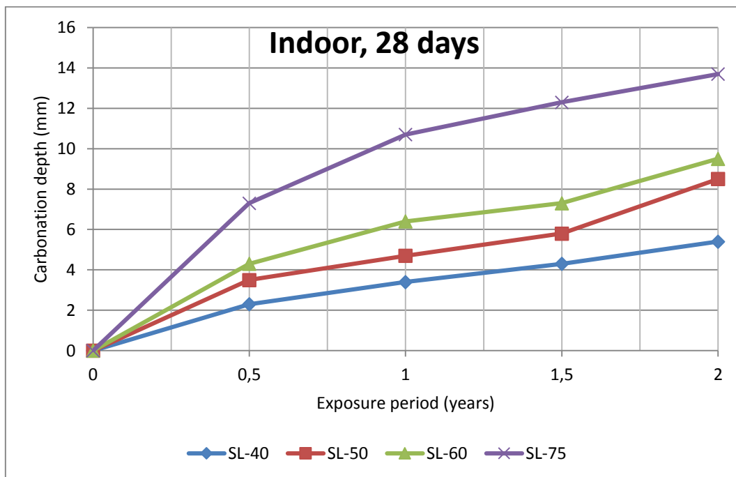
Figure 14 Carbonation depth Vs. Exposure period
