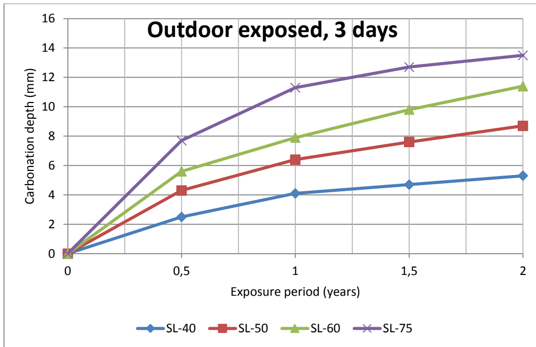
Figure 33 Carbonation depth Vs. Exposure period
