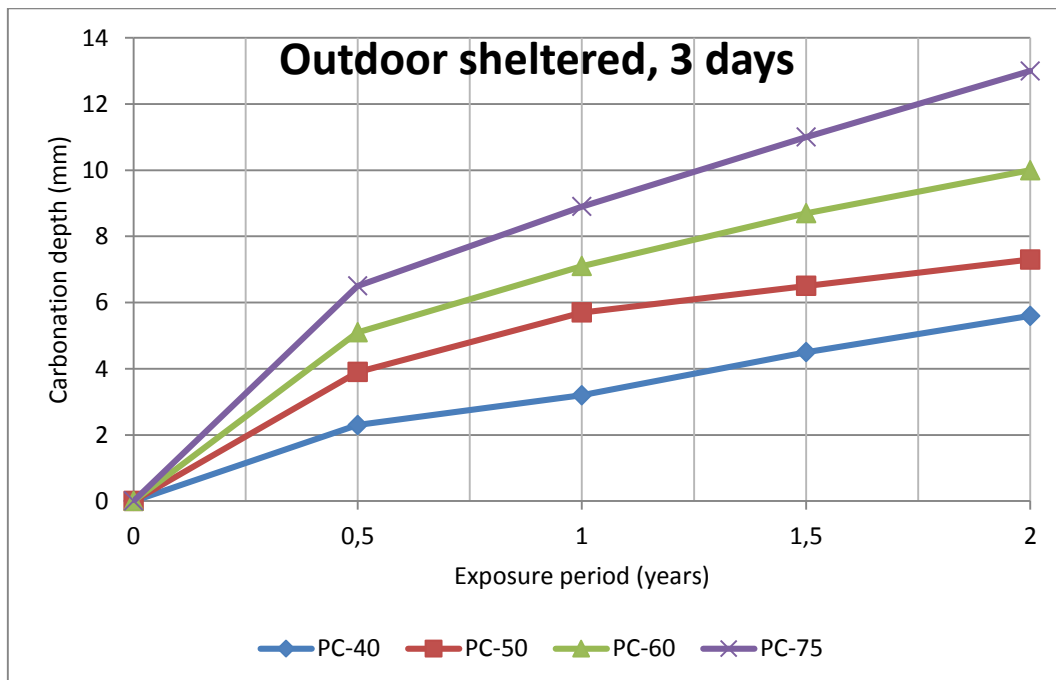
Figure 16 Carbonation depth Vs. Exposure period
