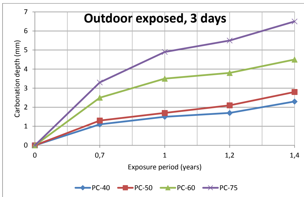
Figure 31 Carbonation depth Vs. Exposure period
