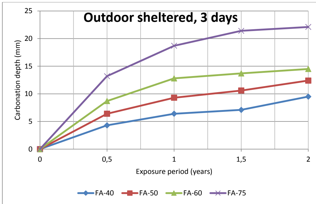
Figure 17 Carbonation depth Vs. Exposure period
