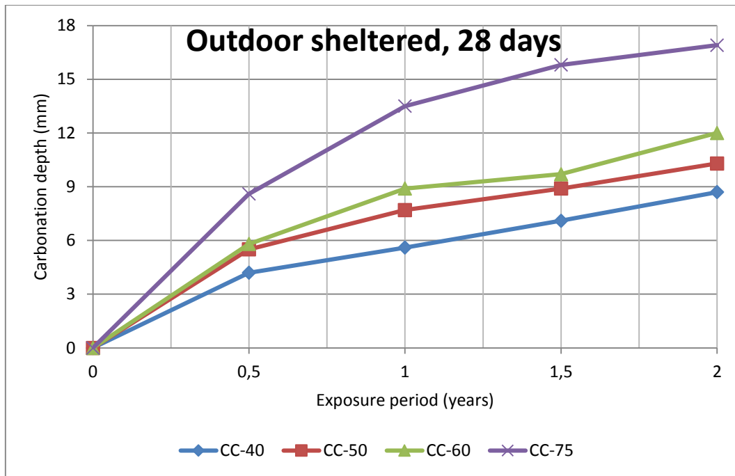
Figure 29 Carbonation depth Vs. Exposure period
