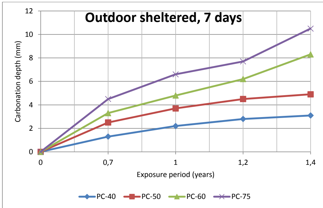
Figure 21 Carbonation depth Vs. Exposure period
