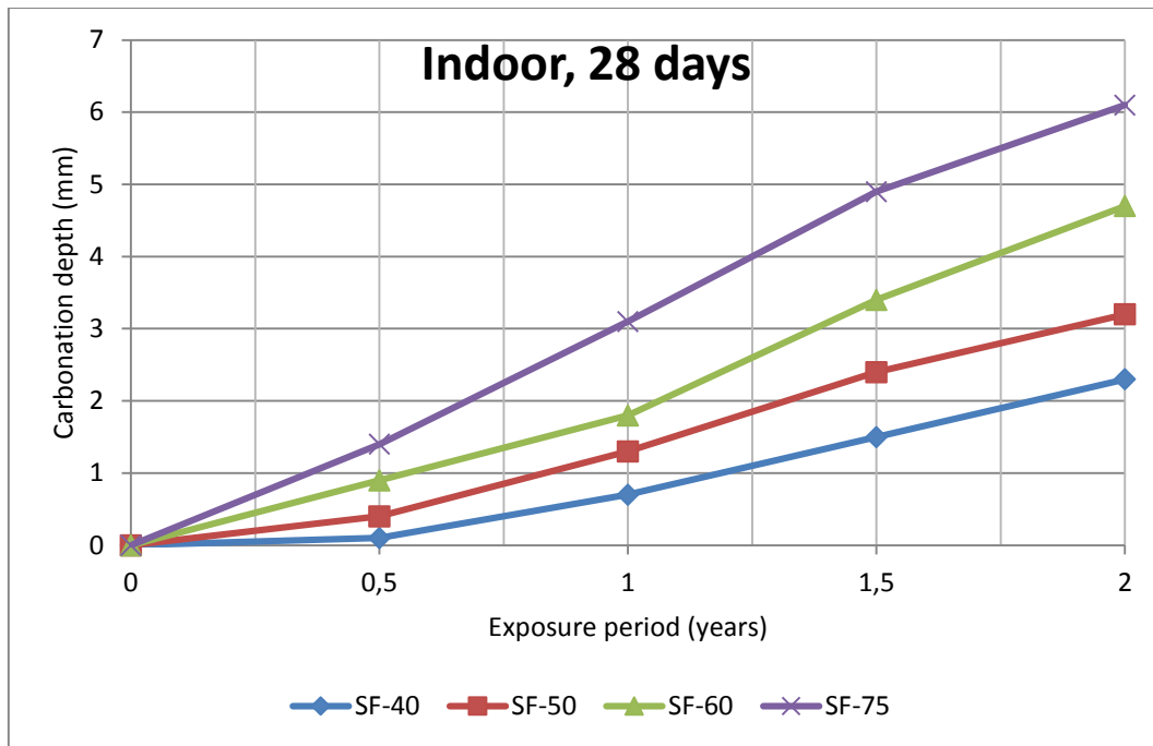
Figure 13 Carbonation depth Vs. Exposure period
