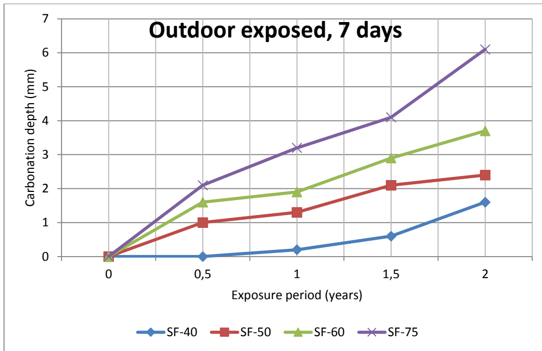
Figure 39 Carbonation depth Vs. Exposure period
