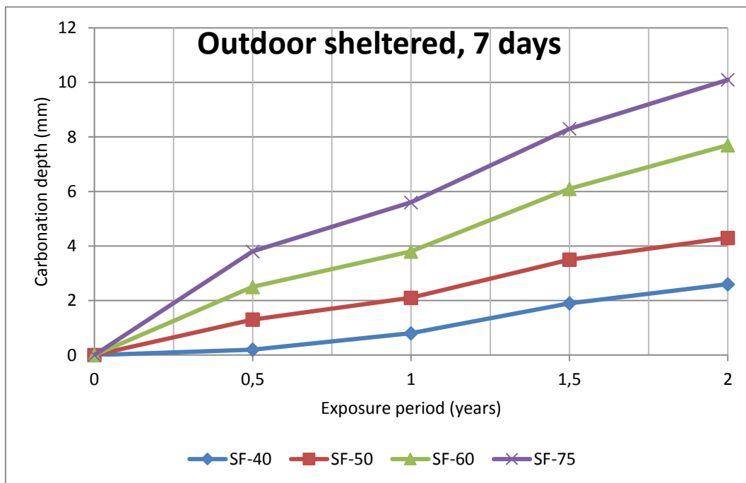
Figure 24 Carbonation depth Vs. Exposure period
