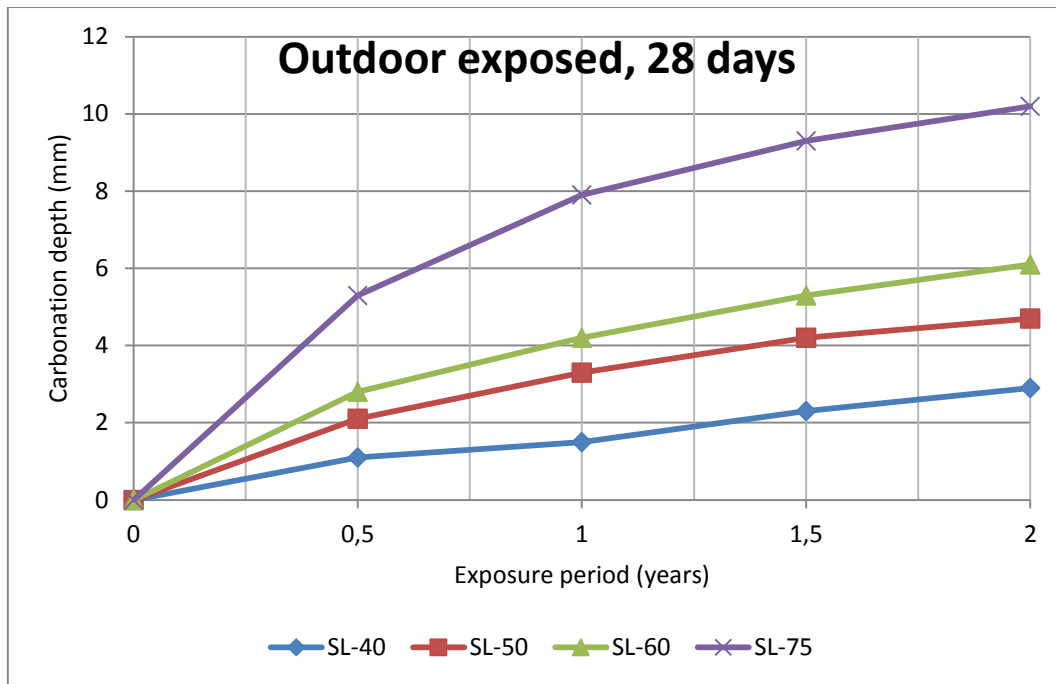
Figure 43 Carbonation depth Vs. Exposure period
