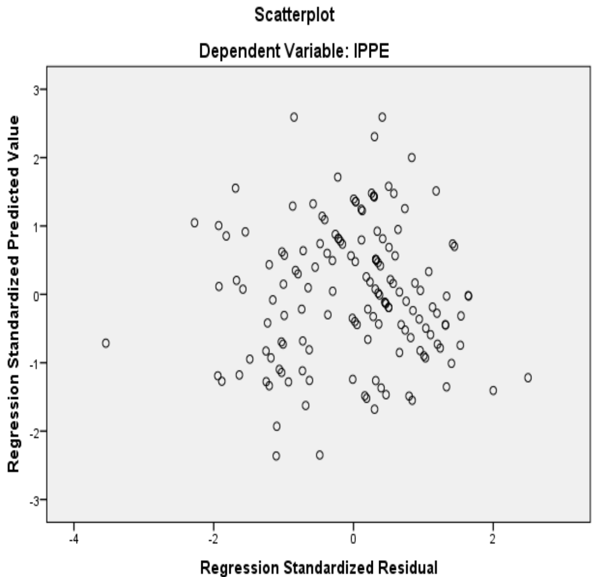
Figure 5.9 Scatter plot of scores
