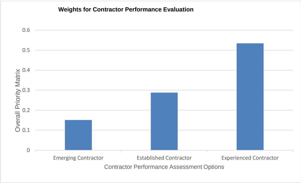
Figure 6.7 Weights for the overall priority matrix for contractor performance evaluation
