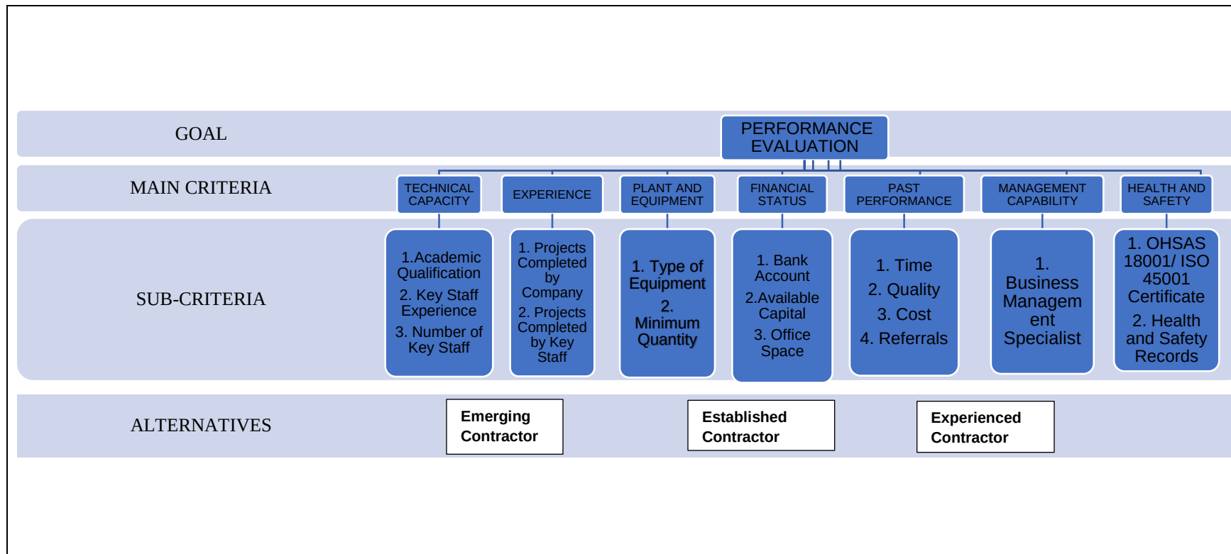
Figure 6.6 AHP for performance evaluation of contractors
