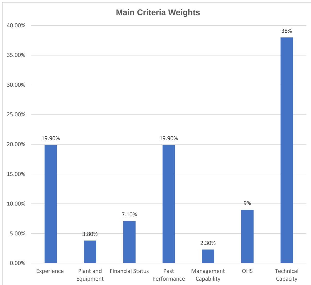
Figure 6.2 Main criteria weights
