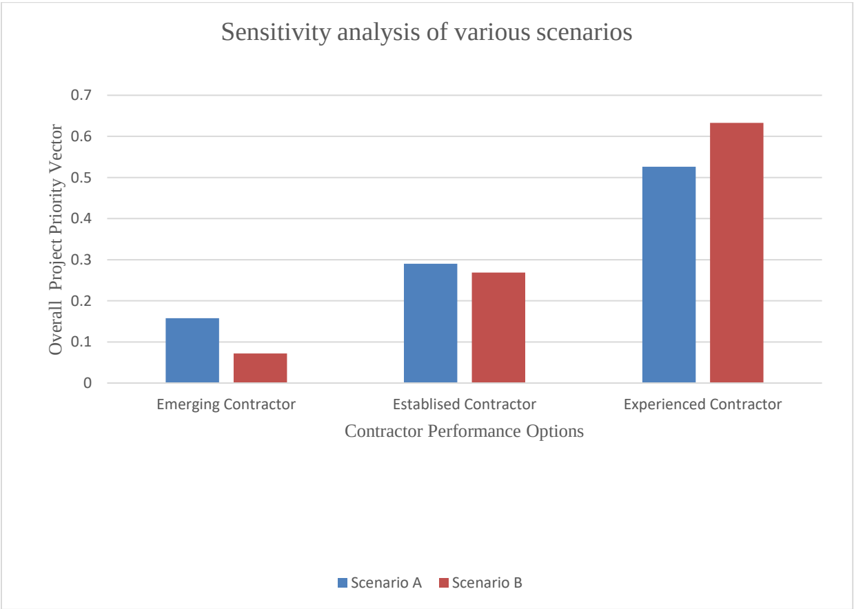
Figure 6.8 Sensitivity analysis of the two scenarios for performance evaluation alternatives
