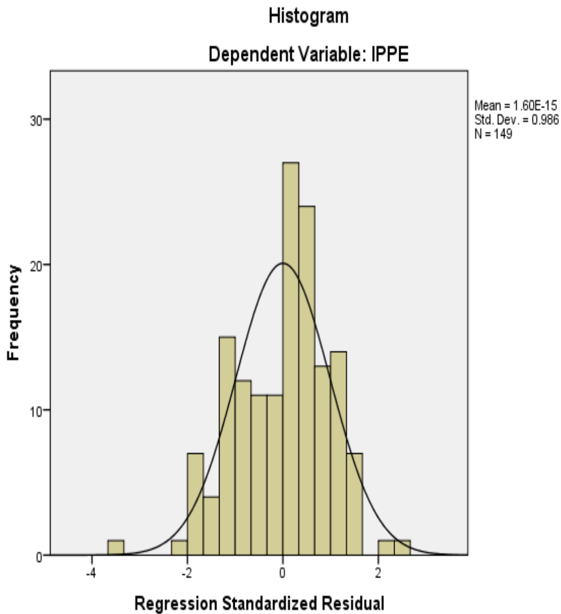
Figure 5.10 Normality of data points
