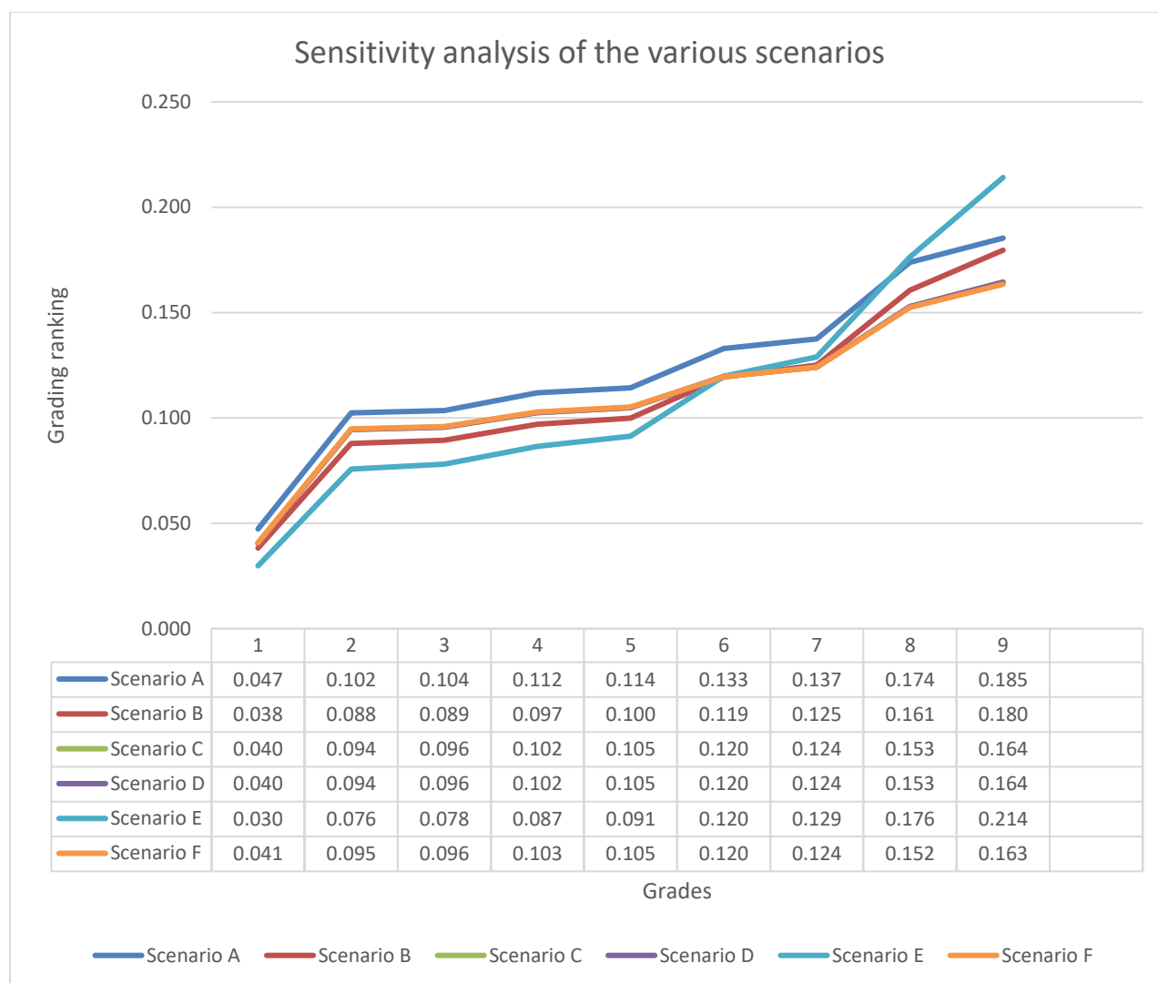
Figure 6.5 Overall grading rankings of the sensitivity analysis
