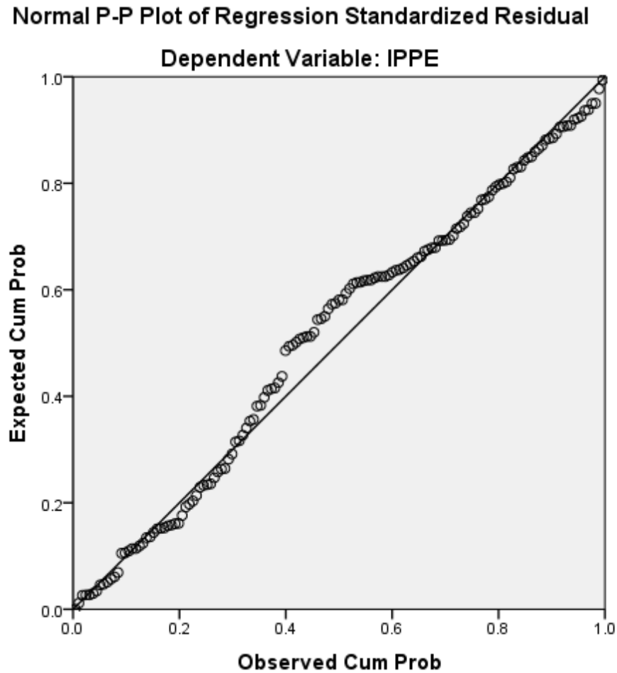
Figure 5.11 Normal P-P plot of regression residuals
