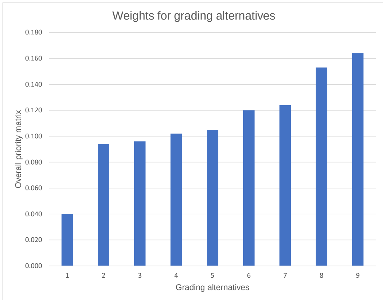
Figure 6.4 Weights of the overall priority matrix for grading alternatives
