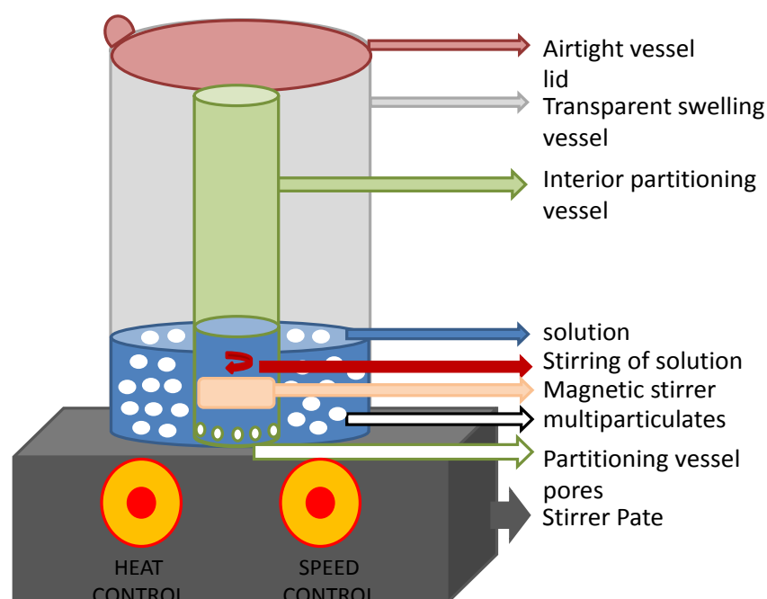
Figure 4.5: Schematic representation of experimental apparatus.
