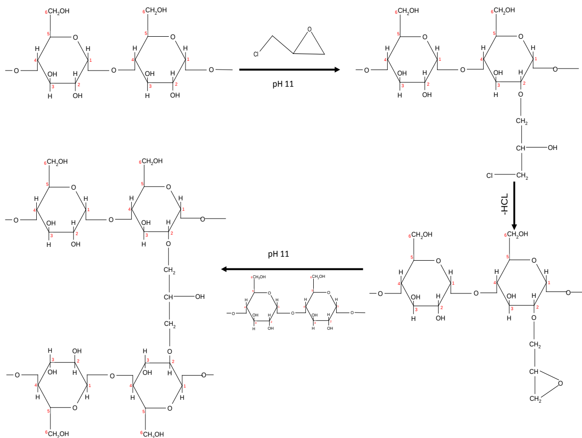
Figure 5.6: ECH-facilitated crosslinking of starch.
