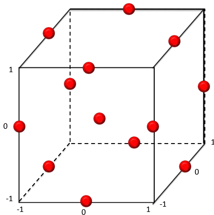
Figure 3.1: Schematic representation of design point of a 3-Factor, 3-level ( 3^3 ) Box-Behnken statistical design.
