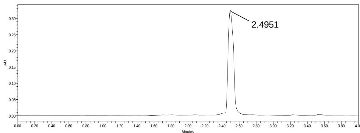
Figure 8.13: Chromatogram illustrating the retention time peak of SSZ (RT=2.4951 minutes).
