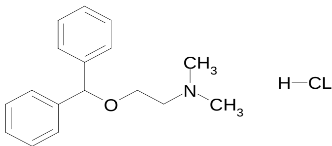
2-(Diphenylmethoxy)-N,N-dimethylethanamine hydrochloride
