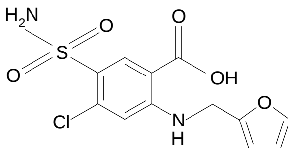
4-Chloro-N-furfuryl-5-sulfamoylanthranilic acid
