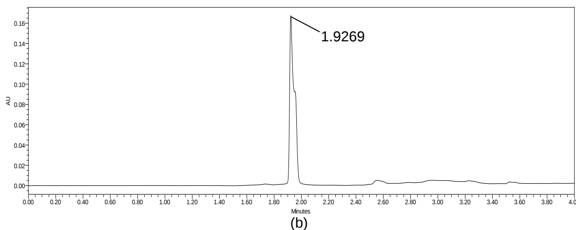
Figure 8.12: Chromatograms illustrating the retention time peaks of a) 5-ASA (RT=1.1928) and b) N-Acetyl-5-ASA (RT=1.9269).
