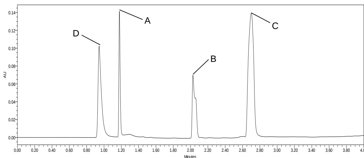
Figure 8.17: Chromatogram illustrating the separation of the retention time peaks of (A) 5-ASA (RT=1.1866 minutes), (B) N-Acetyl-5-ASA (RT=2.0228 minutes) and (C) SSZ (RT=2.6310 minutes) and (D) INH (RT=0.9961 minutes) subsequent to plasma extraction.
