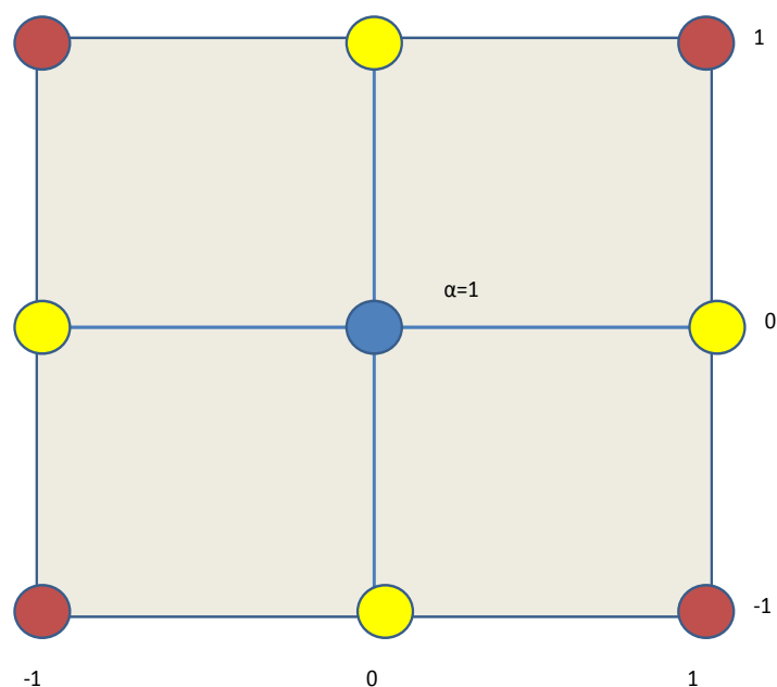
Figure 7.2: Schematic representation of design points for the 3^2 factor FCCCD.
