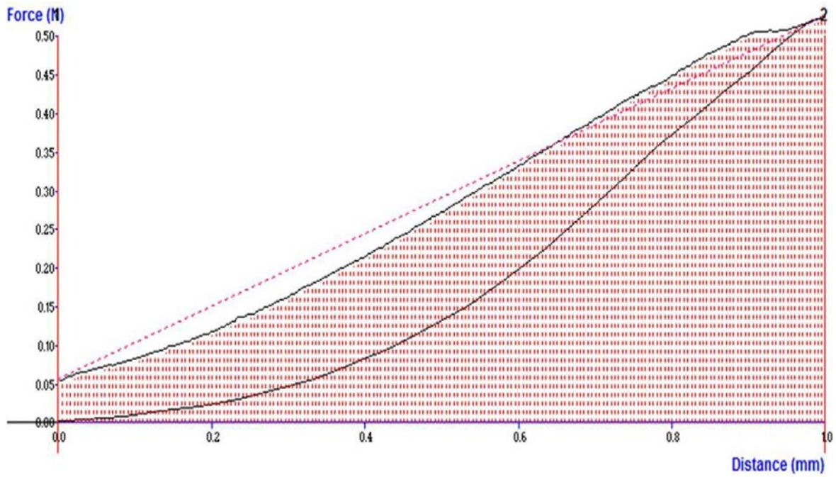
Figure 2.10: Typical Force vs. Distance graph to determine the deformation energy and hardness of SBPs.
