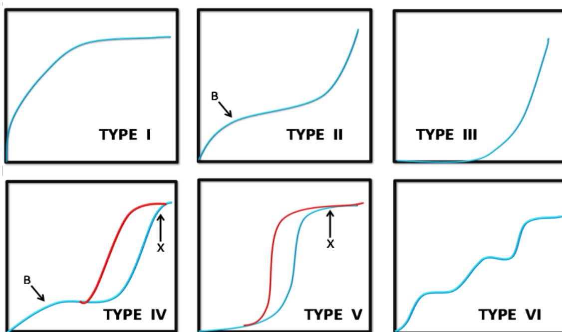
Figure 7.10: IUPAC classification of adsorption isotherms (adapted from Siminiceanu et al. , 2008; Bawa et al. , 2011).
