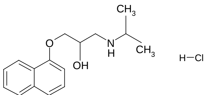
(±) -1-Isopropylamino-3-(1-naphthyloxy)-2-propanol
