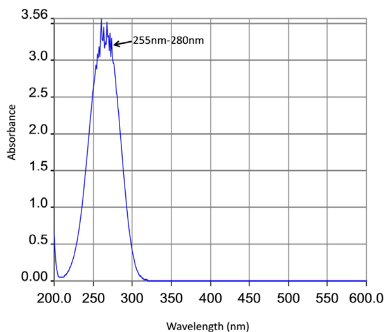
Figure 4.9: UV spectrum of acetone.
