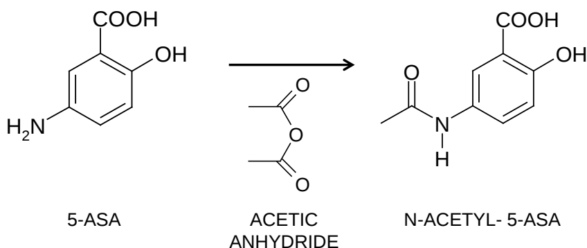
Figure 8.8: Chemical reaction for the synthesis of N-acetyl 5-ASA.
