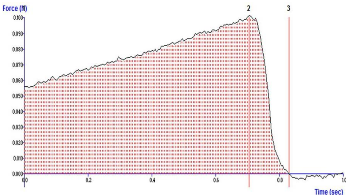
Figure 2.8: Typical Force vs. Time graph to determine the resilience of SBPs.
