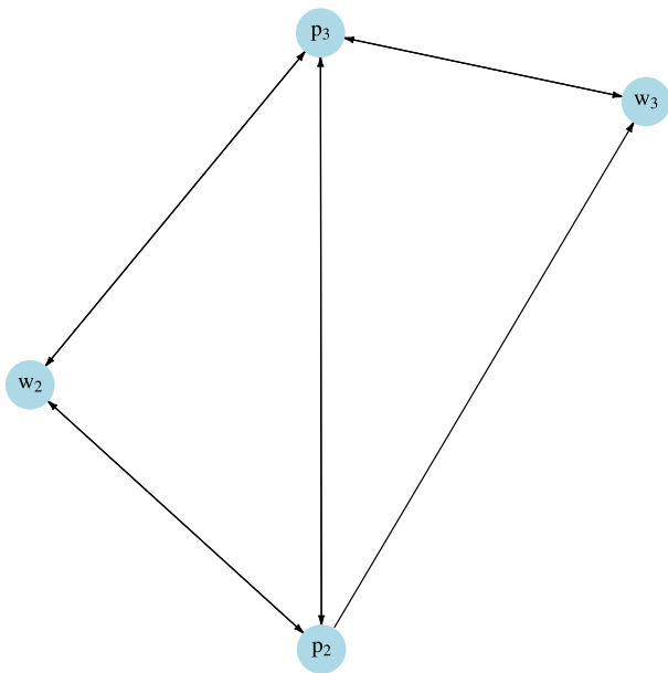
Fig. D.1. Directed Graph of the Jacobian Matrix (D.1).
