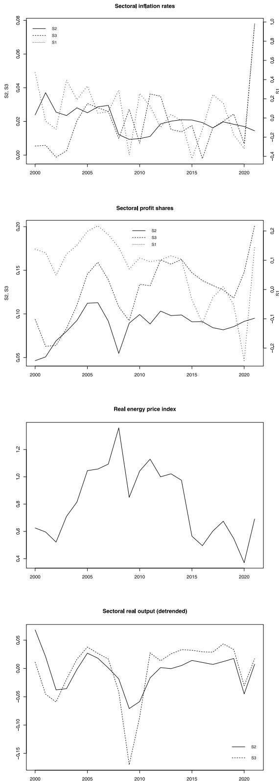
Fig. F.3. Time series used to construct empirical moments.
