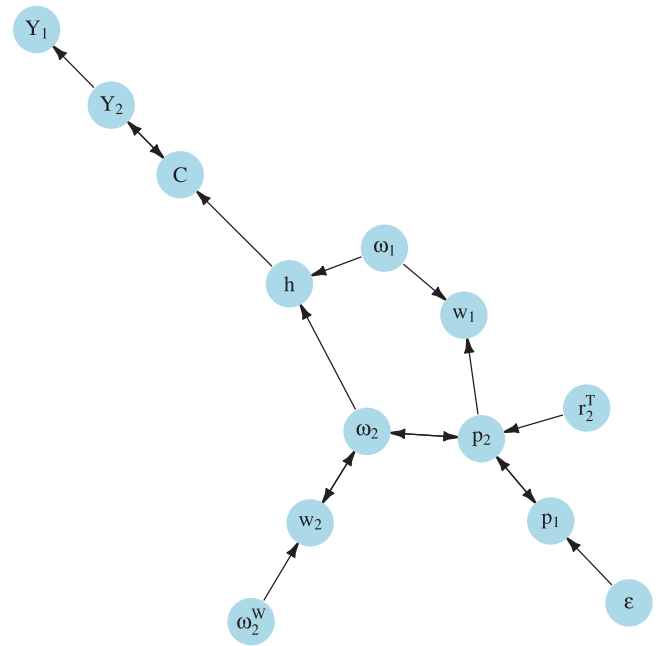
Fig. 2. Directed graph of two-sector model.
