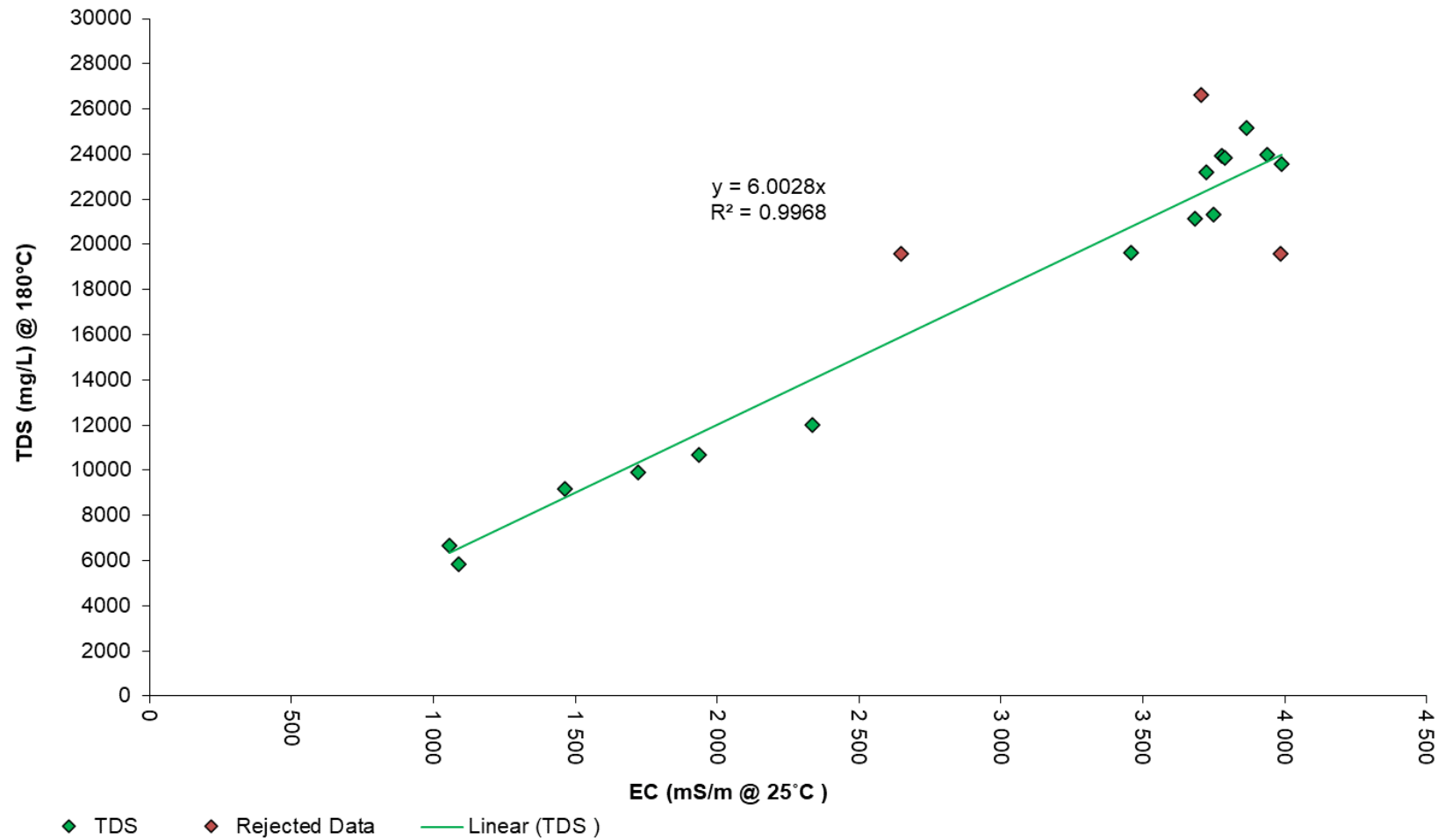
Figure F1.3. Total Dissolved Solids (TDS) vs Electrical Conductivity (EC) - Data pt. 9, 10 & 13 rejected
