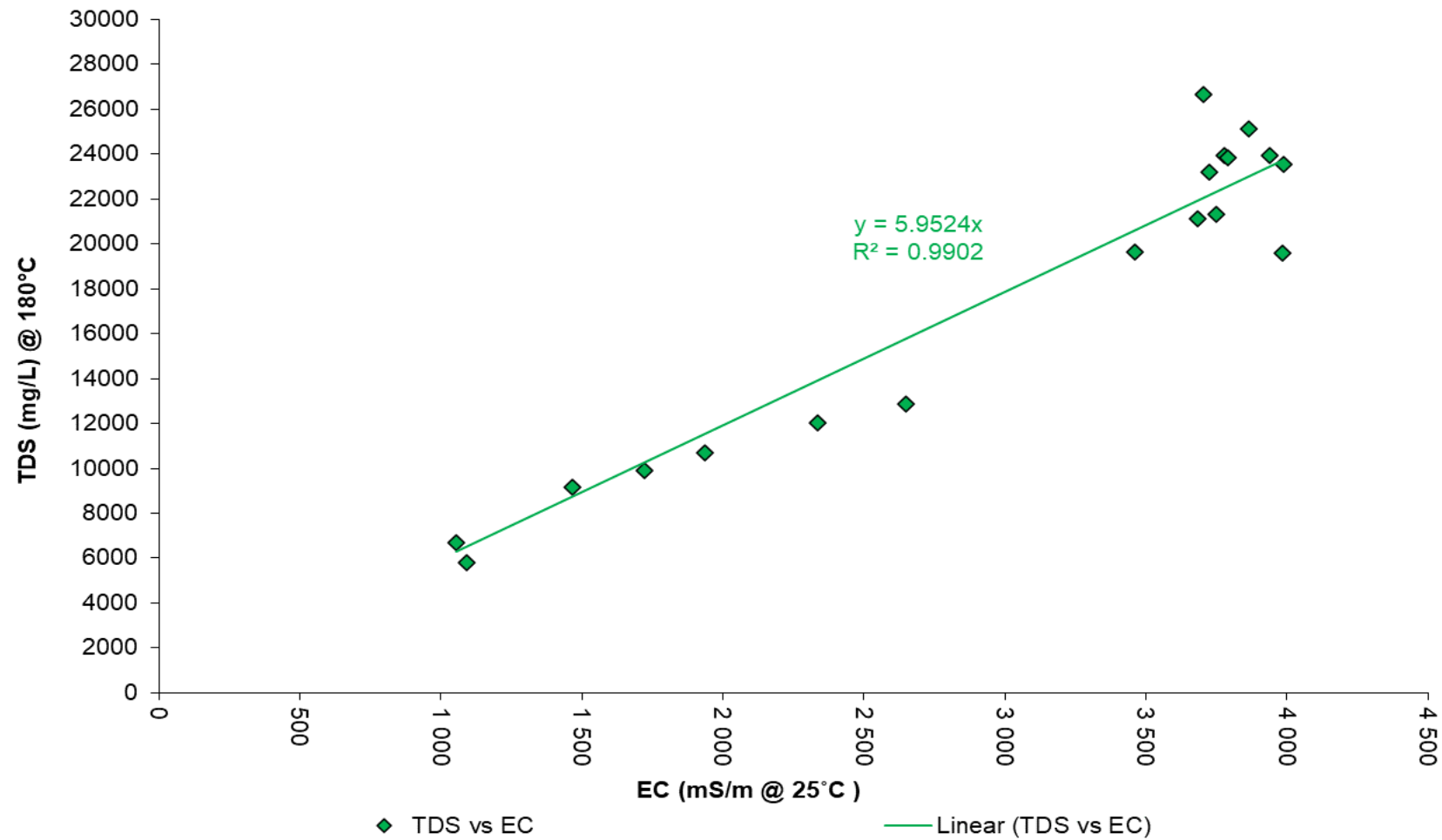
Figure F1.1 Total Dissolved Solids (TDS) vs Electrical Conductivity (EC) - Graphs - All Data
