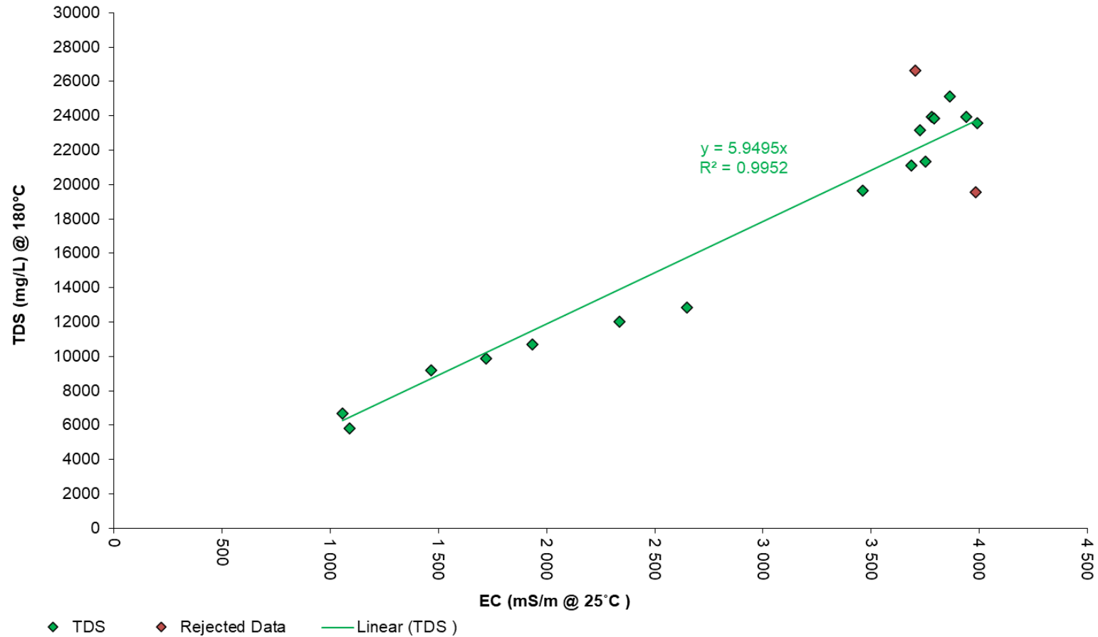
Figure F1.2. Total Dissolved Solids (TDS) vs Electrical Conductivity (EC) - Data pt. 9 & 13 rejected
