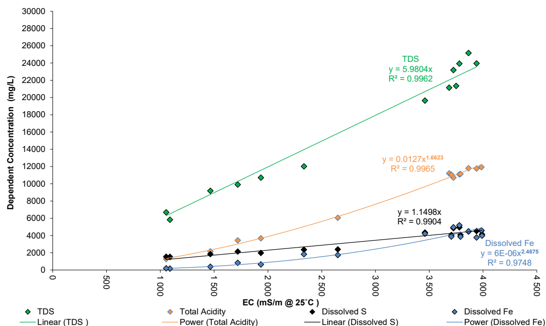
Figure 4.5 Total dissolved solids total acidity, dissolved iron and sulfur as a function of electrical conductivity: Linear regression with the intercept set to zero, and power regression equations after rejection of outliers
