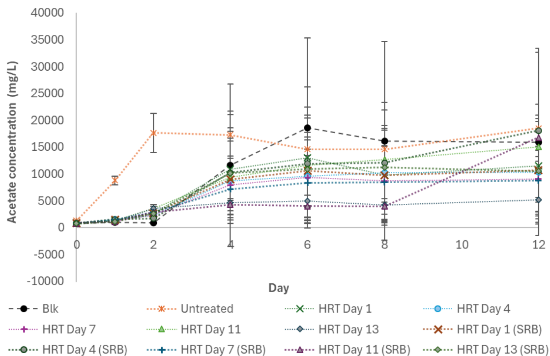
Figure 7.17 Acetate concentrations produced during fermentation of untreated, and pre-treated grass samples, for non- and SRB-amended samples. Error bars represent the standard deviation of duplicate analyses.
