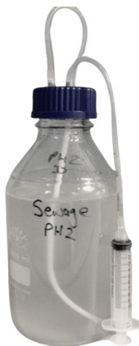
Figure 6.2 Reactor arrangement for experimental work.
