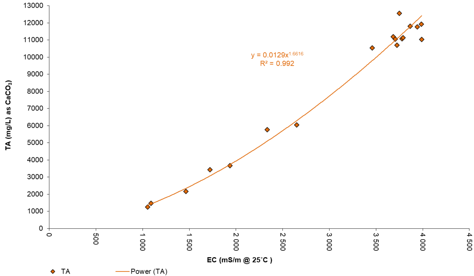
Figure F2.1. Total Acidity (TA) vs Electrical Conductivity (EC) – All Data
