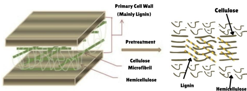
Figure 2.8 Schematic diagram showing the effect of pre-treatment on lignocellulosic biomass. Data from (Tong, Cheng and Pullammanappallil, 2013).
