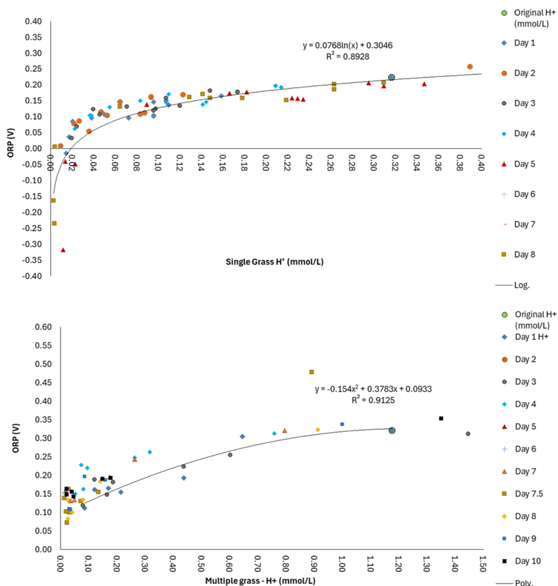
Figure 5.6 Oxidation-reduction potential (ORP) plotted as a function of hydrogen ion concentration ( H^+ ) for single and multiple grass additions
