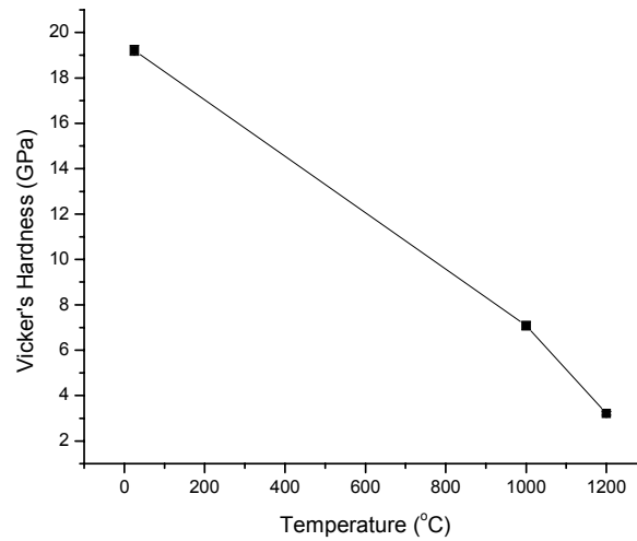
Figure 4.13 Results of the high temperature hardness measurement carried out on the HP3Y5Al material
