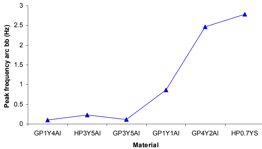
Figure 4.30 Peak frequency for the 2 nd , lower frequency arc observed in the GPS and HP3Y5AI and HP0.7YS materials at 200°C
