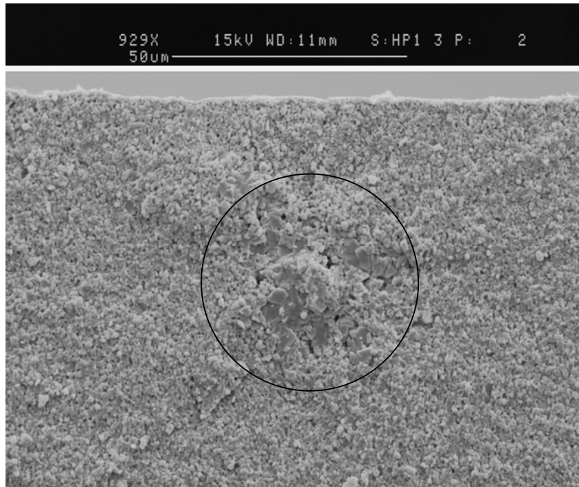
Figure 4.15 SEM micrograph showing origin of failure in HP3Y5Al material. EDS analysis of the marked larger grains, confirmed the presence of iron impurities (in dark region in circle)
