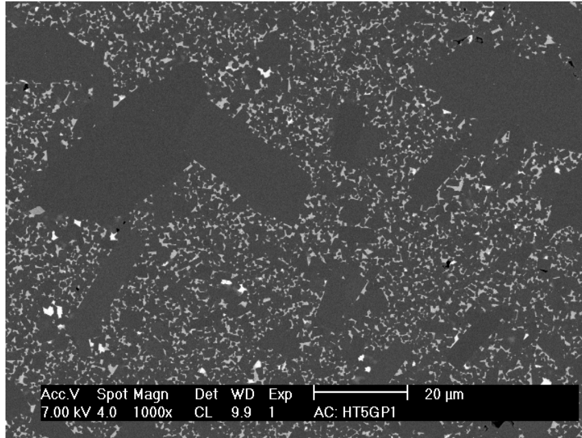
Figure 4.9 FESEM micrograph of HT5GP3Y5Al material
