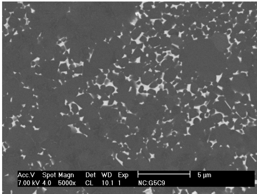
Figure 4.3 FESEM micrograph of GP1Y4Al material
