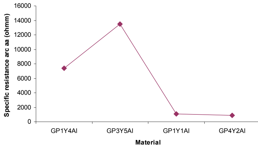
Figure 4.26 Specific resistance (resistivity) results of the 1 st , higher frequency arc observed in the GPS materials at 200°C
