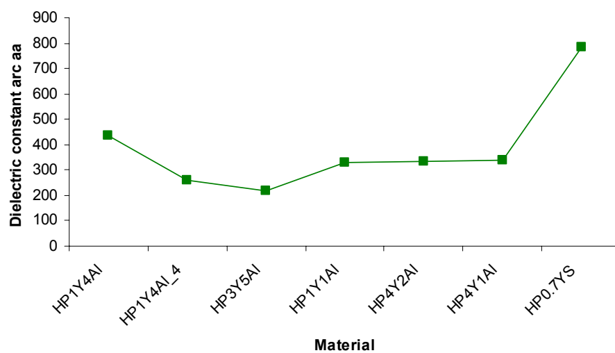
Figure 4.31 Dielectric constant results for the 1 st , higher frequency arc in the HP materials
