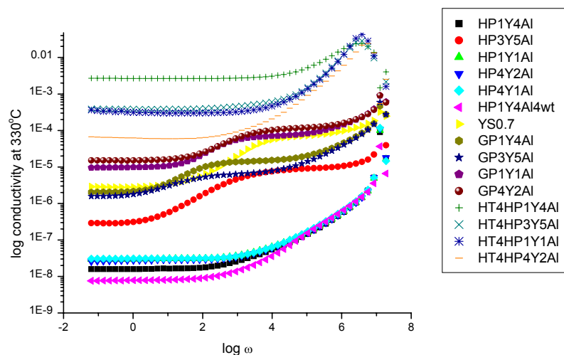
Figure 4.18 Graph of the log of electrical conductivity as a function of the log of angular frequency at 330°C
