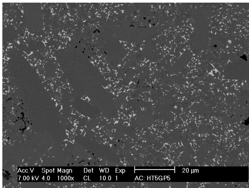
Figure 4.5 FESEM micrograph of HT5GP1Y4Al material
