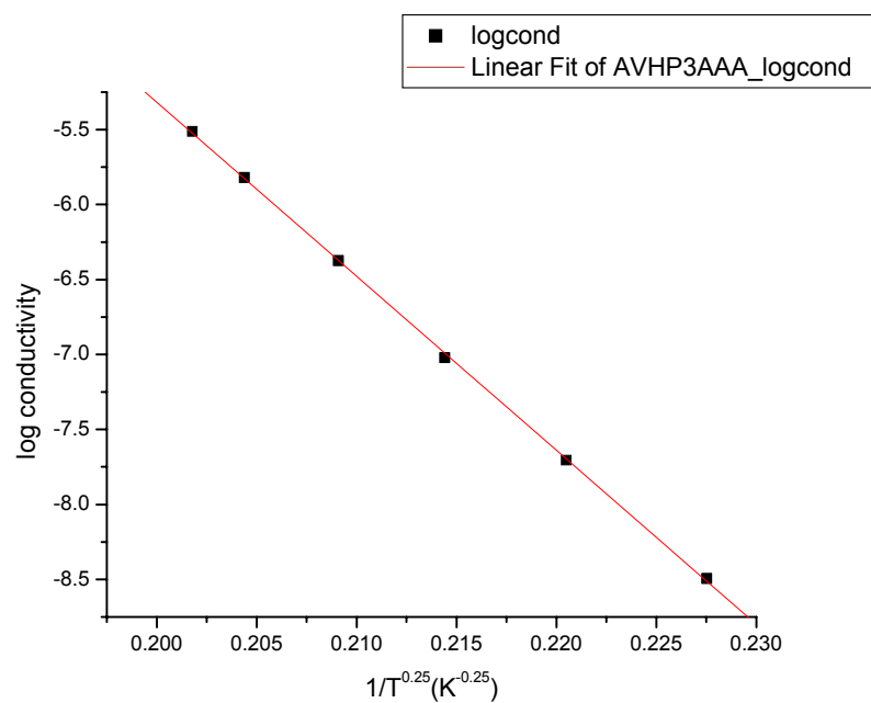
Figure 4.24 Plot of log conductivity vs 1/T^{0.25} , to show the best fit for the temperature dependence of HP1Y1Al
