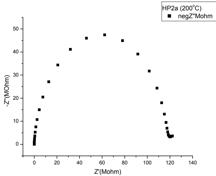
Figure 4.19 Cole- Cole plot of HP4Y2Al material at 200°C
