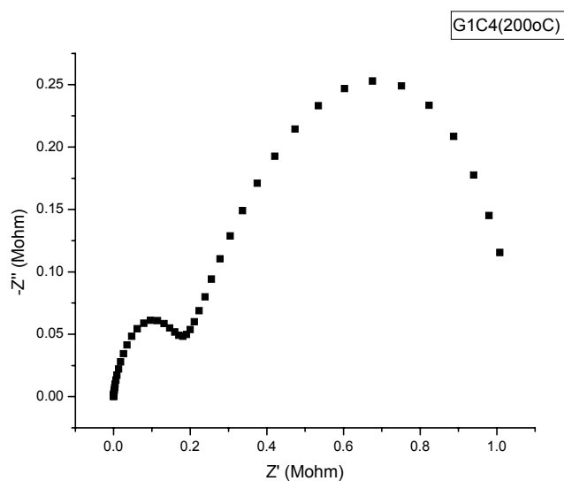
Figure 4.21 Cole-Cole plot of GP3Y5Al material at 200°C
