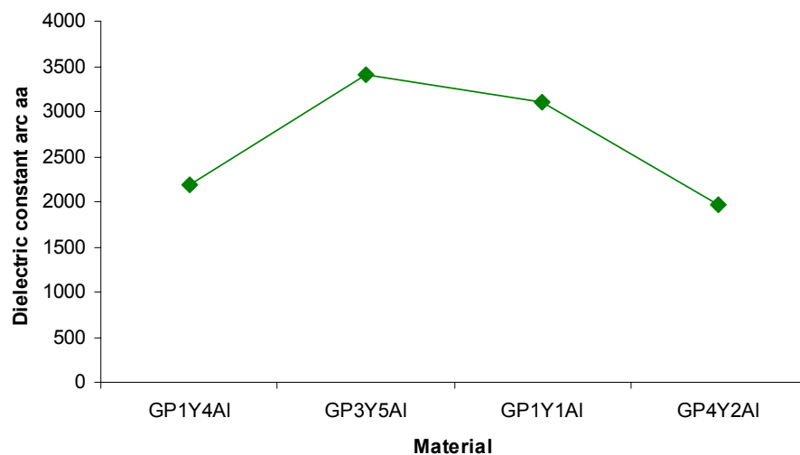
Figure 4.32 Dielectric constant results for the 1 st , higher frequency arc in the GPS materials
