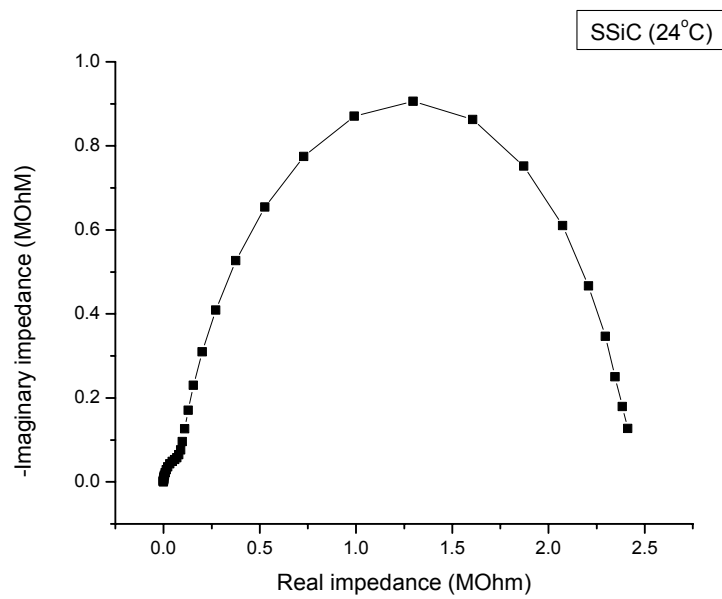
Figure 4.35 Cole-Cole plot for the SSiC material at room temperature
