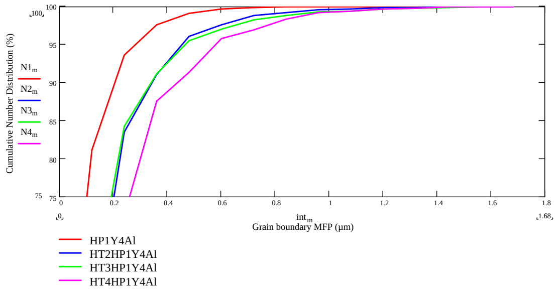
Figure 4.12 Grain boundary mean free path number distribution during HT for the HP1Y4Al material
