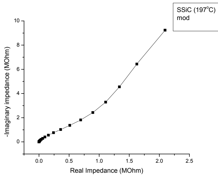
Figure 4.36 Cole-Cole plot for the SSiC material at liquid nitrogen temperature (-196°C)
