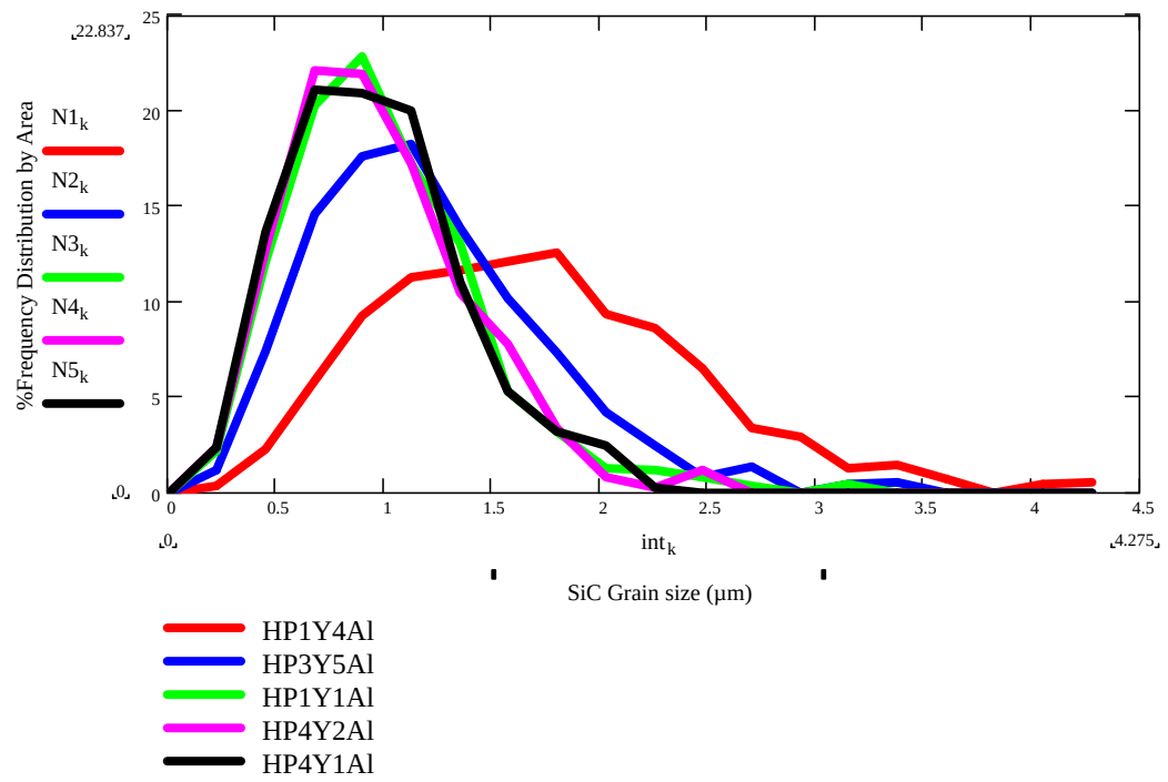
Figure 4.10 Silicon carbide grain size distributions for the HP materials
