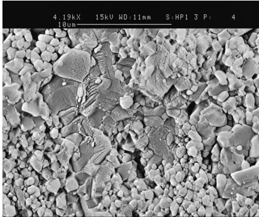
Figure 4.16 SEM micrograph showing the origin in failure (iron impurities), as shown in Figure 4.15, at a higher magnification
