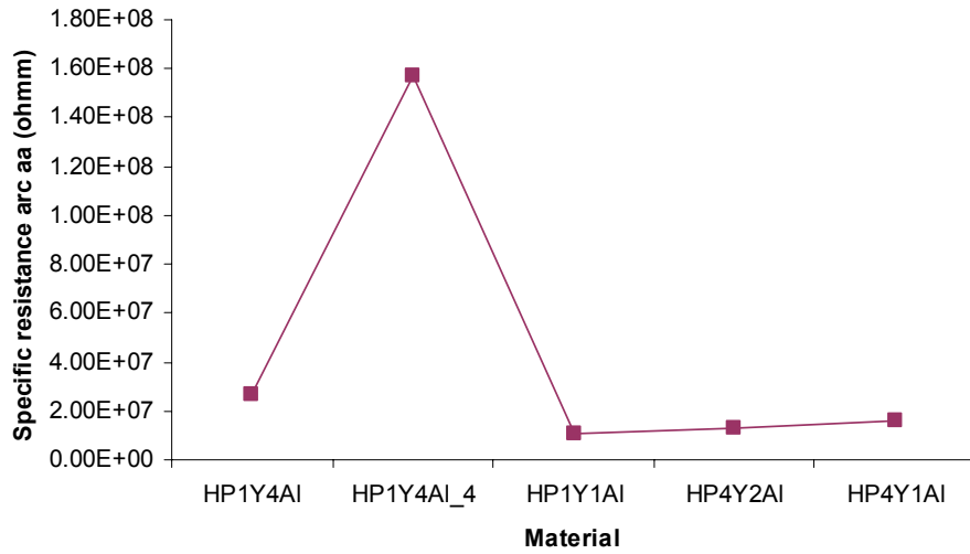
Figure 4.25 Specific resistance (resistivity) results of the only arc observed in the HP materials at 200°C
