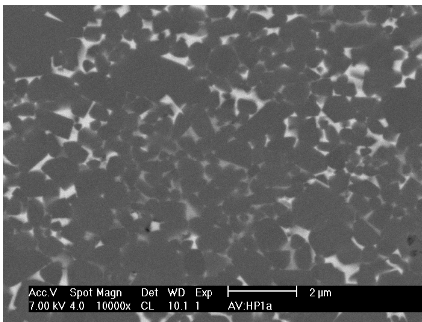
Figure 4.6 FESEM micrograph of HP3Y5Al material
