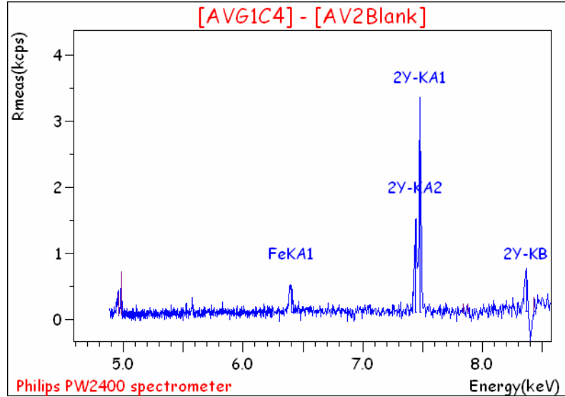
Figure 4.1 Part of XRF scan to show the presence of traces of Fe impurity in the GP3Y5Al material
