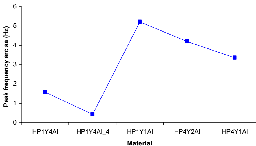
Figure 4.28 Peak frequency of the only arc observed for most of the hot pressed materials at 200°C
