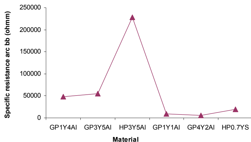
Figure 4.27 Specific resistance (resistivity) results of the 2 nd , lower frequency arc observed in the GPS materials at 200°C
