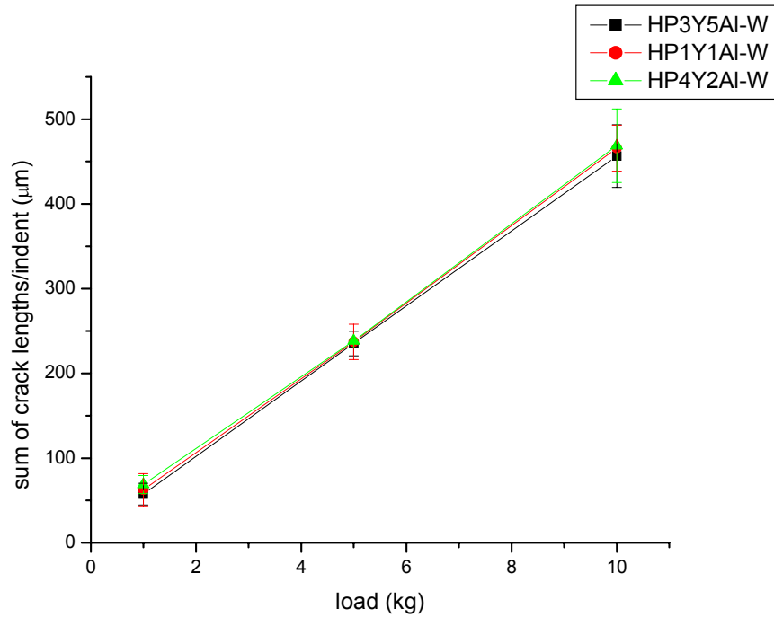
Figure 4.14 Graph showing the crack resistance of HP-W materials (on cross-section of material)
