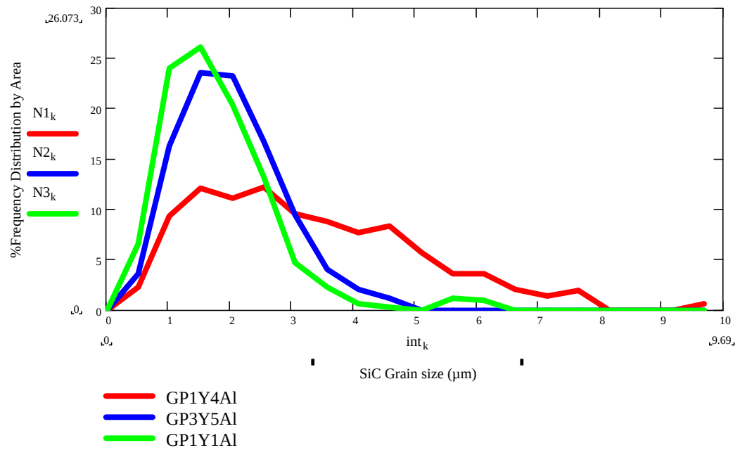
Figure 4.11 Silicon carbide grain size distributions for the GPS materials
