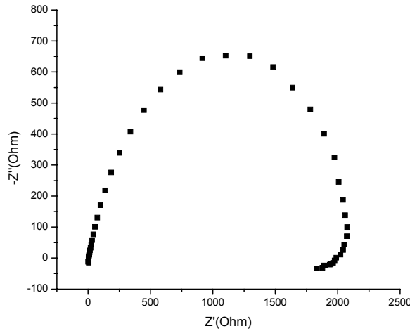
Figure 4.22 Cole-Cole plot of HT4HP4Y2Al at 330°C
