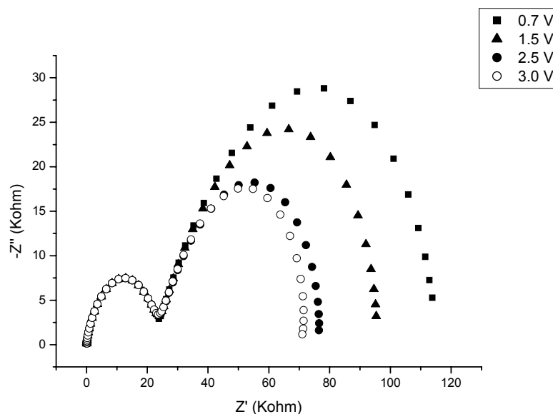
Figure 4.34 Cole-Cole plot of GP3Y5Al material at 330°C showing the non-Ohmic behaviour in the higher resistance phase (Novacontrol)
