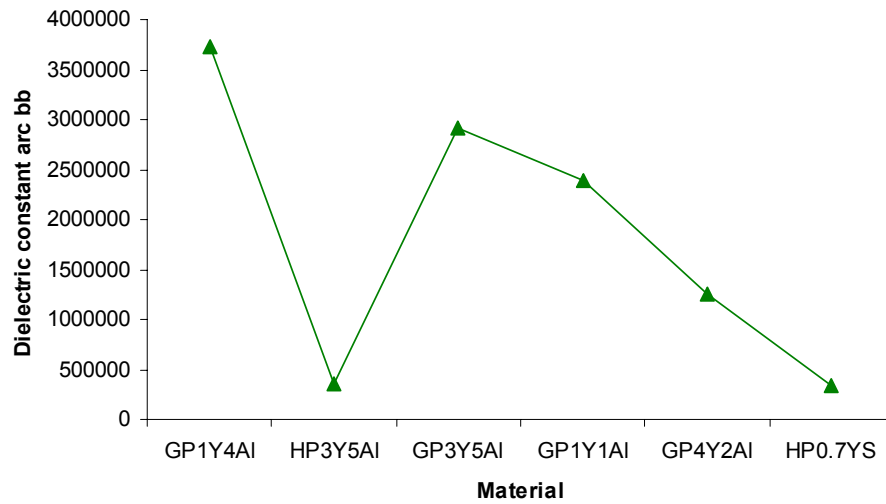
Figure 4.33 Dielectric constant results for the 2nd (lower frequency) arc in the GPS materials
