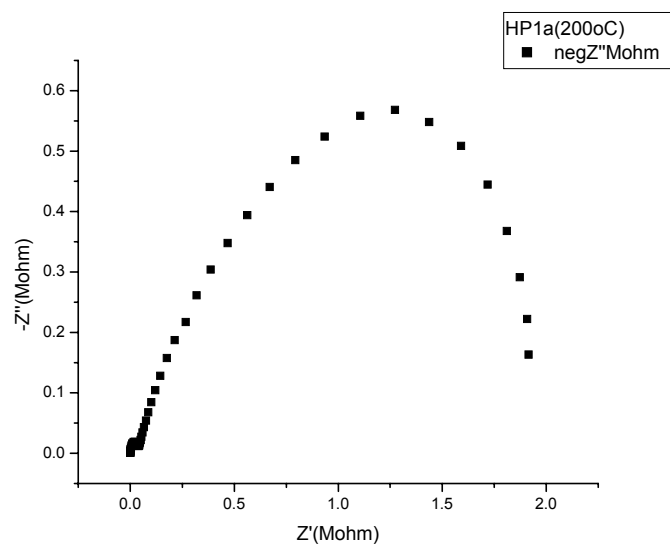
Figure 4.20 Cole –Cole plot of HP3Y5Al material at 200°C
