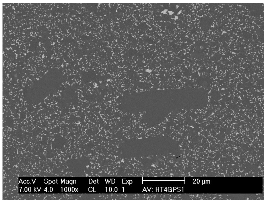
Figure 4.8 FESEM micrograph of HT4GP3Y5Al material
