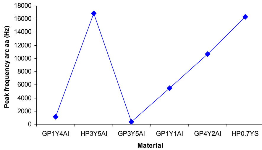
Figure 4.29 Peak frequency of the 1 st , higher frequency arc for GPS and HP3Y5AI materials at 200°C
