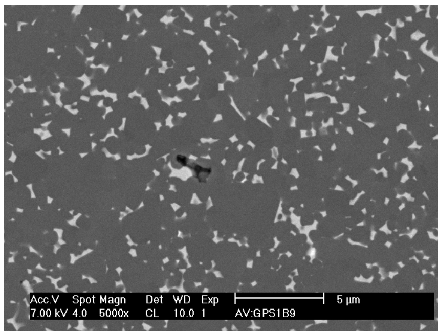
Figure 4.7 FESEM micrograph of GP3Y5Al material
