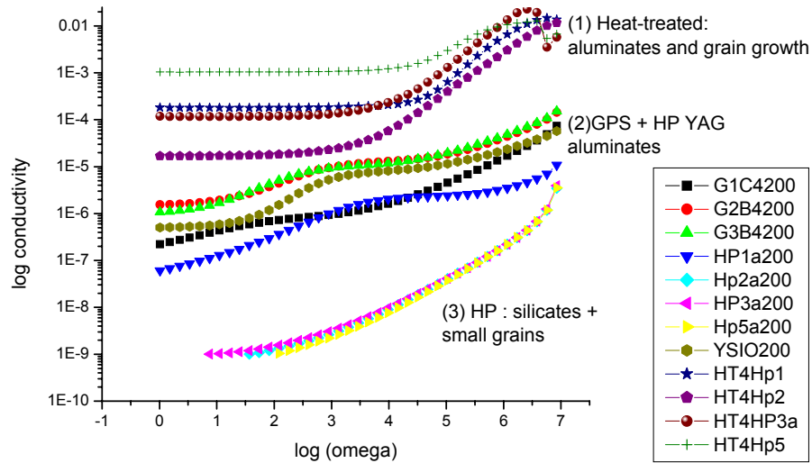
Figure 4.17 Graph of the log of electrical conductivity as a function of the log of angular frequency at 200^{\circ}\text{C} . In the labels 1 = 3Y5Al, 2 = 4Y2Al, 3= 1Y1Al, 4 = 4Y1Al, 5 = 1Y4Al
