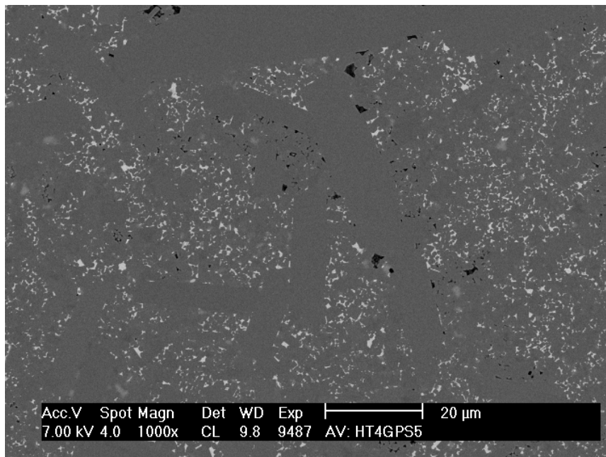
Figure 4.4 FESEM micrograph of HT4GP1Y4Al material
