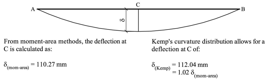
Deflected Shape
