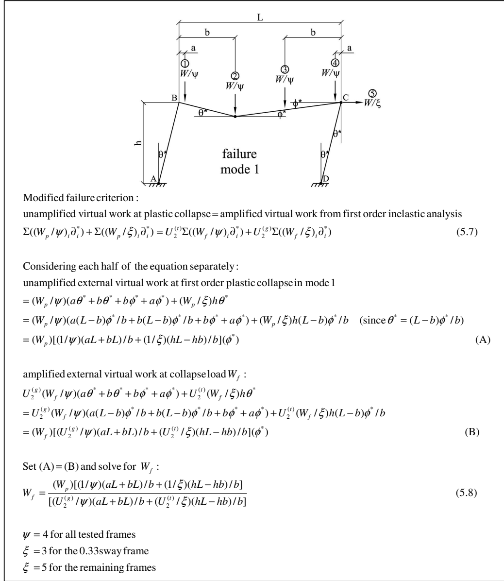
Fig. [5.7] Derivation of the modified failure criterion
