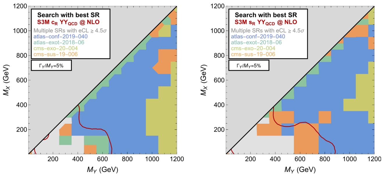
Fig. 6 Search including the most sensitive signal region for the new physics signal emerging from the YY_{\text{QCD}} processes at NLO, for the \text{S3M}_{\text{cR}} (left) and \text{S3M}_{\text{sR}} (right) models with a fixed width-to-mass ratio. The 95% CL exclusion limit is also reported
