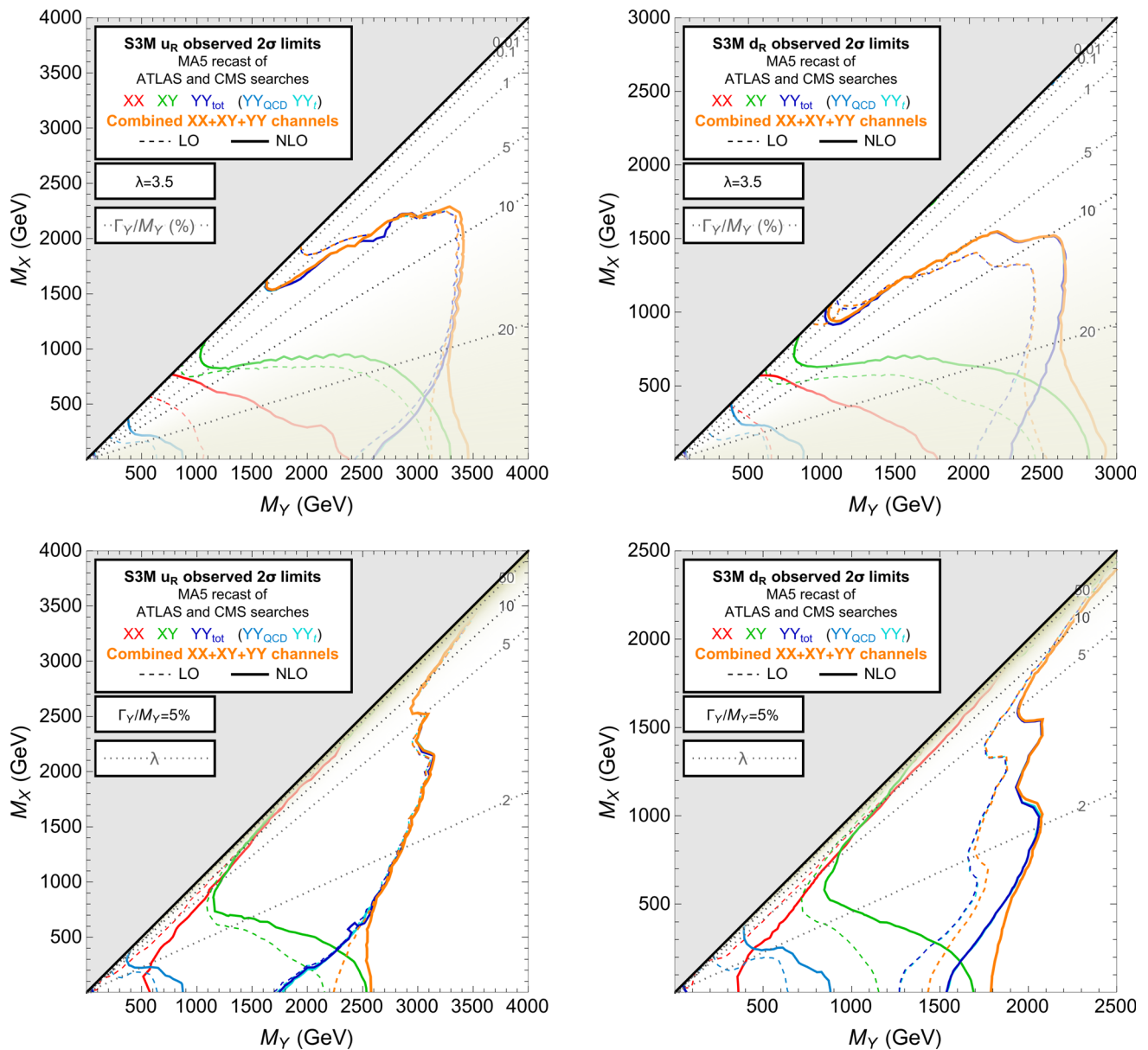
Fig. 1 Exclusion limits at 95% confidence level from the reinterpretation of several Run 2 ATLAS and CMS searches [133–137]. The results are shown for the S3M uR (left) and S3M dR (right) real dark matter scenarios described in Sect. 2.1, considering two configurations: \lambda = 3.5 (top row) and \Gamma_Y/M_Y = 0.05 (bottom row). For scenarios with \lambda = 3.5 , dotted grey lines represent isolines of constant \Gamma_Y/M_Y value. Conversely, for scenarios with \Gamma_Y/M_Y = 0.05 , these lines correspond to isolines of fixed \lambda value. Individual contributions to the
