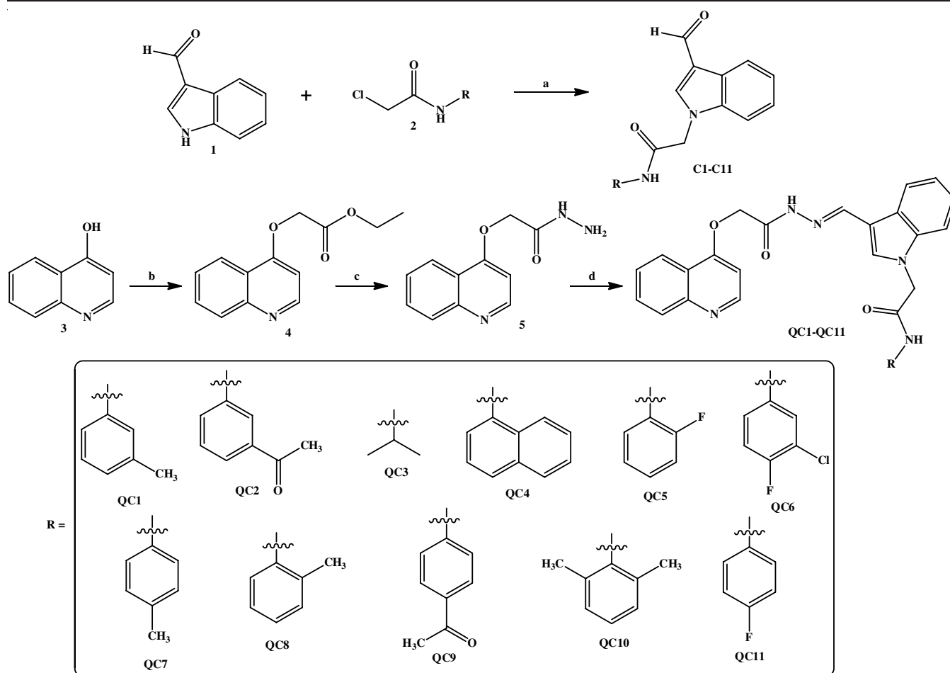
Scheme-I: Synthesis of substituted indole-3-carboxaldehyde ( C1-C11 ) and 2-(3-((2-(quinoline-4-yloxy)acetyl)hydrazineylidene)methyl)-1H-indol-1-yl)acetamide derivatives ( QC1-QC11 ); Reagents and conditions: (a) K_2CO_3 , cat. KI, DMF, reflux, (b) ethylacetoacetate, EtOH, (c) N_2H_4 \cdot xH_2O , EtOH, reflux, (d) substituted indole-3-carboxaldehyde ( C1-C11 ), EtOH, 1-2 drops H_2SO_4
