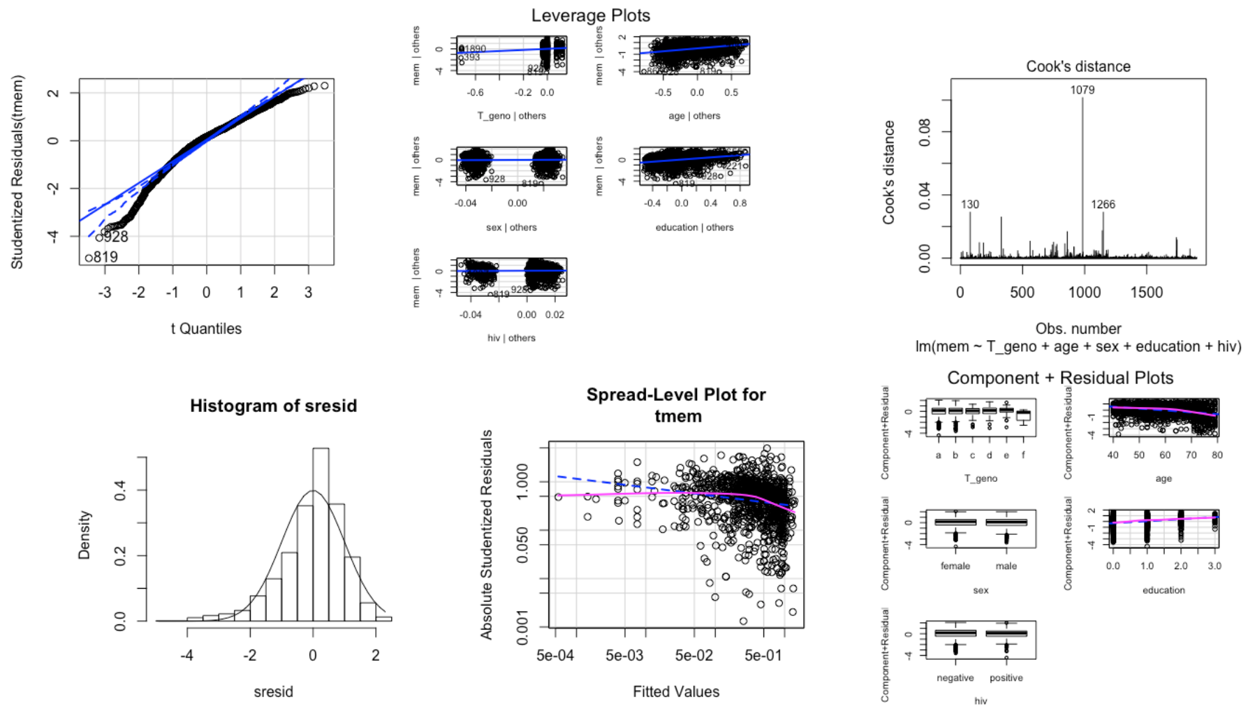
Figure A.4.11: Diagnostic regression plots for the residuals of episodic memory
