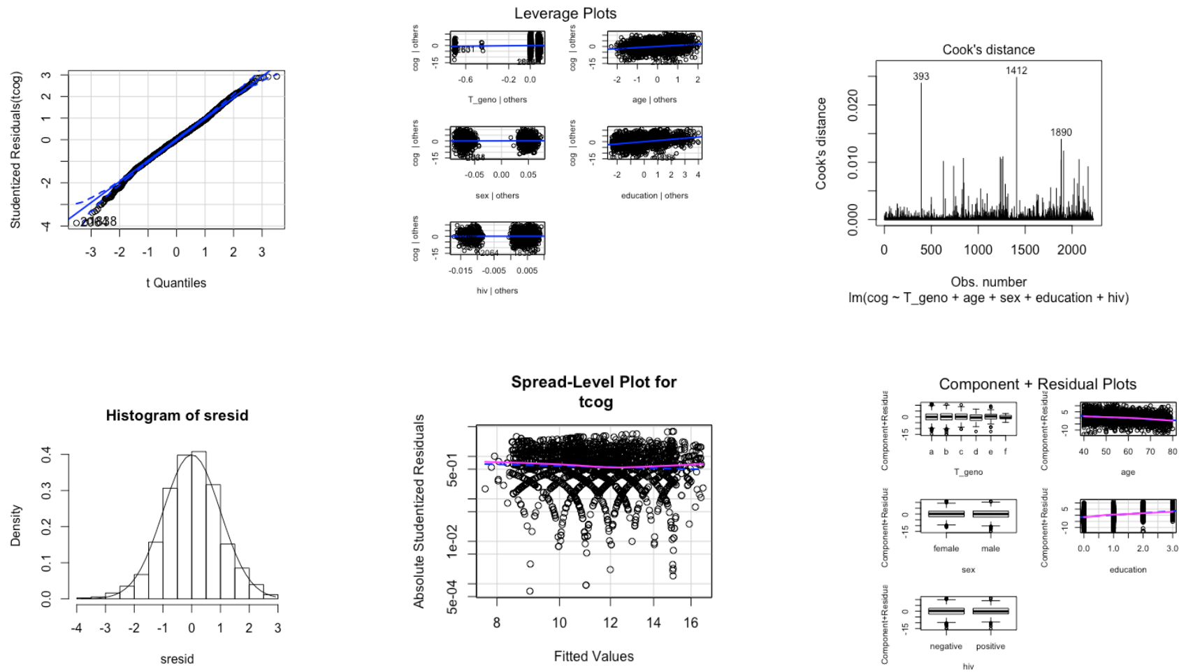
Figure A.4.8: Diagnostic regression plots for the residuals of total cognition score
