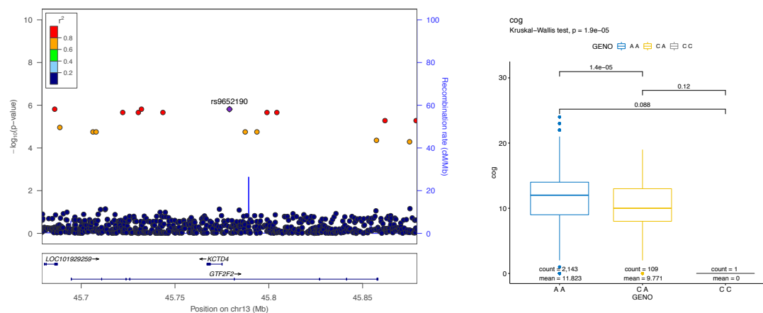
Figure A3.5: rs9652190 on chromosome 13 associated with total cognition score
