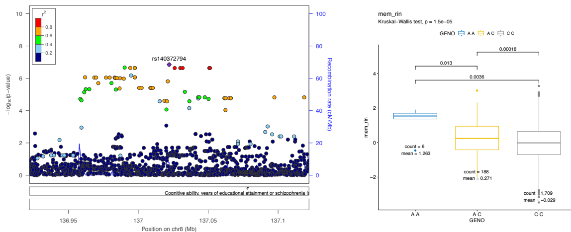
Figure A3.6: rs140372794 on chromosome 8 associated with episodic memory
