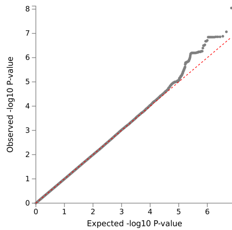
Figure 3.2: Genome-wide and suggestive associations for verbal episodic memory
