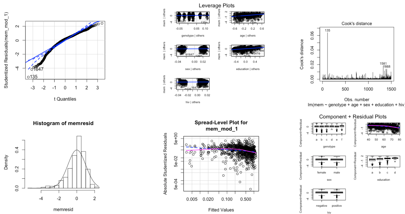
Figure A.2.5: Diagnostic regression plots for the residuals of verbal episodic memory
