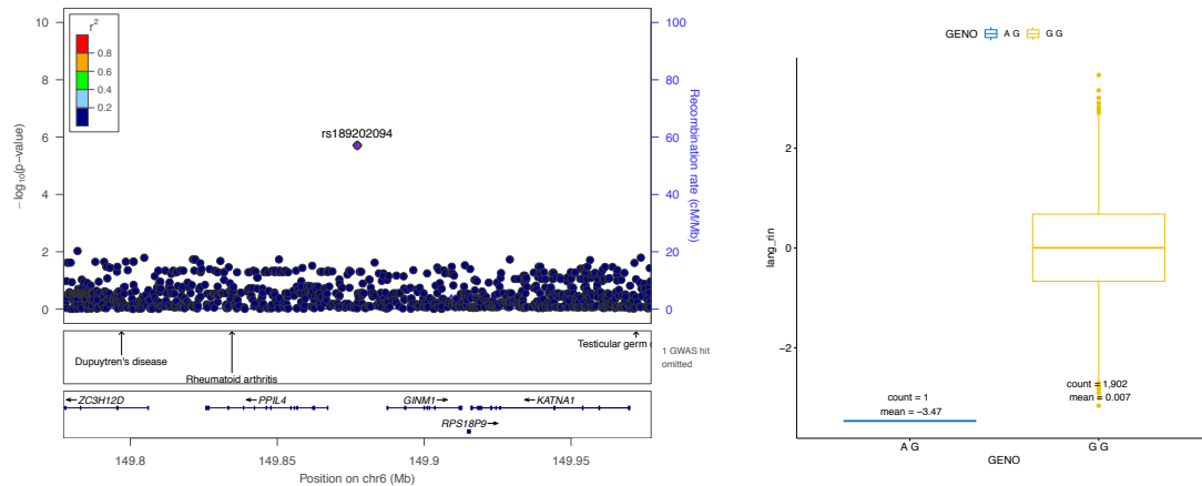
Figure A3.18: rs189202094 on chromosome 6 associated with language
