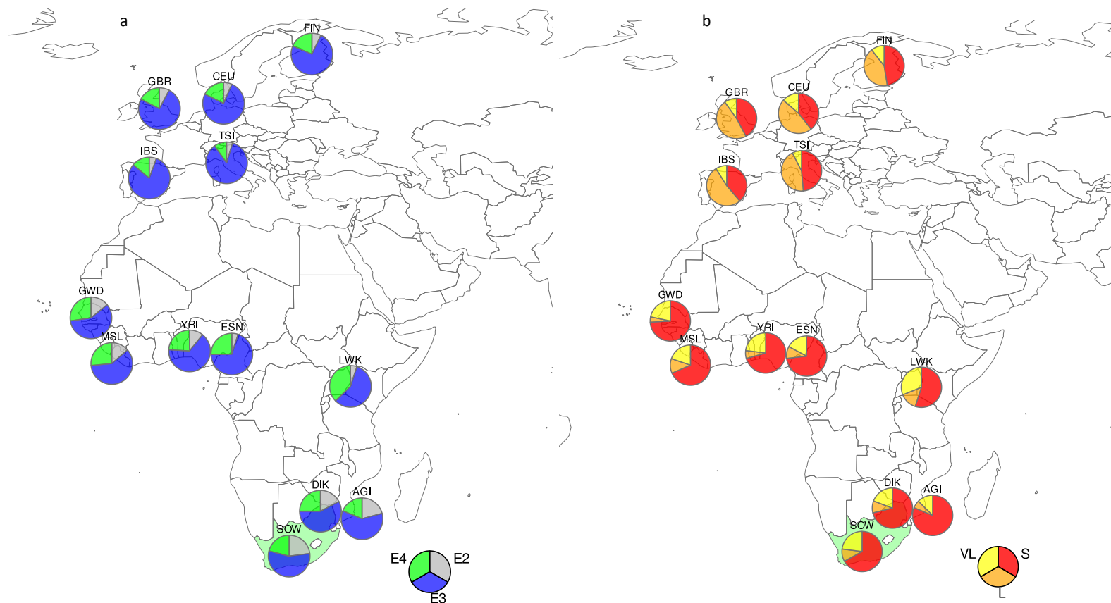
Figure 4.4: Allele distribution of APOE and TOMM40 poly-T length polymorphism in Africans vs Europeans
