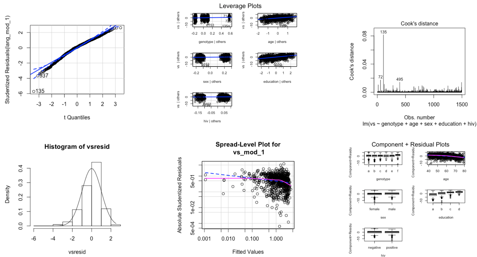
Figure A.2.6: Diagnostic regression plots for the residuals of visuospatial ability
