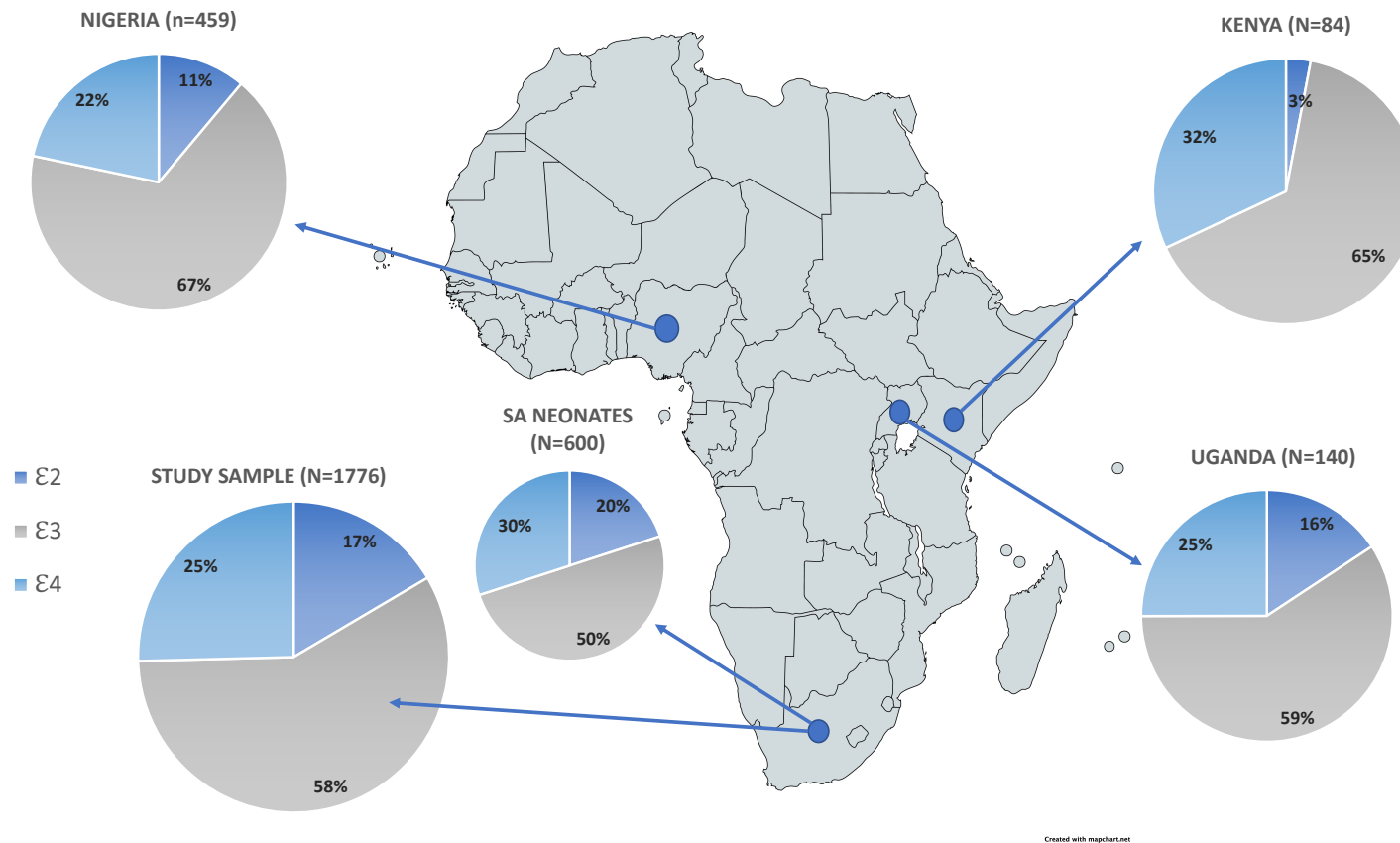
Figure 2.2: Comparison of APOE allele frequency distributions from four African studies, showing sample size for each study
