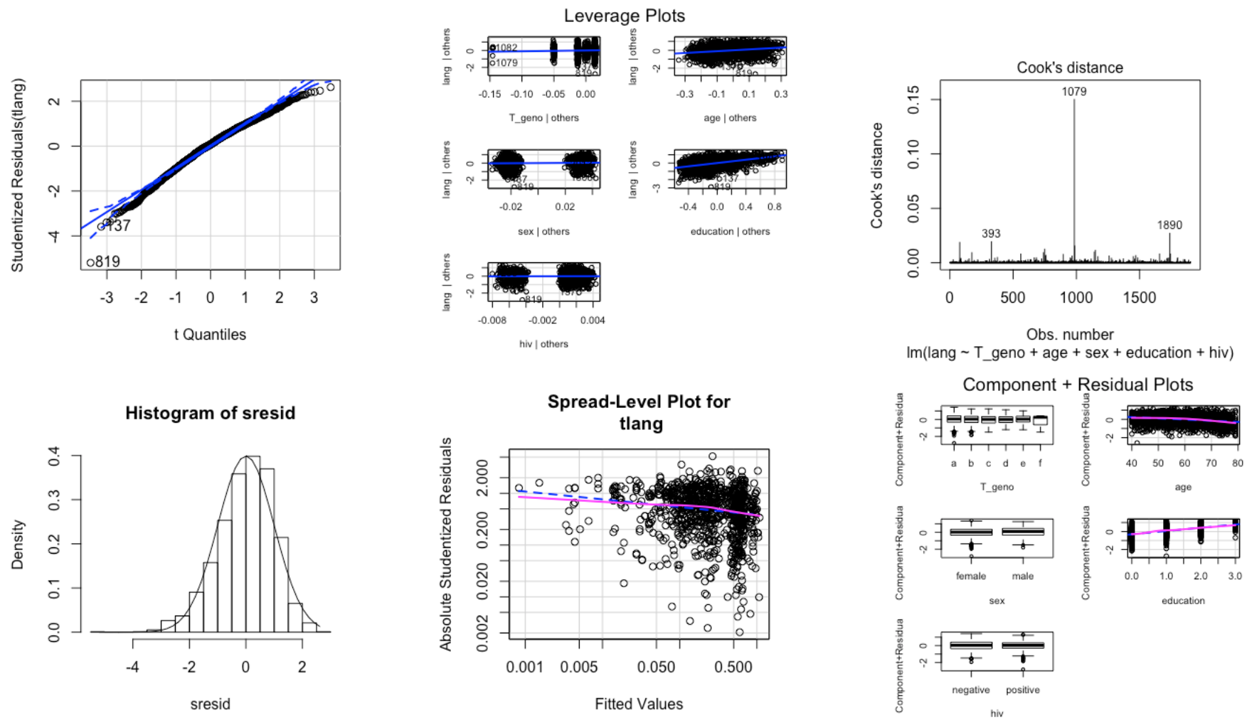
Figure A.4.10: Diagnostic regression plots for the residuals of language
