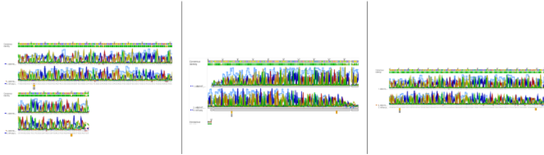
Figure A.2.1: Electrophoretograms for APOE for 27 samples that were successfully sequenced
