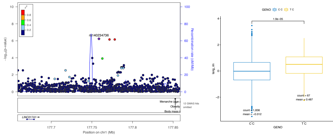
Figure A3.13: rs140234736 on chromosome 1 associated with language
