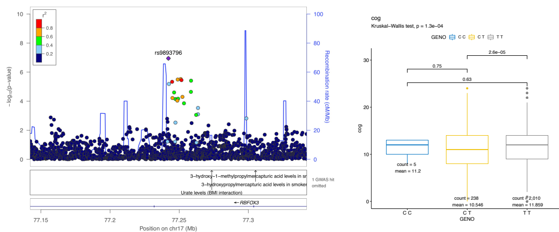
Figure A3.1: rs9893796 on chromosome 17 associated with total cognition score
