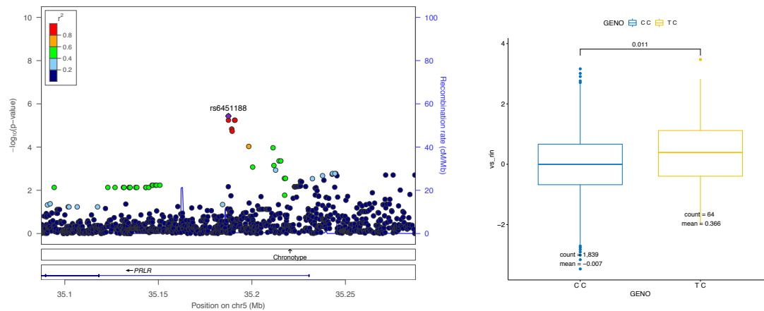
Figure A3.28: rs6451188 on chromosome 5 associated with visuospatial ability
