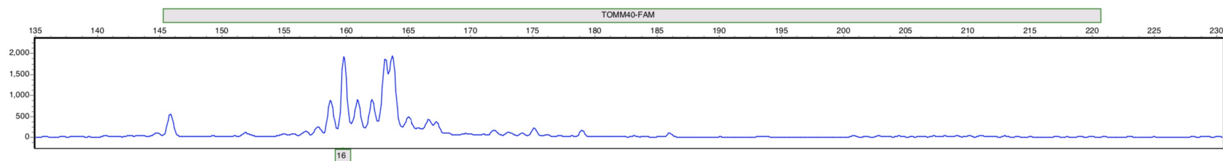
Figure A4.5 Allele report from fragment analysis from PCR fragment analysis for AB0009
