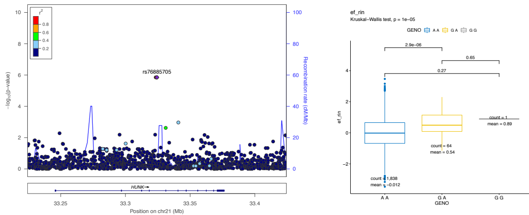
Figure A3.11: rs76885705 on chromosome 21 associated with executive function
