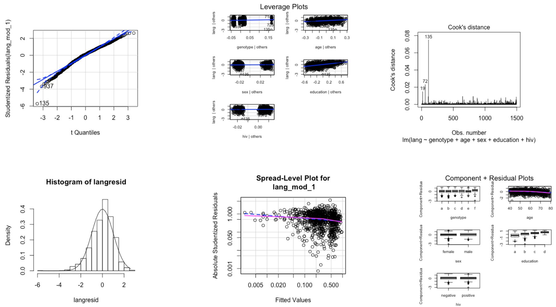
Figure A.2.4: Diagnostic regression plots for the residuals of language
