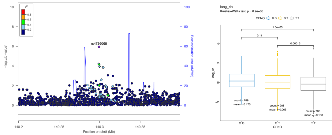
Figure A3.15: rs4736068 on chromosome 8 associated with language
