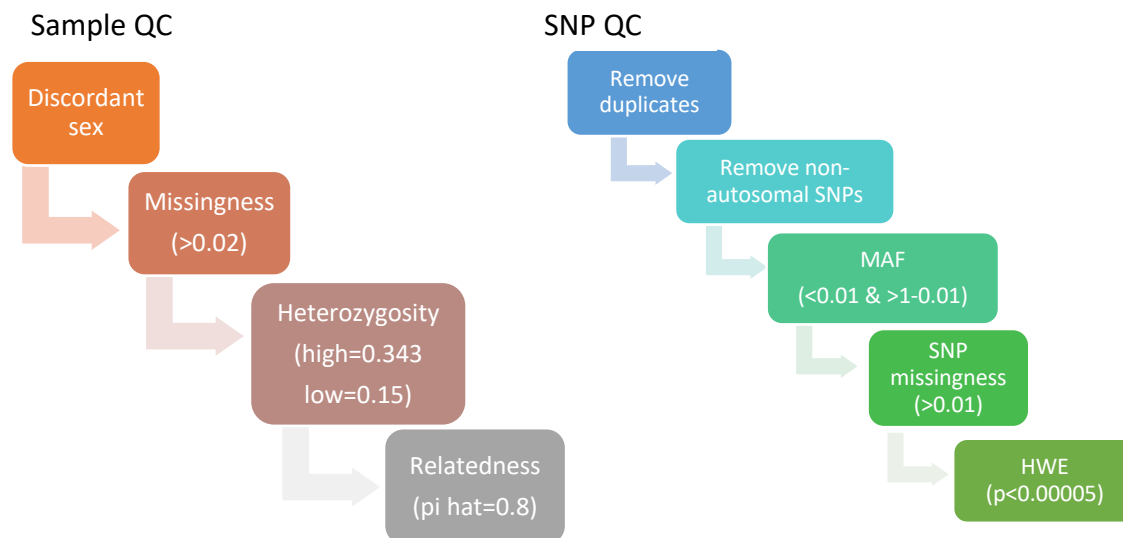
Figure 1.4: Stepwise GWAS QC process for automated pipeline
