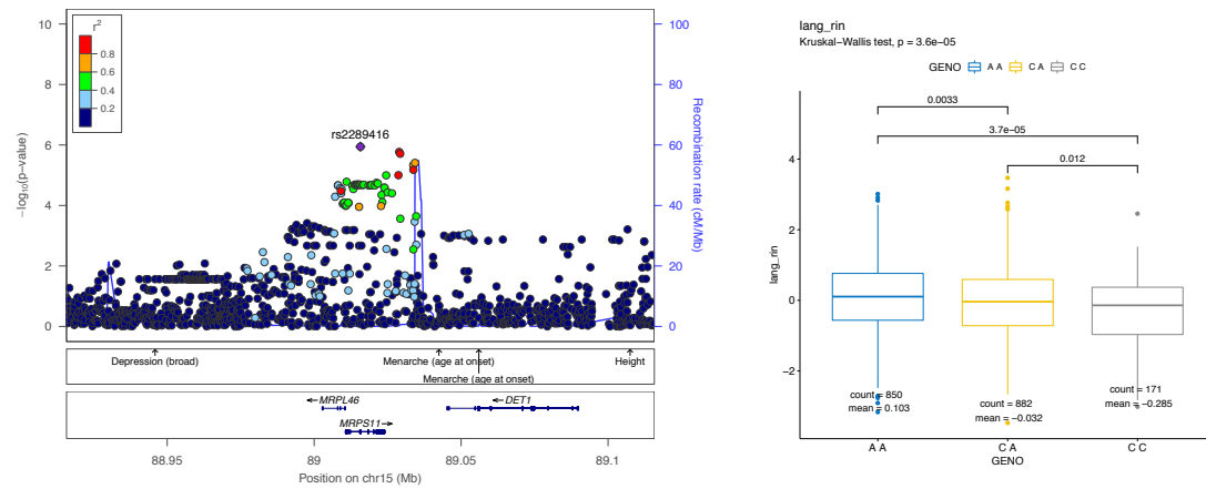
Figure A3.16: rs2289416 on chromosome 15 associated with language
