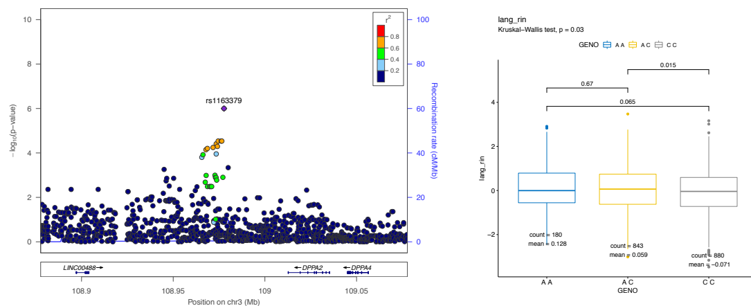
Figure A3.14: rs1163379 on chromosome 3 associated with language
