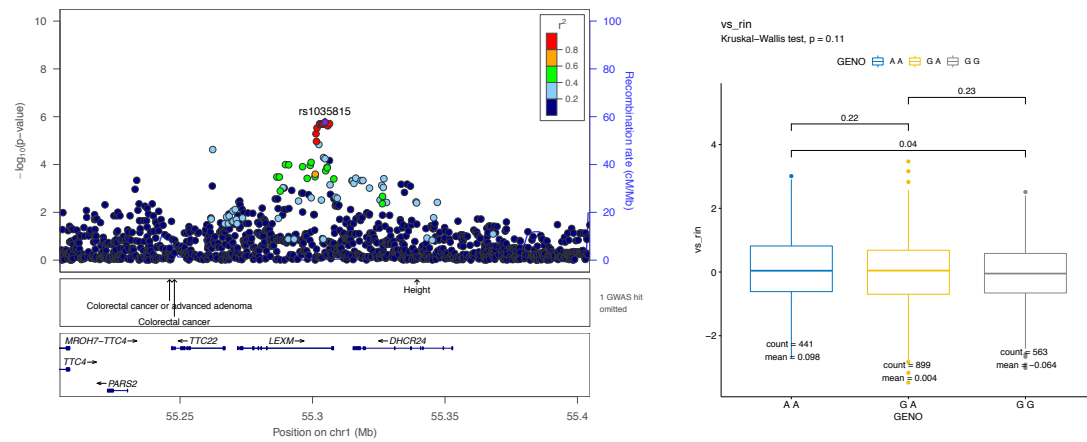
Figure A3.23: rs1035815 on chromosome 1 associated with visuospatial ability
