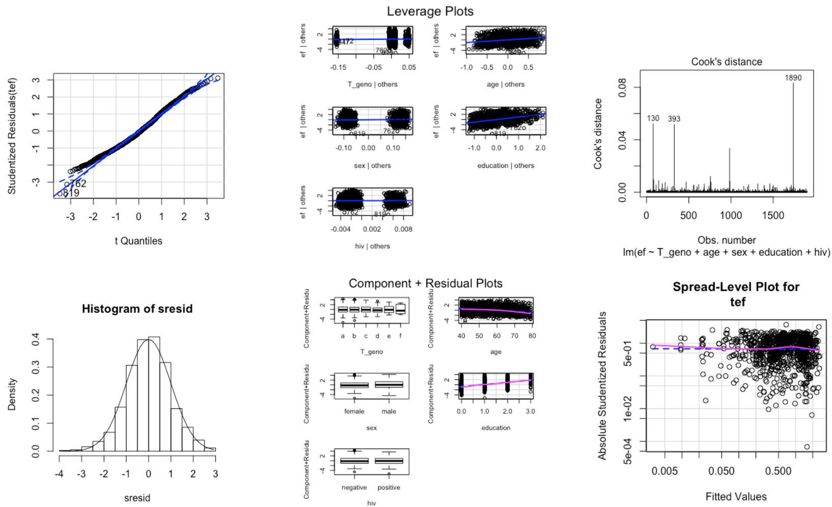
Figure A.4.9: Diagnostic regression plots for the residuals of executive function
