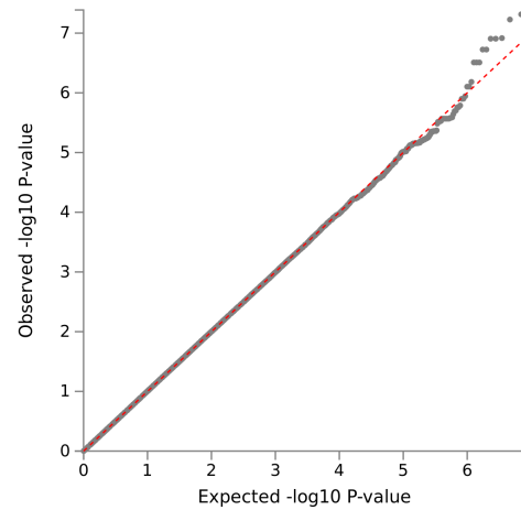
Figure 3.3: Genome-wide and suggestive associations for language
