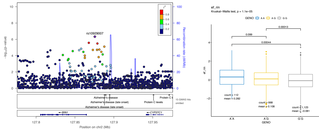
Figure A3.7: rs10929007 on chromosome 2 associated with executive function
