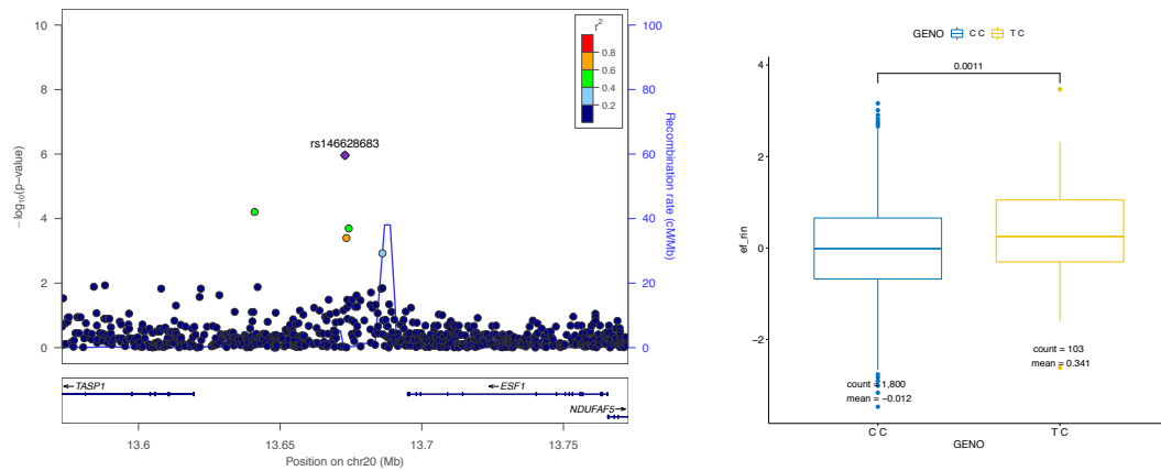
Figure A3.10: rs146628683 on chromosome 20 associated with executive function
