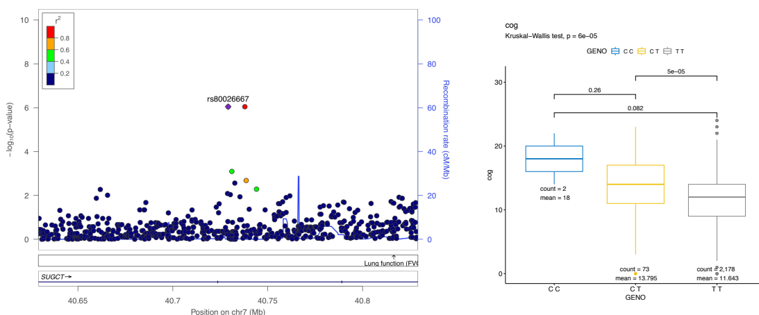
Figure A3.2: rs80026667 on chromosome 7 associated with total cognition score
