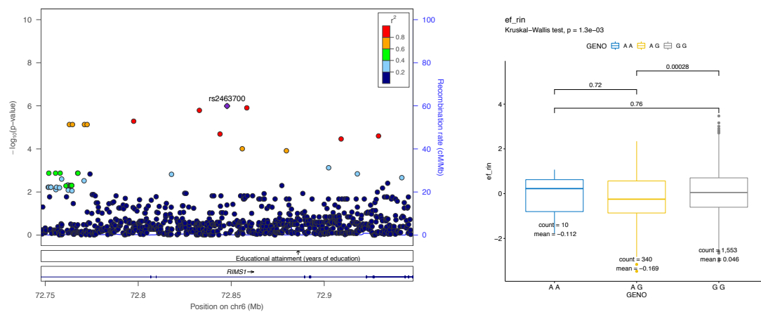
Figure A3.9: rs2463700 on chromosome 6 associated with executive function
