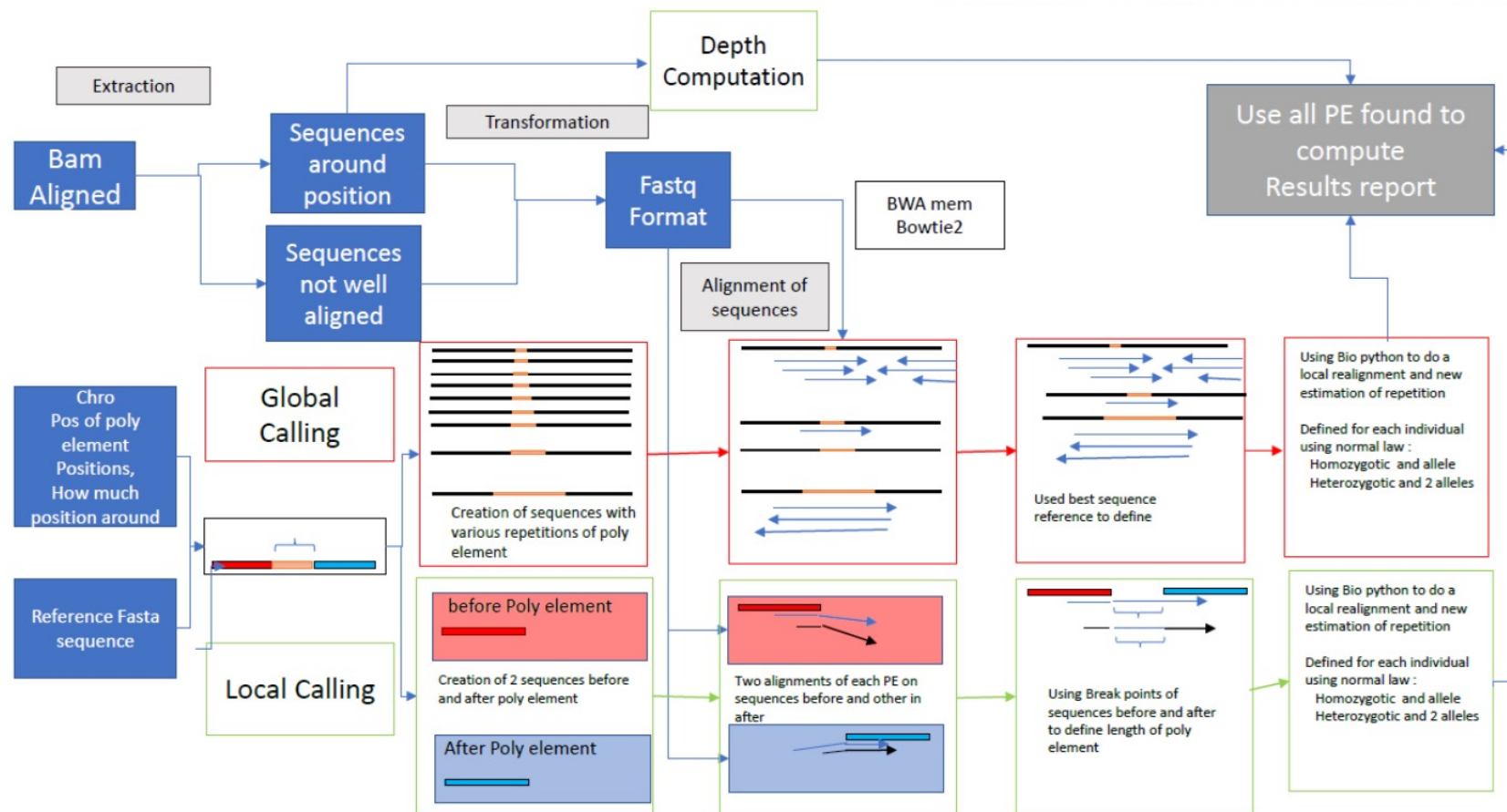
Figure 4.1: Workflow diagram detailing each step in the homopolymer detection pipeline developed inhouse by Dr Brandenburg
