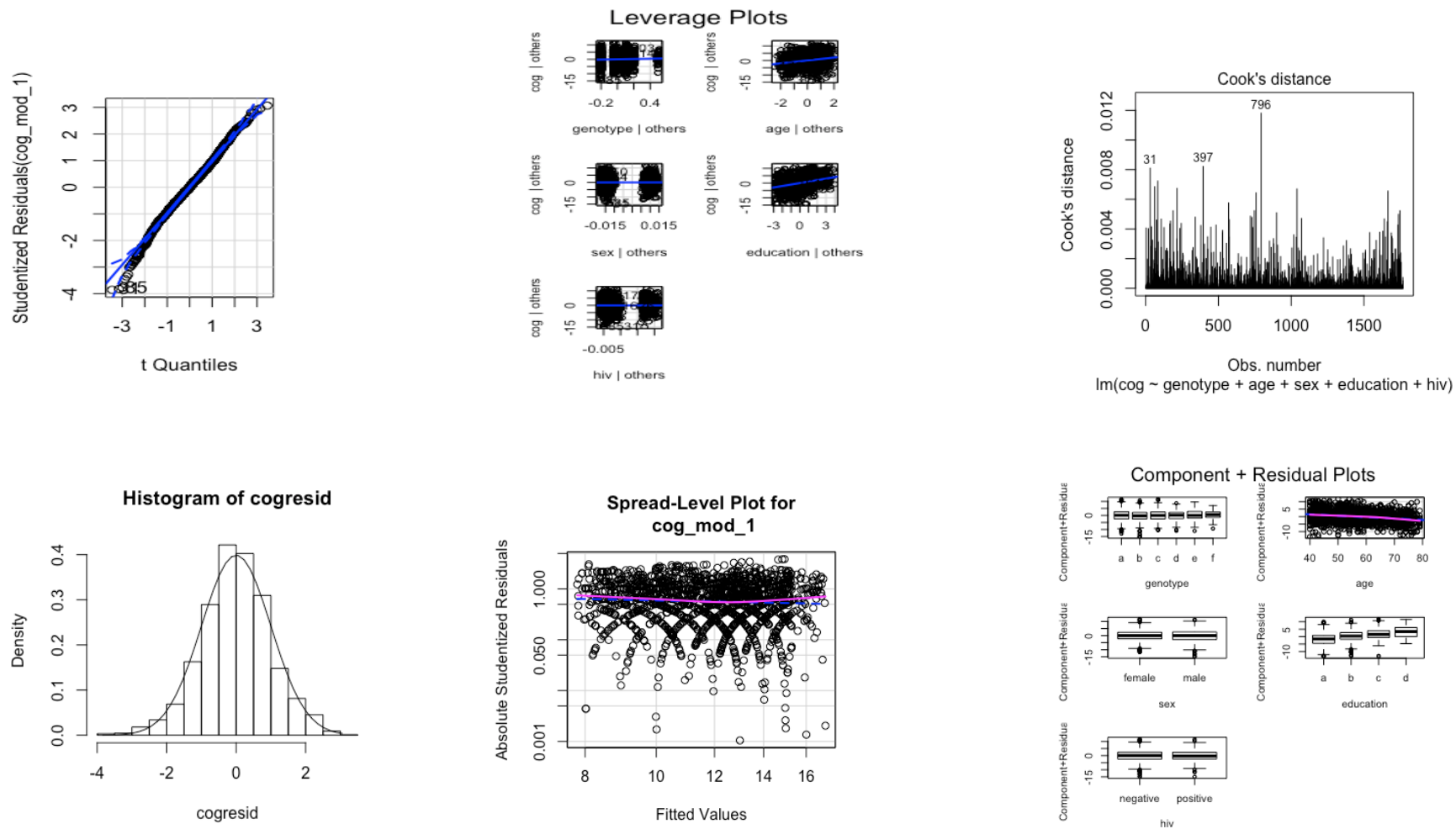
Figure A.2.2: Diagnostic regression plots for the residuals of total cognition score In order: QQ-plot, Leverage plots for each regression term, Cook's plot indicating Cook's distance, histogram showing distribution of residuals, spread level plot, and component-residual plots for each term and its effect on total cognition score
