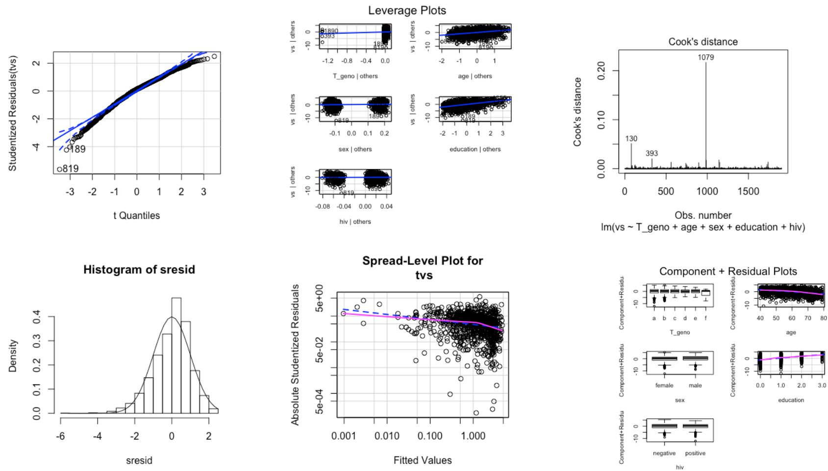
Figure A.4.11: Diagnostic regression plots for the residuals of visuospatial ability
