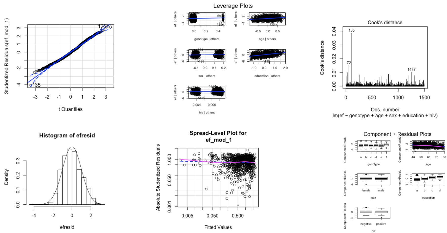
Figure A.2.3: Diagnostic regression plots for the residuals of executive function
