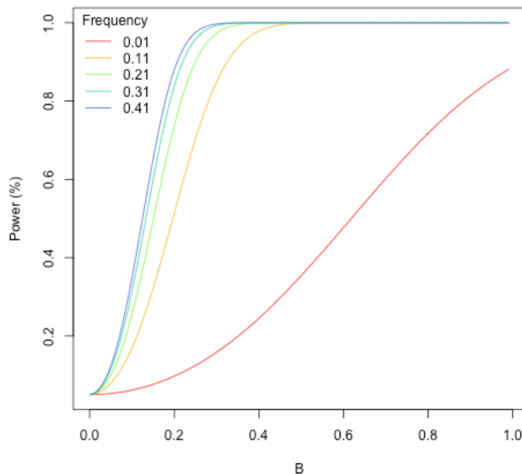
Figure 1.6: Power estimation for GWAS of total cognition score
