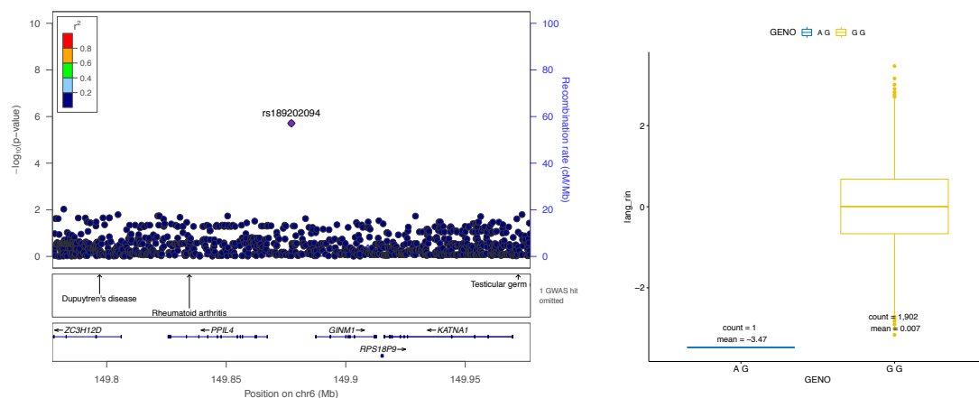
Figure A3.20: rs189202094 on chromosome 6 associated with visuospatial ability Locus zoom (left) and Kruskal-Wallis (right) plots.
