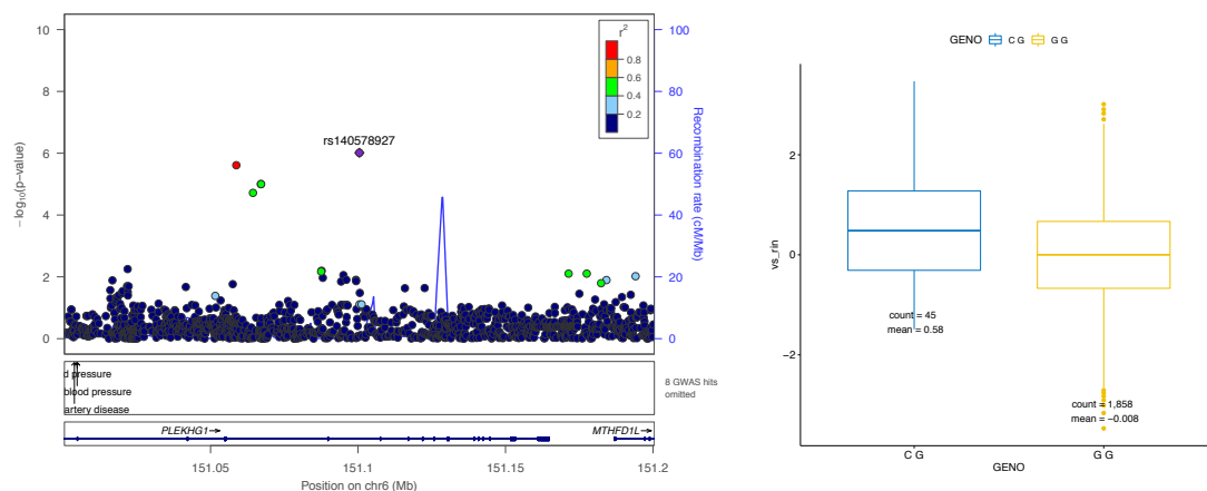
Figure A3.21: rs140578927 on chromosome 6 associated with visuospatial ability Locus zoom (left) and Kruskal-Wallis (right) plots.
