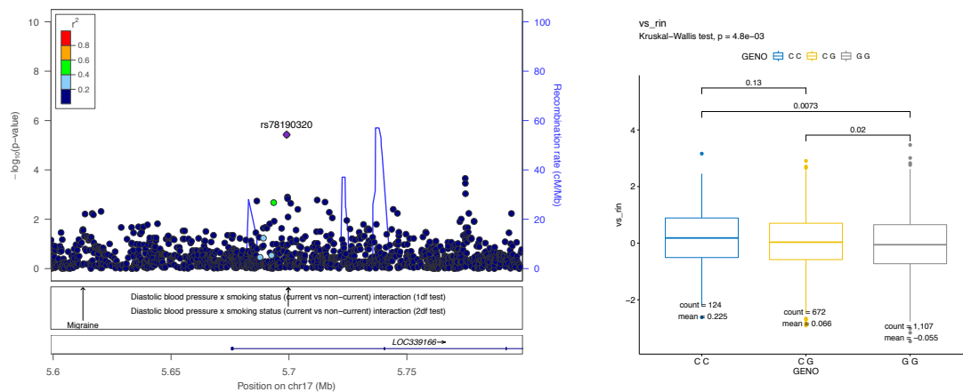
Figure A3.29: rs78190320 on chromosome 17 associated with visuospatial ability
