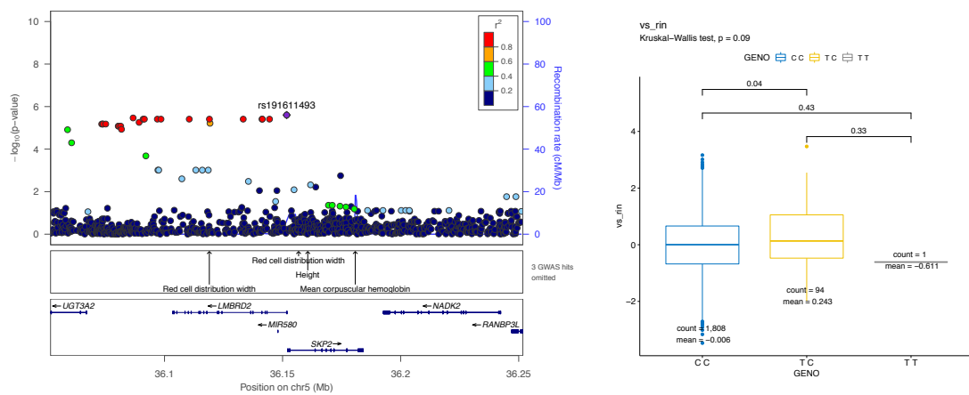
Figure A3.26: rs191611493 on chromosome 5 associated with visuospatial ability
