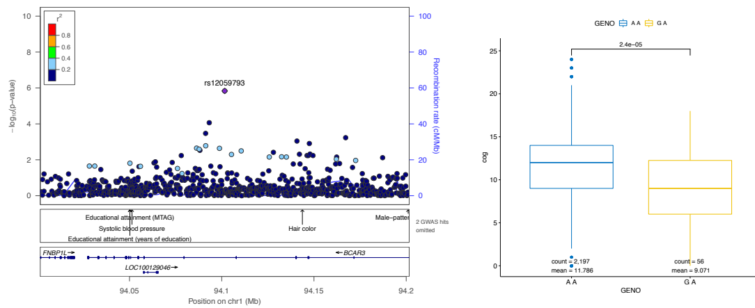
Figure A3.4: rs12059793 on chromosome 1 associated with total cognition score
