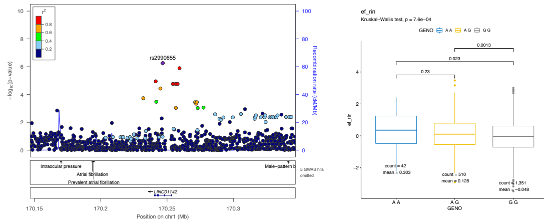
Figure A3.8: rs2990655 on chromosome 1 associated with executive function
