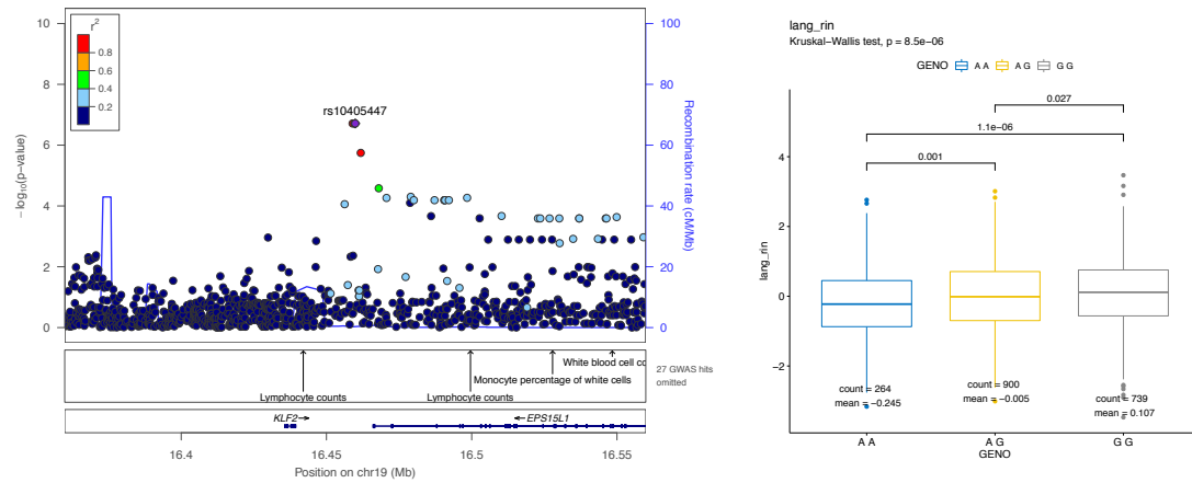
Figure A3.12: rs10405447 on chromosome 19 associated with language
