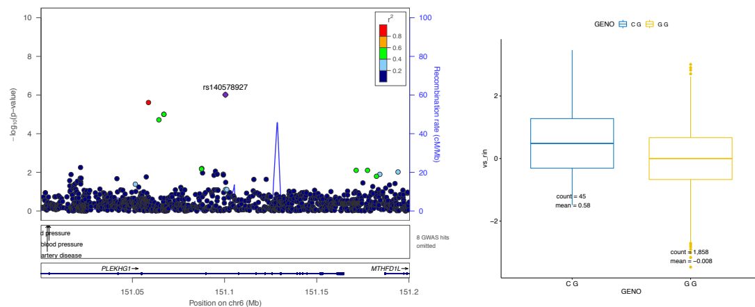
Figure A3.24: rs114096889 on chromosome 6 associated with visuospatial ability
