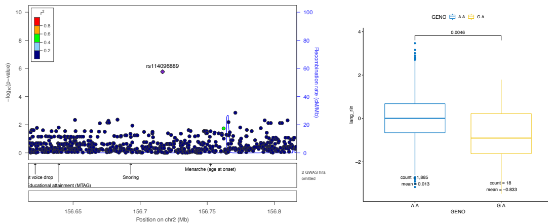
Figure A3.17: rs114096889 on chromosome 2 associated with language
