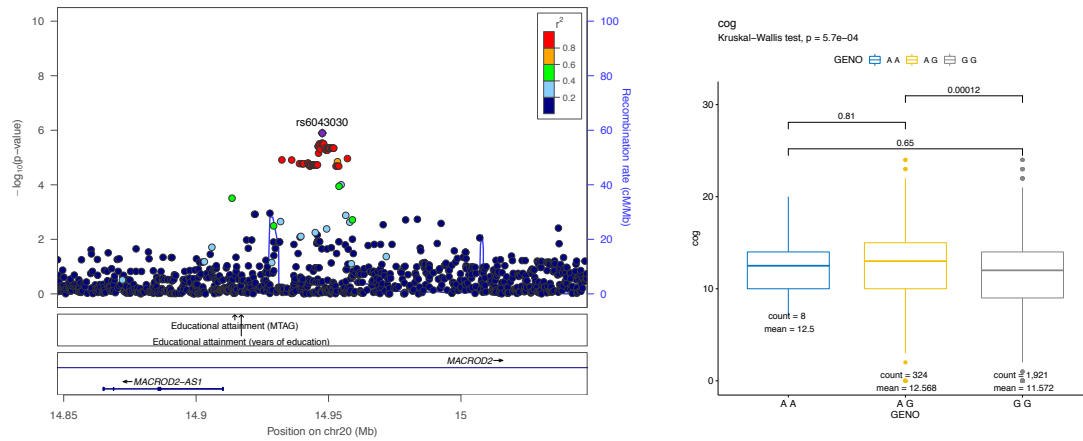
Figure A3.3: rs6043030 on chromosome 20 associated with total cognition score
