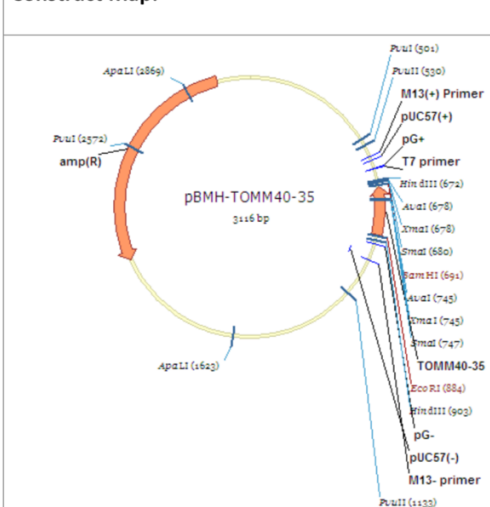
Figure A4.1: Gene synthesis report for clone for fragment length T=35 and T=16
