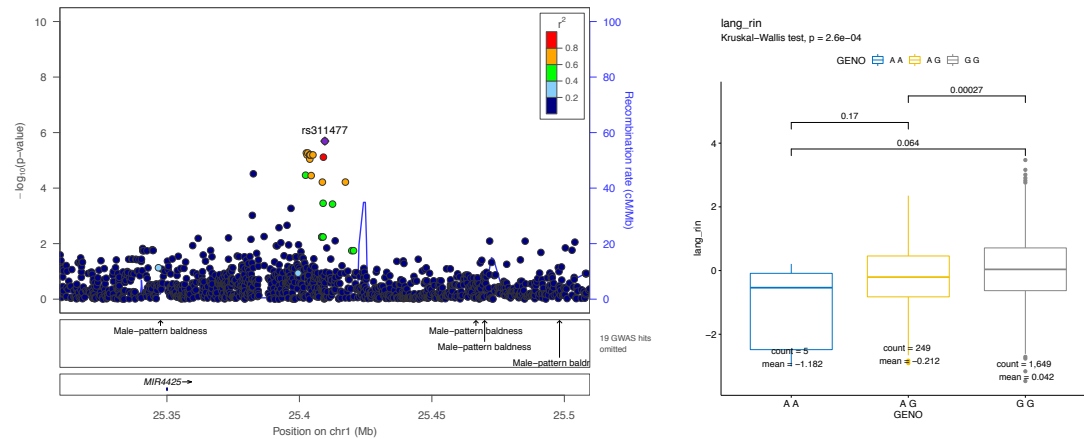
Figure A3.19: rs311477 on chromosome 1 associated with language
