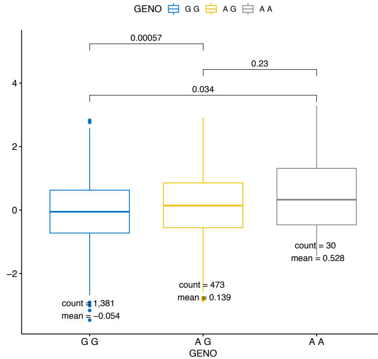
Supplementary Figure 3.1: Box-plots showing effects of variants on cognitive function
