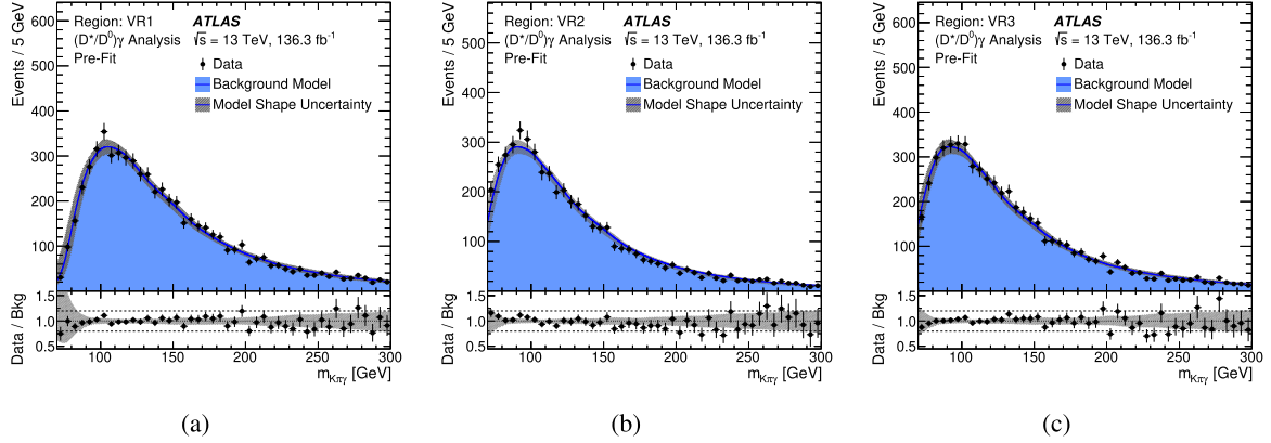
Fig. 4. The m_{K^\pm\pi^\mp\gamma} distribution of the data and pre-fit background model prediction of validation regions for the D^0\gamma final state. VR1 is shown in (a), where the meson candidate is required to satisfy p_T > 39 GeV in addition to the GR requirements. VR2 is shown in (b), where the meson-candidate isolation requirement used in the SR is applied, in addition to the GR requirements. VR3 is shown in (c), where the photon-candidate isolation requirements used in the SR are applied, in addition to the GR requirements. In all cases, the ratio of the data to the prediction of the background model is shown in the lower panel.
