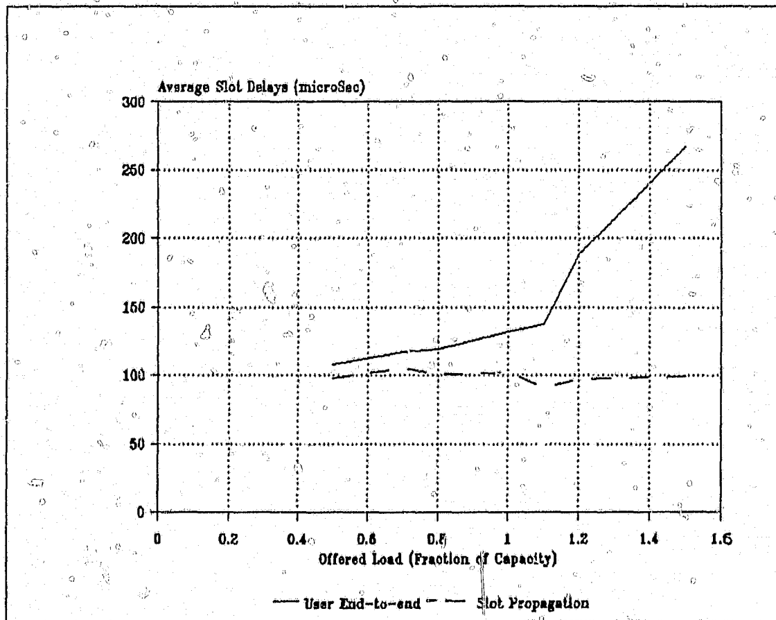
Figure 7.3 Average delays for MANSIM (DQDB test results).
