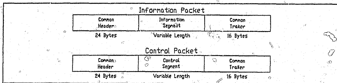
Figure E2 XTP packet types and formats
