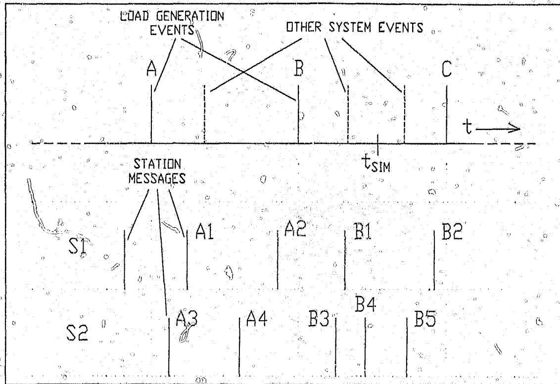
Figure 6.2 An abstract depiction of pseudo-dynamic load generation
