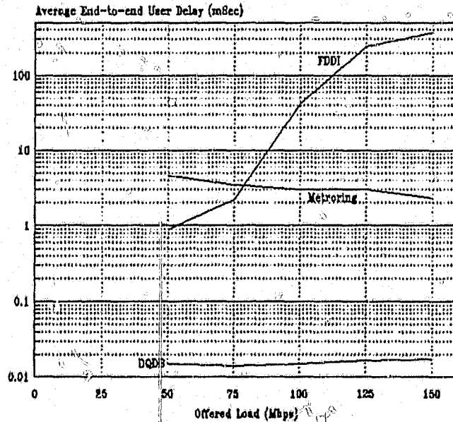
Figure 8.7 Average end-to-end user layer delay vs offered load when using FDDI, DQDB and Metroring for CSIR backbone
