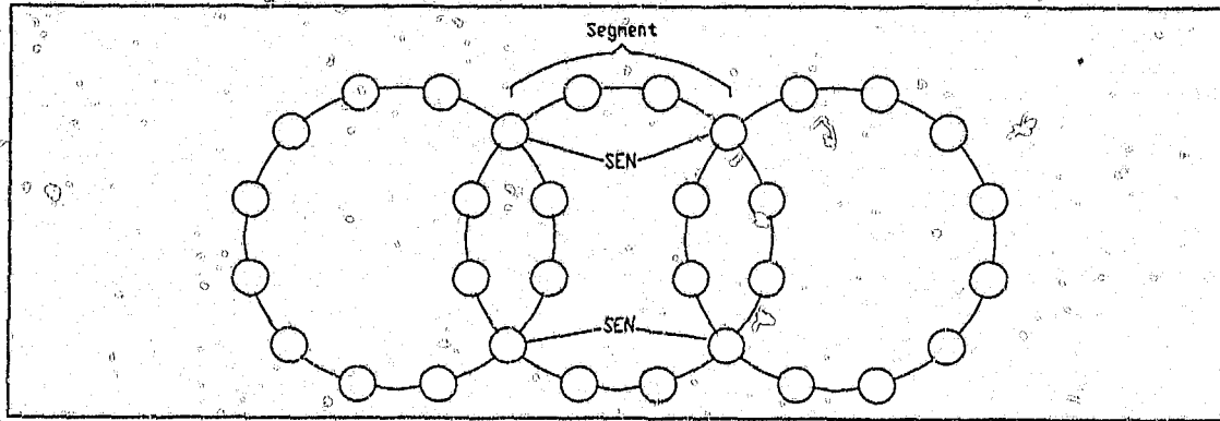
Figure D2 Interconnected rings made from ring segments in Metroring
