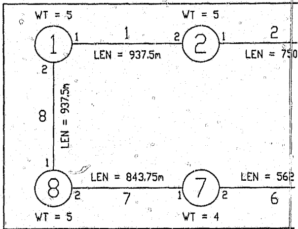
Figure 8.3 Collision domain representation
