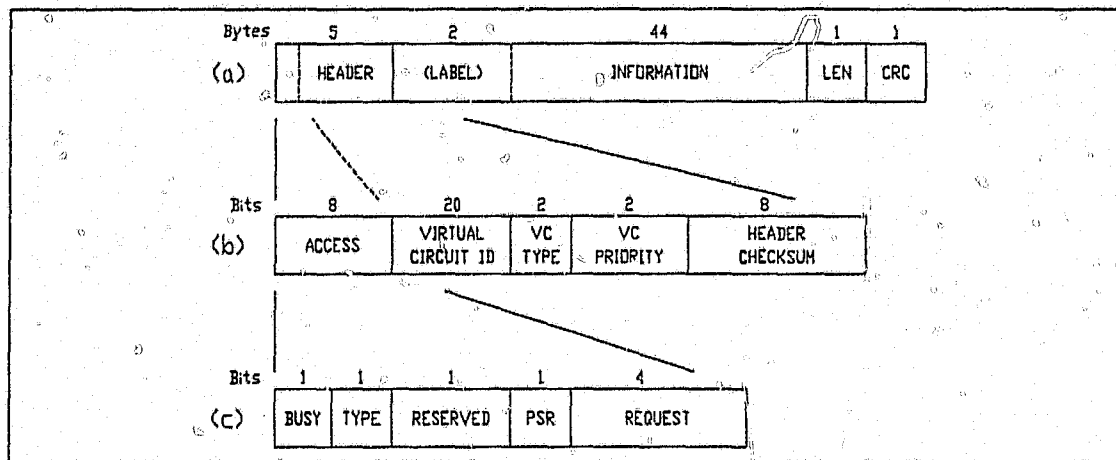
Figure C3 DQDB slot structure showing fields of the (a) slot, (b) slot header and (c) the access control field in the header.
