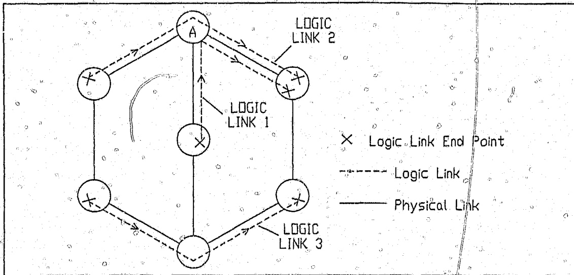
Figure 4.8 Concurrent logical links on a Metroring network
