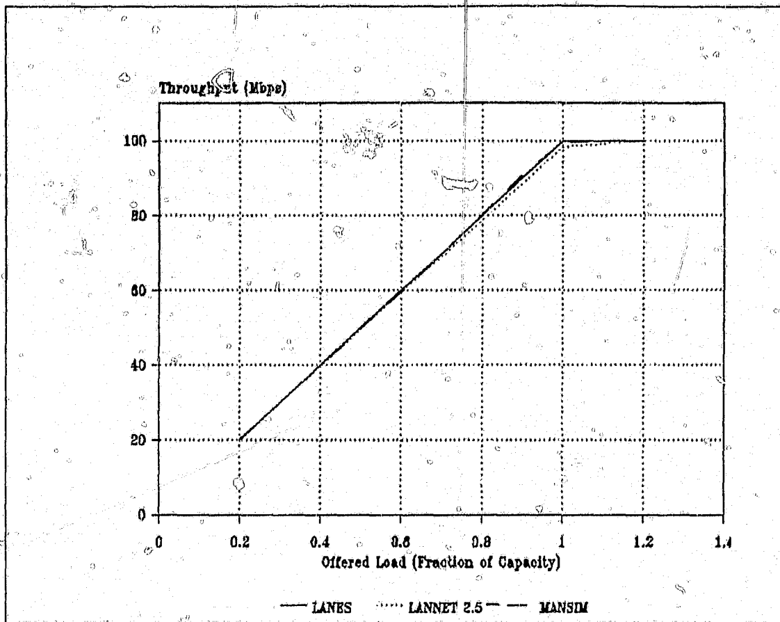
Figure 7.1 Physical layer throughput vs offered load (FDDI test results on three different simulators)
