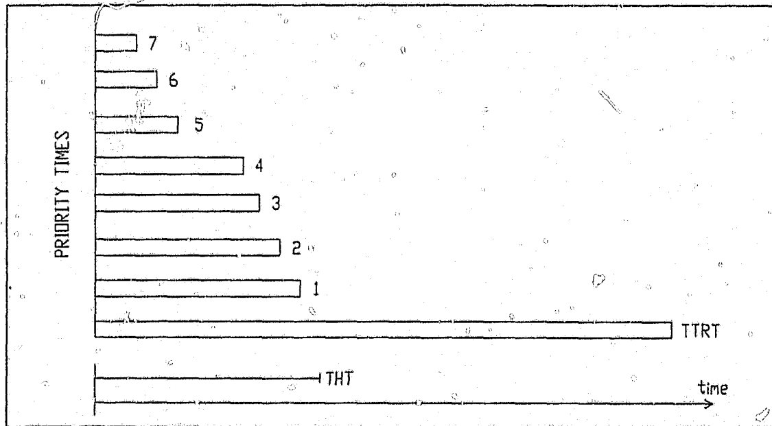
Figure 6.8 Priority class threshold times for FDDI's TTR (Timed Token Rotation) protocol
