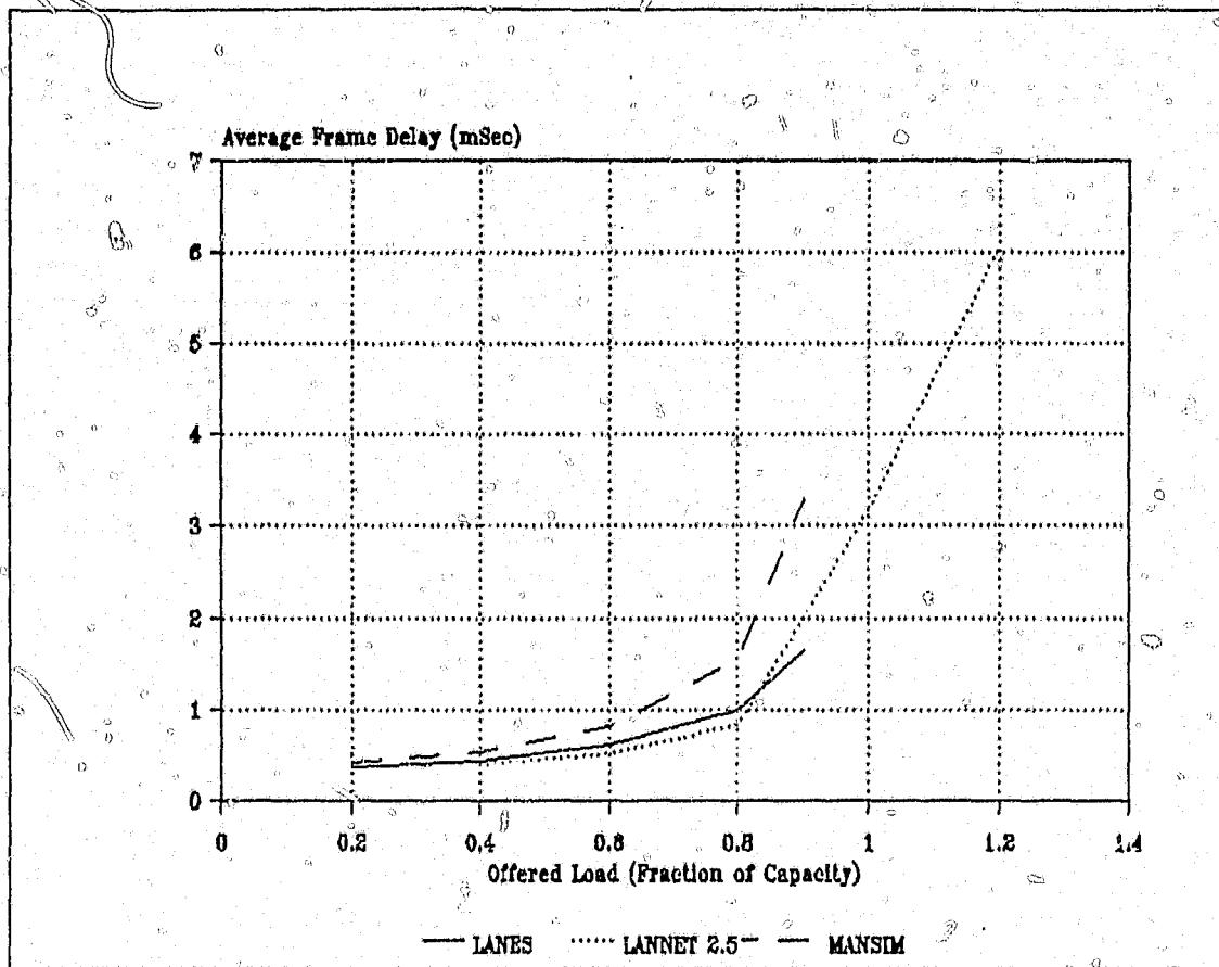
Figure 7.2 Average end-to-end user delay vs offered load (FDDI test results on three different simulators)
