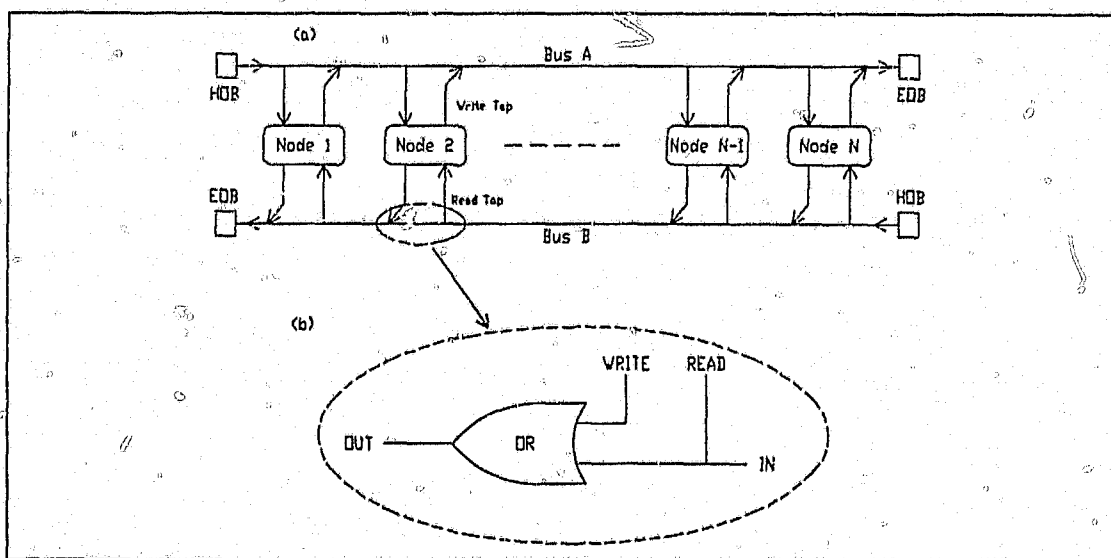
Figure C2 Structure of a DQDB network, (a) the topology and (b) implementation of the read/write tap.
