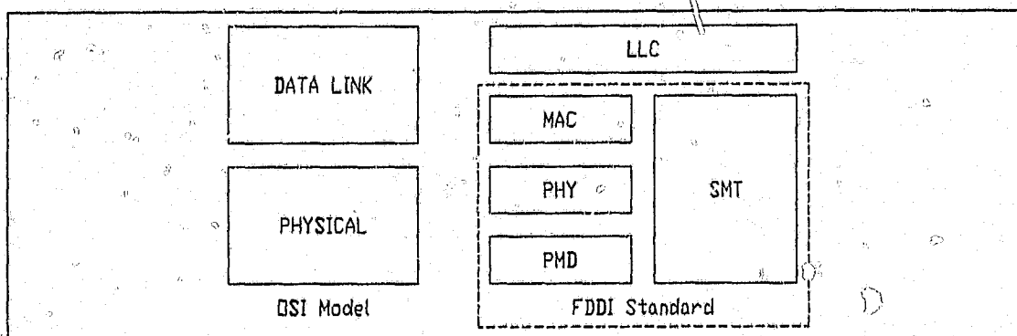
Figure B1 Component entities of a FDDI station
