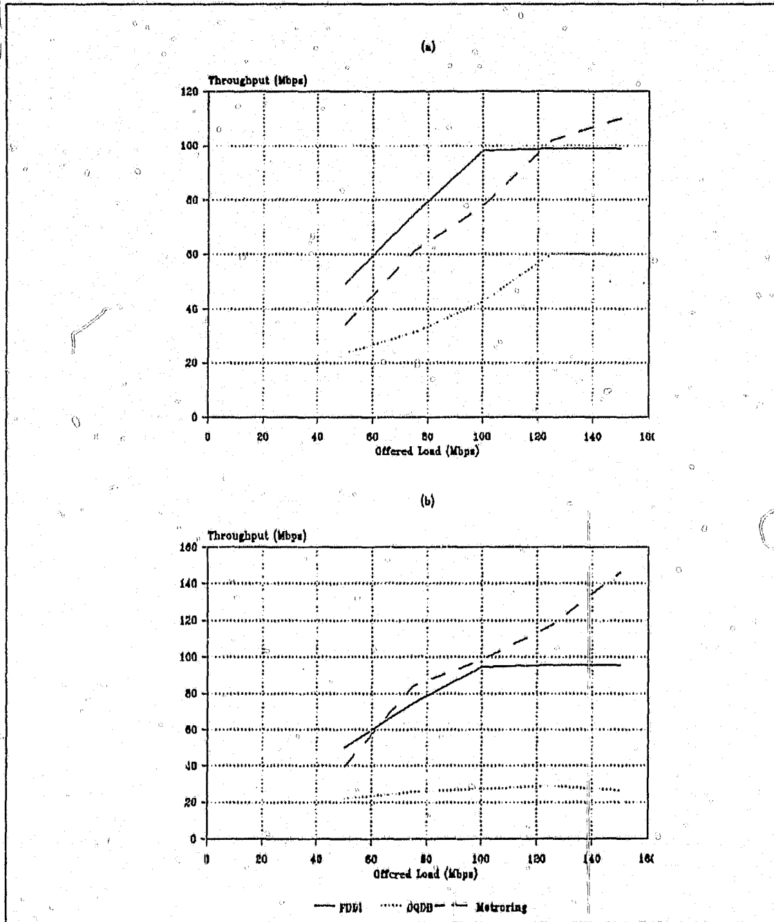
Figure 8.6 User layer throughput vs offered load when using FDDI, DQDB and Metroring for CSIR backbone The graphs allow easy comparisons as the trends for each type of MAN can be easily observed. Virtually all trends are distinct enough for reliable decisions regarding performance.
