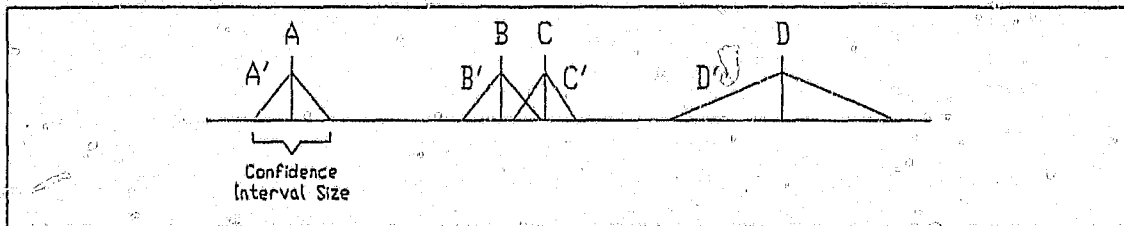
Figure 6.1 Interpreting estimates and confidence intervals
