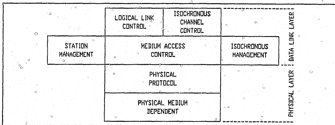
Figure C1 Component entities of a DQDB station
