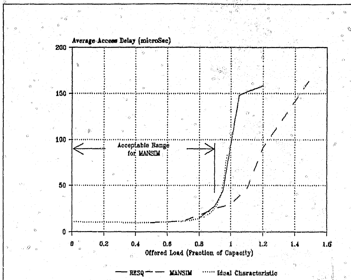
Figure 7.5 Average access delays vs offered load (normalized DQDB test results).
