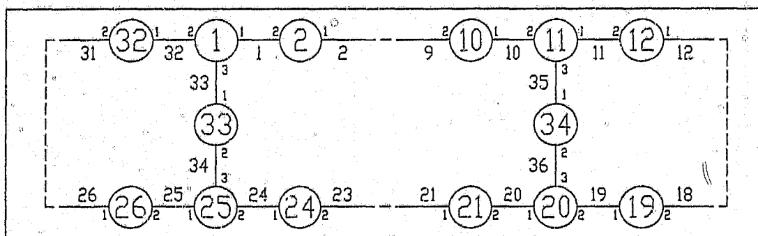
Figure 8.4 Representing Buildings on the backbone for Metroring
