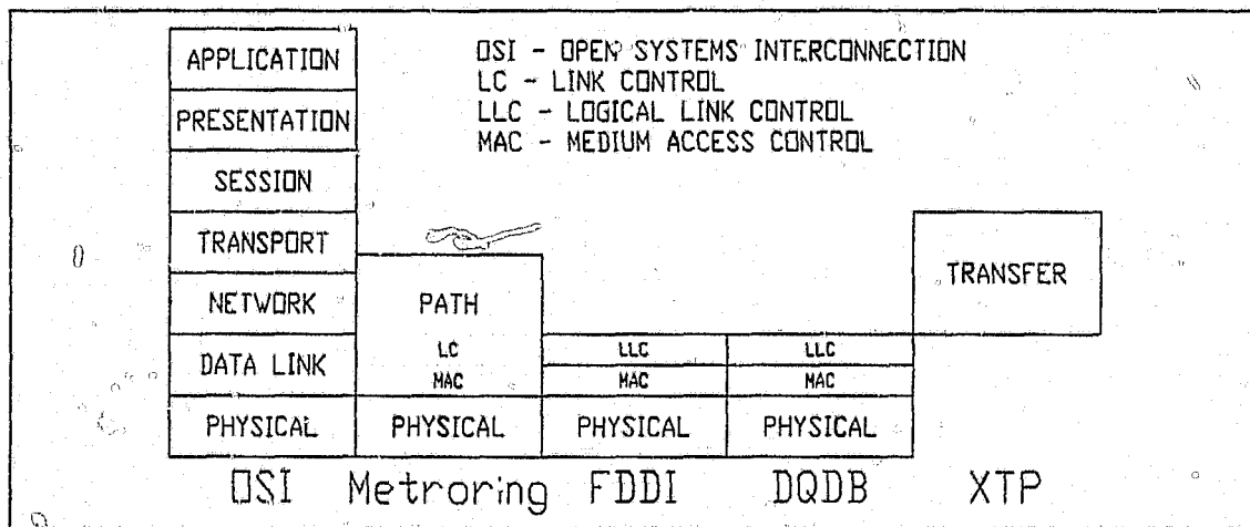
Figure 3.1 Comparison of protocol layers against OSI model
