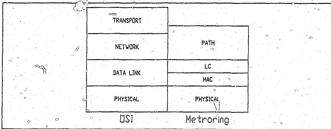
Figure D1 The component entities of Metroring
