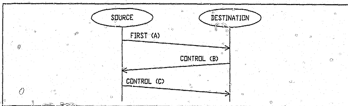
Figure E1 XTP three packet connection mode handshake
