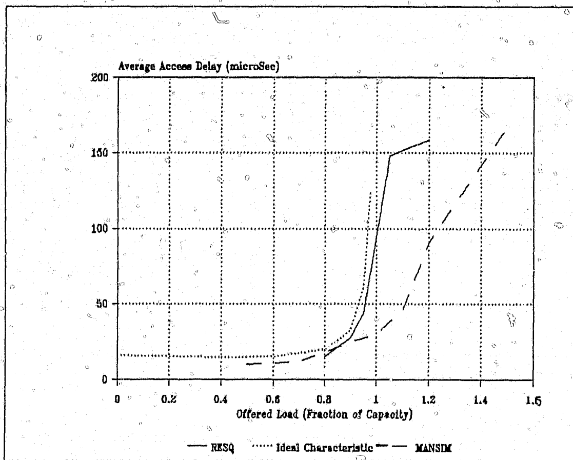
Figure 7.4 Average access delays vs offered load (DQDB test results).
