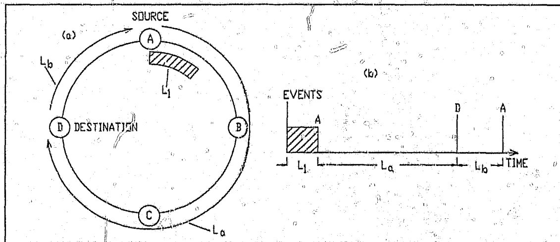
Figure 6.6 Packet transmission representation in FDDI (a) on the network and (b) in the time domain
