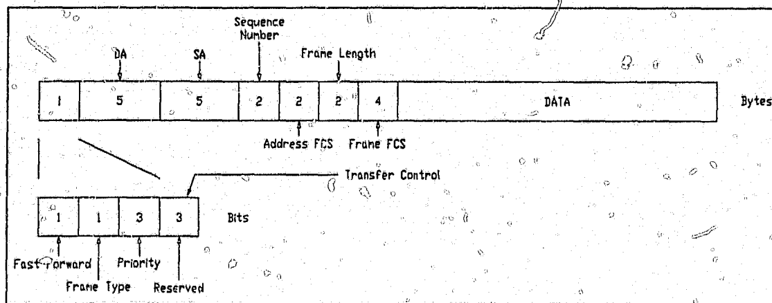
Figure D3 Information and Management frame composition
