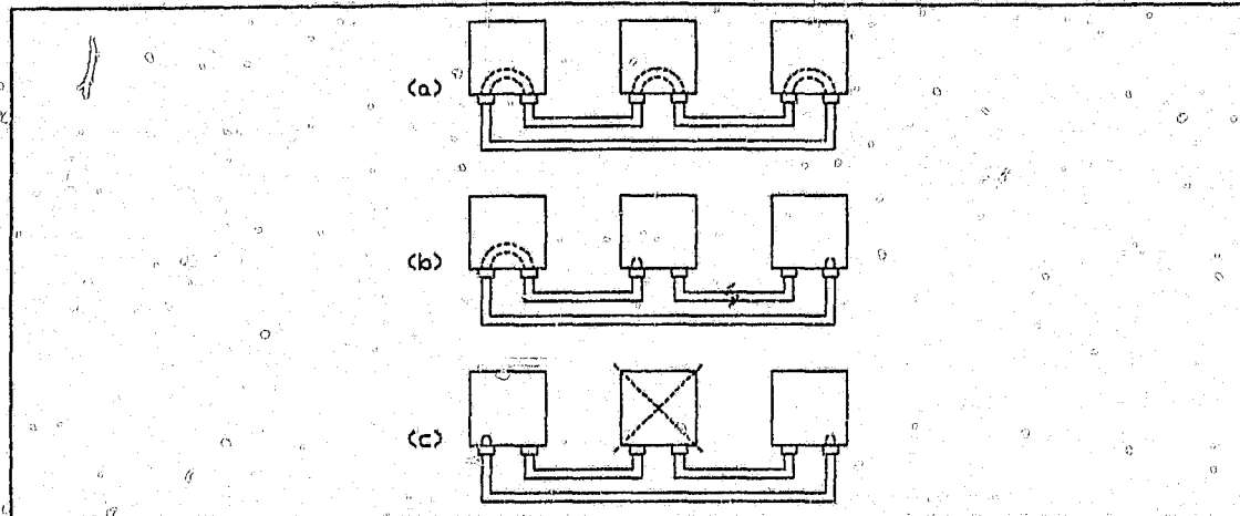
Figure B4 Reconfiguration of FDDI to eliminate a failed component
