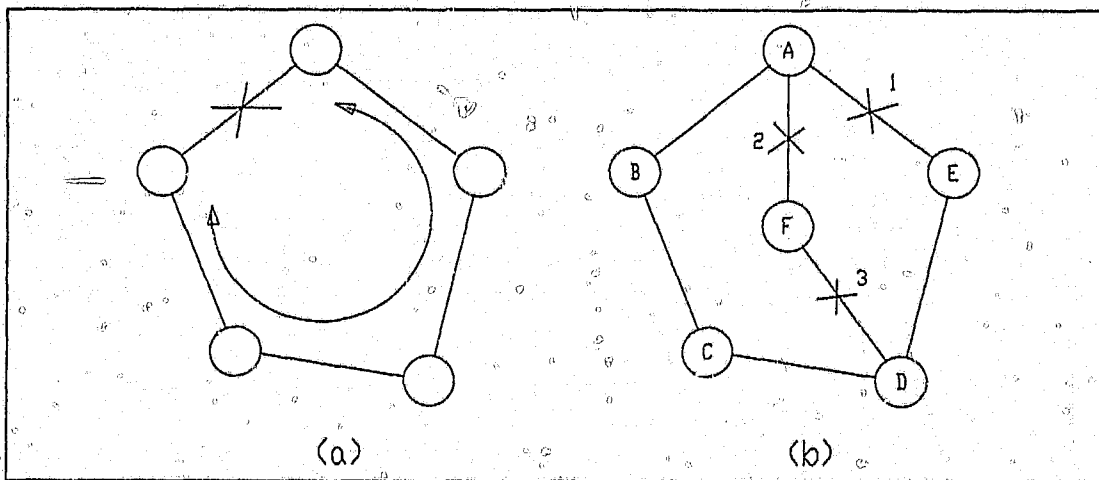
Figure 4.2 Correcting link failures in Metroring.
