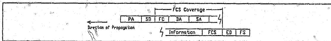
Figure B3 Layout of fields of an FDDI information frame
