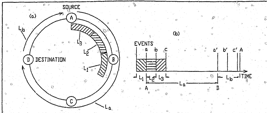
Figure 6.7 Multiple packet transmission representation in FDDI (a) on the network and (b) in the time domain
