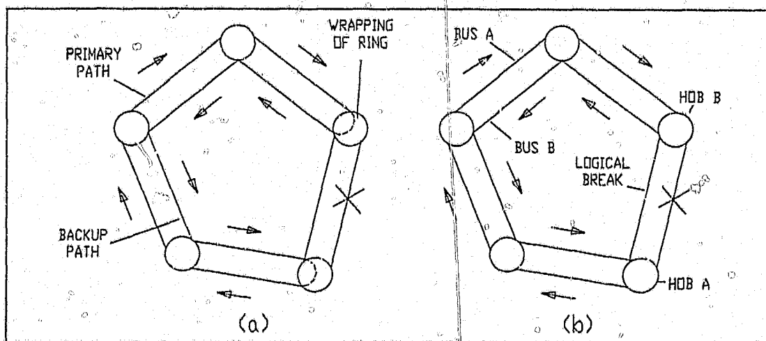
Figure 4.1 Correcting link failures (a) in FDDI and (b) DQDB.
