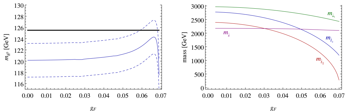
Figure 2. Lightest Higgs mass (left) and various soft masses (right) as a function of g_F for a sample parameter point, as computed with SOFTSUSY 3.3.7 [69] and FeynHiggs 2.9.4 [70–73]. The model parameters are listed in table 1 under MSSM-I. The blue dotted lines in the left panel show the \pm 3 GeV theory uncertainty interval around the theory prediction, while the solid horizontal line shows the LHC central value of 125.5 GeV. As evident from the right panel, the gauge messenger contribution to the soft masses may significantly affect the third-generation squark masses, allowing for maximal stop mixing with only moderately large |A_t| , while the first-generation squarks and the gluino remain heavy enough to evade the LHC bounds.
