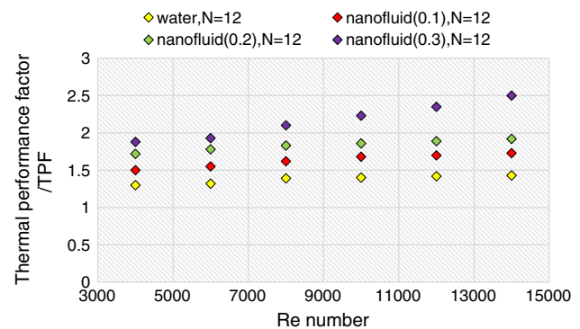
Fig. 24 Values achieved for the heat efficiency factor of the tube with 12 triangular baffles at a 40° angle in the presence of the Nanofluid
