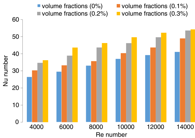
Fig. 12 Nusselt number values achieved for the triangular smooth tubes with 8 triangular baffles embedded at a 70° angle in the presence of carbon/water Nanofluid
