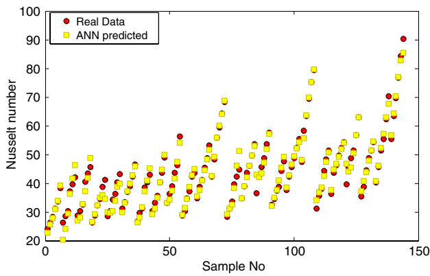
Fig. 29 ANN-predicted and experimental values for Nusselt number based on the samples quantity
