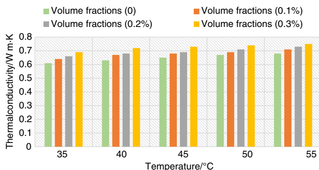
Fig. 5 The temperature-based changes in the coefficient of thermal conductivity for different volume fractions of carbon/water Nanofluid
