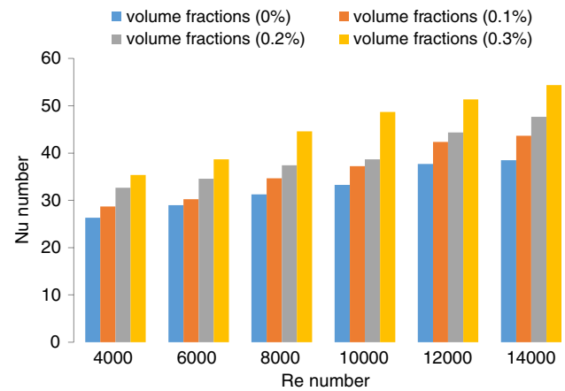
Fig. 14 Nusselt number values achieved for the triangular smooth tubes with 4 triangular baffles embedded at a 40° angle in the presence of carbon/water Nanofluid
