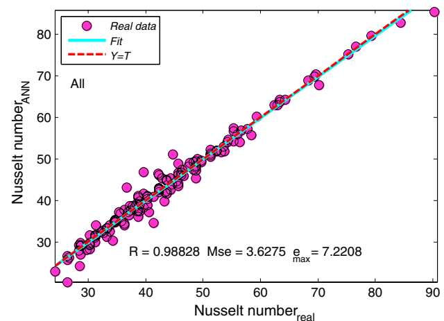
Fig. 36 Values of the coefficient of correlation and MSE value achieved for the experimental and predicted data of Nusselt number with 32 neurons for the total data
