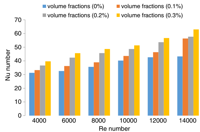
Fig. 13 Nusselt number values achieved for the triangular smooth tubes with 12 triangular baffles embedded at a 70° angle in the presence of carbon/water Nanofluid
