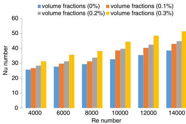
Fig. 11 Nusselt number values achieved for the triangular smooth tubes with 4 triangular baffles embedded at a 70° angle in the presence of carbon/water Nanofluid
