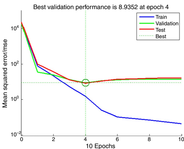
Fig. 31 MSE of the experimental data for Nusselt number (sum of squares-based quantity of repetitions)
