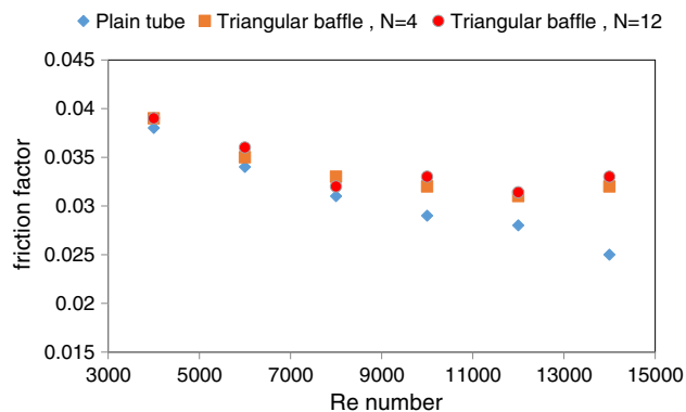
Fig. 19 Values calculated for the coefficient of friction of the smooth tubes and tubes with 4 and 12 triangular baffles at a 70° angle
