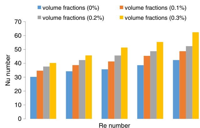
Fig. 15 Nusselt number values achieved for the triangular smooth tubes with 8 triangular baffles embedded at a 40° angle in the presence of carbon/water Nanofluid
