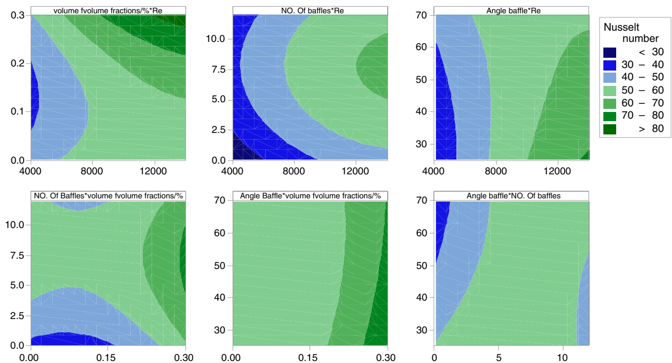
Fig. 18 The effect of binary parameters on the achieved Nusselt number
