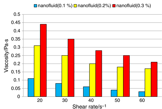
Fig. 6 Viscosity changes with shear stress for different volume fractions of carbon/water Nanofluid
