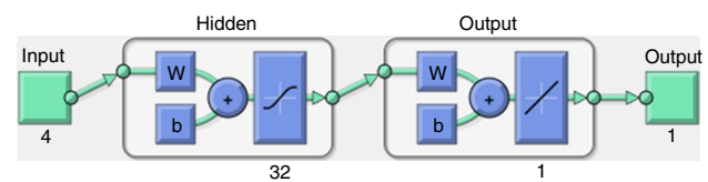
Fig. 4 The schematic structure of a three-layer Perceptron neural network to predict the Nusselt number
