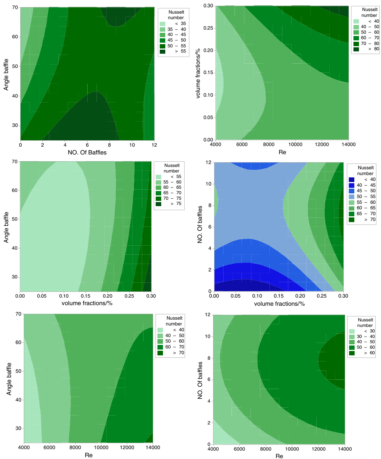
Fig. 17 The simultaneous effect of binary parameters on the achieved Nusselt number
