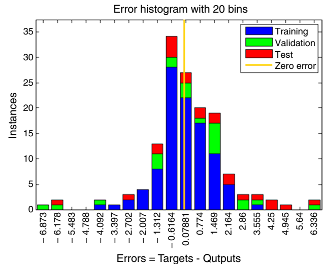
Fig. 32 Error distribution chart for resulted data
