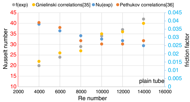
Fig. 7 A comparison between Nusselt number and coefficient of friction factor for the water base fluid in a smooth tube
