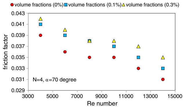
Fig. 21 The coefficient of friction values determined for the tubes with 4 triangular baffles at a 70° angle using the Nanofluid
