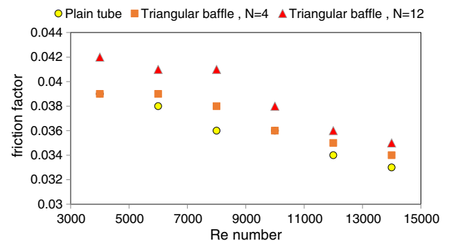
Fig. 20 Values calculated for the coefficient of friction of the smooth tubes and tubes with 4 and 12 triangular baffles at a 40° angle
