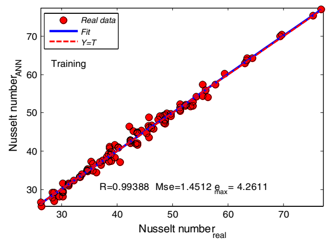
Fig. 33 Coefficient of correlation and MSE values achieved for the experimental and predicted data of Nusselt number with 32 neurons for train data
