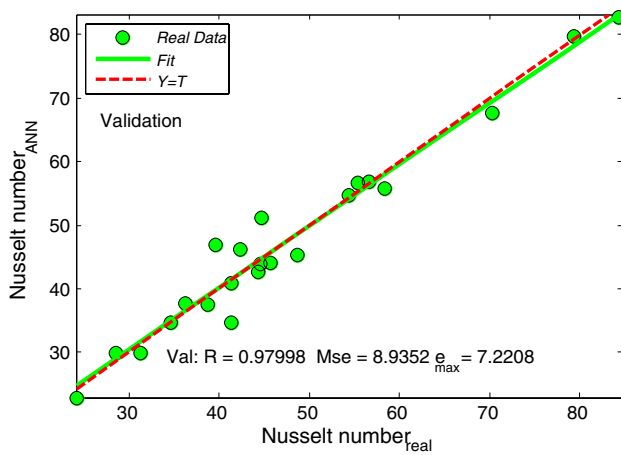
Fig. 34 Values of the coefficient of correlation and MSE value achieved for the experimental and predicted data of Nusselt number with 32 neurons for validation data
