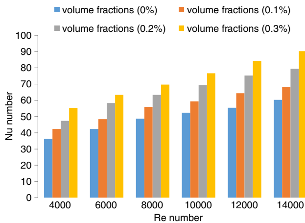
Fig. 16 Nusselt number values achieved for the triangular smooth tubes with 12 triangular baffles embedded at a 40° angle in the presence of carbon/water Nanofluid
