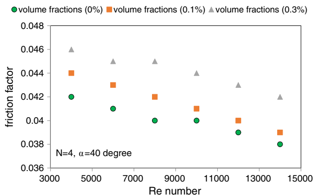
Fig. 22 The coefficient of friction values determined for the tubes with 4 triangular baffles at a 40° angle using the Nanofluid
