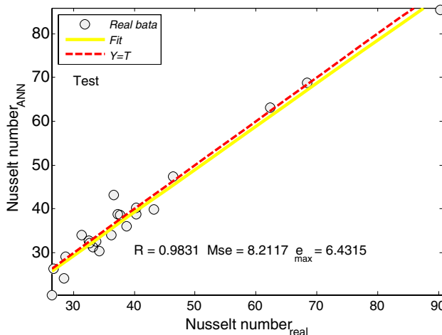
Fig. 35 Values of the coefficient of correlation and MSE value achieved for the experimental and predicted data of Nusselt number with 32 neurons for test data
