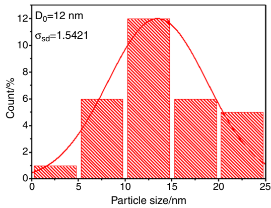
Fig. 8 Particle size distribution fitted with a log normal distribution function for carbon black Nanoparticles. (Color figure online)
