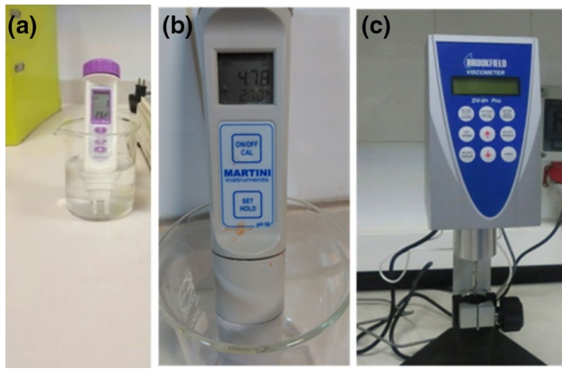
Fig. 3 a AZ electrical conductivity meter; b pH meter; and c Brookfield viscometer
