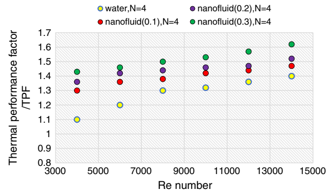
Fig. 23 Values achieved for the heat efficiency factor of the tube with 4 triangular baffles at a 70° angle in the presence of the Nanofluid
