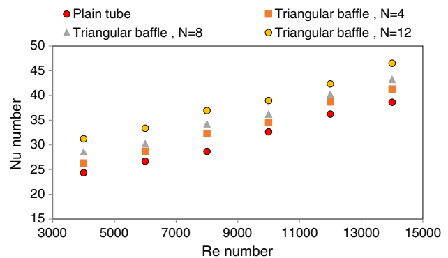
Fig. 10 Nusselt number values achieved for the triangular smooth tubes with 4, 8, and 12 triangular baffles embedded at a 40° angle without the presence of Nanofluid
