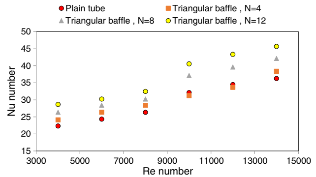
Fig. 9 Nusselt number values achieved for the triangular smooth tubes with 4, 8, and 12 triangular baffles embedded at a 70° angle without the presence of Nanofluid
